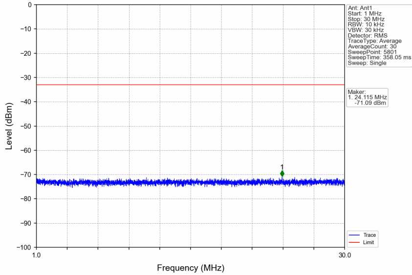
n7_15kHz_SISO_NTNV_40MHz_DFT-s-OFDM QPSK_2520MHz_Edge_1RB_Left
