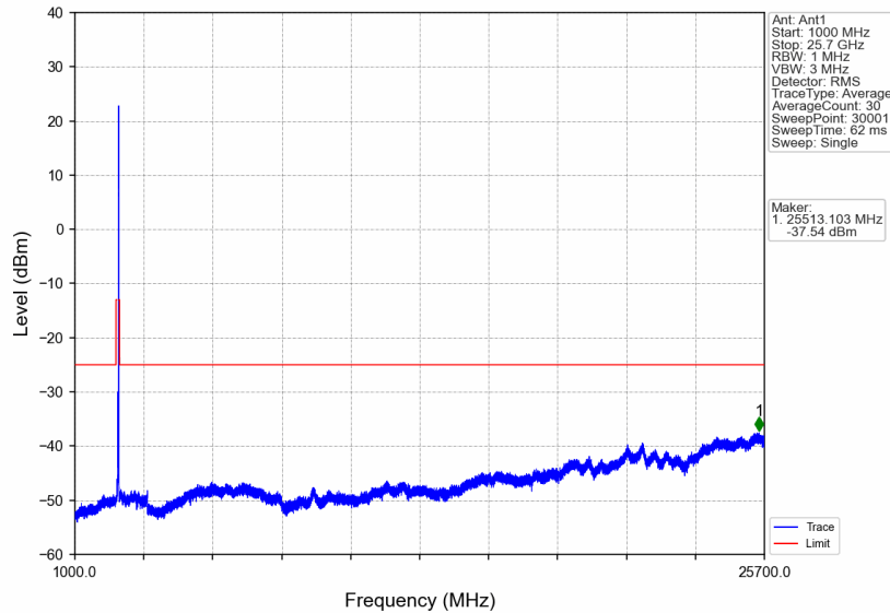
n7_15kHz_SISO_NTNV_30MHz_DFT-s-OFDM QPSK_2555MHz_Edge_1RB_Right
