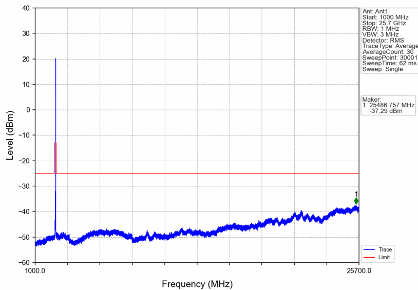
n7_15kHz_SiSO_NTNV_30MHz_CP-OFDM QPSK_2555MHz_Edge_1RB_Right
