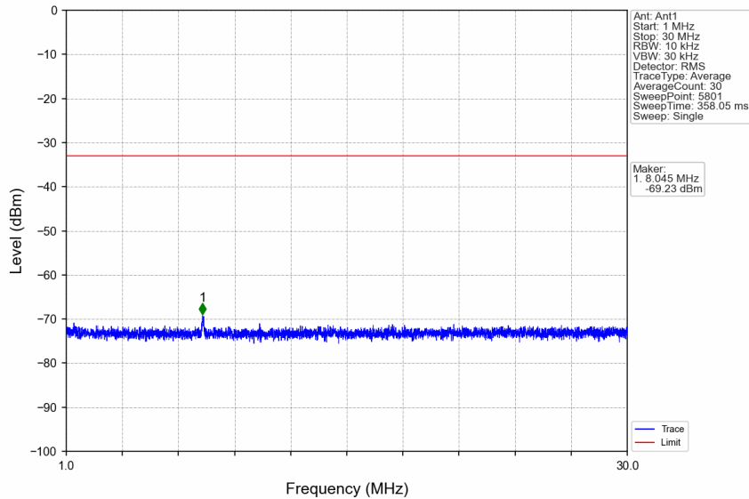
n7_15kHz_SISO_NTNV_30MHz_DFT-s-OFDM QPSK_2555MHz_Edge_1RB_Right
