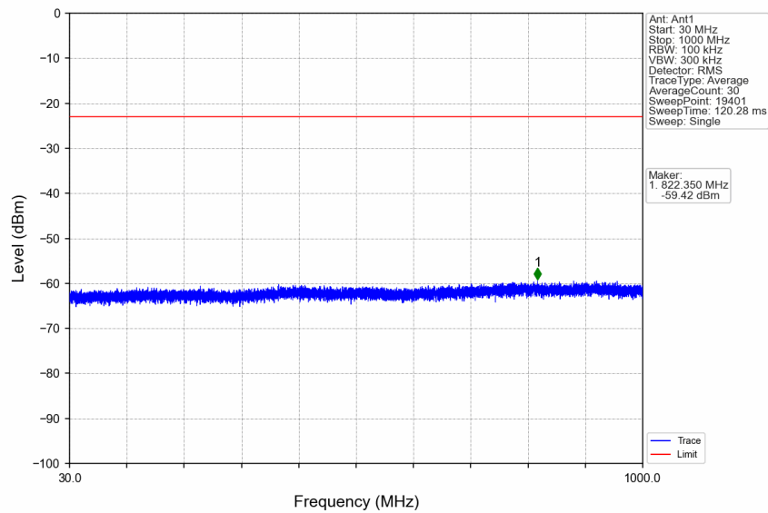
n7_15kHz_SiSO_NTNV_30MHz_CP-OFDM QPSK_2555MHz_Edge_1RB_Right
