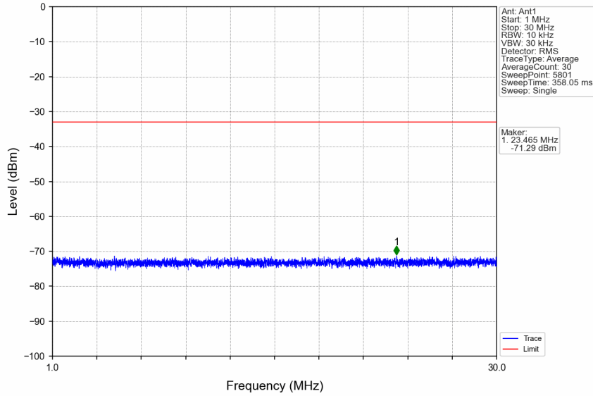
n7_15kHz_SISO_NTNV_30MHz_CP-OFDM QPSK_2515MHz_Edge_1RB_Left
