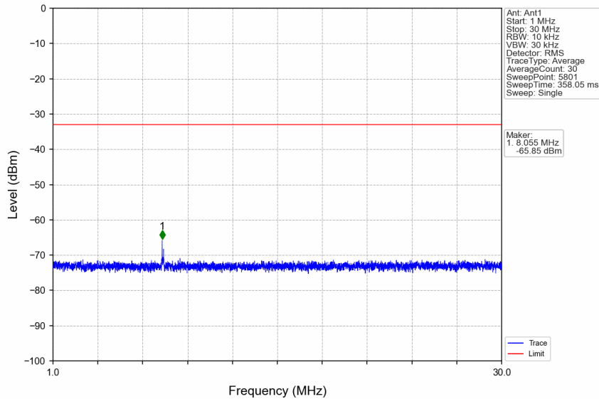
n7_15kHz_SISO_NTNV_40MHz_DFT-s-OFDM PI/2 BPSK_2550MHz_Edge_1RB_Right
