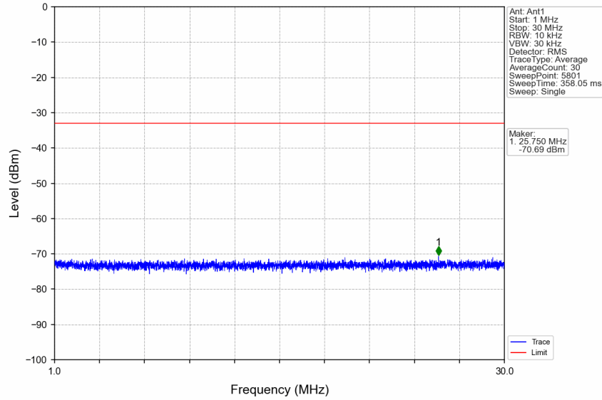
n7_15kHz_SISO_NTNV_30MHz_DFT-s-OFDM QPSK_2535MHz_Edge_1RB_Left
