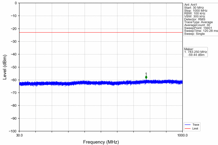
n7_15kHz_SISO_NTNV_30MHz_CP-OFDM QPSK_2535MHz_Edge_1RB_Left
