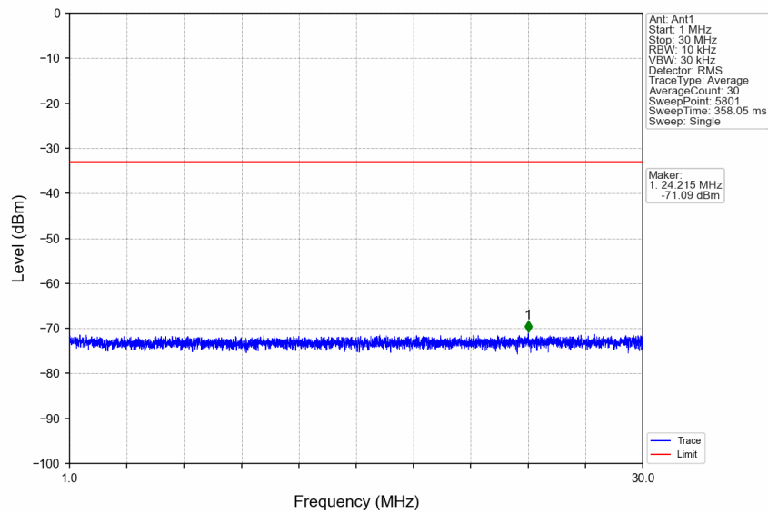
n7_15kHz_SISO_NTNV_40MHz_DFT-s-OFDM PI/2 BPSK_2520MHz_Edge_1RB_Left
