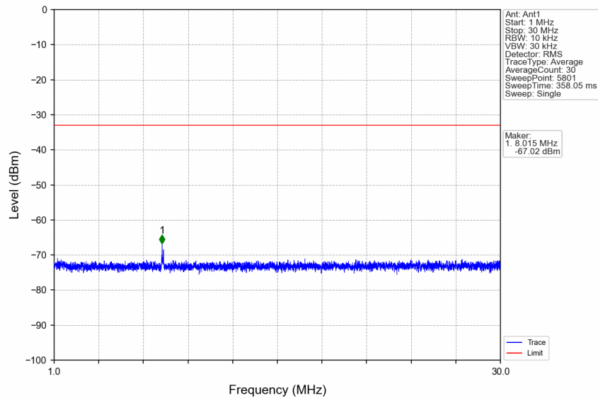
n7_15kHz_SISO_NTNV_30MHz_DFT-s-OFDM PI/2 BPSK_2555MHz_Edge_1RB_Right
