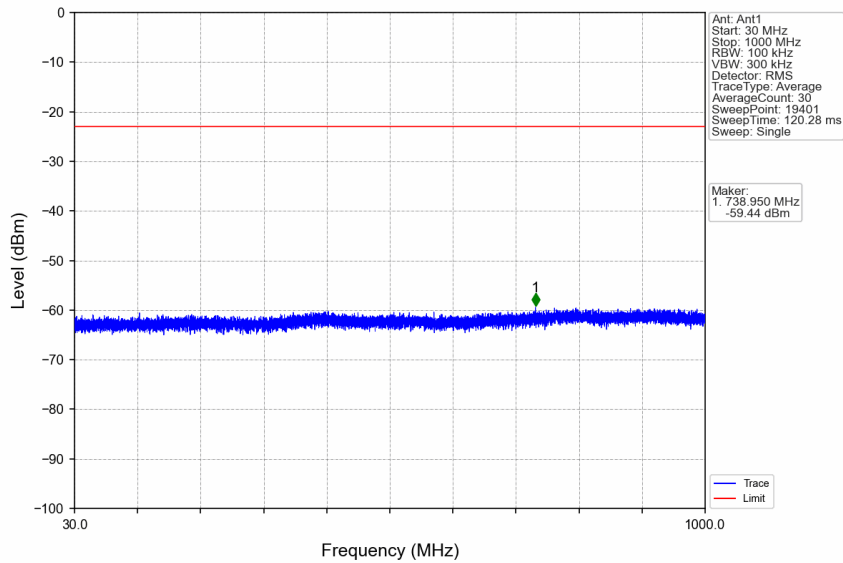
n7_15kHz_SISO_NTNV_25MHz_DFT-s-OFDM_QPSK_2557.5MHz_Edge_1RB_Right
