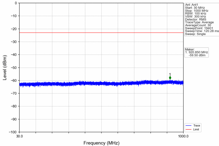
n7_15kHz_SISO_NTNV_30MHz_DFT-s-OFDM PI/2 BPSK_2535MHz_Edge_1RB_Left
