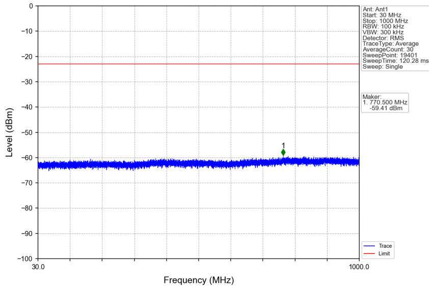
n7_15kHz_SISO_NTNV_25MHz_CP-OFDM QPSK_2535MHz_Edge_1RB_Left
