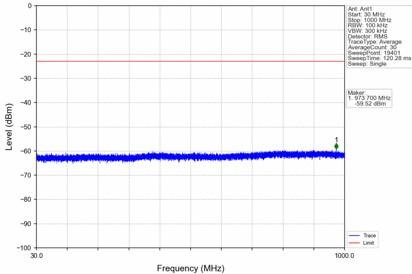
n7_15kHz_SISO_NTNV_25MHz_CP-OFDM QPSK_2512.5MHz_Edge_1RB_Left
