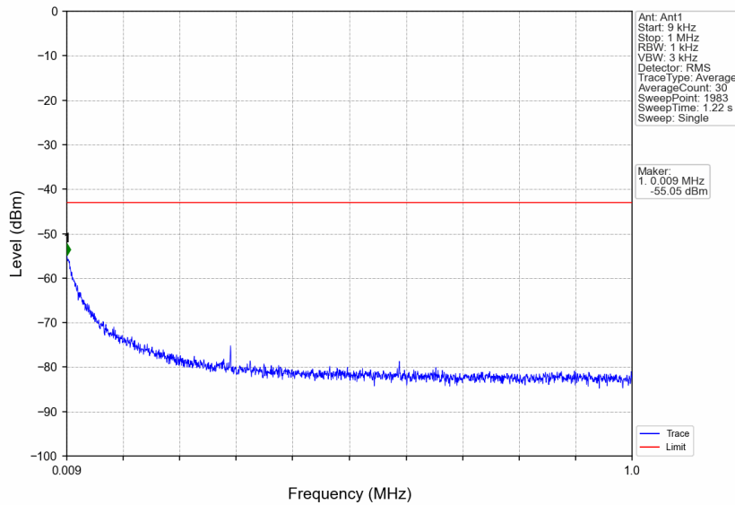
n7_15kHz_SISO_NTNV_25MHz_CP-OFDM QPSK_2557.5MHz_Edge_1RB_Right
