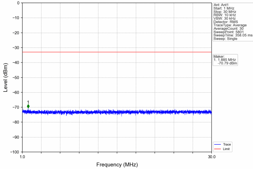
n7_15kHz_SISO_NTNV_25MHz_CP-OFDM QPSK_2512.5MHz_Edge_1RB_Left
