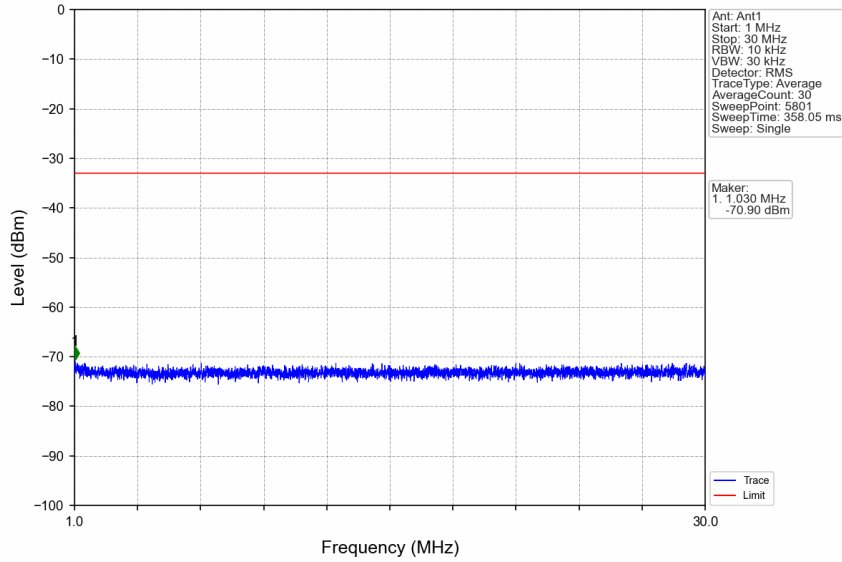
n7_15kHz_SISO_NTNV_30MHz_CP-OFDM QPSK_2535MHz_Edge_1RB_Left
