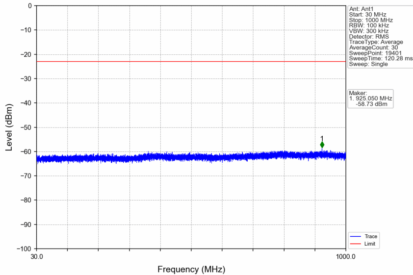
n7_15kHz_SISO_NTNV_30MHz_CP-OFDM QPSK_2515MHz_Edge_1RB_Left
