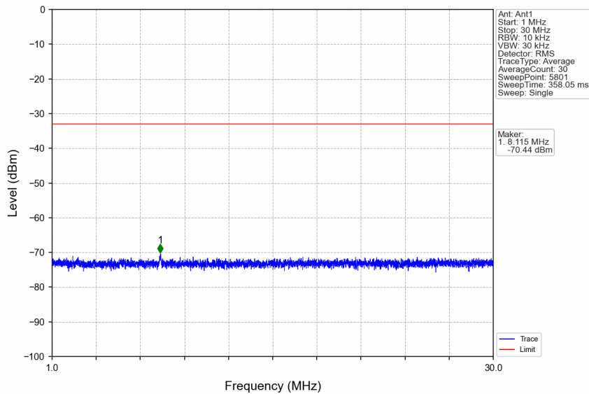
n7_15kHz_SISO_NTNV_25MHz_CP-OFDM QPSK_2557.5MHz_Edge_1RB_Right
