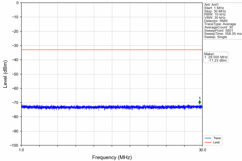
n7_15kHz_SISO_NTNV_30MHz_DFT-s-OFDM PI/2 BPSK_2515MHz_Edge_1RB_Left
