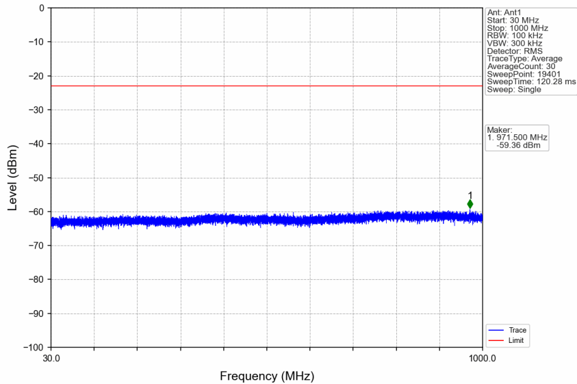
n7_15kHz_SISO_NTNV_40MHz_DFT-s-OFDM QPSK_2520MHz_Edge_1RB_Left
