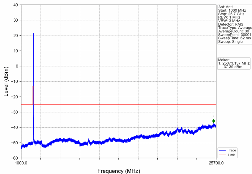
n7_15kHz_SISO_NTNV_25MHz_CP-OFDM QPSK_2557.5MHz_Edge_1RB_Right
