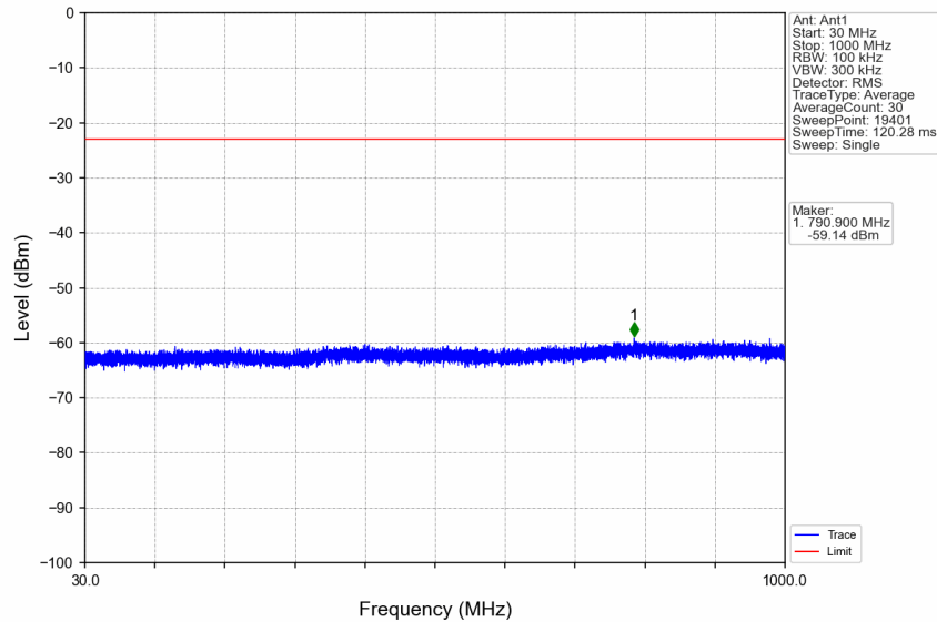
n7_15kHz_SISO_NTNV_30MHz_DFT-s-OFDM QPSK_2535MHz_Edge_1RB_Left
