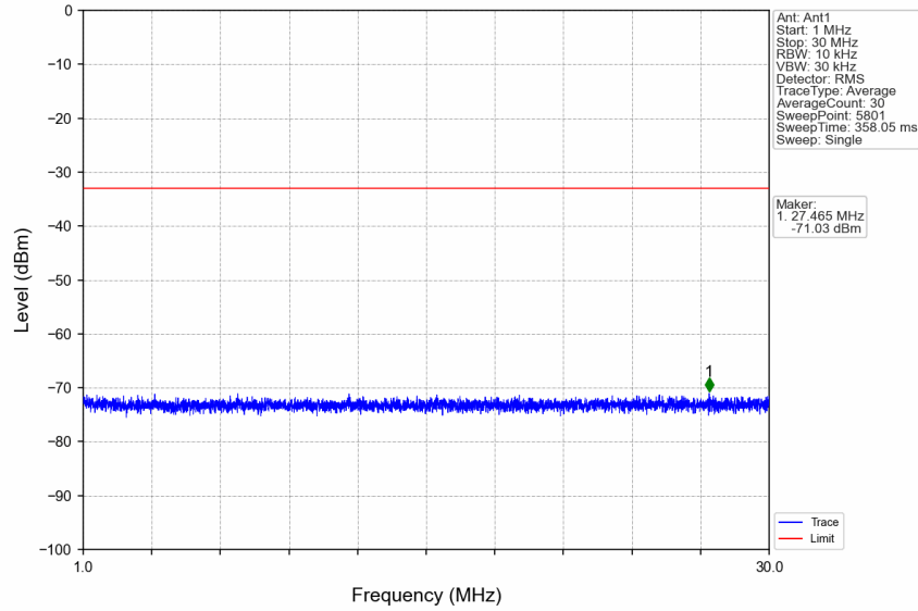
n7_15kHz_SISO_NTNV_20MHz_DFT-s-OFDM QPSK_2535MHz_Edge_1RB_Left
