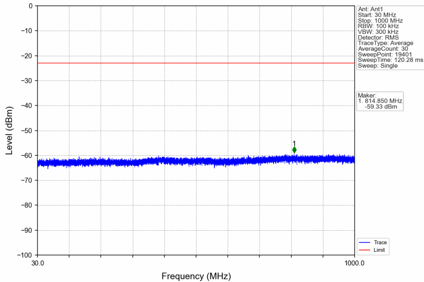
n7_15kHz_SISO_NTNV_15MHz_CP-OFDM QPSK_2535MHz_Edge_1RB_Left
