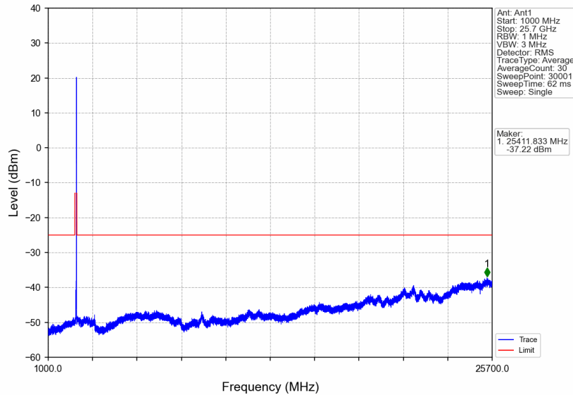
n7_15kHz_SiSO_NTNV_20MHz_CP-OFDM QPSK_2560MHz_Edge_1RB_Right
