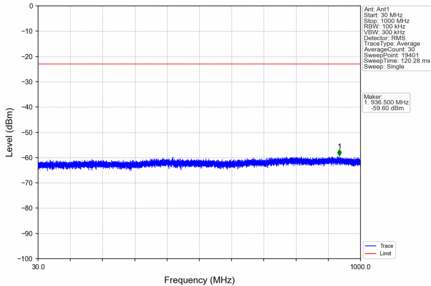
n7_15kHz_SISO_NTNV_25MHz_DFT-s-OFDM QPSK_2535MHz_Edge_1RB_Left
