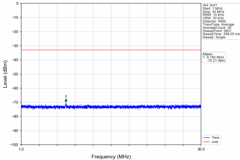
n7_15kHz_SISO_NTNV_20MHz_CP-OFDM QPSK_2560MHz_Edge_1RB_Right
