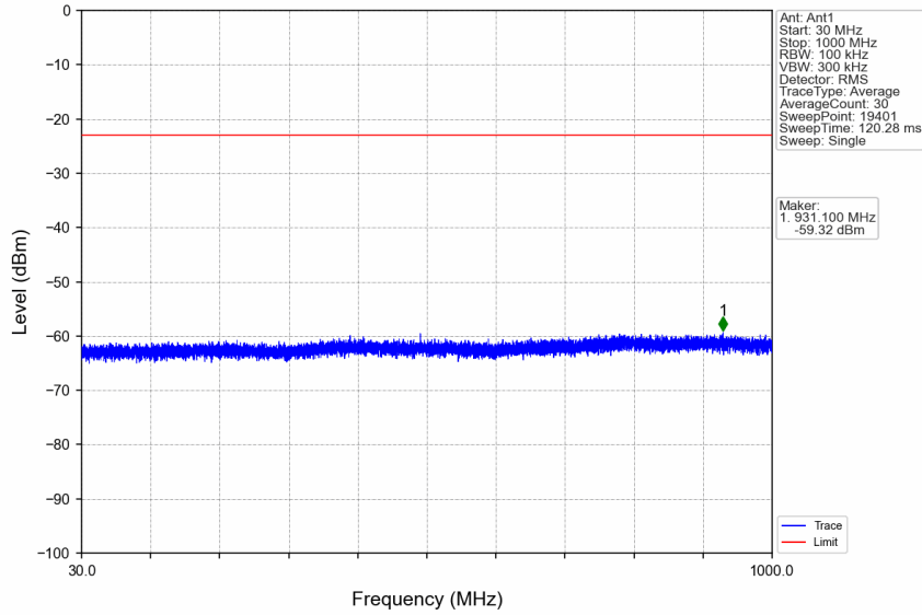
n7_15kHz_SiSO_NTNV_20MHz_CP-OFDM QPSK_2560MHz_Edge_1RB_Right
