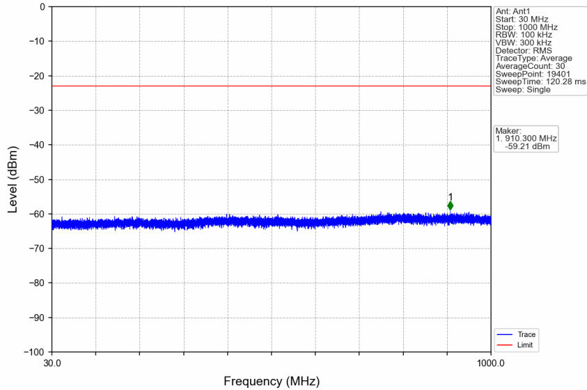
n7_15kHz_SISO_NTNV_20MHz_DFT-s-OFDM QPSK_2560MHz_Edge_1RB_Right
