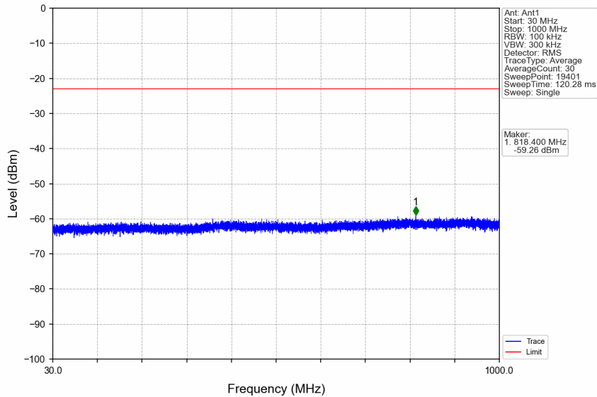
n7_15kHz_SISO_NTNV_25MHz_DFT-s-OFDM QPSK_2512.5MHz_Edge_1RB_Left
