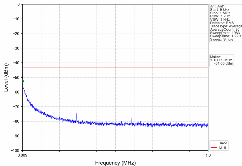
n7_15kHz_SISO_NTNV_20MHz_DFT-s-OFDM QPSK_2560MHz_Edge_1RB_Right
