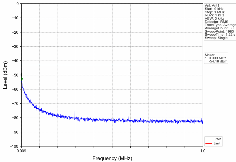
n7_15kHz_SISO_NTNV_15MHz_CP-OFDM QPSK_2562.5MHz_Edge_1RB_Right
