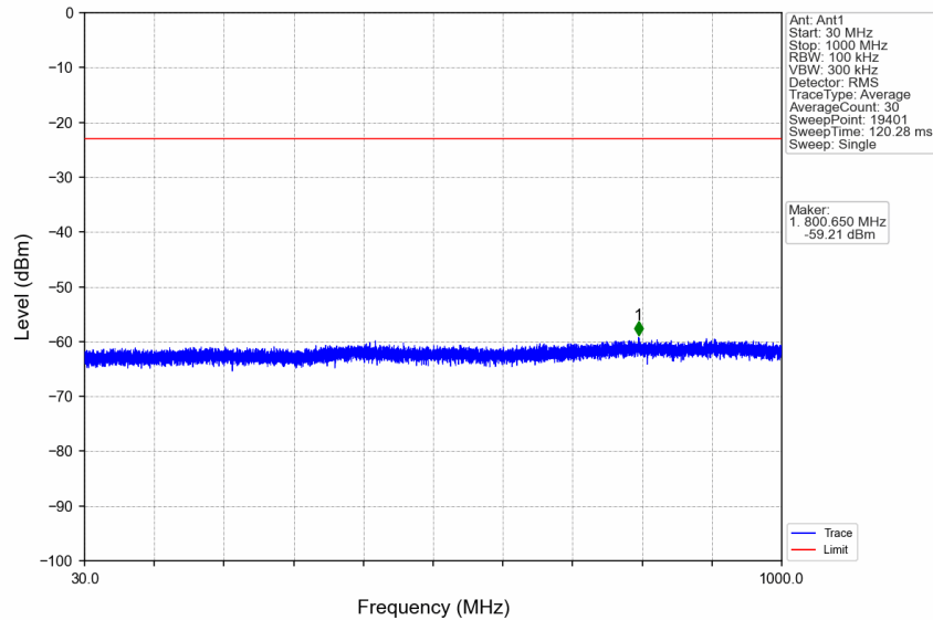
n7_15kHz_SISO_NTNV_20MHz_DFT-s-OFDM QPSK_2535MHz_Edge_1RB_Left
