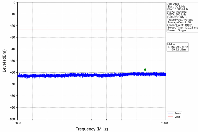
n7_15kHz_SISO_NTNV_15MHz_CP-OFDM QPSK_2562.5MHz_Edge_1RB_Right
