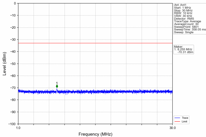
n7_15kHz_SISO_NTNV_15MHz_CP-OFDM QPSK_2562.5MHz_Edge_1RB_Right
