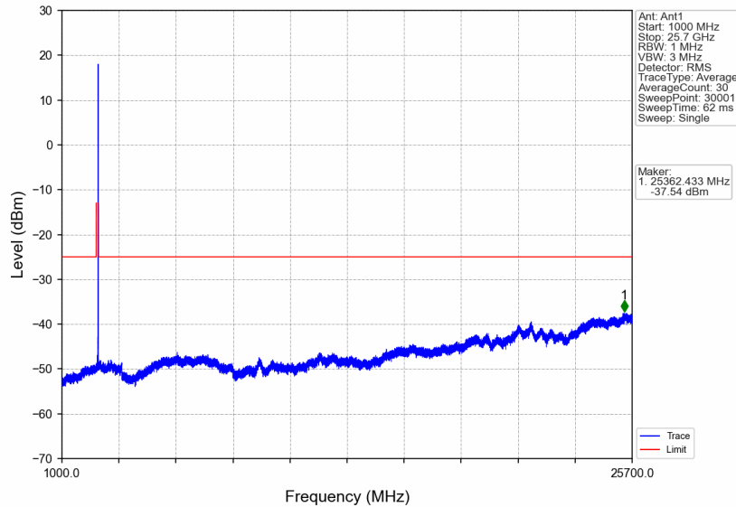
n7_15kHz_SISO_NTNV_15MHz_CP-OFDM QPSK_2562.5MHz_Edge_1RB_Right
