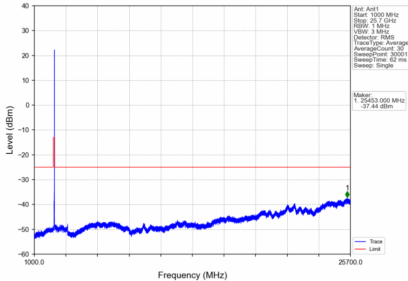
n7_15kHz_SISO_NTNV_20MHz_DFT-s-OFDM QPSK_2560MHz_Edge_1RB_Right
