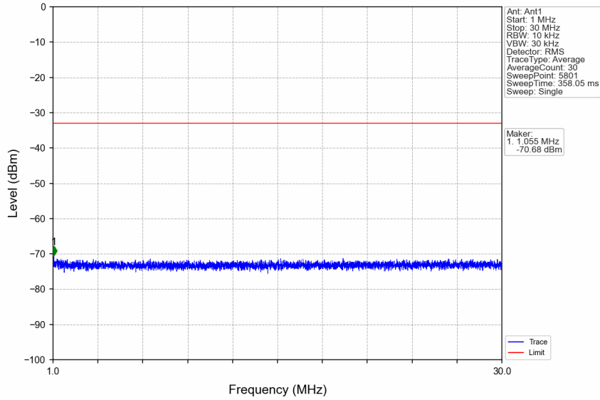
n7_15kHz_SISO_NTNV_25MHz_DFT-s-OFDM QPSK_2535MHz_Edge_1RB_Left
