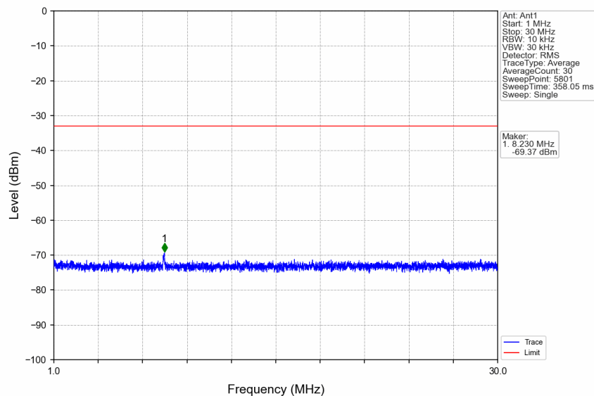
n7_15kHz_SISO_NTNV_20MHz_DFT-s-OFDM QPSK_2560MHz_Edge_1RB_Right
