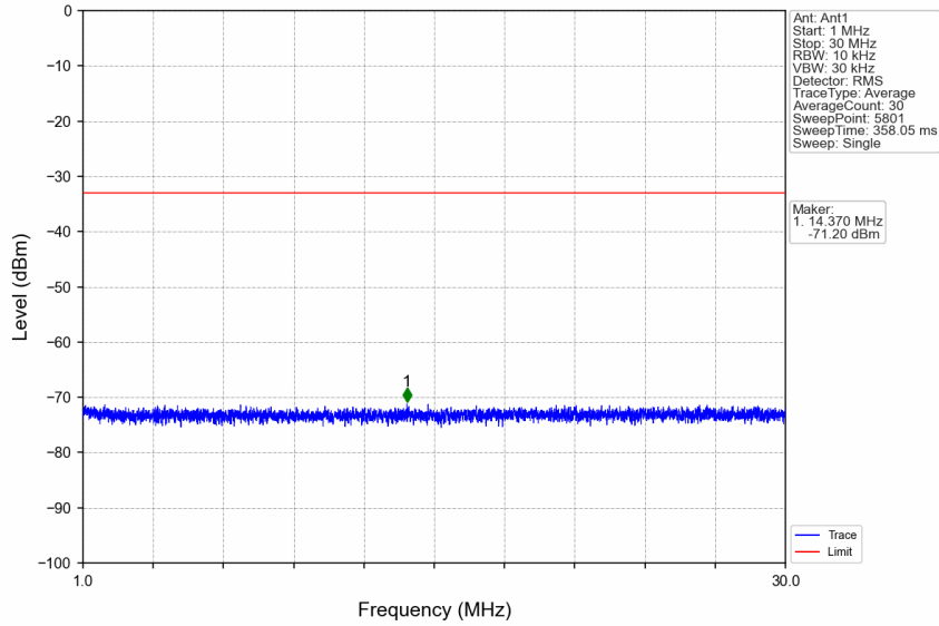
n7_15kHz_SISO_NTNV_15MHz_CP-OFDM QPSK_2535MHz_Edge_1RB_Left
