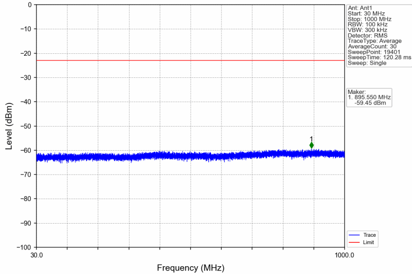
n7_15kHz_SISO_NTNV_10MHz_DFT-s-OFDM QPSK_2565MHz_Edge_1RB_Right
