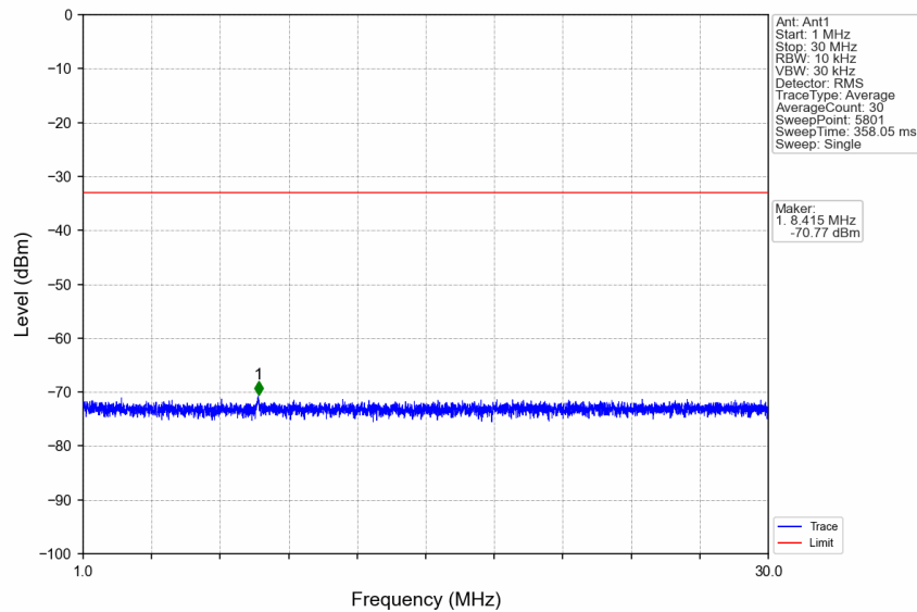
n7_15kHz_SISO_NTNV_5MHz_CP-OFDM QPSK_2567.5MHz_Edge_1RB_Right
