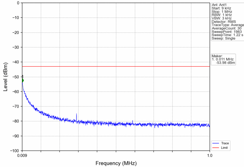
n7_15kHz_SISO_NTNV_15MHz_DFT-s-OFDM_QPSK_2562.5MHz_Edge_1RB_Right
