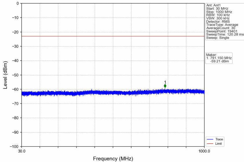
n7_15kHz_SISO_NTNV_10MHz_DFT-s-OFDM QPSK_2505MHz_Edge_1RB_Left
