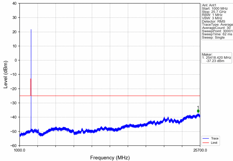
n7_15kHz_SISO_NTNV_15MHz_DFT-s-OFDM_QPSK_2562.5MHz_Edge_1RB_Right
