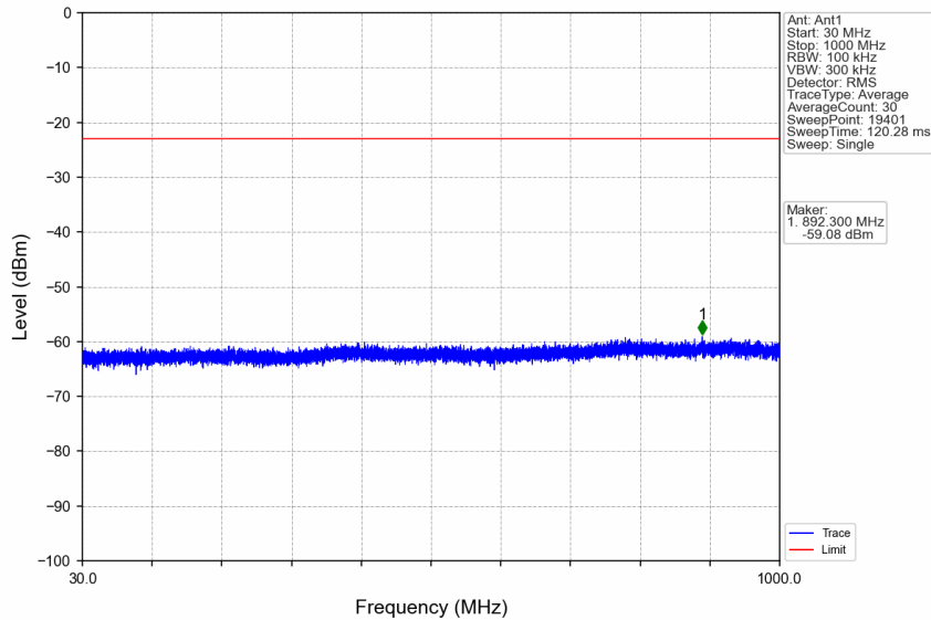
n7_15kHz_SISO_NTNV_15MHz_DFT-s-OFDM QPSK_2507.5MHz_Edge_1RB_Left
