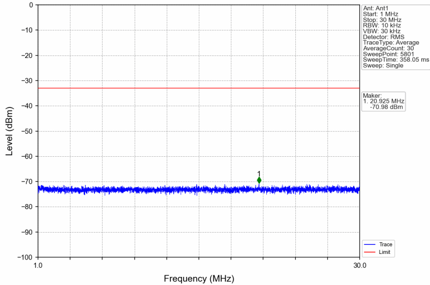
n7_15kHz_SISO_NTNV_10MHz_DFT-s-OFDM QPSK_2535MHz_Edge_1RB_Left
