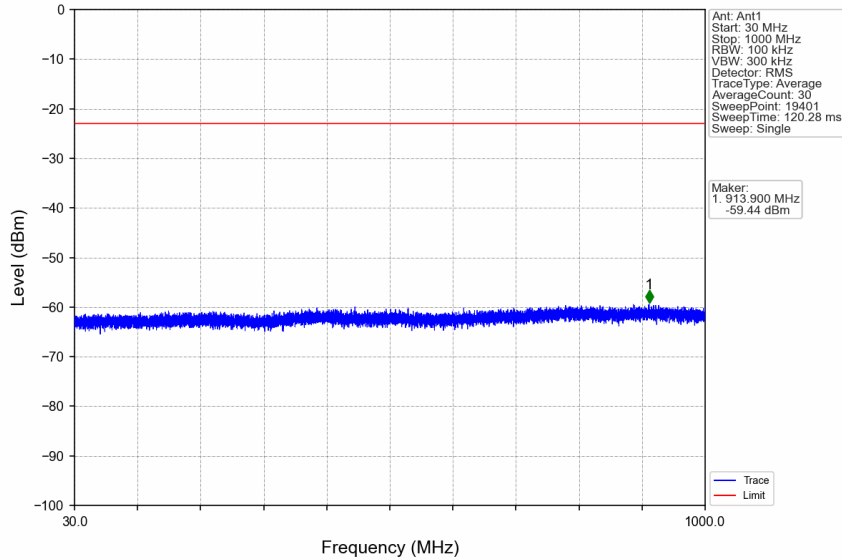
n7_15kHz_SISO_NTNV_10MHz_CP-OFDM QPSK_2565MHz_Edge_1RB_Right
