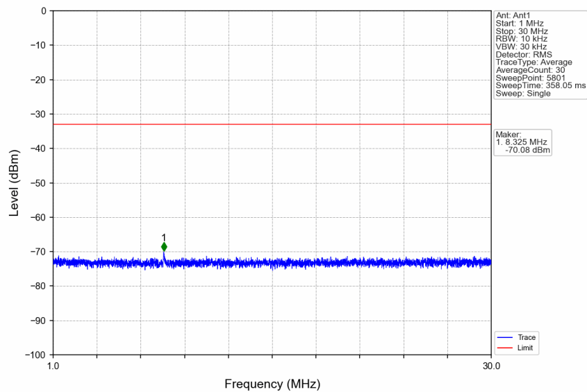
n7_15kHz_SISO_NTNV_10MHz_CP-OFDM QPSK_2565MHz_Edge_1RB_Right
