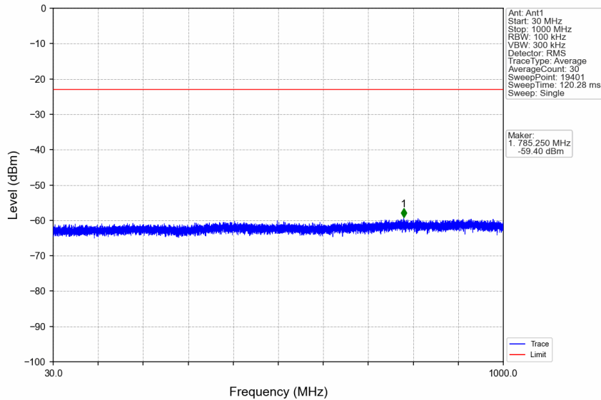
n7_15kHz_SISO_NTNV_10MHz_CP-OFDM QPSK_2505MHz_Edge_1RB_Left
