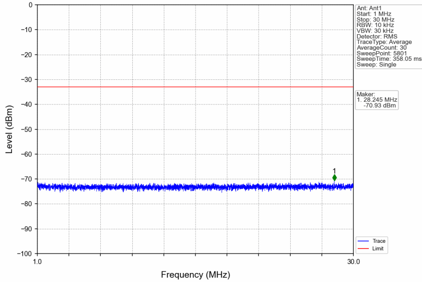
n7_15kHz_SISO_NTNV_15MHz_DFT-s-OFDM QPSK_2507.5MHz_Edge_1RB_Left
