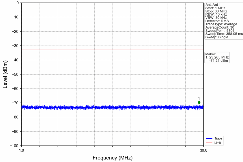
n7_15kHz_SISO_NTNV_10MHz_CP-OFDM QPSK_2505MHz_Edge_1RB_Left
