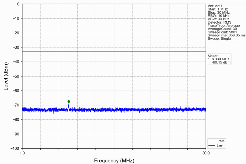
n7_15kHz_SISO_NTNV_10MHz_DFT-s-OFDM QPSK_2565MHz_Edge_1RB_Right
