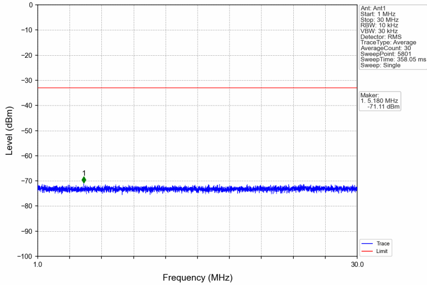
n7_15kHz_SISO_NTNV_10MHz_CP-OFDM QPSK_2535MHz_Edge_1RB_Left
