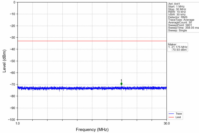
n7_15kHz_SISO_NTNV_10MHz_DFT-s-OFDM QPSK_2505MHz_Edge_1RB_Left
