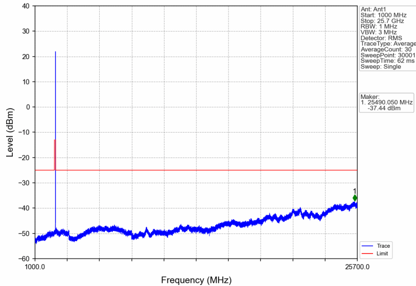
n7_15kHz_SISO_NTNV_10MHz_DFT-s-OFDM QPSK_2565MHz_Edge_1RB_Right
