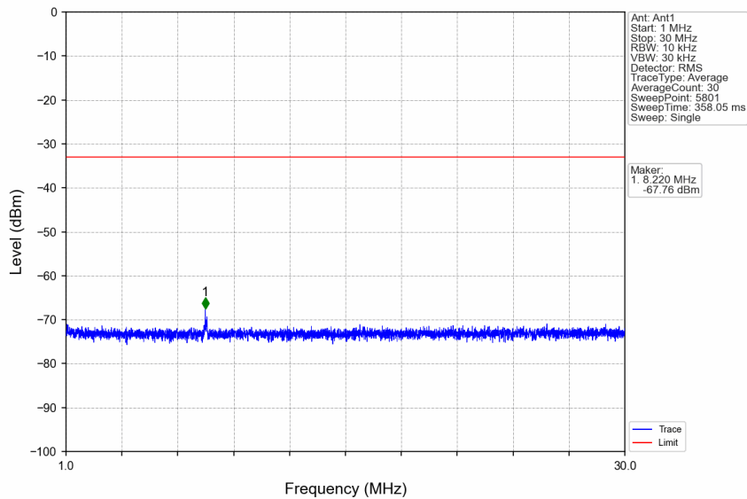
n7_15kHz_SISO_NTNV_15MHz_DFT-s-OFDM PI/2 BPSK_2562.5MHz_Edge_1RB_Right
