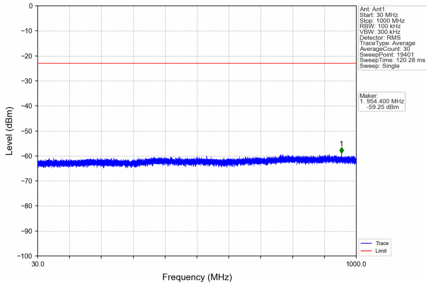
n7_15kHz_SISO_NTNV_10MHz_CP-OFDM QPSK_2535MHz_Edge_1RB_Left
