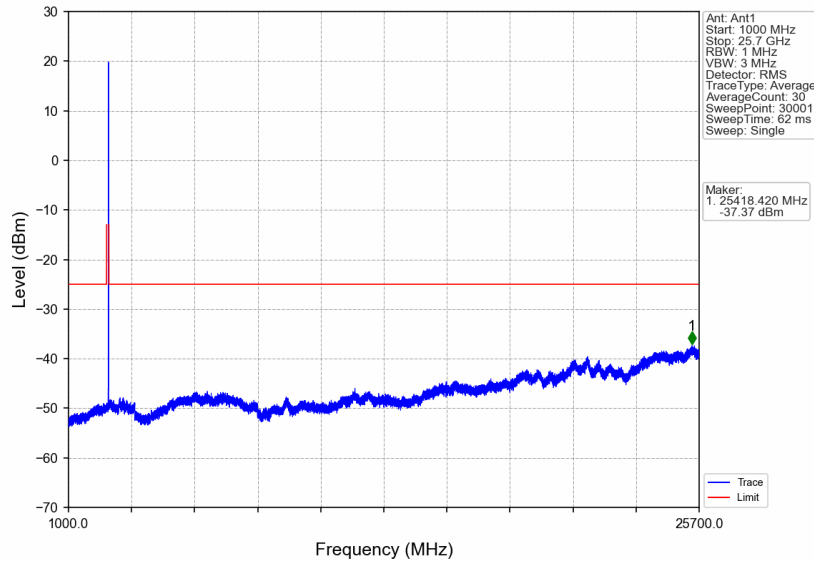
n7_15kHz_SISO_NTNV_10MHz_CP-OFDM QPSK_2565MHz_Edge_1RB_Right
