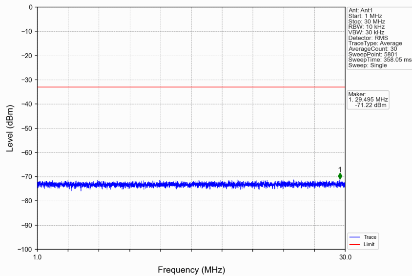
n7_15kHz_SISO_NTNV_15MHz_DFT-s-OFDM QPSK_2535MHz_Edge_1RB_Left
