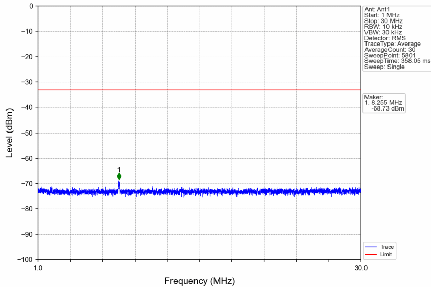
n7_15kHz_SISO_NTNV_15MHz_DFT-s-OFDM_QPSK_2562.5MHz_Edge_1RB_Right
