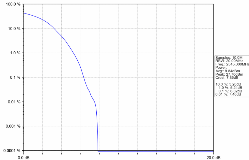
n7_30kHz_SISO_NTNV_50MHz_DFT-s-OFDM QPSK_2545MHz_Outer_Full
