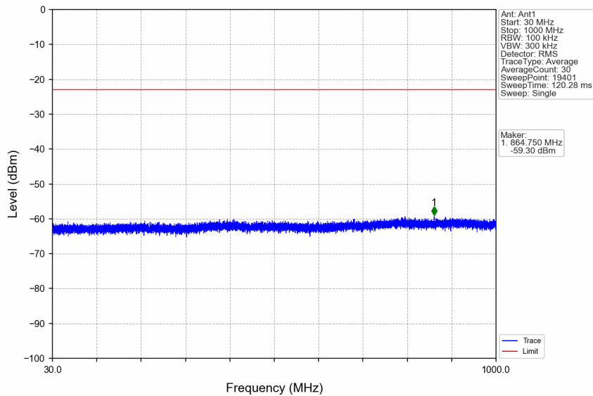
n7_15kHz_SISO_NTNV_5MHz_DFT-s-OFDM QPSK_2535MHz_Edge_1RB_Left
