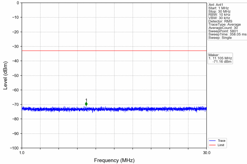
n7_15kHz_SISO_NTNV_5MHz_CP-OFDM QPSK_2502.5MHz_Edge_1RB_Left
