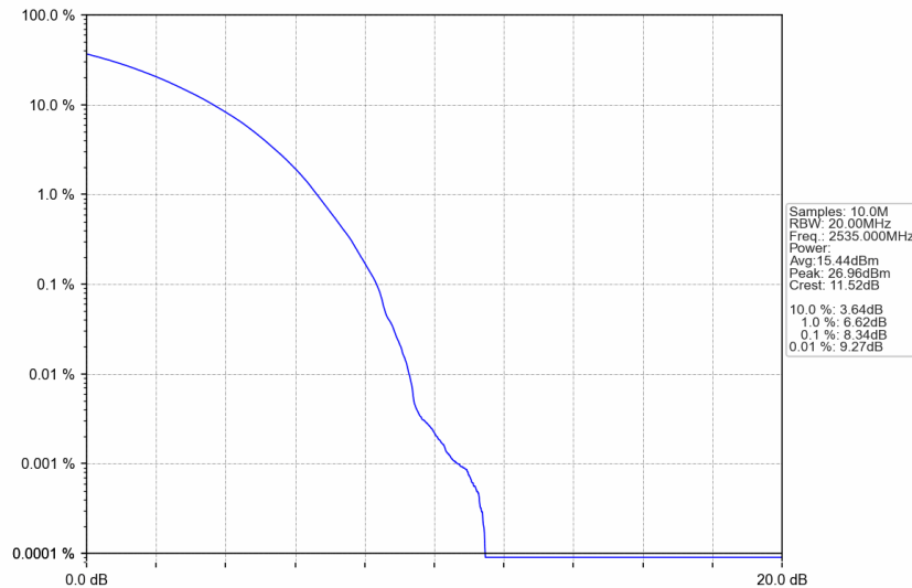
n7_30kHz_SISO_NTNV_40MHz_CP-OFDM 256 QAM_2535MHz_Outer_Full
