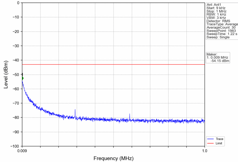
n7_15kHz_SISO_NTNV_5MHz_DFT-s-OFDM QPSK_2567.5MHz_Edge_1RB_Right
