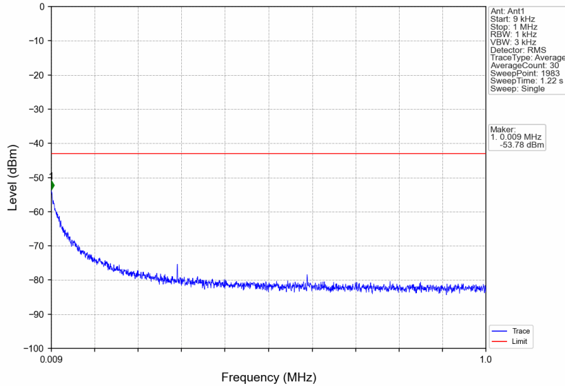
n7_15kHz_SISO_NTNV_5MHz_DFT-s-OFDM PI/2 BPSK_2567.5MHz_Edge_1RB_Right
