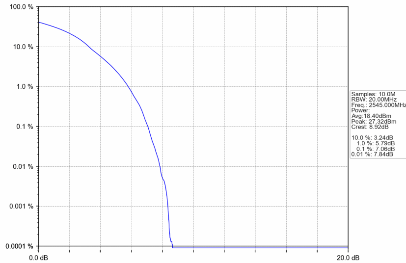
n7_30kHz_SISO_NTNV_50MHz_DFT-s-OFDM 64 QAM_2545MHz_Outer_Full
