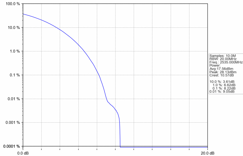
n7_30kHz_SISO_NTNV_50MHz_CP-OFDM 64 QAM_2535MHz_Outer_Full
