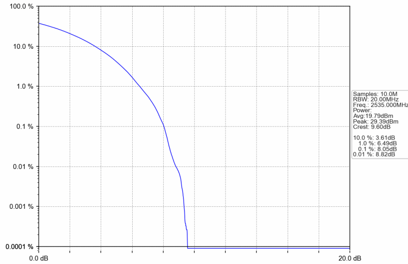
n7_30kHz_SISO_NTNV_30MHz_CP-OFDM 64 QAM_2535MHz_Outer_Full
