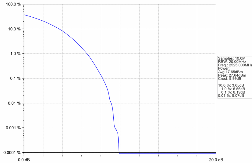
n7_30kHz_SISO_NTNV_50MHz_CP-OFDM QPSK_2525MHz_Outer_Full
