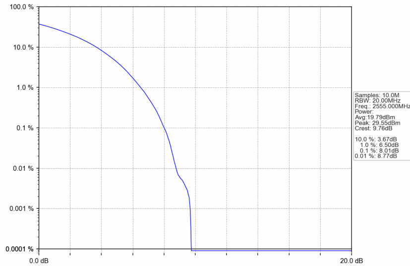
n7_30kHz_SISO_NTNV_30MHz_CP-OFDM QPSK_2555MHz_Outer_Full
