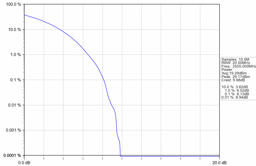
n7_30kHz_SISO_NTNV_30MHz_CP-OFDM 64 QAM_2555MHz_Outer_Full
