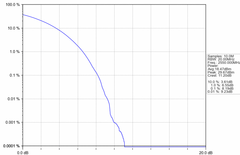
n7_30kHz_SISO_NTNV_40MHz_CP-OFDM QPSK_2550MHz_Outer_Full
