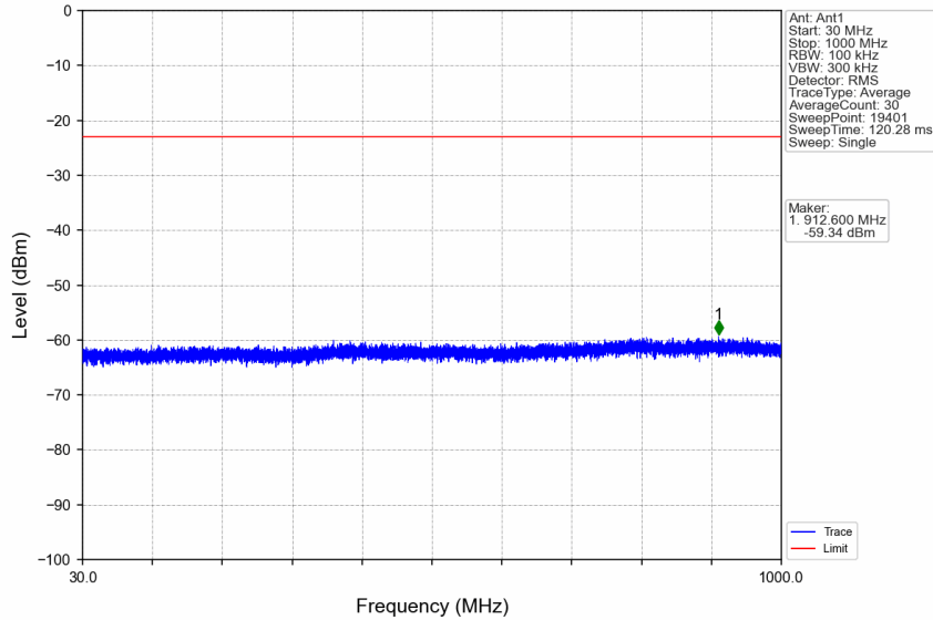
n7_15kHz_SISO_NTNV_5MHz_DFT-s-OFDM QPSK_2567.5MHz_Edge_1RB_Right
