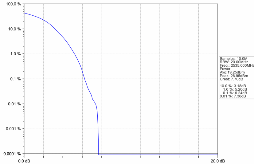
n7_30kHz_SISO_NTNV_50MHz_DFT-s-OFDM QPSK_2535MHz_Outer_Full
