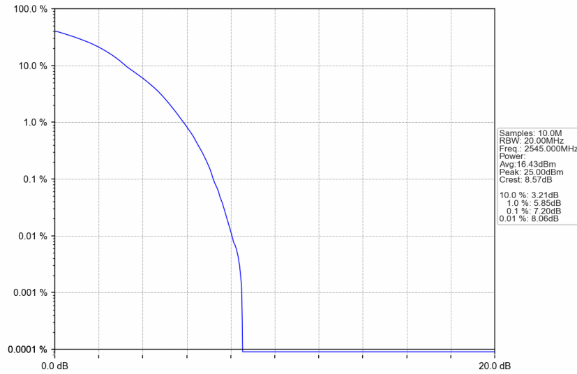
n7_30kHz_SISO_NTNV_50MHz_DFT-s-OFDM 256 QAM_2545MHz_Outer_Full
