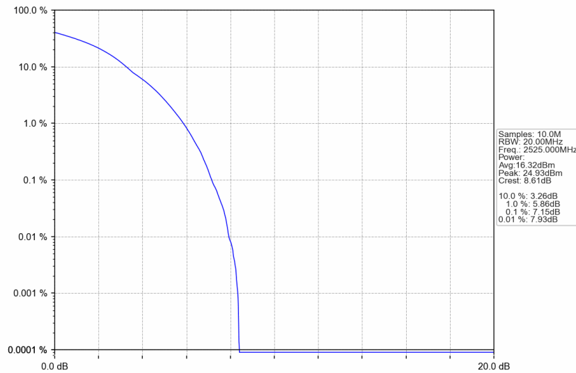
n7_30kHz_SISO_NTNV_50MHz_DFT-s-OFDM 256 QAM_2525MHz_Outer_Full
