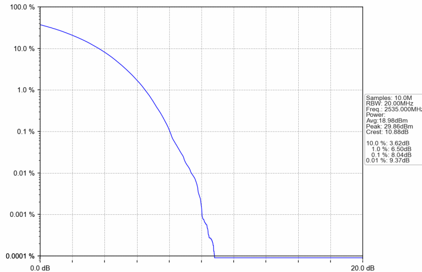
n7_30kHz_SISO_NTNV_40MHz_CP-OFDM 16 QAM_2535MHz_Outer_Full
