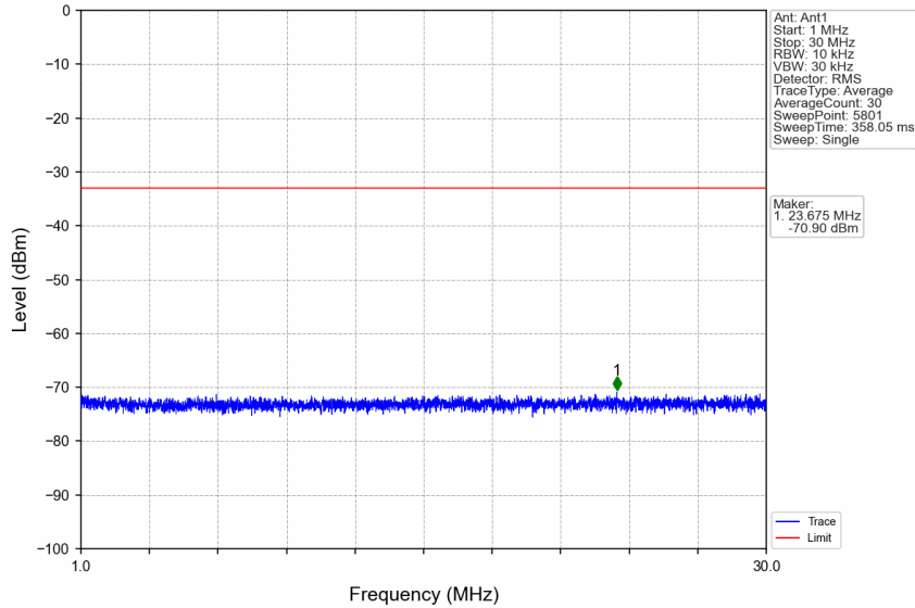
n7_15kHz_SISO_NTNV_5MHz_DFT-s-OFDM PI/2 BPSK_2502.5MHz_Edge_1RB_Left
