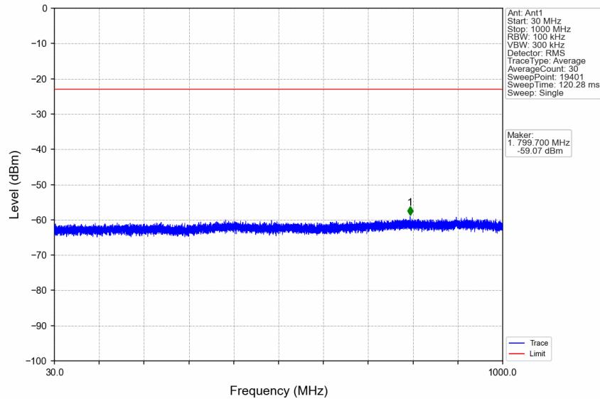
n7_15kHz_SISO_NTNV_5MHz_CP-OFDM QPSK_2535MHz_Edge_1RB_Left
