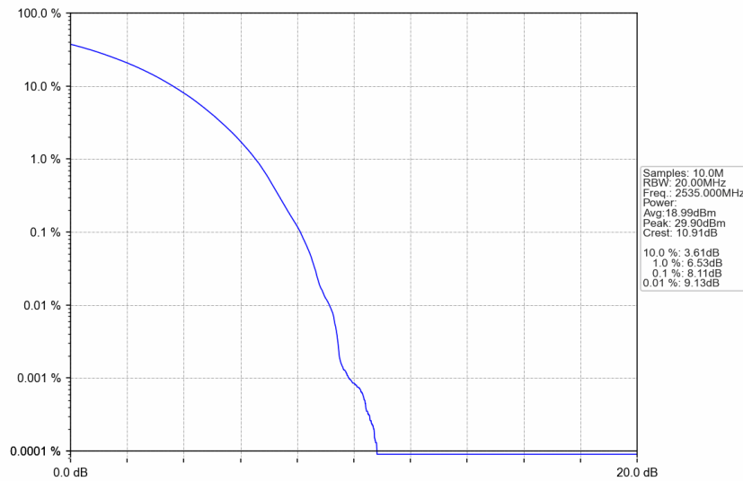
n7_30kHz_SISO_NTNV_40MHz_CP-OFDM QPSK_2535MHz_Outer_Full
