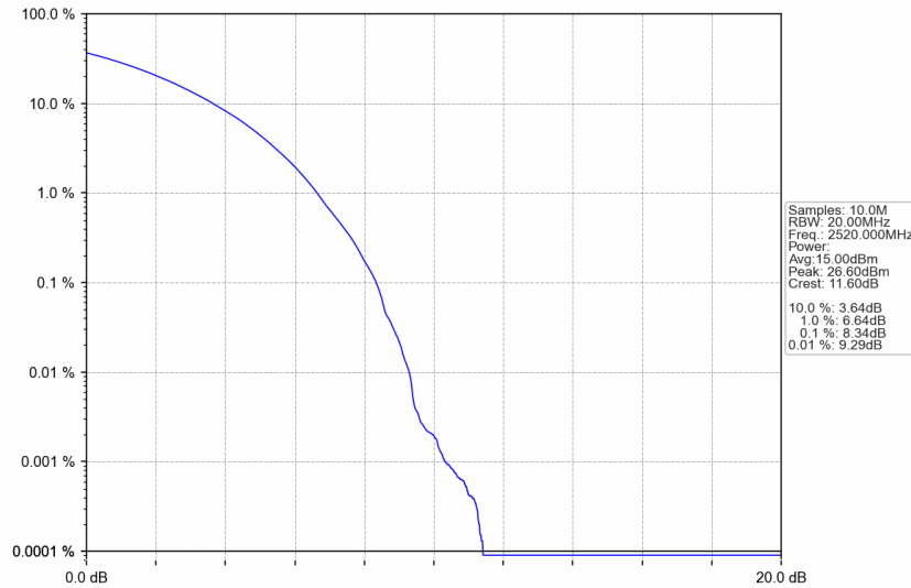
n7_30kHz_SISO_NTNV_40MHz_CP-OFDM 256 QAM_2520MHz_Outer_Full
