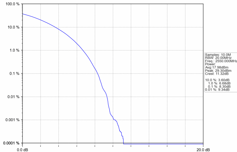
n7_30kHz_SISO_NTNV_40MHz_CP-OFDM 64 QAM_2550MHz_Outer_Full
