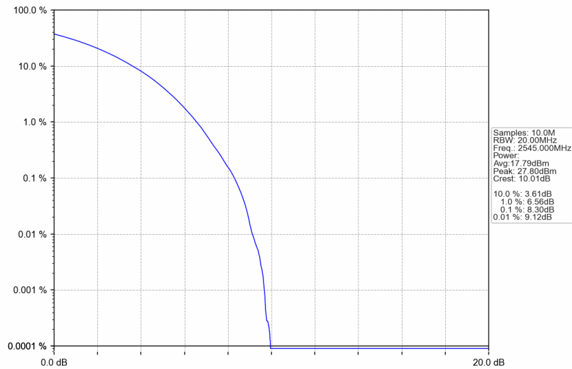
n7_30kHz_SISO_NTNV_50MHz_CP-OFDM 16 QAM_2545MHz_Outer_Full
