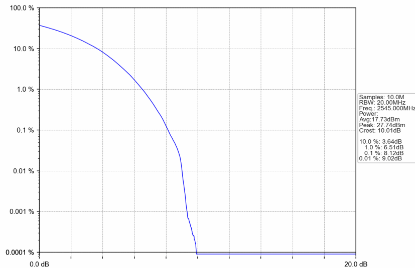
n7_30kHz_SISO_NTNV_50MHz_CP-OFDM QPSK_2545MHz_Outer_Full
