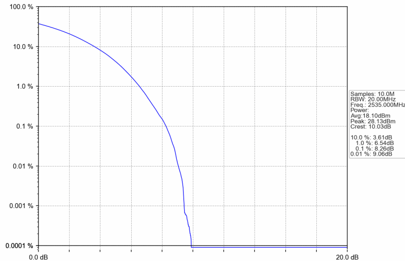
n7_30kHz_SISO_NTNV_50MHz_CP-OFDM 16 QAM_2535MHz_Outer_Full
