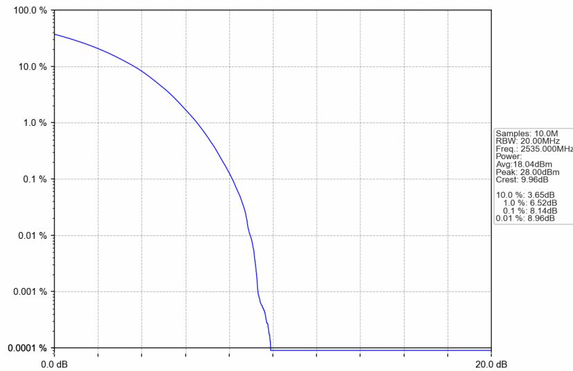
n7_30kHz_SISO_NTNV_50MHz_CP-OFDM QPSK_2535MHz_Outer_Full
