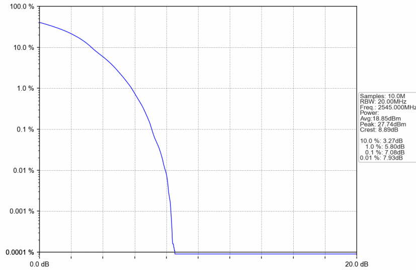
n7_30kHz_SISO_NTNV_50MHz_DFT-s-OFDM 16 QAM_2545MHz_Outer_Full
