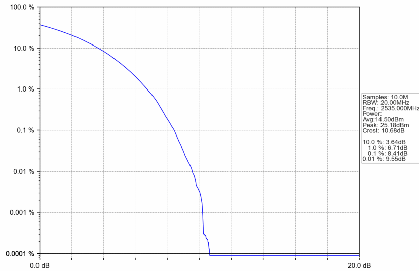
n7_30kHz_SISO_NTNV_50MHz_CP-OFDM 256 QAM_2535MHz_Outer_Full
