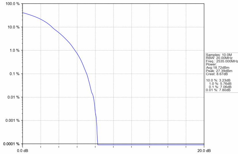
n7_30kHz_SISO_NTNV_50MHz_DFT-s-OFDM 64 QAM_2535MHz_Outer_Full
