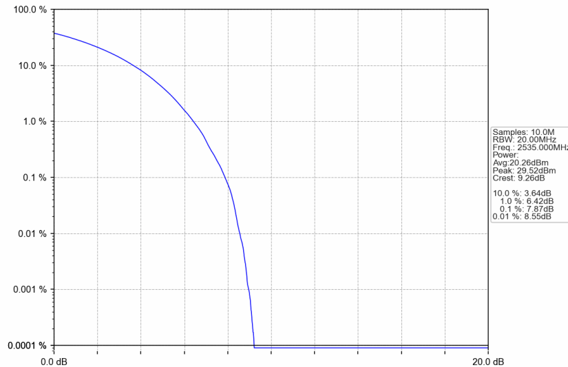
n7_30kHz_SISO_NTNV_30MHz_CP-OFDM 16 QAM_2535MHz_Outer_Full
