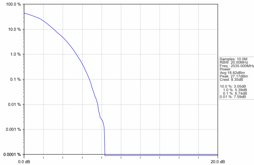
n7_30kHz_SISO_NTNV_30MHz_DFT-s-OFDM 256 QAM_2535MHz_Outer_Full
