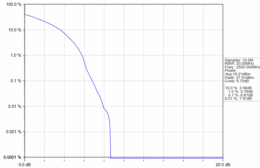
n7_30kHz_SISO_NTNV_40MHz_DFT-s-OFDM 64 QAM_2550MHz_Outer_Full
