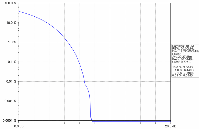
n7_30kHz_SISO_NTNV_30MHz_CP-OFDM QPSK_2535MHz_Outer_Full
