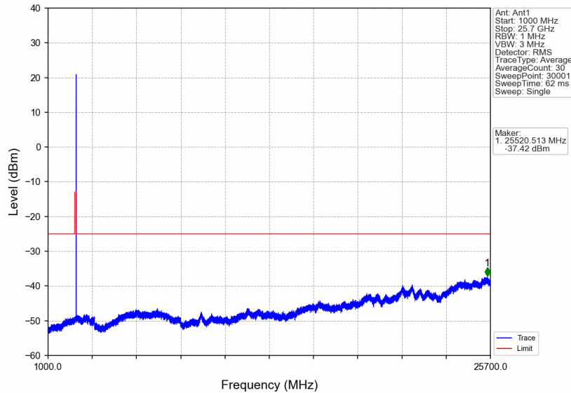
n7_15kHz_SISO_NTNV_5MHz_DFT-s-OFDM QPSK_2567.5MHz_Edge_1RB_Right
