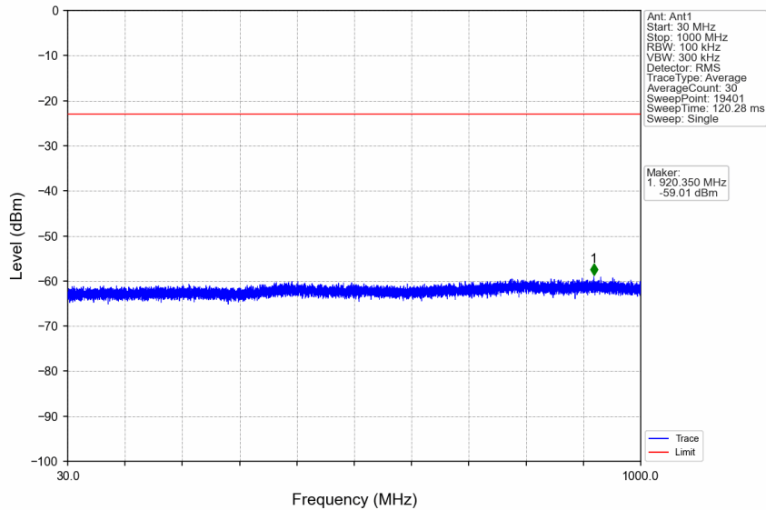
n7_15kHz_SISO_NTNV_5MHz_DFT-s-OFDM QPSK_2502.5MHz_Edge_1RB_Left
