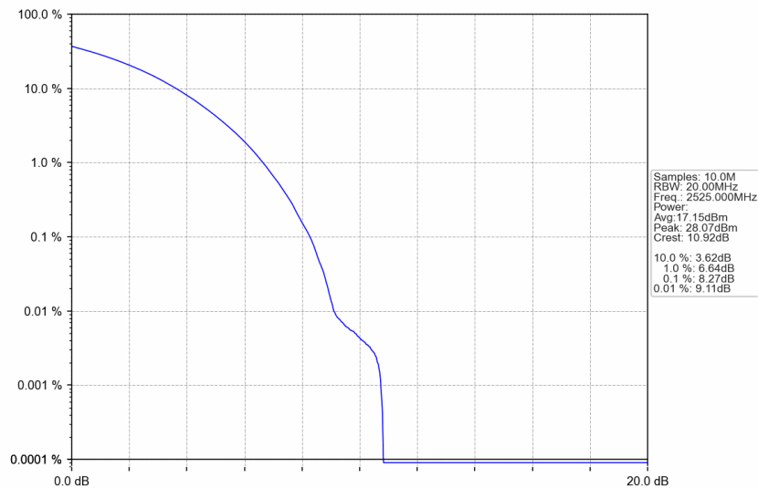
n7_30kHz_SISO_NTNV_50MHz_CP-OFDM 64 QAM_2525MHz_Outer_Full
