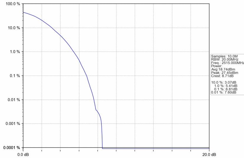
n7_30kHz_SISO_NTNV_30MHz_DFT-s-OFDM 256 QAM_2515MHz_Outer_Full
