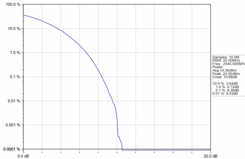
n7_30kHz_SISO_NTNV_50MHz_CP-OFDM 256 QAM_2545MHz_Outer_Full
