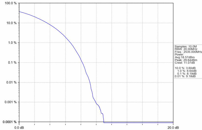
n7_30kHz_SISO_NTNV_40MHz_CP-OFDM 64 QAM_2535MHz_Outer_Full
