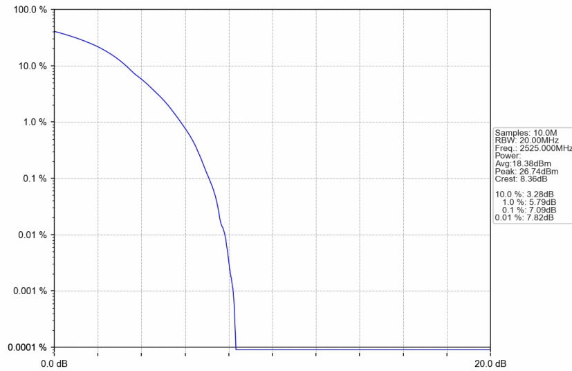
n7_30kHz_SISO_NTNV_50MHz_DFT-s-OFDM 64 QAM_2525MHz_Outer_Full
