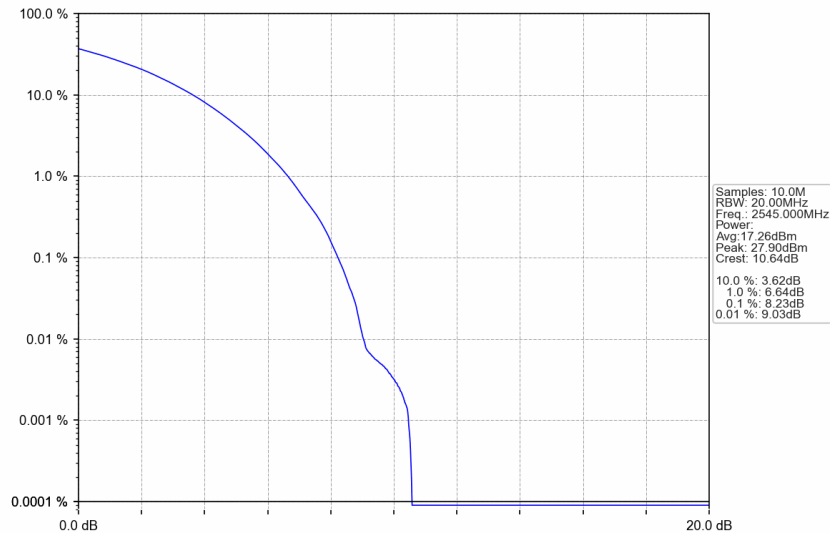
n7_30kHz_SISO_NTNV_50MHz_CP-OFDM 64 QAM_2545MHz_Outer_Full
