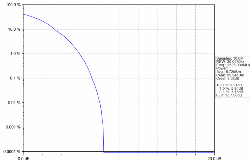
n7_30kHz_SISO_NTNV_50MHz_DFT-s-OFDM 256 QAM_2535MHz_Outer_Full
