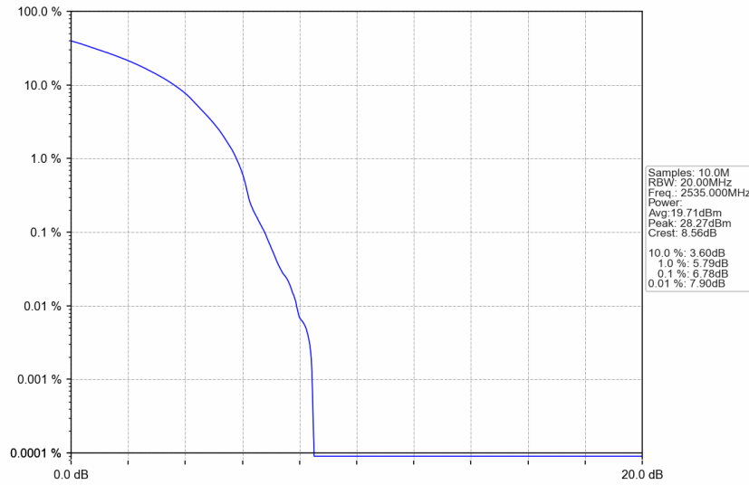
n7_30kHz_SISO_NTNV_40MHz_DFT-s-OFDM 64 QAM_2535MHz_Outer_Full
