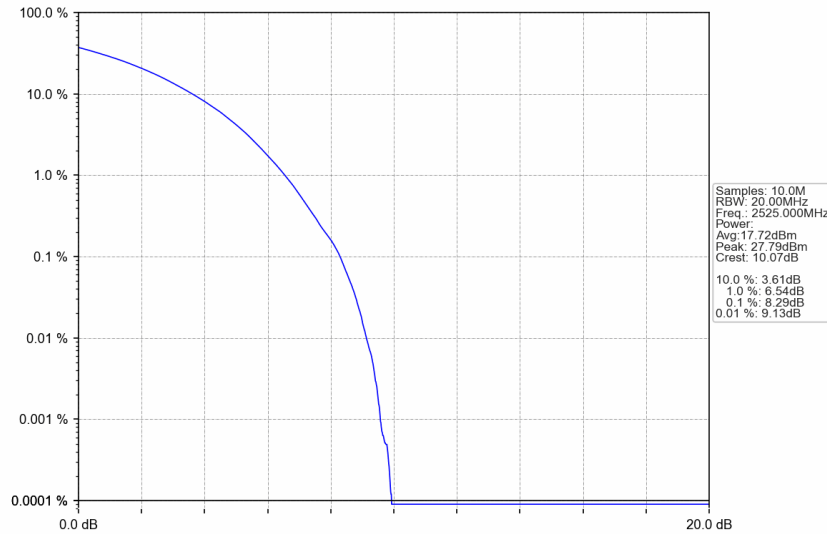
n7_30kHz_SISO_NTNV_50MHz_CP-OFDM 16 QAM_2525MHz_Outer_Full
