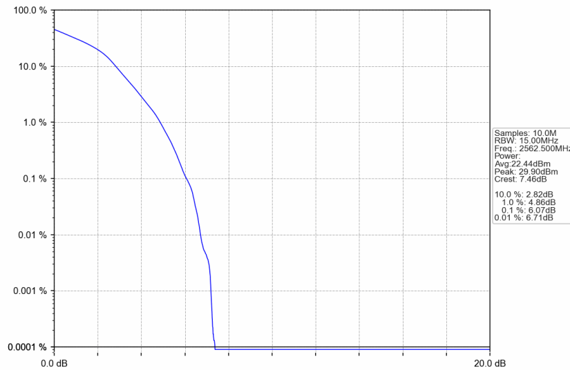
n7_30kHz_SISO_NTNV_15MHz_DFT-s-OFDM 16 QAM_2562.5MHz_Outer_Full
