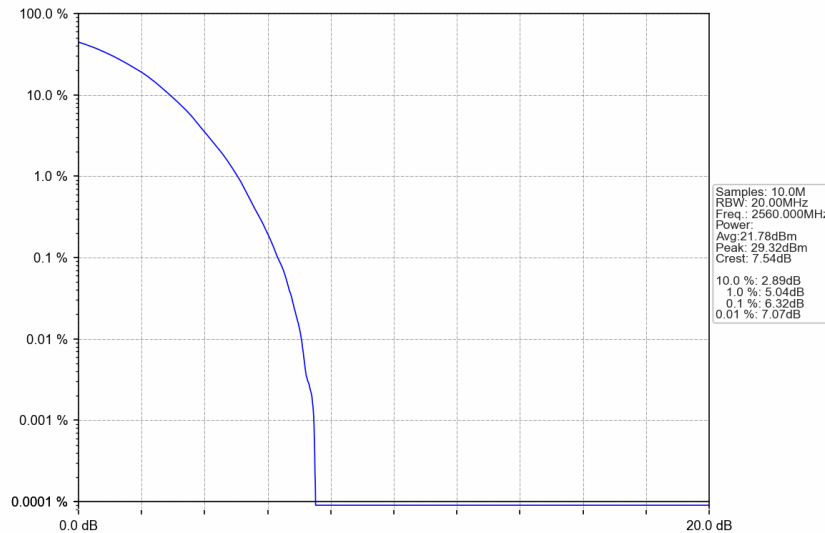
n7_30kHz_SISO_NTNV_20MHz_DFT-s-OFDM 64 QAM_2560MHz_Outer_Full
