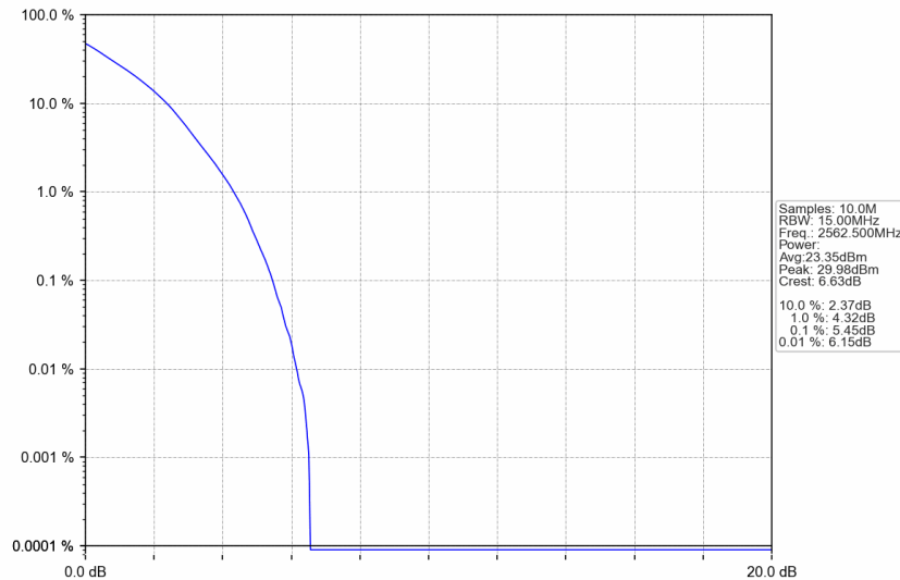
n7_30kHz_SISO_NTNV_15MHz_DFT-s-OFDM QPSK_2562.5MHz_Outer_Full
