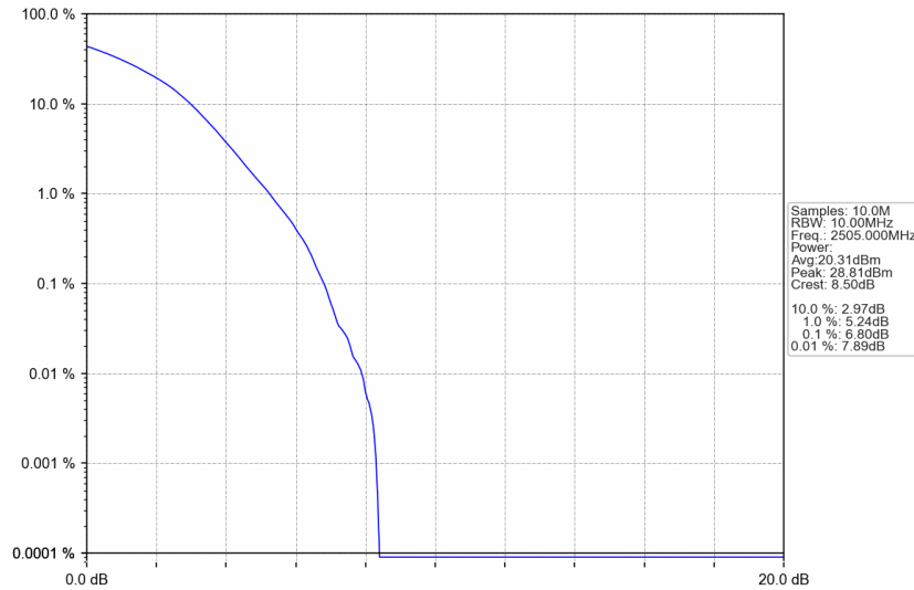
n7_30kHz_SISO_NTNV_10MHz_DFT-s-OFDM 256 QAM_2505MHz_Outer_Full
