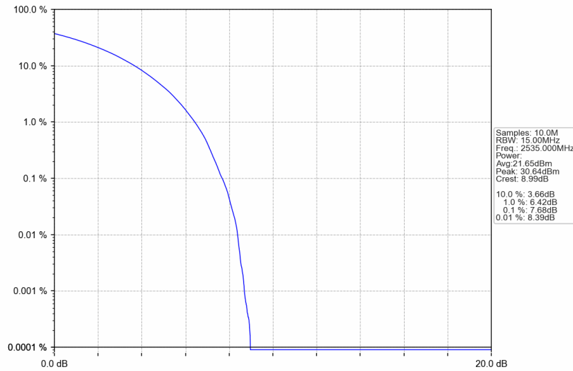
n7_30kHz_SISO_NTNV_15MHz_CP-OFDM 16 QAM_2535MHz_Outer_Full
