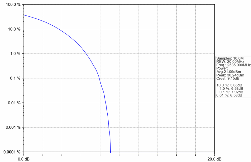
n7_30kHz_SISO_NTNV_20MHz_CP-OFDM 64 QAM_2535MHz_Outer_Full
