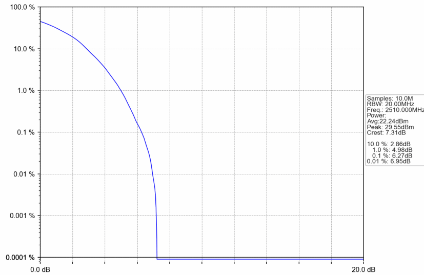
n7_30kHz_SISO_NTNV_20MHz_DFT-s-OFDM 64 QAM_2510MHz_Outer_Full
