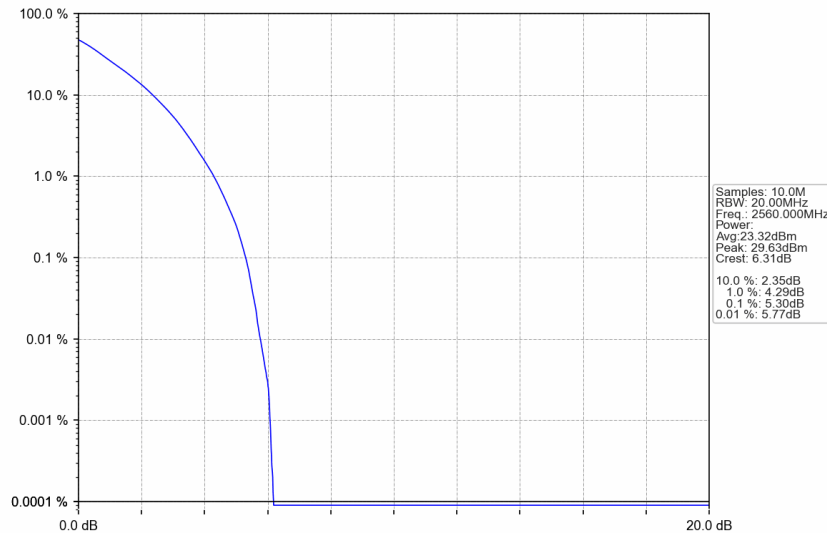
n7_30kHz_SISO_NTNV_20MHz_DFT-s-OFDM QPSK_2560MHz_Outer_Full
