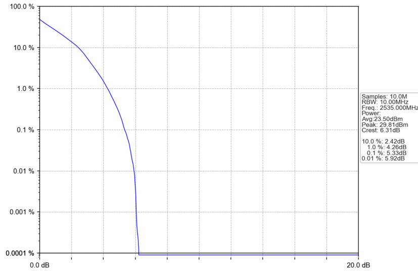
n7_30kHz_SISO_NTNV_10MHz_DFT-s-OFDM QPSK_2535MHz_Outer_Full
