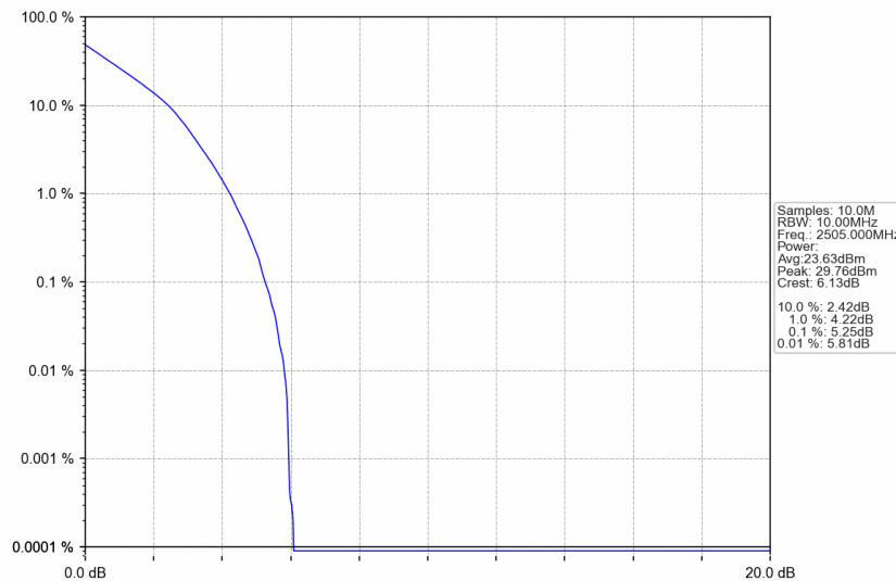
n7_30kHz_SISO_NTNV_10MHz_DFT-s-OFDM QPSK_2505MHz_Outer_Full
