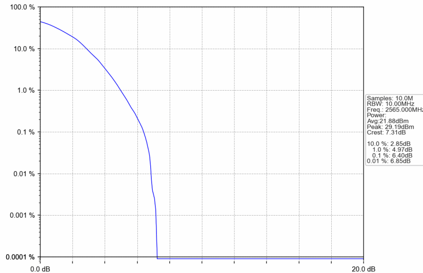
n7_30kHz_SISO_NTNV_10MHz_DFT-s-OFDM 64 QAM_2565MHz_Outer_Full
