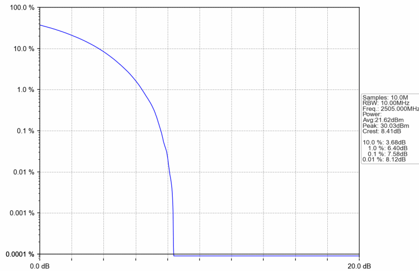
n7_30kHz_SISO_NTNV_10MHz_CP-OFDM 16 QAM_2505MHz_Outer_Full
