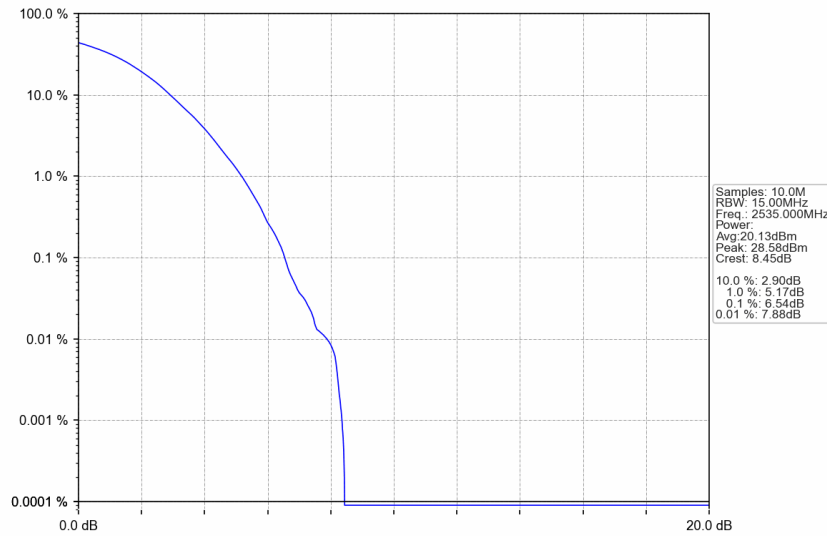
n7_30kHz_SISO_NTNV_15MHz_DFT-s-OFDM 256 QAM_2535MHz_Outer_Full
