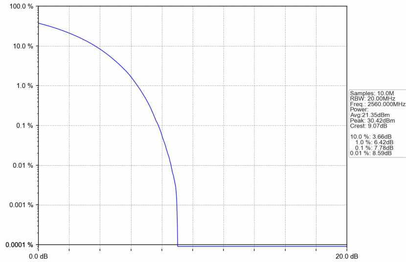
n7_30kHz_SISO_NTNV_20MHz_CP-OFDM 16 QAM_2560MHz_Outer_Full
