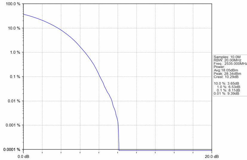
n7_15kHz_SISO_NTNV_50MHz_CP-OFDM QPSK_2535MHz_Outer_Full
