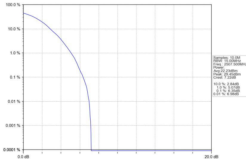
n7_30kHz_SISO_NTNV_15MHz_DFT-s-OFDM 64 QAM_2507.5MHz_Outer_Full
