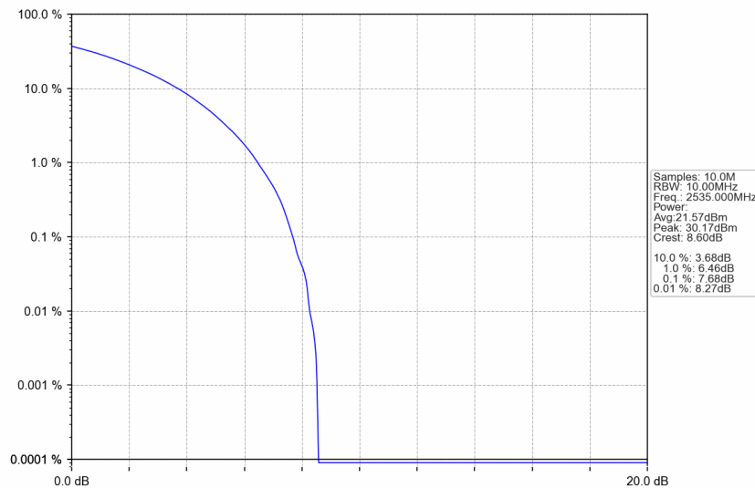
n7_30kHz_SISO_NTNV_10MHz_CP-OFDM 16 QAM_2535MHz_Outer_Full
