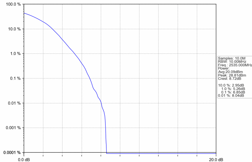
n7_30kHz_SISO_NTNV_10MHz_DFT-s-OFDM 256 QAM_2535MHz_Outer_Full
