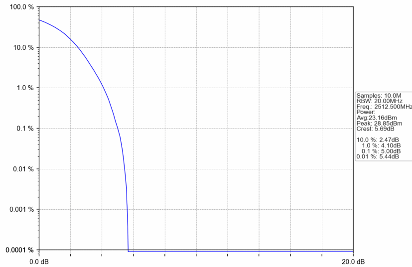
n7_30kHz_SISO_NTNV_25MHz_DFT-s-OFDM QPSK_2512.5MHz_Outer_Full
