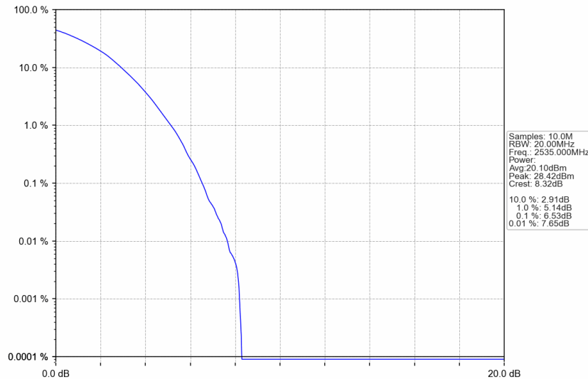
n7_30kHz_SISO_NTNV_20MHz_DFT-s-OFDM 256 QAM_2535MHz_Outer_Full
