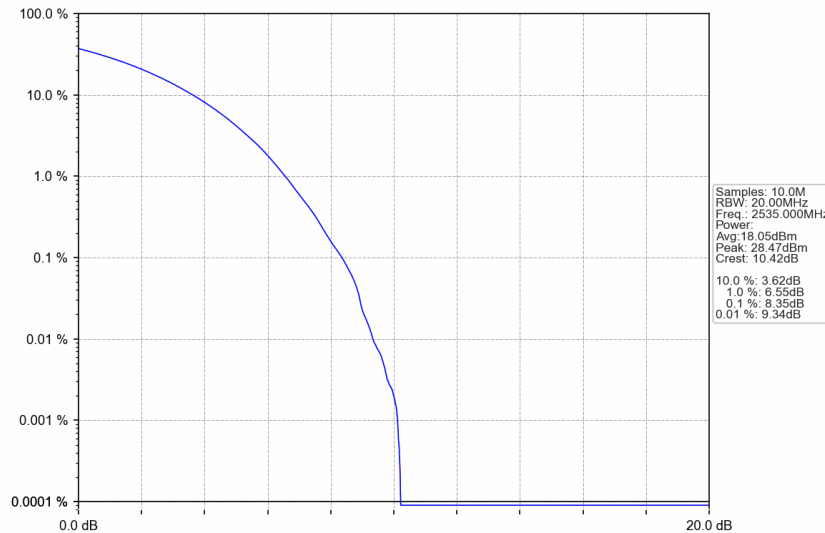
n7_15kHz_SISO_NTNV_50MHz_CP-OFDM 16 QAM_2535MHz_Outer_Full
