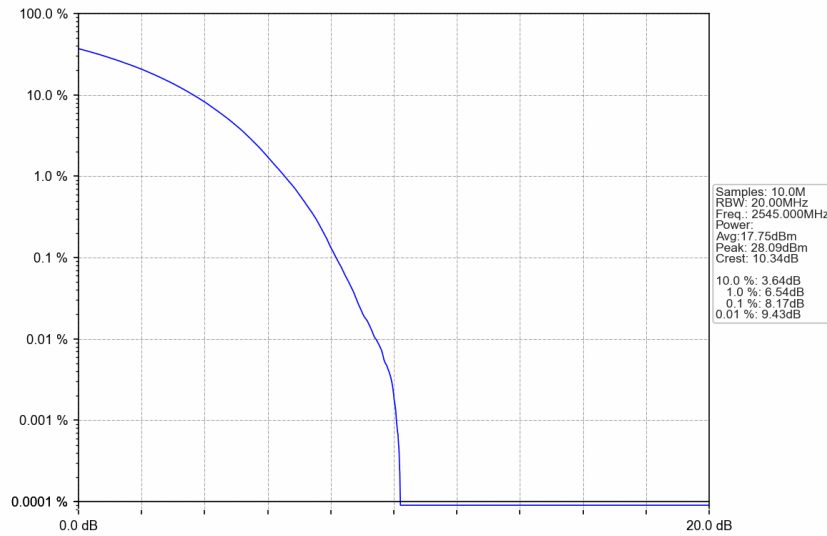
n7_15kHz_SISO_NTNV_50MHz_CP-OFDM QPSK_2545MHz_Outer_Full
