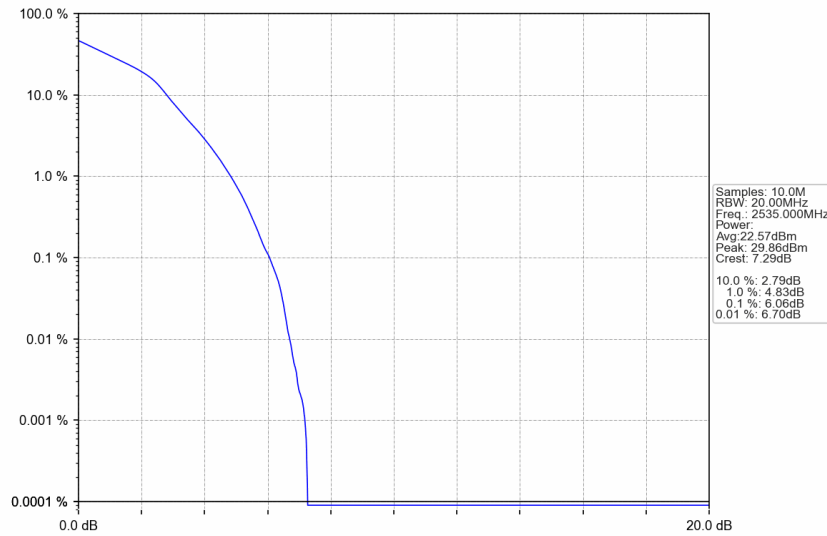
n7_30kHz_SISO_NTNV_20MHz_DFT-s-OFDM_16_QAM_2535MHz_Outer_Full
