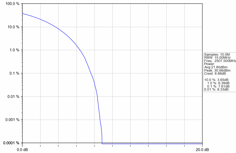
n7_30kHz_SISO_NTNV_15MHz_CP-OFDM 16 QAM_2507.5MHz_Outer_Full
