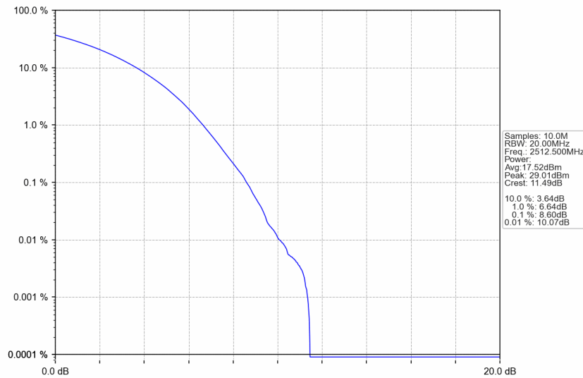
n7_30kHz_SISO_NTNV_25MHz_CP-OFDM 256 QAM_2512.5MHz_Outer_Full
