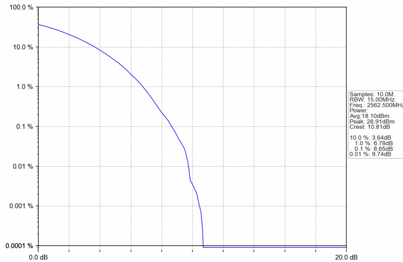
n7_30kHz_SISO_NTNV_15MHz_CP-OFDM 256 QAM_2562.5MHz_Outer_Full
