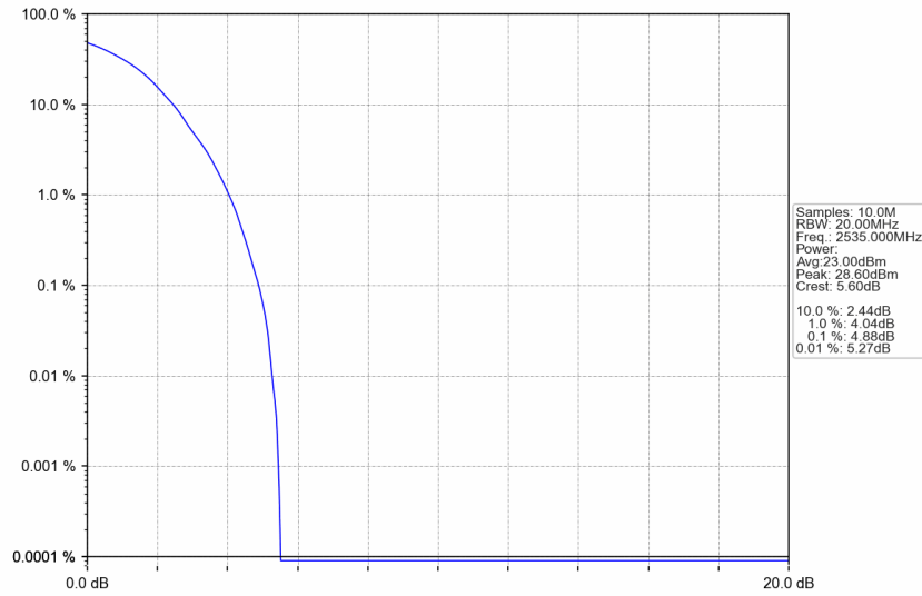
n7_30kHz_SISO_NTNV_25MHz_DFT-s-OFDM QPSK_2535MHz_Outer_Full
