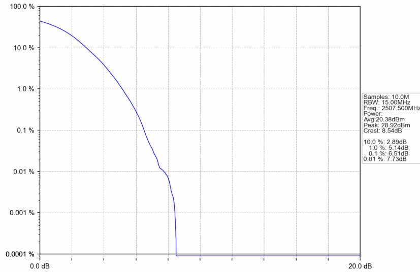
n7_30kHz_SISO_NTNV_15MHz_DFT-s-OFDM 256 QAM_2507.5MHz_Outer_Full
