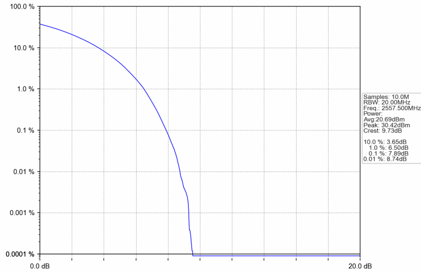
n7_30kHz_SISO_NTNV_25MHz_CP-OFDM 16 QAM_2557.5MHz_Outer_Full
