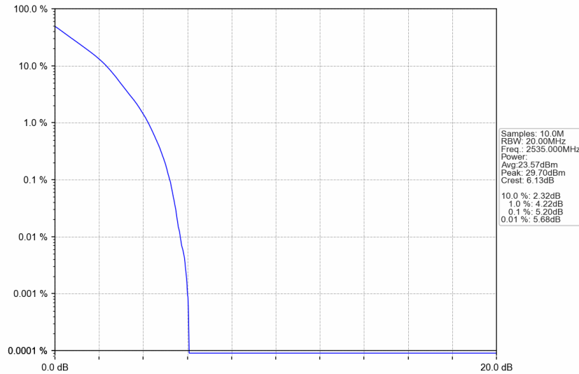
n7_30kHz_SISO_NTNV_20MHz_DFT-s-OFDM QPSK_2535MHz_Outer_Full
