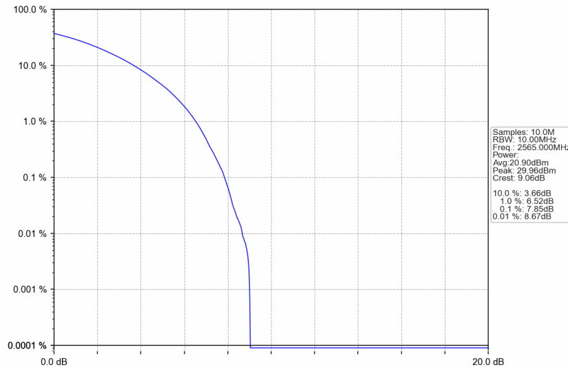
n7_30kHz_SISO_NTNV_10MHz_CP-OFDM 64 QAM_2565MHz_Outer_Full
