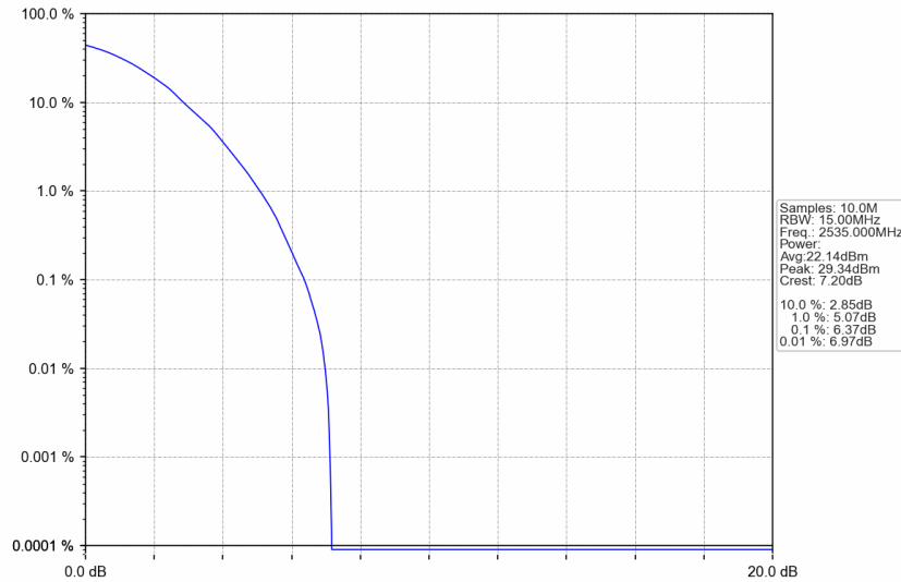
n7_30kHz_SISO_NTNV_15MHz_DFT-s-OFDM 64 QAM_2535MHz_Outer_Full
