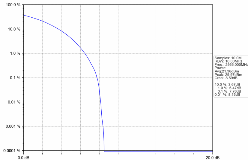
n7_30kHz_SISO_NTNV_10MHz_CP-OFDM QPSK_2565MHz_Outer_Full
