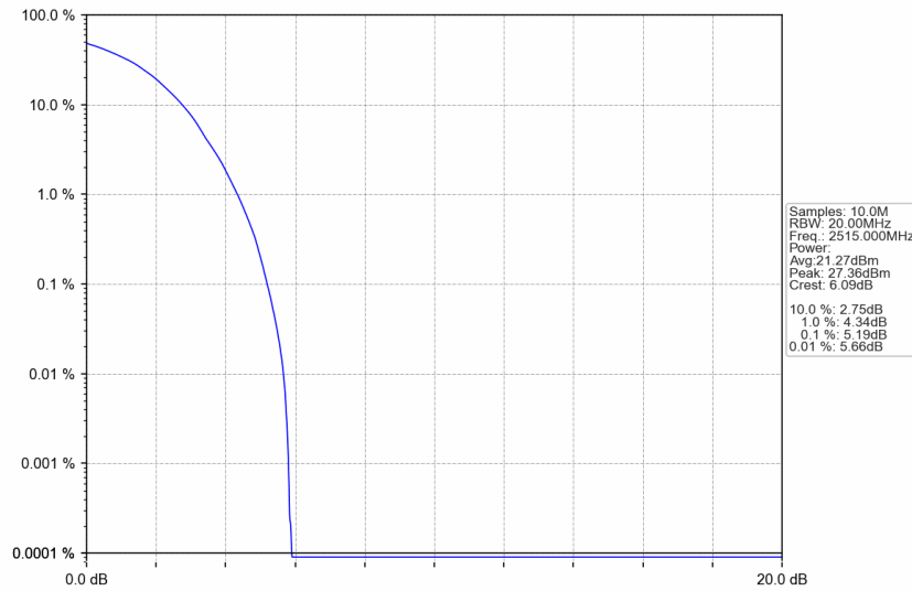
n7_30kHz_SISO_NTNV_30MHz_DFT-s-OFDM QPSK_2515MHz_Outer_Full
