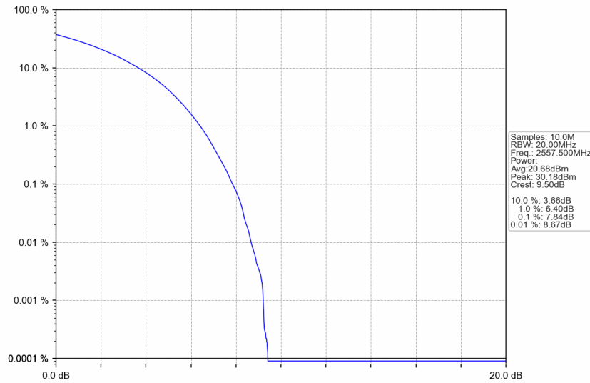
n7_30kHz_SISO_NTNV_25MHz_CP-OFDM QPSK_2557.5MHz_Outer_Full
