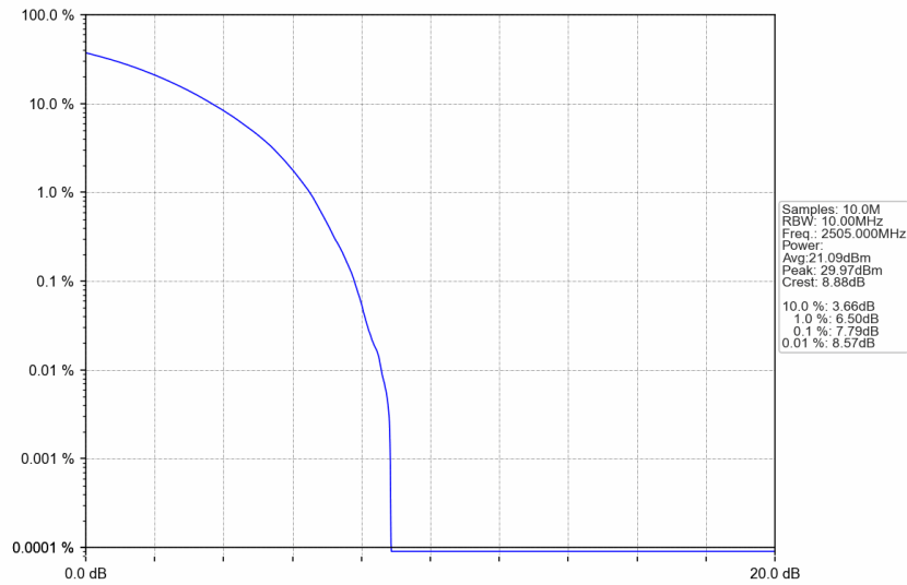
n7_30kHz_SISO_NTNV_10MHz_CP-OFDM 64 QAM_2505MHz_Outer_Full
