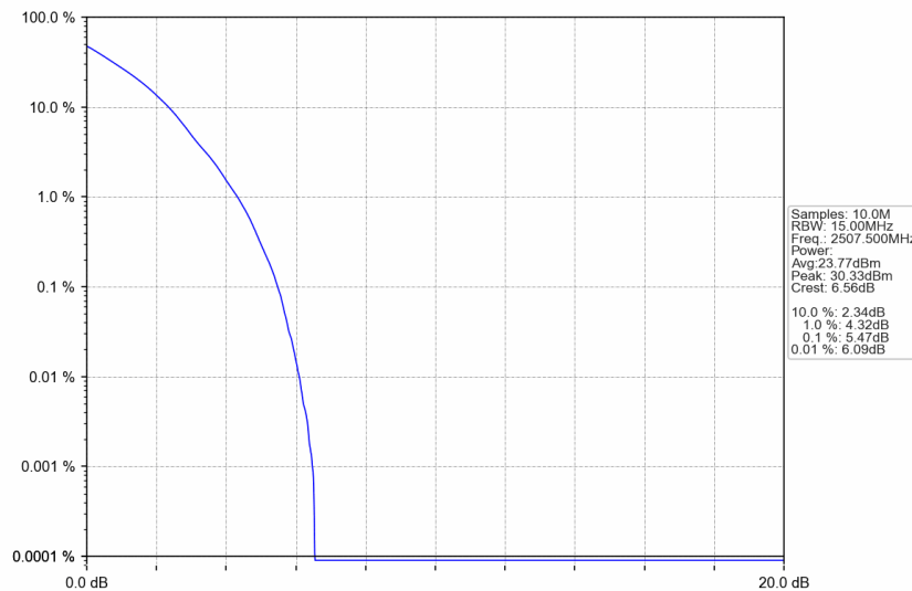
n7_30kHz_SISO_NTNV_15MHz_DFT-s-OFDM QPSK_2507.5MHz_Outer_Full
