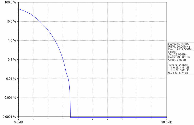
n7_30kHz_SISO_NTNV_25MHz_DFT-s-OFDM 16 QAM_2512.5MHz_Outer_Full
