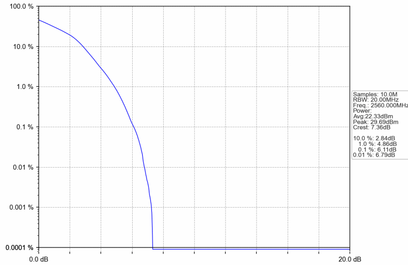
n7_30kHz_SISO_NTNV_20MHz_DFT-s-OFDM 16 QAM_2560MHz_Outer_Full
