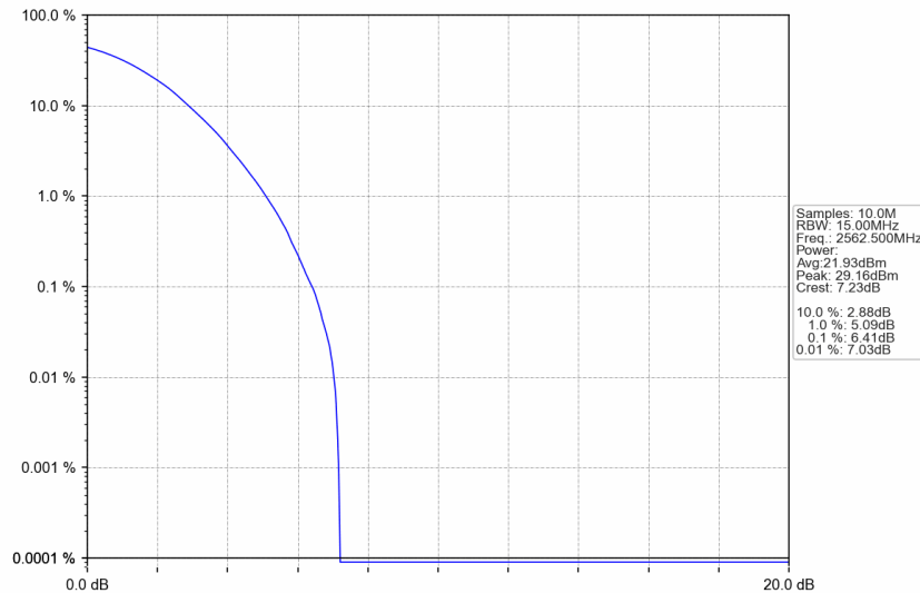
n7_30kHz_SISO_NTNV_15MHz_DFT-s-OFDM 64 QAM_2562.5MHz_Outer_Full
