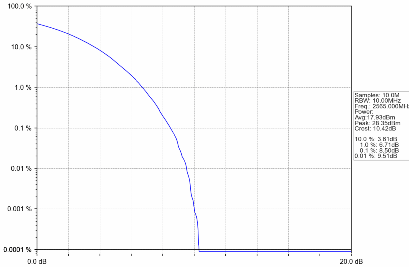
n7_30kHz_SISO_NTNV_10MHz_CP-OFDM 256 QAM_2565MHz_Outer_Full
