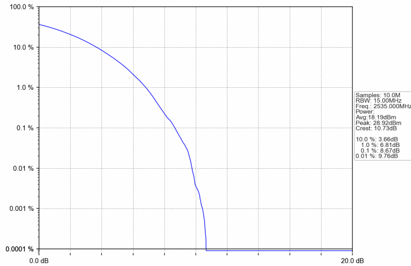
n7_30kHz_SISO_NTNV_15MHz_CP-OFDM 256 QAM_2535MHz_Outer_Full
