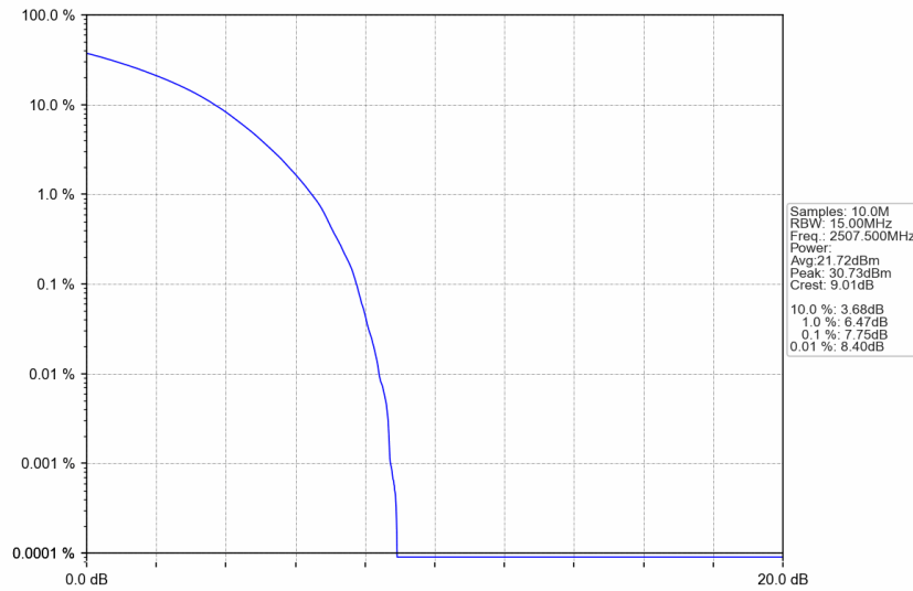
n7_30kHz_SISO_NTNV_15MHz_CP-OFDM QPSK_2507.5MHz_Outer_Full
