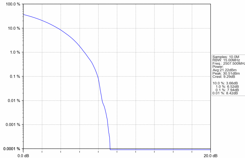
n7_30kHz_SISO_NTNV_15MHz_CP-OFDM 64 QAM_2507.5MHz_Outer_Full
