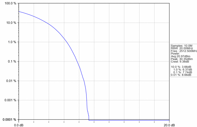
n7_30kHz_SISO_NTNV_25MHz_CP-OFDM QPSK_2512.5MHz_Outer_Full
