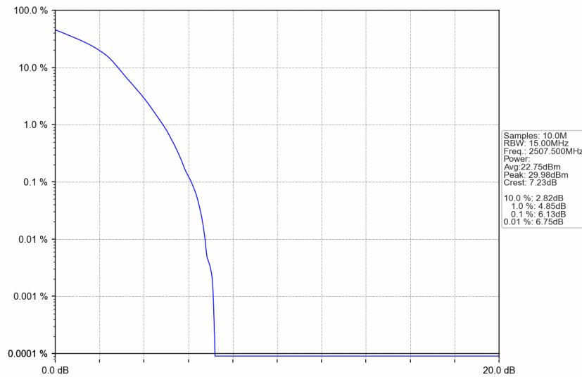
n7_30kHz_SISO_NTNV_15MHz_DFT-s-OFDM 16 QAM_2507.5MHz_Outer_Full
