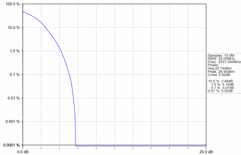
n7_30kHz_SISO_NTNV_25MHz_DFT-s-OFDM QPSK_2557.5MHz_Outer_Full
