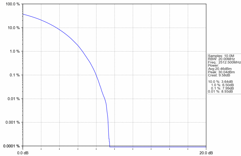
n7_30kHz_SISO_NTNV_25MHz_CP-OFDM 64 QAM_2512.5MHz_Outer_Full
