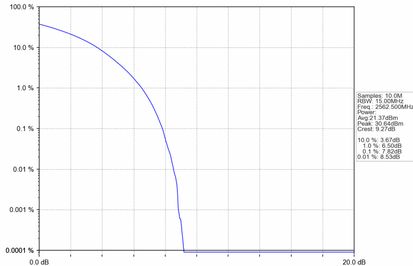
n7_30kHz_SISO_NTNV_15MHz_CP-OFDM QPSK_2562.5MHz_Outer_Full
