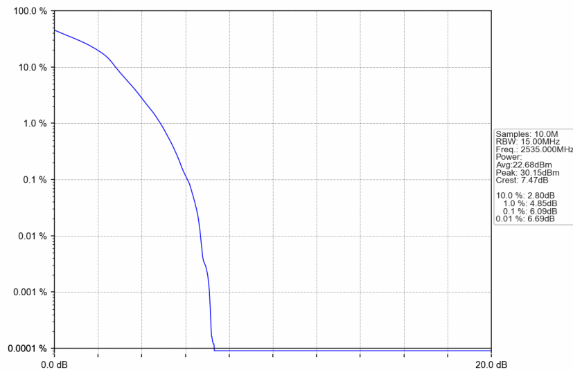
n7_30kHz_SISO_NTNV_15MHz_DFT-s-OFDM 16 QAM_2535MHz_Outer_Full
