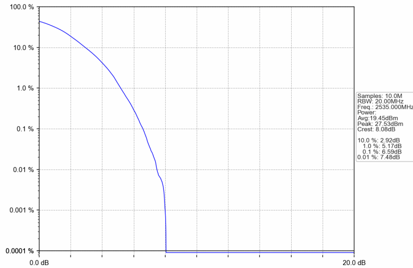
n7_30kHz_SISO_NTNV_25MHz_DFT-s-OFDM 256 QAM_2535MHz_Outer_Full
