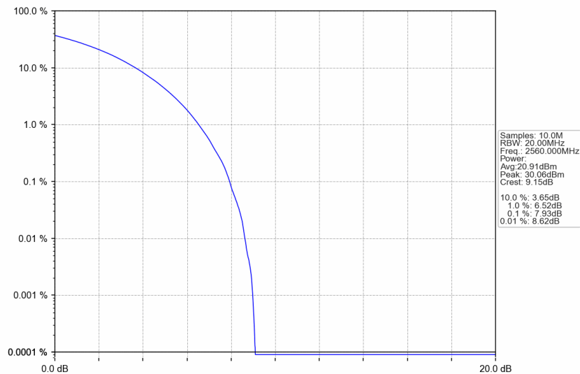
n7_30kHz_SISO_NTNV_20MHz_CP-OFDM 64 QAM_2560MHz_Outer_Full
