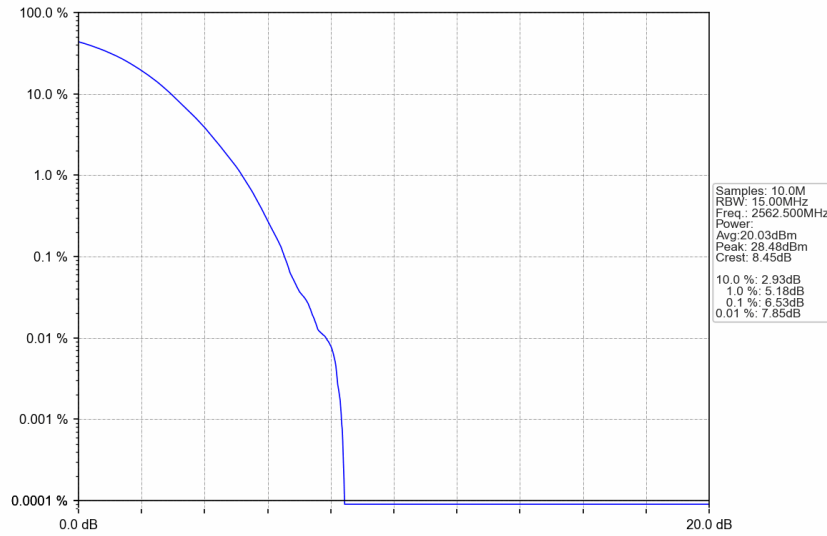
n7_30kHz_SISO_NTNV_15MHz_DFT-s-OFDM 256 QAM_2562.5MHz_Outer_Full
