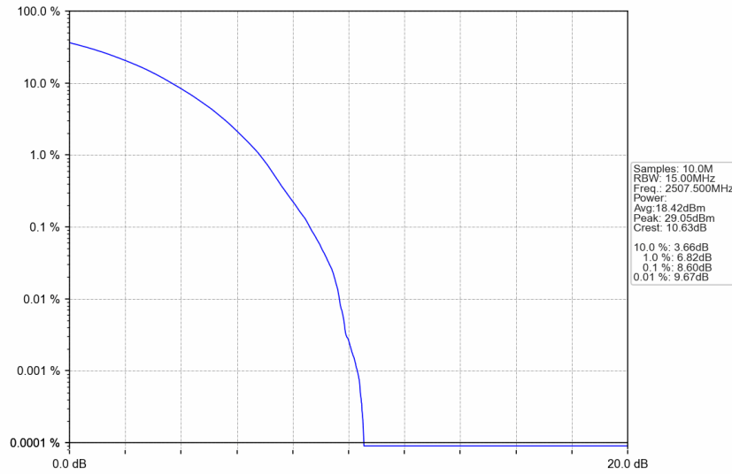
n7_30kHz_SISO_NTNV_15MHz_CP-OFDM 256 QAM_2507.5MHz_Outer_Full
