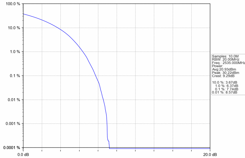
n7_30kHz_SISO_NTNV_25MHz_CP-OFDM QPSK_2535MHz_Outer_Full
