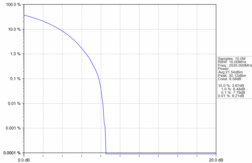
n7_30kHz_SISO_NTNV_10MHz_CP-OFDM QPSK_2535MHz_Outer_Full
