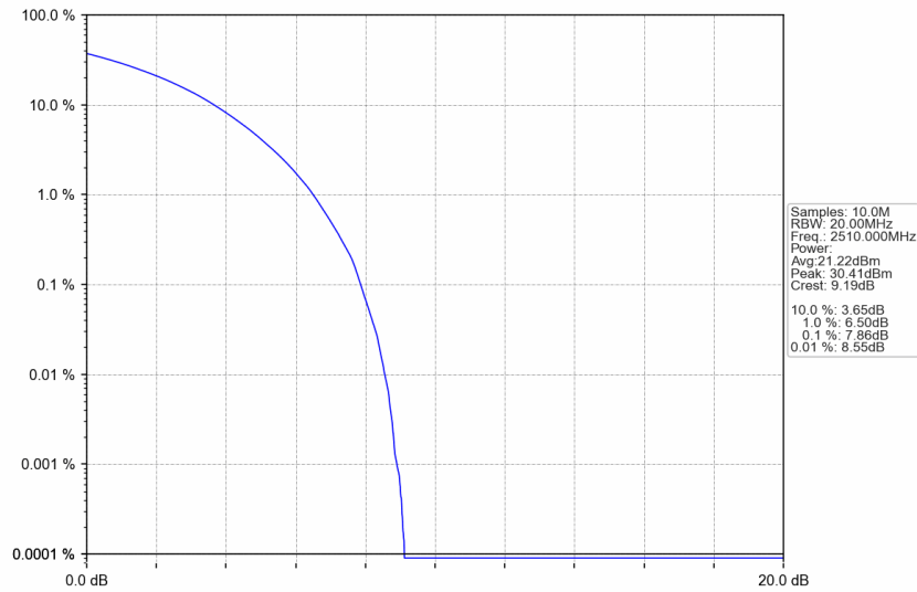
n7_30kHz_SISO_NTNV_20MHz_CP-OFDM 64 QAM_2510MHz_Outer_Full
