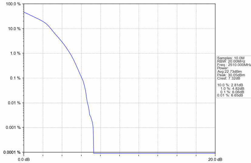
n7_30kHz_SISO_NTNV_20MHz_DFT-s-OFDM_16_QAM_2510MHz_Outer_Full
