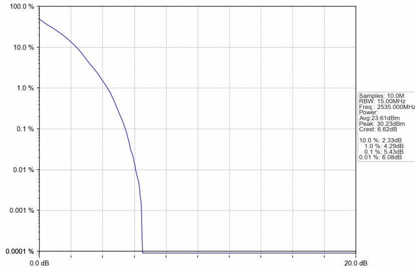
n7_30kHz_SISO_NTNV_15MHz_DFT-s-OFDM QPSK_2535MHz_Outer_Full
