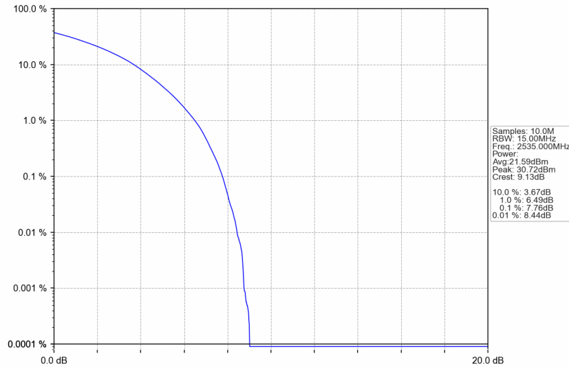
n7_30kHz_SISO_NTNV_15MHz_CP-OFDM QPSK_2535MHz_Outer_Full
