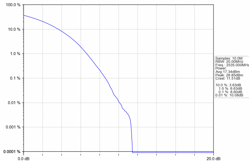
n7_30kHz_SISO_NTNV_25MHz_CP-OFDM 256 QAM_2535MHz_Outer_Full
