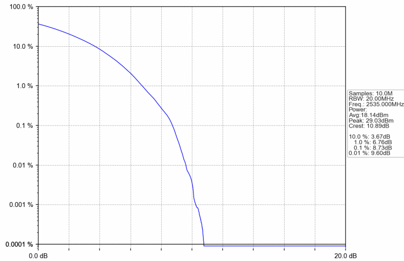
n7_30kHz_SISO_NTNV_20MHz_CP-OFDM 256 QAM_2535MHz_Outer_Full
