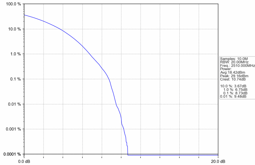
n7_30kHz_SISO_NTNV_20MHz_CP-OFDM 256 QAM_2510MHz_Outer_Full
