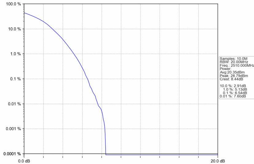
n7_30kHz_SISO_NTNV_20MHz_DFT-s-OFDM 256 QAM_2510MHz_Outer_Full
