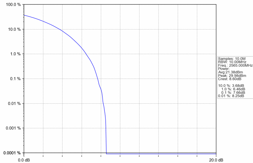
n7_30kHz_SISO_NTNV_10MHz_CP-OFDM 16 QAM_2565MHz_Outer_Full
