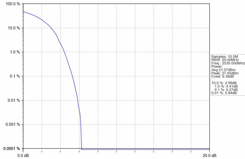
n7_15kHz_SISO_NTNV_30MHz_DFT-s-OFDM QPSK_2535MHz_Outer_Full
