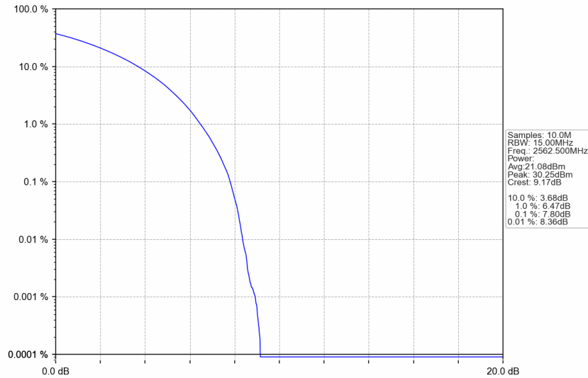
n7_15kHz_SISO_NTNV_15MHz_CP-OFDM 16 QAM_2562.5MHz_Outer_Full
