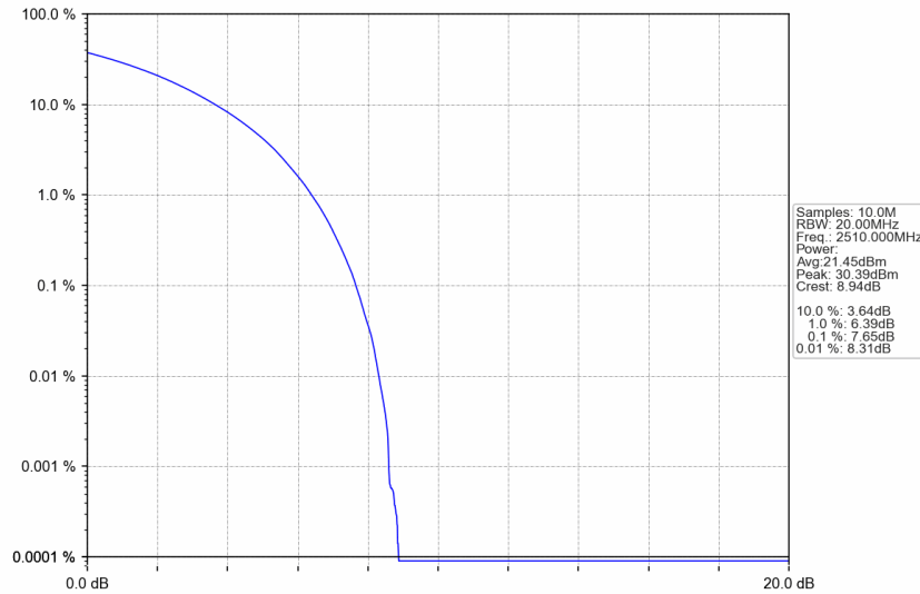
n7_15kHz_SISO_NTNV_20MHz_CP-OFDM 16 QAM_2510MHz_Outer_Full
