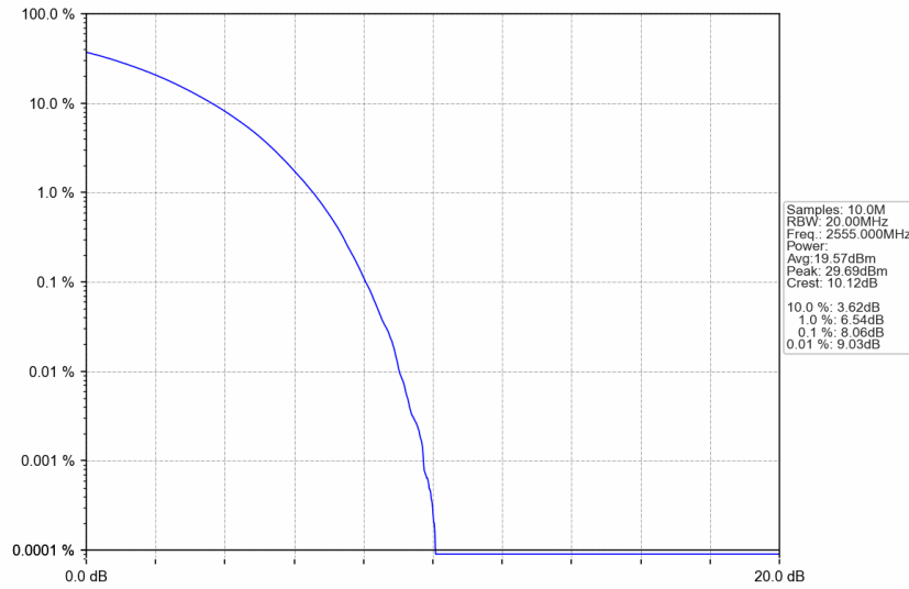
n7_15kHz_SISO_NTNV_30MHz_CP-OFDM 16 QAM_2555MHz_Outer_Full
