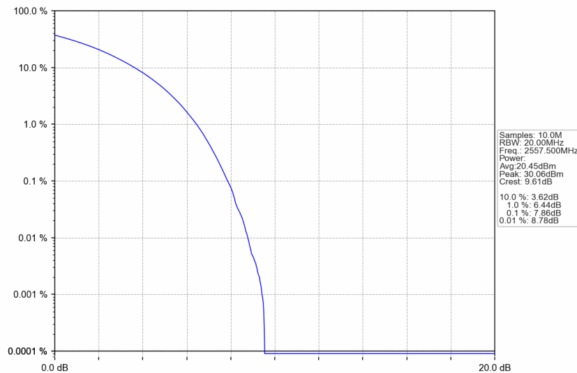
n7_15kHz_SISO_NTNV_25MHz_CP-OFDM QPSK_2557.5MHz_Outer_Full
