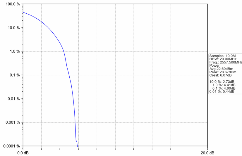
n7_15kHz_SISO_NTNV_25MHz_DFT-s-OFDM QPSK_2557.5MHz_Outer_Full
