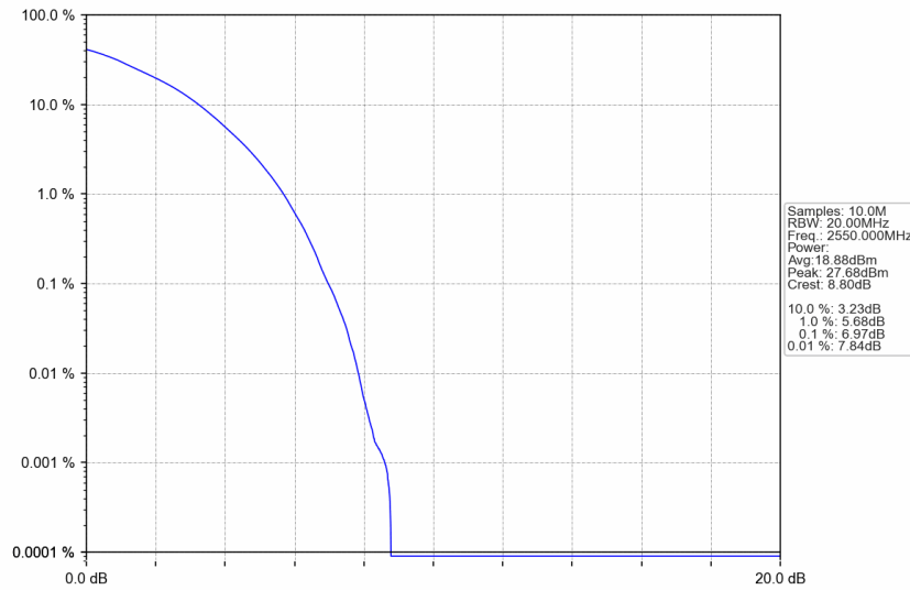
n7_15kHz_SISO_NTNV_40MHz_DFT-s-OFDM 64 QAM_2550MHz_Outer_Full
