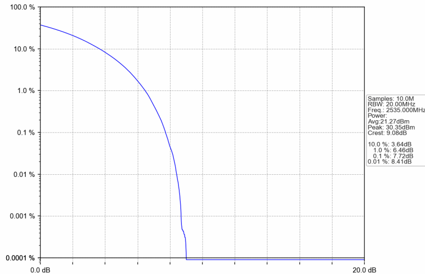
n7_15kHz_SISO_NTNV_20MHz_CP-OFDM 16 QAM_2535MHz_Outer_Full
