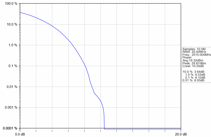
n7_15kHz_SISO_NTNV_30MHz_CP-OFDM 64 QAM_2515MHz_Outer_Full
