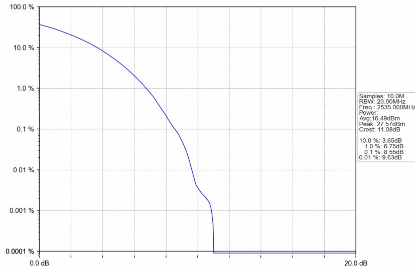
n7_15kHz_SISO_NTNV_30MHz_CP-OFDM 256 QAM_2535MHz_Outer_Full
