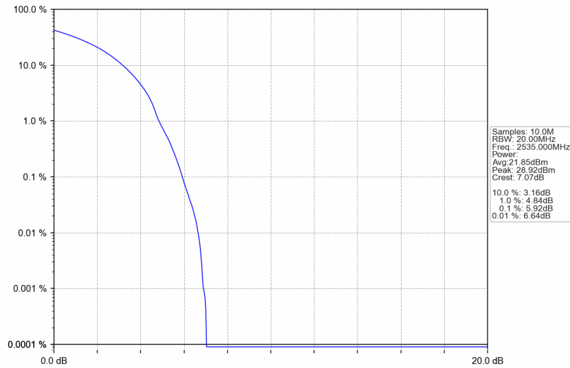
n7_15kHz_SISO_NTNV_25MHz_DFT-s-OFDM 16 QAM_2535MHz_Outer_Full
