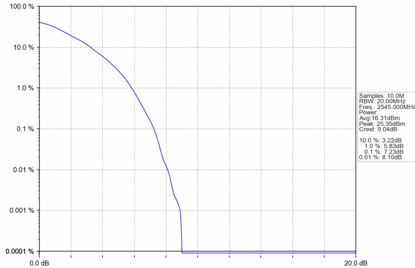
n7_15kHz_SISO_NTNV_50MHz_DFT-s-OFDM 256 QAM_2545MHz_Outer_Full
