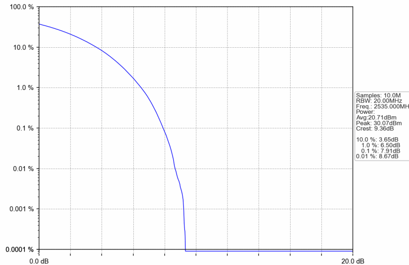
n7_15kHz_SISO_NTNV_25MHz_CP-OFDM 16 QAM_2535MHz_Outer_Full
