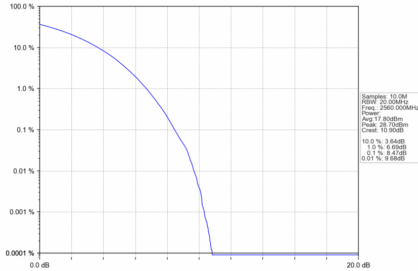
n7_15kHz_SISO_NTNV_20MHz_CP-OFDM 256 QAM_2560MHz_Outer_Full
