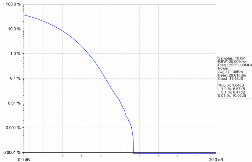
n7_15kHz_SISO_NTNV_25MHz_CP-OFDM 256 QAM_2535MHz_Outer_Full
