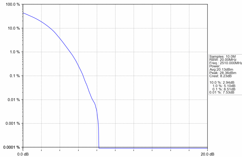
n7_15kHz_SISO_NTNV_20MHz_DFT-s-OFDM 256 QAM_2510MHz_Outer_Full
