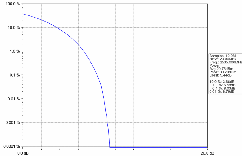
n7_15kHz_SISO_NTNV_20MHz_CP-OFDM 64 QAM_2535MHz_Outer_Full
