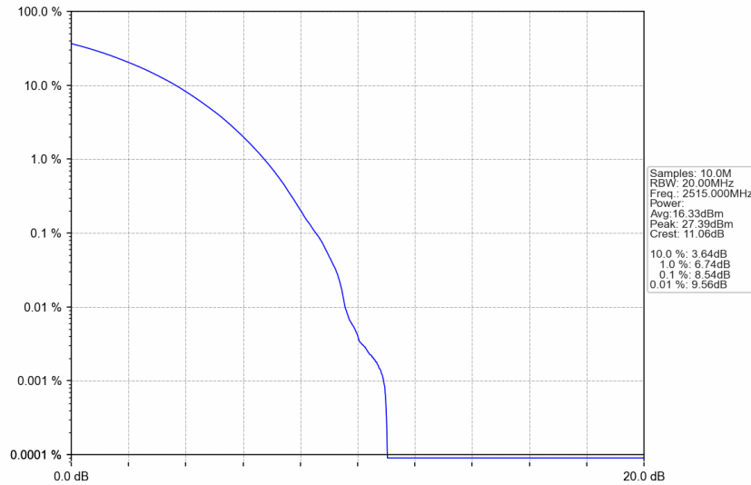
n7_15kHz_SISO_NTNV_30MHz_CP-OFDM 256 QAM_2515MHz_Outer_Full
