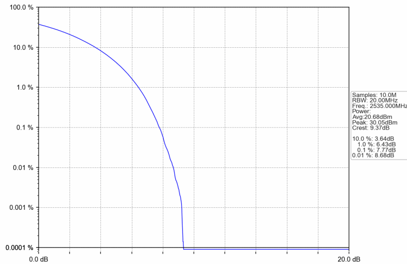
n7_15kHz_SISO_NTNV_25MHz_CP-OFDM QPSK_2535MHz_Outer_Full
