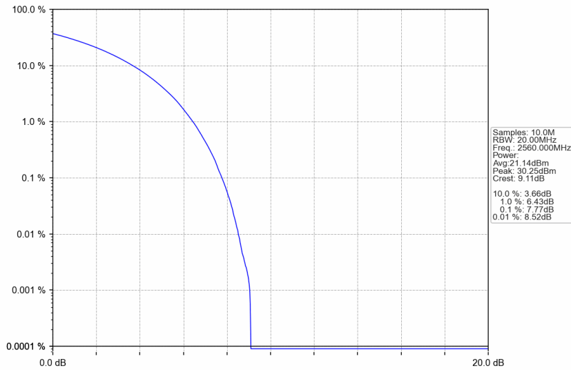
n7_15kHz_SISO_NTNV_20MHz_CP-OFDM QPSK_2560MHz_Outer_Full
