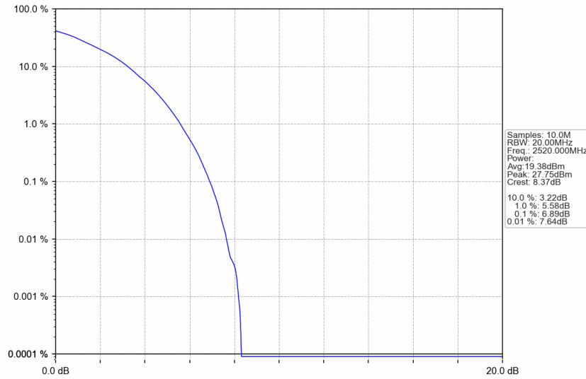
n7_15kHz_SISO_NTNV_40MHz_DFT-s-OFDM 16 QAM_2520MHz_Outer_Full
