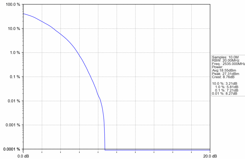
n7_15kHz_SISO_NTNV_50MHz_DFT-s-OFDM 64 QAM_2535MHz_Outer_Full
