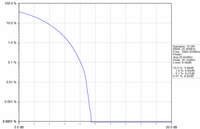
n7_15kHz_SISO_NTNV_20MHz_CP-OFDM 64 QAM_2560MHz_Outer_Full
