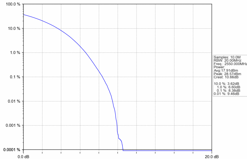
n7_15kHz_SISO_NTNV_40MHz_CP-OFDM 64 QAM_2550MHz_Outer_Full
