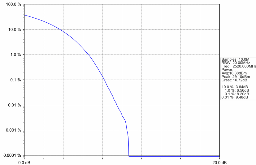
n7_15kHz_SISO_NTNV_40MHz_CP-OFDM QPSK_2520MHz_Outer_Full
