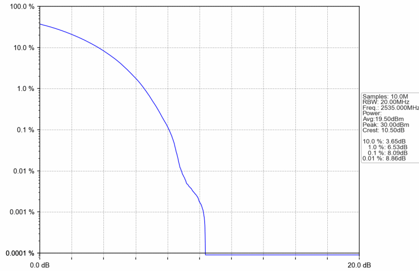
n7_15kHz_SISO_NTNV_30MHz_CP-OFDM 64 QAM_2535MHz_Outer_Full
