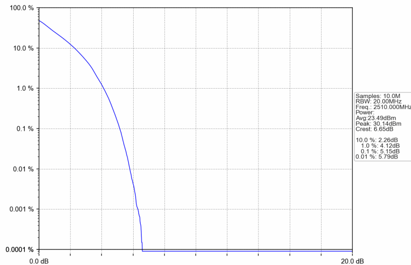
n7_15kHz_SISO_NTNV_20MHz_DFT-s-OFDM QPSK_2510MHz_Outer_Full
