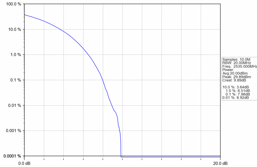
n7_15kHz_SISO_NTNV_30MHz_CP-OFDM QPSK_2535MHz_Outer_Full
