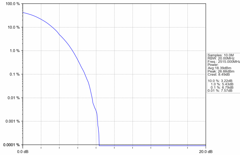
n7_15kHz_SISO_NTNV_30MHz_DFT-s-OFDM 256 QAM_2515MHz_Outer_Full
