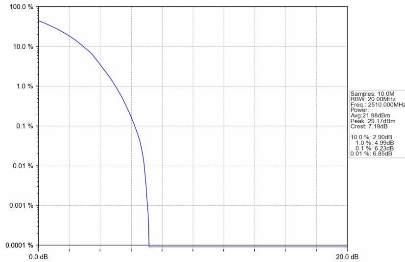
n7_15kHz_SISO_NTNV_20MHz_DFT-s-OFDM 64 QAM_2510MHz_Outer_Full
