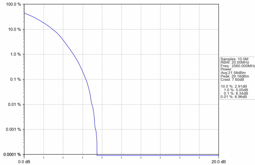
n7_15kHz_SISO_NTNV_20MHz_DFT-s-OFDM 64 QAM_2560MHz_Outer_Full
