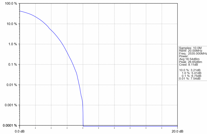
n7_15kHz_SISO_NTNV_30MHz_DFT-s-OFDM 256 QAM_2535MHz_Outer_Full
