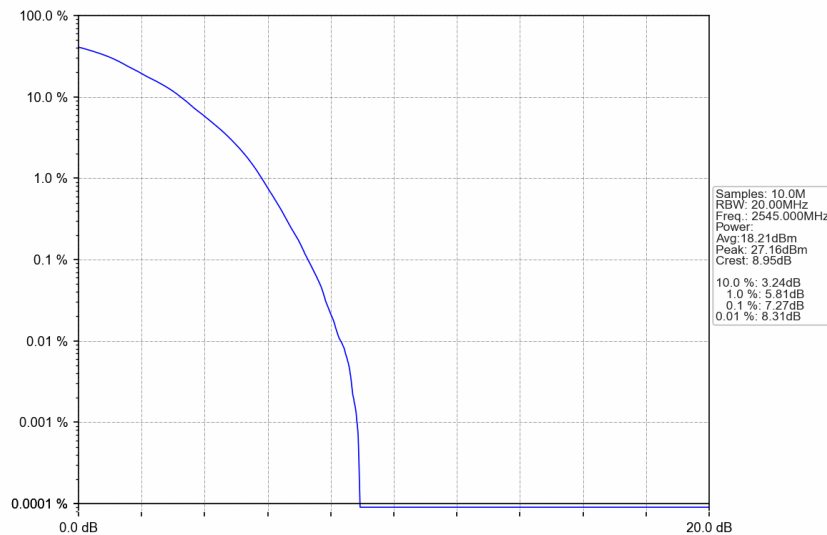
n7_15kHz_SISO_NTNV_50MHz_DFT-s-OFDM 64 QAM_2545MHz_Outer_Full
