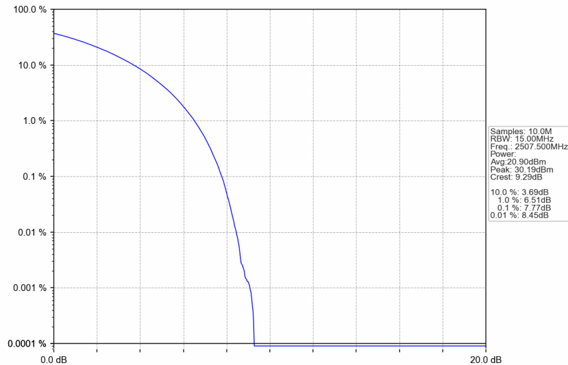
n7_15kHz_SISO_NTNV_15MHz_CP-OFDM 64 QAM_2507.5MHz_Outer_Full
