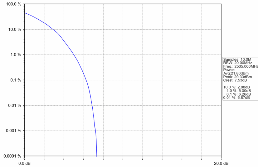
n7_15kHz_SISO_NTNV_20MHz_DFT-s-OFDM 64 QAM_2535MHz_Outer_Full
