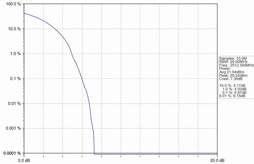
n7_15kHz_SISO_NTNV_25MHz_DFT-s-OFDM 16 QAM_2512.5MHz_Outer_Full
