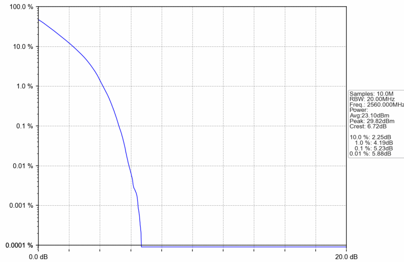
n7_15kHz_SISO_NTNV_20MHz_DFT-s-OFDM QPSK_2560MHz_Outer_Full
