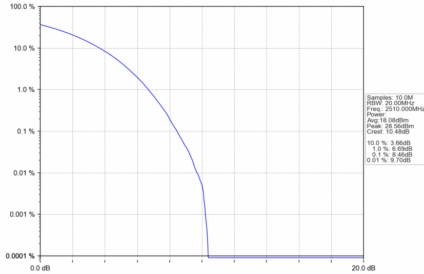
n7_15kHz_SISO_NTNV_20MHz_CP-OFDM 256 QAM_2510MHz_Outer_Full
