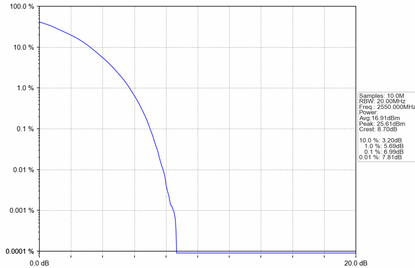
n7_15kHz_SISO_NTNV_40MHz_DFT-s-OFDM 256 QAM_2550MHz_Outer_Full
