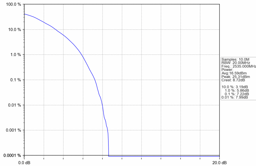
n7_15kHz_SISO_NTNV_50MHz_DFT-s-OFDM 256 QAM_2535MHz_Outer_Full
