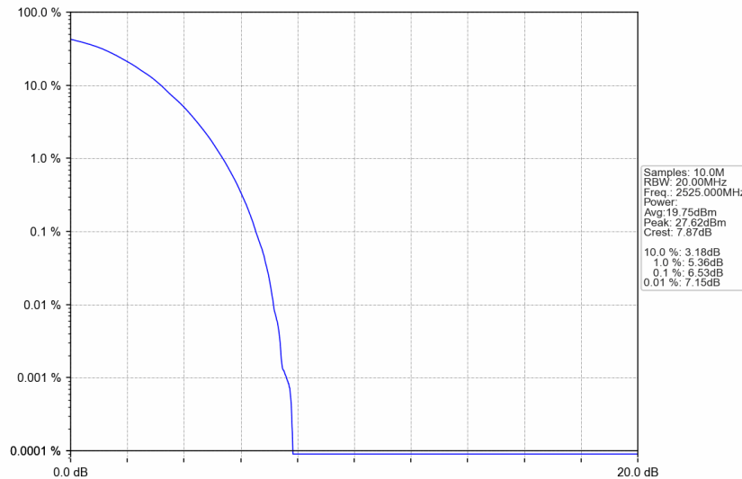
n7_15kHz_SISO_NTNV_50MHz_DFT-s-OFDM QPSK_2525MHz_Outer_Full
