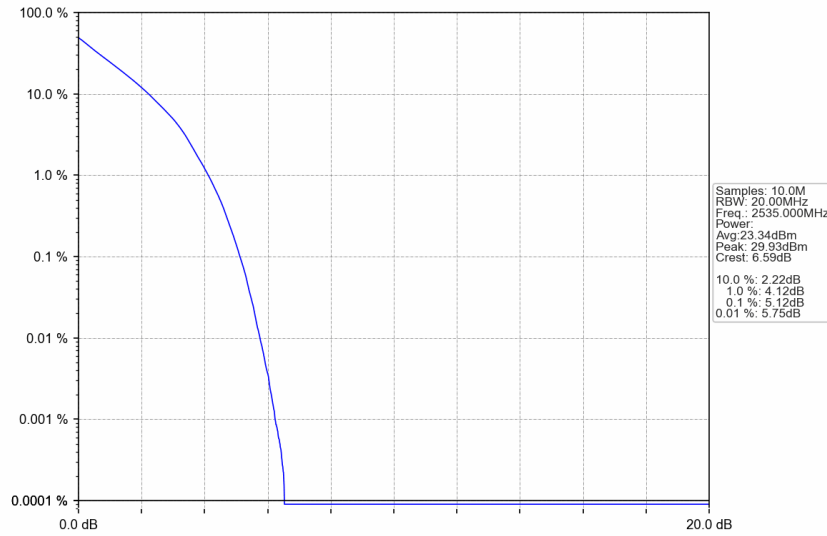
n7_15kHz_SISO_NTNV_20MHz_DFT-s-OFDM QPSK_2535MHz_Outer_Full
