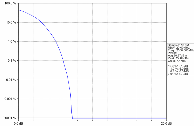
n7_15kHz_SISO_NTNV_40MHz_DFT-s-OFDM QPSK_2550MHz_Outer_Full
