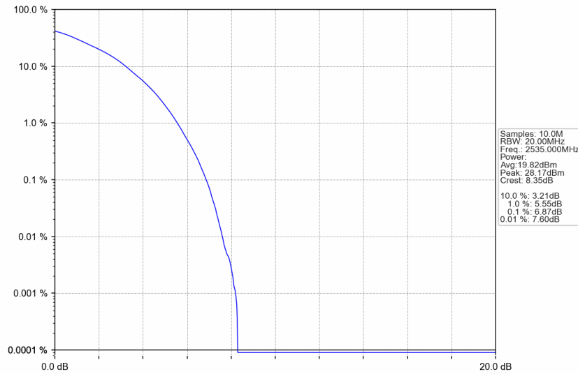
n7_15kHz_SISO_NTNV_40MHz_DFT-s-OFDM 16 QAM_2535MHz_Outer_Full
