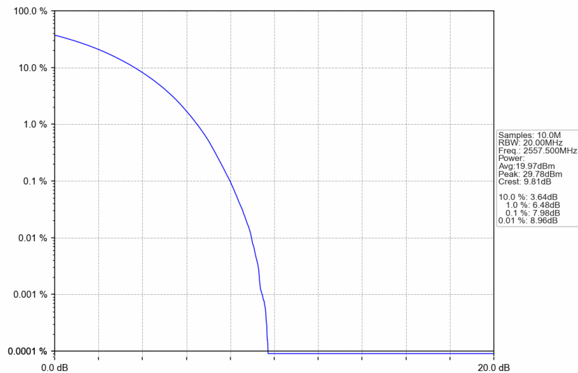
n7_15kHz_SISO_NTNV_25MHz_CP-OFDM 64 QAM_2557.5MHz_Outer_Full
