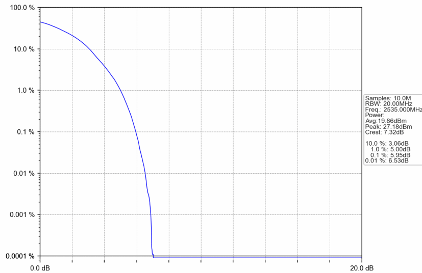
n7_15kHz_SISO_NTNV_40MHz_DFT-s-OFDM QPSK_2535MHz_Outer_Full
