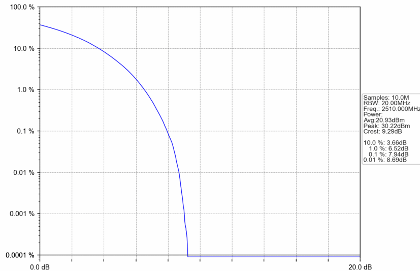
n7_15kHz_SISO_NTNV_20MHz_CP-OFDM 64 QAM_2510MHz_Outer_Full
