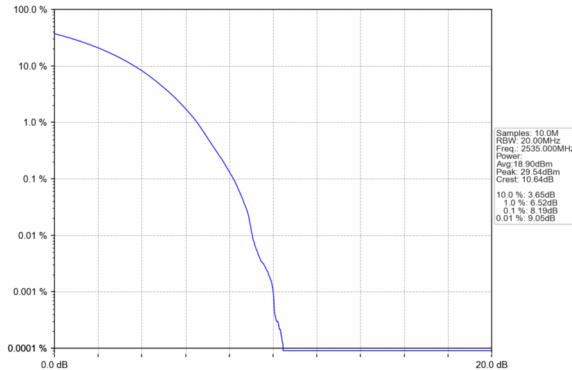
n7_15kHz_SISO_NTNV_40MHz_CP-OFDM 16 QAM_2535MHz_Outer_Full
