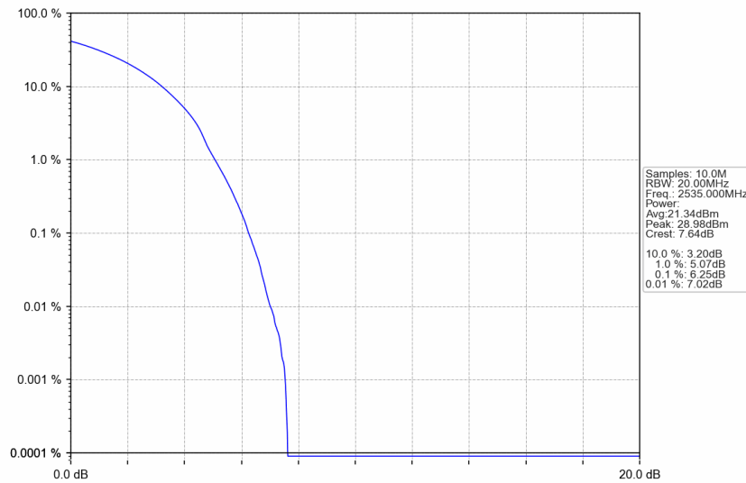
n7_15kHz_SISO_NTNV_25MHz_DFT-s-OFDM 64 QAM_2535MHz_Outer_Full
