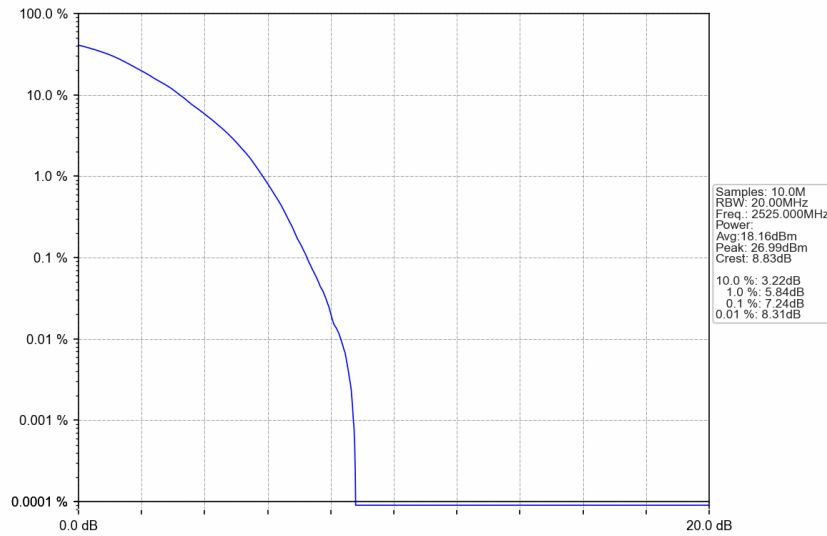
n7_15kHz_SISO_NTNV_50MHz_DFT-s-OFDM 64 QAM_2525MHz_Outer_Full
