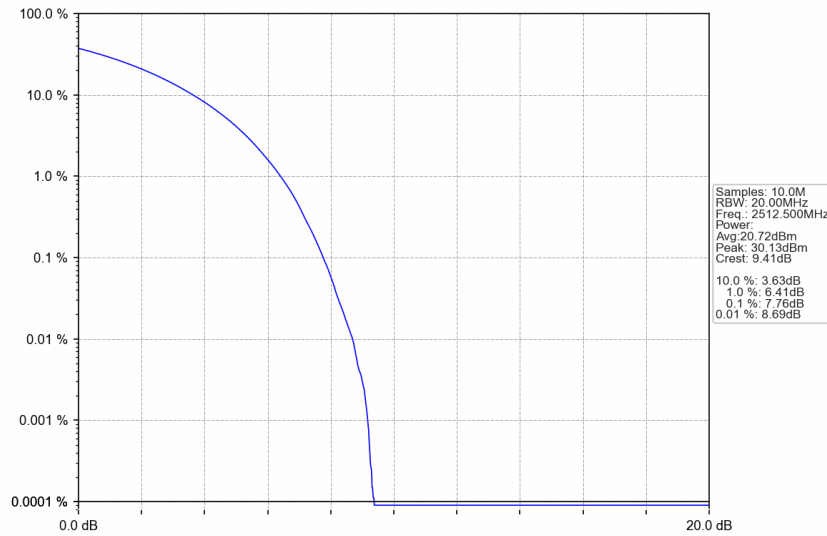
n7_15kHz_SISO_NTNV_25MHz_CP-OFDM QPSK_2512.5MHz_Outer_Full
