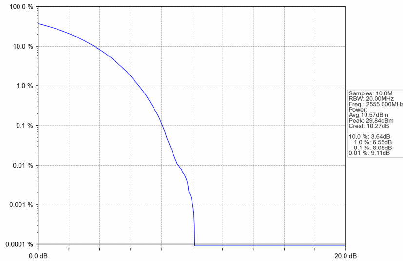
n7_15kHz_SISO_NTNV_30MHz_CP-OFDM QPSK_2555MHz_Outer_Full
