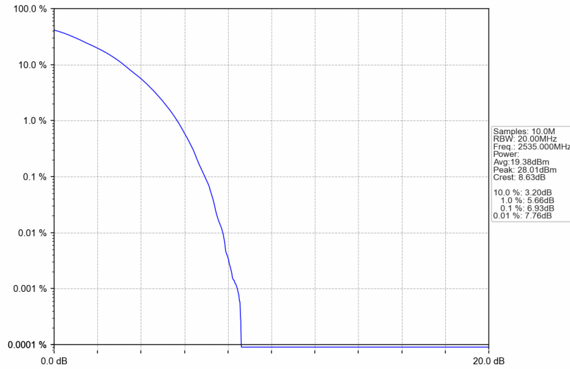
n7_15kHz_SISO_NTNV_40MHz_DFT-s-OFDM 64 QAM_2535MHz_Outer_Full
