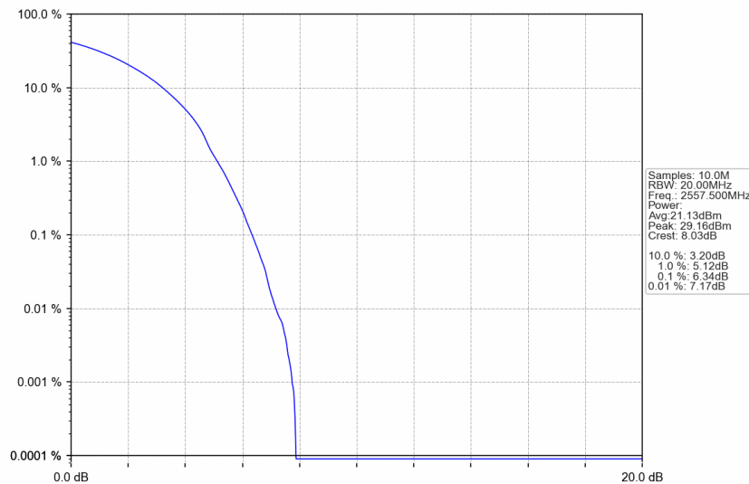
n7_15kHz_SISO_NTNV_25MHz_DFT-s-OFDM 64 QAM_2557.5MHz_Outer_Full
