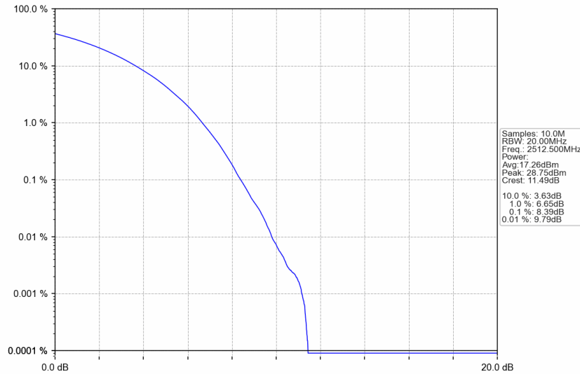
n7_15kHz_SISO_NTNV_25MHz_CP-OFDM 256 QAM_2512.5MHz_Outer_Full
