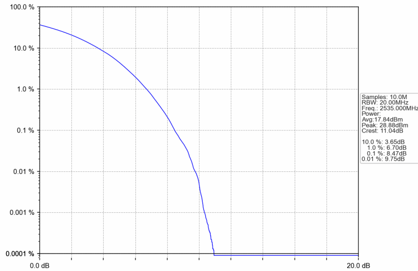
n7_15kHz_SISO_NTNV_20MHz_CP-OFDM 256 QAM_2535MHz_Outer_Full
