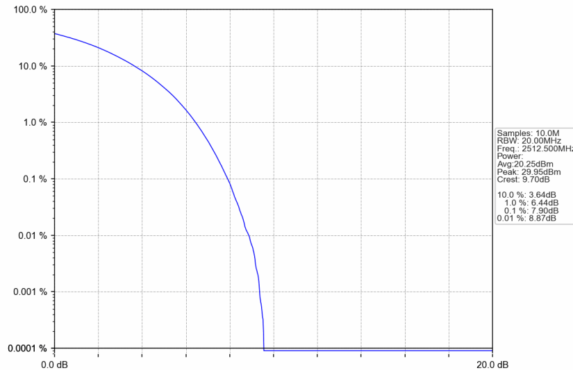
n7_15kHz_SISO_NTNV_25MHz_CP-OFDM 64 QAM_2512.5MHz_Outer_Full
