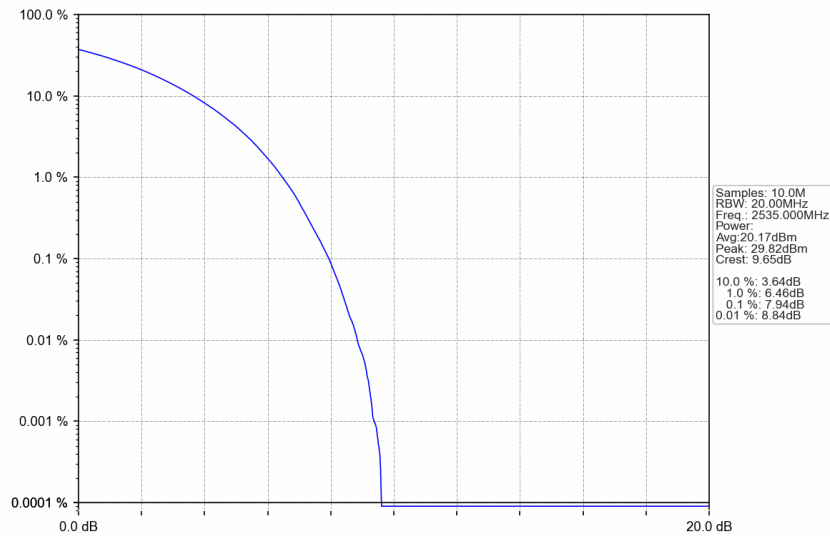
n7_15kHz_SISO_NTNV_25MHz_CP-OFDM 64 QAM_2535MHz_Outer_Full
