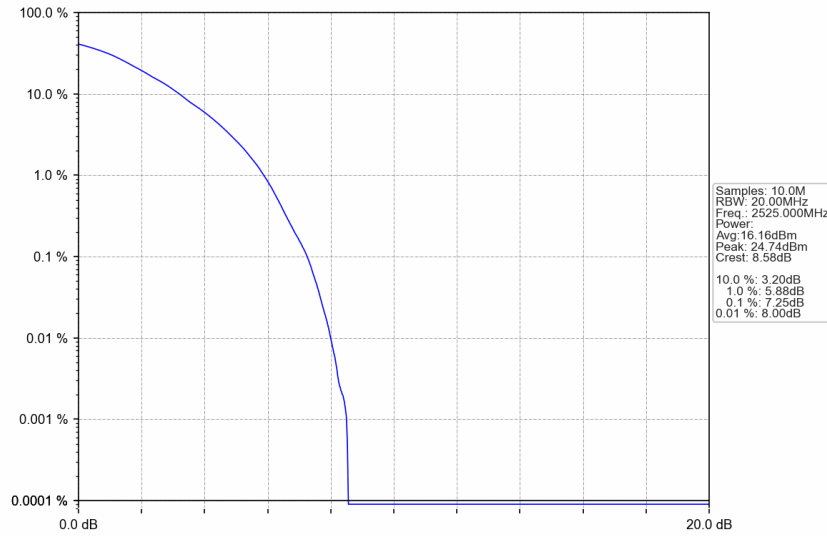
n7_15kHz_SISO_NTNV_50MHz_DFT-s-OFDM 256 QAM_2525MHz_Outer_Full
