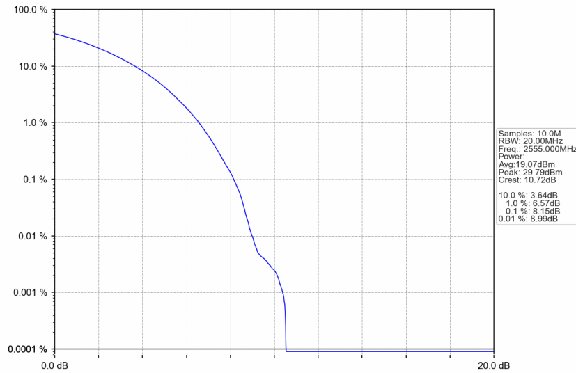
n7_15kHz_SISO_NTNV_30MHz_CP-OFDM 64 QAM_2555MHz_Outer_Full
