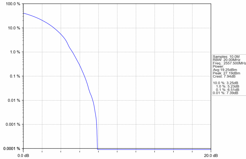
n7_15kHz_SISO_NTNV_25MHz_DFT-s-OFDM 256 QAM_2557.5MHz_Outer_Full
