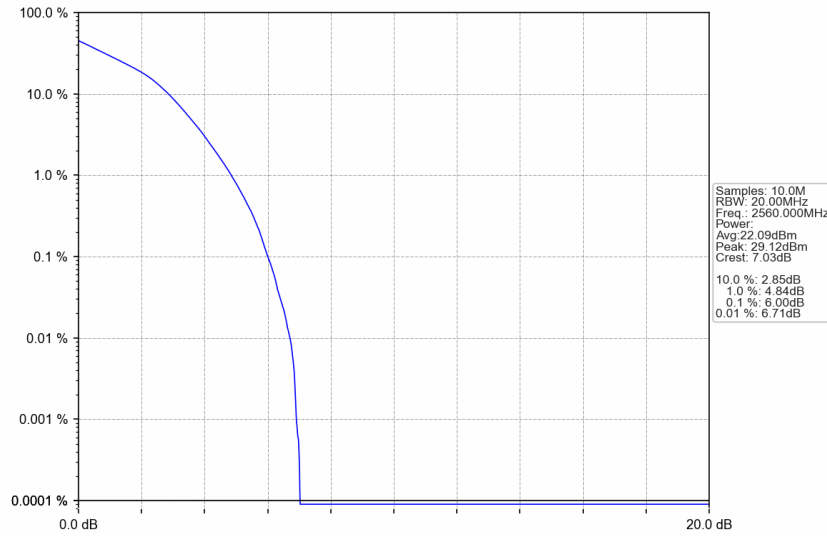
n7_15kHz_SISO_NTNV_20MHz_DFT-s-OFDM 16 QAM_2560MHz_Outer_Full
