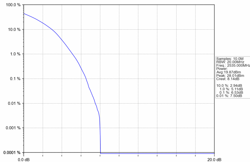
n7_15kHz_SISO_NTNV_20MHz_DFT-s-OFDM 256 QAM_2535MHz_Outer_Full
