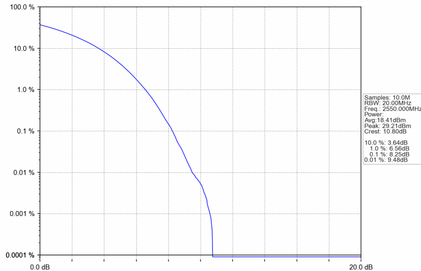
n7_15kHz_SISO_NTNV_40MHz_CP-OFDM QPSK_2550MHz_Outer_Full
