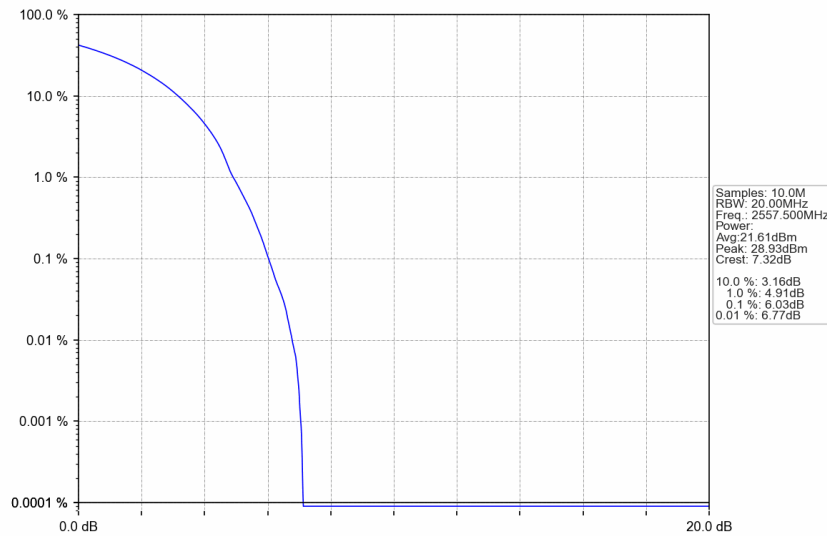
n7_15kHz_SISO_NTNV_25MHz_DFT-s-OFDM 16 QAM_2557.5MHz_Outer_Full
