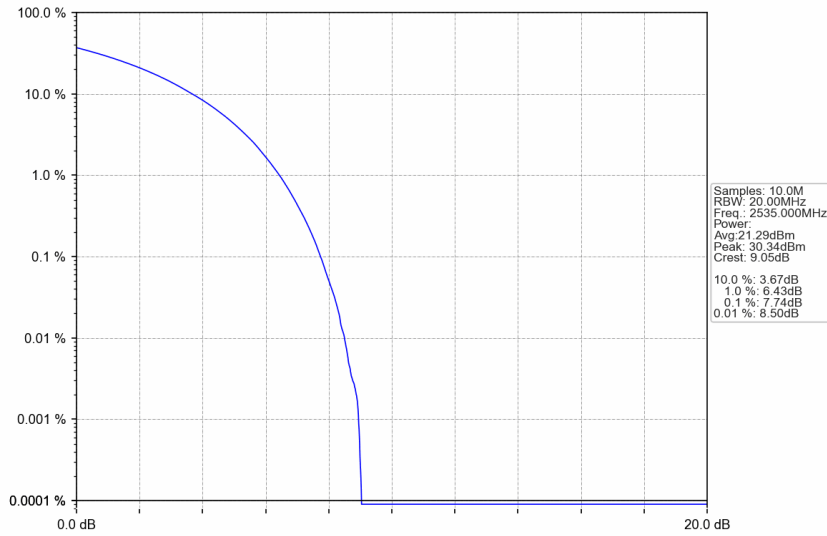
n7_15kHz_SISO_NTNV_20MHz_CP-OFDM QPSK_2535MHz_Outer_Full
