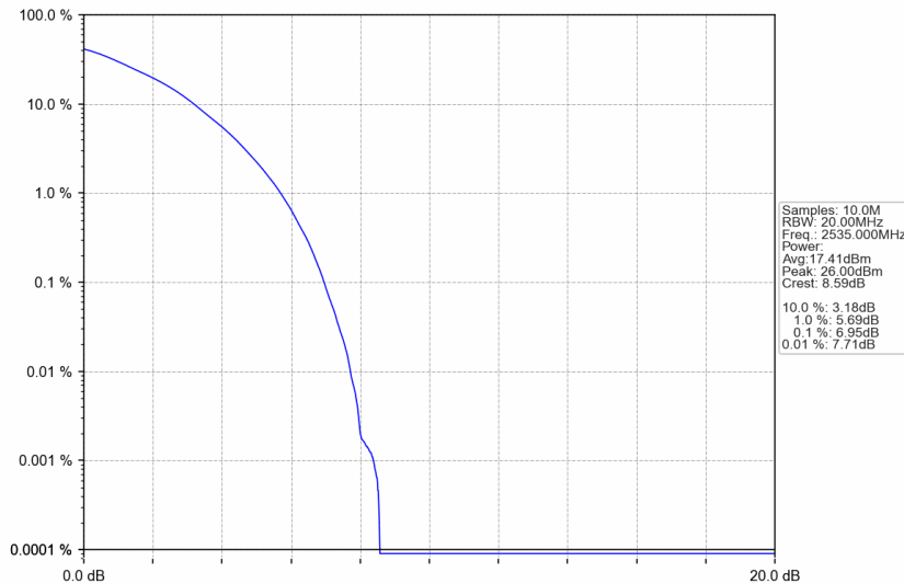
n7_15kHz_SISO_NTNV_40MHz_DFT-s-OFDM 256 QAM_2535MHz_Outer_Full
