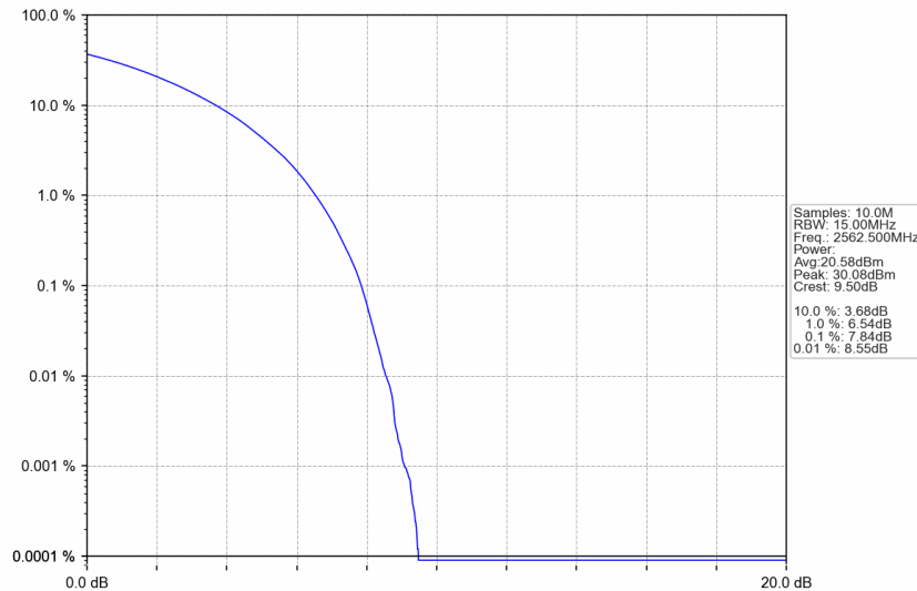
n7_15kHz_SISO_NTNV_15MHz_CP-OFDM 64 QAM_2562.5MHz_Outer_Full
