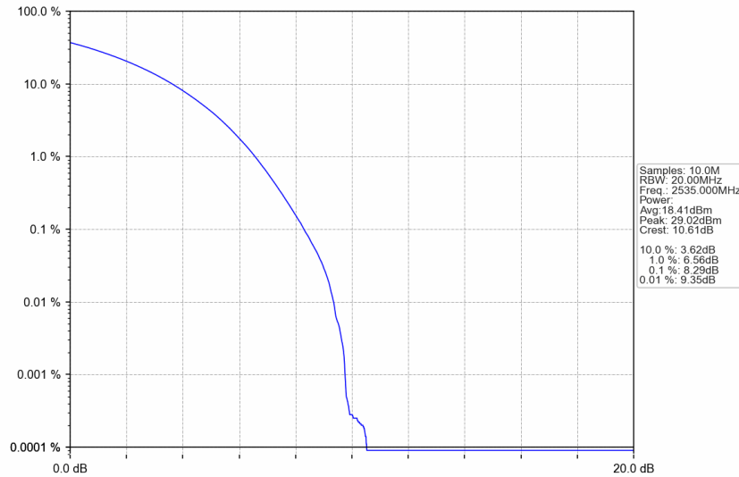
n7_15kHz_SISO_NTNV_40MHz_CP-OFDM 64 QAM_2535MHz_Outer_Full
