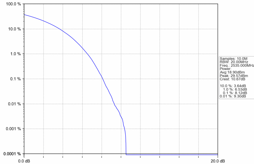
n7_15kHz_SISO_NTNV_40MHz_CP-OFDM QPSK_2535MHz_Outer_Full
