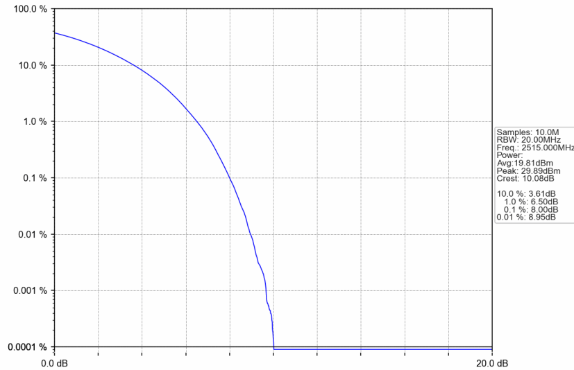
n7_15kHz_SISO_NTNV_30MHz_CP-OFDM 16 QAM_2515MHz_Outer_Full
