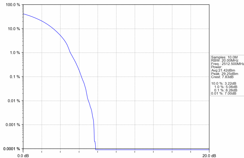
n7_15kHz_SISO_NTNV_25MHz_DFT-s-OFDM 64 QAM_2512.5MHz_Outer_Full
