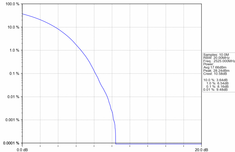
n7_15kHz_SISO_NTNV_50MHz_CP-OFDM QPSK_2525MHz_Outer_Full
