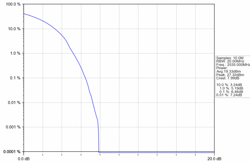
n7_15kHz_SISO_NTNV_25MHz_DFT-s-OFDM 256 QAM_2535MHz_Outer_Full
