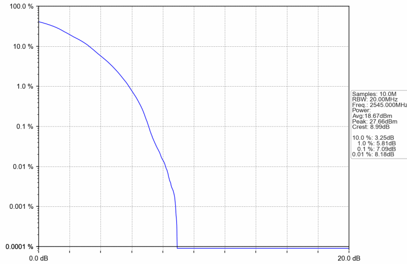
n7_15kHz_SISO_NTNV_50MHz_DFT-s-OFDM 16 QAM_2545MHz_Outer_Full
