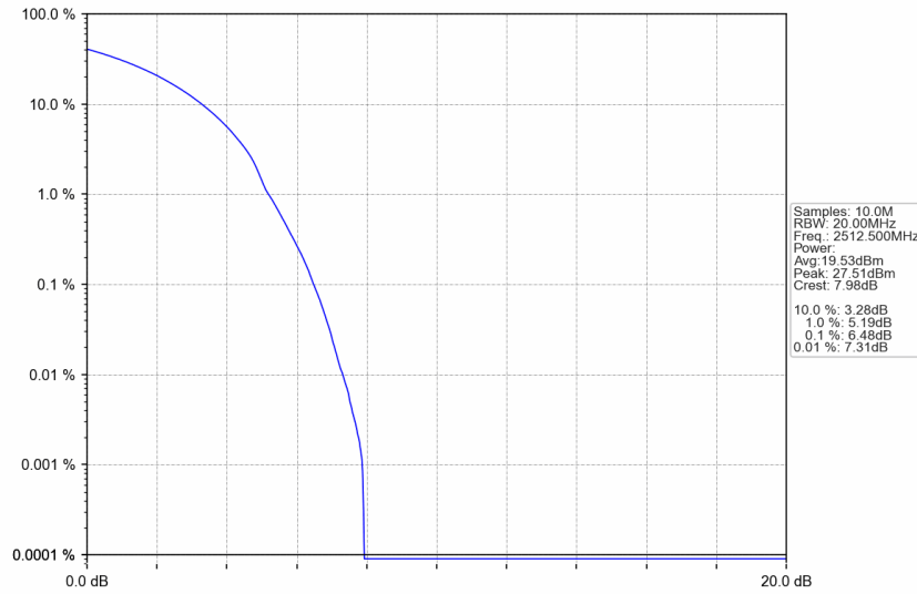
n7_15kHz_SISO_NTNV_25MHz_DFT-s-OFDM 256 QAM_2512.5MHz_Outer_Full
