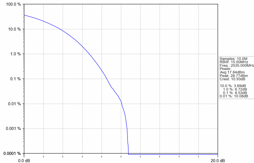
n7_15kHz_SISO_NTNV_15MHz_CP-OFDM 256 QAM_2535MHz_Outer_Full
