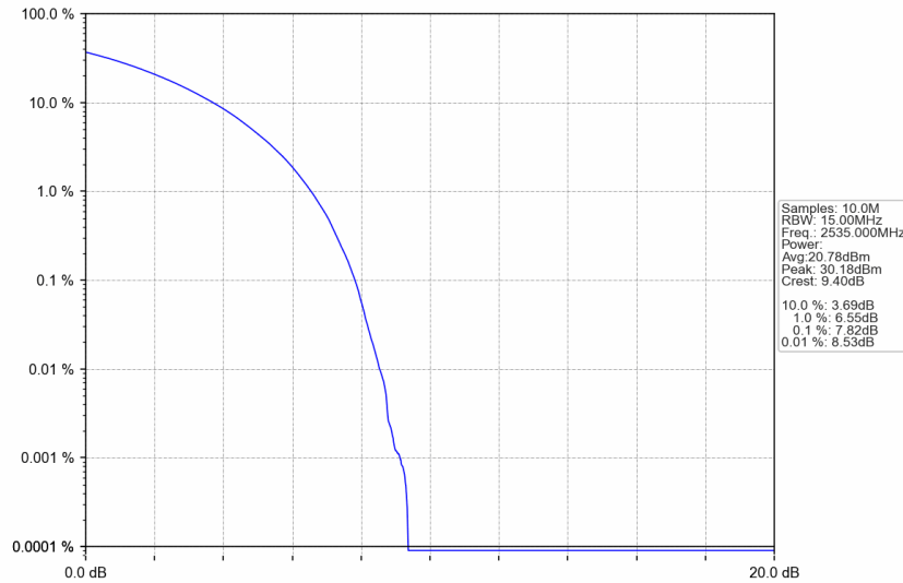
n7_15kHz_SISO_NTNV_15MHz_CP-OFDM 64 QAM_2535MHz_Outer_Full
