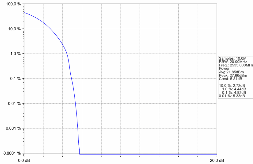
n7_15kHz_SISO_NTNV_25MHz_DFT-s-OFDM QPSK_2535MHz_Outer_Full
