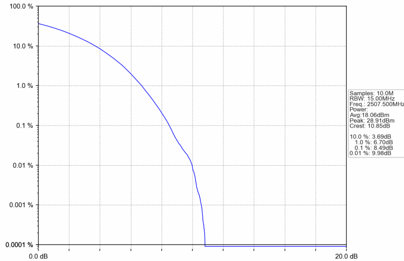
n7_15kHz_SISO_NTNV_15MHz_CP-OFDM 256 QAM_2507.5MHz_Outer_Full
