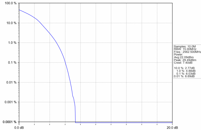
n7_15kHz_SISO_NTNV_15MHz_DFT-s-OFDM 16 QAM_2562.5MHz_Outer_Full
