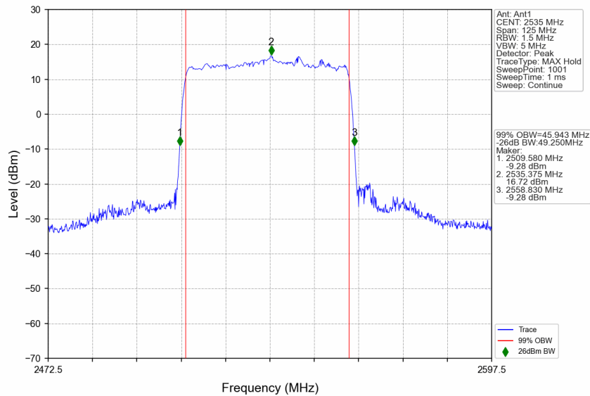
n7_30kHz_SISO_NTNV_50MHz_DFT-s-OFDM 256 QAM_2535MHz_Outer_Full
