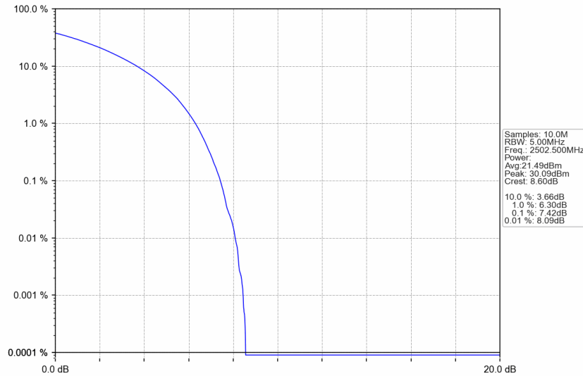
n7_15kHz_SISO_NTNV_5MHz_CP-OFDM 16 QAM_2502.5MHz_Outer_Full
