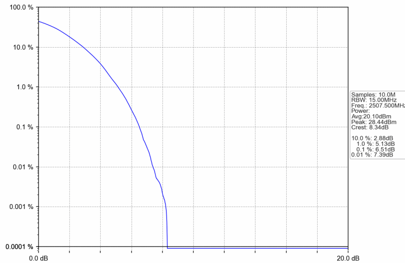
n7_15kHz_SISO_NTNV_15MHz_DFT-s-OFDM 256 QAM_2507.5MHz_Outer_Full
