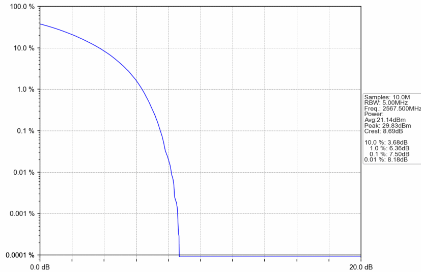
n7_15kHz_SISO_NTNV_5MHz_CP-OFDM 16 QAM_2567.5MHz_Outer_Full
