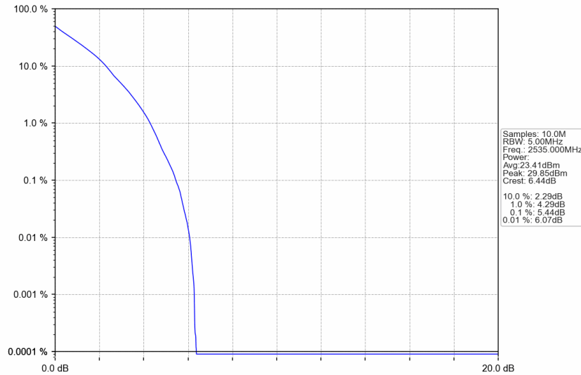
n7_15kHz_SISO_NTNV_5MHz_DFT-s-OFDM QPSK_2535MHz_Outer_Full
