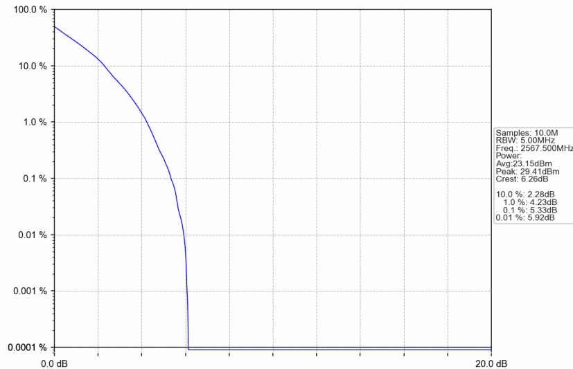
n7_15kHz_SISO_NTNV_5MHz_DFT-s-OFDM QPSK_2567.5MHz_Outer_Full
