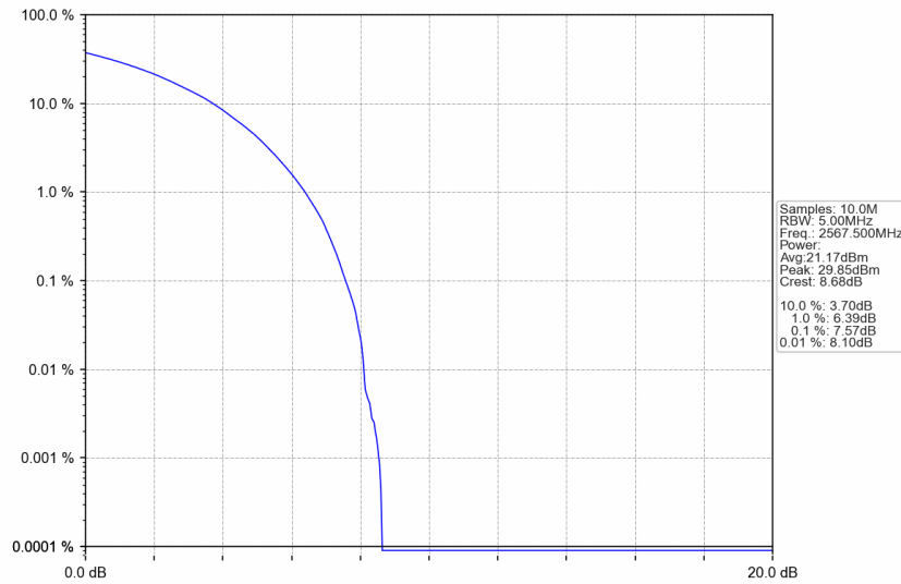
n7_15kHz_SISO_NTNV_5MHz_CP-OFDM QPSK_2567.5MHz_Outer_Full
