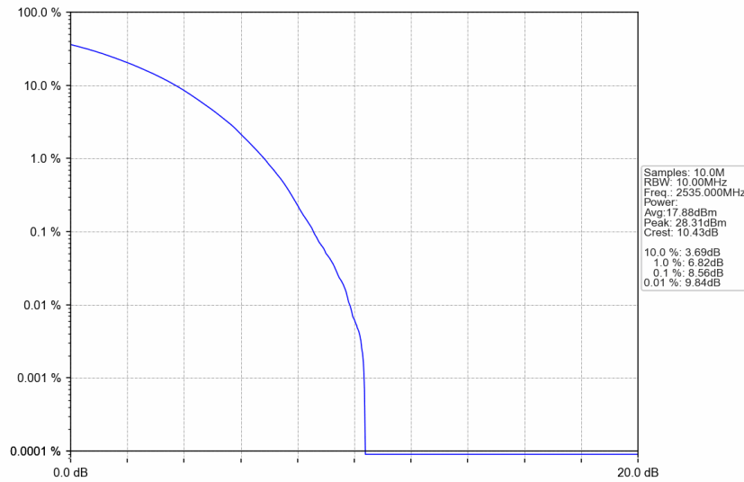
n7_15kHz_SISO_NTNV_10MHz_CP-OFDM 256 QAM_2535MHz_Outer_Full
