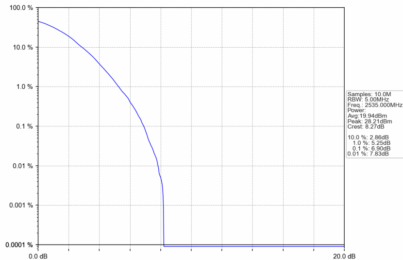
n7_15kHz_SISO_NTNV_5MHz_DFT-s-OFDM 256 QAM_2535MHz_Outer_Full
