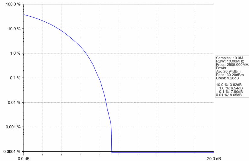
n7_15kHz_SISO_NTNV_10MHz_CP-OFDM 64 QAM_2505MHz_Outer_Full
