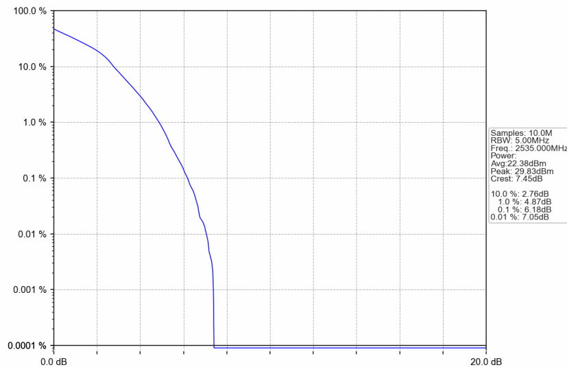
n7_15kHz_SISO_NTNV_5MHz_DFT-s-OFDM 16 QAM_2535MHz_Outer_Full
