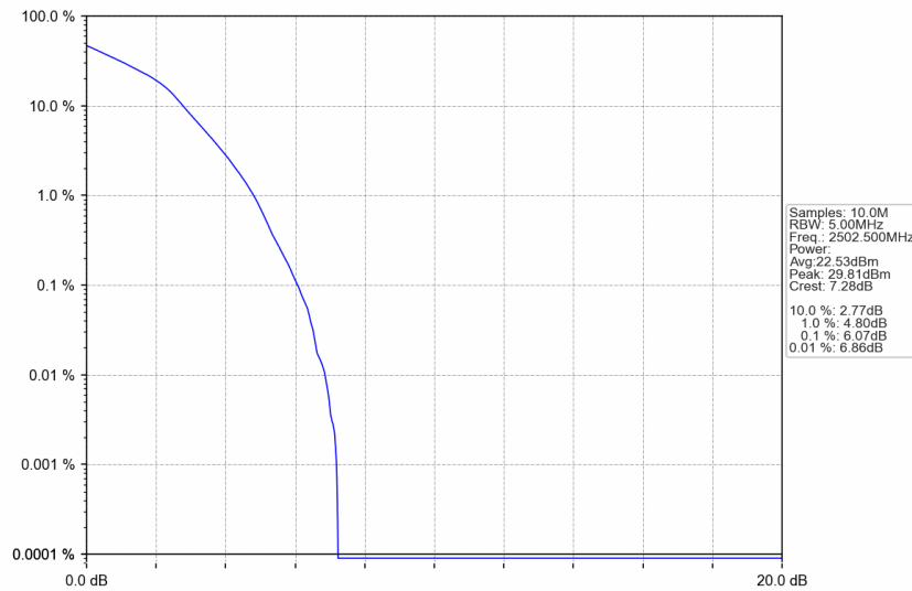
n7_15kHz_SISO_NTNV_5MHz_DFT-s-OFDM 16 QAM_2502.5MHz_Outer_Full
