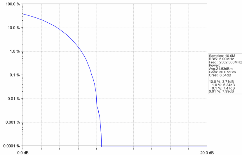
n7_15kHz_SISO_NTNV_5MHz_CP-OFDM QPSK_2502.5MHz_Outer_Full
