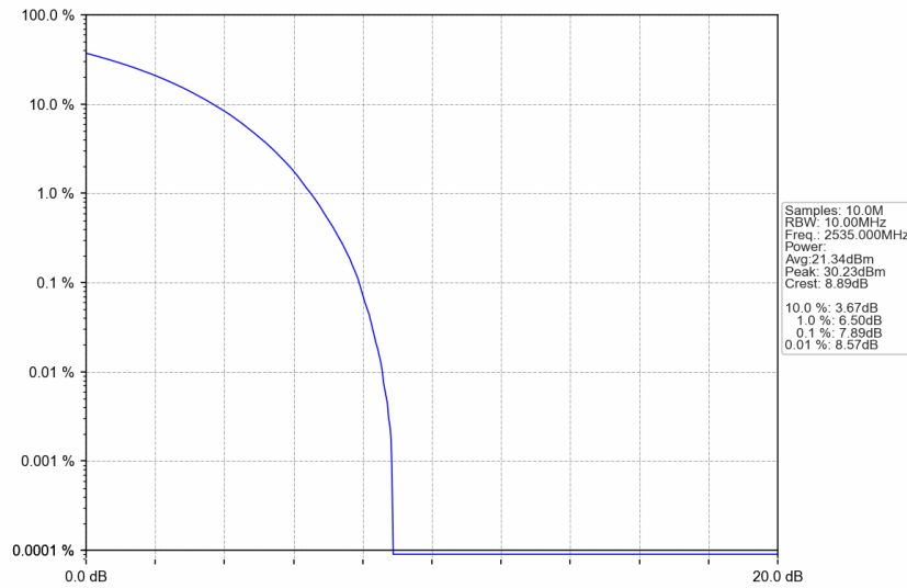
n7_15kHz_SISO_NTNV_10MHz_CP-OFDM 16 QAM_2535MHz_Outer_Full
