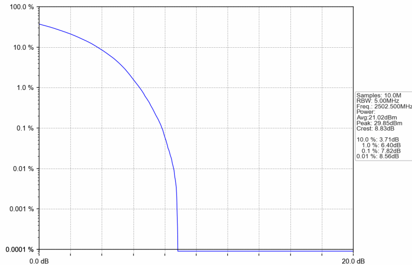
n7_15kHz_SISO_NTNV_5MHz_CP-OFDM 64 QAM_2502.5MHz_Outer_Full
