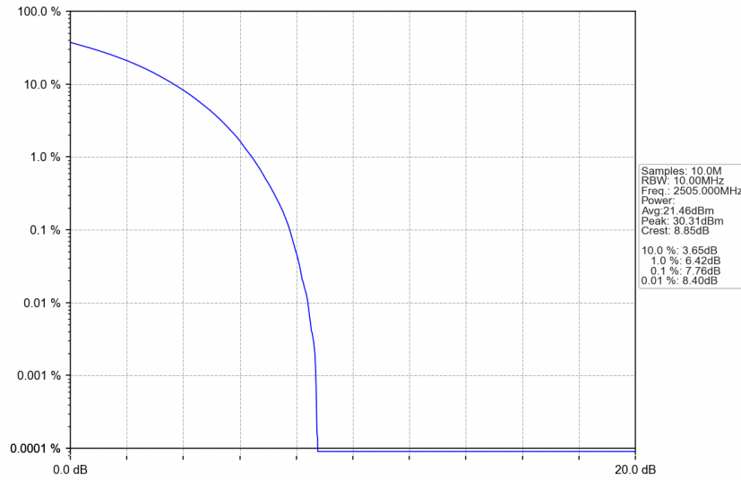
n7_15kHz_SISO_NTNV_10MHz_CP-OFDM 16 QAM_2505MHz_Outer_Full
