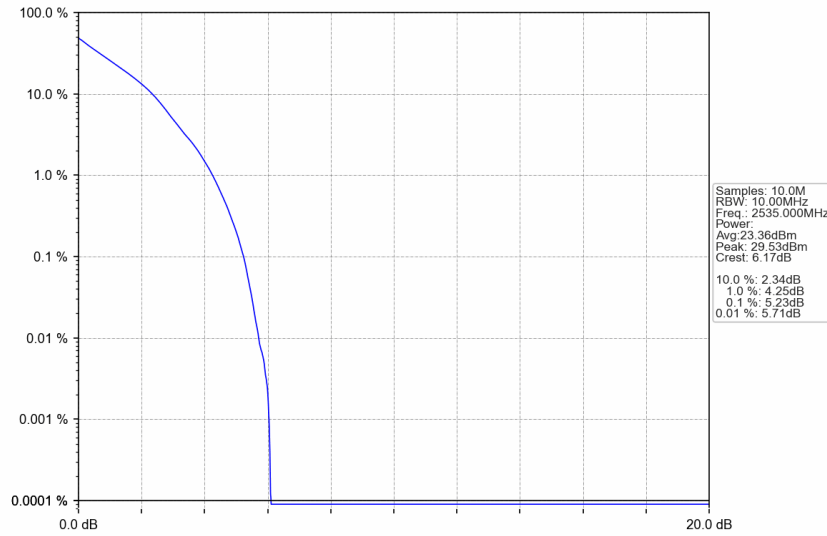
n7_15kHz_SISO_NTNV_10MHz_DFT-s-OFDM QPSK_2535MHz_Outer_Full
