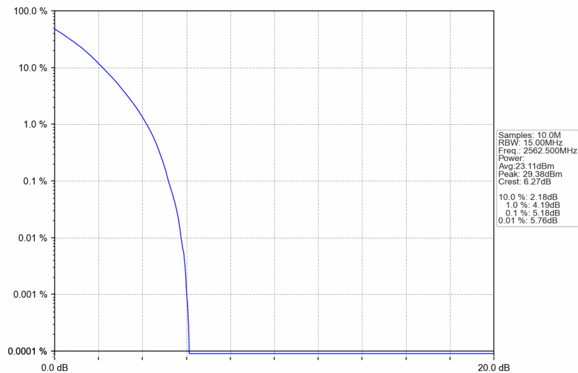
n7_15kHz_SISO_NTNV_15MHz_DFT-s-OFDM QPSK_2562.5MHz_Outer_Full
