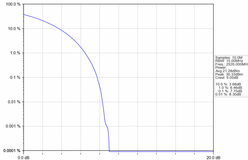
n7_15kHz_SISO_NTNV_15MHz_CP-OFDM 16 QAM_2535MHz_Outer_Full
