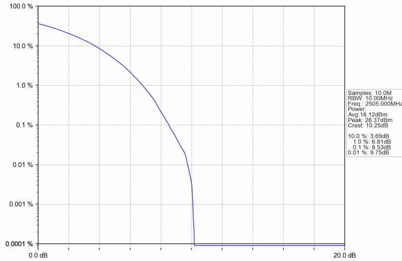
n7_15kHz_SISO_NTNV_10MHz_CP-OFDM 256 QAM_2505MHz_Outer_Full
