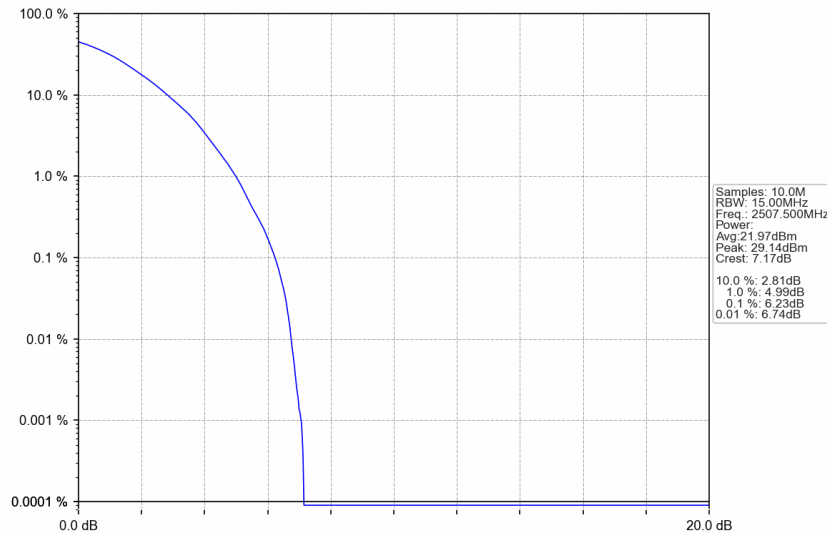
n7_15kHz_SISO_NTNV_15MHz_DFT-s-OFDM 64 QAM_2507.5MHz_Outer_Full
