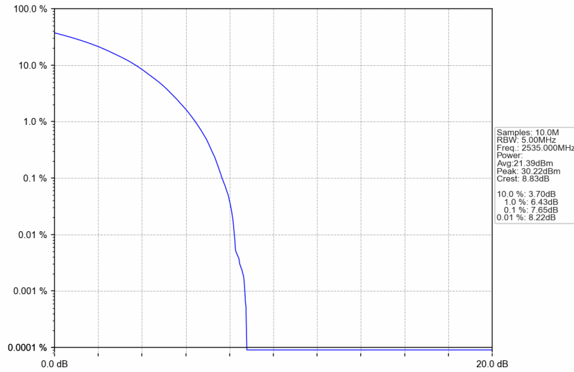
n7_15kHz_SISO_NTNV_5MHz_CP-OFDM QPSK_2535MHz_Outer_Full
