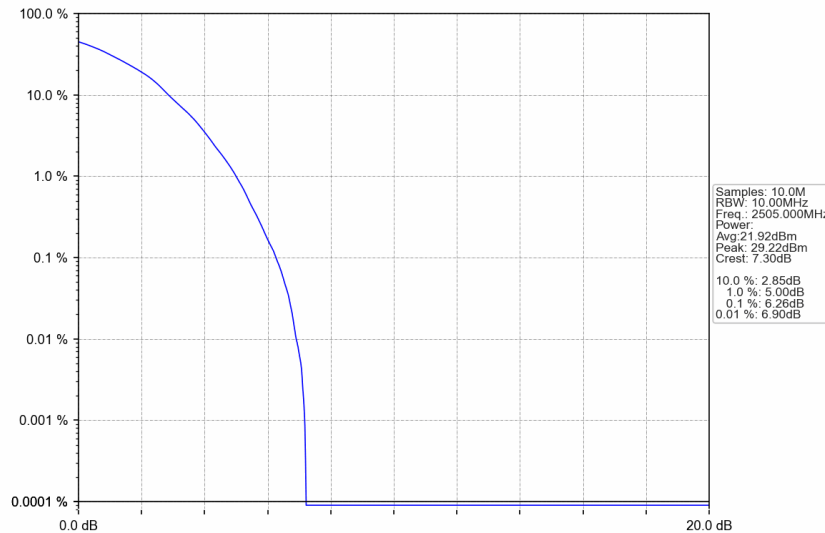
n7_15kHz_SISO_NTNV_10MHz_DFT-s-OFDM 64 QAM_2505MHz_Outer_Full
