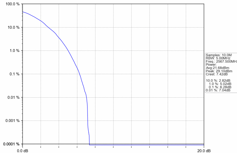
n7_15kHz_SISO_NTNV_5MHz_DFT-s-OFDM 64 QAM_2567.5MHz_Outer_Full
