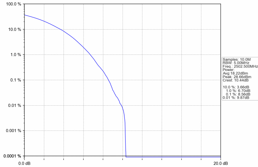
n7_15kHz_SISO_NTNV_5MHz_CP-OFDM 256 QAM_2502.5MHz_Outer_Full
