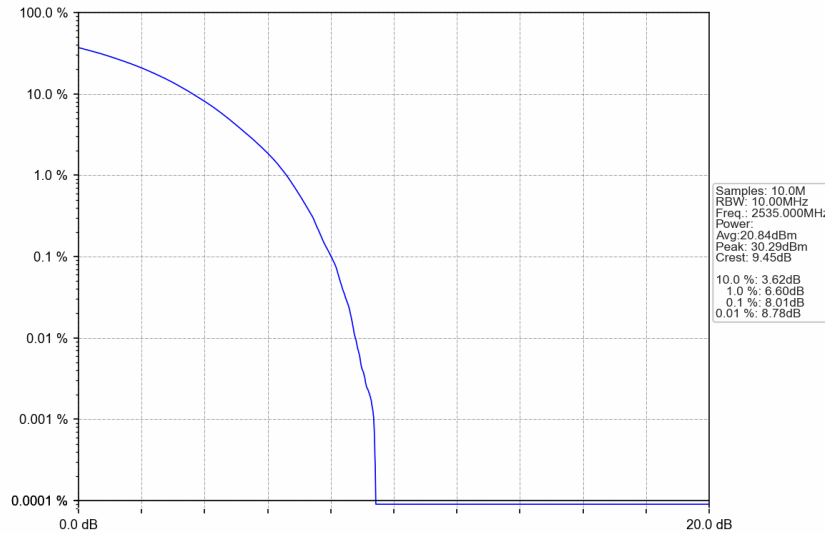
n7_15kHz_SISO_NTV_10MHz_CP-OFDM 64 QAM_2535MHz_Outer_Full
