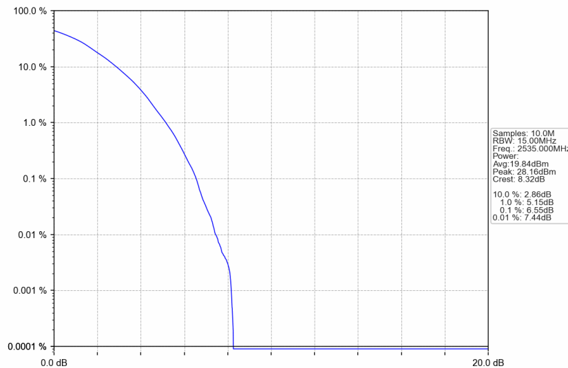
n7_15kHz_SISO_NTNV_15MHz_DFT-s-OFDM 256 QAM_2535MHz_Outer_Full
