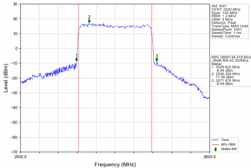
n7_30kHz_SISO_NTNV_40MHz_CP-OFDM 64 QAM_2550MHz_Outer_Full
