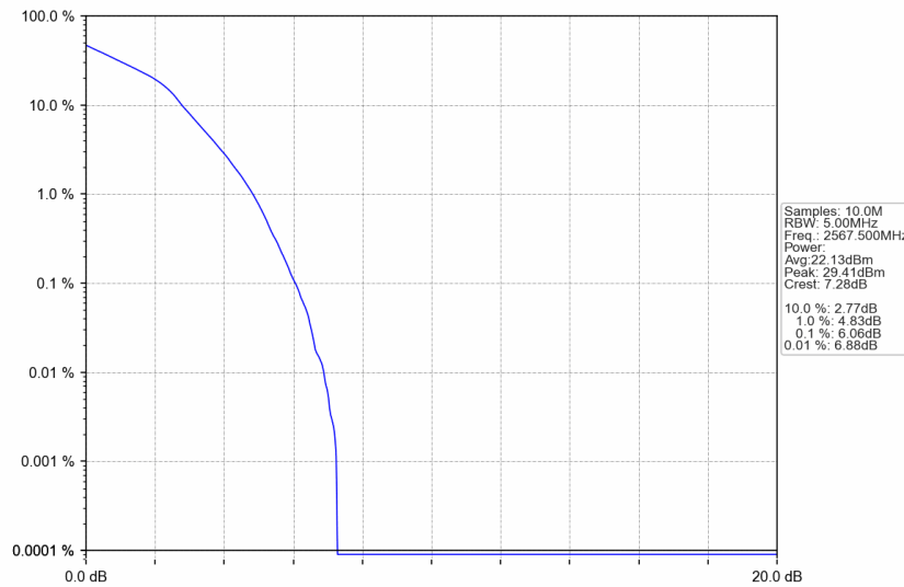
n7_15kHz_SISO_NTNV_5MHz_DFT-s-OFDM 16 QAM_2567.5MHz_Outer_Full
