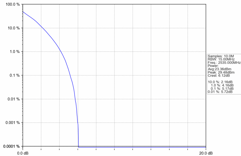
n7_15kHz_SISO_NTNV_15MHz_DFT-s-OFDM QPSK_2535MHz_Outer_Full
