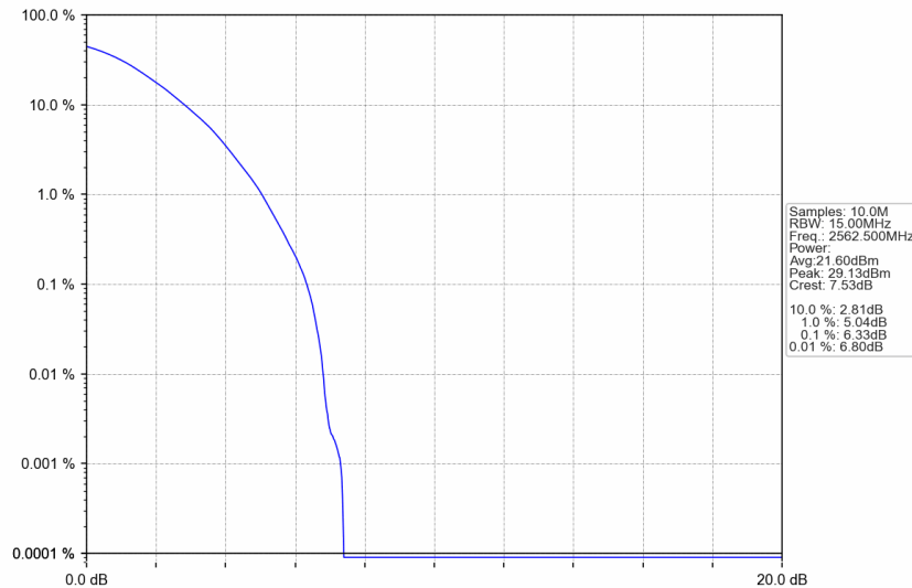
n7_15kHz_SISO_NTNV_15MHz_DFT-s-OFDM 64 QAM_2562.5MHz_Outer_Full
