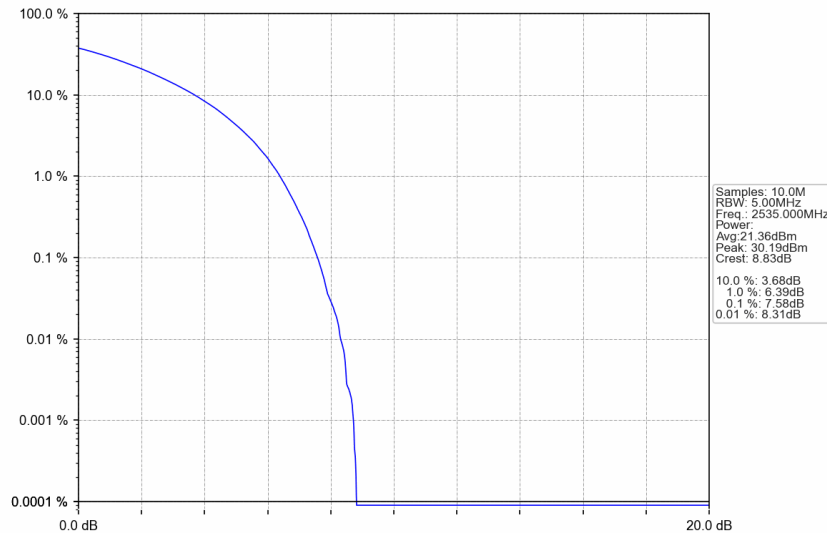
n7_15kHz_SISO_NTNV_5MHz_CP-OFDM 16 QAM_2535MHz_Outer_Full
