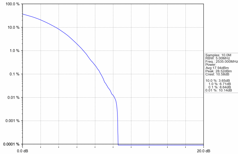
n7_15kHz_SISO_NTNV_5MHz_CP-OFDM 256 QAM_2535MHz_Outer_Full
