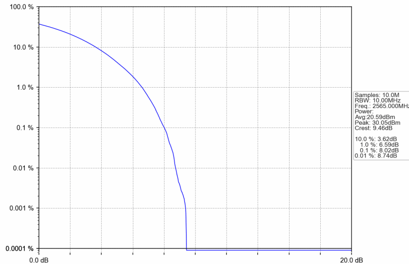
n7_15kHz_SISO_NTV_10MHz_CP-OFDM 64 QAM_2565MHz_Outer_Full
