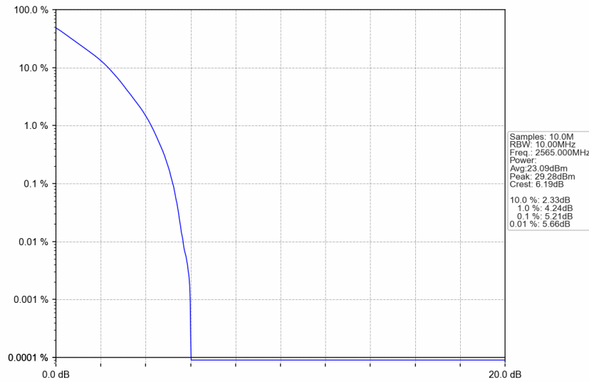
n7_15kHz_SISO_NTNV_10MHz_DFT-s-OFDM QPSK_2565MHz_Outer_Full
