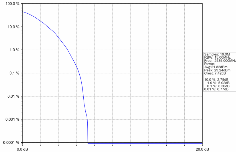
n7_15kHz_SISO_NTNV_15MHz_DFT-s-OFDM 64 QAM_2535MHz_Outer_Full
