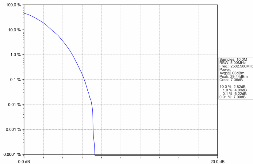
n7_15kHz_SISO_NTNV_5MHz_DFT-s-OFDM 64 QAM_2502.5MHz_Outer_Full
