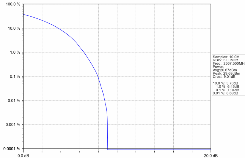
n7_15kHz_SISO_NTNV_5MHz_CP-OFDM 64 QAM_2567.5MHz_Outer_Full
