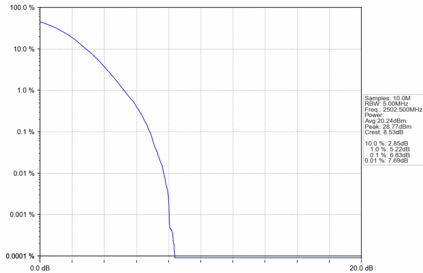
n7_15kHz_SISO_NTNV_5MHz_DFT-s-OFDM 256 QAM_2502.5MHz_Outer_Full
