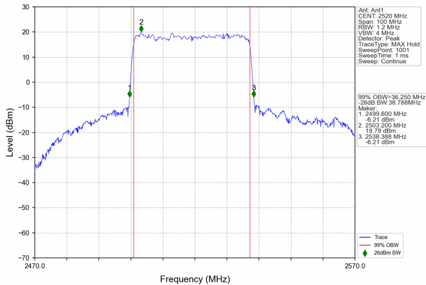
n7_30kHz_SISO_NTNV_40MHz_DFT-s-OFDM QPSK_2520MHz_Outer_Full
