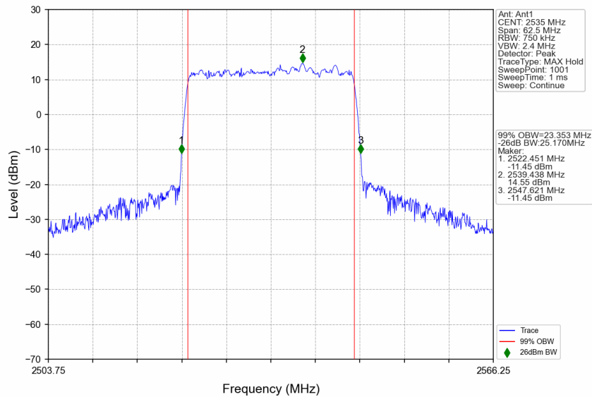
n7_30kHz_SISO_NTNV_25MHz_CP-OFDM 256 QAM_2535MHz_Outer_Full
