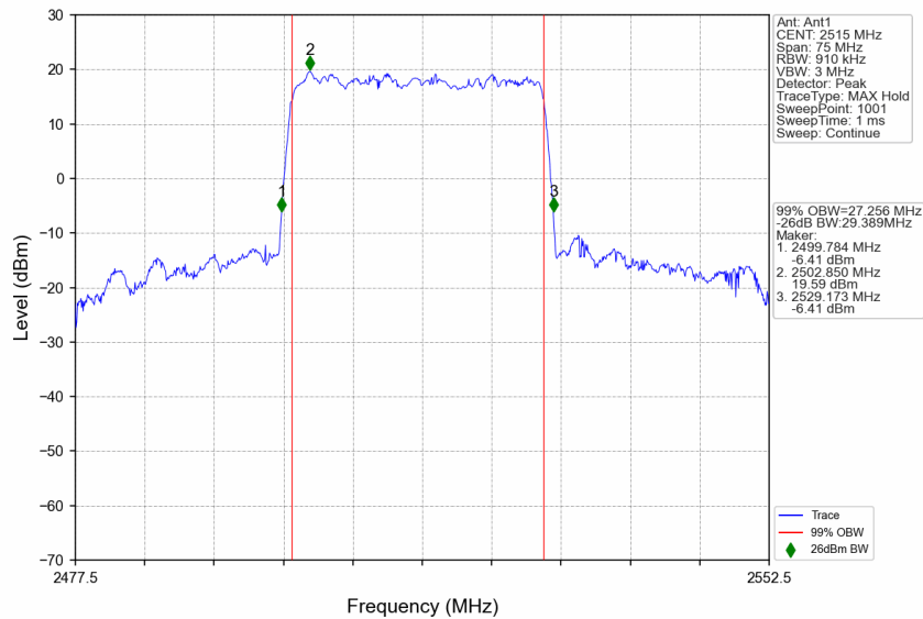
n7_30kHz_SISO_NTNV_30MHz_DFT-s-OFDM QPSK_2515MHz_Outer_Full
