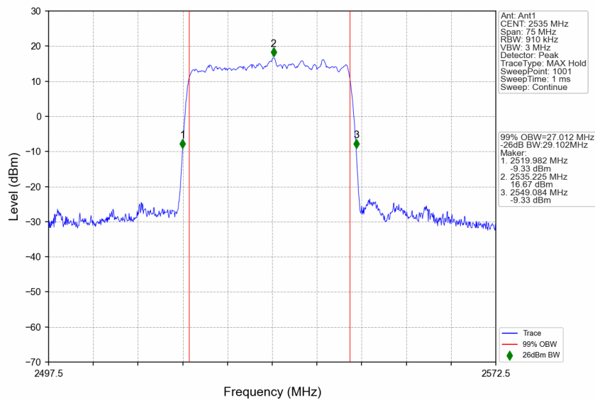
n7_30kHz_SISO_NTNV_30MHz_DFT-s-OFDM 256 QAM_2535MHz_Outer_Full
