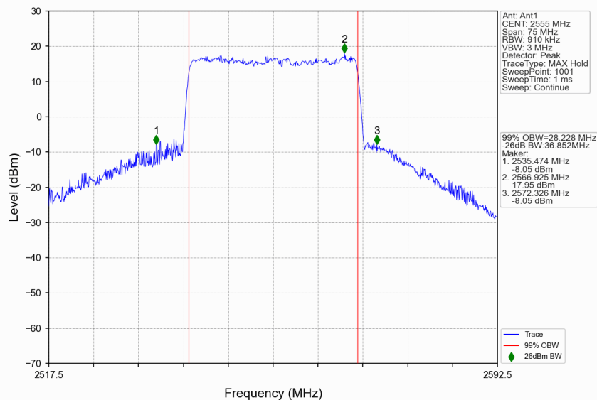
n7_30kHz_SISO_NTNV_30MHz_CP-OFDM QPSK_2555MHz_Outer_Full
