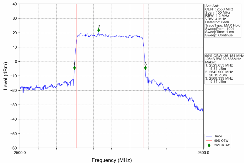
n7_30kHz_SISO_NTNV_40MHz_DFT-s-OFDM QPSK_2550MHz_Outer_Full
