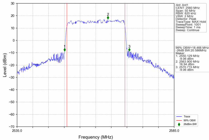
n7_30kHz_SISO_NTNV_20MHz_CP-OFDM 64 QAM_2560MHz_Outer_Full
