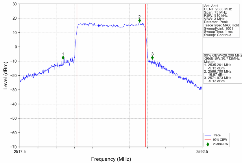
n7_30kHz_SISO_NTNV_30MHz_CP-OFDM 64 QAM_2555MHz_Outer_Full
