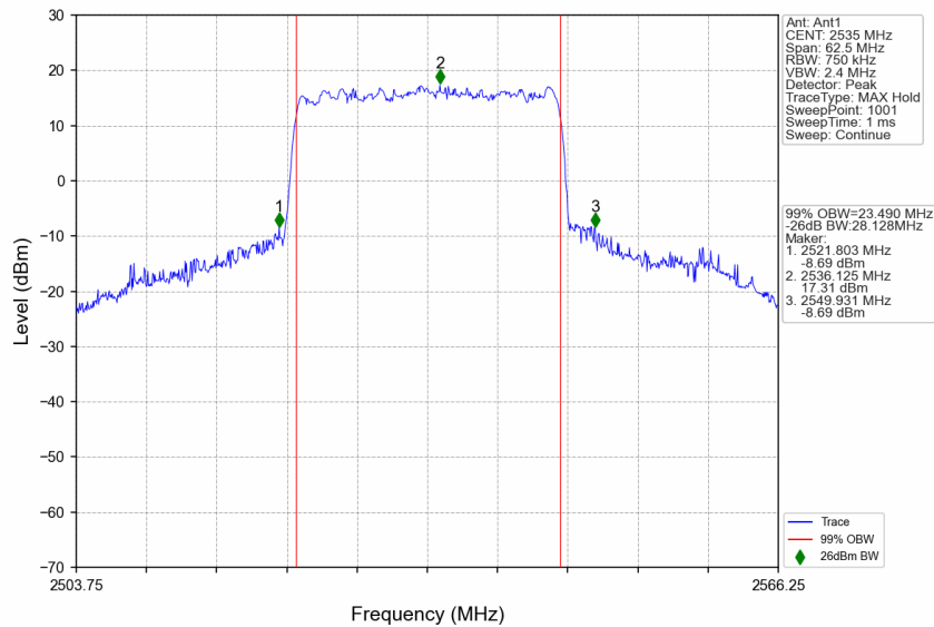
n7_30kHz_SISO_NTNV_25MHz_CP-OFDM 16 QAM_2535MHz_Outer_Full
