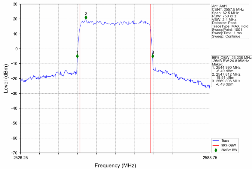
n7_30kHz_SISO_NTNV_25MHz_DFT-s-OFDM QPSK_2557.5MHz_Outer_Full
