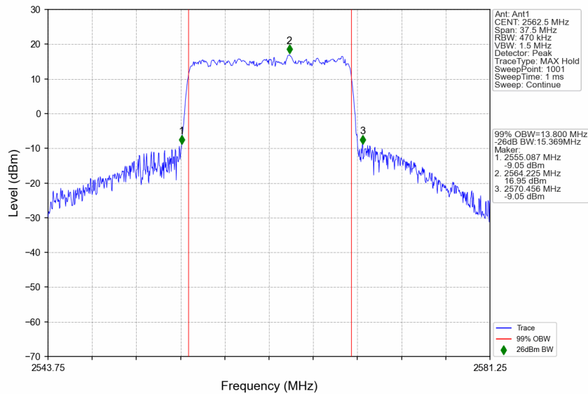
n7_30kHz_SISO_NTNV_15MHz_CP-OFDM 64 QAM_2562.5MHz_Outer_Full
