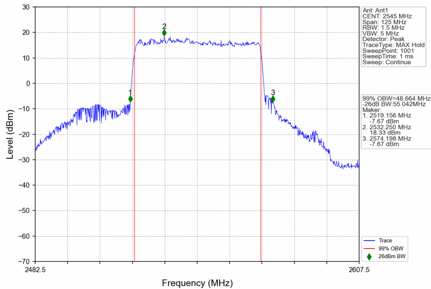
n7_15kHz_SISO_NTNV_50MHz_CP-OFDM QPSK_2545MHz_Outer_Full
