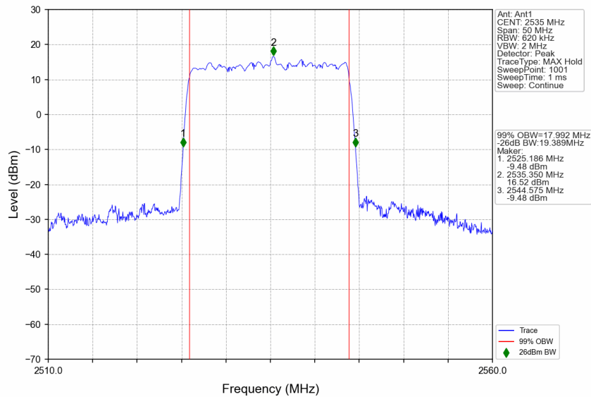
n7_30kHz_SISO_NTNV_20MHz_DFT-s-OFDM 256 QAM_2535MHz_Outer_Full
