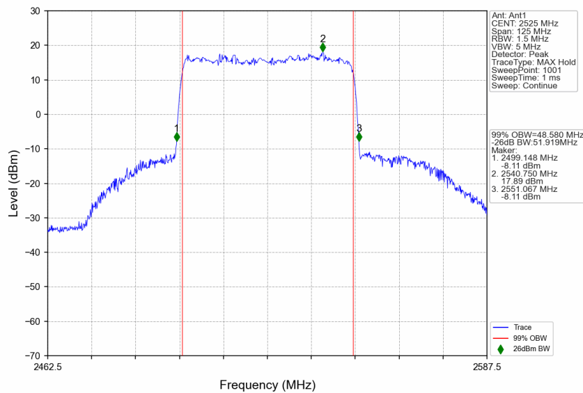
n7_15kHz_SISO_NTNV_50MHz_CP-OFDM 64 QAM_2525MHz_Outer_Full
