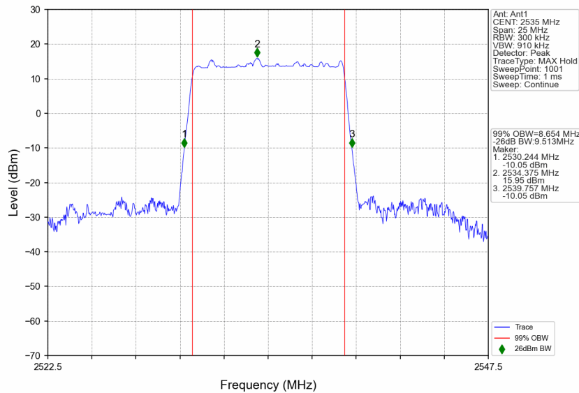
n7_30kHz_SISO_NTNV_10MHz_DFT-s-OFDM 256 QAM_2535MHz_Outer_Full
