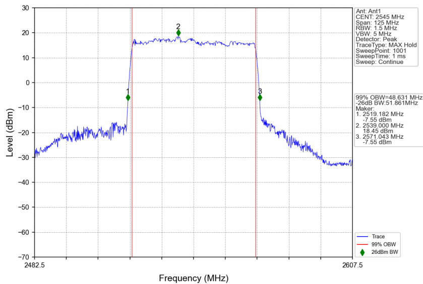
n7_15kHz_SISO_NTNV_50MHz_DFT-s-OFDM 64 QAM_2545MHz_Outer_Full
