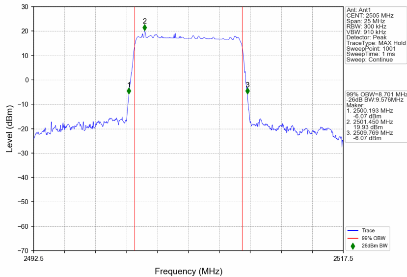
n7_30kHz_SISO_NTNV_10MHz_DFT-s-OFDM QPSK_2505MHz_Outer_Full
