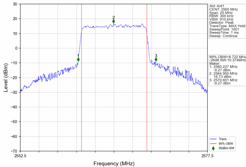
n7_30kHz_SISO_NTNV_10MHz_CP-OFDM QPSK_2565MHz_Outer_Full
