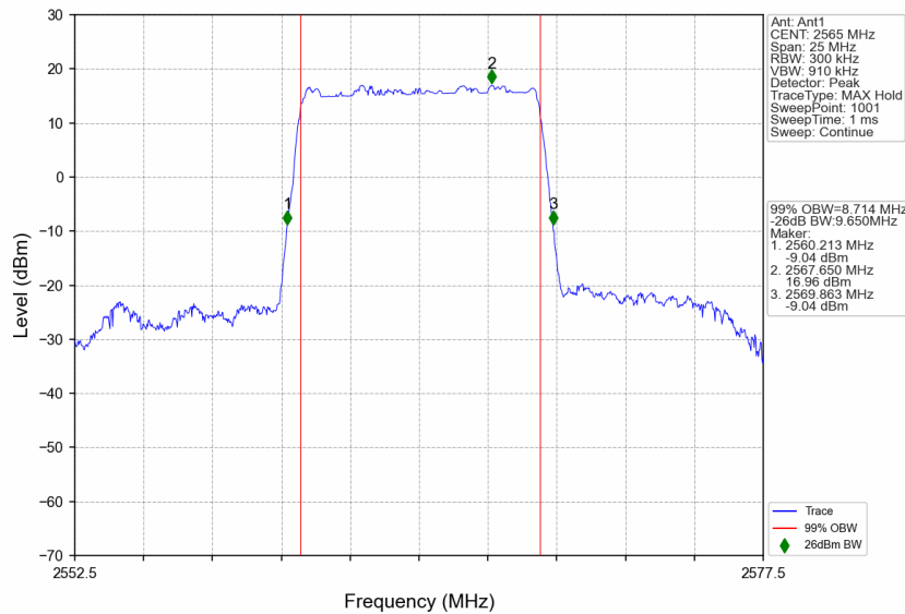
n7_30kHz_SISO_NTNV_10MHz_DFT-s-OFDM 64 QAM_2565MHz_Outer_Full
