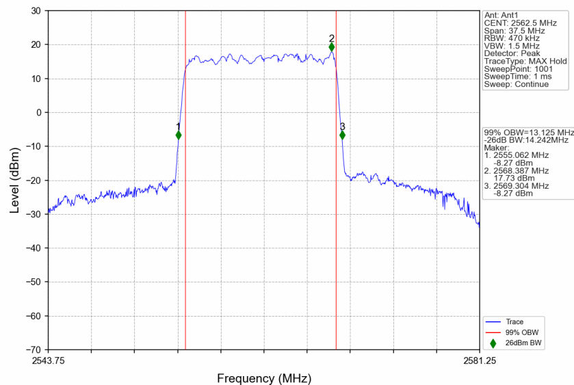
n7_30kHz_SISO_NTNV_15MHz_DFT-s-OFDM 64 QAM_2562.5MHz_Outer_Full
