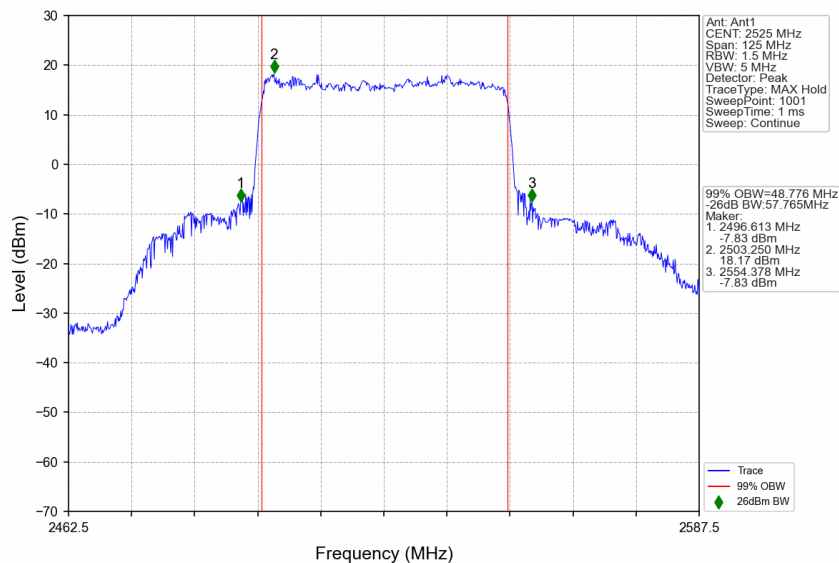
n7_15kHz_SISO_NTNV_50MHz_CP-OFDM QPSK_2525MHz_Outer_Full
