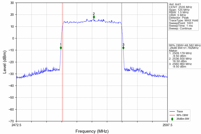
n7_15kHz_SISO_NTNV_50MHz_DFT-s-OFDM 256 QAM_2535MHz_Outer_Full
