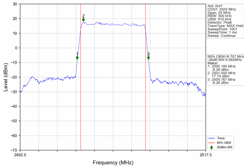
n7_30kHz_SISO_NTNV_10MHz_DFT-s-OFDM 64 QAM_2505MHz_Outer_Full
