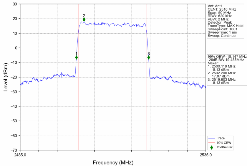
n7_30kHz_SISO_NTNV_20MHz_DFT-s-OFDM 64 QAM_2510MHz_Outer_Full
