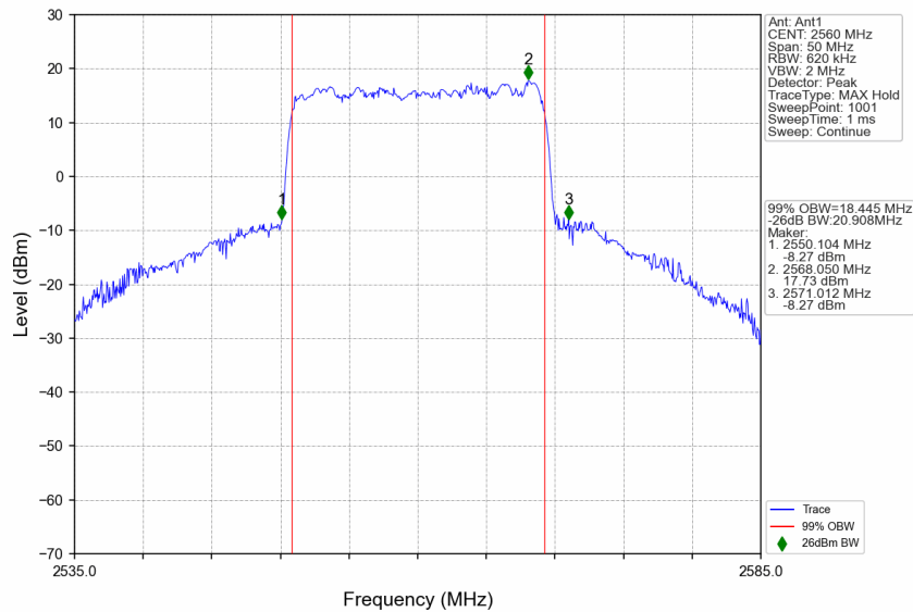
n7_30kHz_SISO_NTNV_20MHz_CP-OFDM QPSK_2560MHz_Outer_Full
