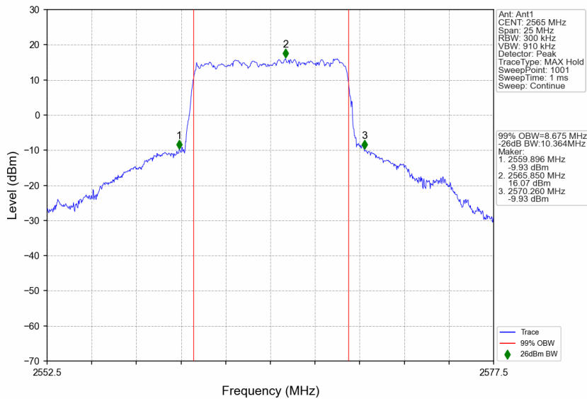
n7_30kHz_SISO_NTNV_10MHz_CP-OFDM 64 QAM_2565MHz_Outer_Full
