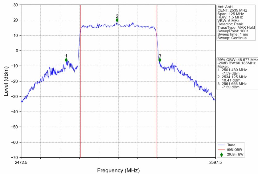
n7_15kHz_SISO_NTNV_50MHz_CP-OFDM 16 QAM_2535MHz_Outer_Full
