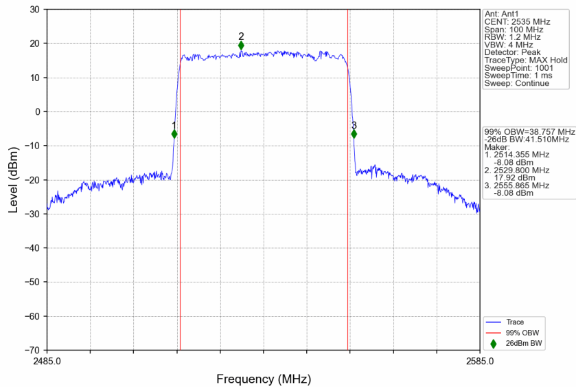
n7_15kHz_SISO_NTNV_40MHz_DFT-s-OFDM 16 QAM_2535MHz_Outer_Full
