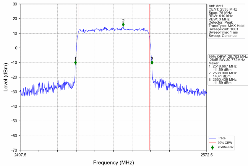
n7_15kHz_SISO_NTNV_30MHz_CP-OFDM 256 QAM_2535MHz_Outer_Full
