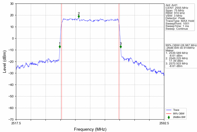
n7_15kHz_SISO_NTNV_30MHz_DFT-s-OFDM 64 QAM_2555MHz_Outer_Full
