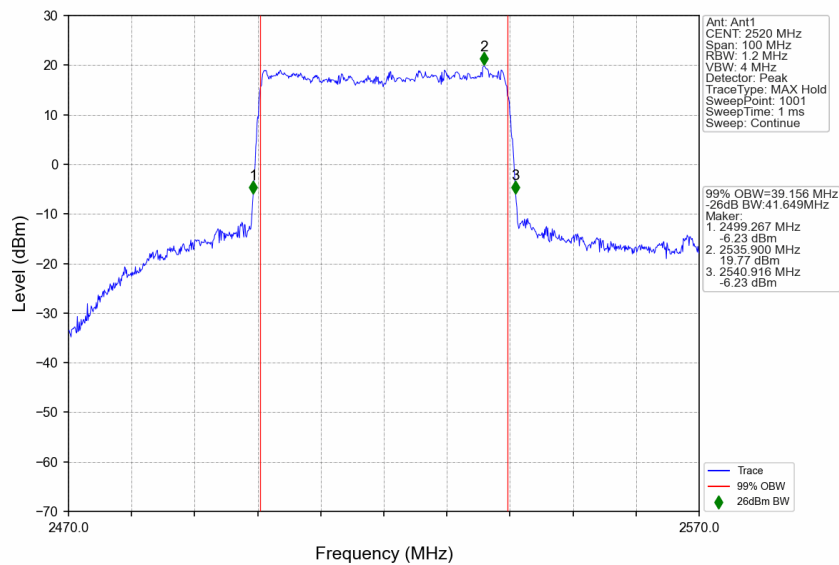
n7_15kHz_SISO_NTNV_40MHz_DFT-s-OFDM QPSK_2520MHz_Outer_Full
