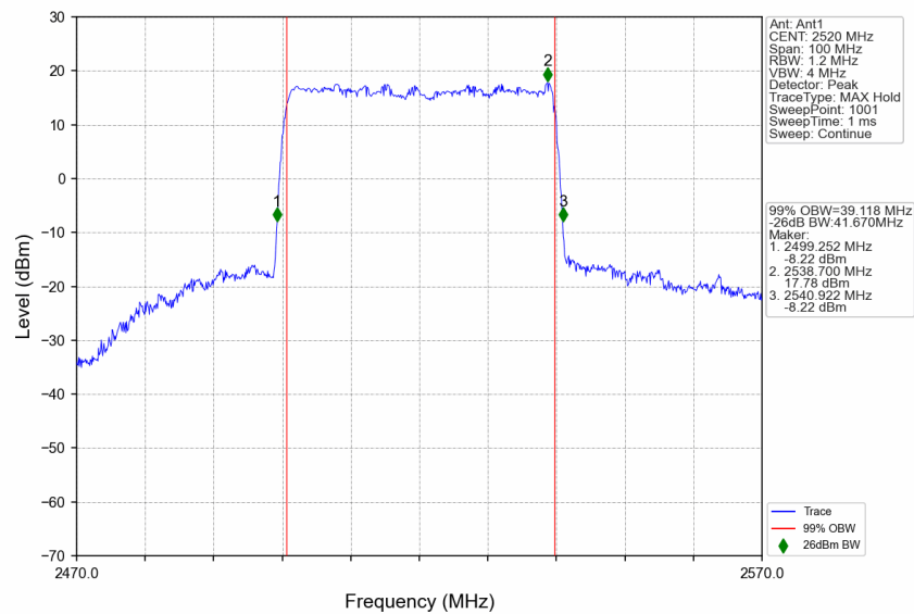
n7_15kHz_SISO_NTNV_40MHz_DFT-s-OFDM 64 QAM_2520MHz_Outer_Full
