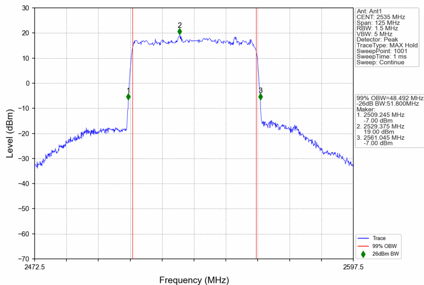
n7_15kHz_SISO_NTNV_50MHz_DFT-s-OFDM 16 QAM_2535MHz_Outer_Full
