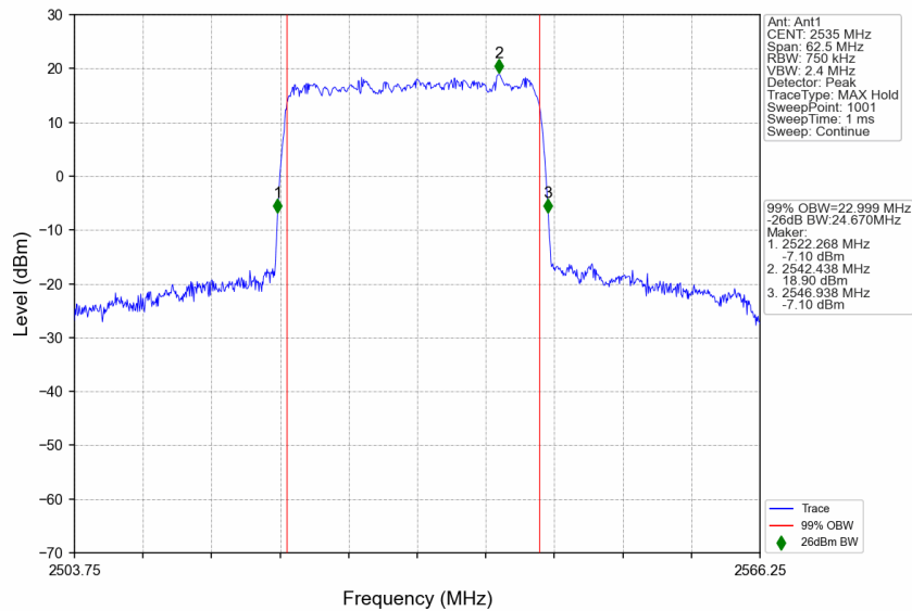
n7_15kHz_SISO_NTNV_25MHz_DFT-s-OFDM 16 QAM_2535MHz_Outer_Full
