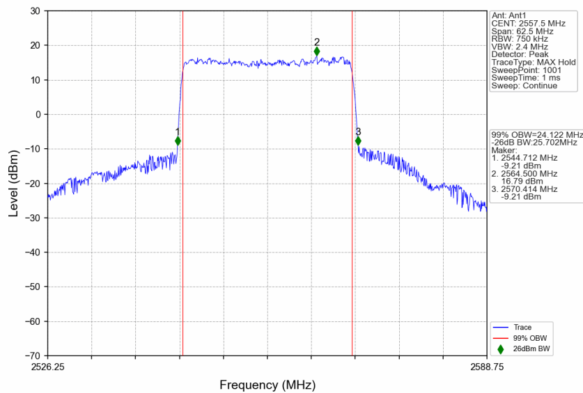
n7_15kHz_SISO_NTNV_25MHz_CP-OFDM 64 QAM_2557.5MHz_Outer_Full
