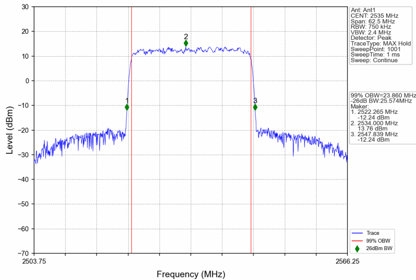
n7_15kHz_SISO_NTNV_25MHz_CP-OFDM 256 QAM_2535MHz_Outer_Full
