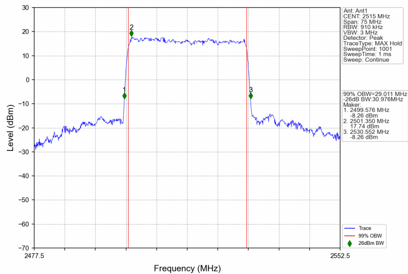
n7_15kHz_SISO_NTNV_30MHz_DFT-s-OFDM 64 QAM_2515MHz_Outer_Full
