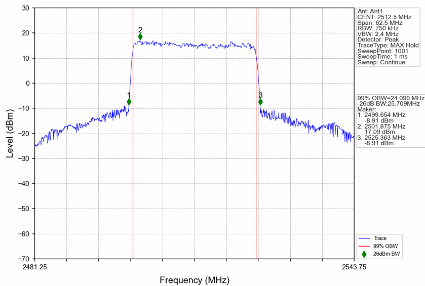
n7_15kHz_SISO_NTNV_25MHz_CP-OFDM 64 QAM_2512.5MHz_Outer_Full
