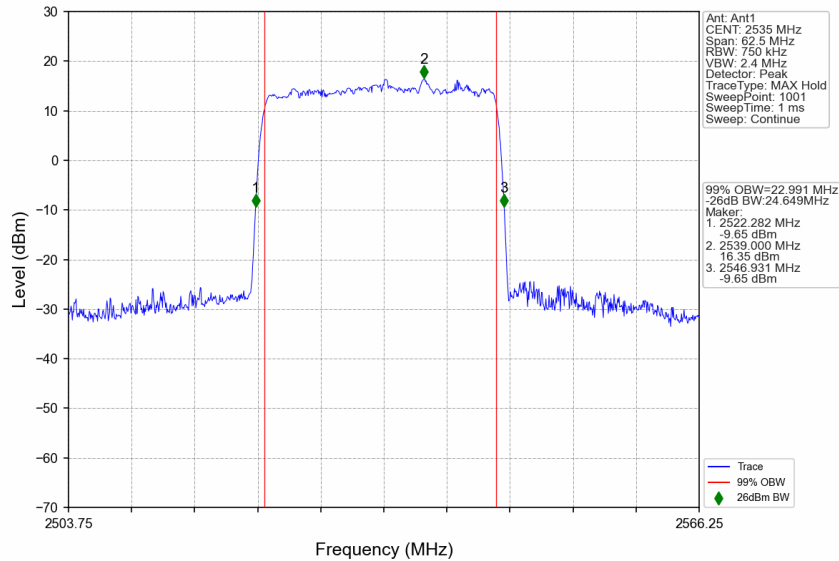
n7_15kHz_SISO_NTNV_25MHz_DFT-s-OFDM 256 QAM_2535MHz_Outer_Full
