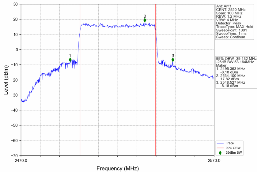
n7_15kHz_SISO_NTNV_40MHz_CP-OFDM QPSK_2520MHz_Outer_Full
