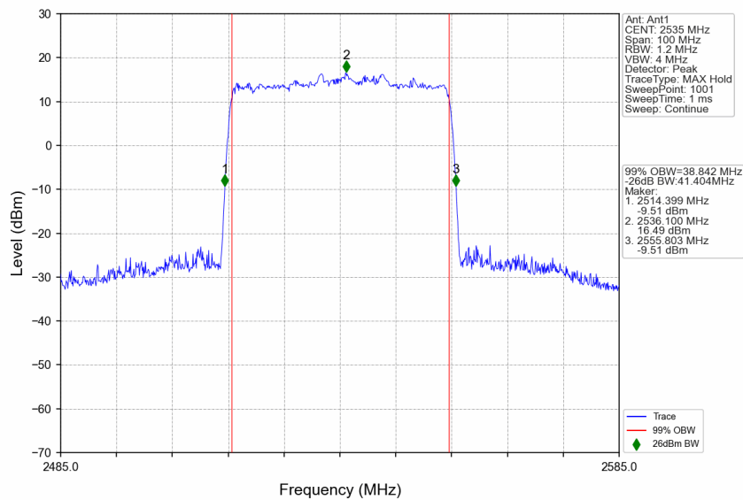
n7_15kHz_SISO_NTNV_40MHz_DFT-s-OFDM 256 QAM_2535MHz_Outer_Full
