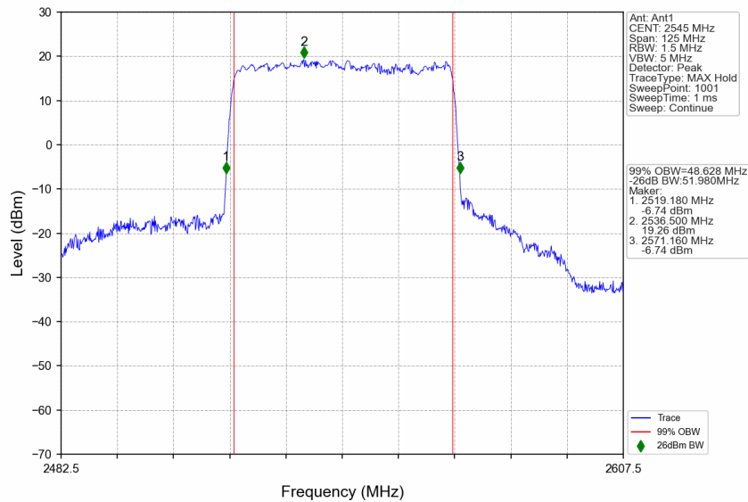
n7_15kHz_SISO_NTNV_50MHz_DFT-s-OFDM QPSK_2545MHz_Outer_Full
