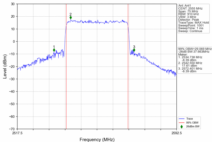
n7_15kHz_SISO_NTNV_30MHz_CP-OFDM QPSK_2555MHz_Outer_Full
