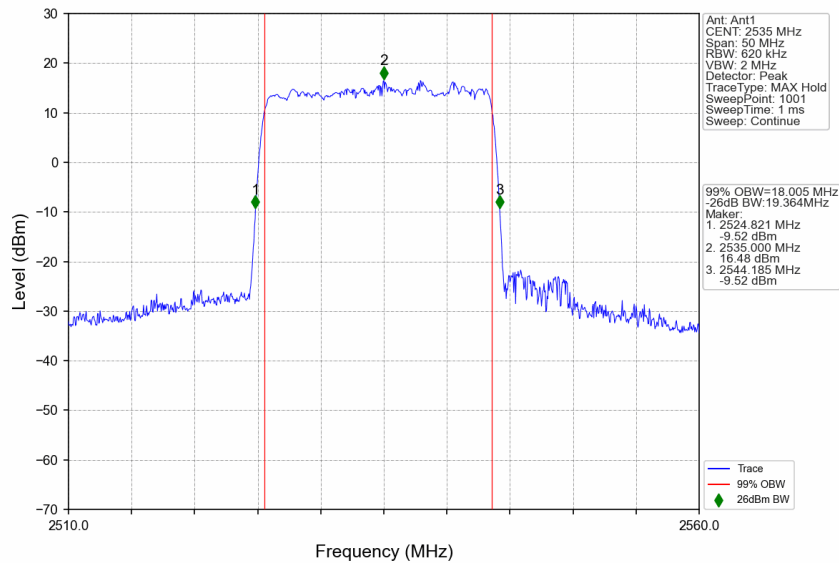
n7_15kHz_SISO_NTNV_20MHz_DFT-s-OFDM 256 QAM_2535MHz_Outer_Full
