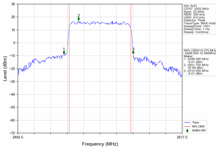
n7_15kHz_SISO_NTNV_10MHz_CP-OFDM QPSK_2505MHz_Outer_Full
