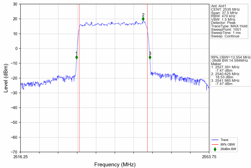
n7_15kHz_SISO_NTNV_15MHz_DFT-s-OFDM 16 QAM_2535MHz_Outer_Full
