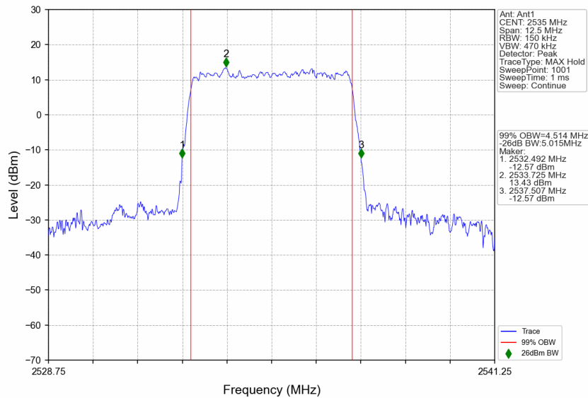
n7_15kHz_SISO_NTNV_5MHz_CP-OFDM 256 QAM_2535MHz_Outer_Full
