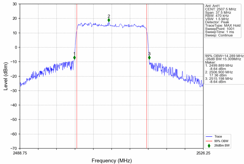
n7_15kHz_SISO_NTNV_15MHz_CP-OFDM 64 QAM_2507.5MHz_Outer_Full
