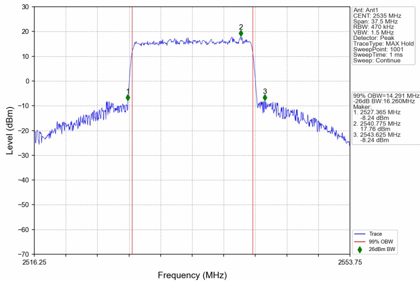
n7_15kHz_SISO_NTNV_15MHz_CP-OFDM 16 QAM_2535MHz_Outer_Full
