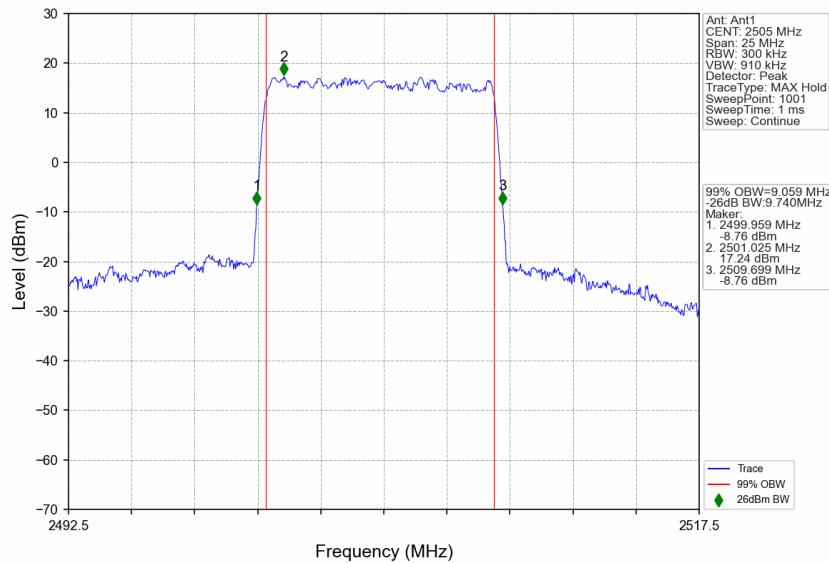
n7_15kHz_SISO_NTNV_10MHz_DFT-s-OFDM 64 QAM_2505MHz_Outer_Full
