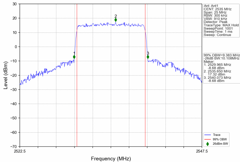
n7_15kHz_SISO_NTNV_10MHz_CP-OFDM 16 QAM_2535MHz_Outer_Full
