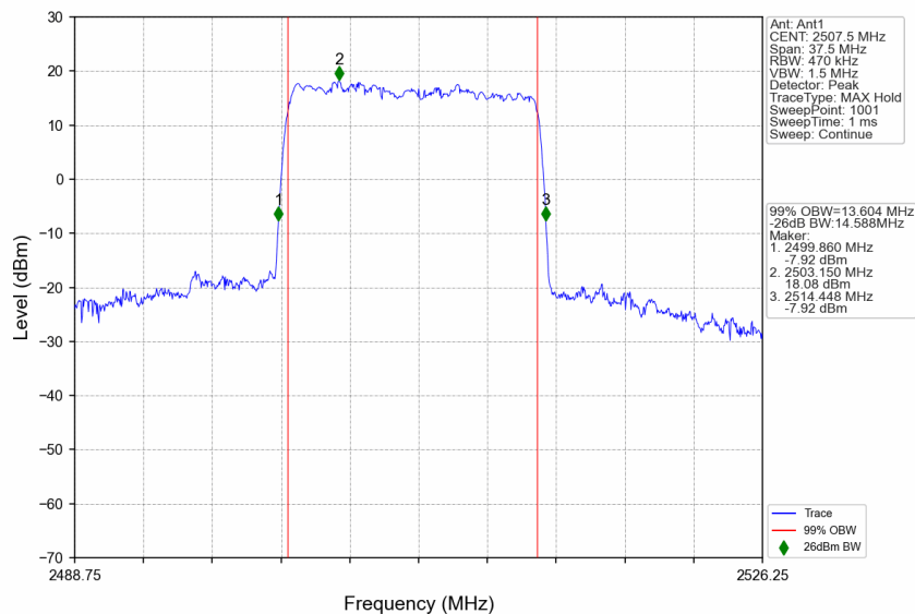
n7_15kHz_SISO_NTNV_15MHz_DFT-s-OFDM 64 QAM_2507.5MHz_Outer_Full
