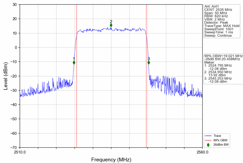
n7_15kHz_SISO_NTNV_20MHz_CP-OFDM 256 QAM_2535MHz_Outer_Full
