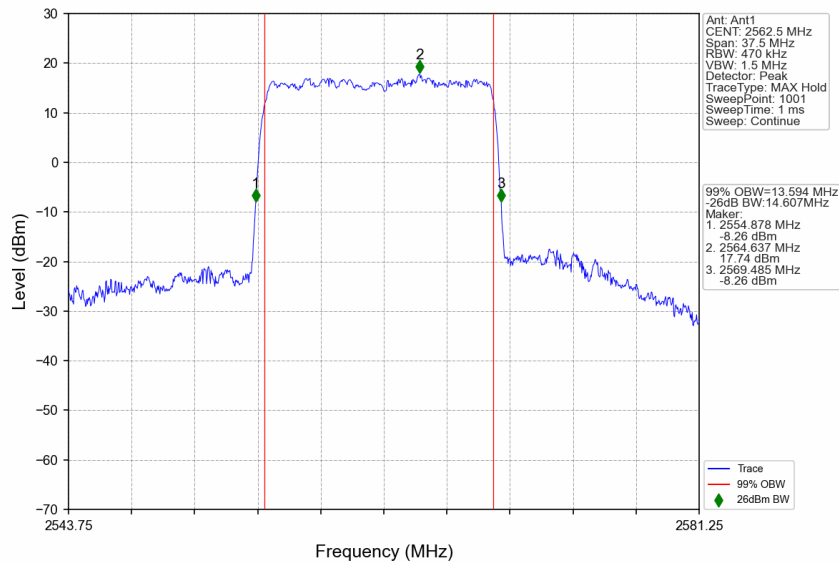
n7_15kHz_SISO_NTNV_15MHz_DFT-s-OFDM 64 QAM_2562.5MHz_Outer_Full
