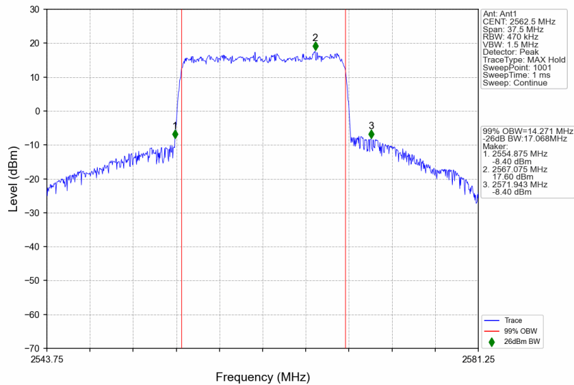
n7_15kHz_SISO_NTNV_15MHz_CP-OFDM QPSK_2562.5MHz_Outer_Full
