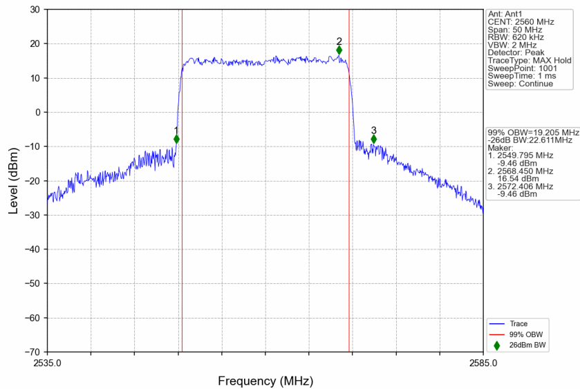
n7_15kHz_SISO_NTNV_20MHz_CP-OFDM 64 QAM_2560MHz_Outer_Full
