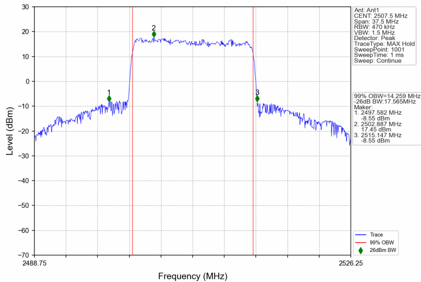
n7_15kHz_SISO_NTNV_15MHz_CP-OFDM QPSK_2507.5MHz_Outer_Full
