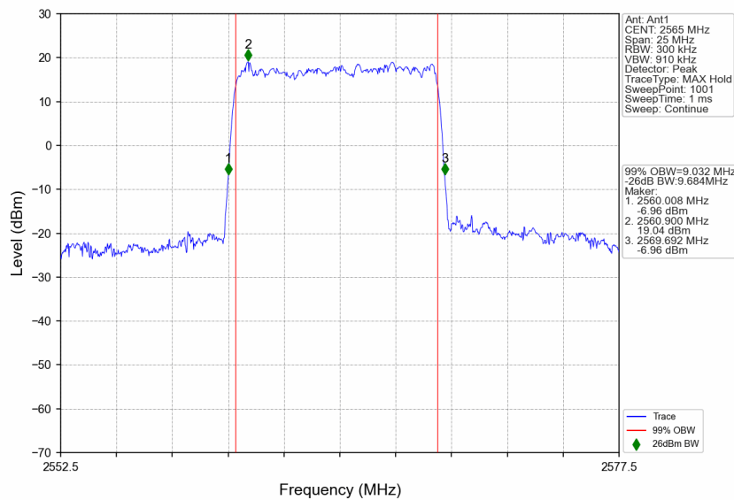
n7_15kHz_SISO_NTNV_10MHz_DFT-s-OFDM QPSK_2565MHz_Outer_Full
