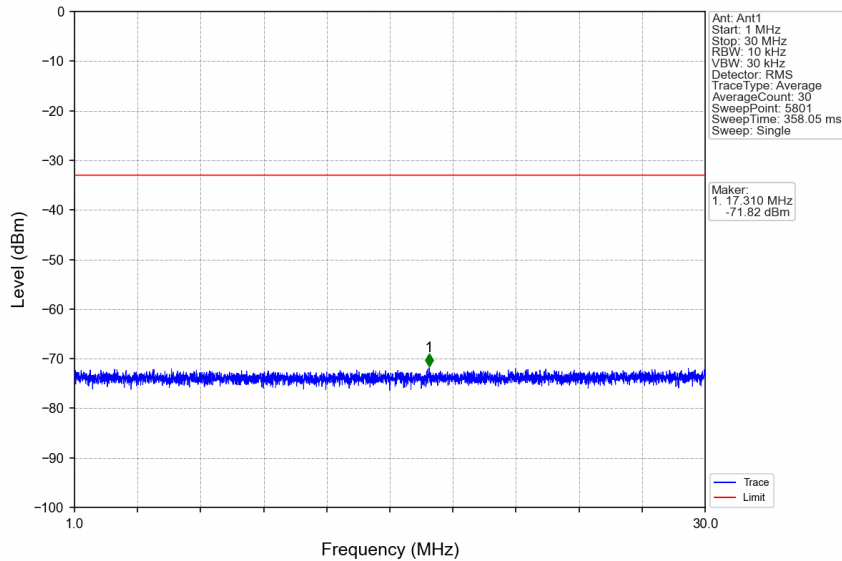
n5_30kHz_SISO_NTNV_10MHz_DFT-s-OFDM QPSK_844MHz_Edge_1RB_Right
