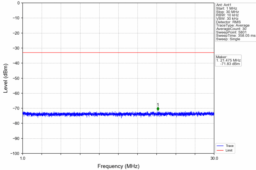
n5_15kHz_SISO_NTNV_15MHz_CP-OFDM QPSK_836.5MHz_Edge_1RB_Left
