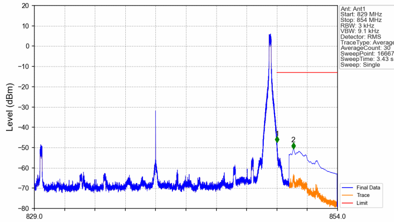
n5_15kHz_SISO_NTNV_20MHz_CP-OFDM QPSK_839MHz_Edge_1RB_Right
