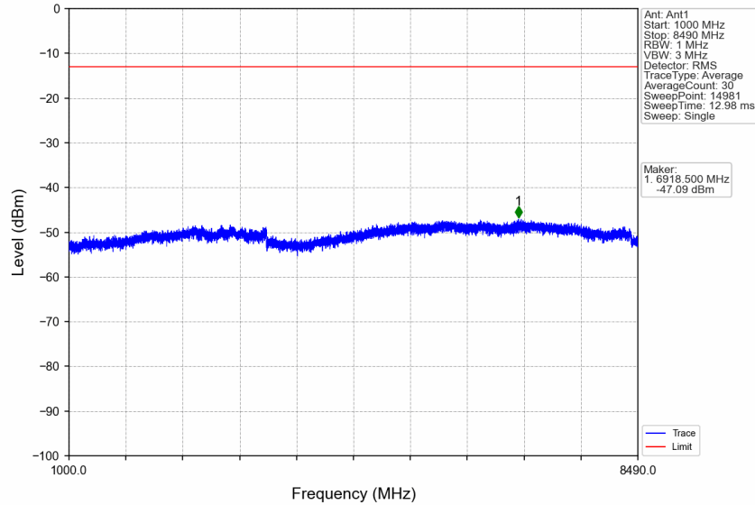
n5_15kHz_SISO_NTNV_20MHz_DFT-s-OFDM QPSK_839MHz_Edge_1RB_Right
