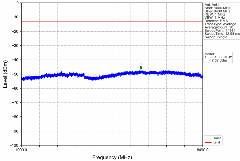
n5_15kHz_SISO_NTNV_20MHz_CP-OFDM QPSK_834MHz_Outer_Full
