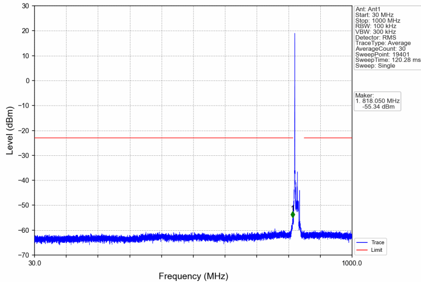
n5_30kHz_SISO_NTNV_10MHz_DFT-s-OFDM QPSK_829MHz_Edge_1RB_Left
