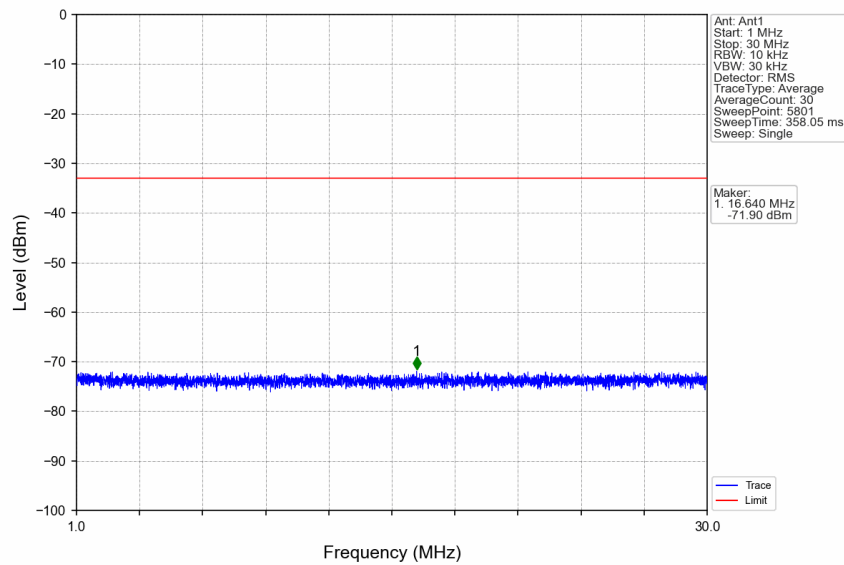
n5_15kHz_SISO_NTNV_20MHz_DFT-s-OFDM QPSK_834MHz_Edge_1RB_Left
