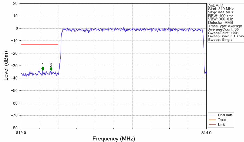
n5_15kHz_SISO_NTNV_20MHz_CP-OFDM QPSK_834MHz_Outer_Full
