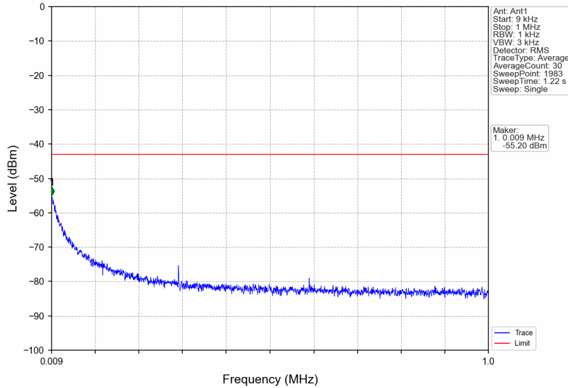
n5_15kHz_SISO_NTNV_20MHz_CP-OFDM QPSK_839MHz_Edge_1RB_Right
