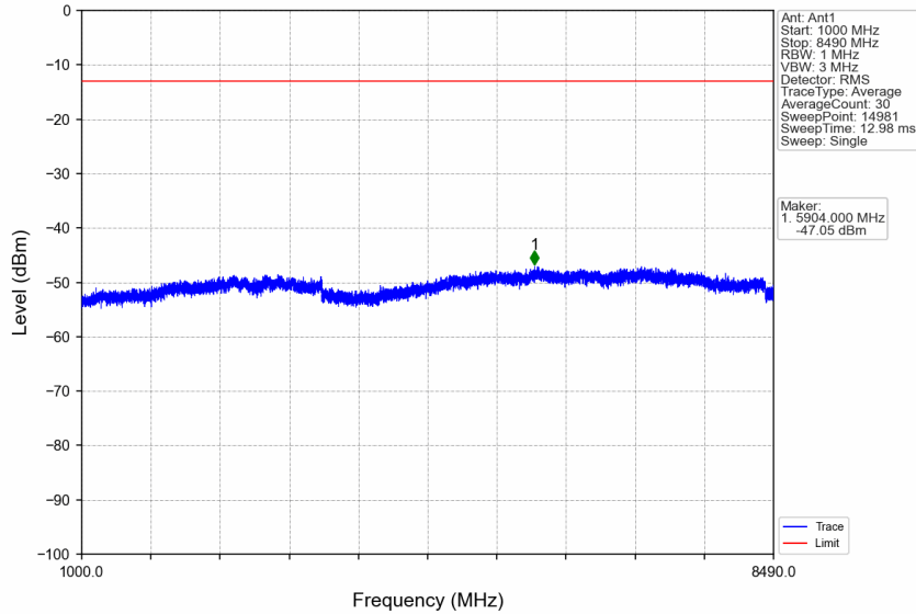
n5_15kHz_SISO_NTNV_20MHz_CP-OFDM QPSK_839MHz_Edge_1RB_Right
