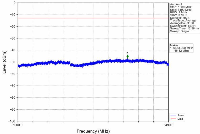
n5_30kHz_SISO_NTNV_10MHz_DFT-s-OFDM QPSK_844MHz_Edge_1RB_Right
