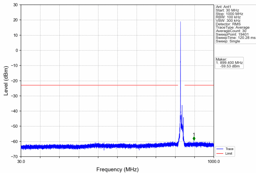
n5_30kHz_SISO_NTNV_10MHz_DFT-s-OFDM_QPSK_836.5MHz_Edge_1RB_Left
