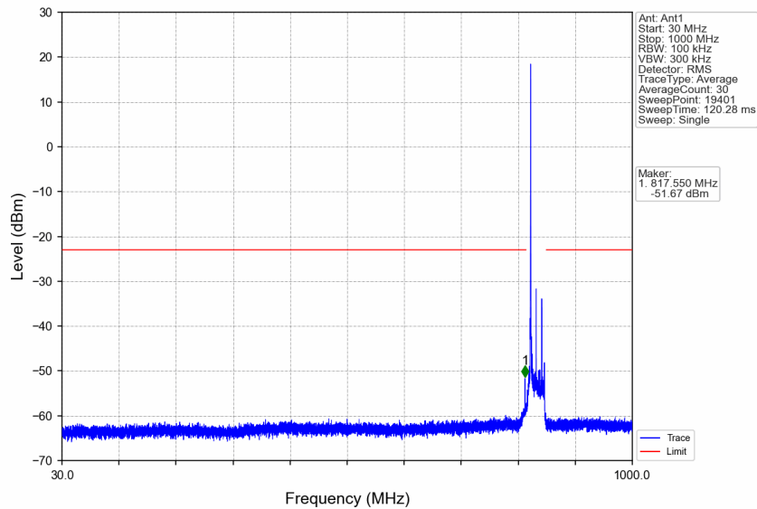
n5_15kHz_SISO_NTNV_20MHz_CP-OFDM QPSK_836.5MHz_Edge_1RB_Left
