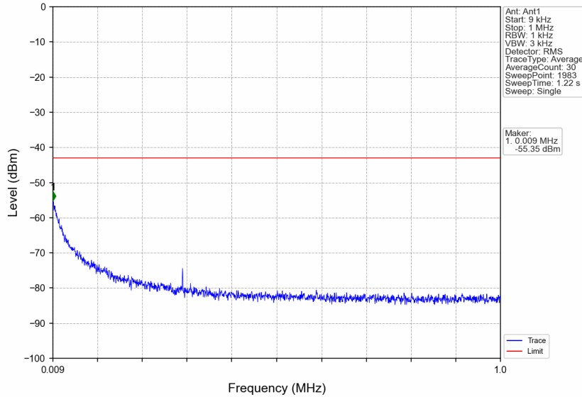
n5_30kHz_SISO_NTNV_10MHz_DFT-s-OFDM PI/2 BPSK_844MHz_Edge_1RB_Right
