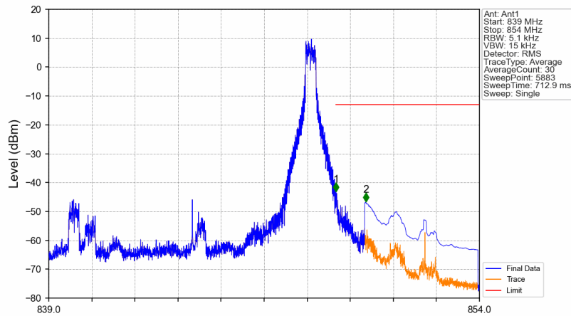
n5_30kHz_SISO_NTNV_10MHz_DFT-s-OFDM PI/2 BPSK_844MHz_Edge_1RB_Right
