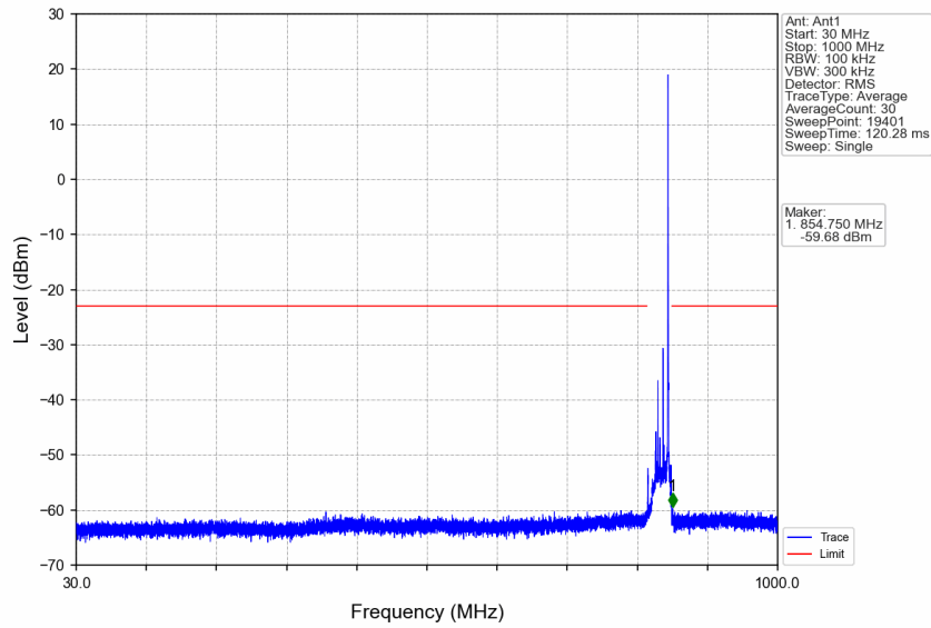
n5_15kHz_SISO_NTNV_15MHz_CP-OFDM QPSK_841.5MHz_Edge_1RB_Right
