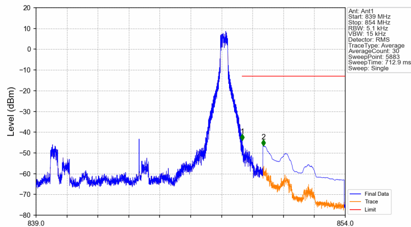
n5_30kHz_SISO_NTNV_10MHz_DFT-s-OFDM QPSK_844MHz_Edge_1RB_Right
