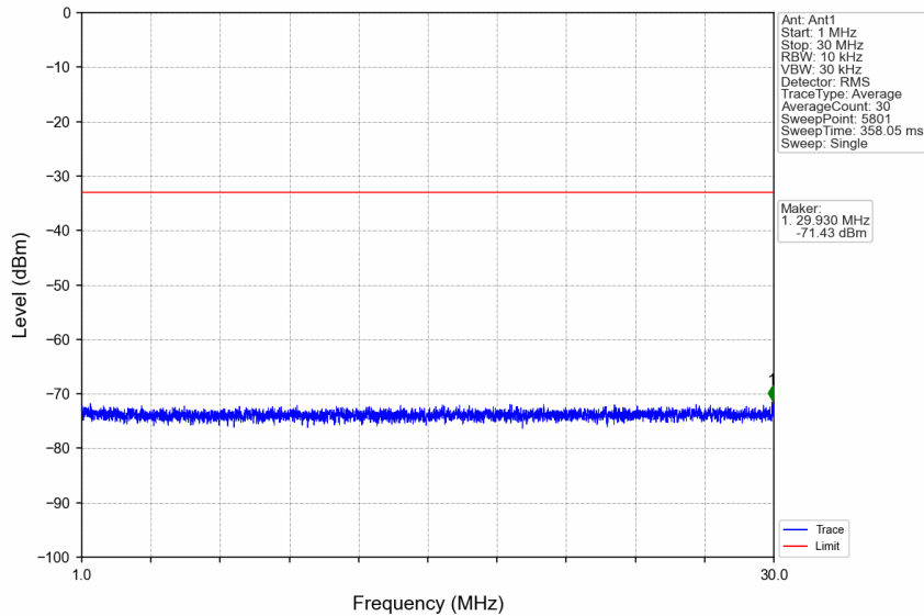
n5_15kHz_SISO_NTNV_20MHz_CP-OFDM QPSK_839MHz_Edge_1RB_Right
