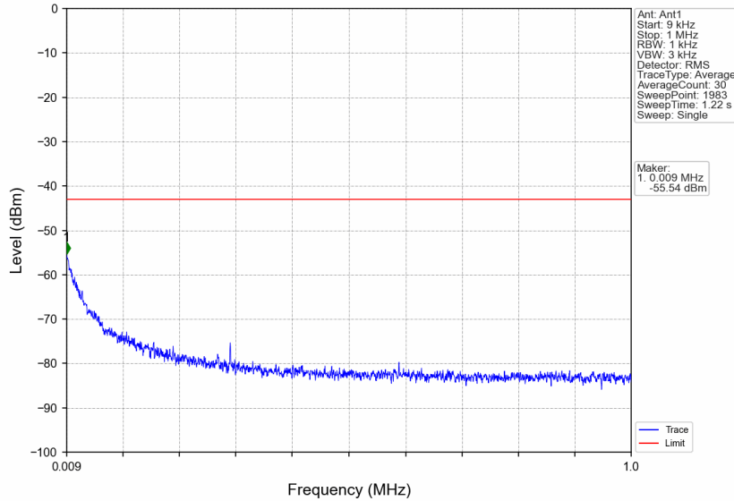
n5_30kHz_SISO_NTNV_10MHz_DFT-s-OFDM QPSK_844MHz_Edge_1RB_Right
