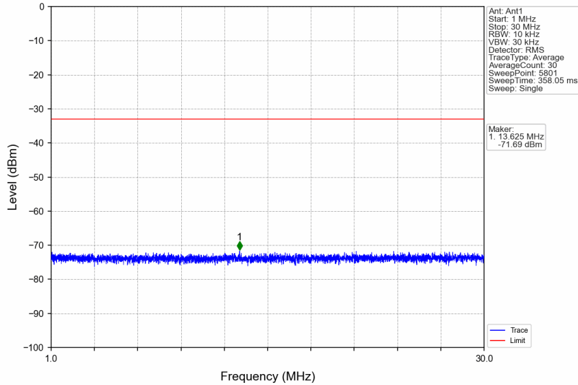
n5_15kHz_SISO_NTNV_20MHz_DFT-s-OFDM_QPSK_836.5MHz_Edge_1RB_Left
