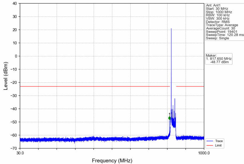
n5_15kHz_SISO_NTNV_20MHz_DFT-s-OFDM_QPSK_836.5MHz_Edge_1RB_Left
