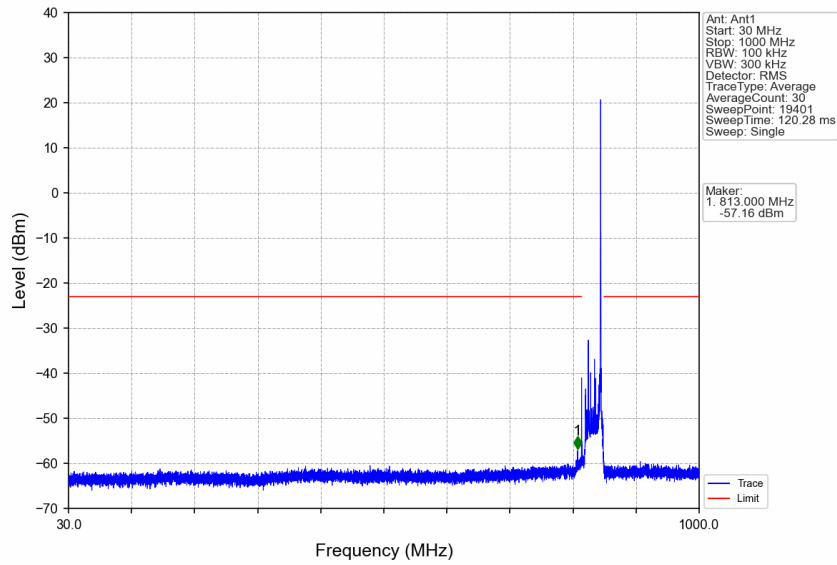
n5_15kHz_SISO_NTNV_20MHz_DFT-s-OFDM QPSK_839MHz_Edge_1RB_Right
