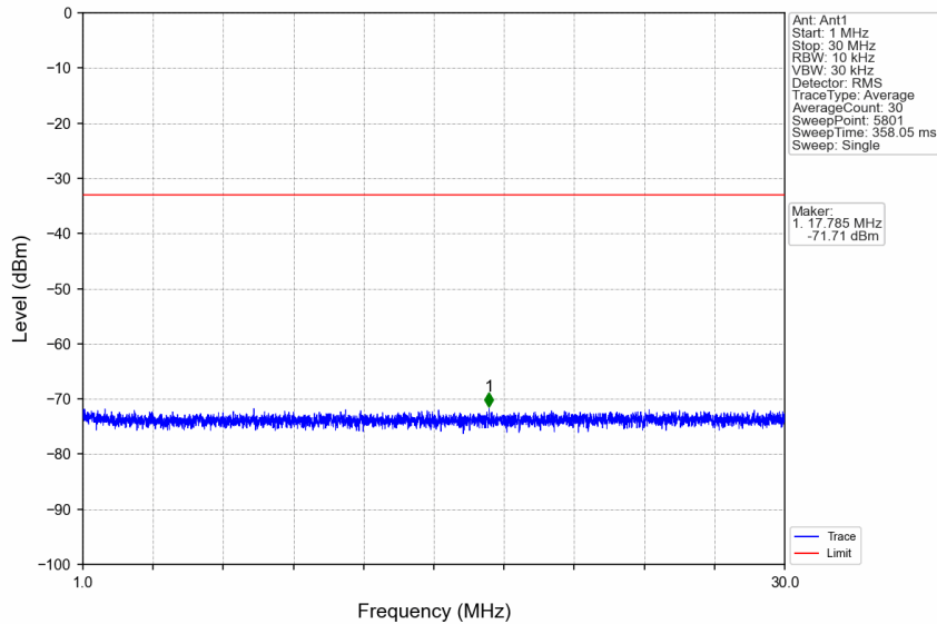
n5_15kHz_SISO_NTNV_20MHz_DFT-s-OFDM QPSK_839MHz_Edge_1RB_Right
