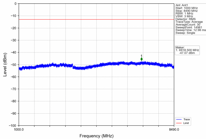
n5_30kHz_SISO_NTNV_10MHz_DFT-s-OFDM QPSK_844MHz_Edge_1RB_Right
