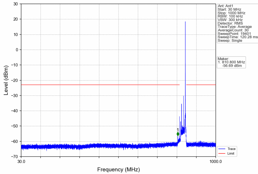
n5_15kHz_SISO_NTNV_20MHz_CP-OFDM QPSK_839MHz_Edge_1RB_Right
