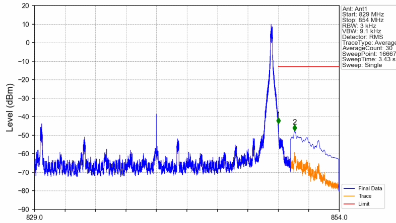
n5_15kHz_SISO_NTNV_20MHz_DFT-s-OFDM QPSK_839MHz_Edge_1RB_Right
