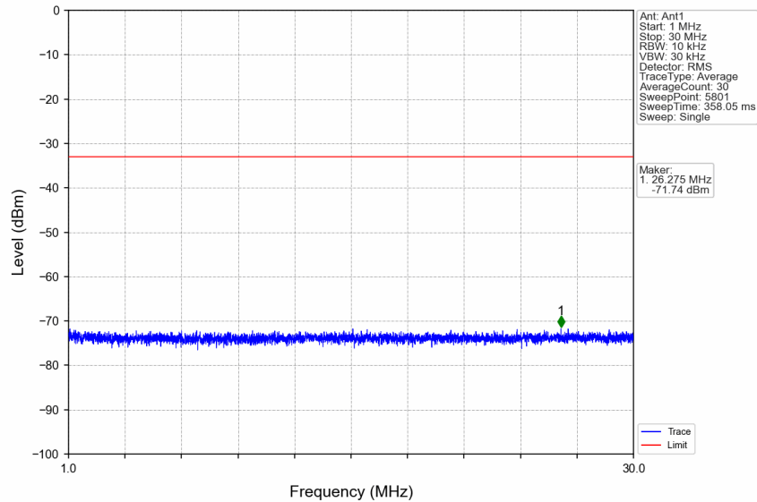
n5_15kHz_SISO_NTNV_15MHz_CP-OFDM QPSK_841.5MHz_Edge_1RB_Right
