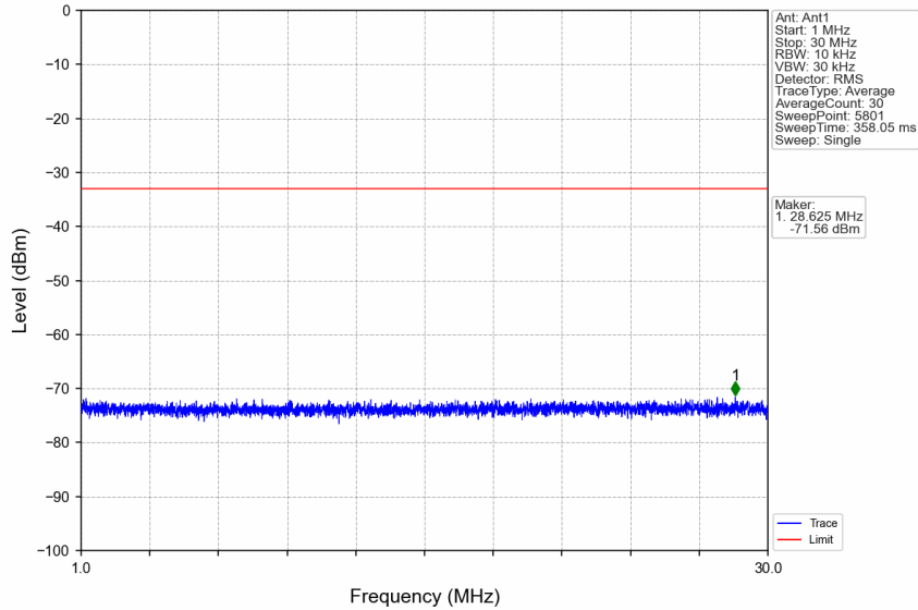
n5_30kHz_SISO_NTNV_10MHz_DFT-s-OFDM PI/2 BPSK_829MHz_Edge_1RB_Left
