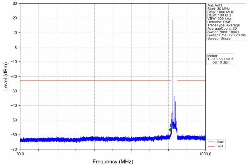
n5_15kHz_SISO_NTNV_15MHz_CP-OFDM QPSK_836.5MHz_Edge_1RB_Left
