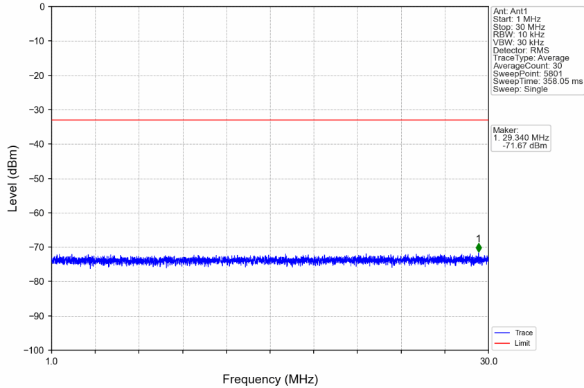
n5_15kHz_SISO_NTNV_20MHz_CP-OFDM QPSK_836.5MHz_Edge_1RB_Left
