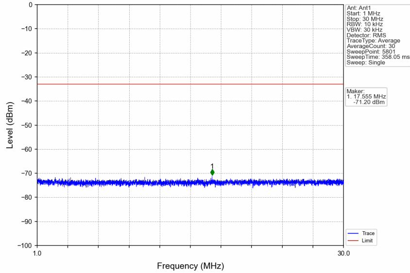
n5_30kHz_SISO_NTNV_10MHz_DFT-s-OFDM QPSK_829MHz_Edge_1RB_Left
