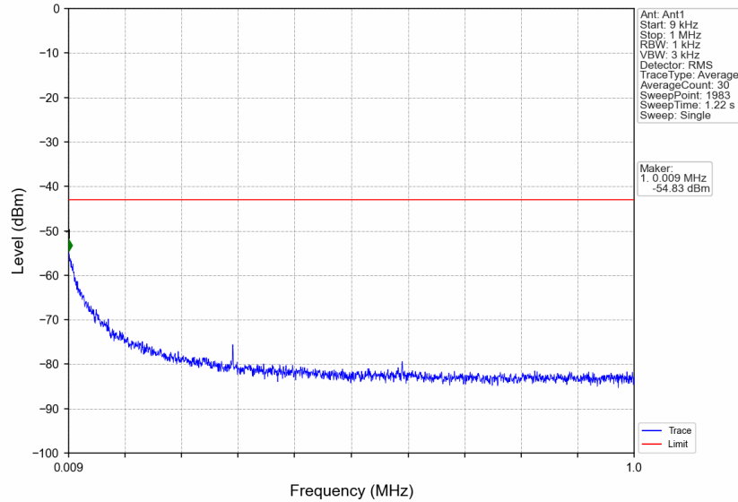
n5_15kHz_SISO_NTNV_15MHz_CP-OFDM QPSK_841.5MHz_Edge_1RB_Right
