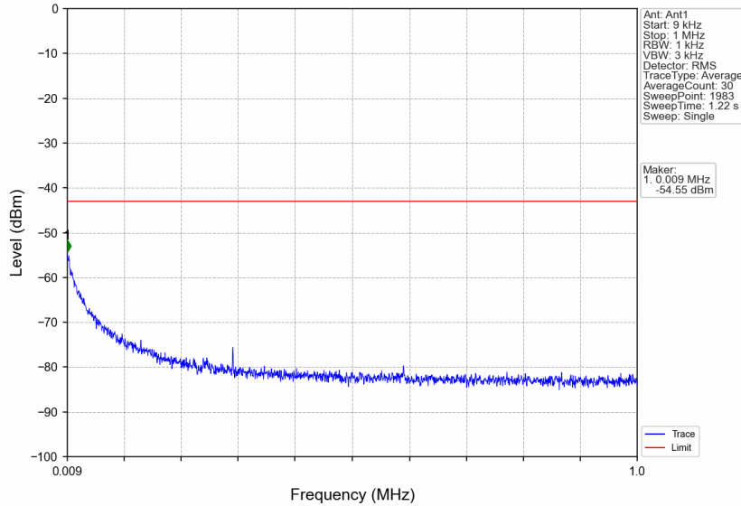
n5_15kHz_SISO_NTNV_20MHz_DFT-s-OFDM QPSK_839MHz_Edge_1RB_Right
