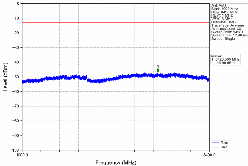
n5_15kHz_SISO_NTNV_15MHz_CP-OFDM QPSK_841.5MHz_Edge_1RB_Right
