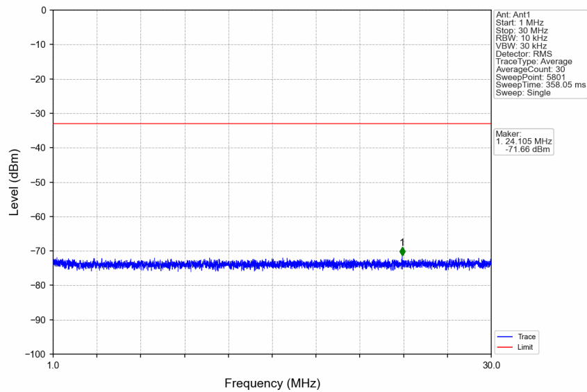
n5_30kHz_SISO_NTNV_10MHz_DFT-s-OFDM_QPSK_836.5MHz_Edge_1RB_Left
