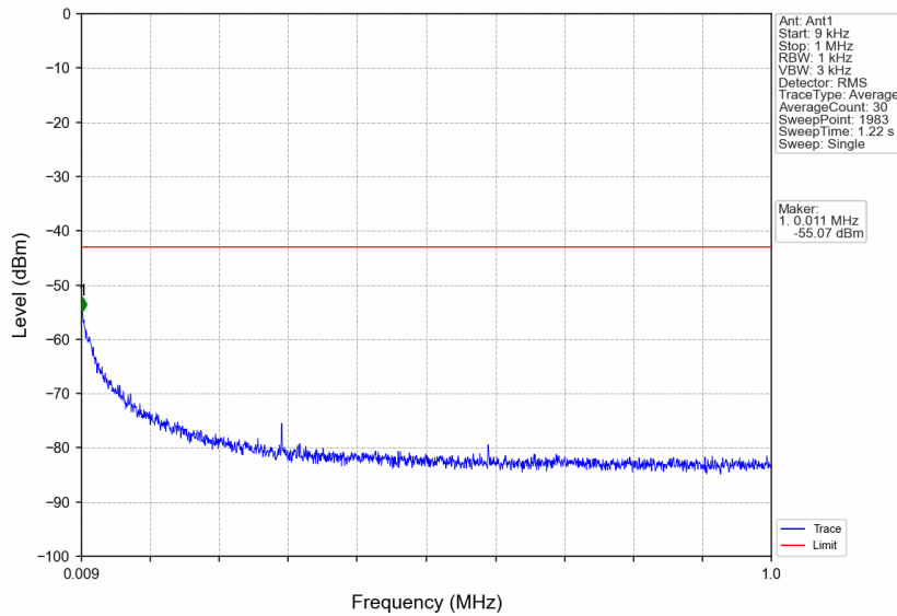
n5_15kHz_SISO_NTNV_10MHz_DFT-s-OFDM PI/2 BPSK_844MHz_Edge_1RB_Right
