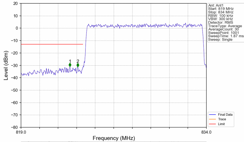
n5_15kHz_SISO_NTNV_10MHz_CP-OFDM QPSK_829MHz_Outer_Full
