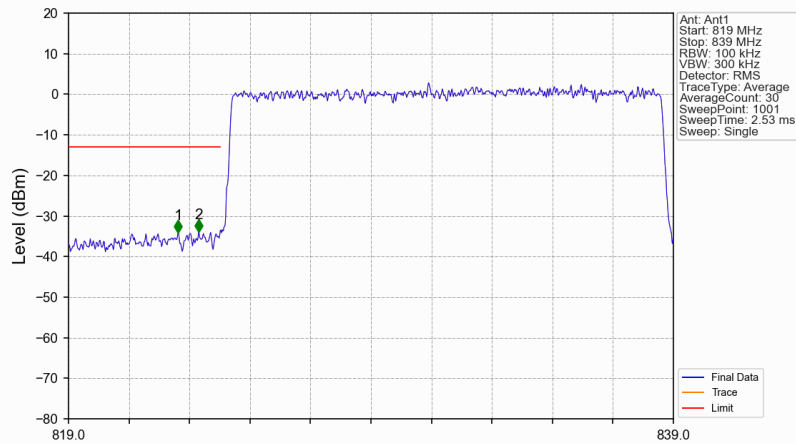
n5_15kHz_SISO_NTNV_15MHz_CP-OFDM QPSK_831.5MHz_Outer_Full
