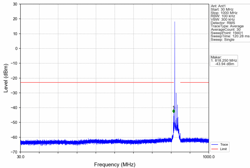
n5_15kHz_SISO_NTNV_15MHz_CP-OFDM QPSK_831.5MHz_Edge_1RB_Left
