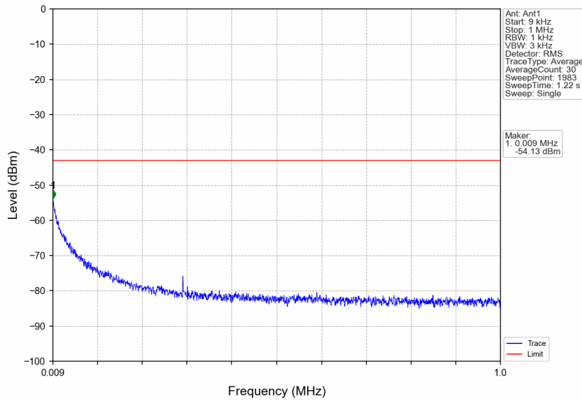
n5_15kHz_SISO_NTNV_15MHz_DFT-s-OFDM QPSK_841.5MHz_Edge_1RB_Right
