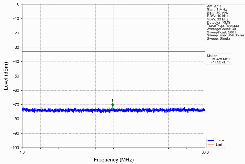
n5_15kHz_SISO_NTNV_10MHz_CP-OFDM QPSK_836.5MHz_Edge_1RB_Left
