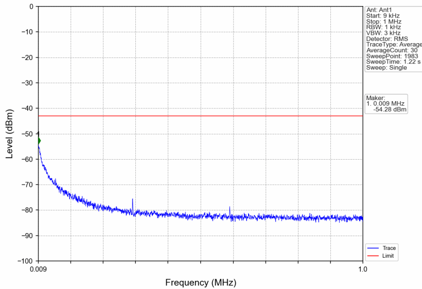
n5_15kHz_SISO_NTNV_15MHz_DFT-s-OFDM PI/2 BPSK_841.5MHz_Edge_1RB_Right
