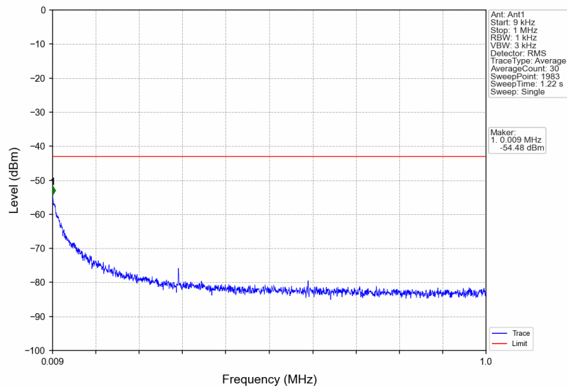
n5_15kHz_SISO_NTNV_10MHz_DFT-s-OFDM_QPSK_844MHz_Edge_1RB_Right
