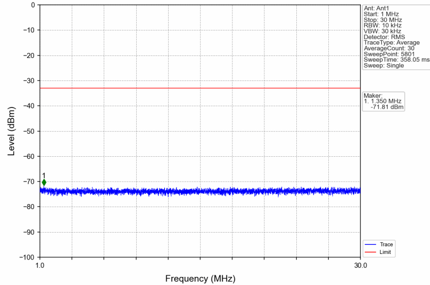
n5_15kHz_SISO_NTNV_10MHz_CP-OFDM QPSK_829MHz_Edge_1RB_Left
