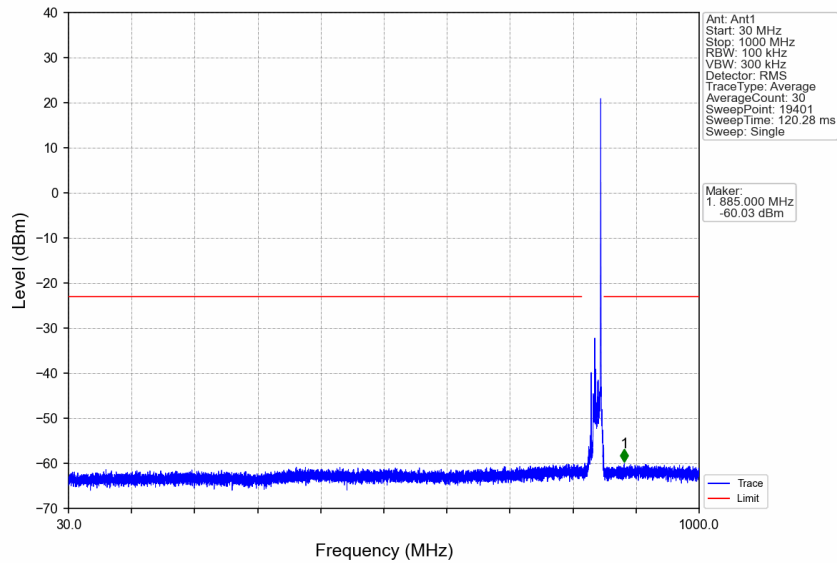
n5_15kHz_SISO_NTNV_10MHz_DFT-s-OFDM QPSK_844MHz_Edge_1RB_Right
