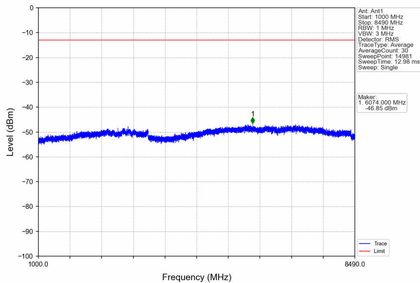
n5_15kHz_SISO_NTNV_10MHz_CP-OFDM QPSK_844MHz_Edge_1RB_Right
