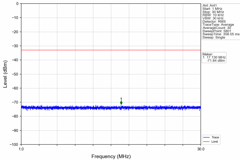
n5_15kHz_SISO_NTNV_15MHz_CP-OFDM QPSK_831.5MHz_Edge_1RB_Left
