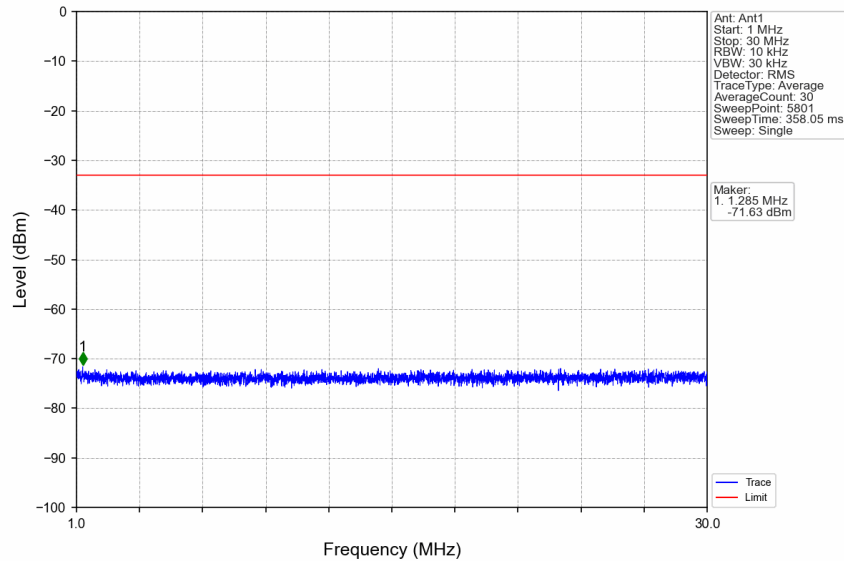
n5_15kHz_SISO_NTNV_10MHz_CP-OFDM_QPSK_844MHz_Edge_1RB_Right
