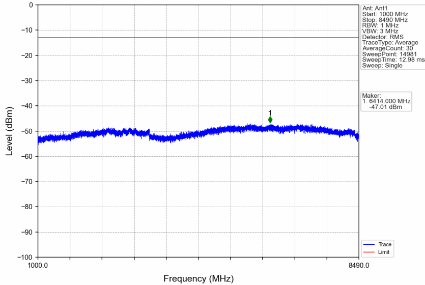
n5_15kHz_SISO_NTNV_15MHz_CP-OFDM QPSK_831.5MHz_Outer_Full
