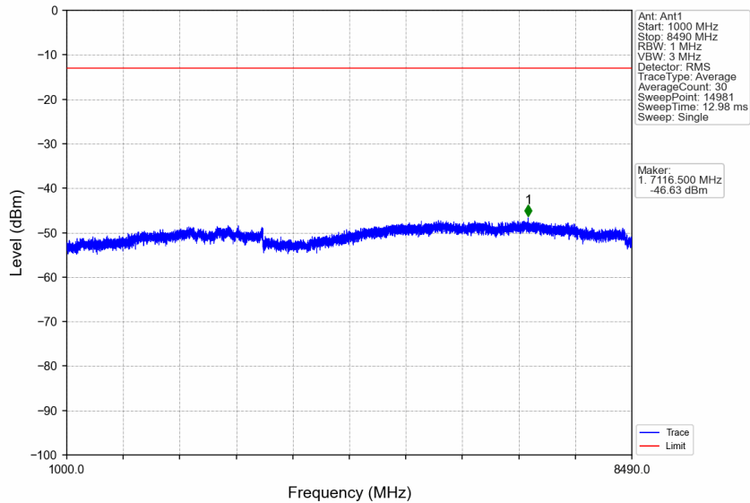
n5_15kHz_SISO_NTNV_10MHz_DFT-s-OFDM QPSK_844MHz_Edge_1RB_Right
