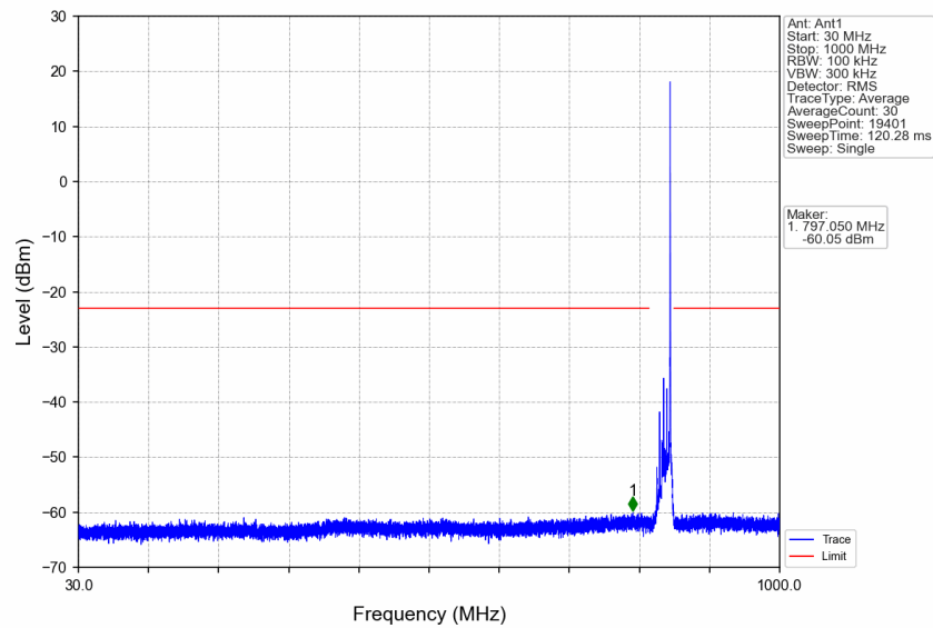
n5_15kHz_SISO_NTNV_10MHz_CP-OFDM QPSK_844MHz_Edge_1RB_Right
