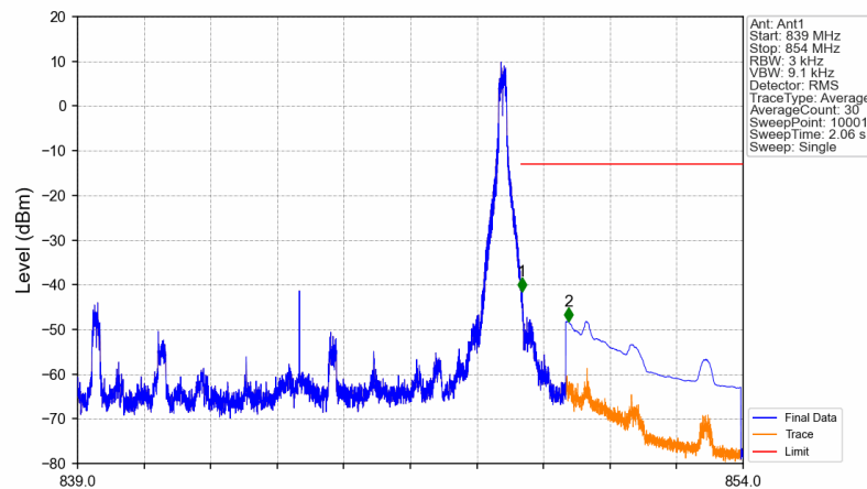
n5_15kHz_SISO_NTNV_10MHz_DFT-s-OFDM QPSK_844MHz_Edge_1RB_Right
