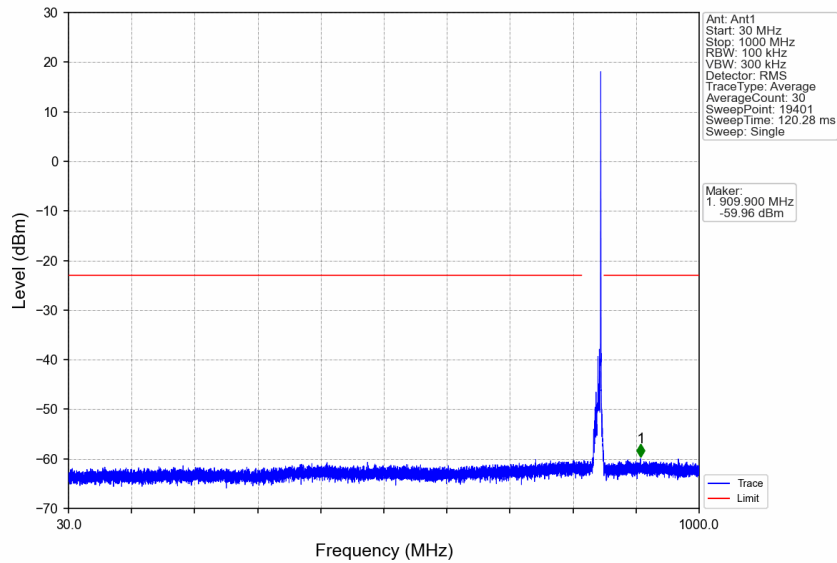
n5_15kHz_SISO_NTNV_5MHz_CP-OFDM QPSK_846.5MHz_Edge_1RB_Right
