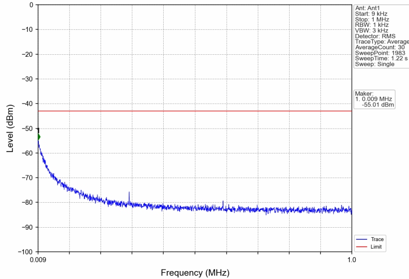
n5_15kHz_SISO_NTNV_10MHz_CP-OFDM_QPSK_844MHz_Edge_1RB_Right
