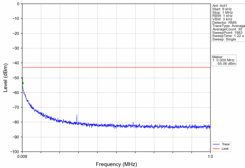
n5_15kHz_SISO_NTNV_5MHz_CP-OFDM QPSK_846.5MHz_Edge_1RB_Right
