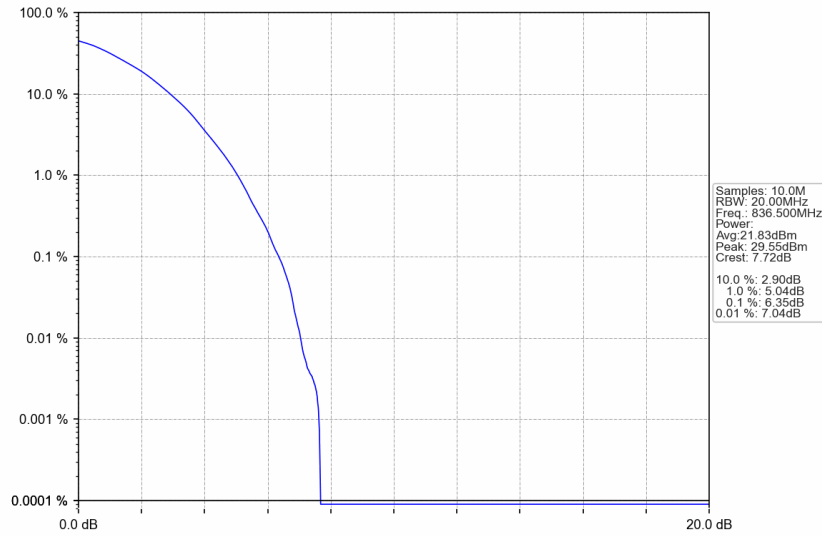
n5_30kHz_SISO_NTNV_20MHz_DFT-s-OFDM 64 QAM_836.5MHz_Outer_Full
