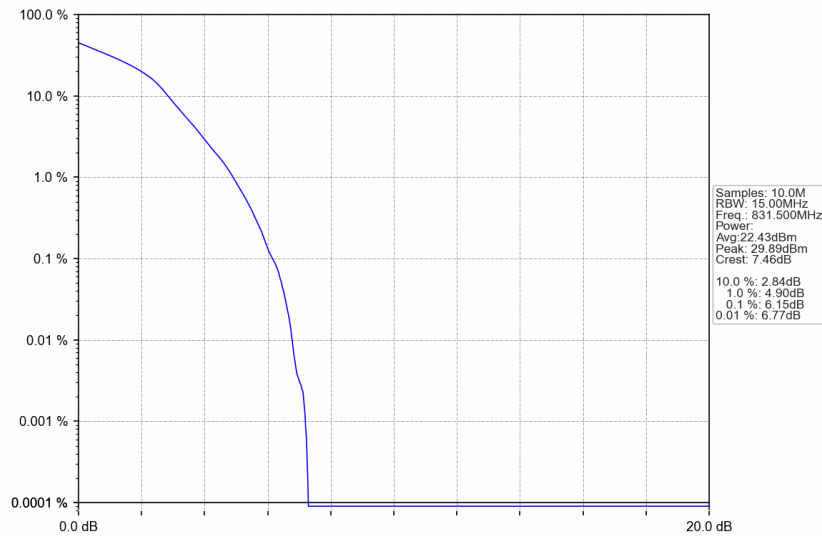
n5_30kHz_SISO_NTNV_15MHz_DFT-s-OFDM_16_QAM_831.5MHz_Outer_Full
