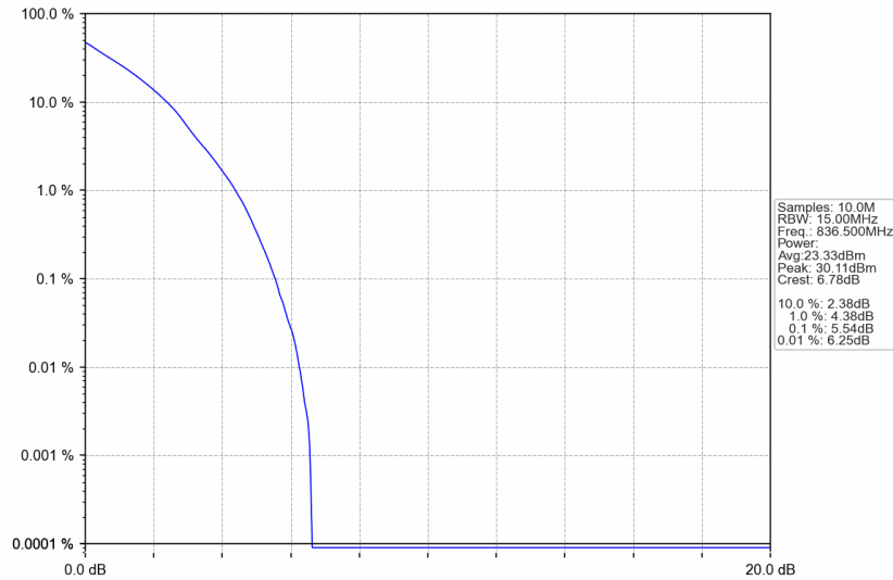
n5_30kHz_SISO_NTNV_15MHz_DFT-s-OFDM QPSK_836.5MHz_Outer_Full
