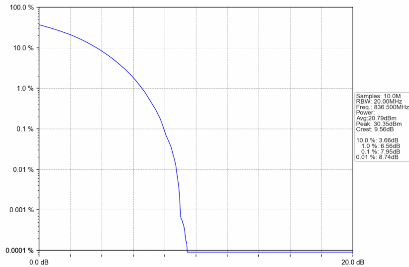
n5_30kHz_SISO_NTNV_20MHz_CP-OFDM 64 QAM_836.5MHz_Outer_Full
