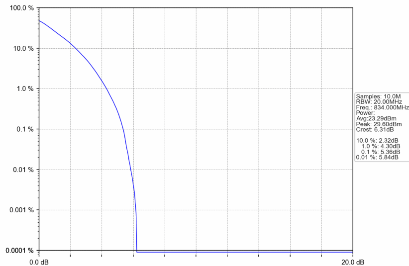
n5_30kHz_SISO_NTNV_20MHz_DFT-s-OFDM QPSK_834MHz_Outer_Full
