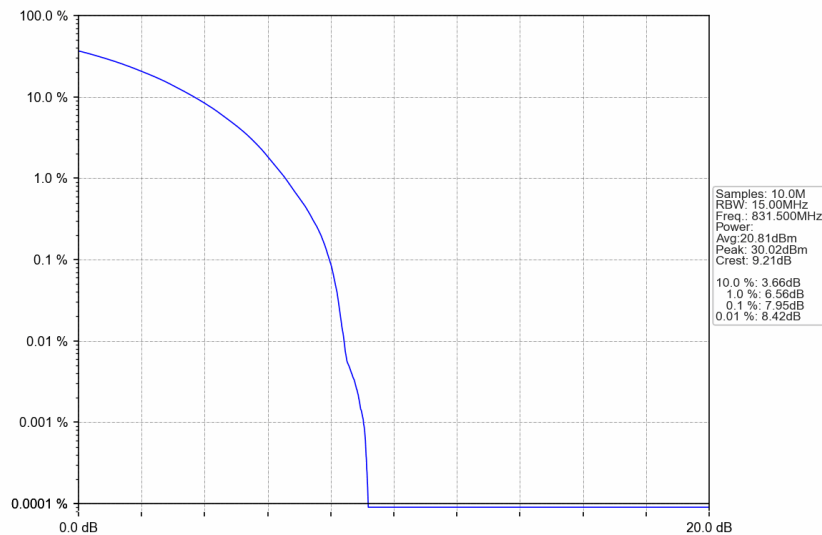
n5_30kHz_SISO_NTNV_15MHz_CP-OFDM 64 QAM_831.5MHz_Outer_Full
