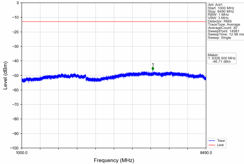
n5_15kHz_SISO_NTNV_5MHz_CP-OFDM QPSK_826.5MHz_Outer_Full
