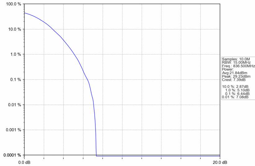
n5_30kHz_SISO_NTNV_15MHz_DFT-s-OFDM 64 QAM_836.5MHz_Outer_Full
