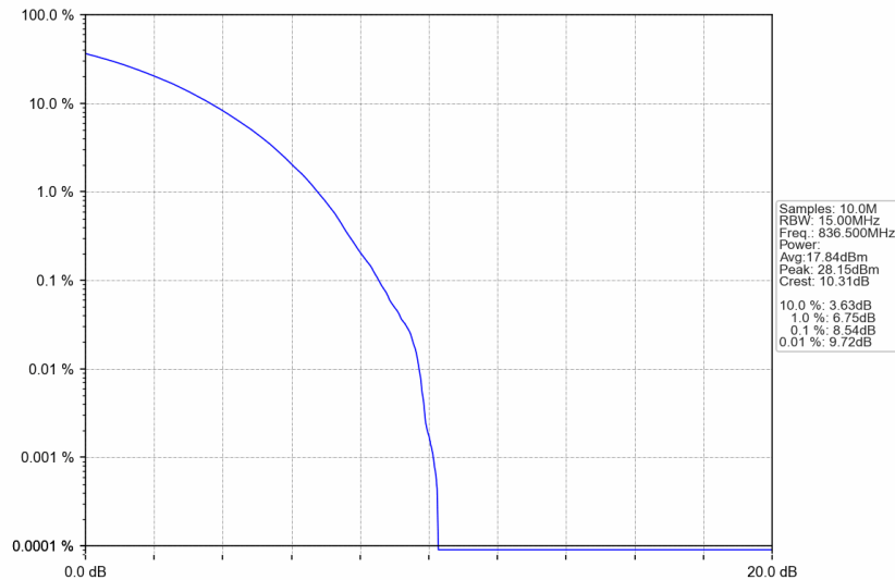
n5_30kHz_SISO_NTNV_15MHz_CP-OFDM 256 QAM_836.5MHz_Outer_Full
