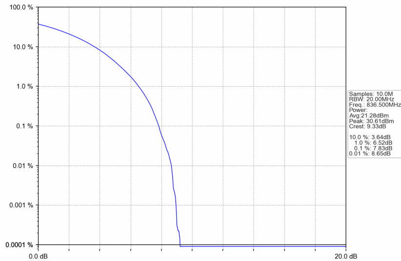
n5_30kHz_SISO_NTNV_20MHz_CP-OFDM QPSK_836.5MHz_Outer_Full
