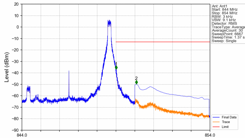
n5_15kHz_SISO_NTNV_5MHz_CP-OFDM QPSK_846.5MHz_Edge_1RB_Right
