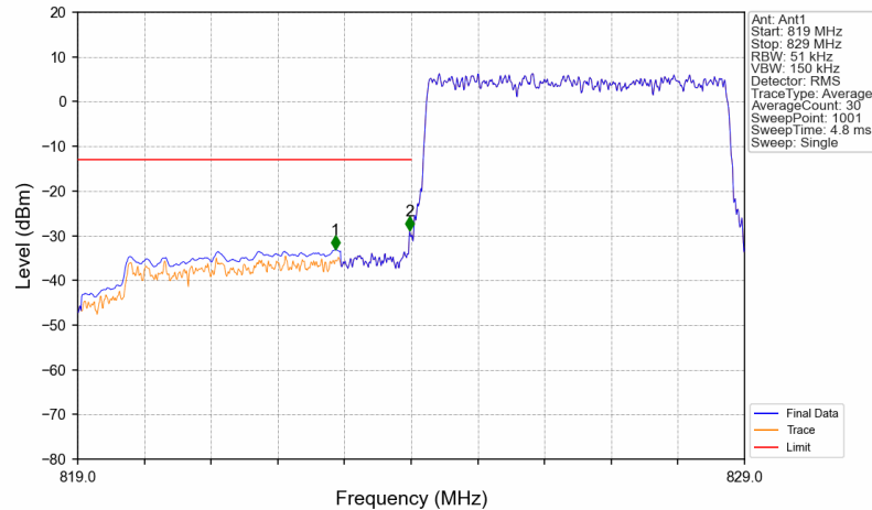
n5_15kHz_SISO_NTNV_5MHz_DFT-s-OFDM QPSK_826.5MHz_Outer_Full
