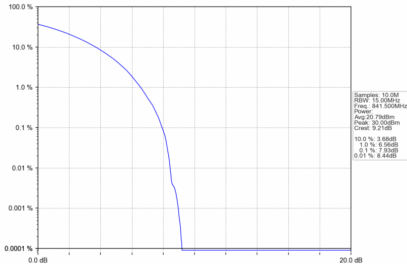
n5_30kHz_SISO_NTNV_15MHz_CP-OFDM 64 QAM_841.5MHz_Outer_Full
