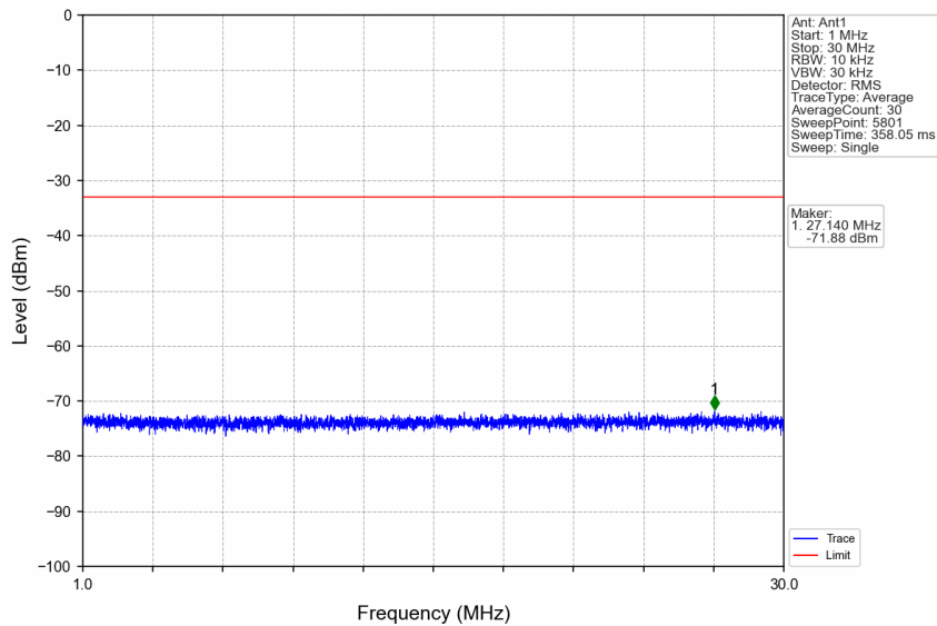
n5_15kHz_SISO_NTNV_5MHz_CP-OFDM QPSK_846.5MHz_Edge_1RB_Right
