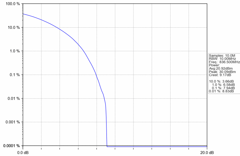
n5_30kHz_SISO_NTNV_10MHz_CP-OFDM 64 QAM_836.5MHz_Outer_Full
