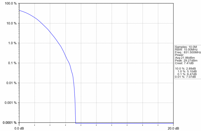
n5_30kHz_SISO_NTNV_15MHz_DFT-s-OFDM 64 QAM_831.5MHz_Outer_Full
