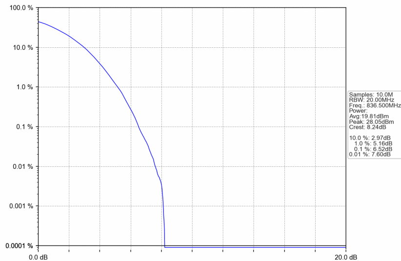
n5_30kHz_SISO_NTNV_20MHz_DFT-s-OFDM 256 QAM_836.5MHz_Outer_Full
