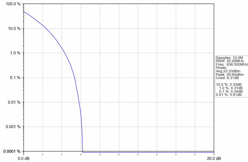
n5_30kHz_SISO_NTNV_20MHz_DFT-s-OFDM QPSK_836.5MHz_Outer_Full
