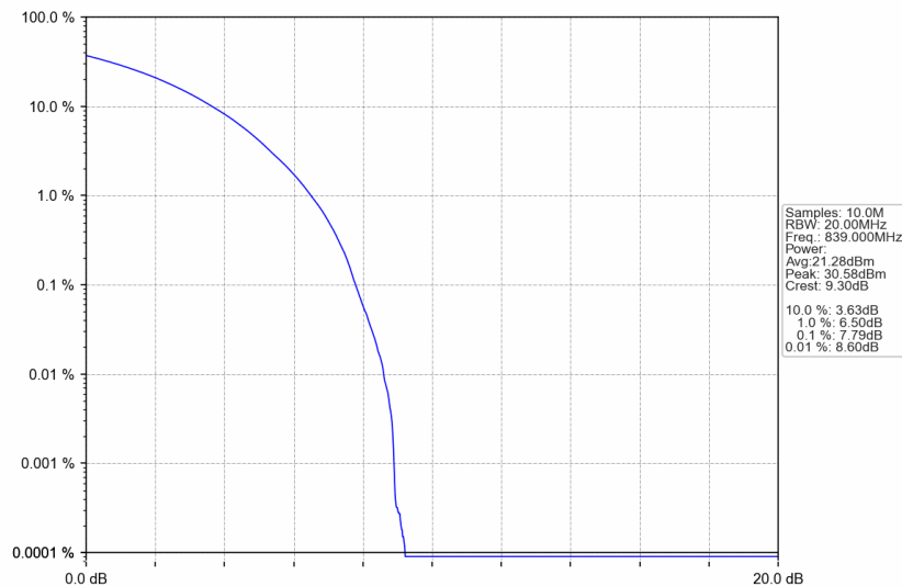
n5_30kHz_SISO_NTNV_20MHz_CP-OFDM QPSK_839MHz_Outer_Full
