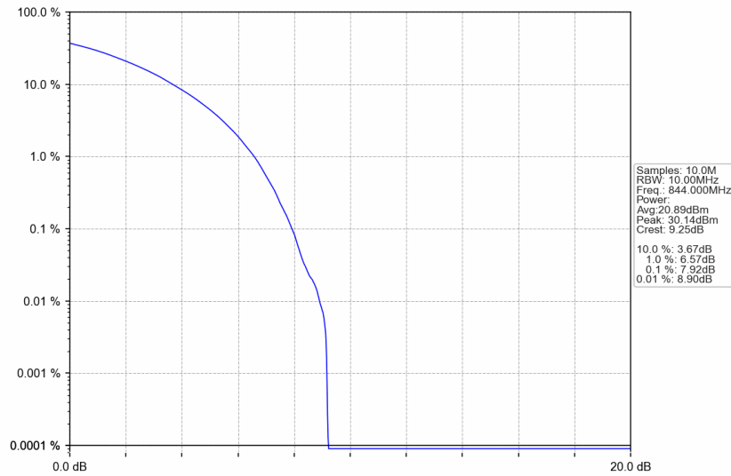
n5_30kHz_SISO_NTNV_10MHz_CP-OFDM 64 QAM_844MHz_Outer_Full
