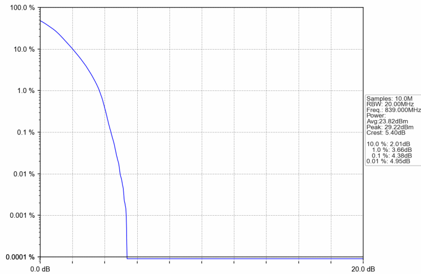
n5_30kHz_SISO_NTNV_20MHz_DFT-s-OFDM PI/2 BPSK_839MHz_Outer_Full
