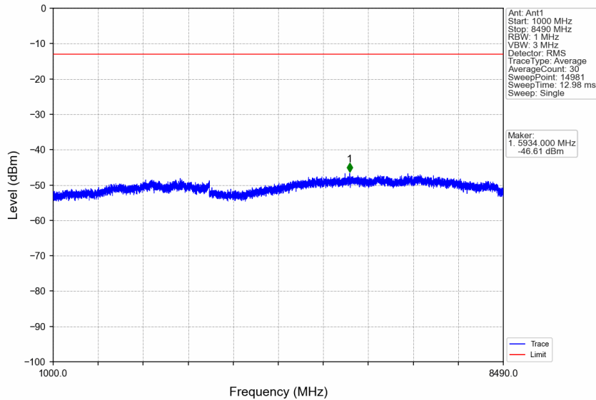
n5_15kHz_SISO_NTNV_5MHz_DFT-s-OFDM QPSK_846.5MHz_Edge_1RB_Right
