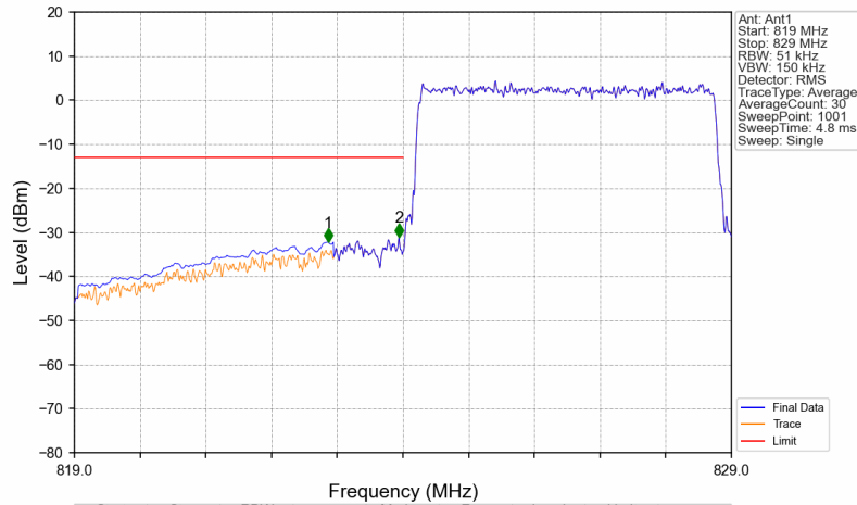
n5_15kHz_SISO_NTNV_5MHz_CP-OFDM QPSK_826.5MHz_Outer_Full
