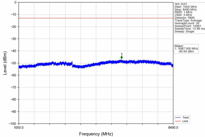
n5_15kHz_SISO_NTNV_5MHz_CP-OFDM QPSK_846.5MHz_Edge_1RB_Right
