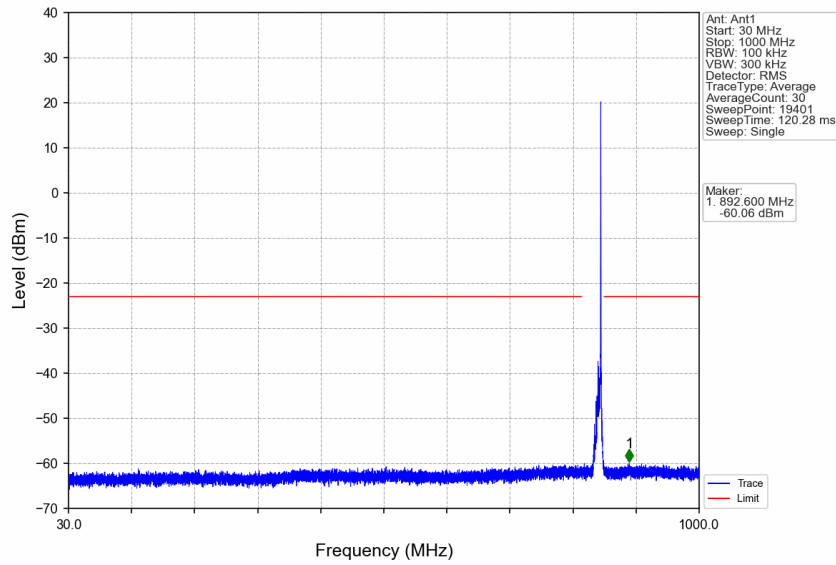
n5_15kHz_SISO_NTNV_5MHz_DFT-s-OFDM QPSK_846.5MHz_Edge_1RB_Right
