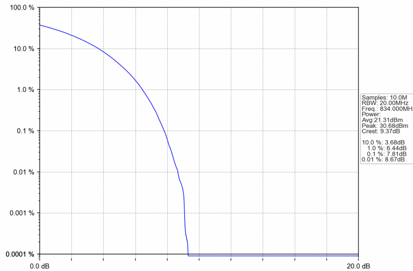
n5_30kHz_SISO_NTNV_20MHz_CP-OFDM 16 QAM_834MHz_Outer_Full
