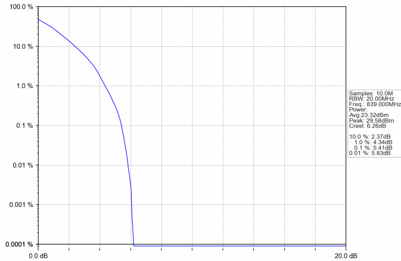
n5_30kHz_SISO_NTNV_20MHz_DFT-s-OFDM QPSK_839MHz_Outer_Full
