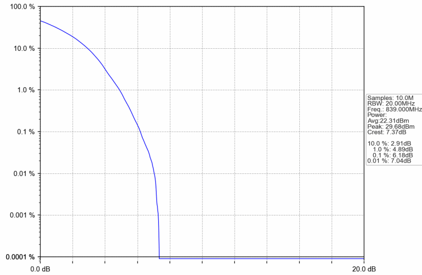
n5_30kHz_SISO_NTNV_20MHz_DFT-s-OFDM 16 QAM_839MHz_Outer_Full
