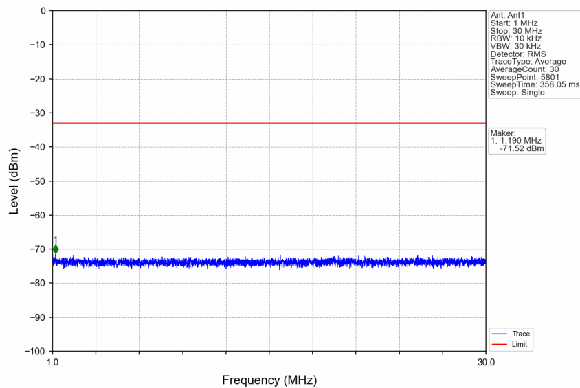
n5_15kHz_SISO_NTNV_5MHz_DFT-s-OFDM QPSK_846.5MHz_Edge_1RB_Right
