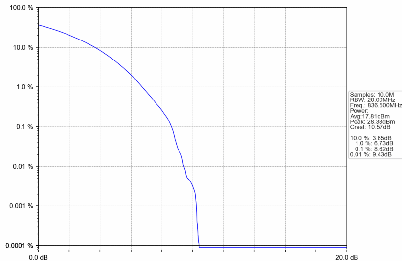
n5_30kHz_SISO_NTNV_20MHz_CP-OFDM 256 QAM_836.5MHz_Outer_Full
