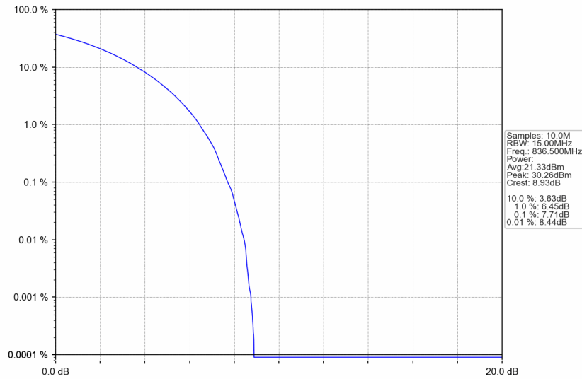
n5_30kHz_SISO_NTNV_15MHz_CP-OFDM 16 QAM_836.5MHz_Outer_Full
