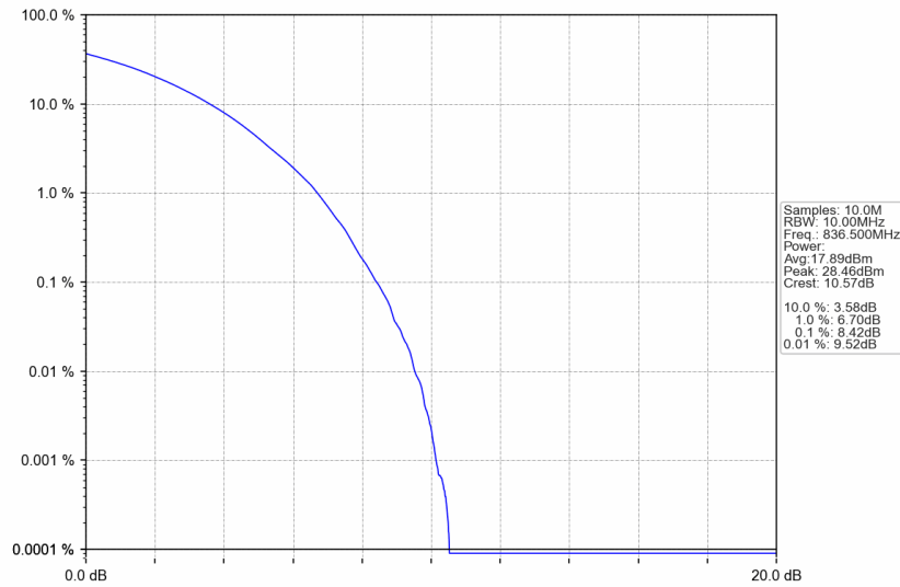
n5_30kHz_SISO_NTNV_10MHz_CP-OFDM 256 QAM_836.5MHz_Outer_Full
