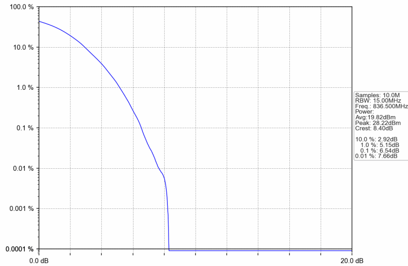
n5_30kHz_SISO_NTNV_15MHz_DFT-s-OFDM 256 QAM_836.5MHz_Outer_Full
