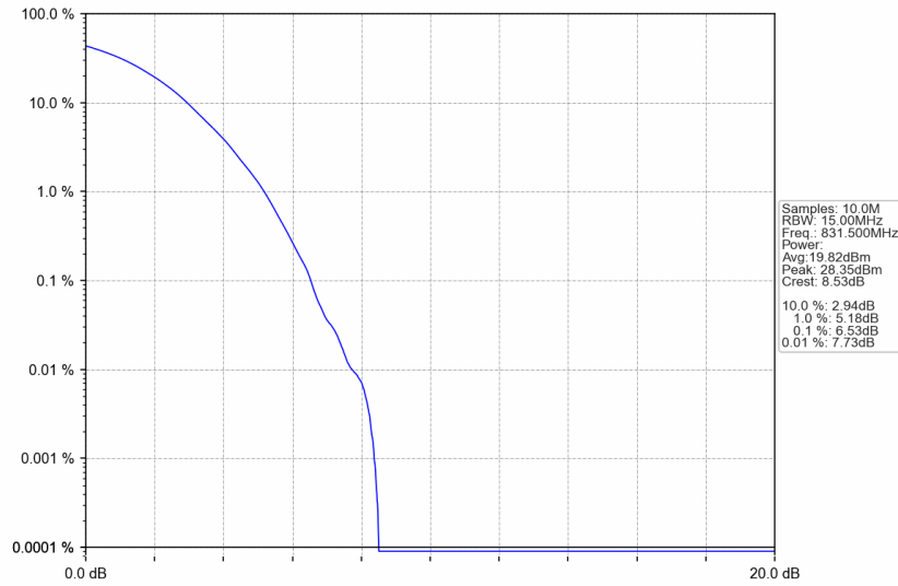
n5_30kHz_SISO_NTNV_15MHz_DFT-s-OFDM 256 QAM_831.5MHz_Outer_Full
