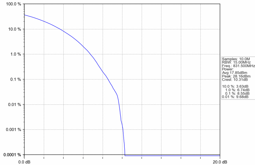
n5_30kHz_SISO_NTNV_15MHz_CP-OFDM 256 QAM_831.5MHz_Outer_Full
