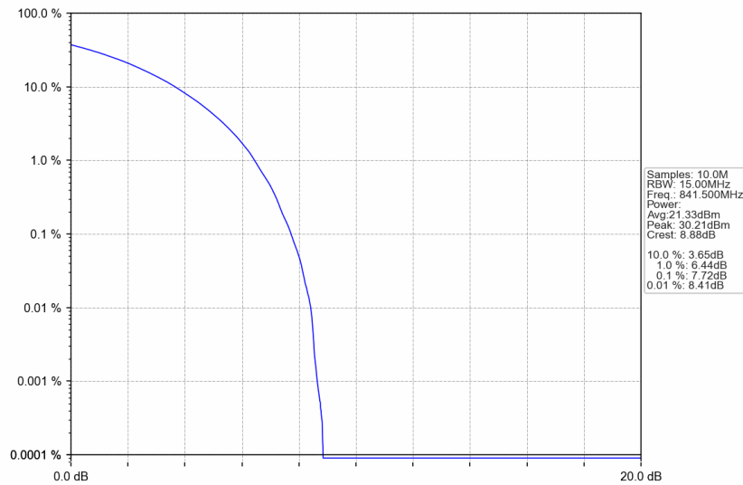
n5_30kHz_SISO_NTNV_15MHz_CP-OFDM 16 QAM_841.5MHz_Outer_Full
