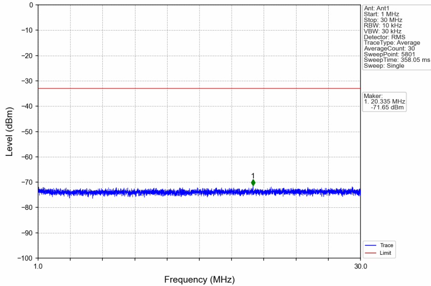
n5_15kHz_SISO_NTNV_5MHz_CP-OFDM QPSK_826.5MHz_Edge_1RB_Left
