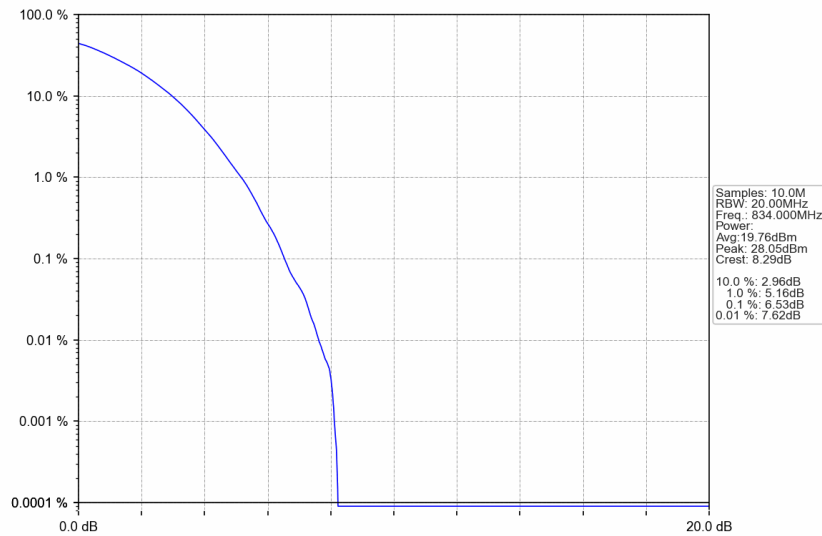
n5_30kHz_SISO_NTNV_20MHz_DFT-s-OFDM 256 QAM_834MHz_Outer_Full
