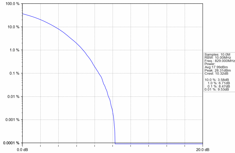
n5_30kHz_SISO_NTNV_10MHz_CP-OFDM 256 QAM_829MHz_Outer_Full
