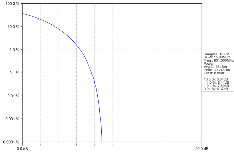
n5_30kHz_SISO_NTNV_15MHz_CP-OFDM 16 QAM_831.5MHz_Outer_Full
