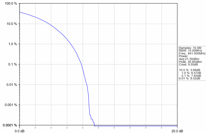
n5_30kHz_SISO_NTNV_15MHz_CP-OFDM QPSK_841.5MHz_Outer_Full
