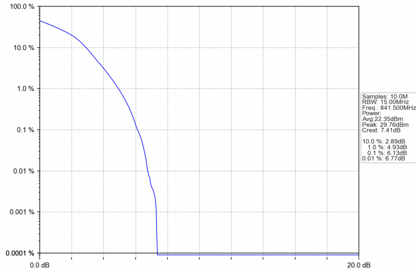
n5_30kHz_SISO_NTNV_15MHz_DFT-s-OFDM 16 QAM_841.5MHz_Outer_Full
