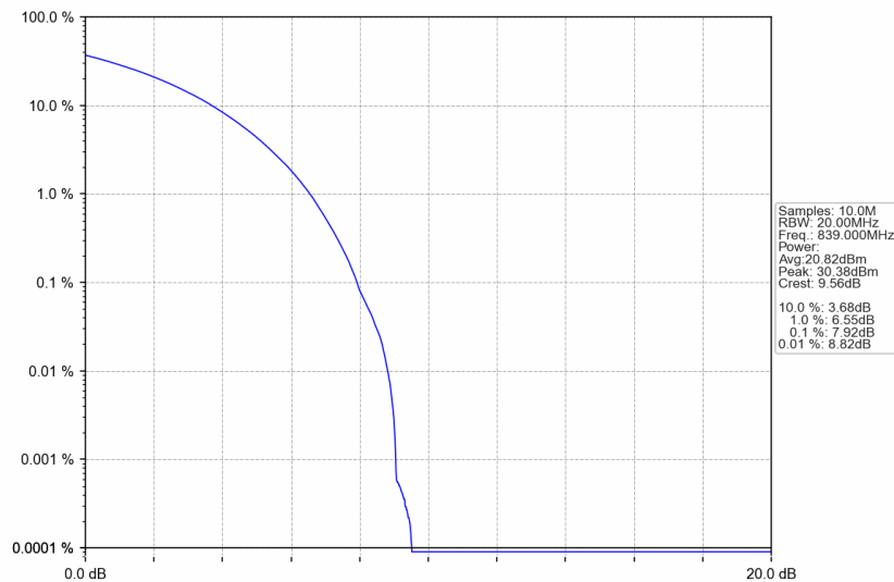
n5_30kHz_SISO_NTNV_20MHz_CP-OFDM 64 QAM_839MHz_Outer_Full
