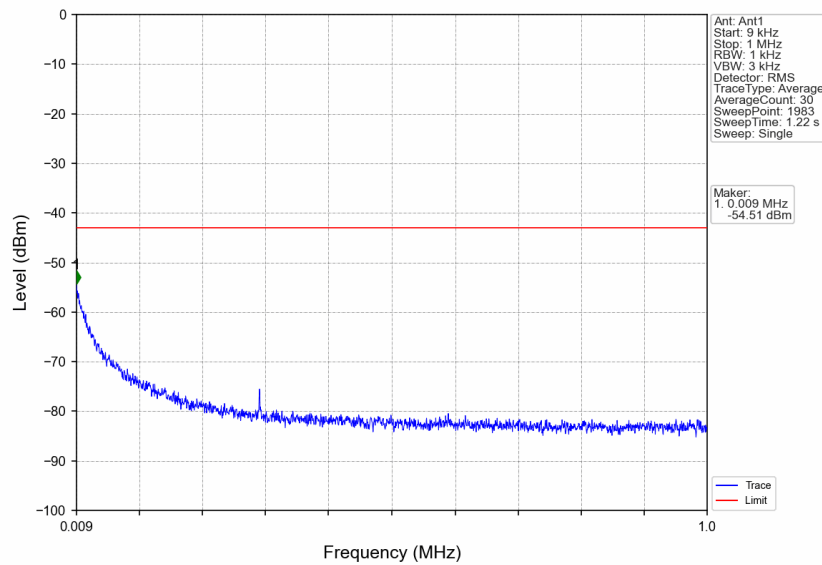
n5_15kHz_SISO_NTNV_5MHz_DFT-s-OFDM QPSK_846.5MHz_Edge_1RB_Right
