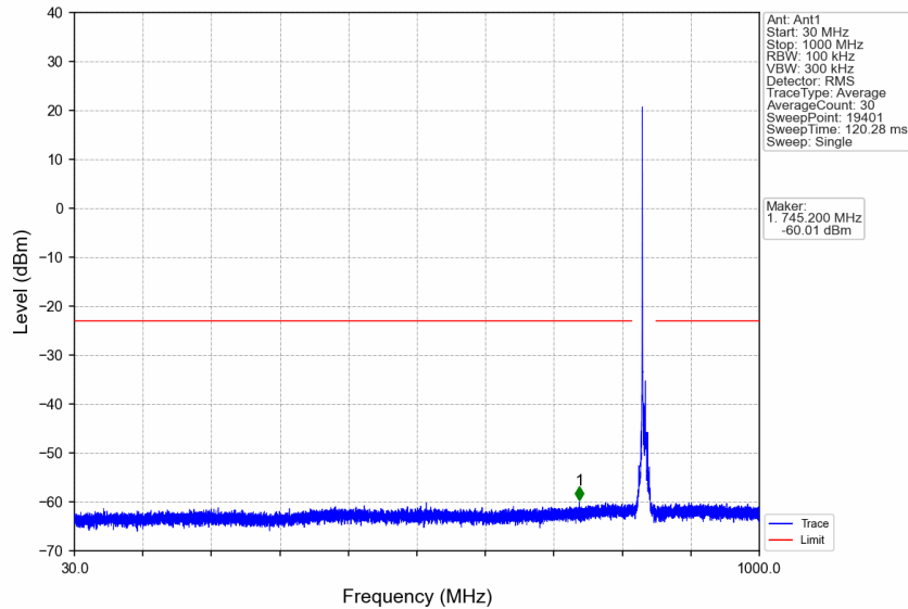
n5_15kHz_SISO_NTNV_5MHz_DFT-s-OFDM QPSK_836.5MHz_Edge_1RB_Left
