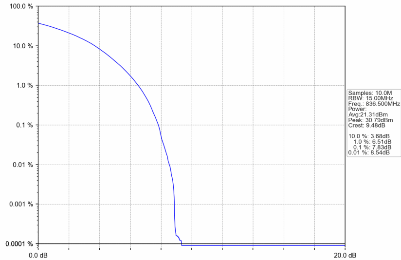
n5_30kHz_SISO_NTNV_15MHz_CP-OFDM QPSK_836.5MHz_Outer_Full
