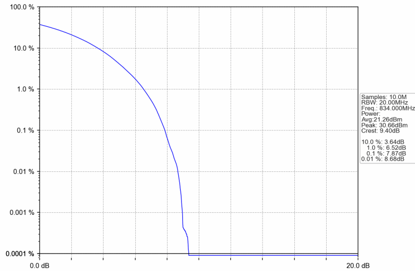
n5_30kHz_SISO_NTNV_20MHz_CP-OFDM QPSK_834MHz_Outer_Full
