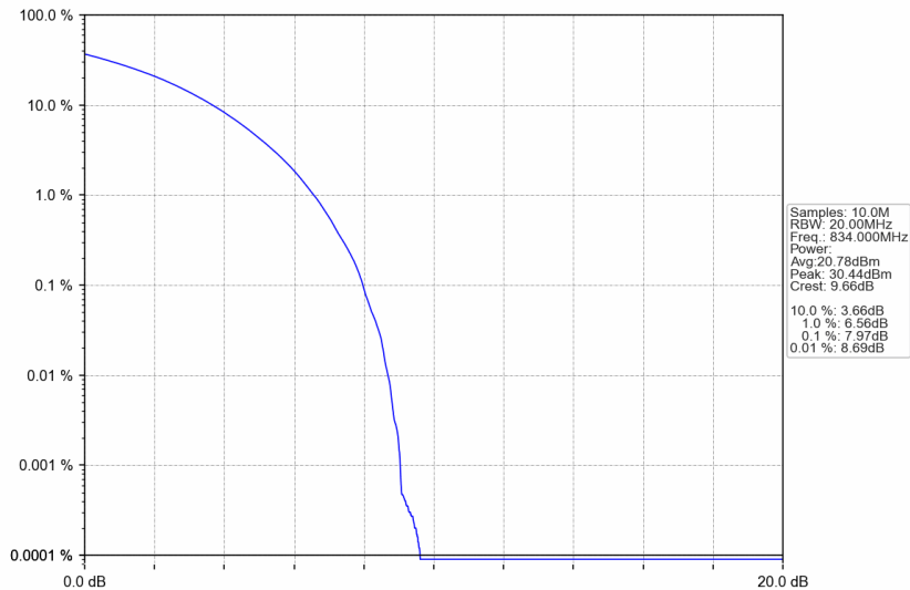
n5_30kHz_SISO_NTNV_20MHz_CP-OFDM 64 QAM_834MHz_Outer_Full
