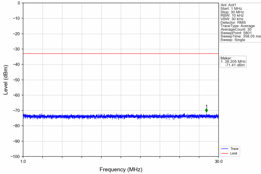
n5_15kHz_SISO_NTNV_5MHz_DFT-s-OFDM QPSK_836.5MHz_Edge_1RB_Left
