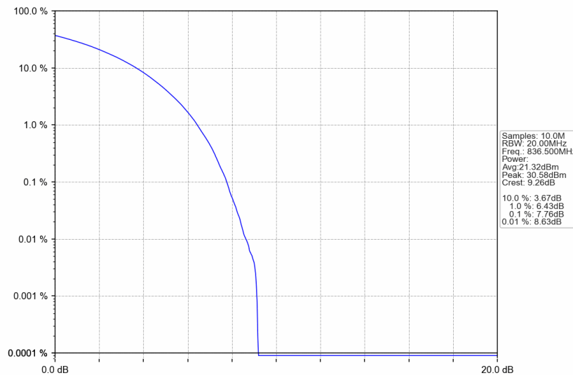
n5_30kHz_SISO_NTNV_20MHz_CP-OFDM 16 QAM_836.5MHz_Outer_Full
