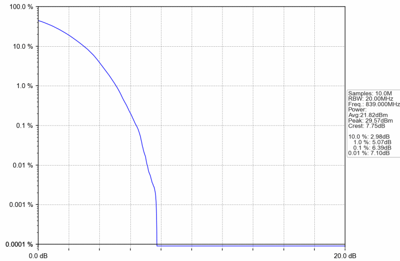
n5_30kHz_SISO_NTNV_20MHz_DFT-s-OFDM 64 QAM_839MHz_Outer_Full
