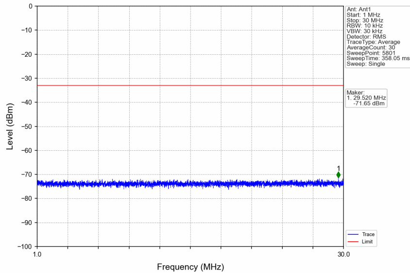
n5_15kHz_SISO_NTNV_5MHz_DFT-s-OFDM QPSK_826.5MHz_Edge_1RB_Left
