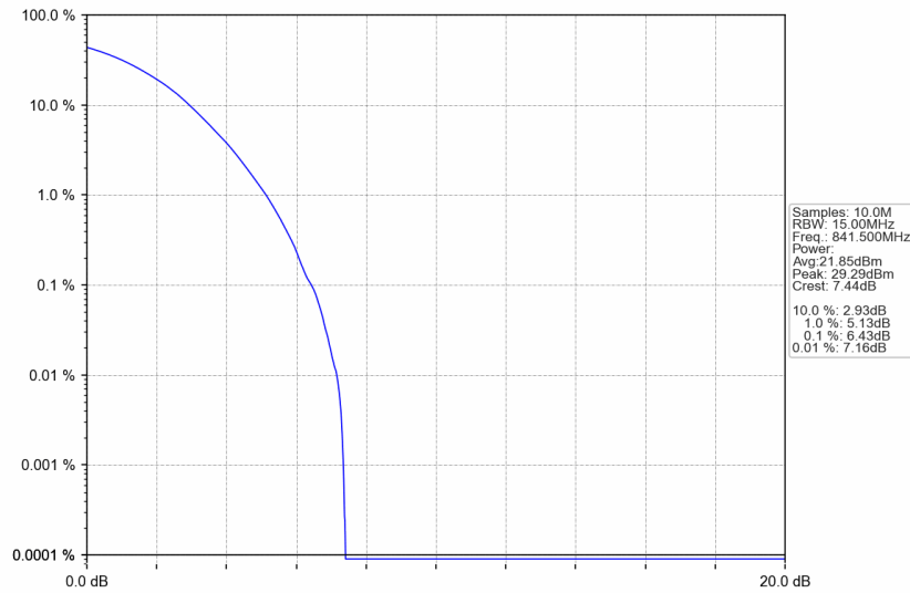
n5_30kHz_SISO_NTNV_15MHz_DFT-s-OFDM 64 QAM_841.5MHz_Outer_Full
