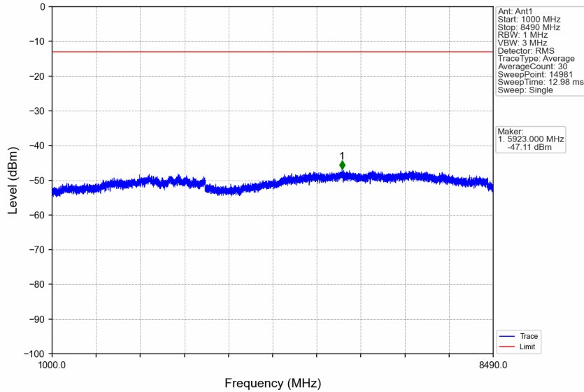
n5_15kHz_SISO_NTNV_5MHz_DFT-s-OFDM QPSK_826.5MHz_Outer_Full
