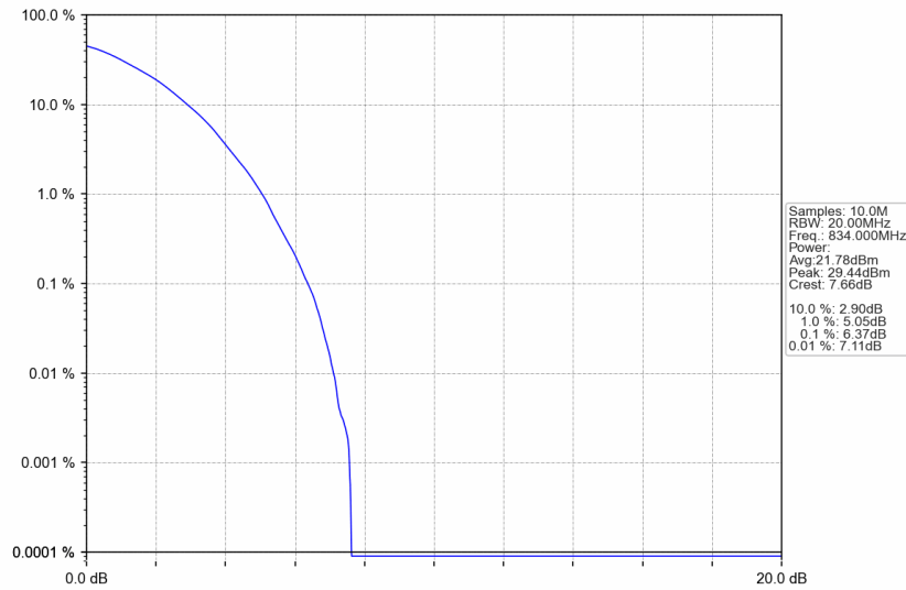
n5_30kHz_SISO_NTNV_20MHz_DFT-s-OFDM 64 QAM_834MHz_Outer_Full
