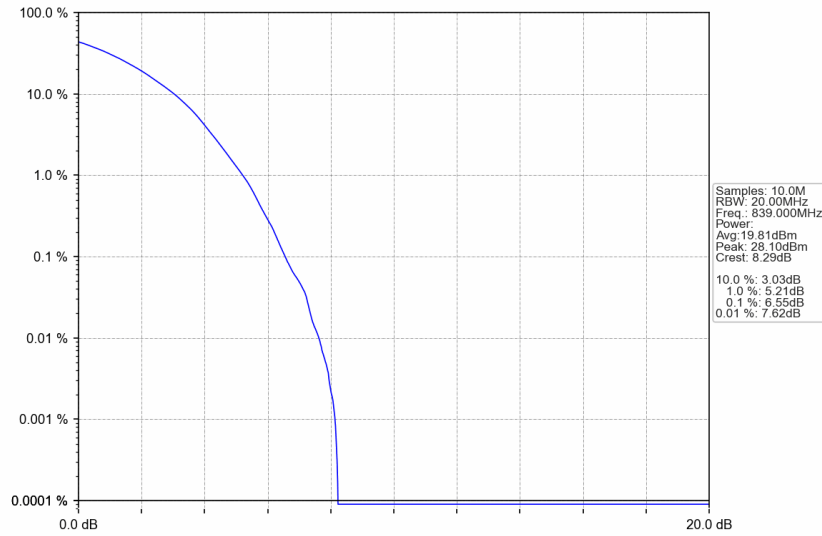
n5_30kHz_SISO_NTNV_20MHz_DFT-s-OFDM 256 QAM_839MHz_Outer_Full
