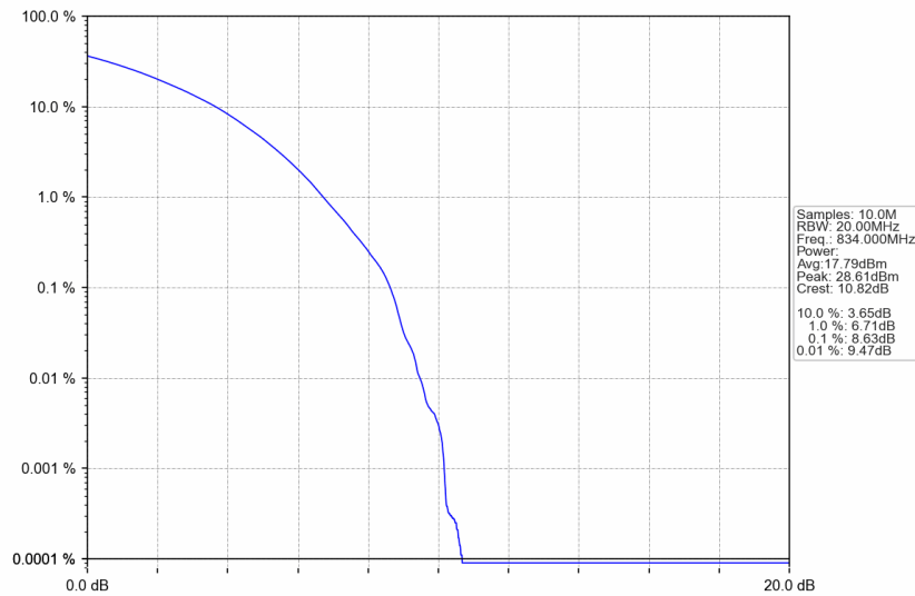
n5_30kHz_SISO_NTNV_20MHz_CP-OFDM 256 QAM_834MHz_Outer_Full
