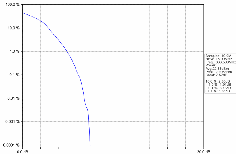
n5_30kHz_SISO_NTNV_15MHz_DFT-s-OFDM_16_QAM_836.5MHz_Outer_Full
