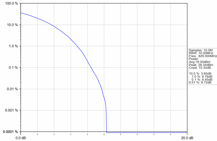
n5_15kHz_SISO_NTNV_10MHz_CP-OFDM 256 QAM_829MHz_Outer_Full
