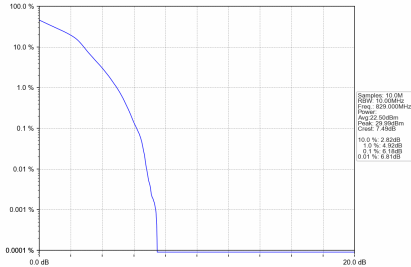
n5_15kHz_SISO_NTNV_10MHz_DFT-s-OFDM 16 QAM_829MHz_Outer_Full
