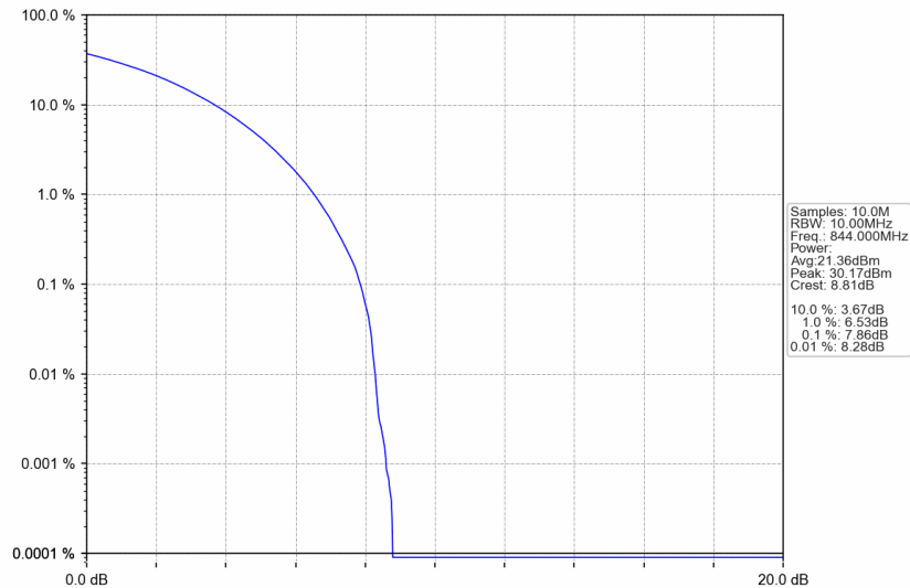
n5_30kHz_SISO_NTNV_10MHz_CP-OFDM QPSK_844MHz_Outer_Full
