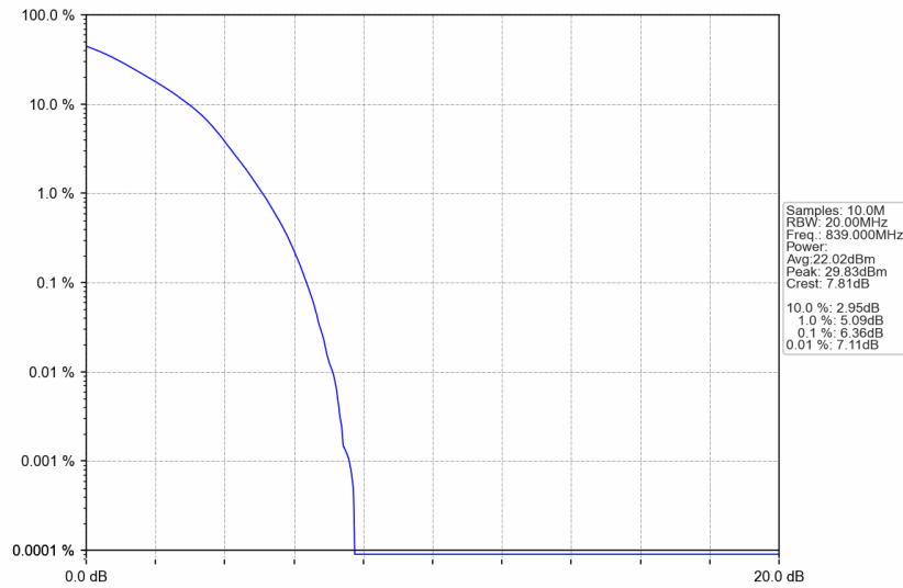
n5_15kHz_SISO_NTNV_20MHz_DFT-s-OFDM 64 QAM_839MHz_Outer_Full
