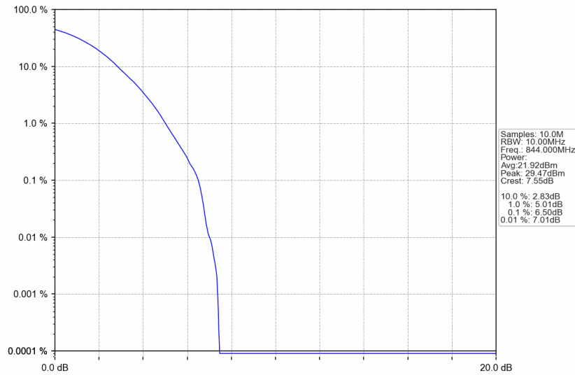
n5_30kHz_SISO_NTNV_10MHz_DFT-s-OFDM 64 QAM_844MHz_Outer_Full
