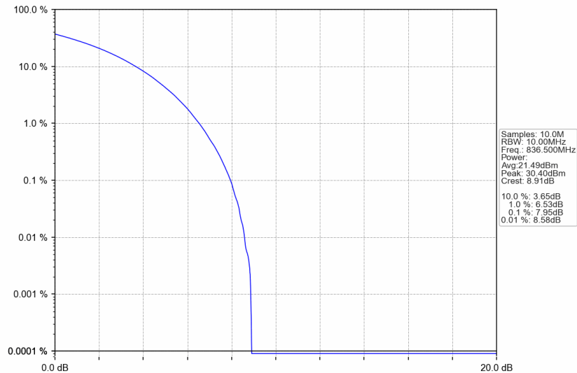
n5_15kHz_SISO_NTNV_10MHz_CP-OFDM 16 QAM_836.5MHz_Outer_Full
