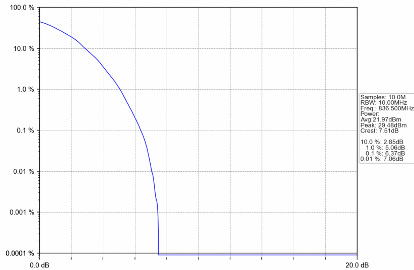
n5_15kHz_SISO_NTNV_10MHz_DFT-s-OFDM 64 QAM_836.5MHz_Outer_Full
