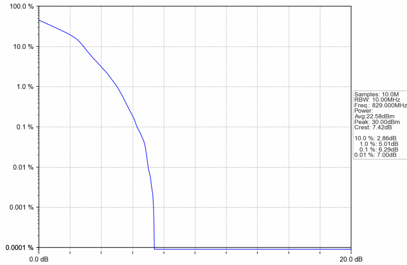
n5_30kHz_SISO_NTNV_10MHz_DFT-s-OFDM 16 QAM_829MHz_Outer_Full
