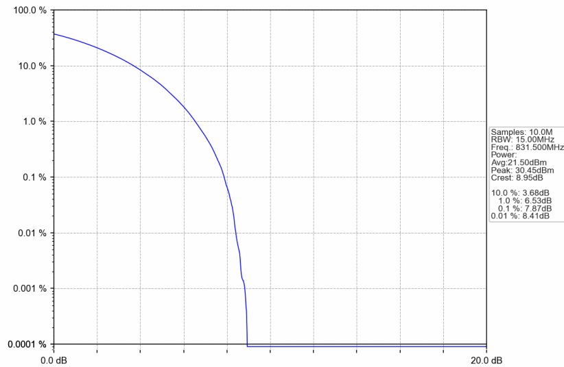
n5_15kHz_SISO_NTNV_15MHz_CP-OFDM 16 QAM_831.5MHz_Outer_Full
