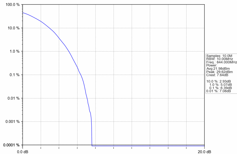
n5_15kHz_SISO_NTNV_10MHz_DFT-s-OFDM 64 QAM_844MHz_Outer_Full
