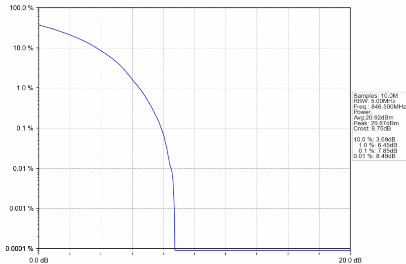
n5_15kHz_SISO_NTV_5MHz_CP-OFDM 64 QAM_846.5MHz_Outer_Full
