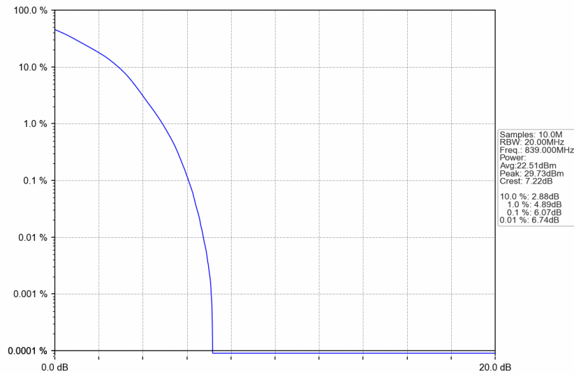
n5_15kHz_SISO_NTNV_20MHz_DFT-s-OFDM 16 QAM_839MHz_Outer_Full
