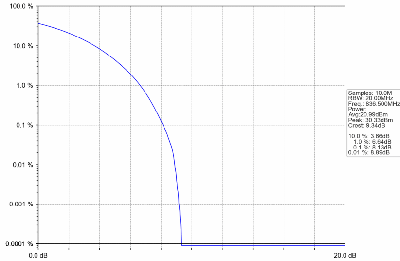
n5_15kHz_SISO_NTNV_20MHz_CP-OFDM 64 QAM_836.5MHz_Outer_Full
