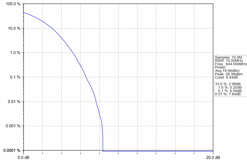
n5_15kHz_SISO_NTNV_10MHz_DFT-s-OFDM 256 QAM_844MHz_Outer_Full
