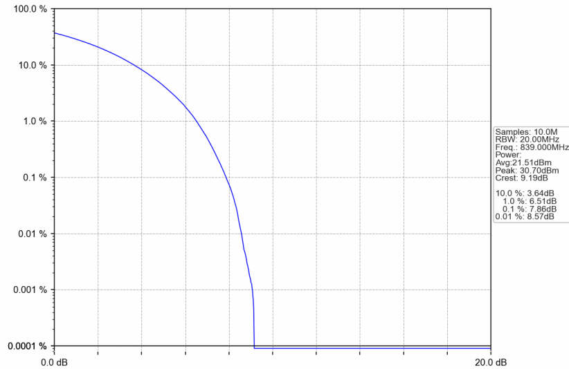
n5_15kHz_SISO_NTNV_20MHz_CP-OFDM 16 QAM_839MHz_Outer_Full
