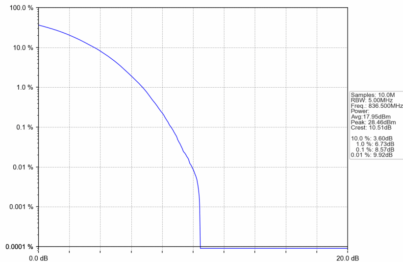
n5_15kHz_SISO_NTNV_5MHz_CP-OFDM 256 QAM_836.5MHz_Outer_Full
