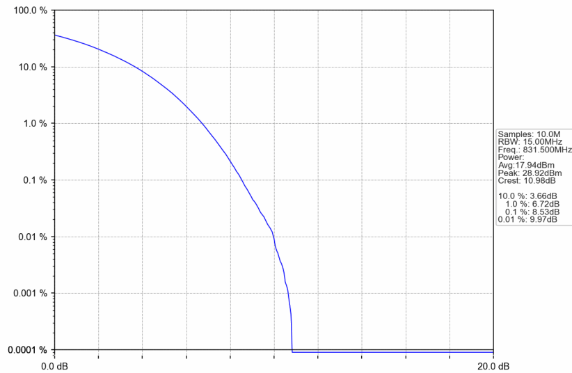
n5_15kHz_SISO_NTNV_15MHz_CP-OFDM 256 QAM_831.5MHz_Outer_Full
