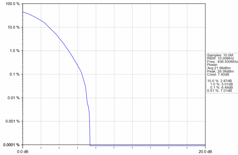
n5_30kHz_SISO_NTNV_10MHz_DFT-s-OFDM 64 QAM_836.5MHz_Outer_Full
