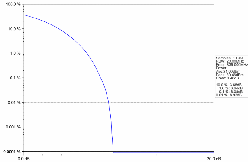
n5_15kHz_SISO_NTNV_20MHz_CP-OFDM 64 QAM_839MHz_Outer_Full
