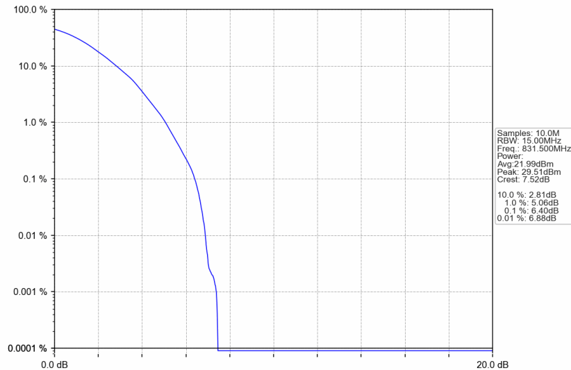
n5_15kHz_SISO_NTNV_15MHz_DFT-s-OFDM 64 QAM_831.5MHz_Outer_Full
