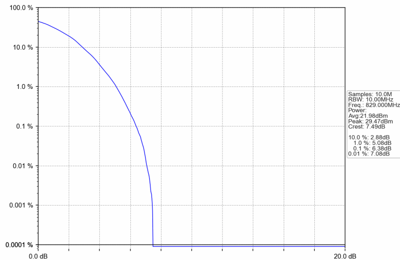
n5_15kHz_SISO_NTNV_10MHz_DFT-s-OFDM 64 QAM_829MHz_Outer_Full
