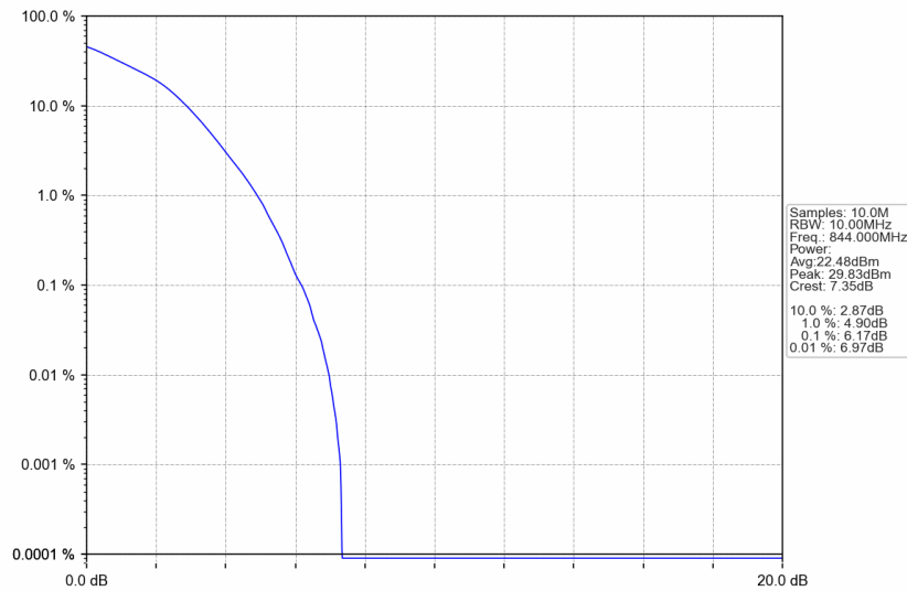
n5_15kHz_SISO_NTNV_10MHz_DFT-s-OFDM 16 QAM_844MHz_Outer_Full
