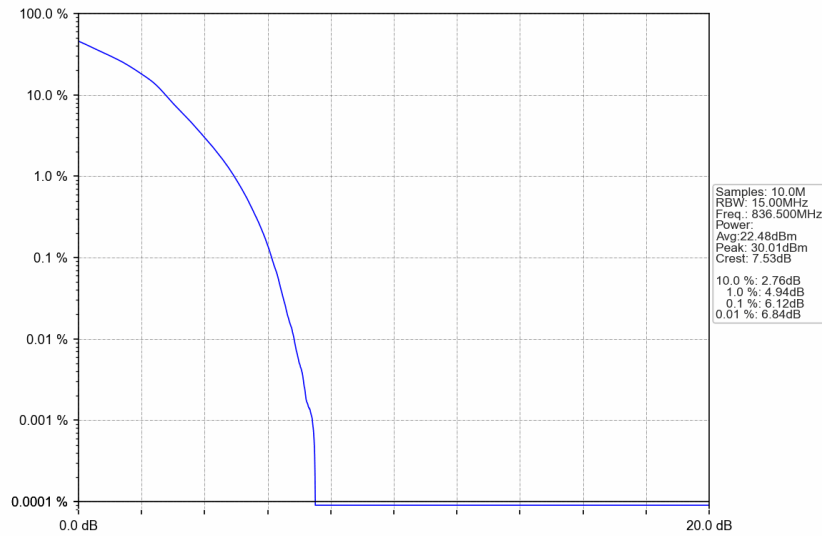
n5_15kHz_SISO_NTNV_15MHz_DFT-s-OFDM 16 QAM_836.5MHz_Outer_Full
