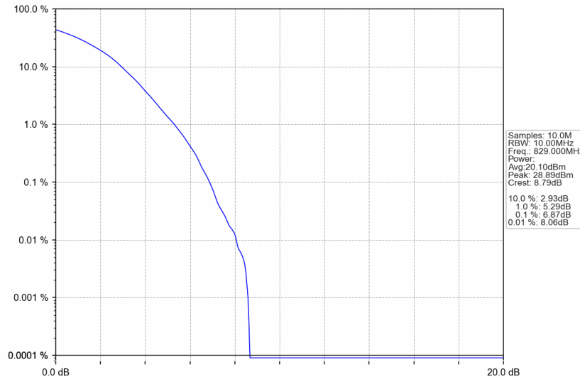
n5_30kHz_SISO_NTNV_10MHz_DFT-s-OFDM 256 QAM_829MHz_Outer_Full
