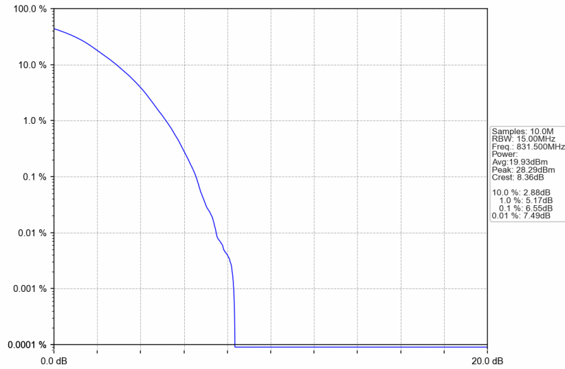
n5_15kHz_SISO_NTNV_15MHz_DFT-s-OFDM 256 QAM_831.5MHz_Outer_Full
