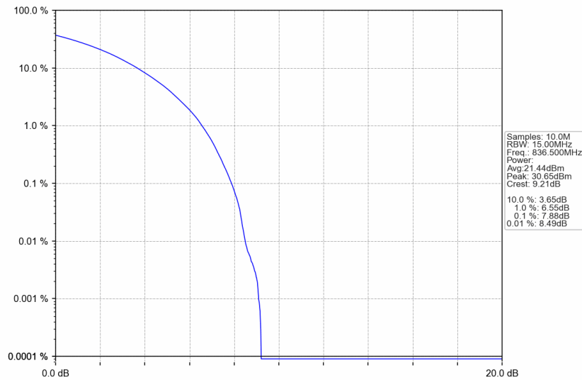
n5_15kHz_SISO_NTNV_15MHz_CP-OFDM QPSK_836.5MHz_Outer_Full
