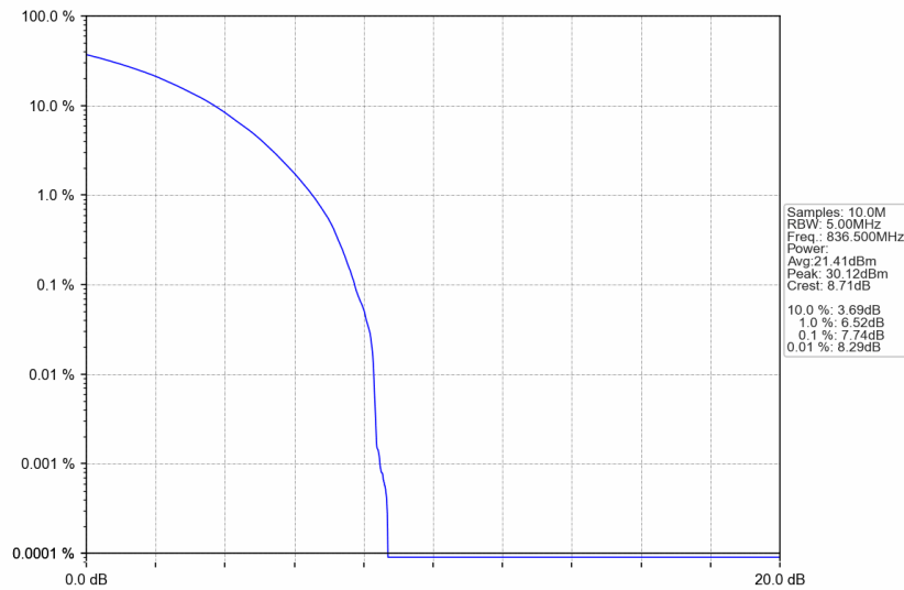
n5_15kHz_SISO_NTNV_5MHz_CP-OFDM QPSK_836.5MHz_Outer_Full
