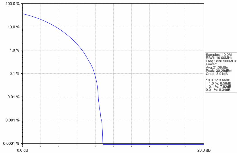
n5_30kHz_SISO_NTNV_10MHz_CP-OFDM QPSK_836.5MHz_Outer_Full
