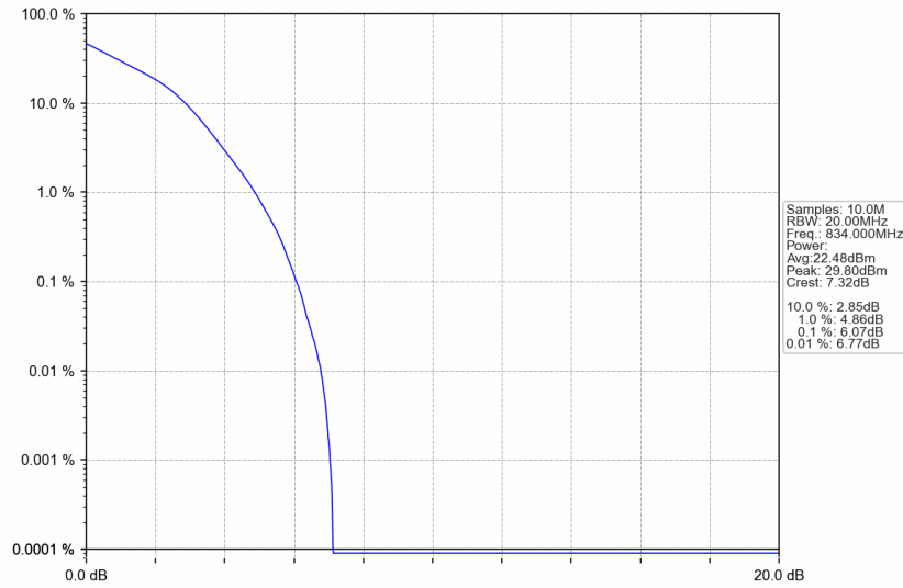
n5_15kHz_SISO_NTNV_20MHz_DFT-s-OFDM 16 QAM_834MHz_Outer_Full
