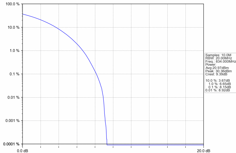
n5_15kHz_SISO_NTNV_20MHz_CP-OFDM 64 QAM_834MHz_Outer_Full
