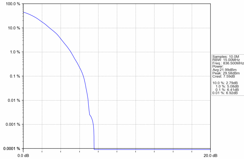
n5_15kHz_SISO_NTNV_15MHz_DFT-s-OFDM 64 QAM_836.5MHz_Outer_Full
