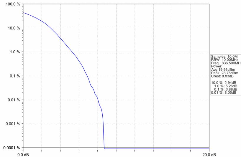
n5_30kHz_SISO_NTNV_10MHz_DFT-s-OFDM 256 QAM_836.5MHz_Outer_Full
