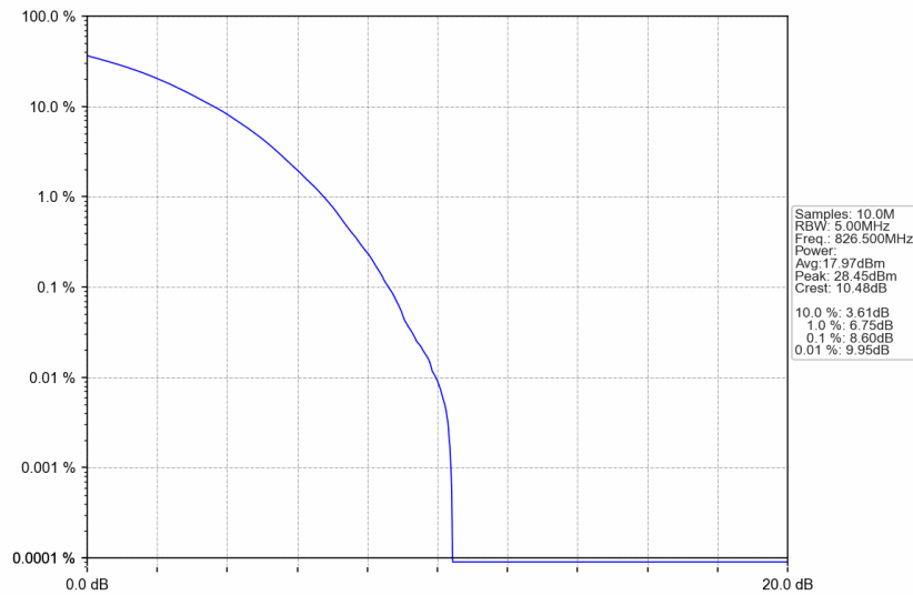
n5_15kHz_SISO_NTNV_5MHz_CP-OFDM 256 QAM_826.5MHz_Outer_Full
