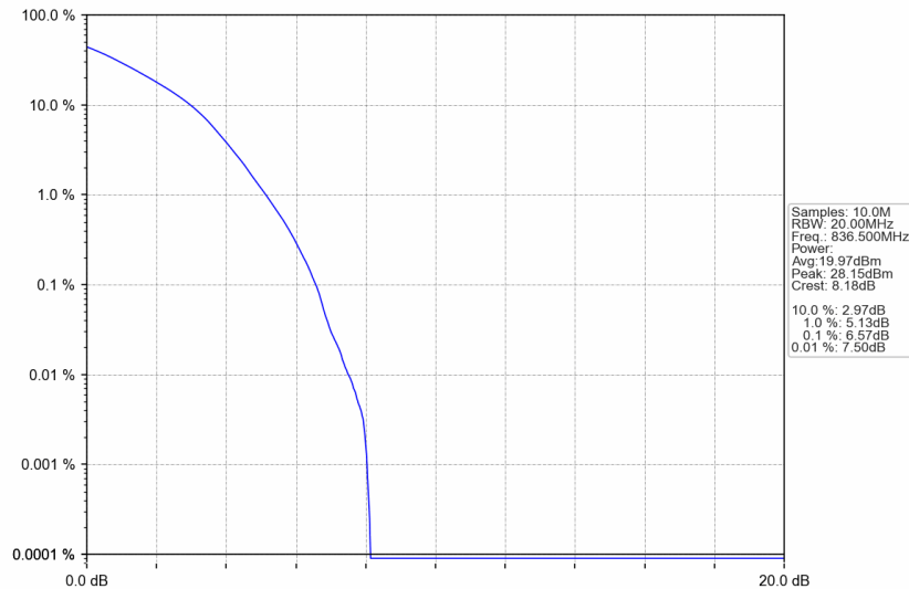
n5_15kHz_SISO_NTNV_20MHz_DFT-s-OFDM 256 QAM_836.5MHz_Outer_Full
