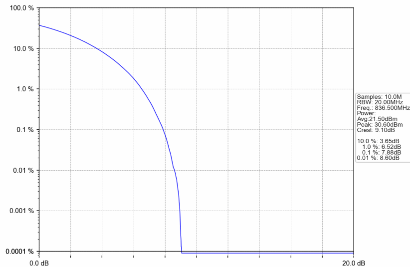
n5_15kHz_SISO_NTNV_20MHz_CP-OFDM 16 QAM_836.5MHz_Outer_Full
