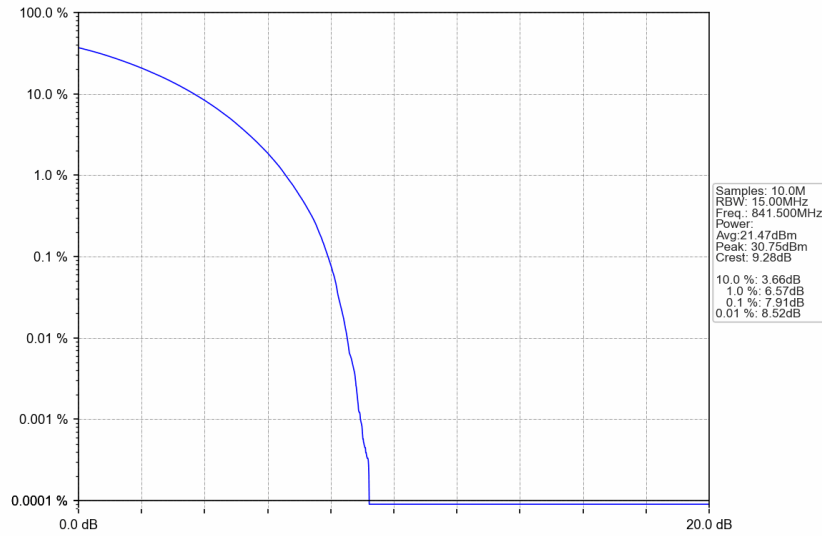
n5_15kHz_SISO_NTNV_15MHz_CP-OFDM 16 QAM_841.5MHz_Outer_Full
