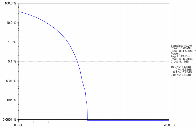
n5_15kHz_SISO_NTNV_15MHz_CP-OFDM QPSK_831.5MHz_Outer_Full
