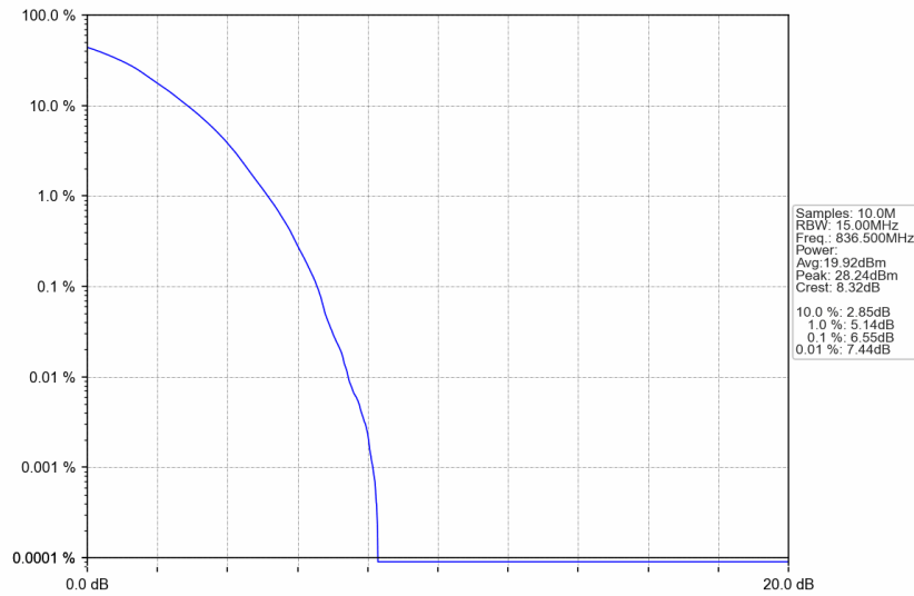
n5_15kHz_SISO_NTNV_15MHz_DFT-s-OFDM 256 QAM_836.5MHz_Outer_Full
