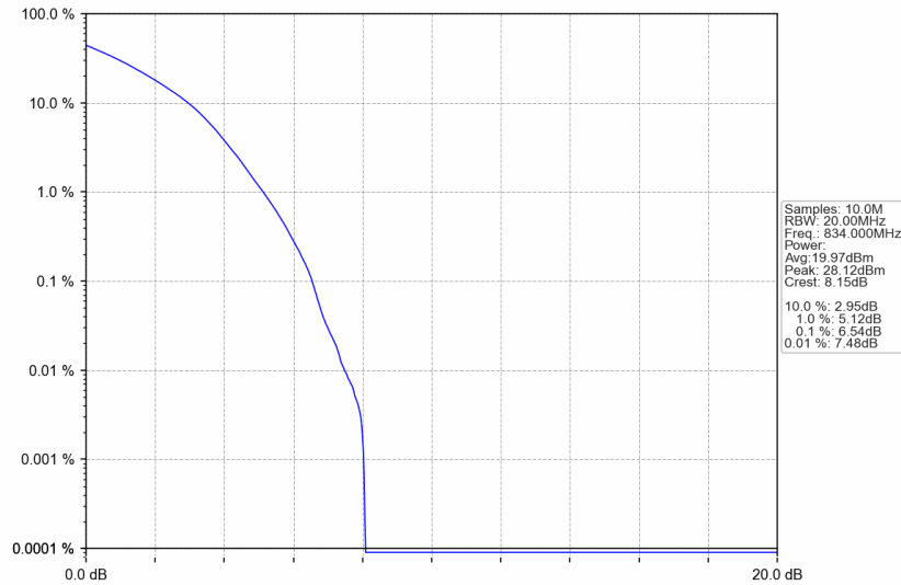
n5_15kHz_SISO_NTNV_20MHz_DFT-s-OFDM 256 QAM_834MHz_Outer_Full
