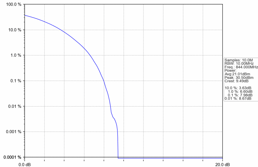
n5_15kHz_SISO_NTNV_10MHz_CP-OFDM 64 QAM_844MHz_Outer_Full
