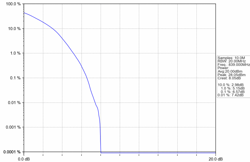
n5_15kHz_SISO_NTNV_20MHz_DFT-s-OFDM 256 QAM_839MHz_Outer_Full
