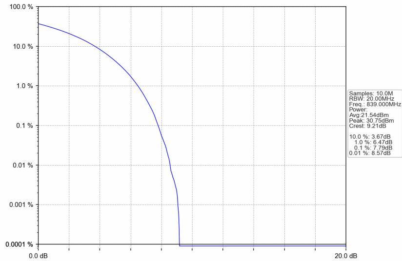
n5_15kHz_SISO_NTNV_20MHz_CP-OFDM QPSK_839MHz_Outer_Full
