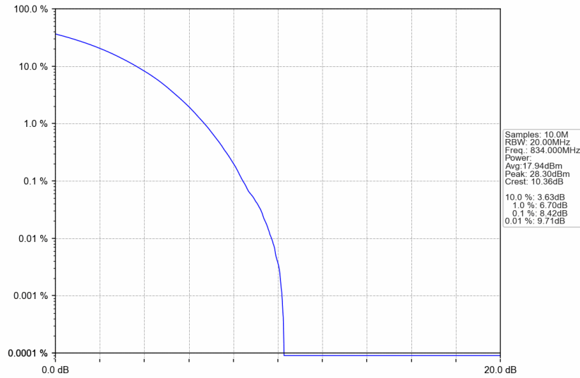
n5_15kHz_SISO_NTNV_20MHz_CP-OFDM 256 QAM_834MHz_Outer_Full
