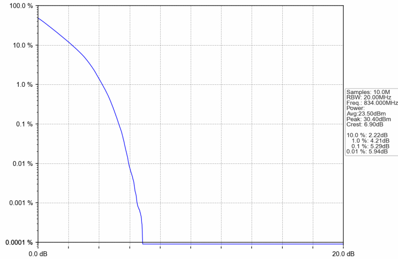
n5_15kHz_SISO_NTNV_20MHz_DFT-s-OFDM QPSK_834MHz_Outer_Full
