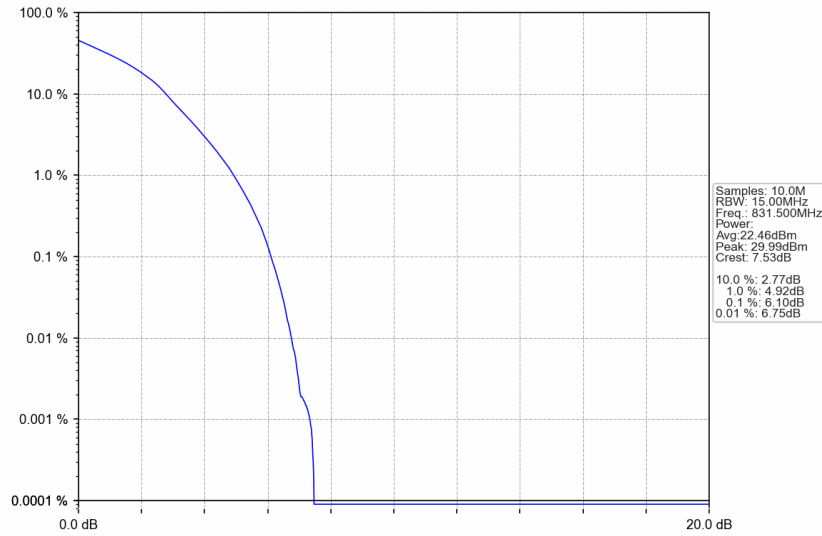
n5_15kHz_SISO_NTNV_15MHz_DFT-s-OFDM 16 QAM_831.5MHz_Outer_Full
