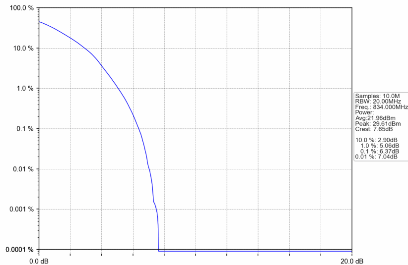
n5_15kHz_SISO_NTNV_20MHz_DFT-s-OFDM 64 QAM_834MHz_Outer_Full
