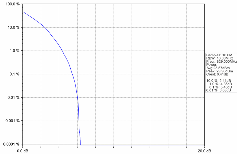
n5_30kHz_SISO_NTNV_10MHz_DFT-s-OFDM QPSK_829MHz_Outer_Full
