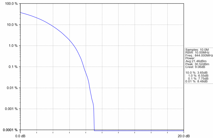
n5_15kHz_SISO_NTNV_10MHz_CP-OFDM QPSK_844MHz_Outer_Full
