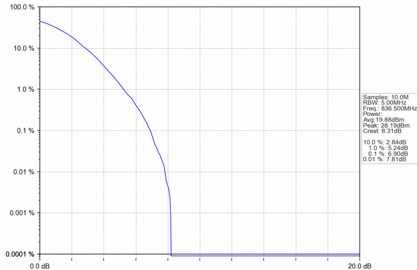
n5_15kHz_SISO_NTNV_5MHz_DFT-s-OFDM 256 QAM_836.5MHz_Outer_Full
