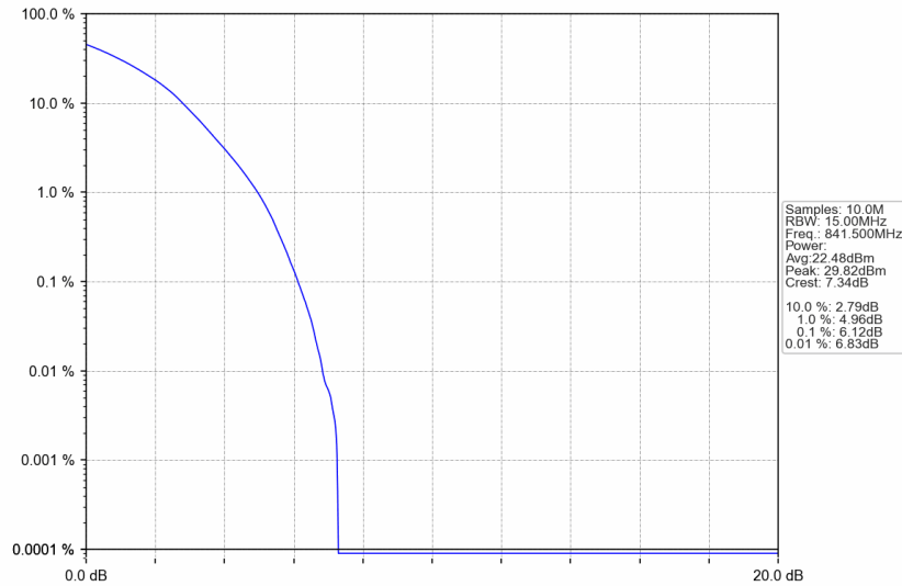
n5_15kHz_SISO_NTNV_15MHz_DFT-s-OFDM 16 QAM_841.5MHz_Outer_Full
