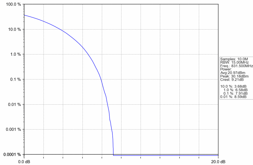
n5_15kHz_SISO_NTNV_15MHz_CP-OFDM 64 QAM_831.5MHz_Outer_Full
