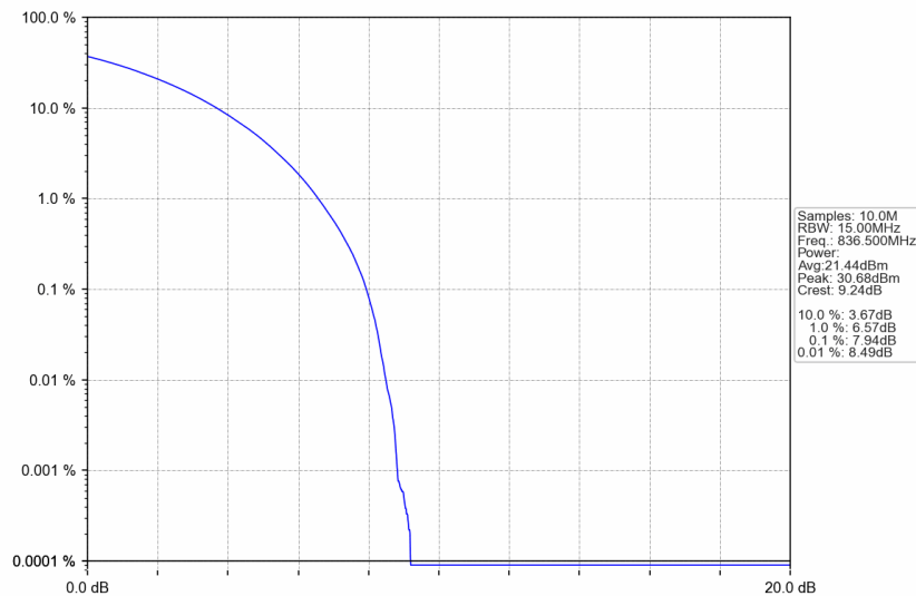
n5_15kHz_SISO_NTNV_15MHz_CP-OFDM 16 QAM_836.5MHz_Outer_Full
