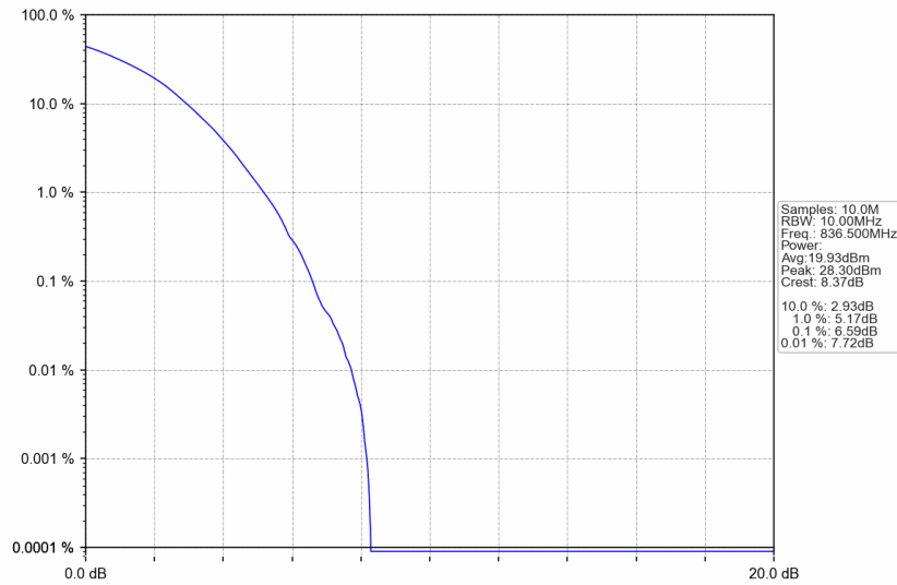
n5_15kHz_SISO_NTNV_10MHz_DFT-s-OFDM 256 QAM_836.5MHz_Outer_Full
