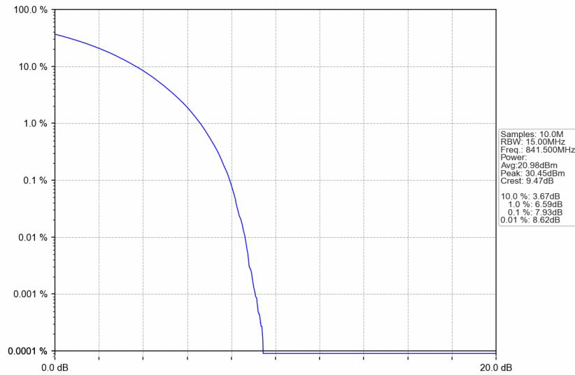
n5_15kHz_SISO_NTNV_15MHz_CP-OFDM 64 QAM_841.5MHz_Outer_Full
