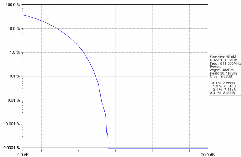
n5_15kHz_SISO_NTNV_15MHz_CP-OFDM QPSK_841.5MHz_Outer_Full
