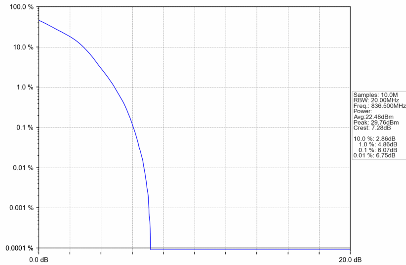
n5_15kHz_SISO_NTNV_20MHz_DFT-s-OFDM 16 QAM_836.5MHz_Outer_Full
