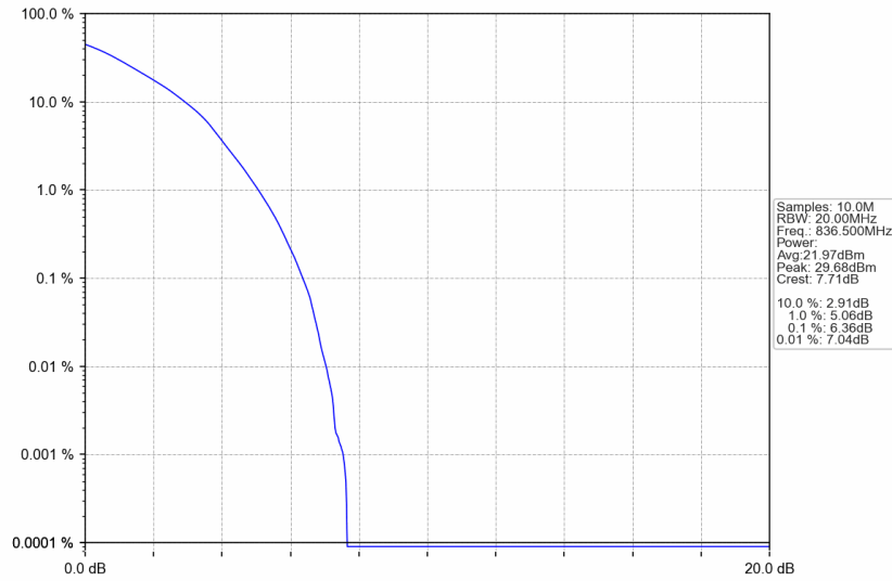
n5_15kHz_SISO_NTNV_20MHz_DFT-s-OFDM 64 QAM_836.5MHz_Outer_Full
