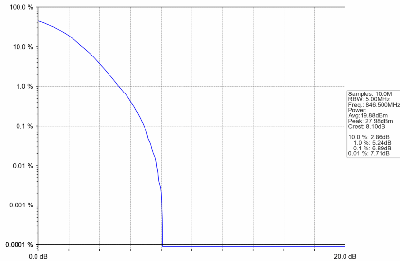
n5_15kHz_SISO_NTNV_5MHz_DFT-s-OFDM 256 QAM_846.5MHz_Outer_Full
