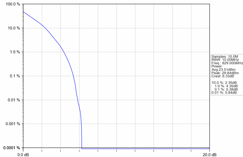
n5_15kHz_SISO_NTNV_10MHz_DFT-s-OFDM QPSK_829MHz_Outer_Full
