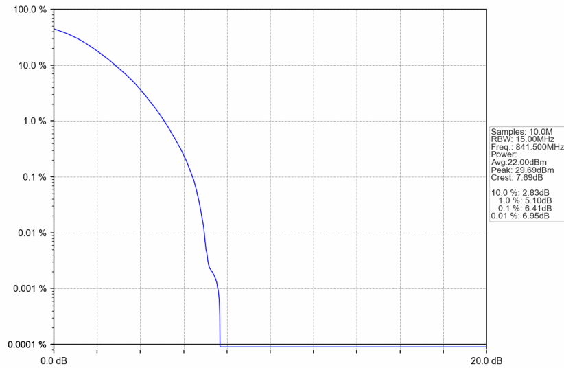
n5_15kHz_SISO_NTNV_15MHz_DFT-s-OFDM 64 QAM_841.5MHz_Outer_Full
