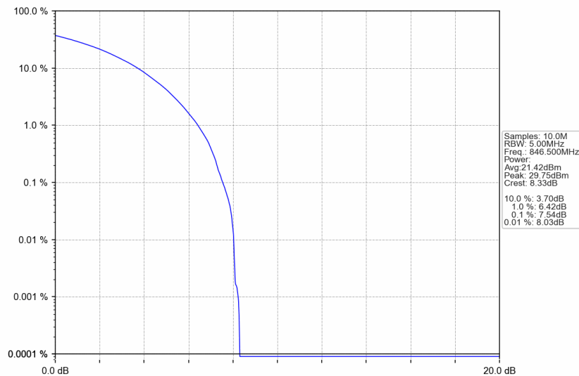
n5_15kHz_SISO_NTNV_5MHz_CP-OFDM QPSK_846.5MHz_Outer_Full
