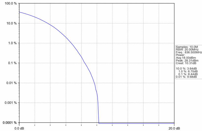
n5_15kHz_SISO_NTNV_20MHz_CP-OFDM 256 QAM_836.5MHz_Outer_Full
