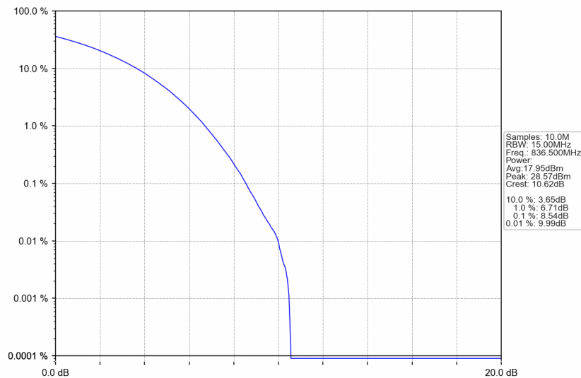
n5_15kHz_SISO_NTNV_15MHz_CP-OFDM 256 QAM_836.5MHz_Outer_Full
