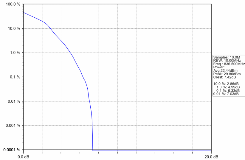
n5_30kHz_SISO_NTNV_10MHz_DFT-s-OFDM 16 QAM_836.5MHz_Outer_Full
