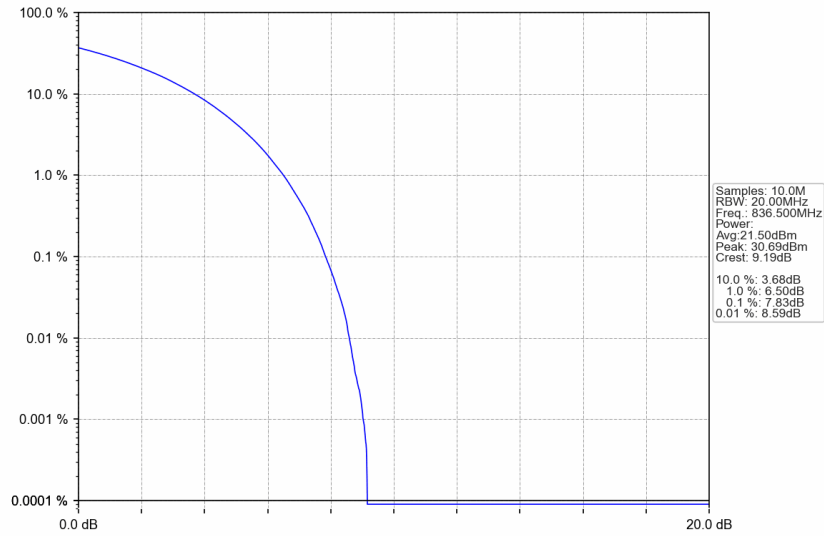
n5_15kHz_SISO_NTNV_20MHz_CP-OFDM QPSK_836.5MHz_Outer_Full
