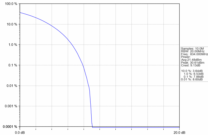
n5_15kHz_SISO_NTNV_20MHz_CP-OFDM 16 QAM_834MHz_Outer_Full
