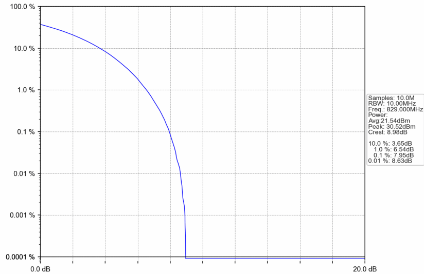
n5_15kHz_SISO_NTNV_10MHz_CP-OFDM 16 QAM_829MHz_Outer_Full
