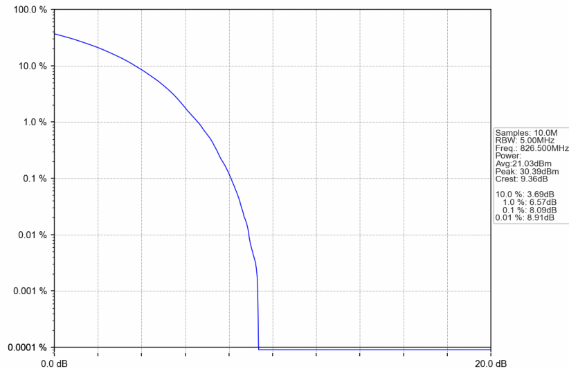
n5_15kHz_SISO_NTNV_5MHz_CP-OFDM 64 QAM_826.5MHz_Outer_Full
