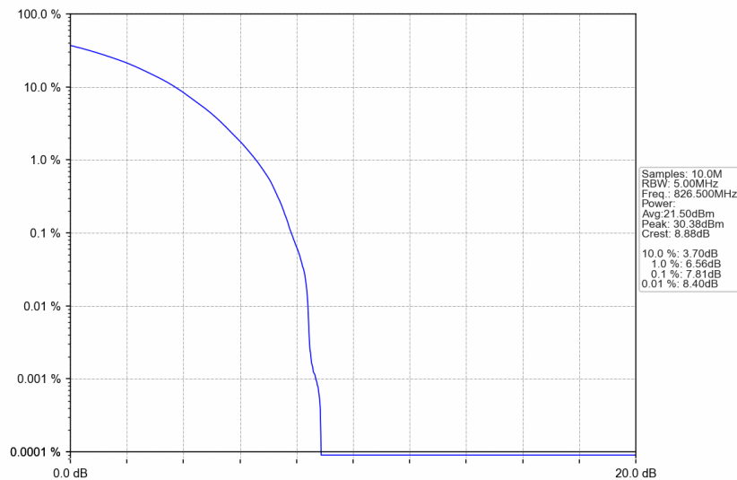
n5_15kHz_SISO_NTNV_5MHz_CP-OFDM QPSK_826.5MHz_Outer_Full
