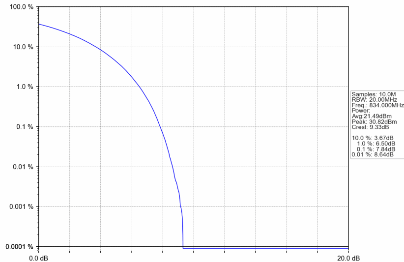
n5_15kHz_SISO_NTNV_20MHz_CP-OFDM QPSK_834MHz_Outer_Full
