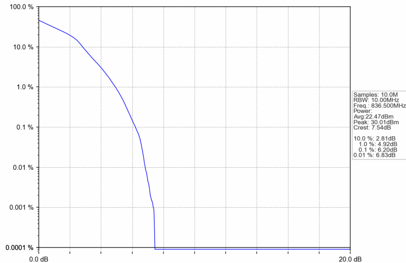
n5_15kHz_SISO_NTNV_10MHz_DFT-s-OFDM 16 QAM_836.5MHz_Outer_Full
