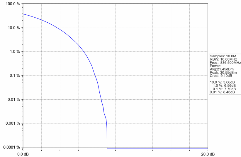
n5_15kHz_SISO_NTNV_10MHz_CP-OFDM QPSK_836.5MHz_Outer_Full
