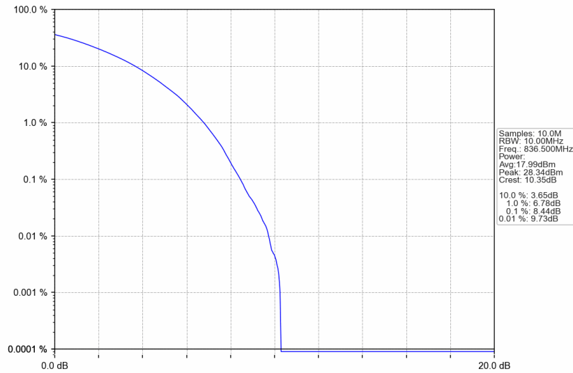
n5_15kHz_SISO_NTNV_10MHz_CP-OFDM 256 QAM_836.5MHz_Outer_Full
