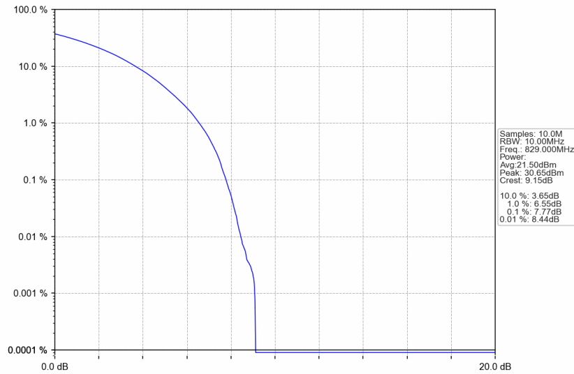
n5_15kHz_SISO_NTNV_10MHz_CP-OFDM QPSK_829MHz_Outer_Full
