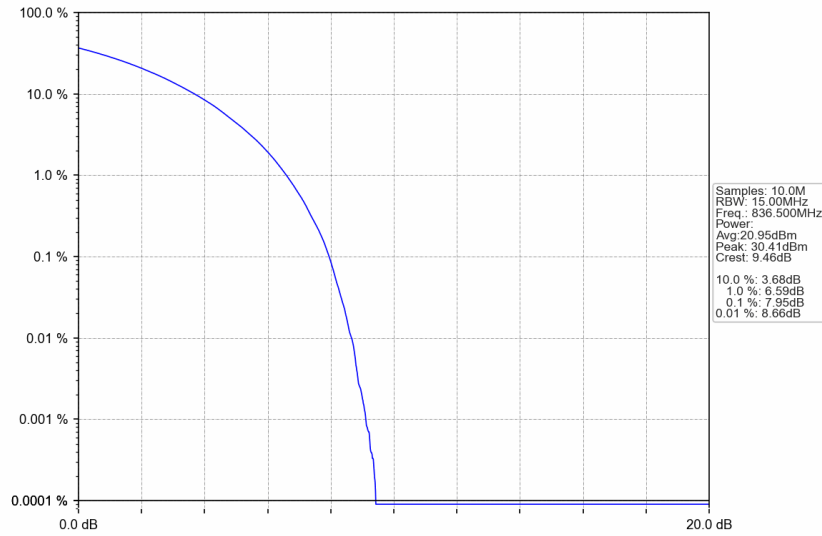
n5_15kHz_SISO_NTNV_15MHz_CP-OFDM 64 QAM_836.5MHz_Outer_Full
