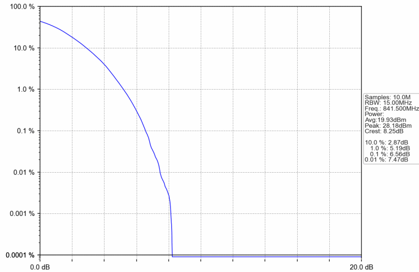
n5_15kHz_SISO_NTNV_15MHz_DFT-s-OFDM 256 QAM_841.5MHz_Outer_Full
