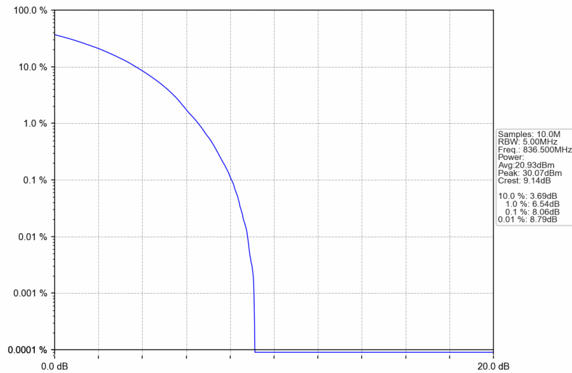
n5_15kHz_SISO_NTV_5MHz_CP-OFDM 64 QAM_836.5MHz_Outer_Full
