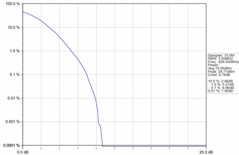
n5_15kHz_SISO_NTNV_5MHz_DFT-s-OFDM 256 QAM_826.5MHz_Outer_Full
