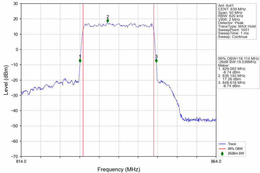
n5_30kHz_SISO_NTNV_20MHz_DFT-s-OFDM 64 QAM_839MHz_Outer_Full
