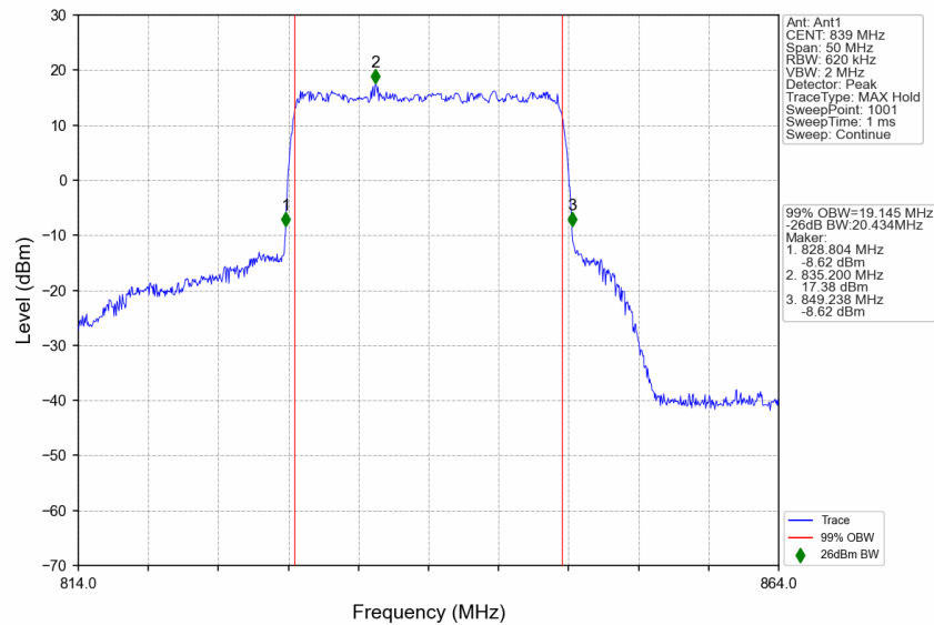
n5_15kHz_SISO_NTNV_20MHz_CP-OFDM 64 QAM_839MHz_Outer_Full
