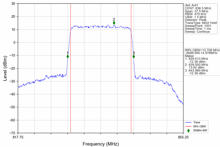
n5_30kHz_SISO_NTNV_15MHz_CP-OFDM 256 QAM_836.5MHz_Outer_Full
