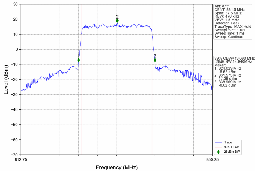
n5_30kHz_SISO_NTNV_15MHz_CP-OFDM QPSK_831.5MHz_Outer_Full
