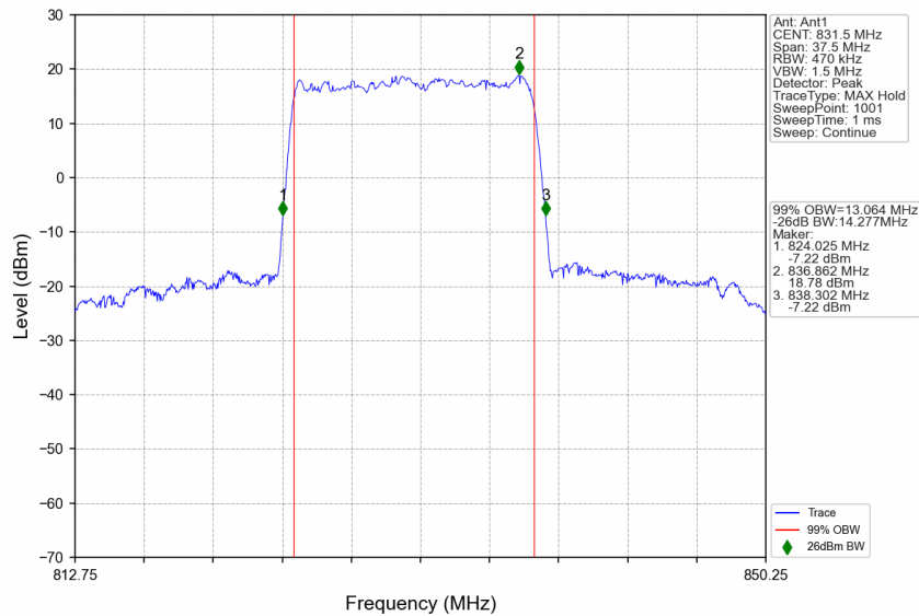
n5_30kHz_SISO_NTNV_15MHz_DFT-s-OFDM QPSK_831.5MHz_Outer_Full
