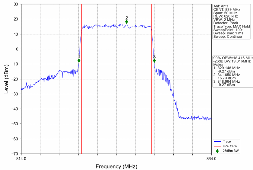
n5_30kHz_SISO_NTNV_20MHz_CP-OFDM 64 QAM_839MHz_Outer_Full
