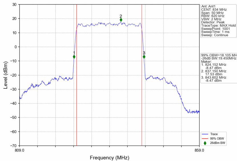
n5_30kHz_SISO_NTNV_20MHz_DFT-s-OFDM 64 QAM_834MHz_Outer_Full
