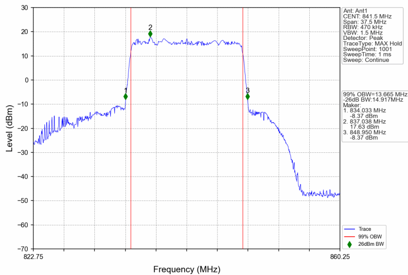
n5_30kHz_SISO_NTNV_15MHz_CP-OFDM QPSK_841.5MHz_Outer_Full
