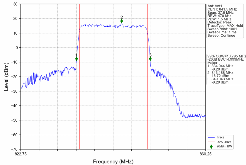
n5_30kHz_SISO_NTNV_15MHz_CP-OFDM 64 QAM_841.5MHz_Outer_Full
