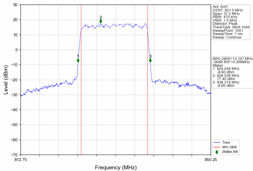
n5_30kHz_SISO_NTNV_15MHz_DFT-s-OFDM 64 QAM_831.5MHz_Outer_Full
