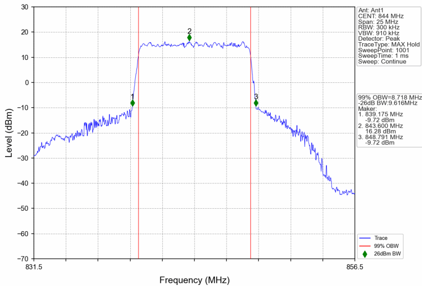
n5_30kHz_SISO_NTNV_10MHz_CP-OFDM QPSK_844MHz_Outer_Full
