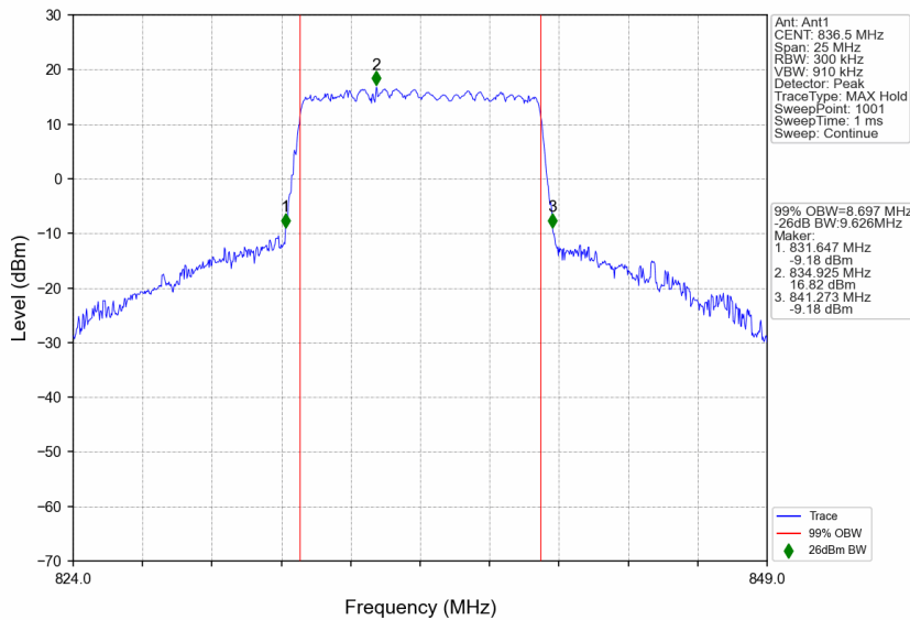
n5_30kHz_SISO_NTNV_10MHz_CP-OFDM 16 QAM_836.5MHz_Outer_Full
