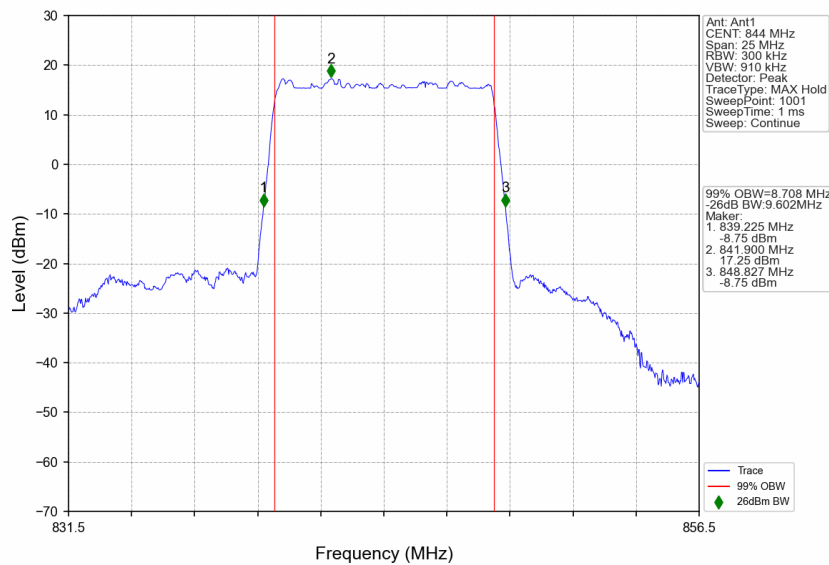
n5_30kHz_SISO_NTNV_10MHz_DFT-s-OFDM 64 QAM_844MHz_Outer_Full
