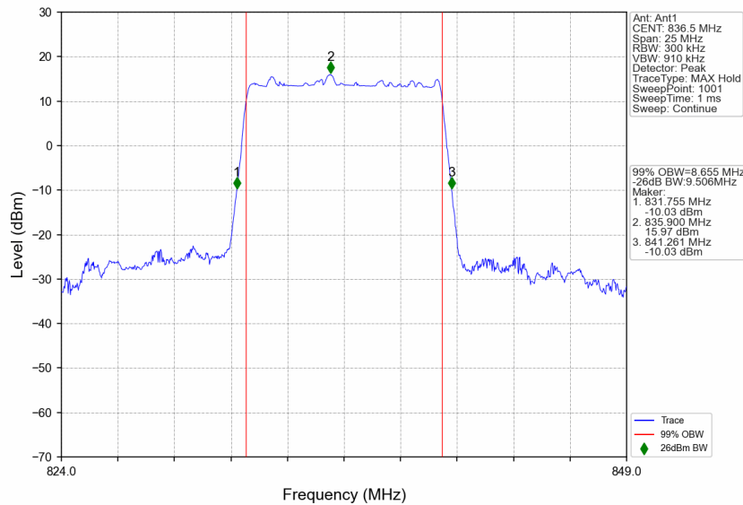
n5_30kHz_SISO_NTNV_10MHz_DFT-s-OFDM 256 QAM_836.5MHz_Outer_Full
