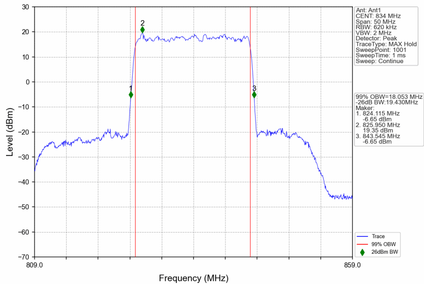
n5_30kHz_SISO_NTNV_20MHz_DFT-s-OFDM QPSK_834MHz_Outer_Full
