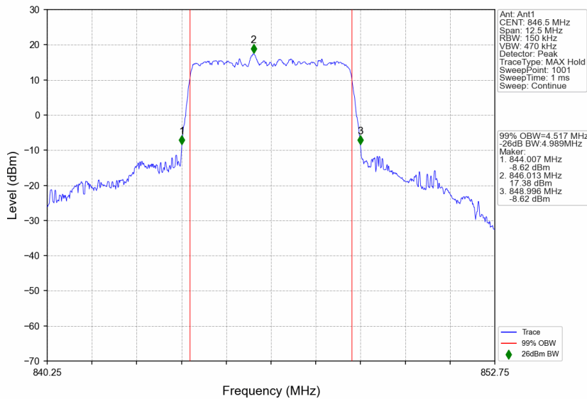
n5_15kHz_SISO_NTNV_5MHz_CP-OFDM QPSK_846.5MHz_Outer_Full
