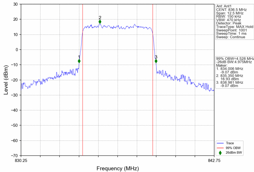
n5_15kHz_SISO_NTNV_5MHz_CP-OFDM 16 QAM_836.5MHz_Outer_Full
