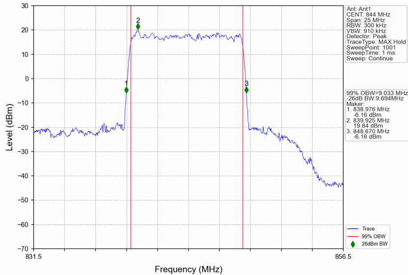
n5_15kHz_SISO_NTNV_10MHz_DFT-s-OFDM QPSK_844MHz_Outer_Full
