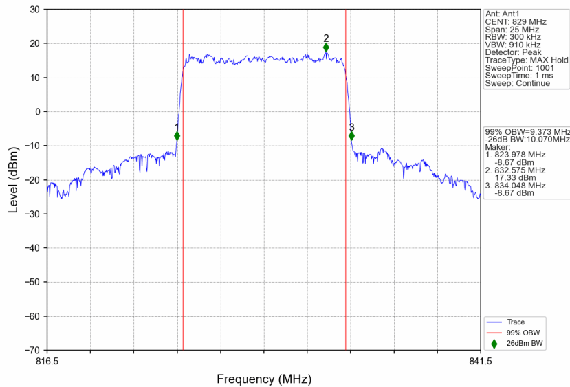
n5_15kHz_SISO_NTNV_10MHz_CP-OFDM QPSK_829MHz_Outer_Full
