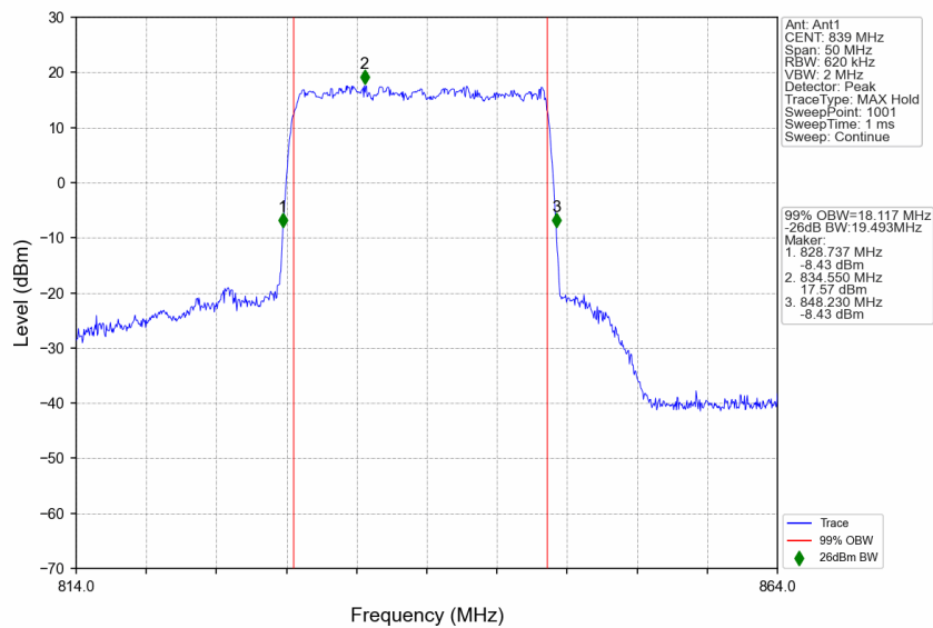
n5_15kHz_SISO_NTNV_20MHz_DFT-s-OFDM 64 QAM_839MHz_Outer_Full
