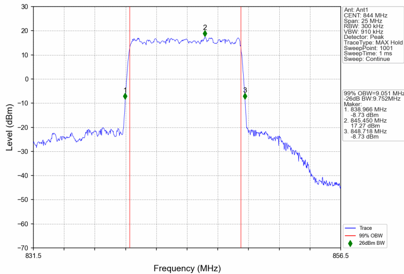
n5_15kHz_SISO_NTNV_10MHz_DFT-s-OFDM 64 QAM_844MHz_Outer_Full
