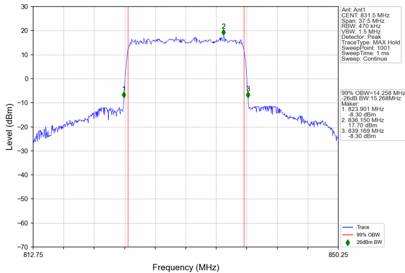
n5_15kHz_SISO_NTNV_15MHz_CP-OFDM QPSK_831.5MHz_Outer_Full
