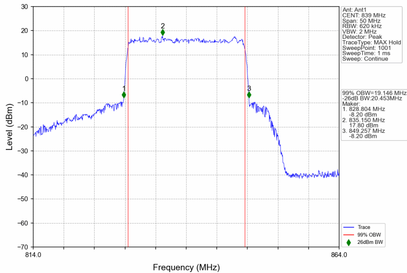
n5_15kHz_SISO_NTNV_20MHz_CP-OFDM QPSK_839MHz_Outer_Full
