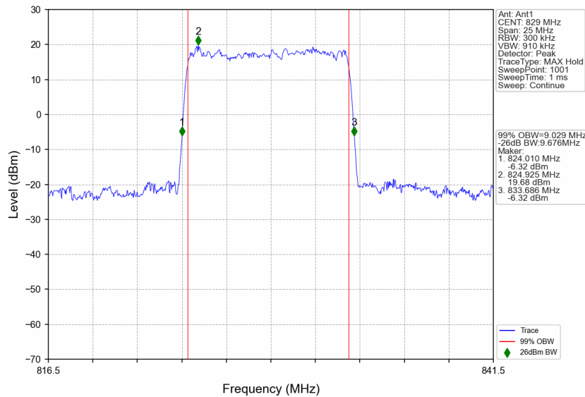
n5_15kHz_SISO_NTNV_10MHz_DFT-s-OFDM QPSK_829MHz_Outer_Full
