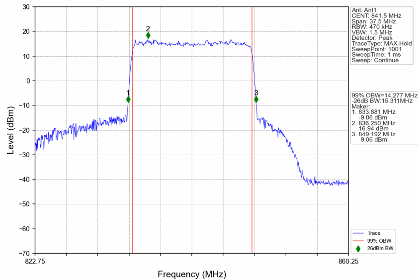
n5_15kHz_SISO_NTNV_15MHz_CP-OFDM 64 QAM_841.5MHz_Outer_Full
