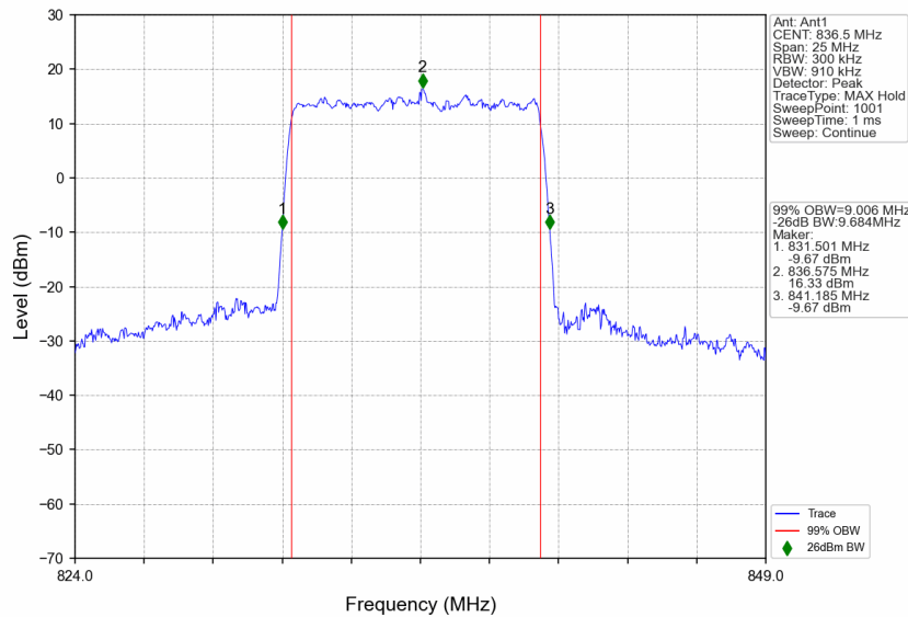
n5_15kHz_SISO_NTNV_10MHz_DFT-s-OFDM 256 QAM_836.5MHz_Outer_Full
