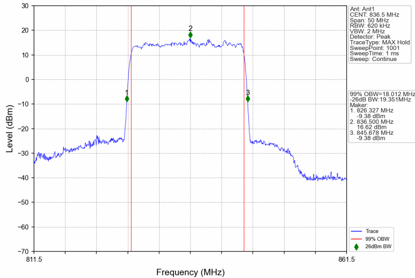
n5_15kHz_SISO_NTNV_20MHz_DFT-s-OFDM 256 QAM_836.5MHz_Outer_Full
