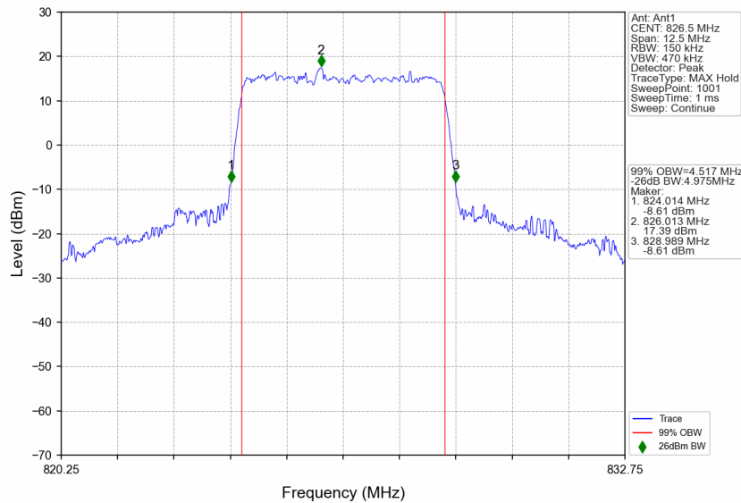
n5_15kHz_SISO_NTNV_5MHz_CP-OFDM QPSK_826.5MHz_Outer_Full
