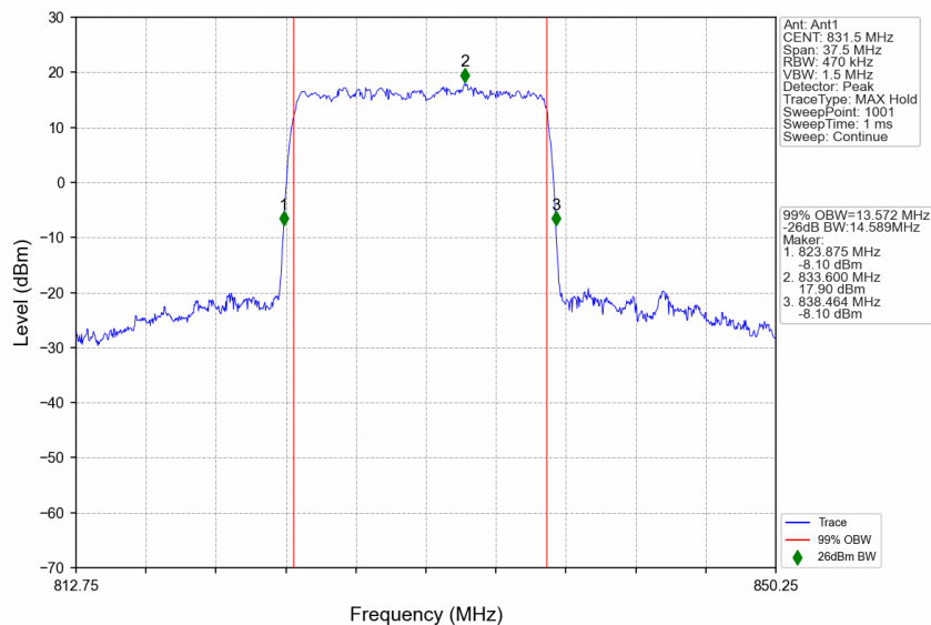
n5_15kHz_SISO_NTNV_15MHz_DFT-s-OFDM 64 QAM_831.5MHz_Outer_Full
