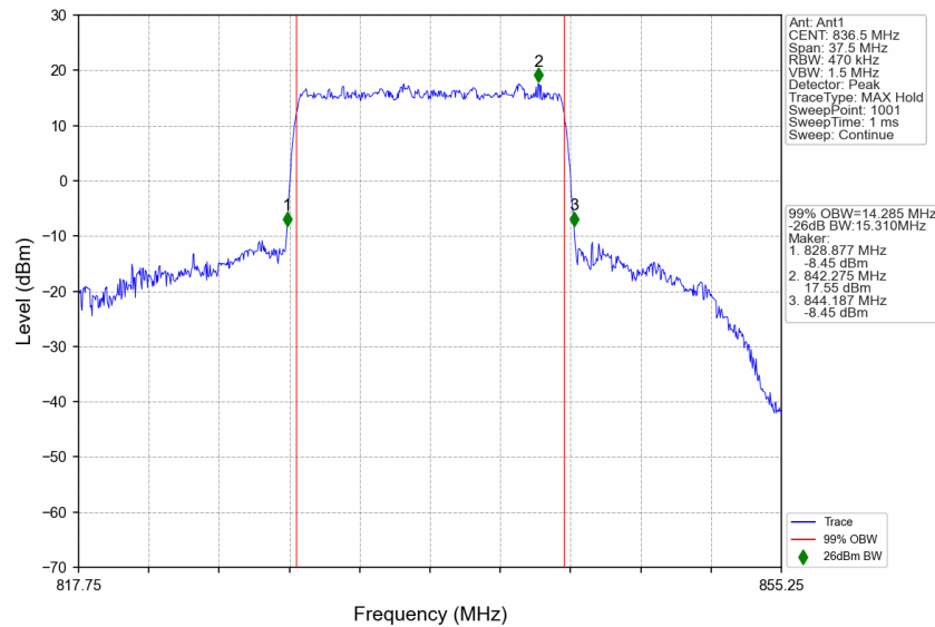
n5_15kHz_SISO_NTNV_15MHz_CP-OFDM 16 QAM_836.5MHz_Outer_Full
