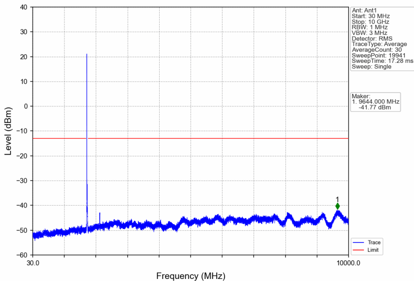
Band66_15MHz_16QAM_MCH_1745MHz_RB_1_0_NTNV
