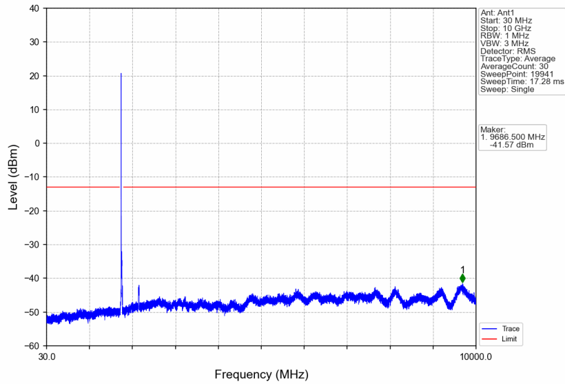
Band66_20MHz_16QAM_HCH_1770MHz_RB_1_0_NTNV
