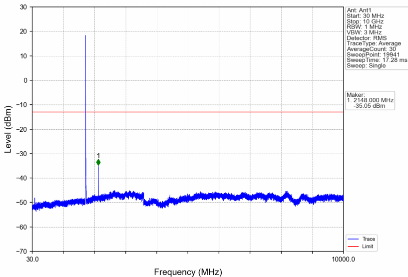
Band66_10MHz_256QAM_MCH_1745MHz_RB_1_0_NTNV
