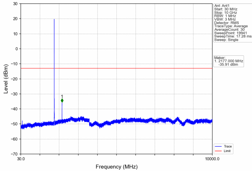
Band66_10MHz_256QAM_HCH_1775MHz_RB_1_0_NTNV
