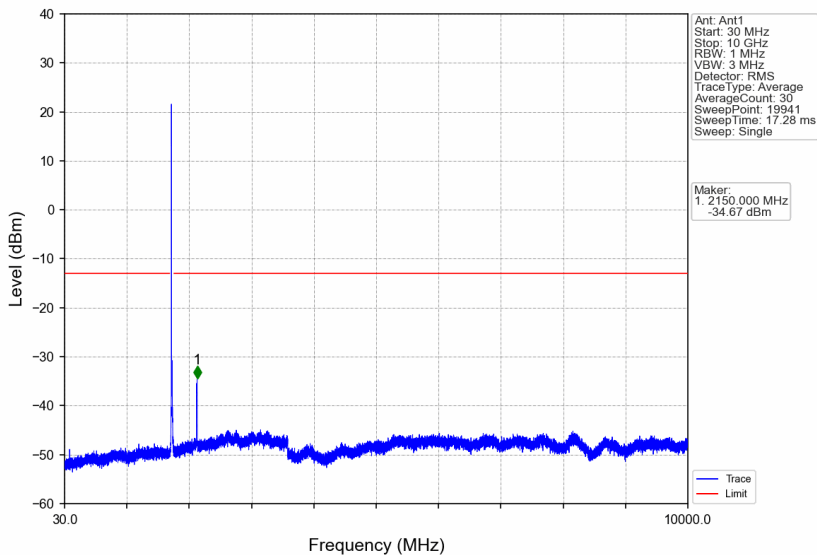
Band66_15MHz_64QAM_MCH_1745MHz_RB_1_0_NTNV
