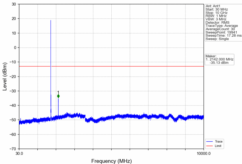
Band66_15MHz_256QAM_MCH_1745MHz_RB_1_0_NTNV
