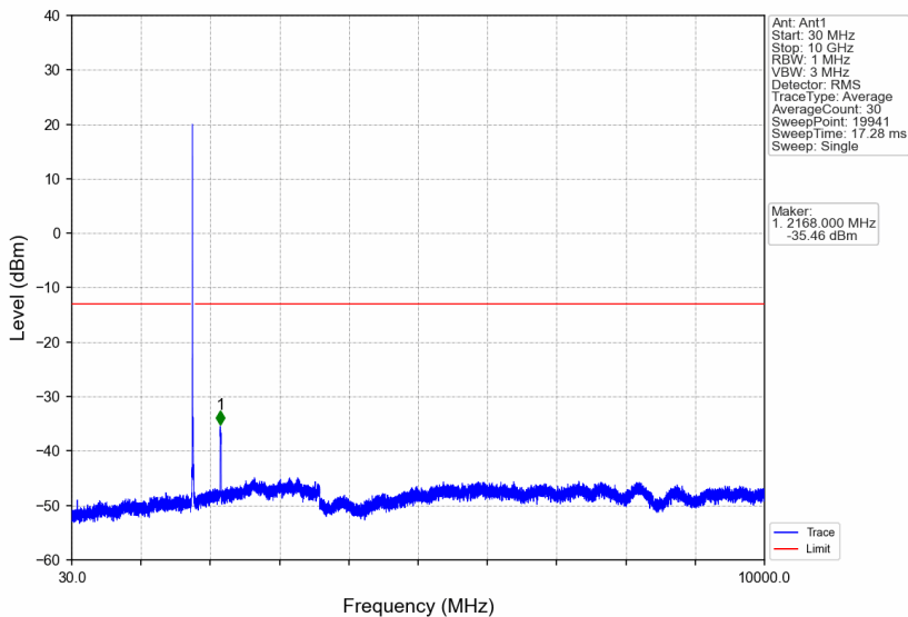
Band66_15MHz_256QAM_HCH_1772.5MHz_RB_1_0_NTNV
