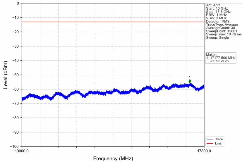
Band66_20MHz_16QAM_HCH_1770MHz_RB_1_0_NTNV
