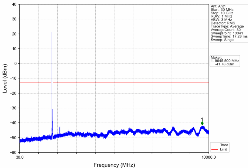
Band66_20MHz_16QAM_MCH_1745MHz_RB_1_0_NTNV
