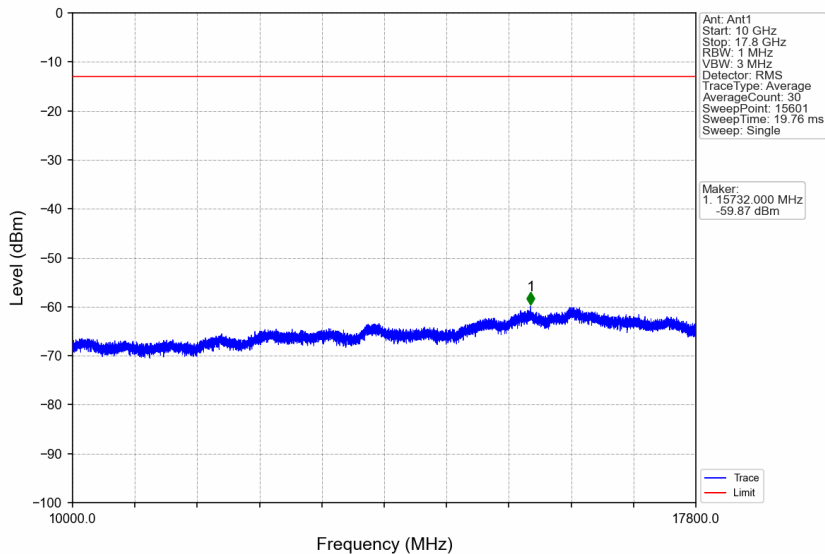
Band66_10MHz_256QAM_MCH_1745MHz_RB_1_0_NTNV
