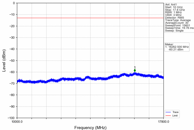
Band66_15MHz_256QAM_MCH_1745MHz_RB_1_0_NTNV
