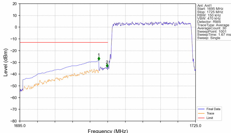
Band66_15MHz_16QAM_LCH_1717.5MHz_RB_75_0_NTNV
