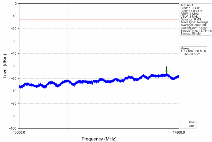
Band66_15MHz_16QAM_LCH_1717.5MHz_RB_75_0_NTNV
