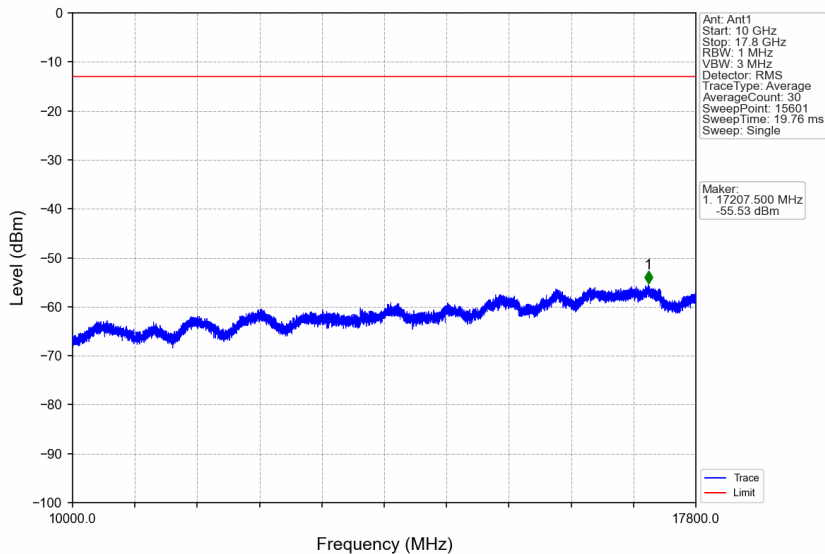
Band66_20MHz_16QAM_MCH_1745MHz_RB_1_0_NTNV
