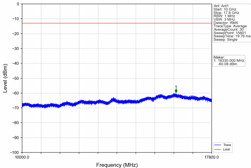
Band66_15MHz_64QAM_MCH_1745MHz_RB_1_0_NTNV
