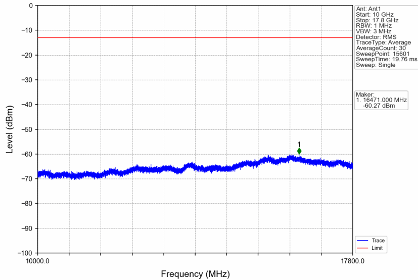
Band66_10MHz_256QAM_HCH_1775MHz_RB_1_0_NTNV
