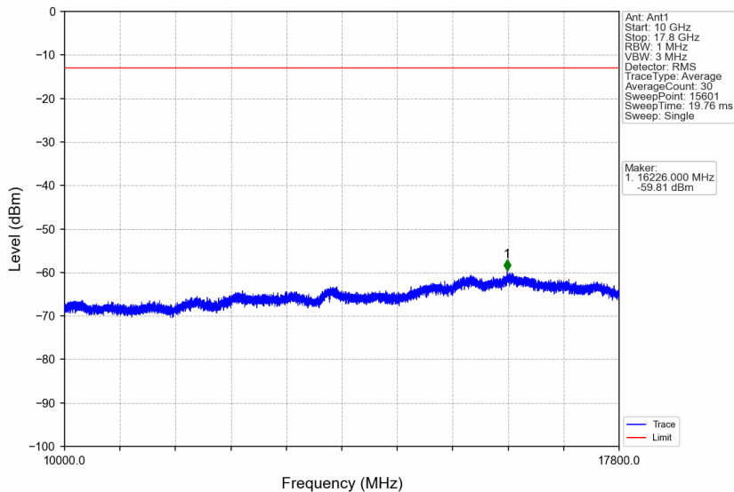
Band66_15MHz_256QAM_HCH_1772.5MHz_RB_1_0_NTNV
