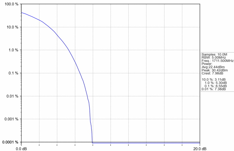
Band66_3MHz_64QAM_LCH_1711.5MHz_RB_15_0_NTNV
