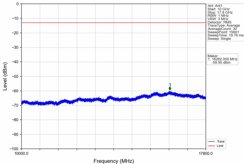
Band66_1.4MHz_64QAM_HCH_1779.3MHz_RB_1_0_NTNV
