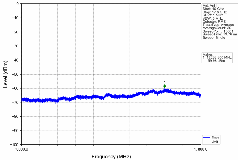
Band66_1.4MHz_256QAM_HCH_1779.3MHz_RB_1_0_NTNV
