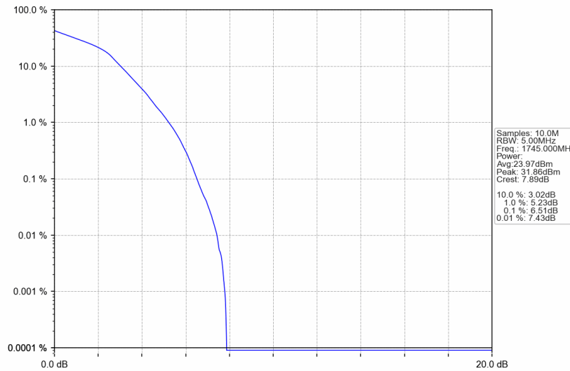
Band66_1.4MHz_16QAM_MCH_1745MHz_RB_6_0_NTNV
