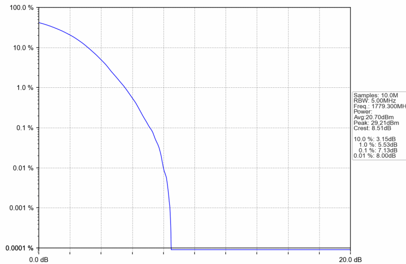
Band66_1.4MHz_256QAM_HCH_1779.3MHz_RB_6_0_NTNV
