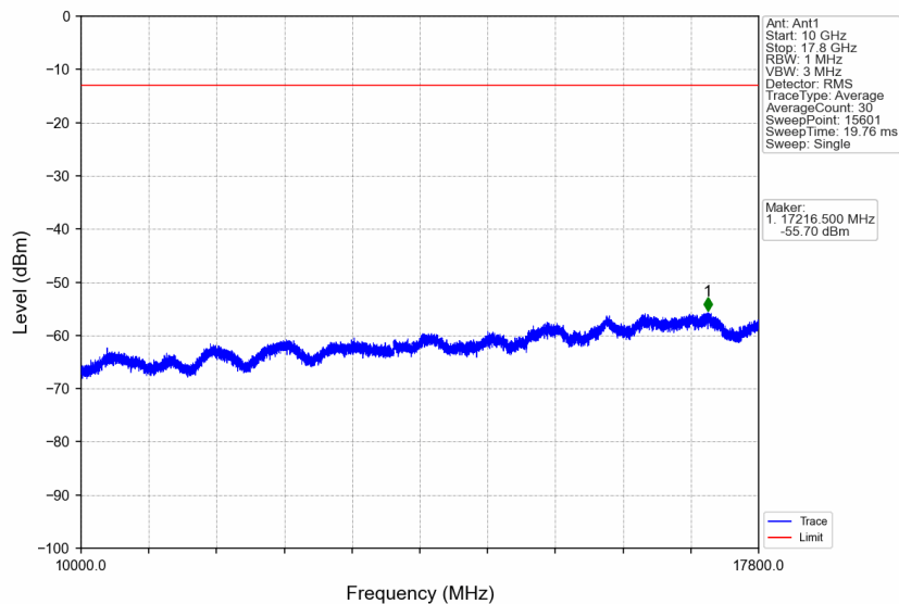
Band66_1.4MHz_16QAM_MCH_1745MHz_RB_1_0_NTNV
