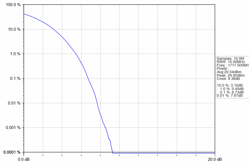
Band66_15MHz_256QAM_LCH_1717.5MHz_RB_75_0_NTNV
