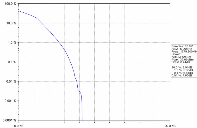
Band66_1.4MHz_16QAM_HCH_1779.3MHz_RB_6_0_NTNV
