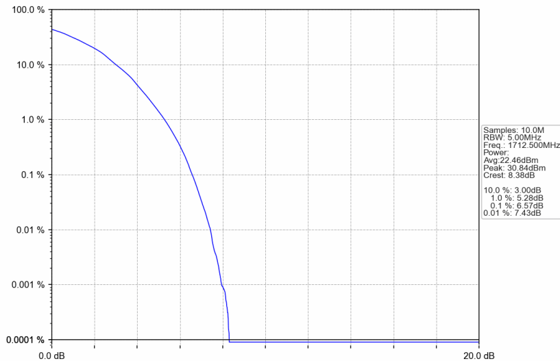
Band66_5MHz_64QAM_LCH_1712.5MHz_RB_25_0_NTNV
