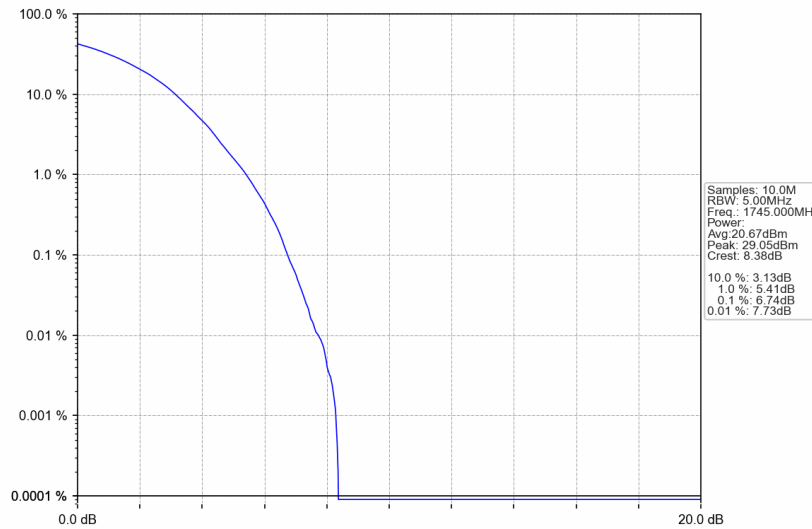
Band66_1.4MHz_256QAM_MCH_1745MHz_RB_6_0_NTNV
