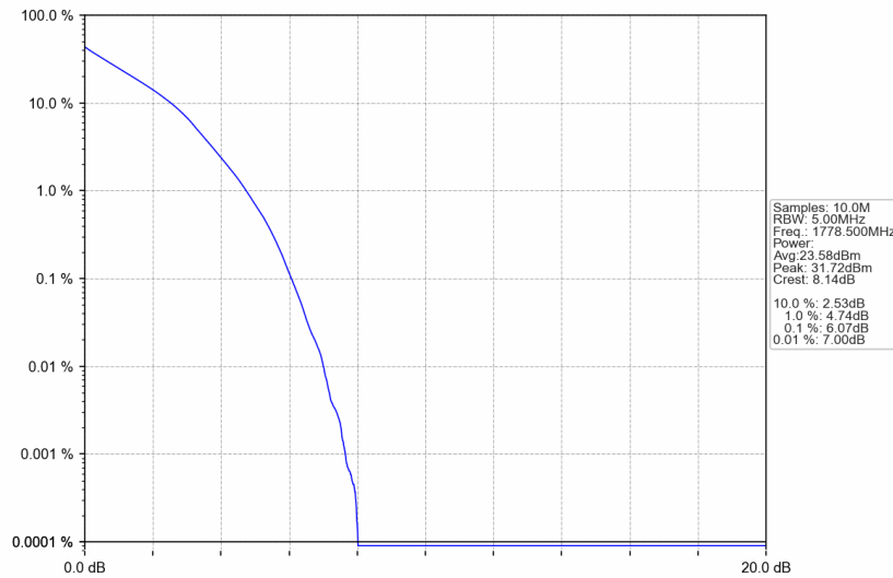
Band66_3MHz_QPSK_HCH_1778.5MHz_RB_15_0_NTNV
