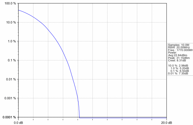
Band66_20MHz_64QAM_HCH_1770MHz_RB_100_0_NTNV
