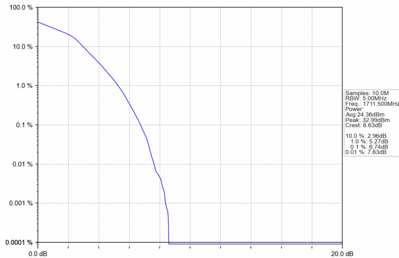
Band66_3MHz_16QAM_LCH_1711.5MHz_RB_15_0_NTNV
