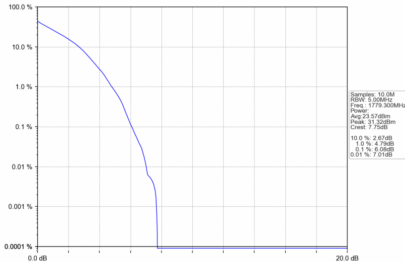
Band66_1.4MHz_QPSK_HCH_1779.3MHz_RB_6_0_NTNV
