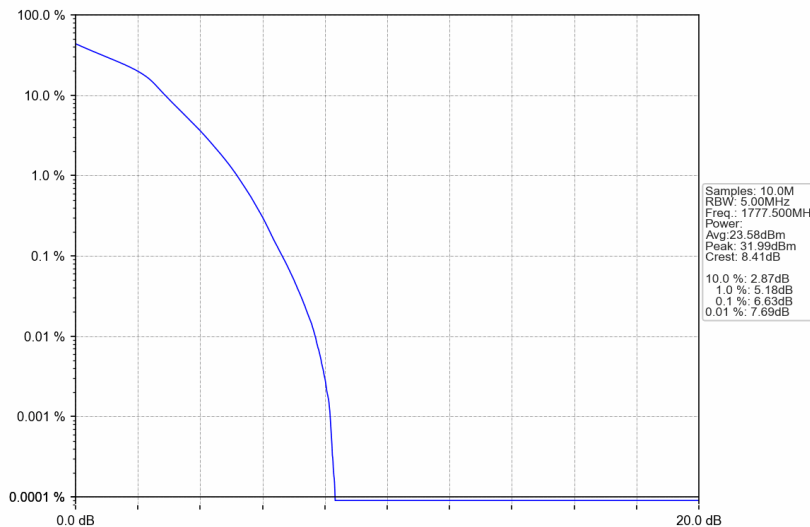
Band66_5MHz_16QAM_HCH_1777.5MHz_RB_25_0_NTNV
