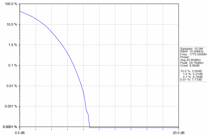
Band66_10MHz_256QAM_HCH_1775MHz_RB_50_0_NTNV
