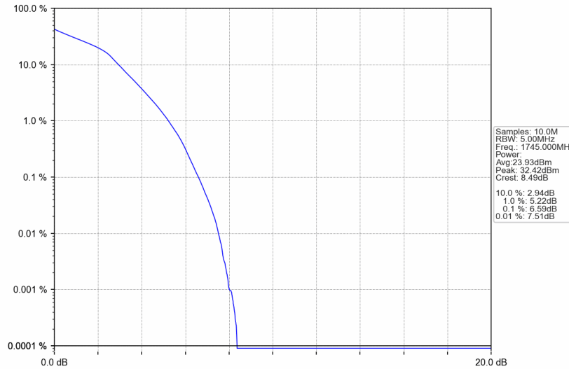
Band66_3MHz_16QAM_MCH_1745MHz_RB_15_0_NTNV
