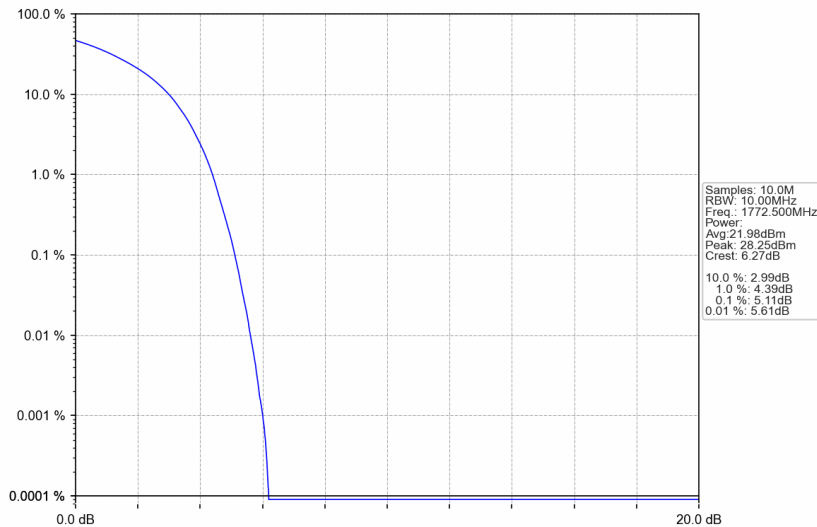
Band66_15MHz_QPSK_HCH_1772.5MHz_RB_75_0_NTNV
