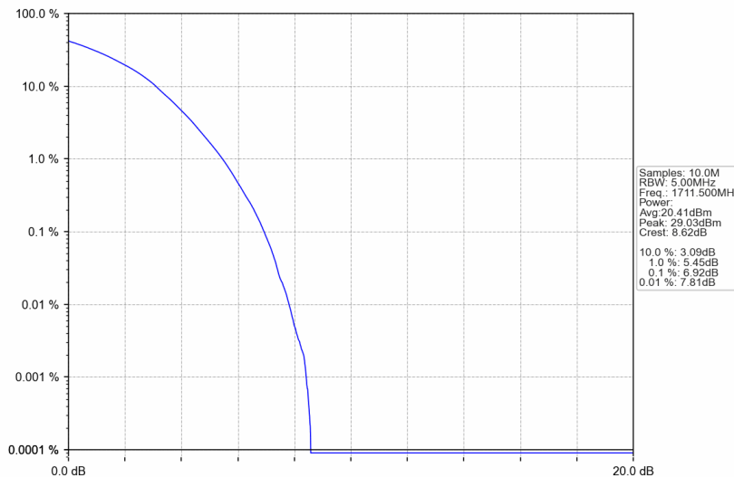
Band66_3MHz_256QAM_LCH_1711.5MHz_RB_15_0_NTNV
