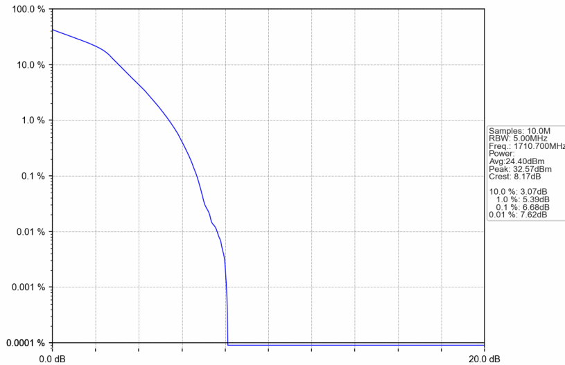
Band66_1.4MHz_16QAM_LCH_1710.7MHz_RB_6_0_NTNV
