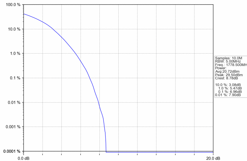
Band66_3MHz_256QAM_HCH_1778.5MHz_RB_15_0_NTNV
