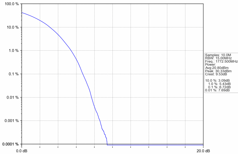
Band66_15MHz_256QAM_HCH_1772.5MHz_RB_75_0_NTNV
