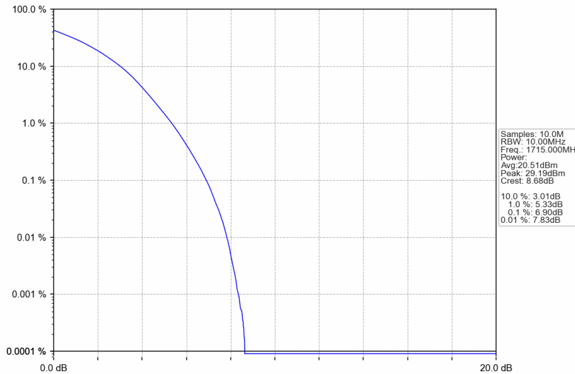
Band66_10MHz_256QAM_LCH_1715MHz_RB_50_0_NTNV
