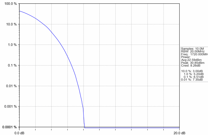
Band66_20MHz_64QAM_LCH_1720MHz_RB_100_0_NTNV
