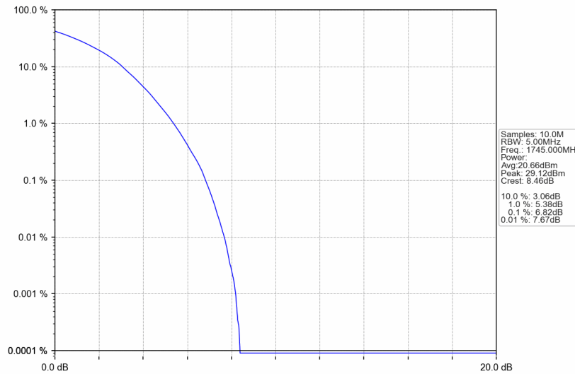
Band66_3MHz_256QAM_MCH_1745MHz_RB_15_0_NTNV
