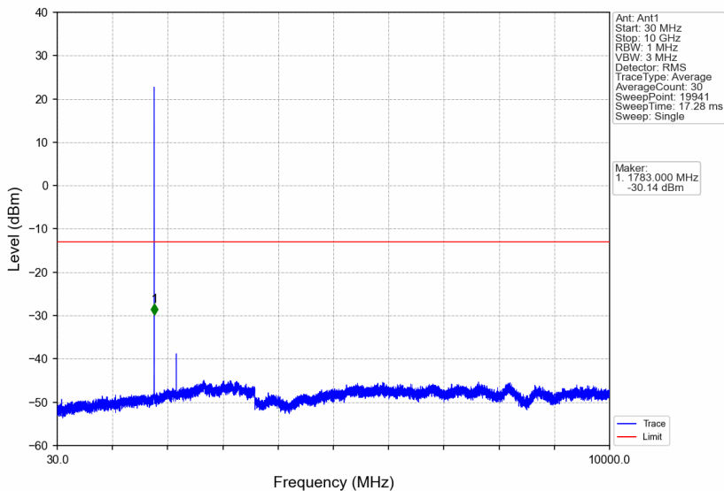
Band66_1.4MHz_64QAM_HCH_1779.3MHz_RB_1_0_NTNV
