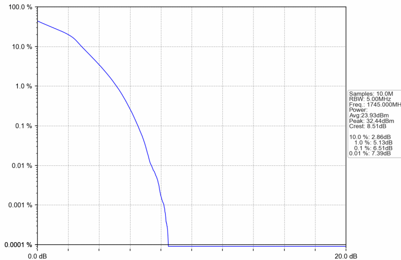
Band66_5MHz_16QAM_MCH_1745MHz_RB_25_0_NTNV
