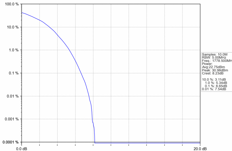
Band66_3MHz_64QAM_HCH_1778.5MHz_RB_15_0_NTNV
