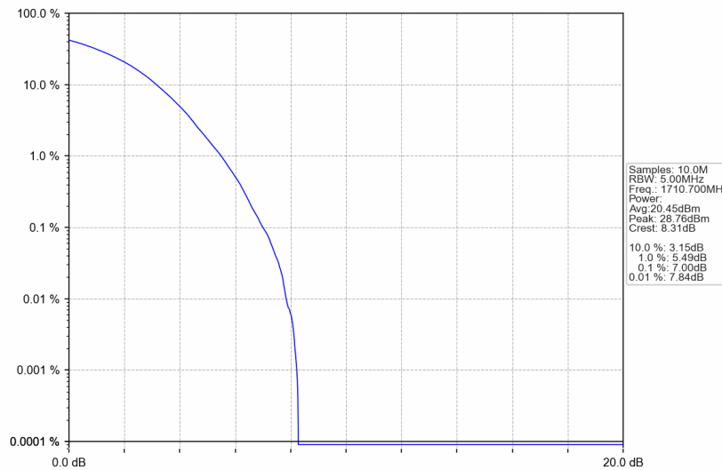
Band66_1.4MHz_256QAM_LCH_1710.7MHz_RB_6_0_NTNV
