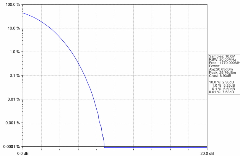
Band66_20MHz_256QAM_HCH_1770MHz_RB_100_0_NTNV
