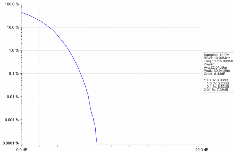
Band66_10MHz_64QAM_LCH_1715MHz_RB_50_0_NTNV
