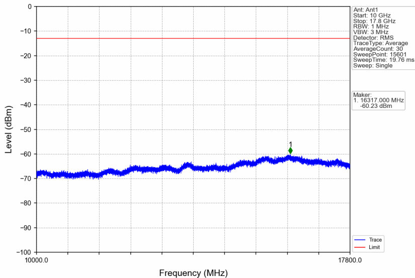
Band66_1.4MHz_256QAM_MCH_1745MHz_RB_1_0_NTNV
