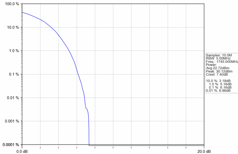
Band66_1.4MHz_64QAM_MCH_1745MHz_RB_6_0_NTNV
