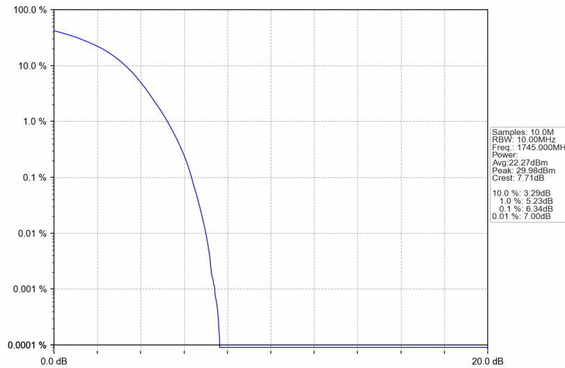
Band66_15MHz_16QAM_MCH_1745MHz_RB_75_0_NTNV
