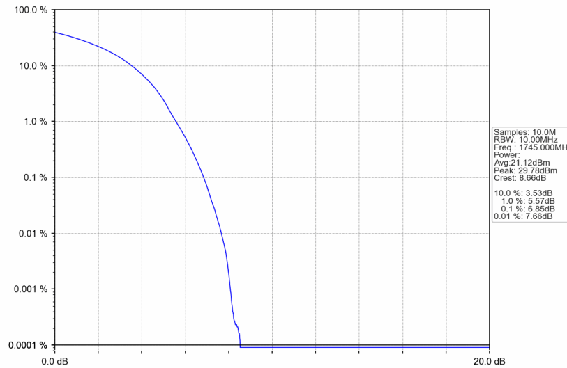
Band66_20MHz_16QAM_MCH_1745MHz_RB_100_0_NTNV
