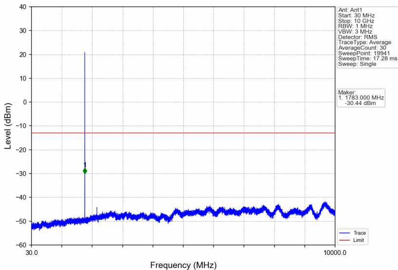
Band66_1.4MHz_16QAM_HCH_1779.3MHz_RB_1_0_NTNV
