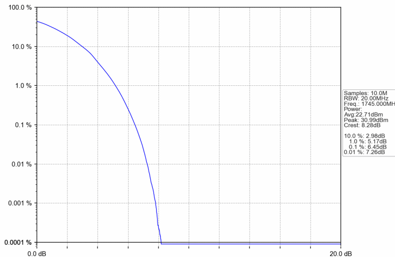
Band66_20MHz_64QAM_MCH_1745MHz_RB_100_0_NTNV
