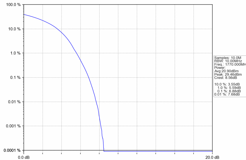
Band66_20MHz_16QAM_HCH_1770MHz_RB_100_0_NTNV
