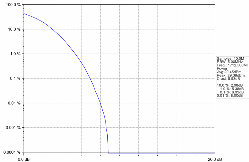
Band66_5MHz_256QAM_LCH_1712.5MHz_RB_25_0_NTNV
