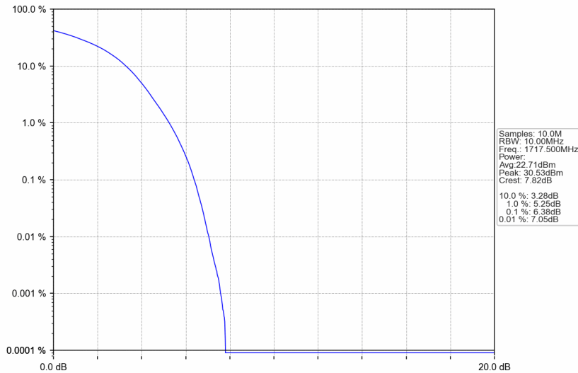
Band66_15MHz_16QAM_LCH_1717.5MHz_RB_75_0_NTNV
