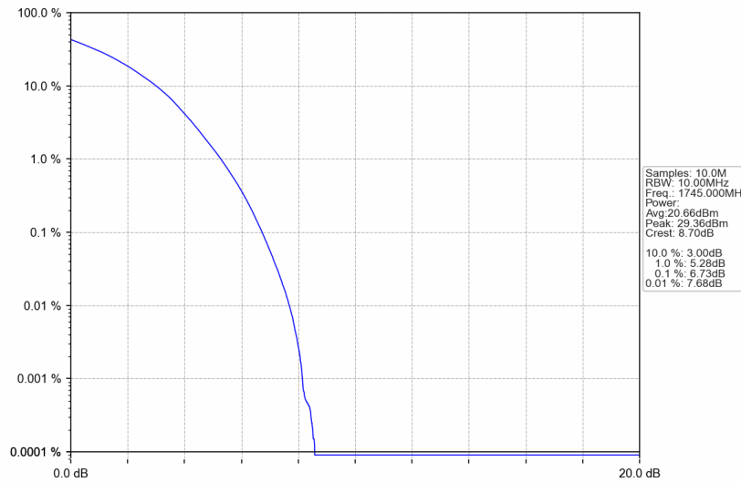
Band66_10MHz_256QAM_MCH_1745MHz_RB_50_0_NTNV
