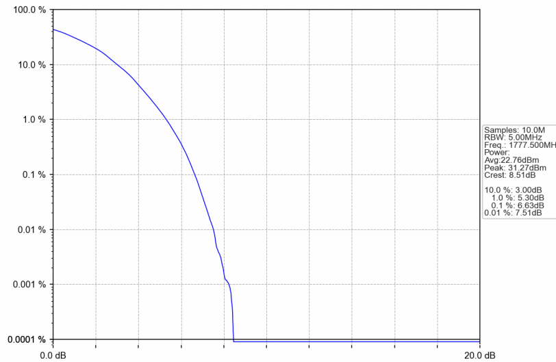
Band66_5MHz_64QAM_HCH_1777.5MHz_RB_25_0_NTNV
