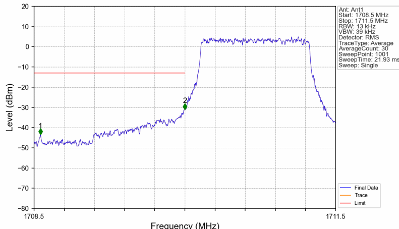
Band66_1.4MHz_QPSK_LCH_1710.7MHz_RB_6_0_NTNV
