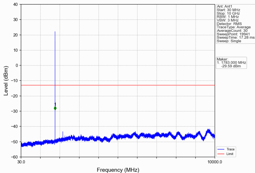
Band66_1.4MHz_QPSK_HCH_1779.3MHz_RB_1_0_NTNV
