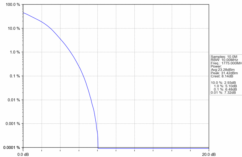
Band66_10MHz_16QAM_HCH_1775MHz_RB_50_0_NTNV
