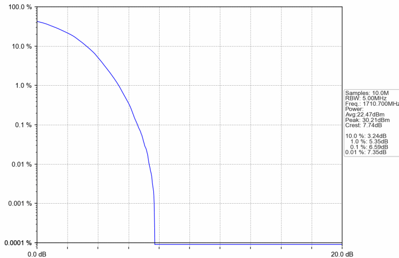
Band66_1.4MHz_64QAM_LCH_1710.7MHz_RB_6_0_NTNV
