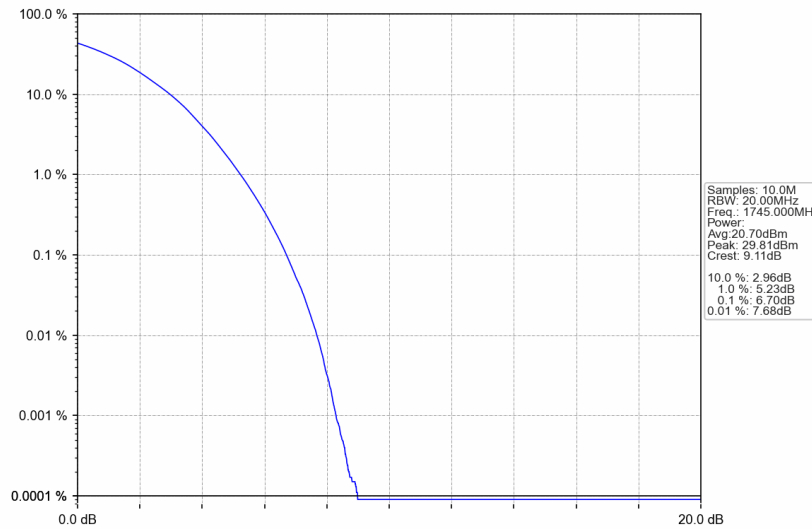
Band66_20MHz_256QAM_MCH_1745MHz_RB_100_0_NTNV
