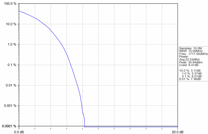
Band66_15MHz_64QAM_LCH_1717.5MHz_RB_75_0_NTNV
