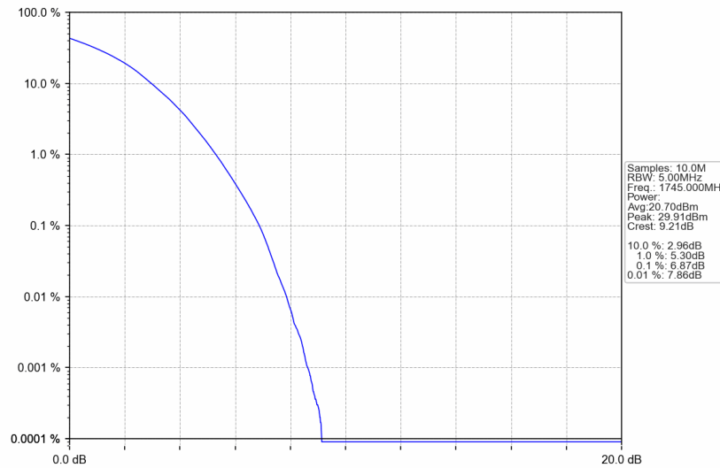
Band66_5MHz_256QAM_MCH_1745MHz_RB_25_0_NTNV
