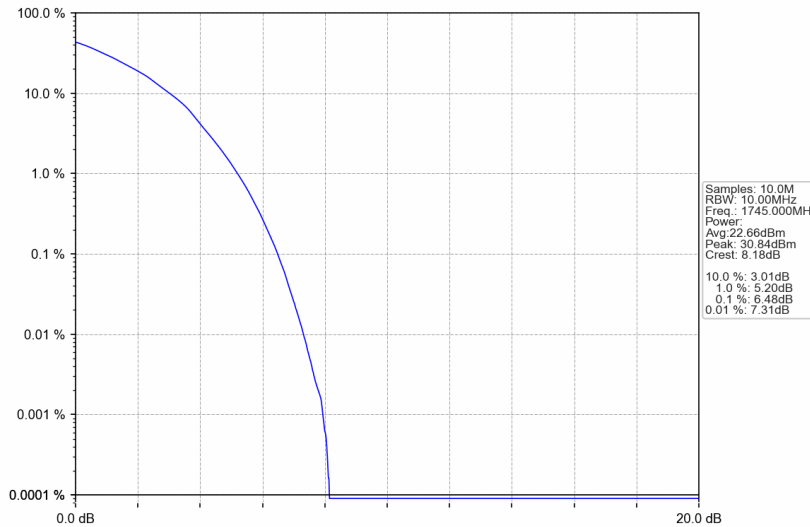
Band66_10MHz_64QAM_MCH_1745MHz_RB_50_0_NTNV
