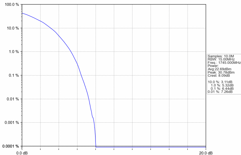
Band66_15MHz_64QAM_MCH_1745MHz_RB_75_0_NTNV
