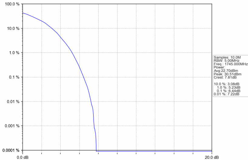
Band66_3MHz_64QAM_MCH_1745MHz_RB_15_0_NTNV
