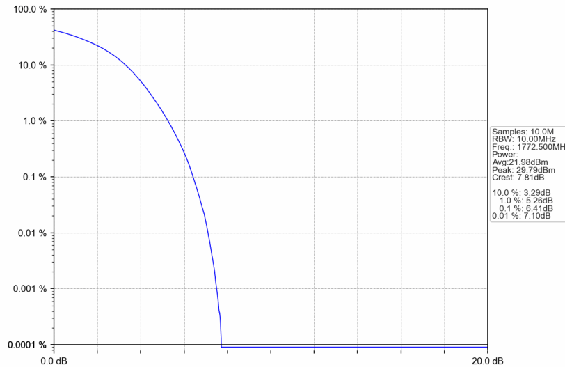
Band66_15MHz_16QAM_HCH_1772.5MHz_RB_75_0_NTNV
