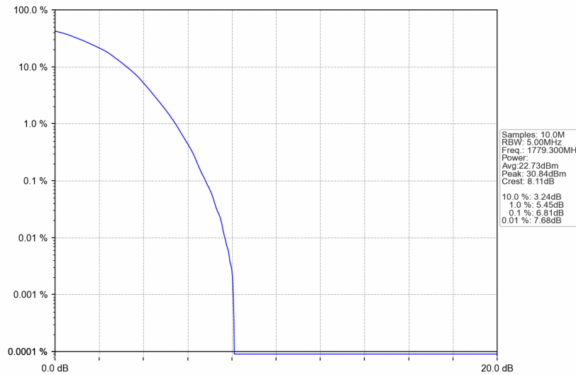
Band66_1.4MHz_64QAM_HCH_1779.3MHz_RB_6_0_NTNV
