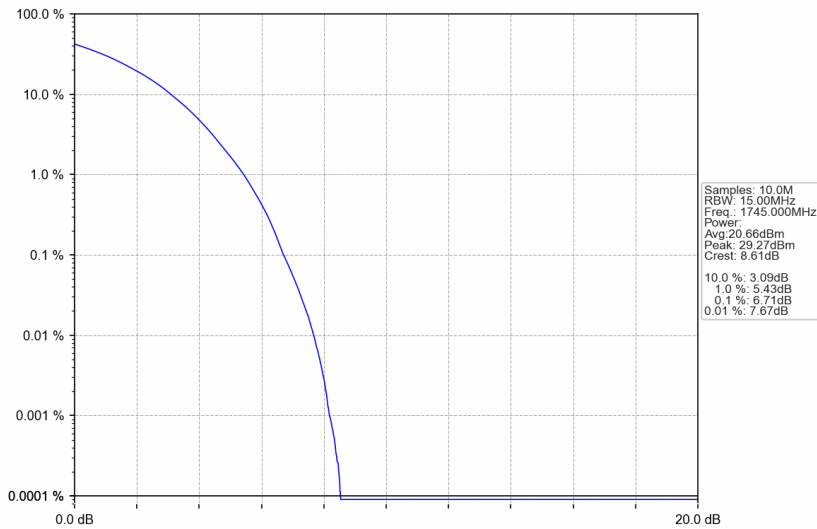
Band66_15MHz_256QAM_MCH_1745MHz_RB_75_0_NTNV
