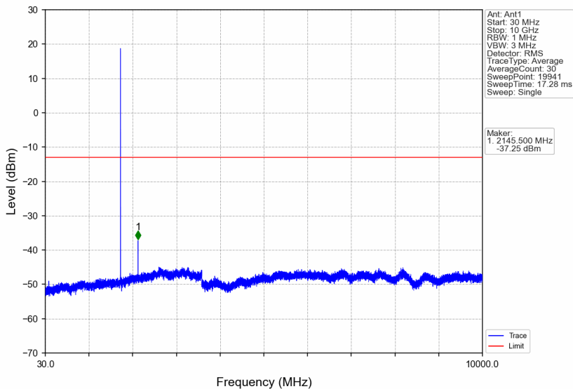
Band66_1.4MHz_256QAM_MCH_1745MHz_RB_1_0_NTNV
