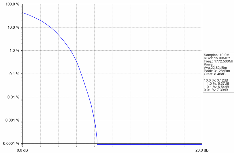
Band66_15MHz_64QAM_HCH_1772.5MHz_RB_75_0_NTNV
