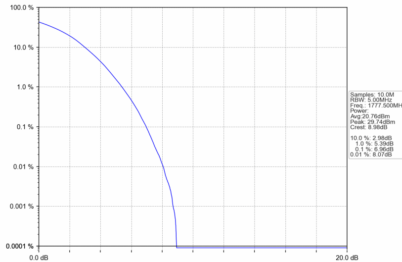
Band66_5MHz_256QAM_HCH_1777.5MHz_RB_25_0_NTNV
