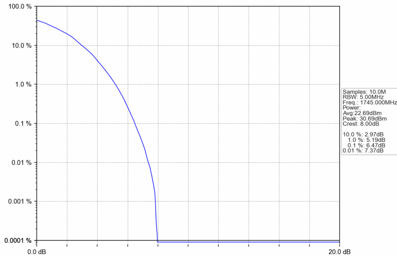
Band66_5MHz_64QAM_MCH_1745MHz_RB_25_0_NTNV
