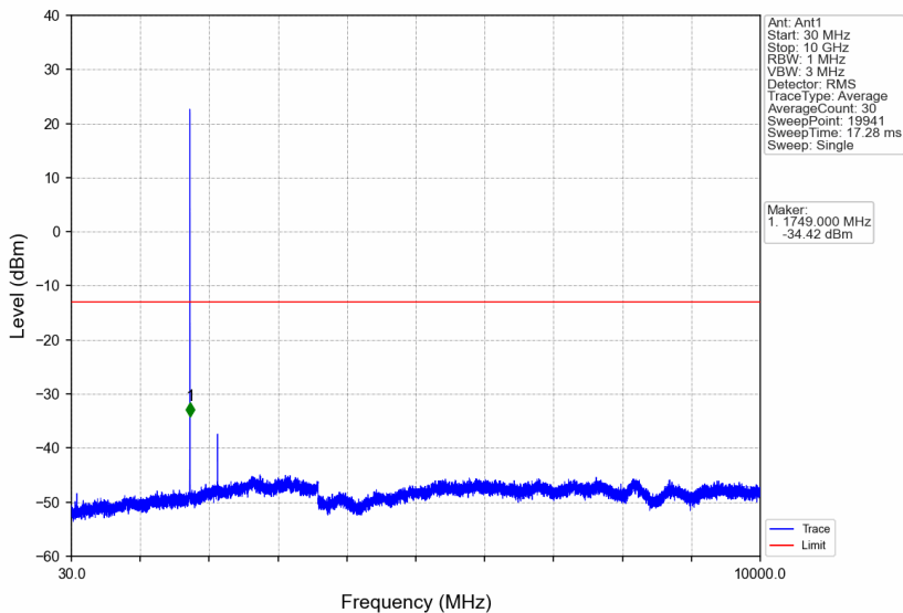
Band66_1.4MHz_64QAM_MCH_1745MHz_RB_1_0_NTNV
