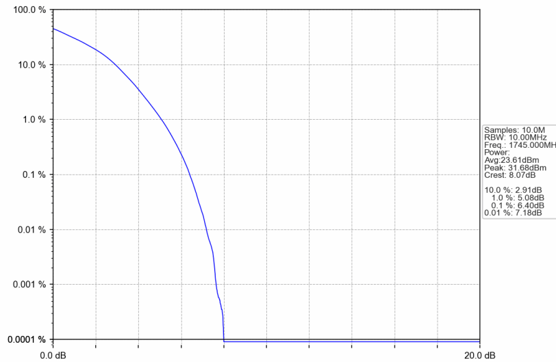
Band66_10MHz_16QAM_MCH_1745MHz_RB_50_0_NTNV
