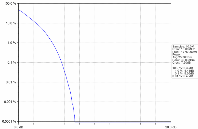
Band66_10MHz_QPSK_HCH_1775MHz_RB_50_0_NTNV
