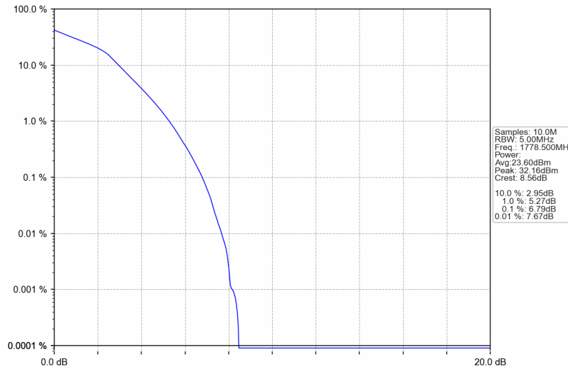
Band66_3MHz_16QAM_HCH_1778.5MHz_RB_15_0_NTNV
