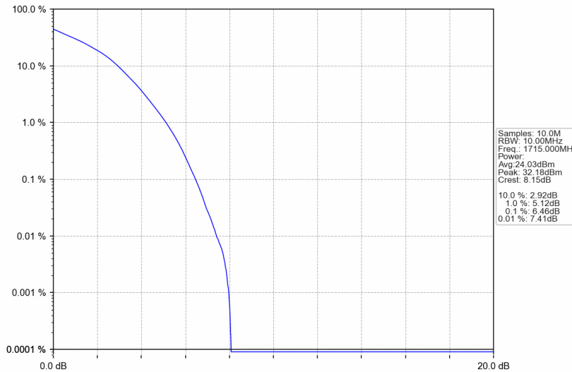
Band66_10MHz_16QAM_LCH_1715MHz_RB_50_0_NTNV
