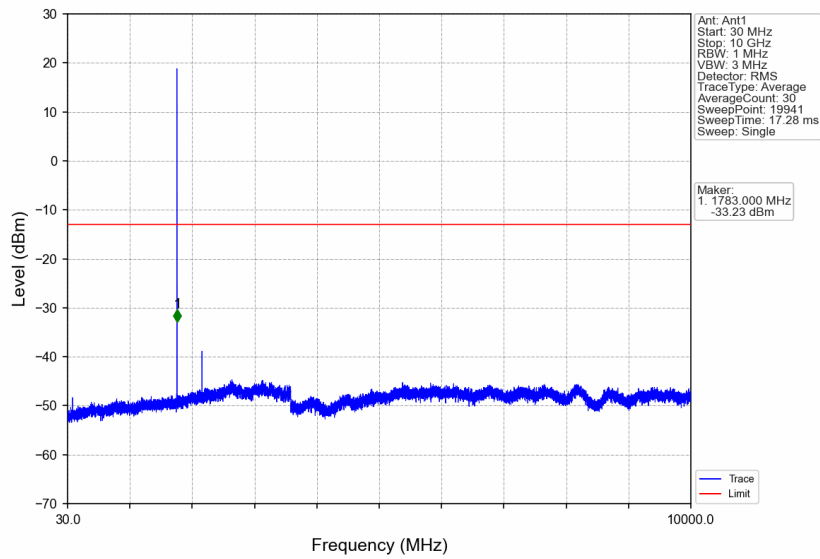
Band66_1.4MHz_256QAM_HCH_1779.3MHz_RB_1_0_NTNV
