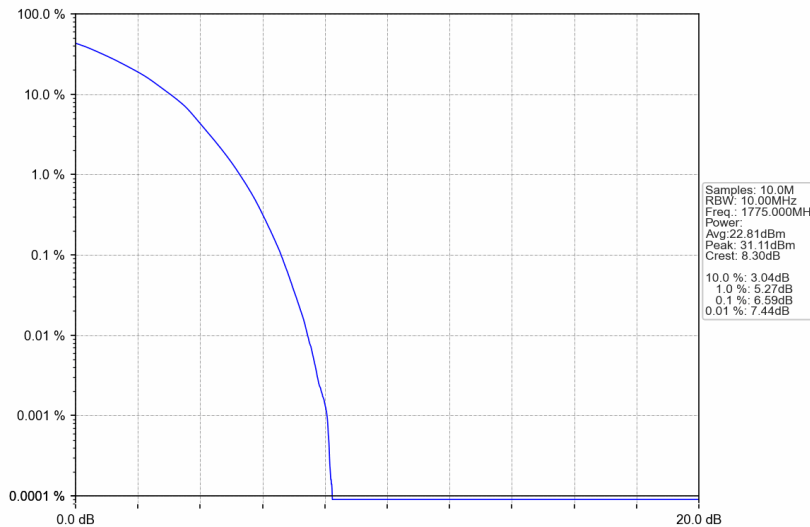
Band66_10MHz_64QAM_HCH_1775MHz_RB_50_0_NTNV
