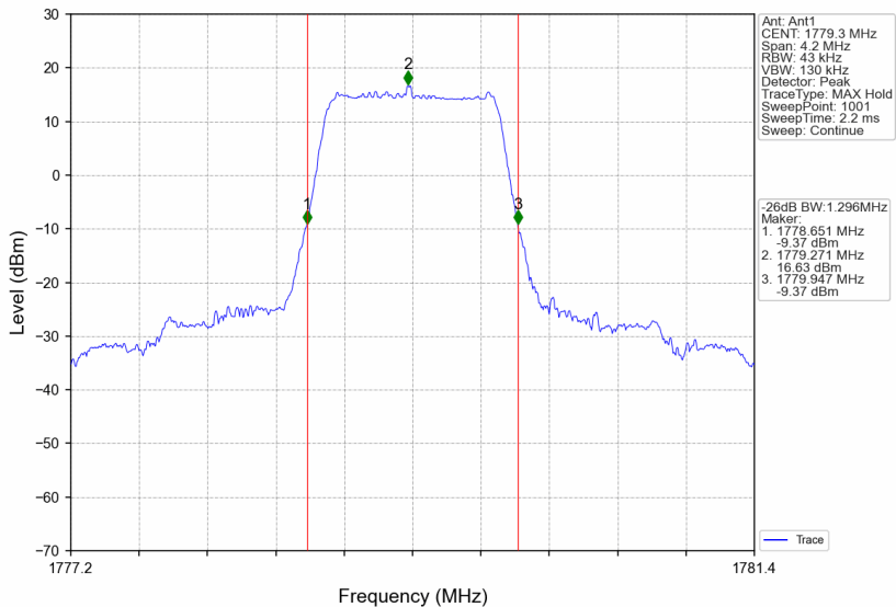
Band66_1.4MHz_256QAM_HCH_1779.3MHz_RB_6_0_NTNV
