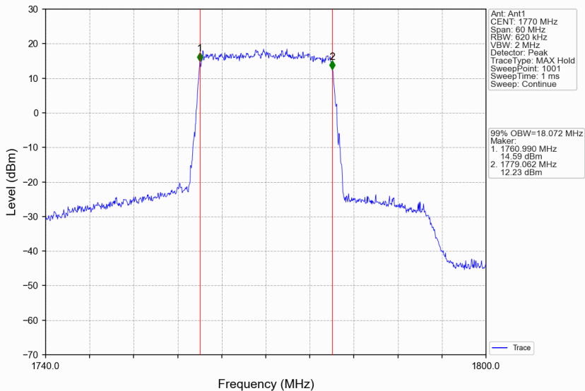
Band66_20MHz_16QAM_HCH_1770MHz_RB_100_0_NTNV
