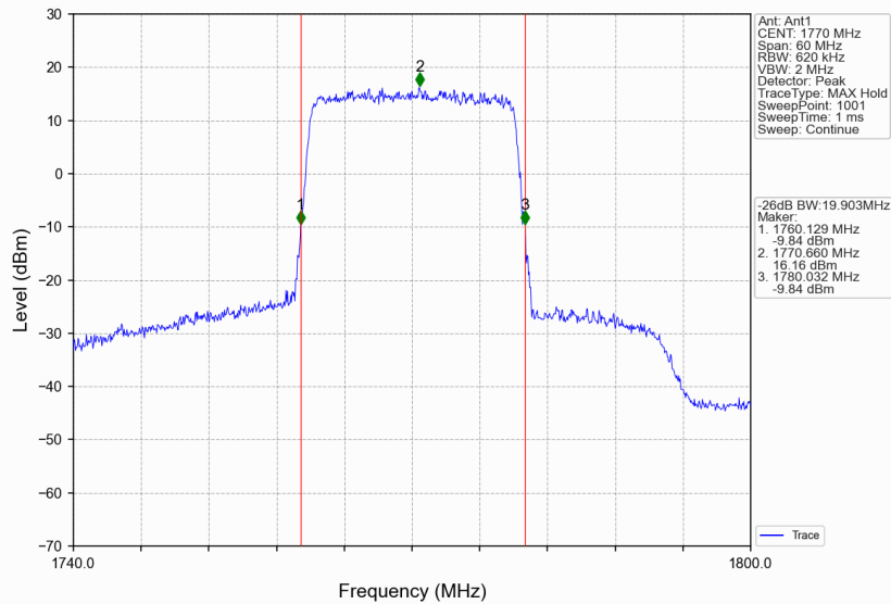
Band66_20MHz_256QAM_HCH_1770MHz_RB_100_0_NTNV
