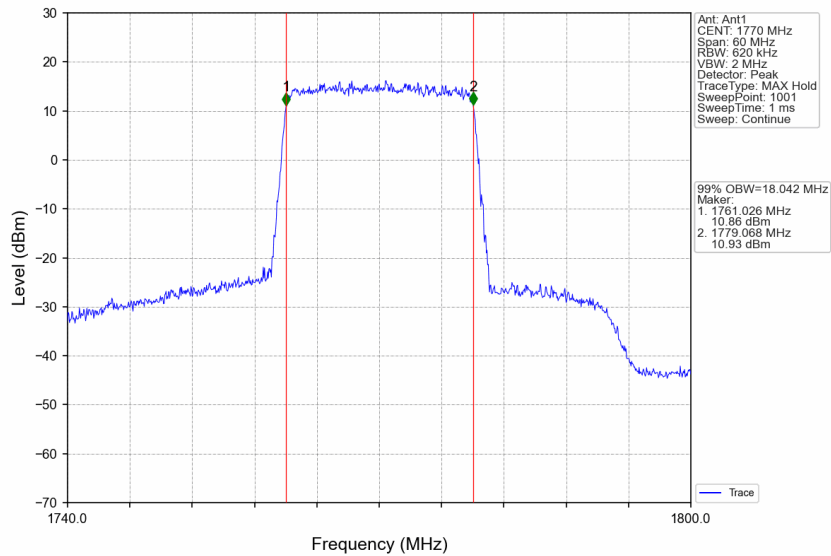
Band66_20MHz_256QAM_HCH_1770MHz_RB_100_0_NTNV
