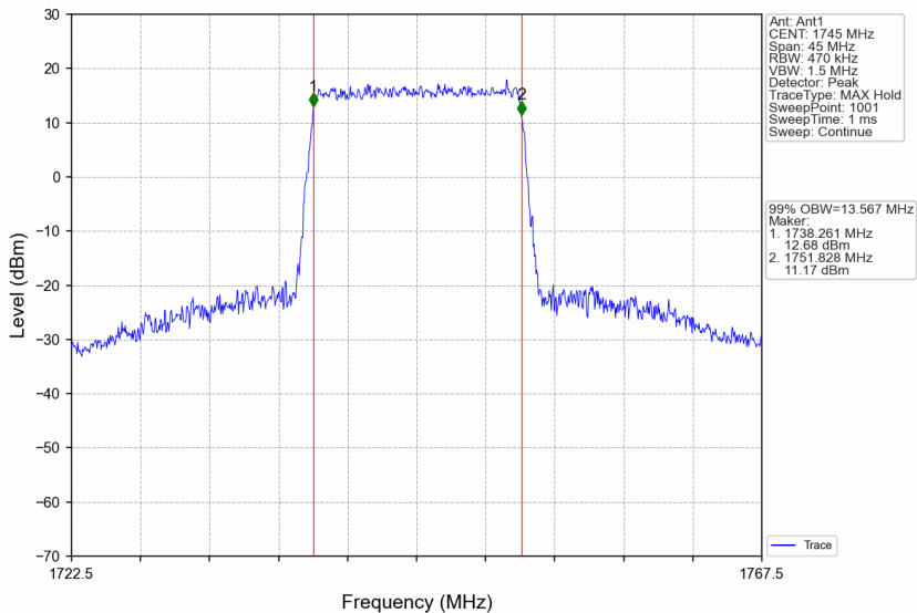
Band66_15MHz_64QAM_MCH_1745MHz_RB_75_0_NTNV
