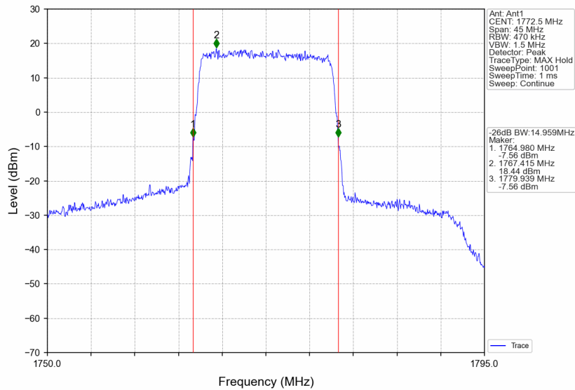
Band66_15MHz_16QAM_HCH_1772.5MHz_RB_75_0_NTNV
