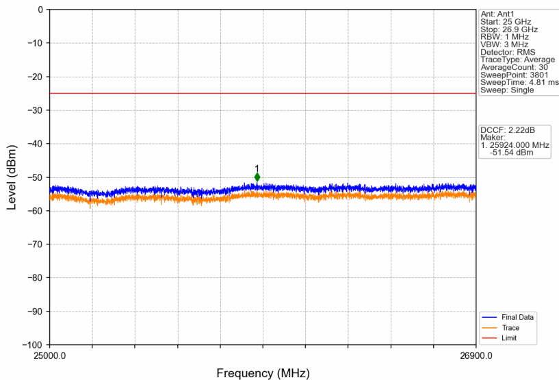
Band41_20MHz_256QAM_LCH_2506MHz_RB_100_0_NTNV
