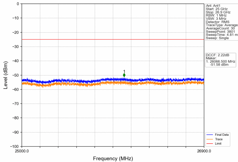
Band41_20MHz_256QAM_HCH_2680MHz_RB_1_0_NTNV
