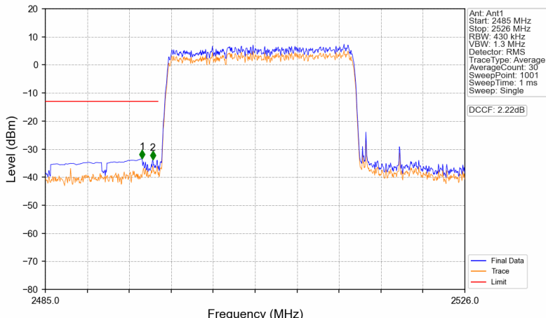
Band41_20MHz_256QAM_LCH_2506MHz_RB_100_0_NTNV
