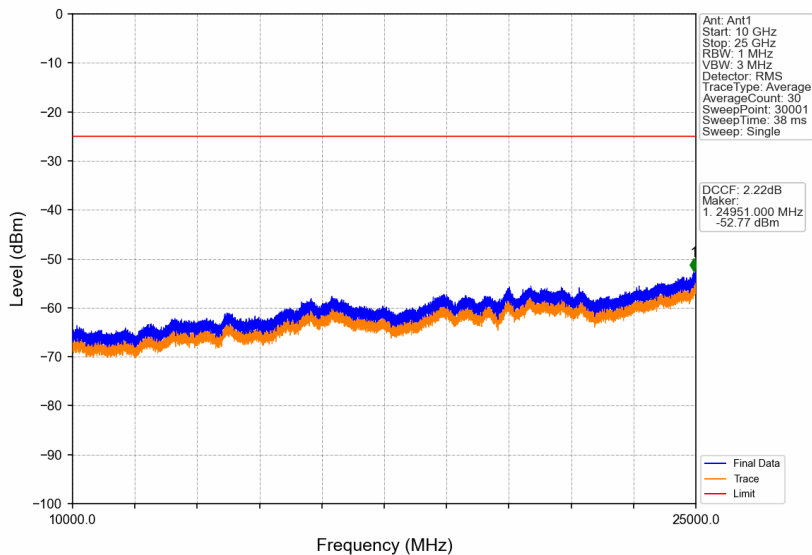
Band41_10MHz_64QAM_MCH_2593MHz_RB_1_0_NTNV
