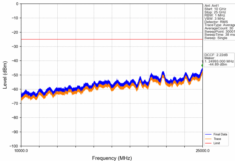
Band41_5MHz_16QAM_MCH_2593MHz_RB_1_0_NTNV
