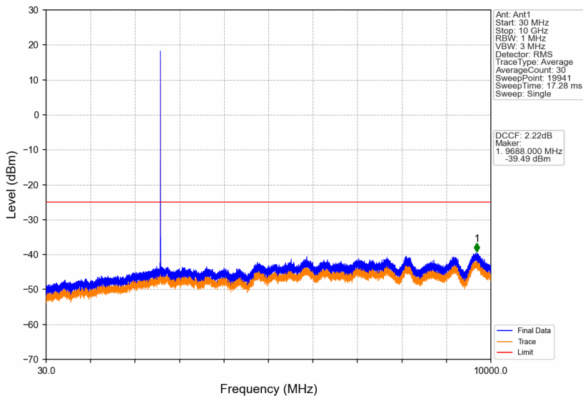
Band41_5MHz_16QAM_MCH_2593MHz_RB_1_0_NTNV
