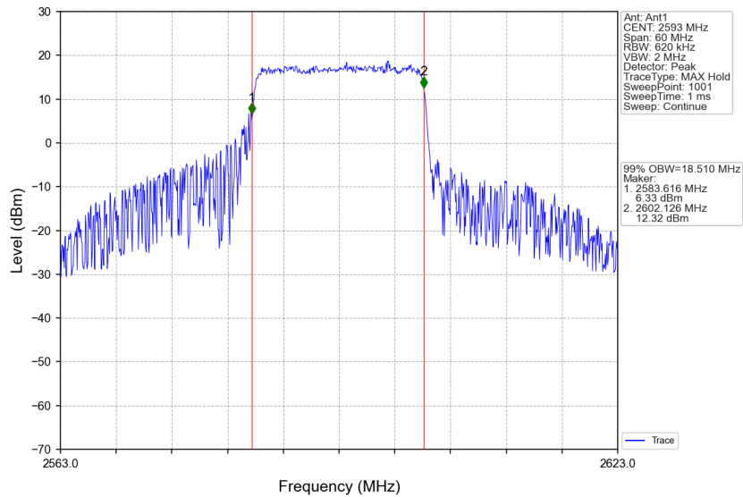
Band41_20MHz_64QAM_MCH_2593MHz_RB_100_0_NTNV
