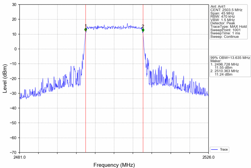
Band41_15MHz_256QAM_LCH_2503.5MHz_RB_75_0_NTNV
