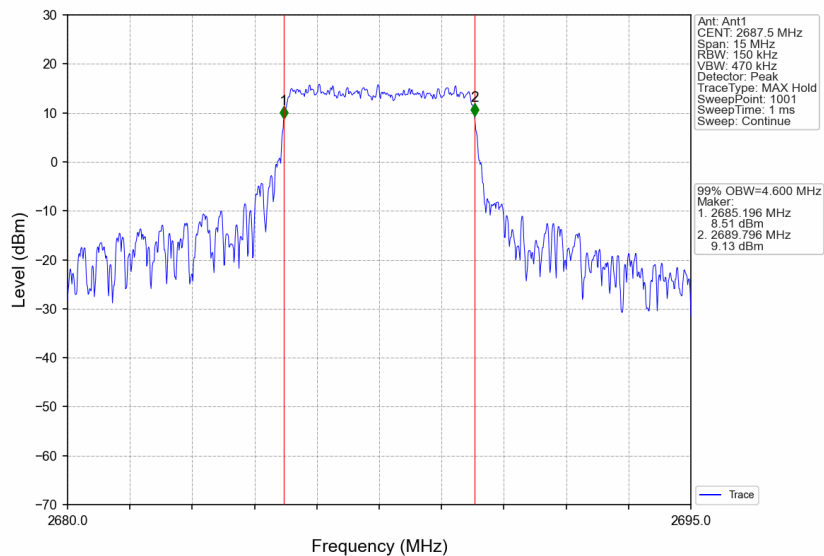
Band41_5MHz_256QAM_HCH_2687.5MHz_RB_25_0_NTNV
