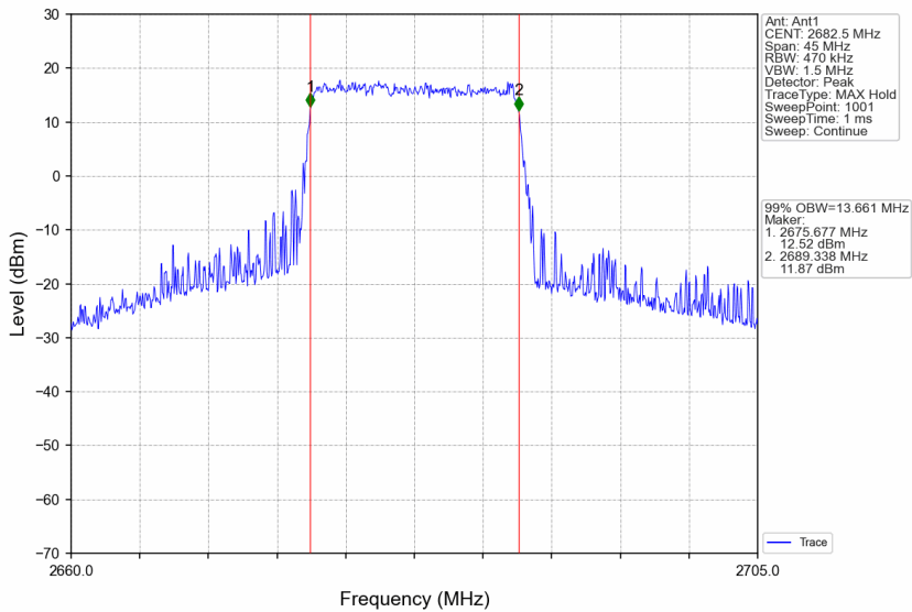
Band41_15MHz_16QAM_HCH_2682.5MHz_RB_75_0_NTNV
