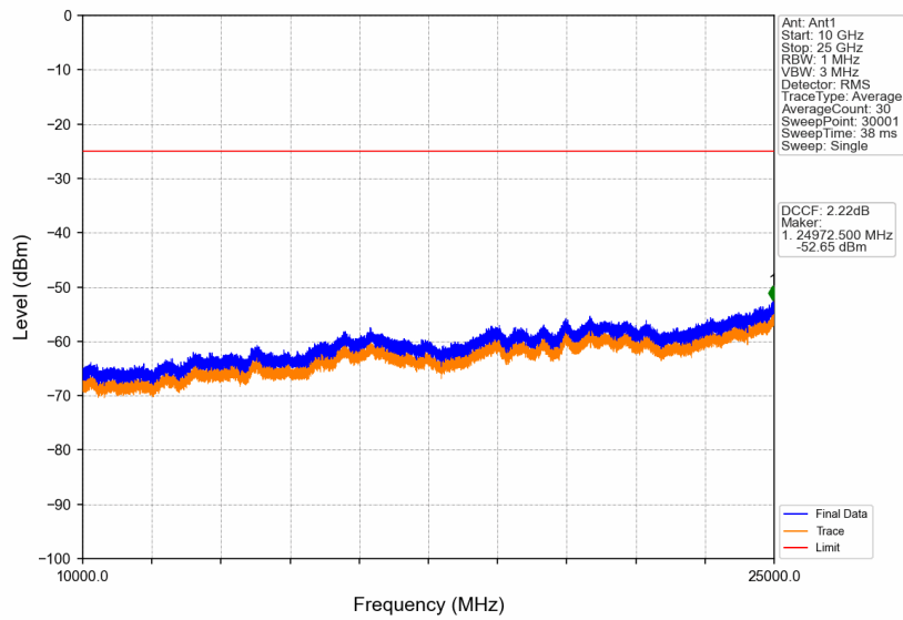
Band38_20MHz_64QAM_LCH_2580MHz_RB_1_0_NTNV
