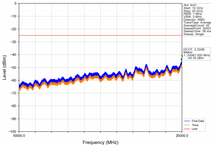
Band38_15MHz_16QAM_LCH_2577.5MHz_RB_1_0_NTNV
