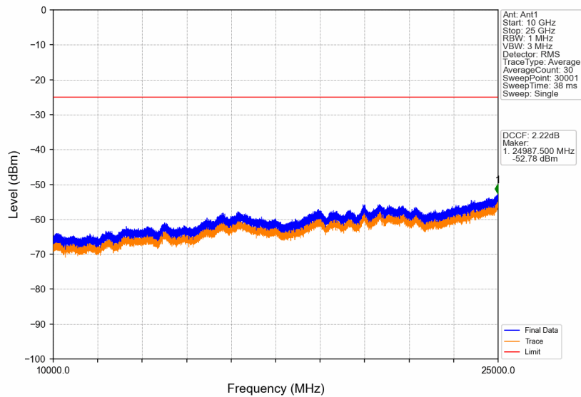
Band38_15MHz_256QAM_HCH_2612.5MHz_RB_1_0_NTNV
