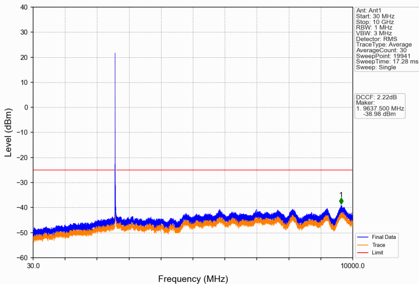
Band38_15MHz_16QAM_MCH_2595MHz_RB_1_0_NTNV
