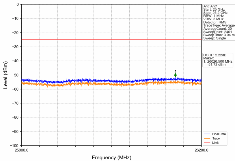
Band38_15MHz_256QAM_HCH_2612.5MHz_RB_1_0_NTNV
