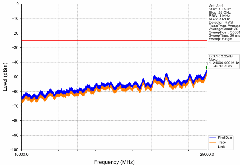
Band38_15MHz_16QAM_MCH_2595MHz_RB_1_0_NTNV
