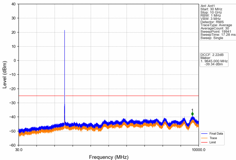
Band38_15MHz_16QAM_LCH_2577.5MHz_RB_1_0_NTNV
