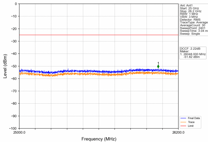
Band38_10MHz_256QAM_HCH_2615MHz_RB_1_0_NTNV
