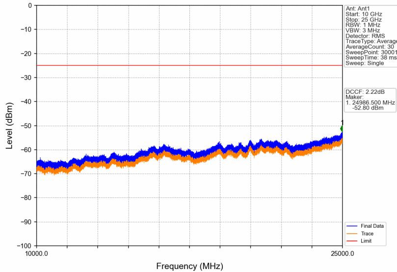
Band38_15MHz_256QAM_LCH_2577.5MHz_RB_1_0_NTNV
