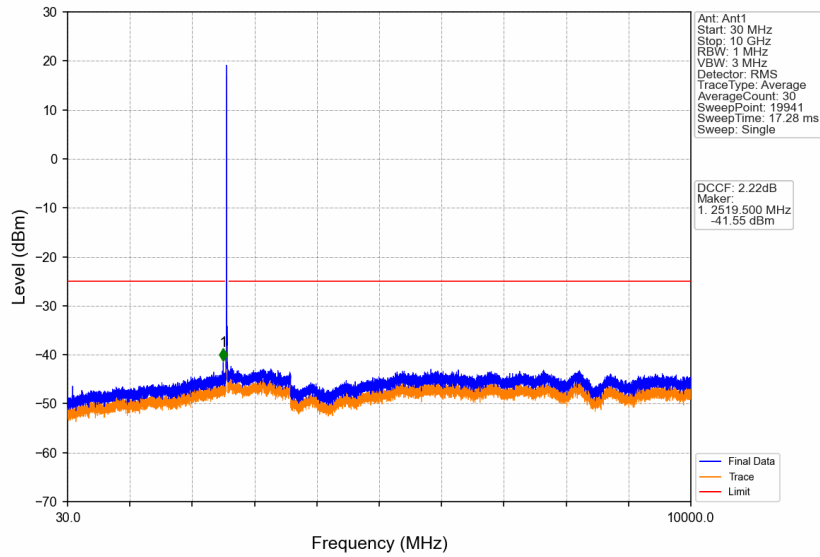
Band38_15MHz_256QAM_LCH_2577.5MHz_RB_1_0_NTNV
