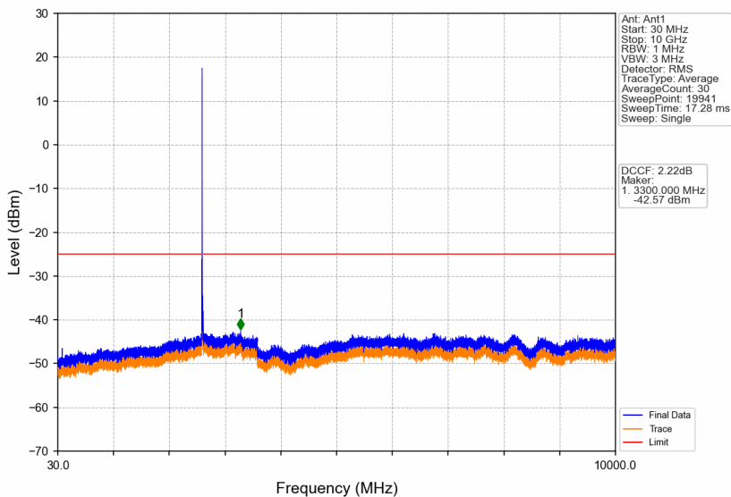
Band38_10MHz_256QAM_HCH_2615MHz_RB_1_0_NTNV
