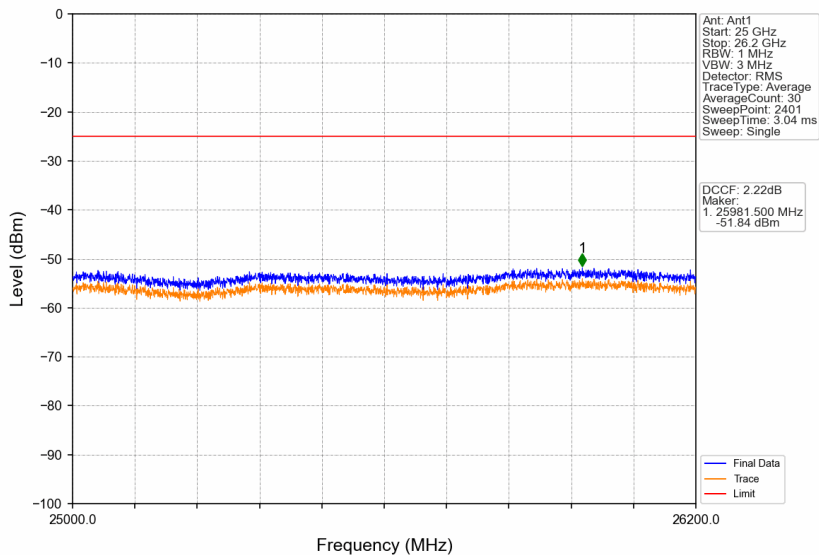
Band38_15MHz_256QAM_HCH_2612.5MHz_RB_1_0_NTNV
