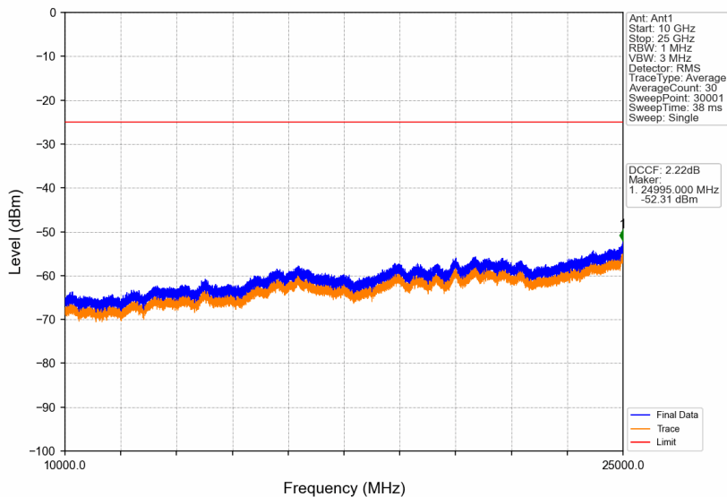
Band38_15MHz_64QAM_LCH_2577.5MHz_RB_1_0_NTNV
