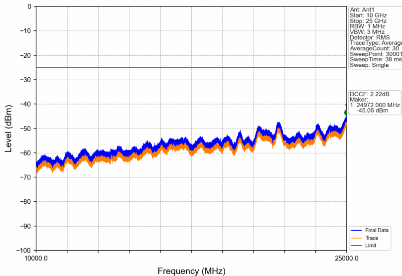
Band38_10MHz_16QAM_LCH_2575MHz_RB_1_0_NTNV
