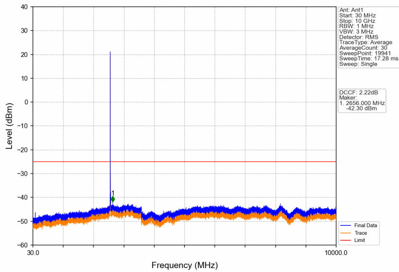
Band38_10MHz_256QAM_LCH_2575MHz_RB_1_0_NTNV
