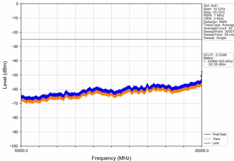
Band38_5MHz_256QAM_LCH_2572.5MHz_RB_1_0_NTNV
