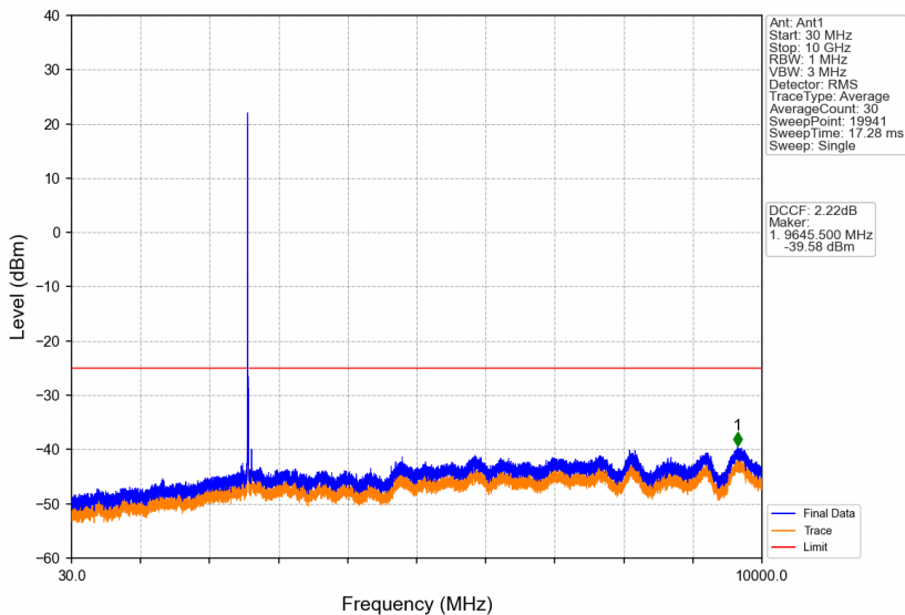
Band38_10MHz_16QAM_LCH_2575MHz_RB_1_0_NTNV
