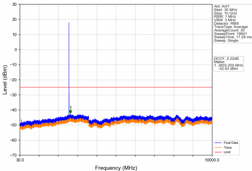
Band38_5MHz_256QAM_LCH_2572.5MHz_RB_1_0_NTNV
