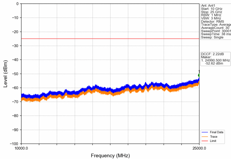
Band38_10MHz_256QAM_LCH_2575MHz_RB_1_0_NTNV
