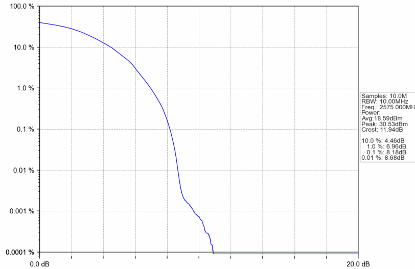
Band38_10MHz_64QAM_LCH_2575MHz_RB_50_0_NTNV
