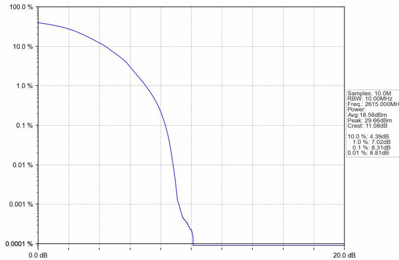
Band38_10MHz_64QAM_HCH_2615MHz_RB_50_0_NTNV
