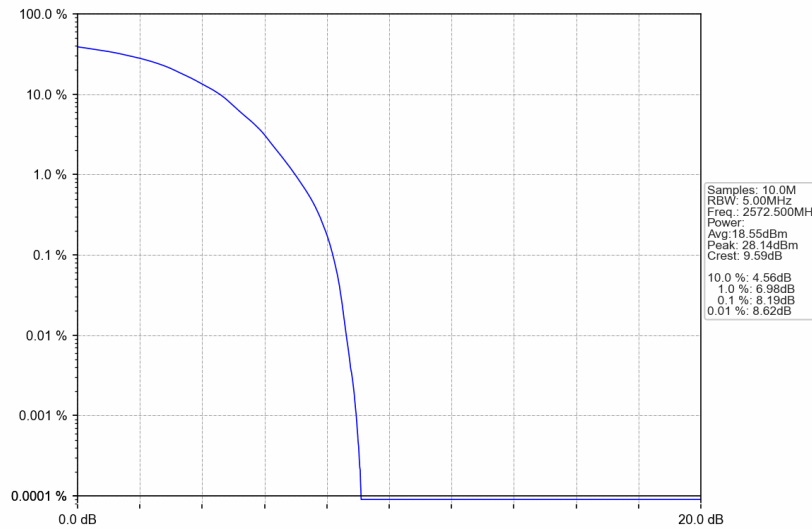
Band38_5MHz_64QAM_LCH_2572.5MHz_RB_25_0_NTNV
