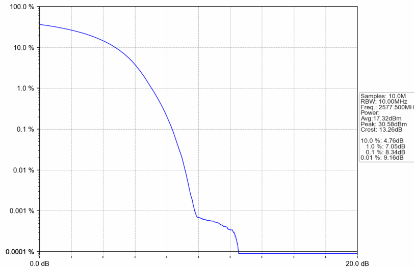
Band38_15MHz_16QAM_LCH_2577.5MHz_RB_75_0_NTNV
