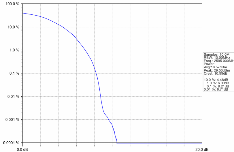
Band38_10MHz_64QAM_MCH_2595MHz_RB_50_0_NTNV
