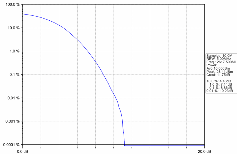
Band38_5MHz_256QAM_HCH_2617.5MHz_RB_25_0_NTNV
