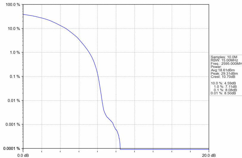
Band38_15MHz_64QAM_MCH_2595MHz_RB_75_0_NTNV
