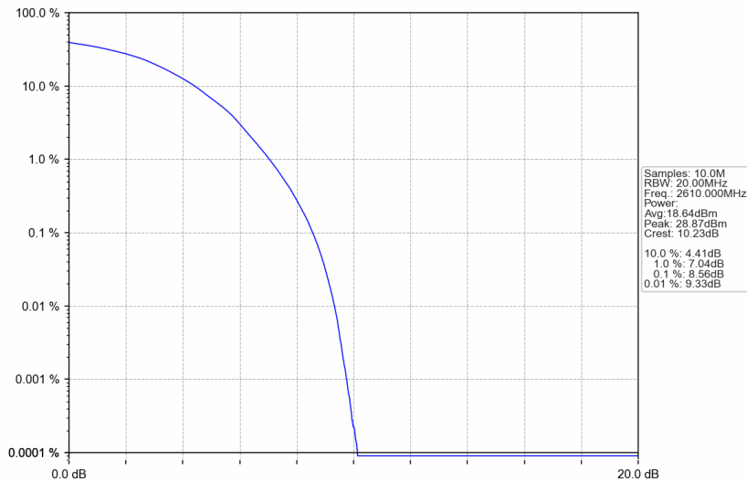
Band38_20MHz_64QAM_HCH_2610MHz_RB_100_0_NTNV
