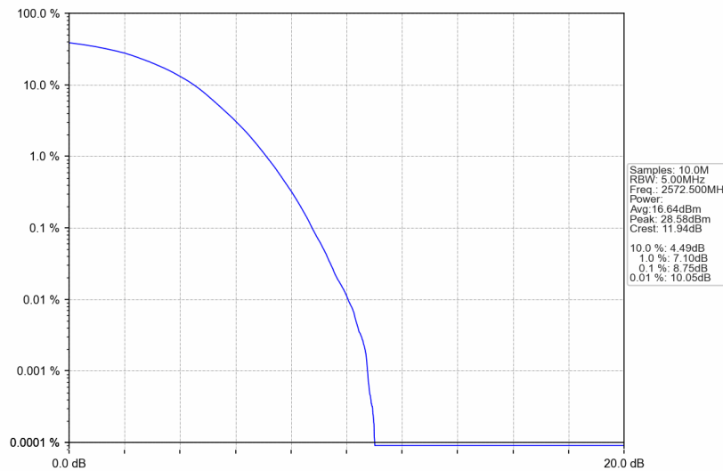
Band38_5MHz_256QAM_LCH_2572.5MHz_RB_25_0_NTNV
