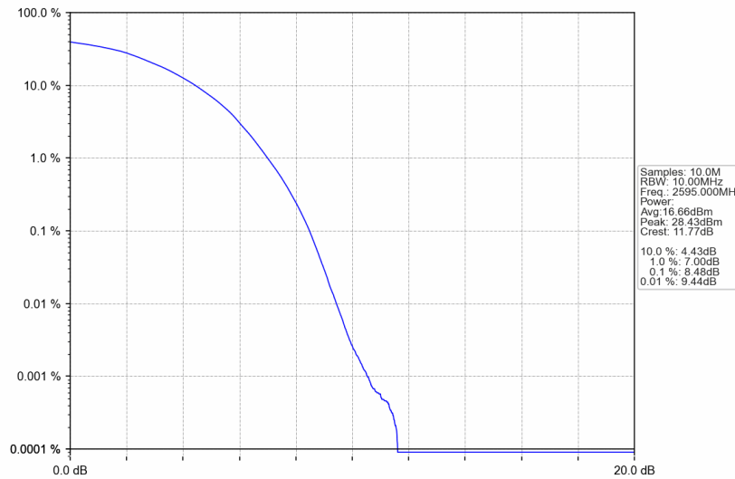
Band38_10MHz_256QAM_MCH_2595MHz_RB_50_0_NTNV
