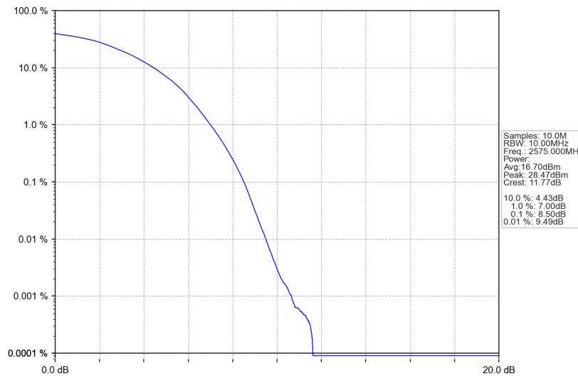
Band38_10MHz_256QAM_LCH_2575MHz_RB_50_0_NTNV
