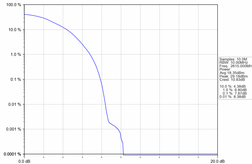
Band38_10MHz_16QAM_HCH_2615MHz_RB_50_0_NTNV
