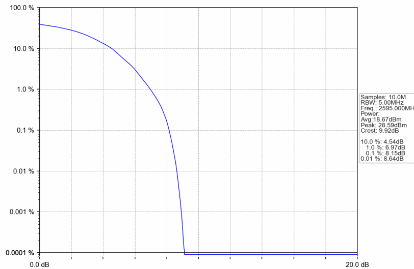
Band38_5MHz_64QAM_MCH_2595MHz_RB_25_0_NTNV
