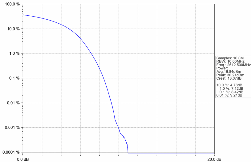
Band38_15MHz_16QAM_HCH_2612.5MHz_RB_75_0_NTNV
