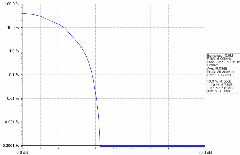
Band38_5MHz_16QAM_LCH_2572.5MHz_RB_25_0_NTNV
