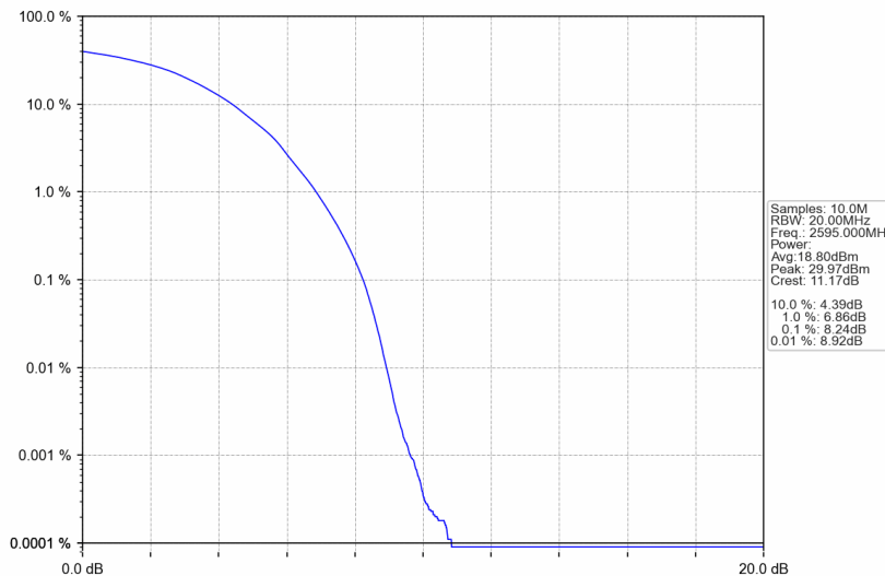
Band38_20MHz_64QAM_MCH_2595MHz_RB_100_0_NTNV
