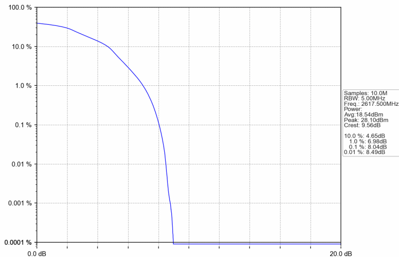
Band38_5MHz_16QAM_HCH_2617.5MHz_RB_25_0_NTNV
