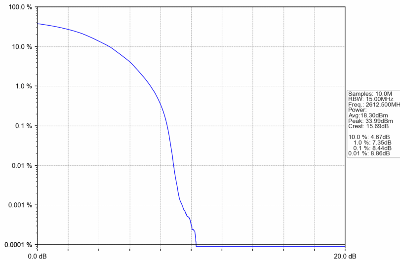
Band38_15MHz_64QAM_HCH_2612.5MHz_RB_75_0_NTNV
