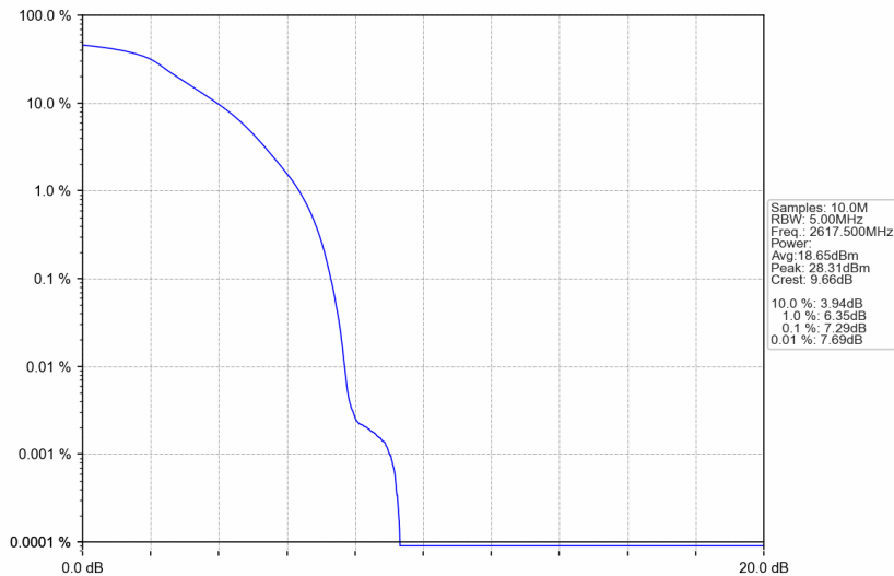
Band38_5MHz_QPSK_HCH_2617.5MHz_RB_25_0_NTNV
