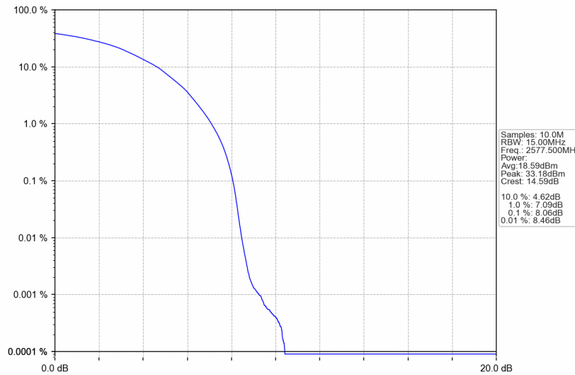
Band38_15MHz_64QAM_LCH_2577.5MHz_RB_75_0_NTNV
