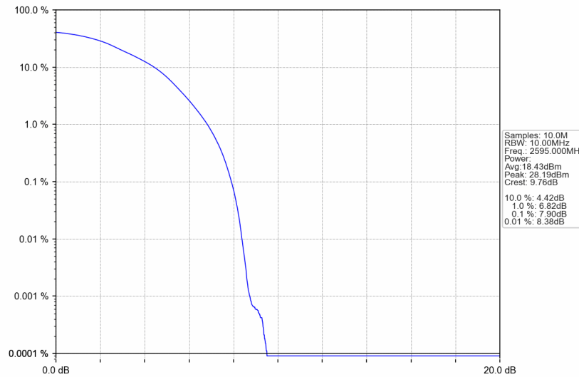
Band38_10MHz_16QAM_MCH_2595MHz_RB_50_0_NTNV
