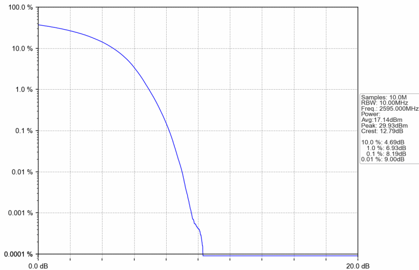
Band38_15MHz_16QAM_MCH_2595MHz_RB_75_0_NTNV
