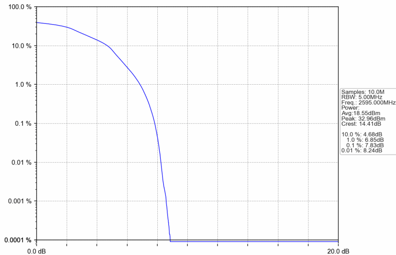
Band38_5MHz_16QAM_MCH_2595MHz_RB_25_0_NTNV
