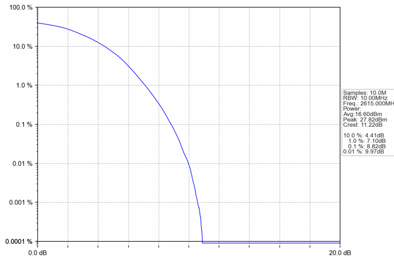
Band38_10MHz_256QAM_HCH_2615MHz_RB_50_0_NTNV
