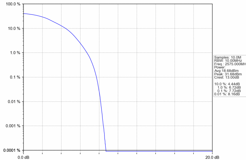
Band38_10MHz_16QAM_LCH_2575MHz_RB_50_0_NTNV
