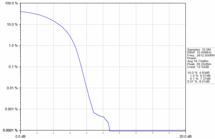
Band38_15MHz_QPSK_HCH_2612.5MHz_RB_75_0_NTNV
