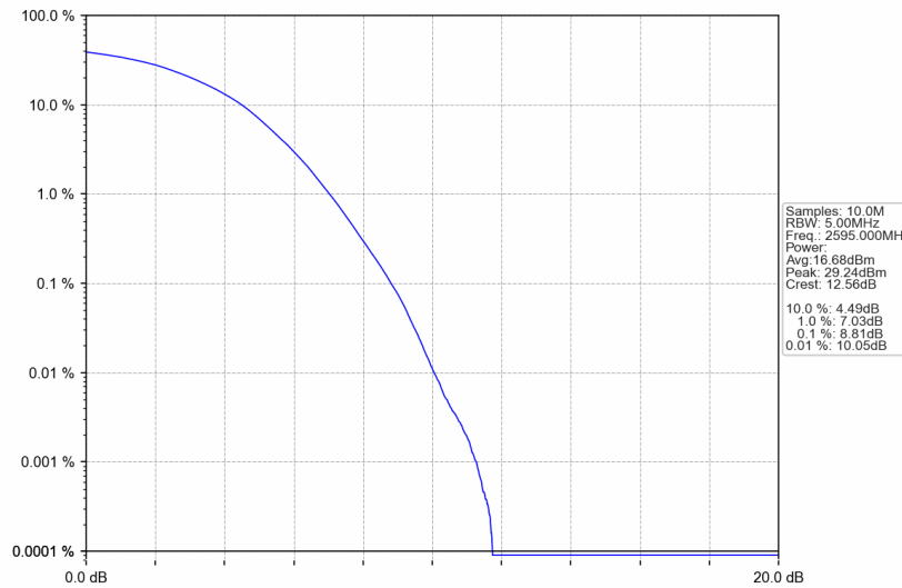
Band38_5MHz_256QAM_MCH_2595MHz_RB_25_0_NTNV
