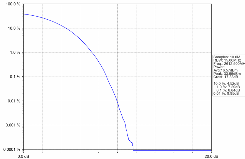
Band38_15MHz_256QAM_HCH_2612.5MHz_RB_75_0_NTNV
