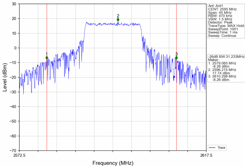
Band38_15MHz_QPSK_MCH_2595MHz_RB_75_0_NTNV
