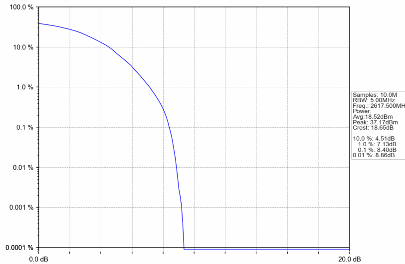
Band38_5MHz_64QAM_HCH_2617.5MHz_RB_25_0_NTNV
