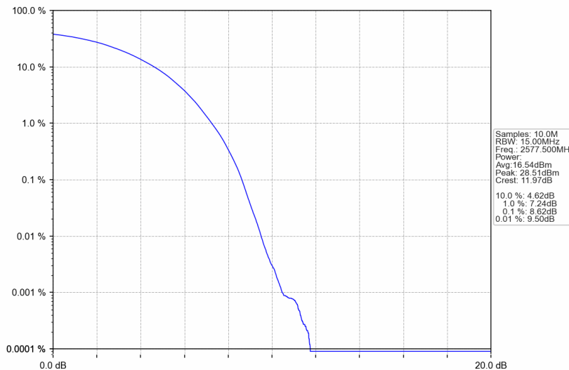
Band38_15MHz_256QAM_LCH_2577.5MHz_RB_75_0_NTNV
