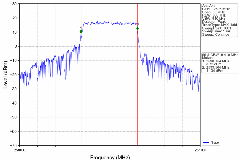
Band38_10MHz_64QAM_MCH_2595MHz_RB_50_0_NTNV
