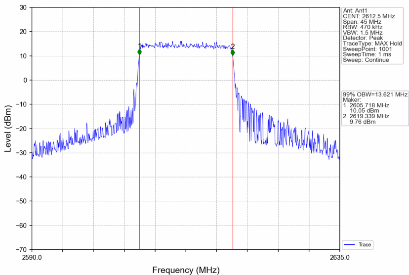
Band38_15MHz_256QAM_HCH_2612.5MHz_RB_75_0_NTNV
