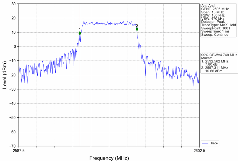
Band38_5MHz_64QAM_MCH_2595MHz_RB_25_0_NTNV
