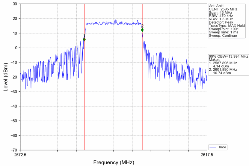
Band38_15MHz_64QAM_MCH_2595MHz_RB_75_0_NTNV
