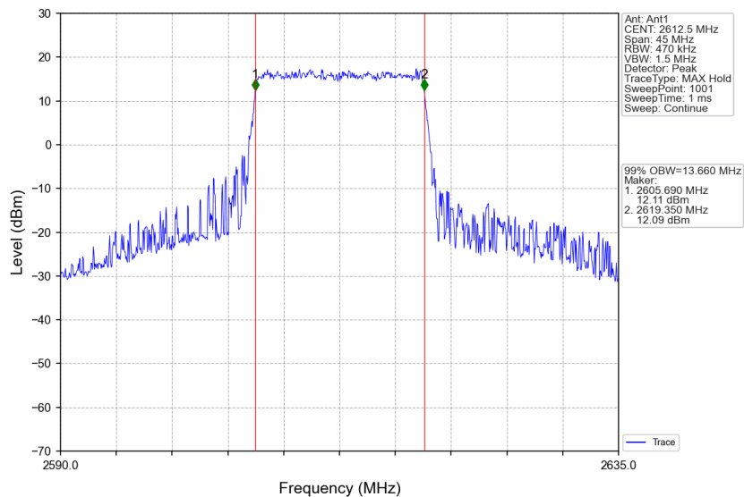
Band38_15MHz_16QAM_HCH_2612.5MHz_RB_75_0_NTNV
