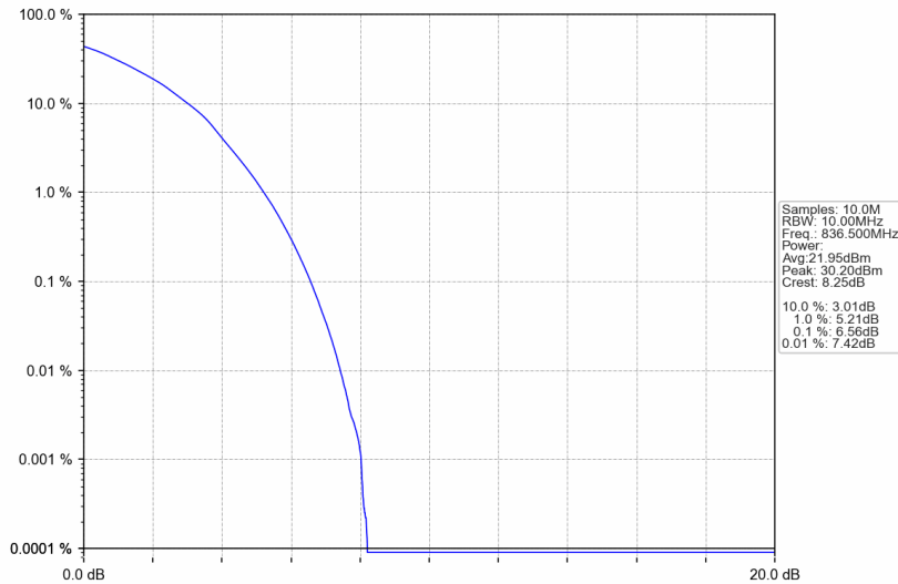
Band26b_10MHz_64QAM_MCH_836.5MHz_RB_50_0_NTNV
