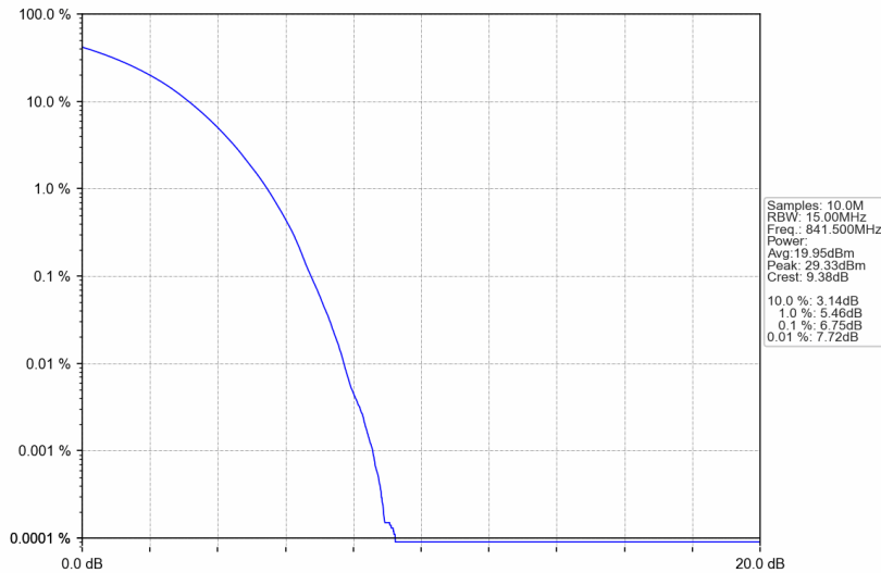
Band26c_15MHz_256QAM_HCH_841.5MHz_RB_75_0_NTNV
