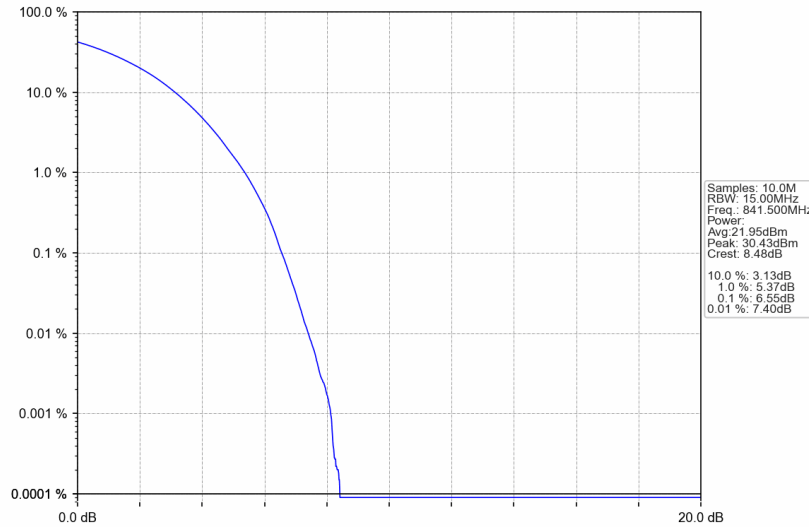
Band26c_15MHz_64QAM_HCH_841.5MHz_RB_75_0_NTNV
