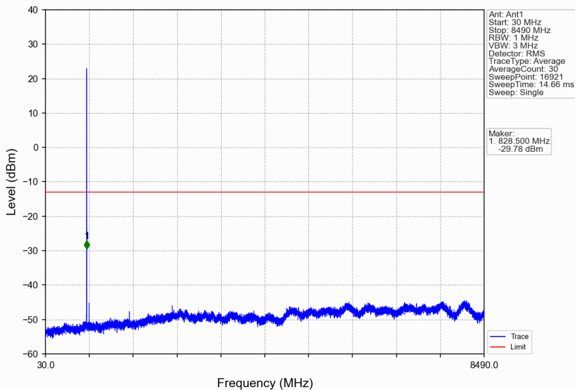
Band26b_1.4MHz_16QAM_LCH_824.7MHz_RB_6_0_NTNV
