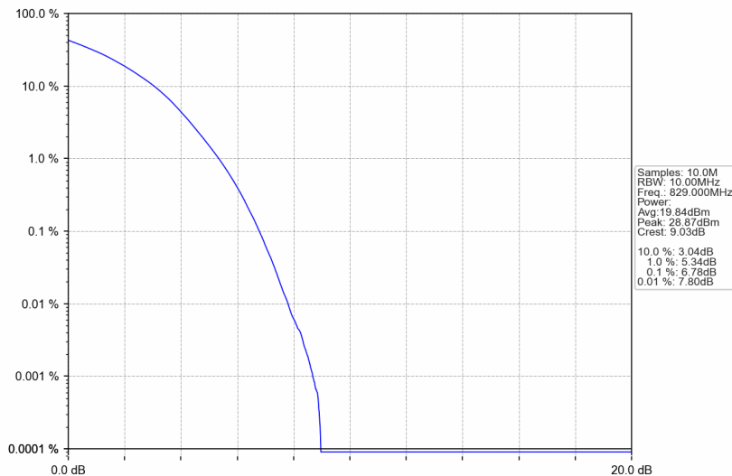
Band26b_10MHz_256QAM_LCH_829MHz_RB_50_0_NTNV
