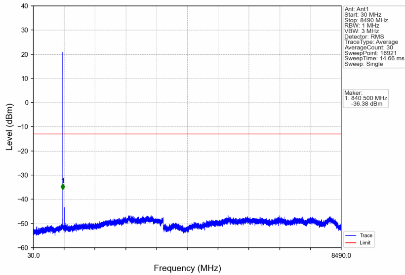
Band26b_1.4MHz_256QAM_HCH_848.3MHz_RB_1_0_NTNV
