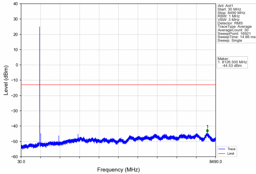
Band26b_5MHz_16QAM_HCH_846.5MHz_RB_1_0_NTNV
