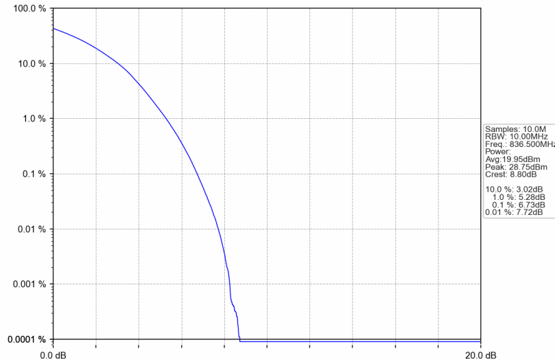
Band26b_10MHz_256QAM_MCH_836.5MHz_RB_50_0_NTNV
