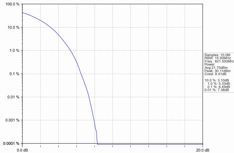
Band26c_15MHz_64QAM_LCH_821.5MHz_RB_75_0_NTNV
