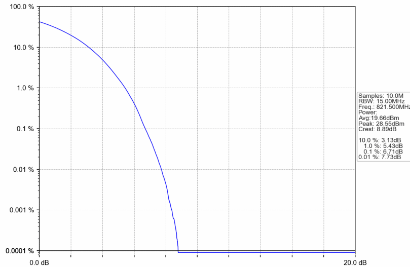
Band26c_15MHz_256QAM_LCH_821.5MHz_RB_75_0_NTNV
