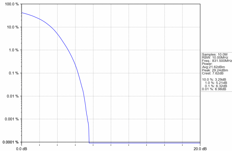
Band26c_15MHz_16QAM_MCH_831.5MHz_RB_75_0_NTNV
