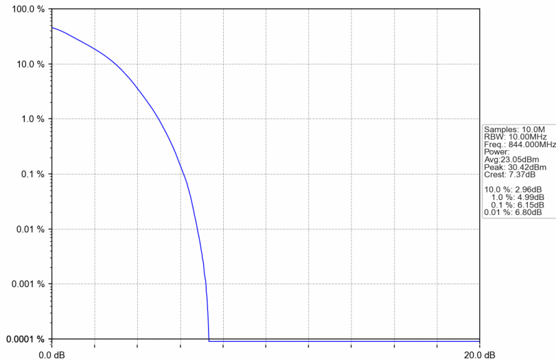
Band26b_10MHz_16QAM_HCH_844MHz_RB_50_0_NTNV
