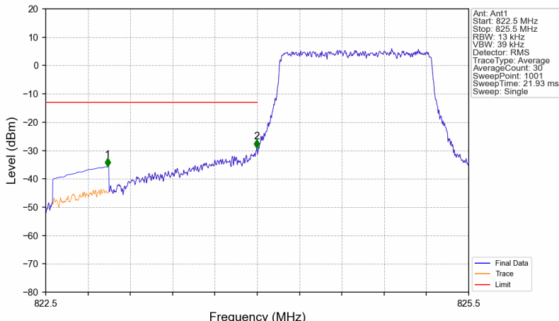
Band26b_1.4MHz_16QAM_LCH_824.7MHz_RB_6_0_NTNV
