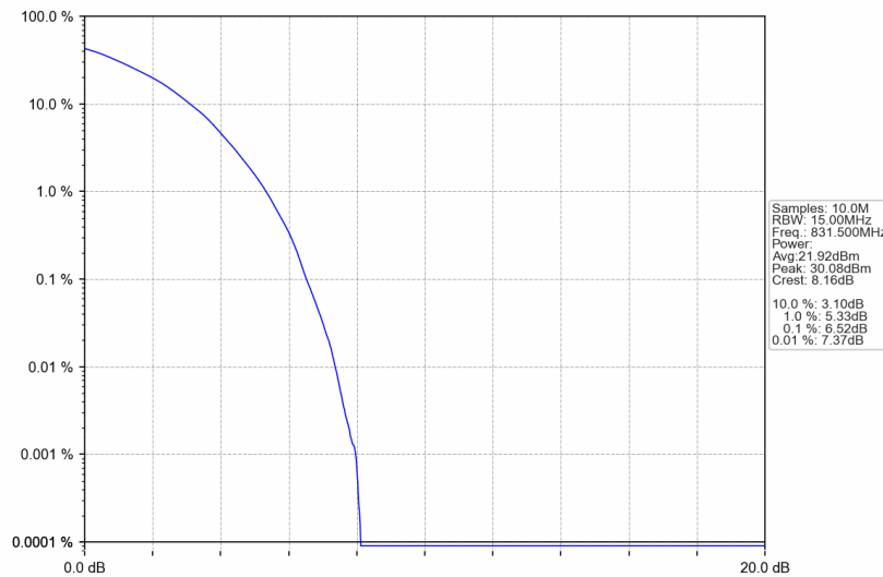
Band26c_15MHz_64QAM_MCH_831.5MHz_RB_75_0_NTNV
