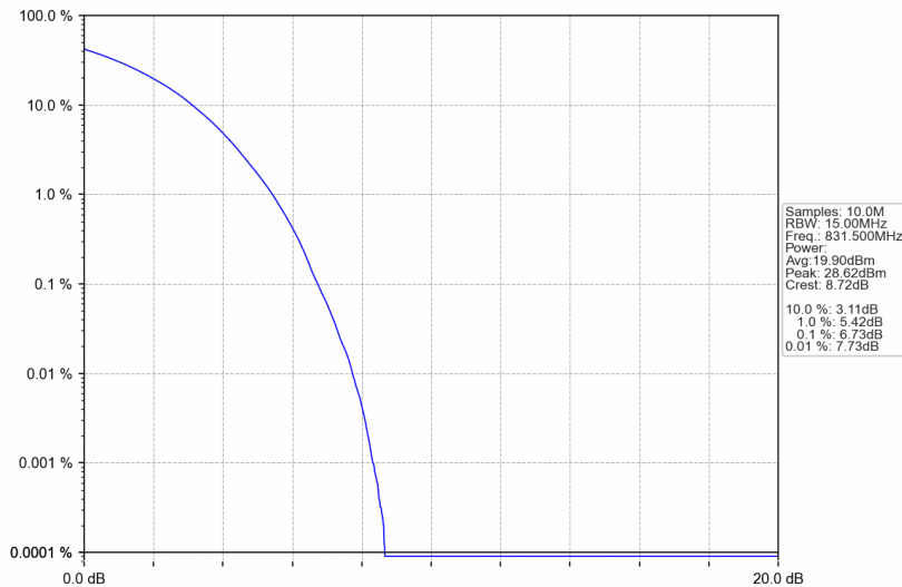
Band26c_15MHz_256QAM_MCH_831.5MHz_RB_75_0_NTNV
