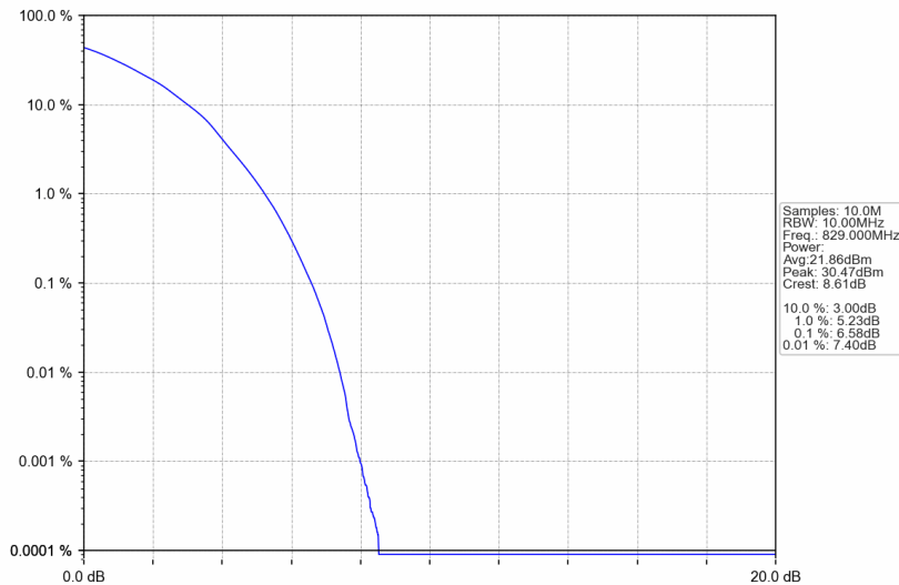
Band26b_10MHz_64QAM_LCH_829MHz_RB_50_0_NTNV
