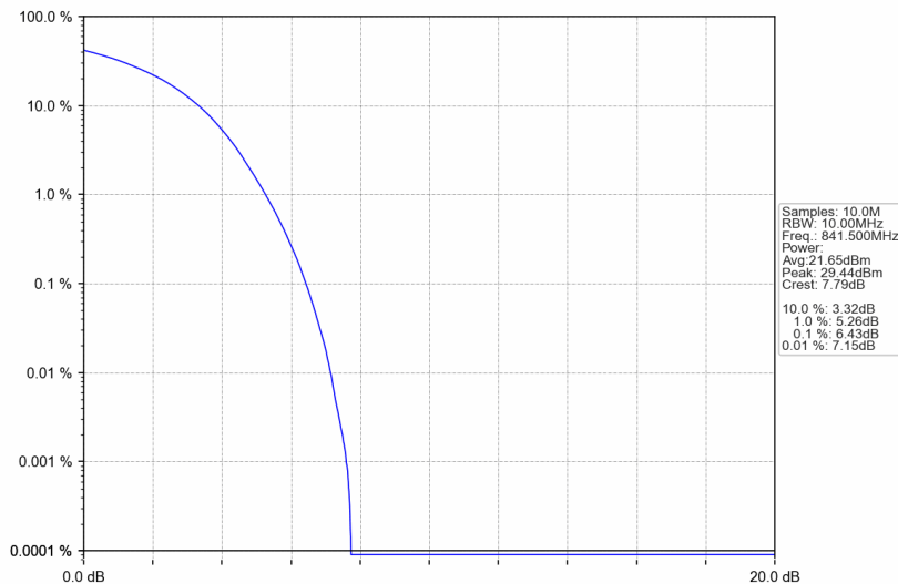
Band26c_15MHz_16QAM_HCH_841.5MHz_RB_75_0_NTNV
