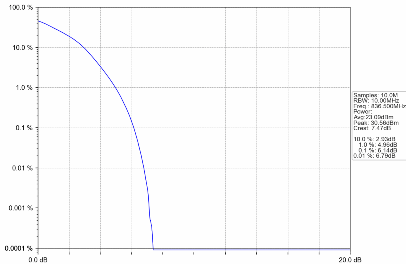
Band26b_10MHz_16QAM_MCH_836.5MHz_RB_50_0_NTNV
