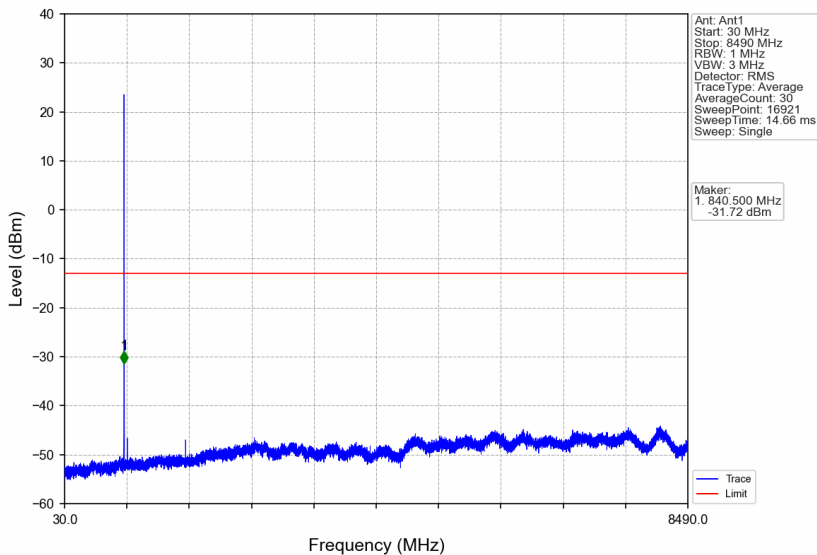
Band26b_1.4MHz_16QAM_HCH_848.3MHz_RB_1_0_NTNV
