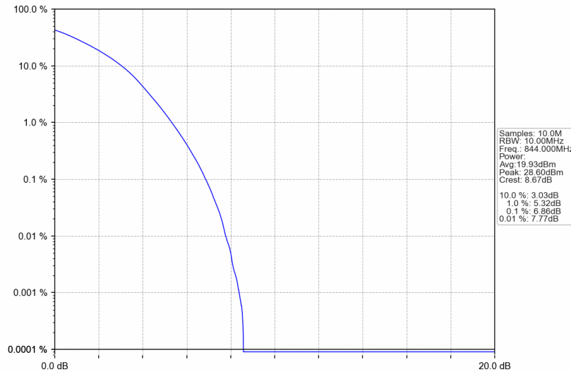
Band26b_10MHz_256QAM_HCH_844MHz_RB_50_0_NTNV
