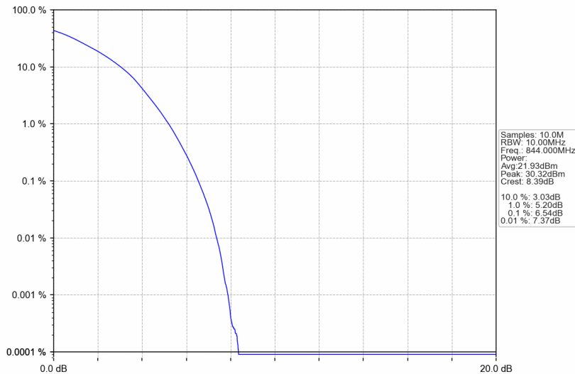
Band26b_10MHz_64QAM_HCH_844MHz_RB_50_0_NTNV
