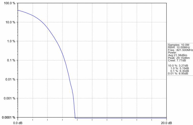
Band26c_15MHz_16QAM_LCH_821.5MHz_RB_75_0_NTNV
