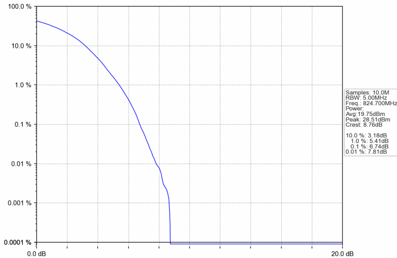
Band26b_1.4MHz_256QAM_LCH_824.7MHz_RB_6_0_NTNV
