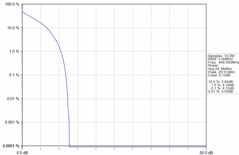
Band26b_1.4MHz_QPSK_HCH_848.3MHz_RB_6_0_NTNV
