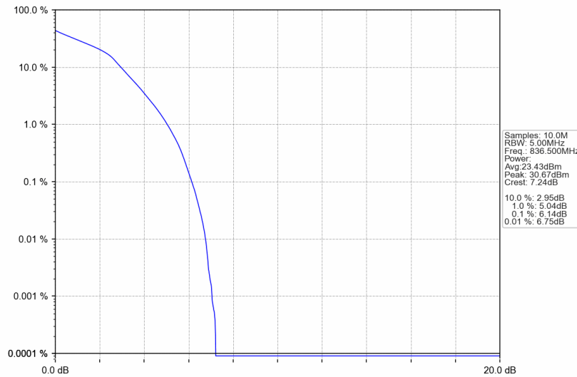
Band26b_3MHz_16QAM_MCH_836.5MHz_RB_15_0_NTNV
