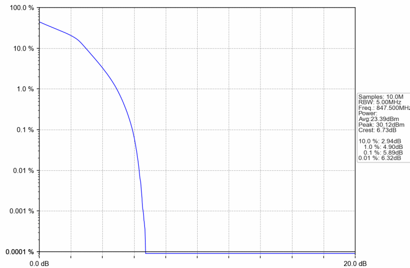
Band26b_3MHz_16QAM_HCH_847.5MHz_RB_15_0_NTNV
