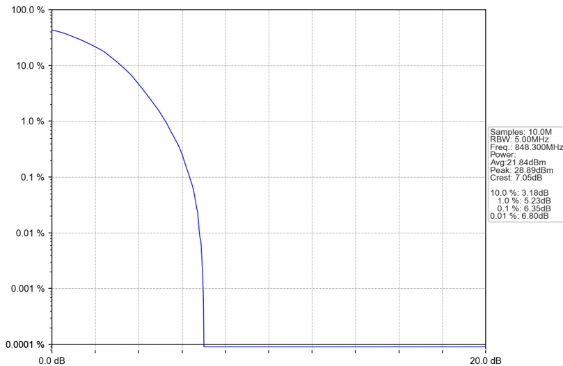
Band26b_1.4MHz_64QAM_HCH_848.3MHz_RB_6_0_NTNV
