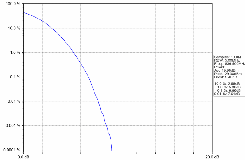
Band26b_5MHz_256QAM_MCH_836.5MHz_RB_25_0_NTNV
