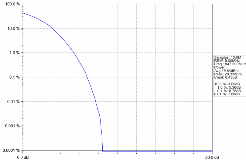
Band26b_3MHz_256QAM_HCH_847.5MHz_RB_15_0_NTNV
