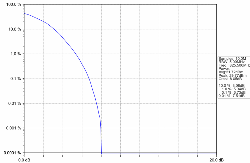
Band26b_3MHz_64QAM_LCH_825.5MHz_RB_15_0_NTNV
