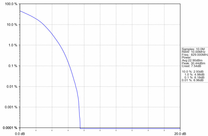
Band26b_10MHz_16QAM_LCH_829MHz_RB_50_0_NTNV
