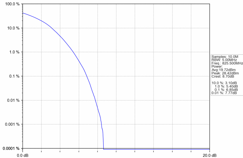
Band26b_3MHz_256QAM_LCH_825.5MHz_RB_15_0_NTNV
