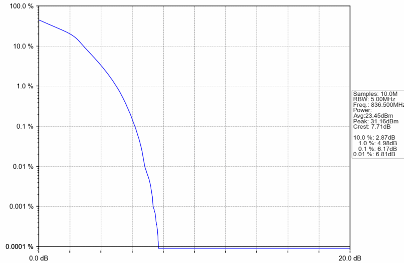
Band26b_5MHz_16QAM_MCH_836.5MHz_RB_25_0_NTNV
