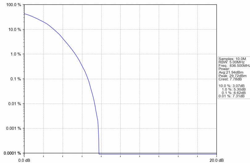
Band26b_3MHz_64QAM_MCH_836.5MHz_RB_15_0_NTNV
