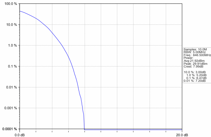
Band26b_5MHz_64QAM_HCH_846.5MHz_RB_25_0_NTNV
