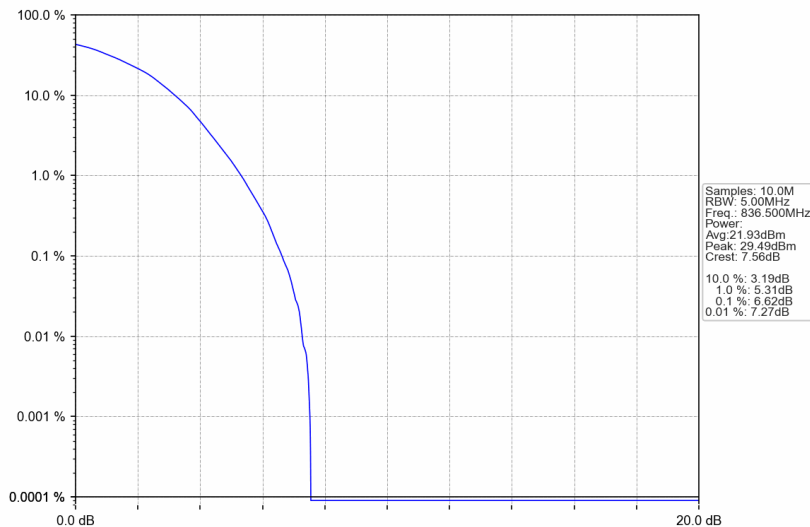
Band26b_1.4MHz_64QAM_MCH_836.5MHz_RB_6_0_NTNV
