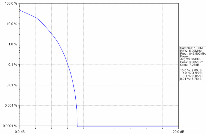
Band26b_5MHz_16QAM_HCH_846.5MHz_RB_25_0_NTNV
