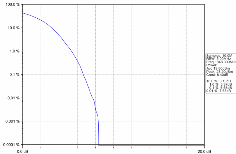
Band26b_1.4MHz_256QAM_HCH_848.3MHz_RB_6_0_NTNV
