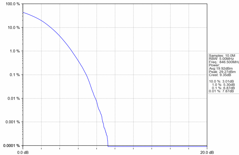
Band26b_5MHz_256QAM_HCH_846.5MHz_RB_25_0_NTNV
