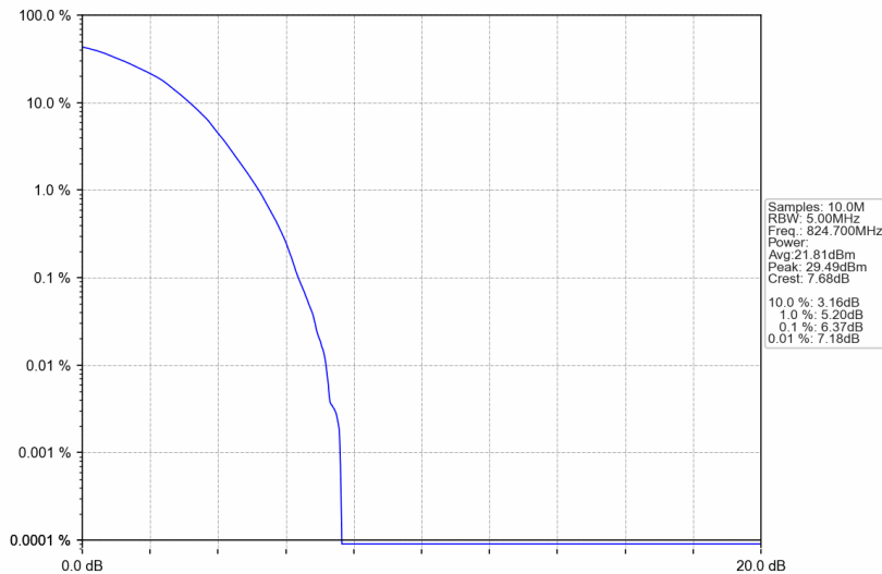
Band26b_1.4MHz_64QAM_LCH_824.7MHz_RB_6_0_NTNV
