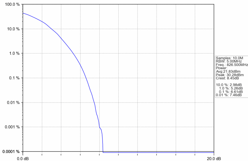
Band26b_5MHz_64QAM_LCH_826.5MHz_RB_25_0_NTNV
