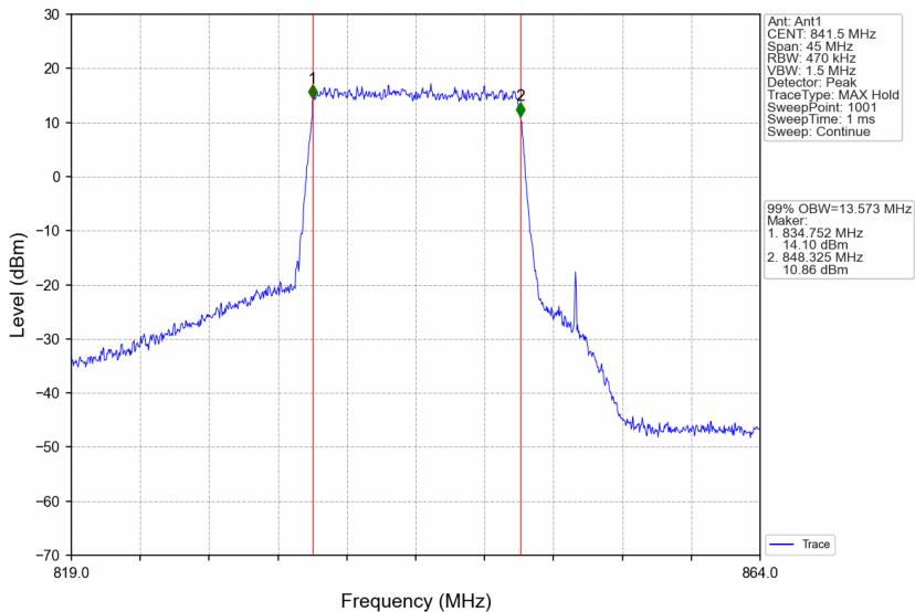
Band26c_15MHz_256QAM_HCH_841.5MHz_RB_75_0_NTNV
