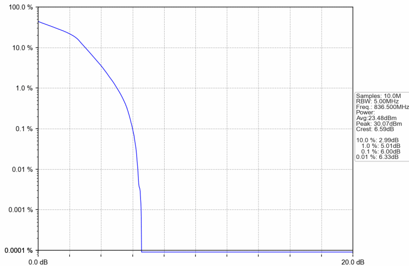
Band26b_1.4MHz_16QAM_MCH_836.5MHz_RB_6_0_NTNV
