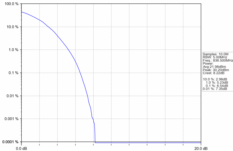
Band26b_5MHz_64QAM_MCH_836.5MHz_RB_25_0_NTNV
