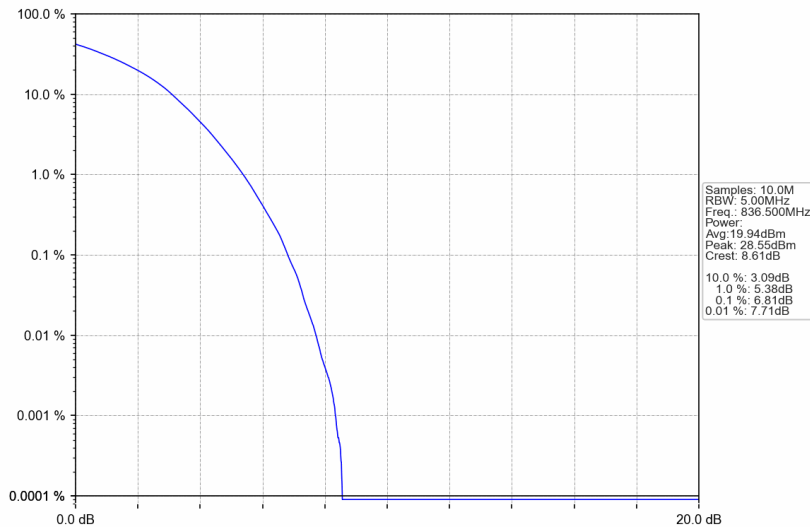
Band26b_3MHz_256QAM_MCH_836.5MHz_RB_15_0_NTNV
