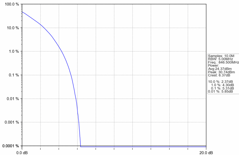
Band26b_5MHz_QPSK_HCH_846.5MHz_RB_25_0_NTNV
