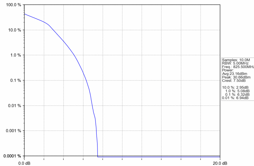
Band26b_3MHz_16QAM_LCH_825.5MHz_RB_15_0_NTNV
