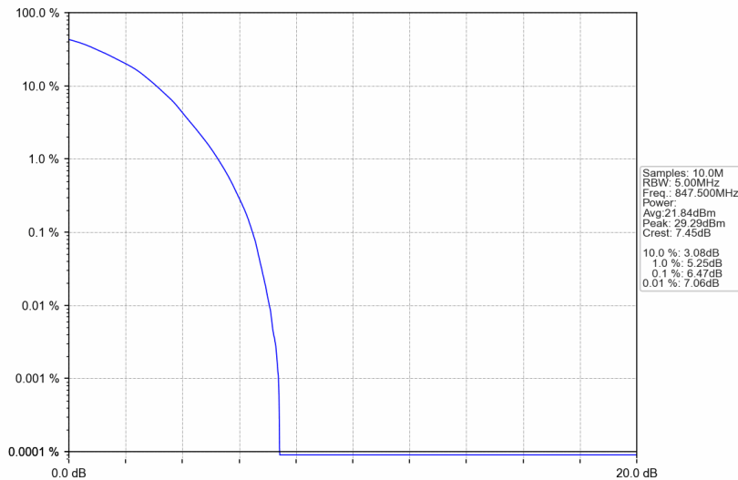
Band26b_3MHz_64QAM_HCH_847.5MHz_RB_15_0_NTNV
