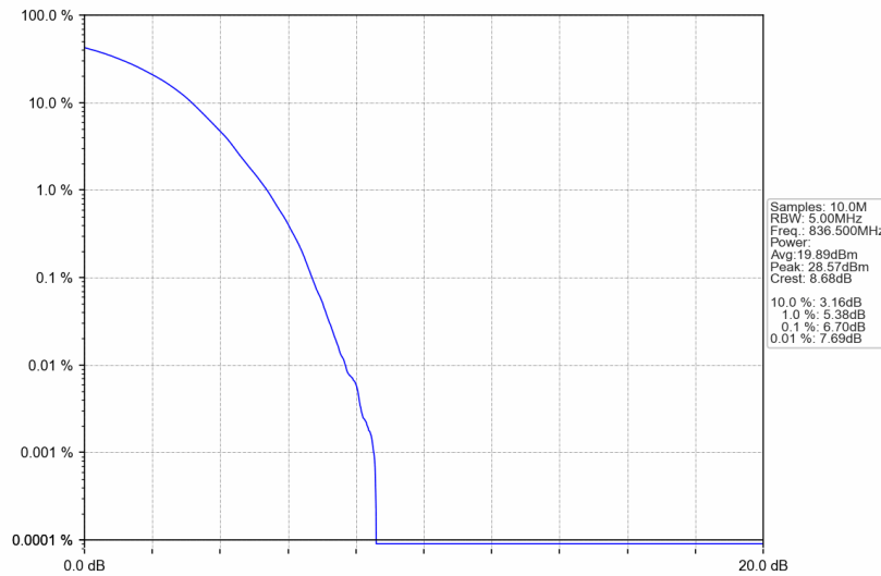
Band26b_1.4MHz_256QAM_MCH_836.5MHz_RB_6_0_NTNV
