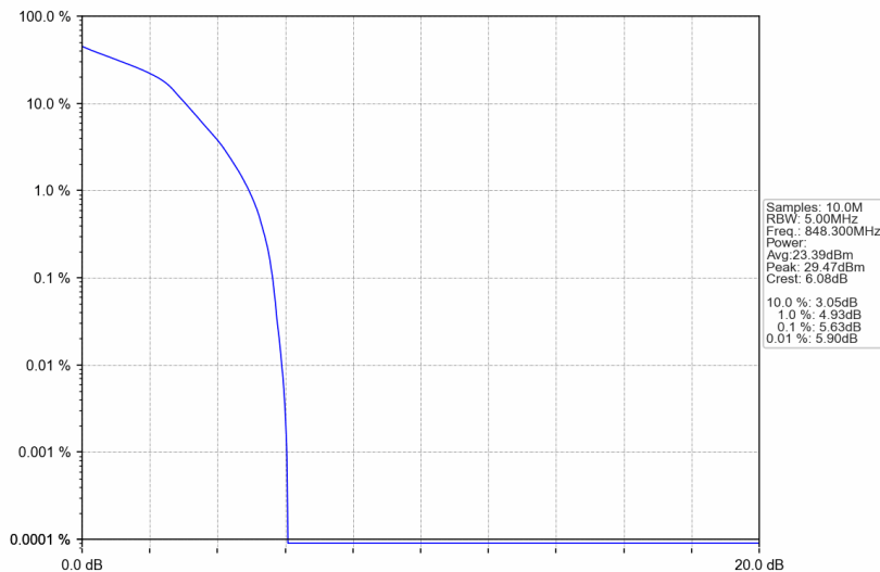
Band26b_1.4MHz_16QAM_HCH_848.3MHz_RB_6_0_NTNV
