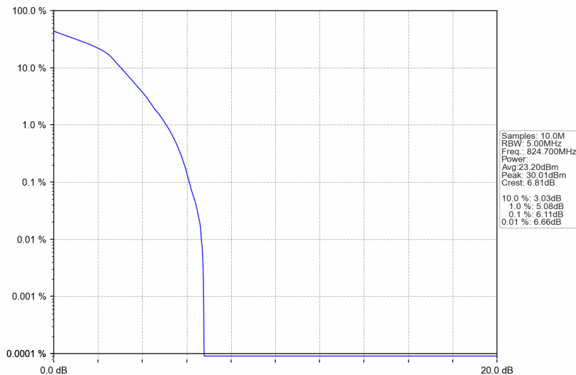
Band26b_1.4MHz_16QAM_LCH_824.7MHz_RB_6_0_NTNV
