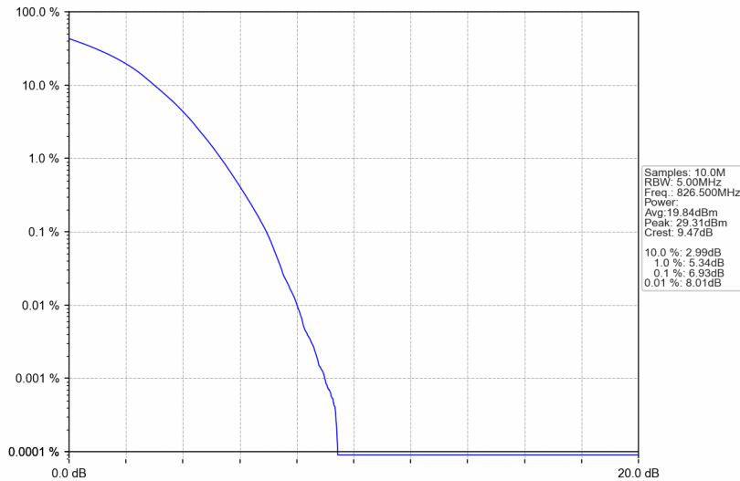
Band26b_5MHz_256QAM_LCH_826.5MHz_RB_25_0_NTNV
