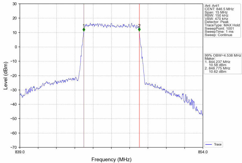
Band26b_5MHz_256QAM_HCH_846.5MHz_RB_25_0_NTNV
