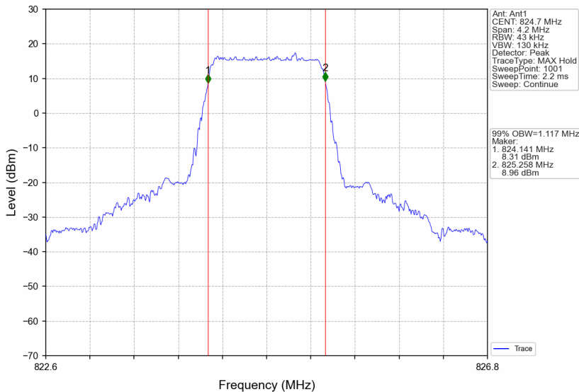
Band26b_1.4MHz_256QAM_LCH_824.7MHz_RB_6_0_NTNV
