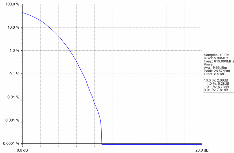
Band26a_5MHz_256QAM_MCH_819MHz_RB_25_0_NTNV
