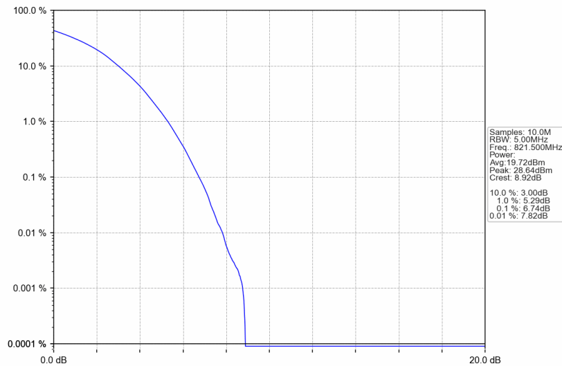
Band26a_5MHz_256QAM_HCH_821.5MHz_RB_25_0_NTNV
