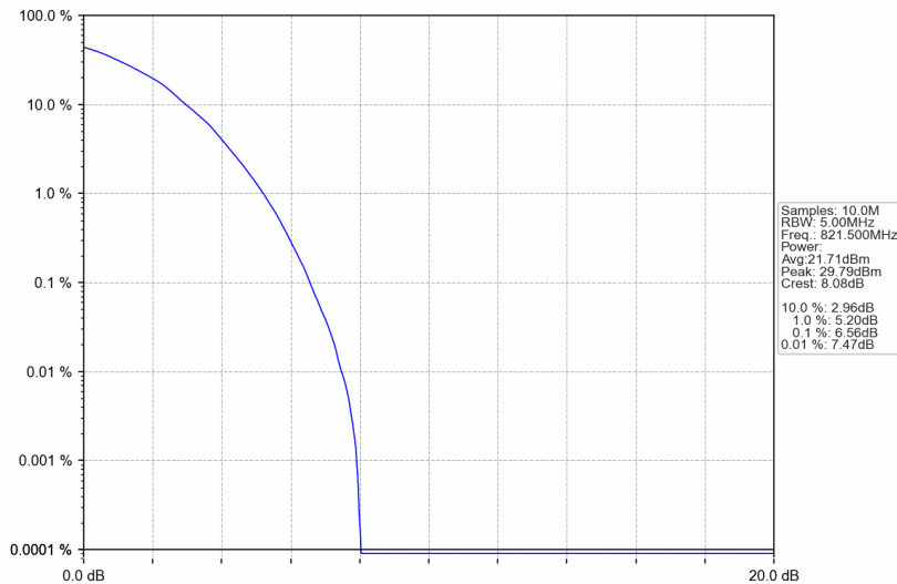
Band26a_5MHz_64QAM_HCH_821.5MHz_RB_25_0_NTNV
