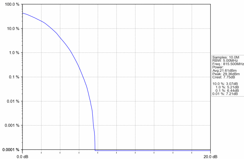
Band26a_3MHz_64QAM_LCH_815.5MHz_RB_15_0_NTNV
