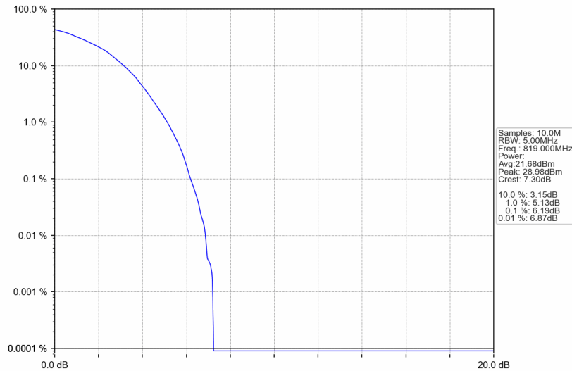
Band26a_1.4MHz_64QAM_MCH_819MHz_RB_6_0_NTNV
