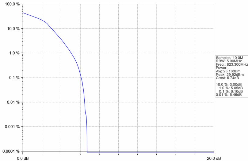
Band26a_1.4MHz_16QAM_HCH_823.3MHz_RB_6_0_NTNV
