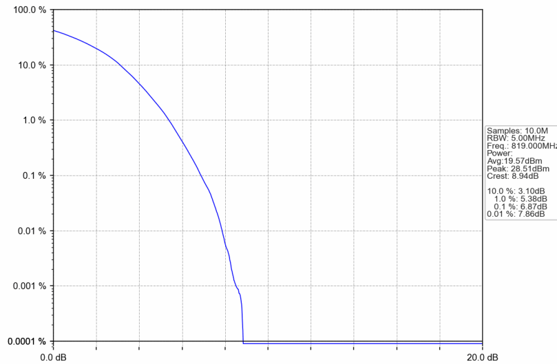
Band26a_3MHz_256QAM_MCH_819MHz_RB_15_0_NTNV
