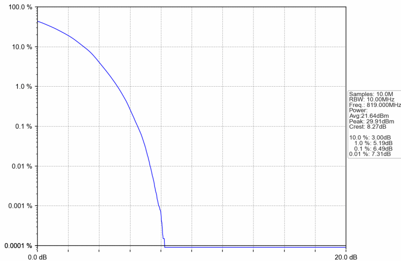
Band26a_10MHz_64QAM_MCH_819MHz_RB_50_0_NTNV
