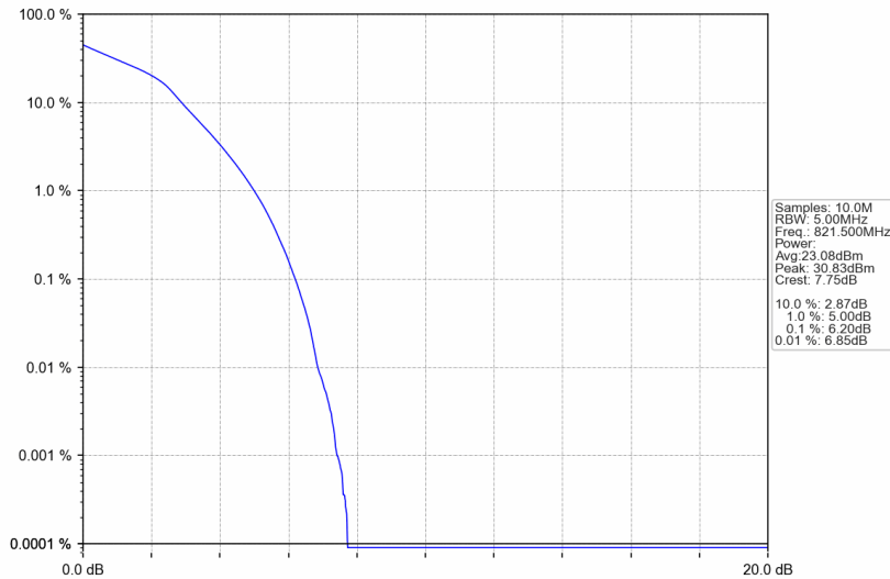
Band26a_5MHz_16QAM_HCH_821.5MHz_RB_25_0_NTNV
