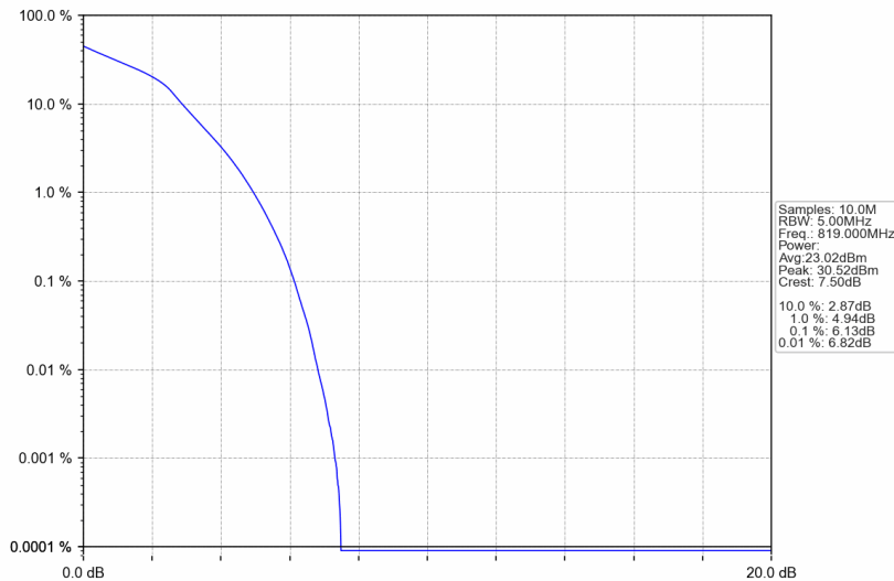
Band26a_5MHz_16QAM_MCH_819MHz_RB_25_0_NTNV
