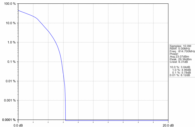
Band26a_1.4MHz_16QAM_LCH_814.7MHz_RB_6_0_NTNV
