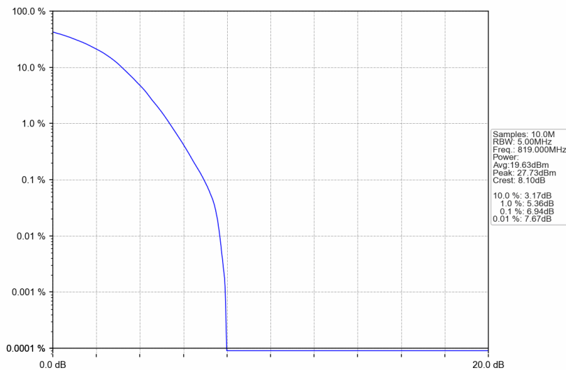
Band26a_1.4MHz_256QAM_MCH_819MHz_RB_6_0_NTNV
