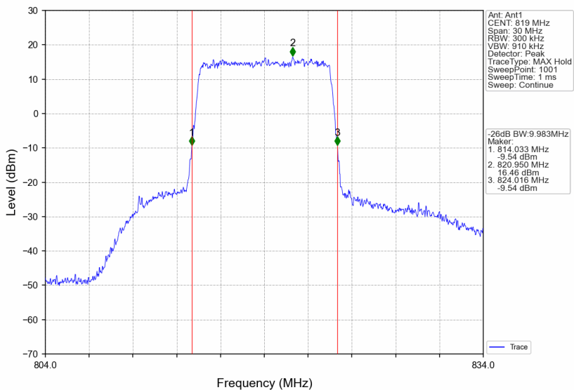
Band26a_10MHz_256QAM_MCH_819MHz_RB_50_0_NTNV
