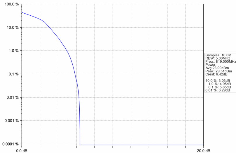
Band26a_1.4MHz_16QAM_MCH_819MHz_RB_6_0_NTNV
