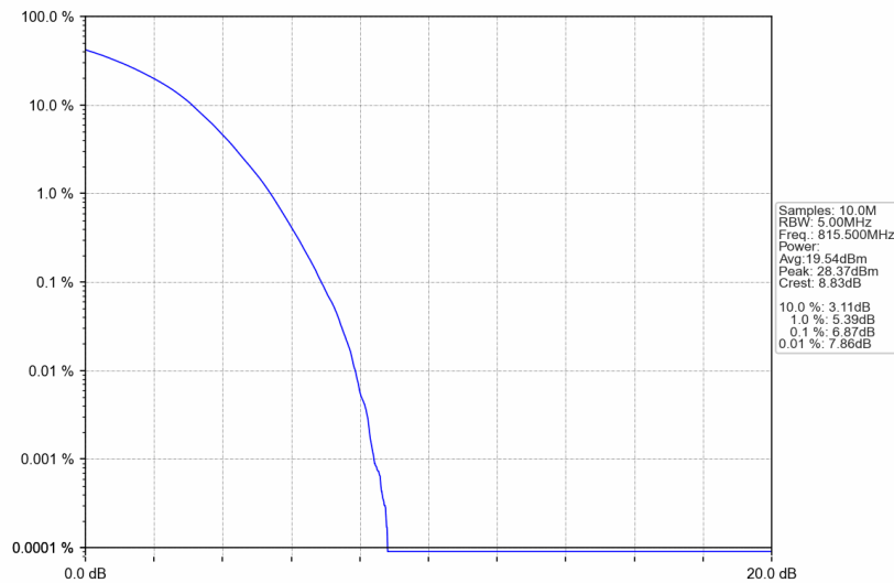
Band26a_3MHz_256QAM_LCH_815.5MHz_RB_15_0_NTNV
