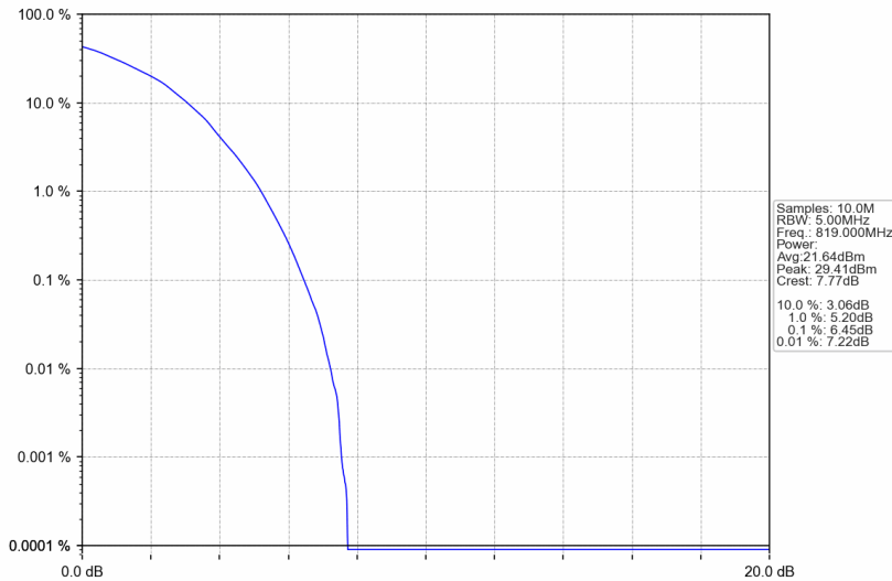
Band26a_3MHz_64QAM_MCH_819MHz_RB_15_0_NTNV
