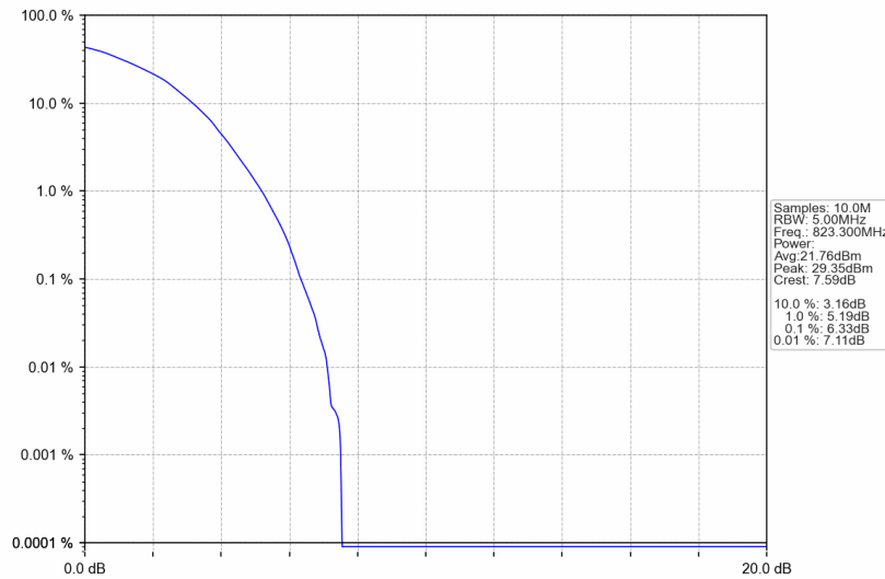
Band26a_1.4MHz_64QAM_HCH_823.3MHz_RB_6_0_NTNV
