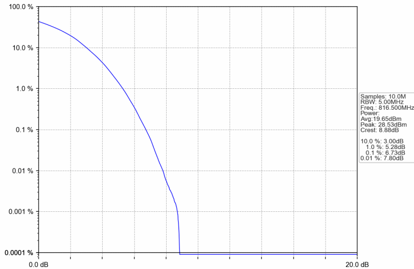
Band26a_5MHz_256QAM_LCH_816.5MHz_RB_25_0_NTNV
