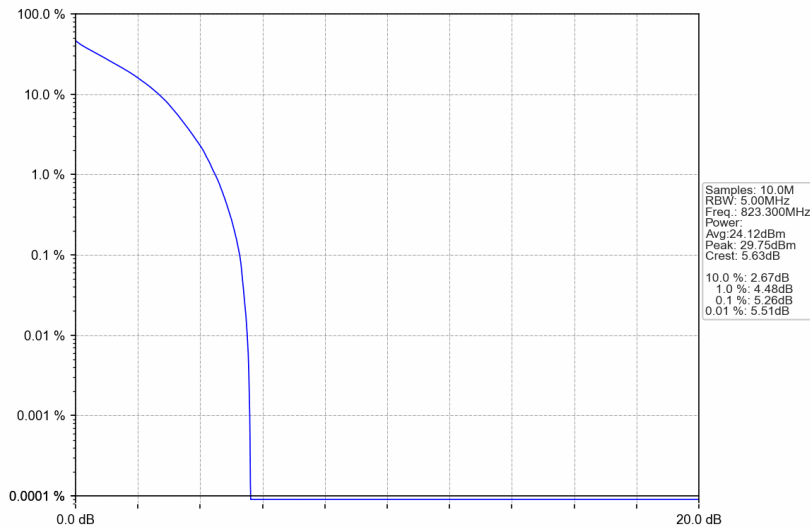
Band26a_1.4MHz_QPSK_HCH_823.3MHz_RB_6_0_NTNV
