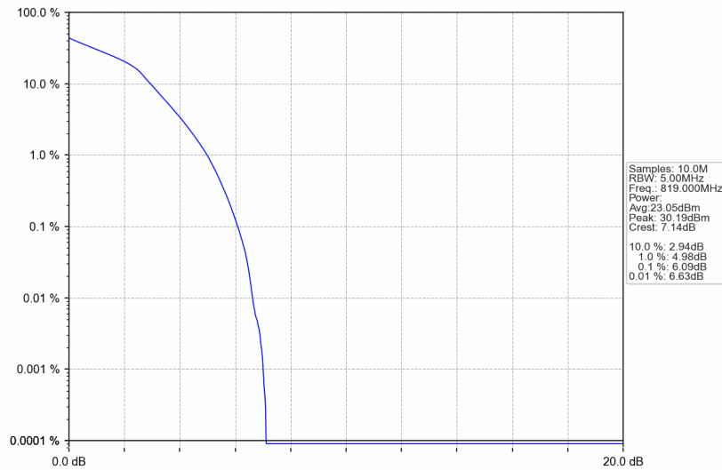
Band26a_3MHz_16QAM_MCH_819MHz_RB_15_0_NTNV
