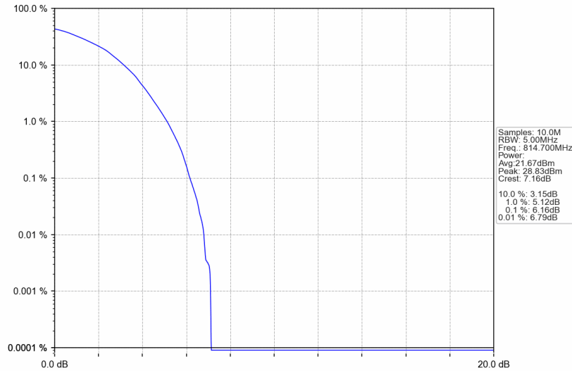
Band26a_1.4MHz_64QAM_LCH_814.7MHz_RB_6_0_NTNV
