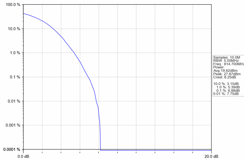
Band26a_1.4MHz_256QAM_LCH_814.7MHz_RB_6_0_NTNV
