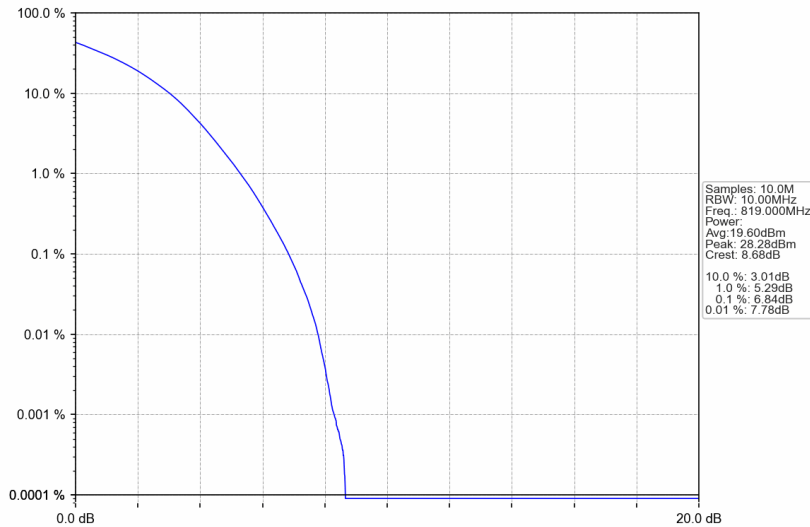
Band26a_10MHz_256QAM_MCH_819MHz_RB_50_0_NTNV
