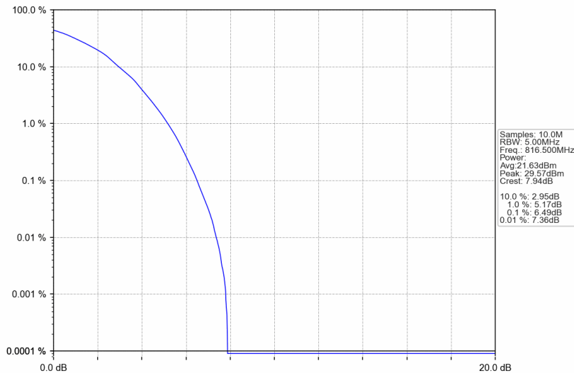
Band26a_5MHz_64QAM_LCH_816.5MHz_RB_25_0_NTNV
