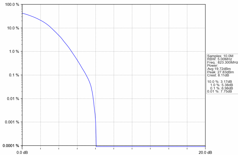
Band26a_1.4MHz_256QAM_HCH_823.3MHz_RB_6_0_NTNV
