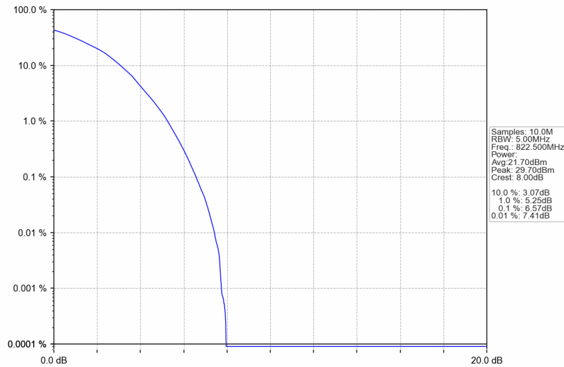
Band26a_3MHz_64QAM_HCH_822.5MHz_RB_15_0_NTNV
