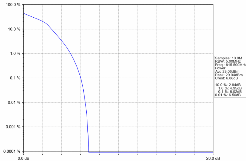
Band26a_3MHz_16QAM_LCH_815.5MHz_RB_15_0_NTNV
