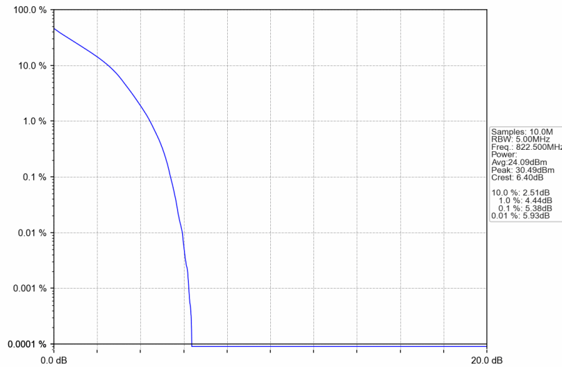
Band26a_3MHz_QPSK_HCH_822.5MHz_RB_15_0_NTNV
