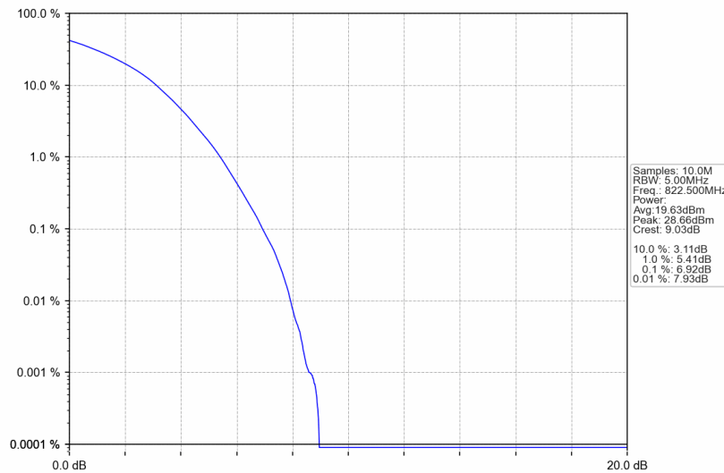
Band26a_3MHz_256QAM_HCH_822.5MHz_RB_15_0_NTNV
