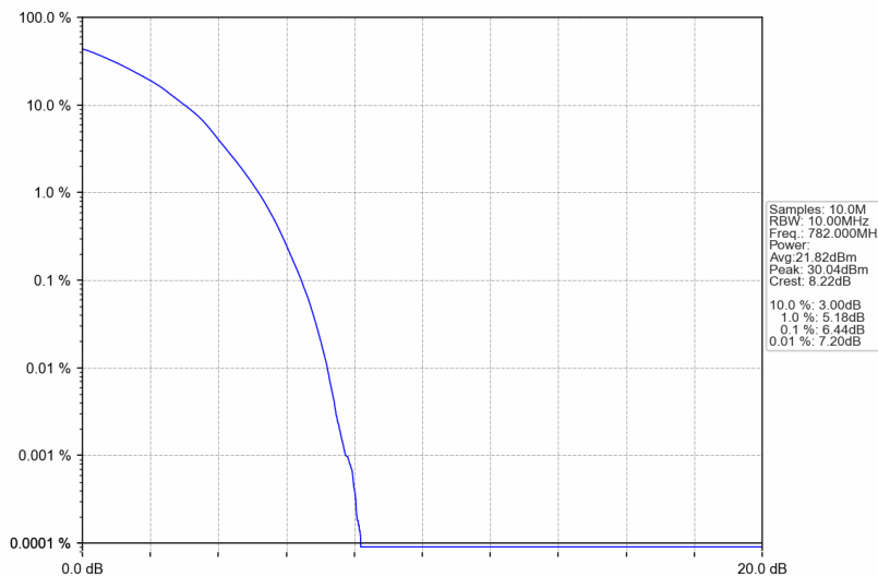
Band13_10MHz_64QAM_MCH_782MHz_RB_50_0_NTNV
