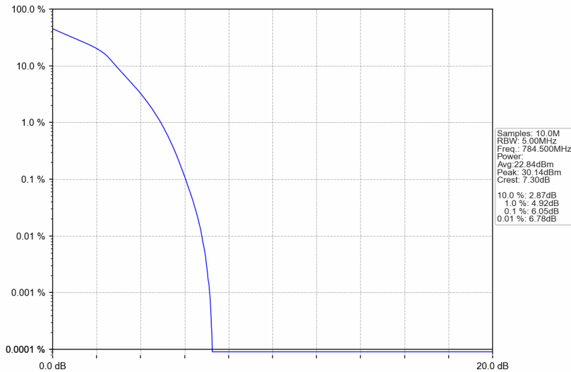
Band13_5MHz_16QAM_HCH_784.5MHz_RB_25_0_NTNV
