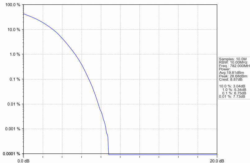
Band13_10MHz_256QAM_MCH_782MHz_RB_50_0_NTNV
