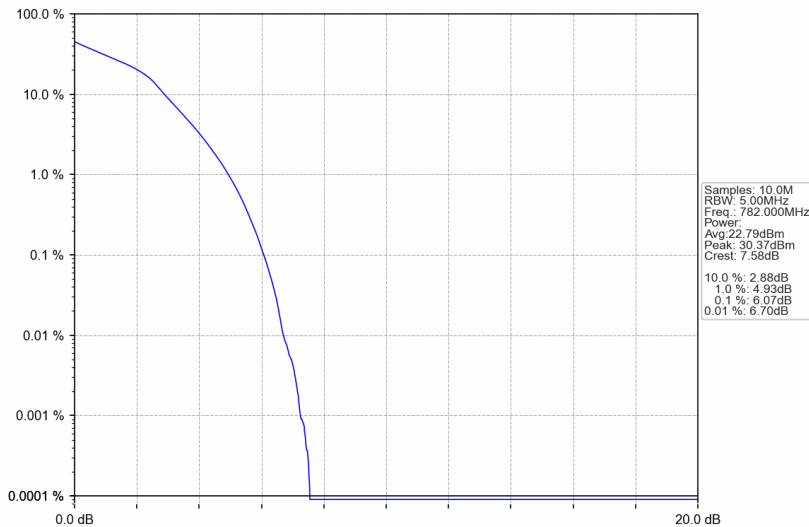
Band13_5MHz_16QAM_MCH_782MHz_RB_25_0_NTNV
