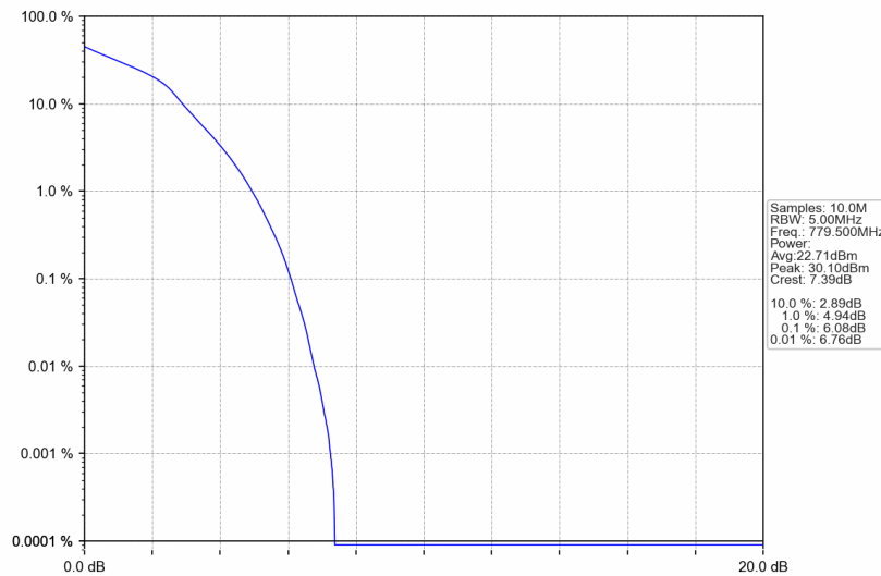
Band13_5MHz_16QAM_LCH_779.5MHz_RB_25_0_NTNV
