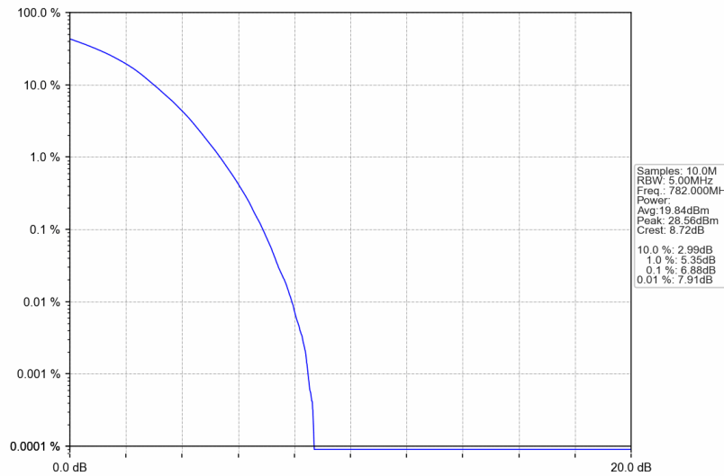
Band13_5MHz_256QAM_MCH_782MHz_RB_25_0_NTNV
