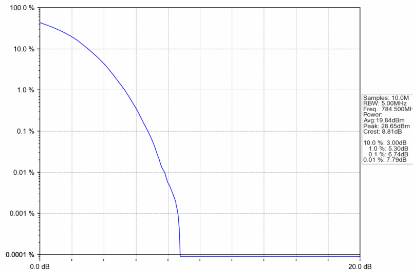
Band13_5MHz_256QAM_HCH_784.5MHz_RB_25_0_NTNV
