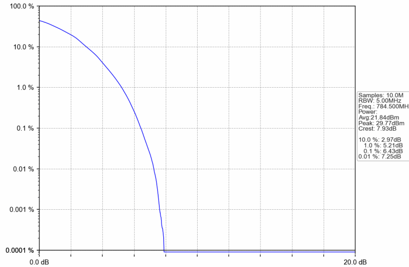
Band13_5MHz_64QAM_HCH_784.5MHz_RB_25_0_NTNV
