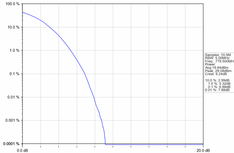
Band13_5MHz_256QAM_LCH_779.5MHz_RB_25_0_NTNV
