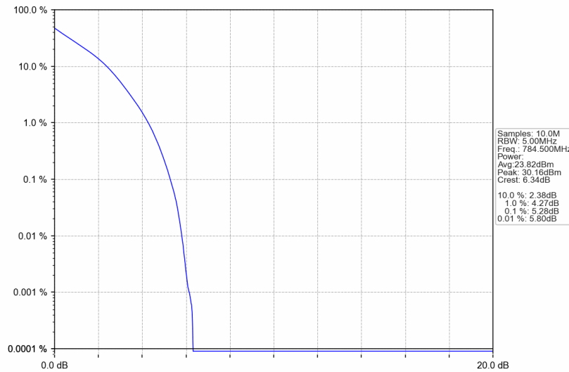
Band13_5MHz_QPSK_HCH_784.5MHz_RB_25_0_NTNV
