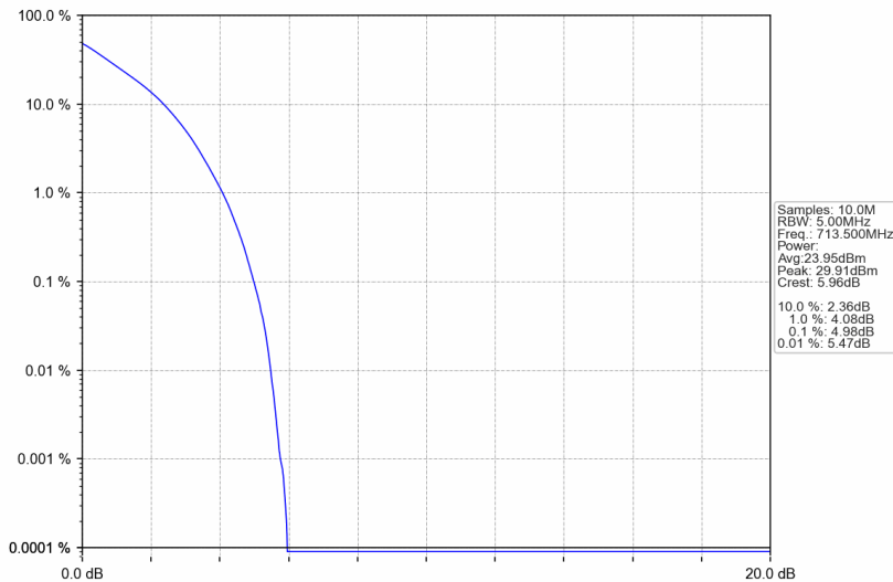
Band12_5MHz_QPSK_HCH_713.5MHz_RB_25_0_NTNV
