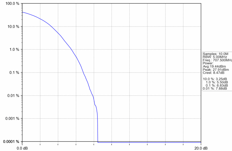
Band12_1.4MHz_256QAM_MCH_707.5MHz_RB_6_0_NTNV
