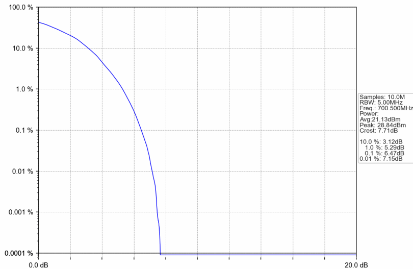
Band12_3MHz_64QAM_LCH_700.5MHz_RB_15_0_NTNV
