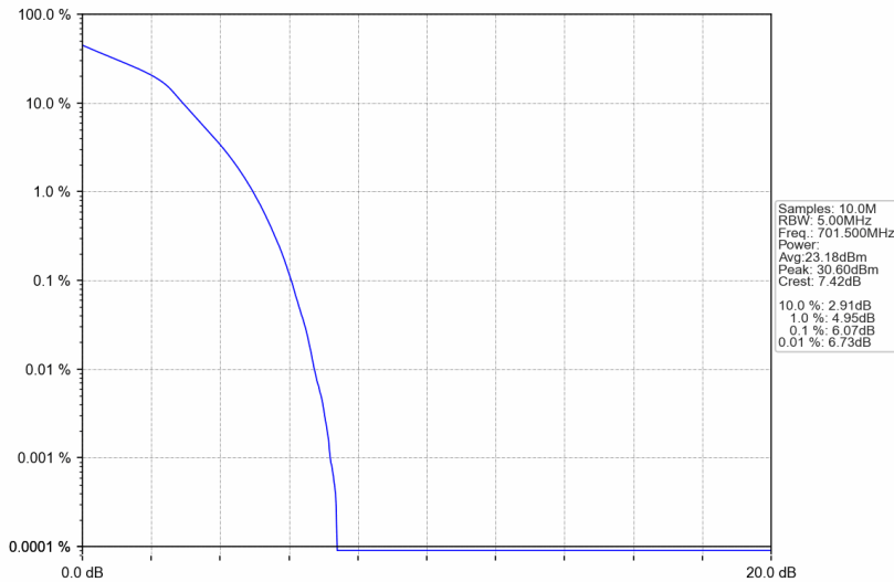
Band12_5MHz_16QAM_LCH_701.5MHz_RB_25_0_NTNV
