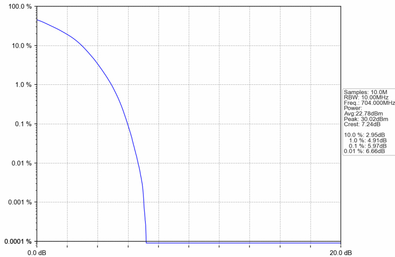
Band12_10MHz_16QAM_LCH_704MHz_RB_50_0_NTNV
