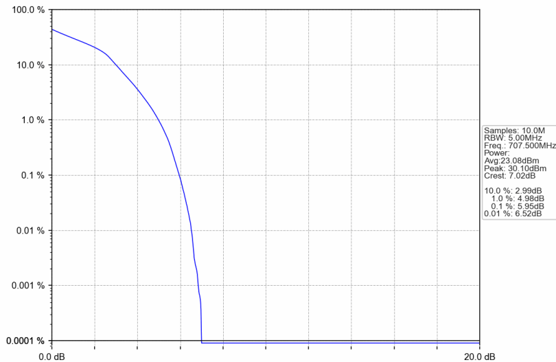
Band12_3MHz_16QAM_MCH_707.5MHz_RB_15_0_NTNV
