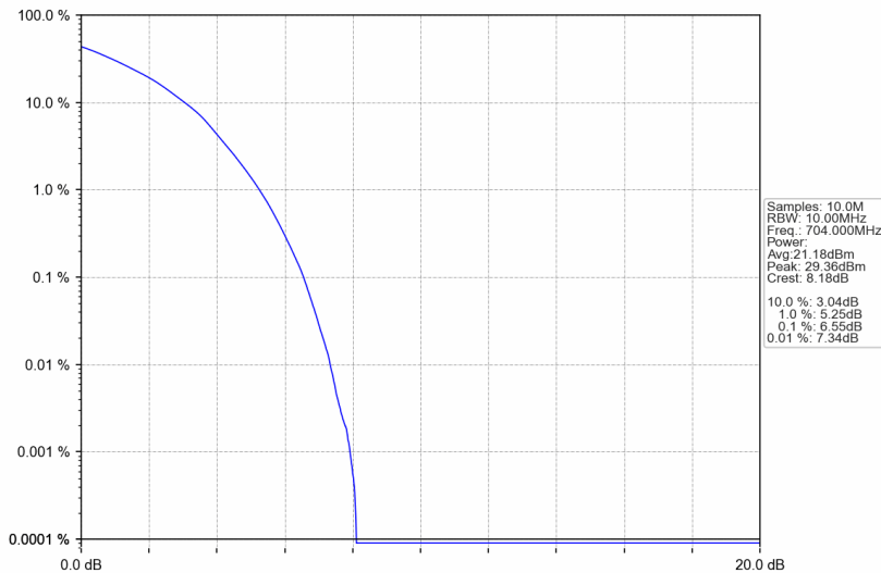
Band12_10MHz_64QAM_LCH_704MHz_RB_50_0_NTNV
