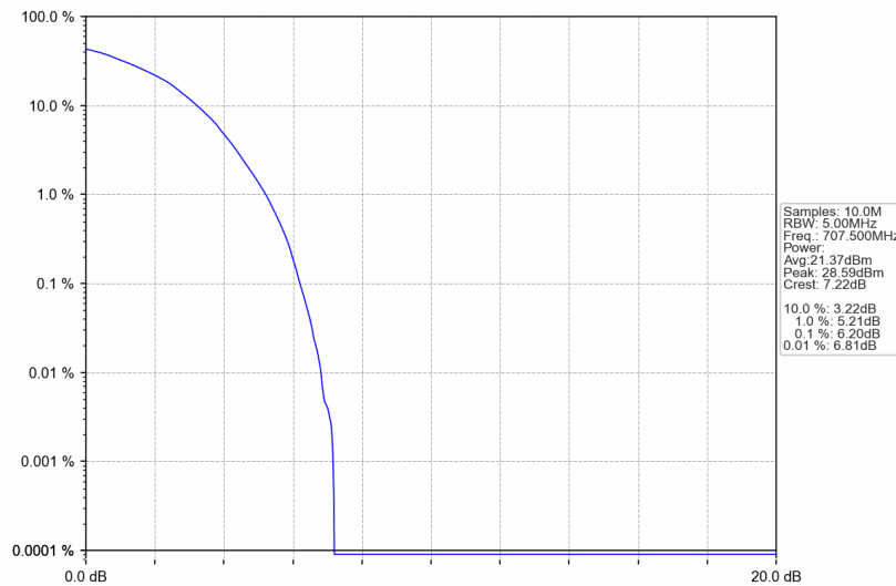
Band12_1.4MHz_64QAM_MCH_707.5MHz_RB_6_0_NTNV
