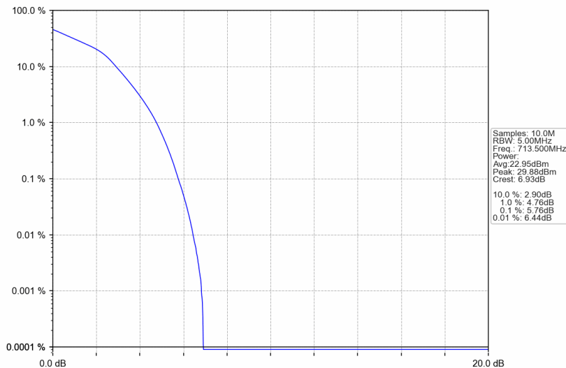
Band12_5MHz_16QAM_HCH_713.5MHz_RB_25_0_NTNV
