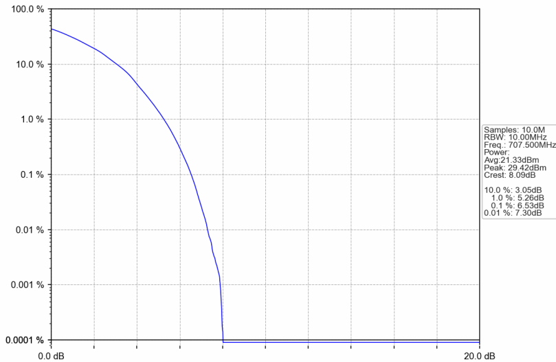
Band12_10MHz_64QAM_MCH_707.5MHz_RB_50_0_NTNV
