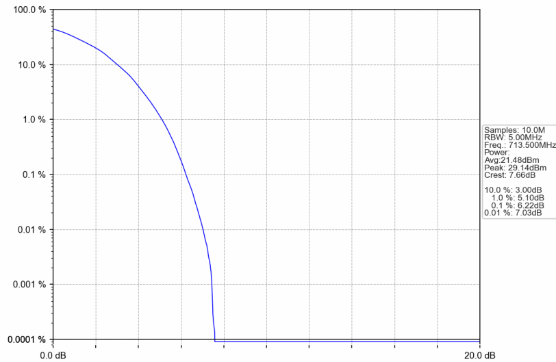
Band12_5MHz_64QAM_HCH_713.5MHz_RB_25_0_NTNV
