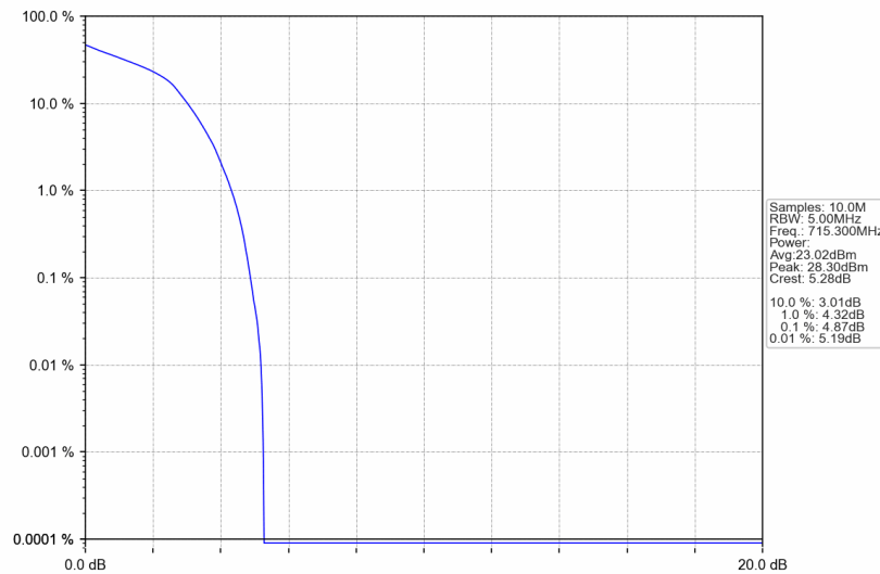
Band12_1.4MHz_16QAM_HCH_715.3MHz_RB_6_0_NTNV
