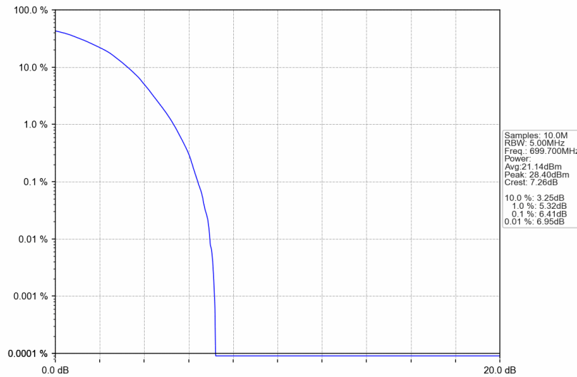
Band12_1.4MHz_64QAM_LCH_699.7MHz_RB_6_0_NTNV
