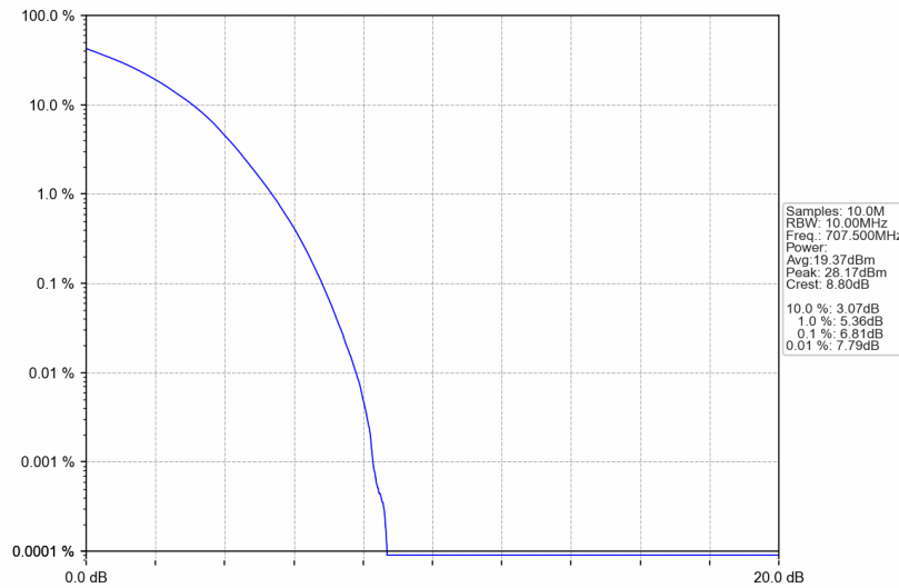
Band12_10MHz_256QAM_MCH_707.5MHz_RB_50_0_NTNV
