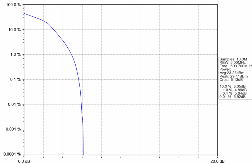
Band12_1.4MHz_16QAM_LCH_699.7MHz_RB_6_0_NTNV
