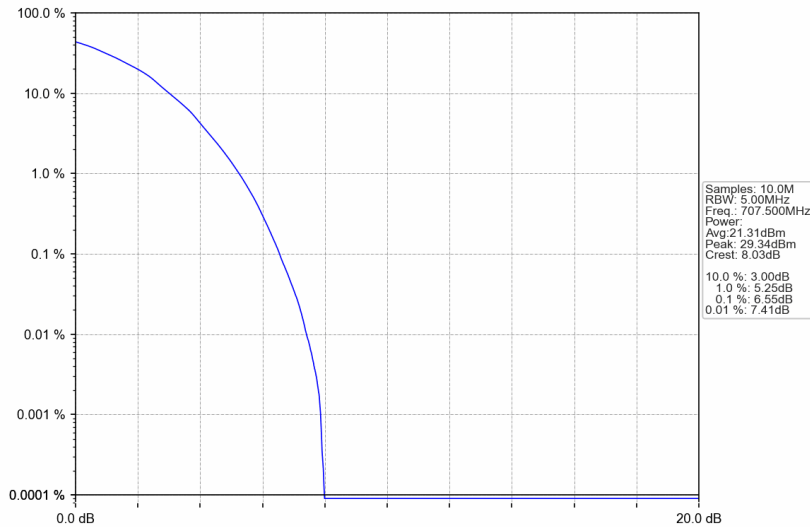
Band12_5MHz_64QAM_MCH_707.5MHz_RB_25_0_NTNV
