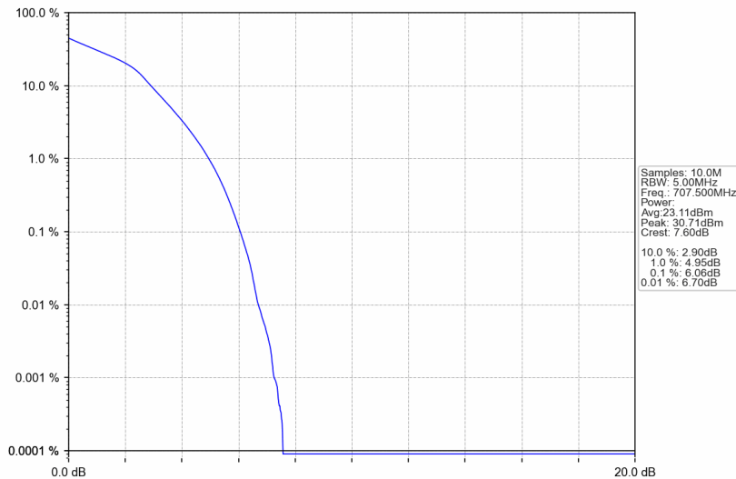
Band12_5MHz_16QAM_MCH_707.5MHz_RB_25_0_NTNV
