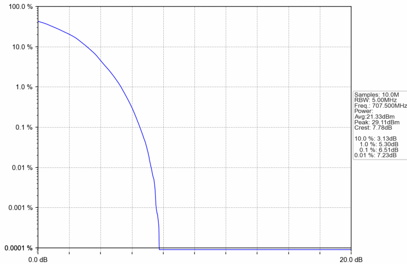
Band12_3MHz_64QAM_MCH_707.5MHz_RB_15_0_NTNV
