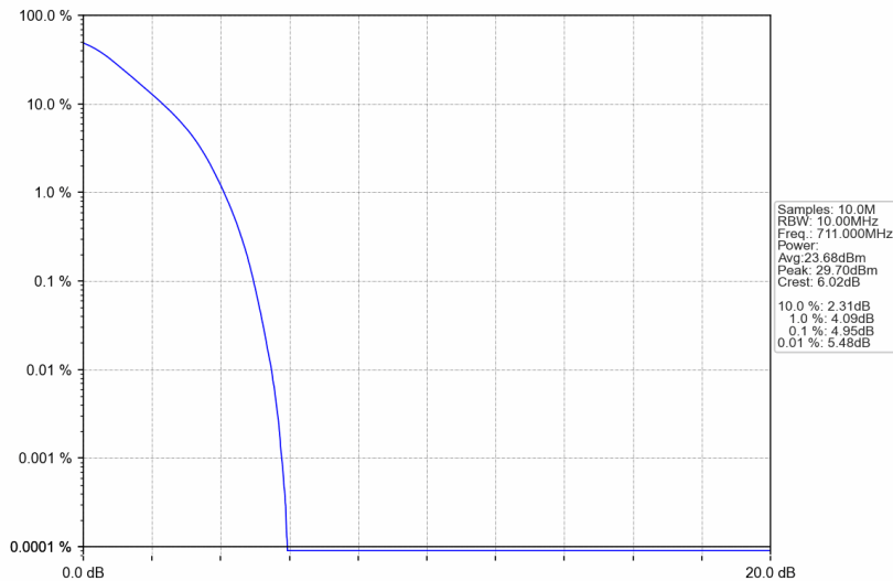
Band12_10MHz_QPSK_HCH_711MHz_RB_50_0_NTNV
