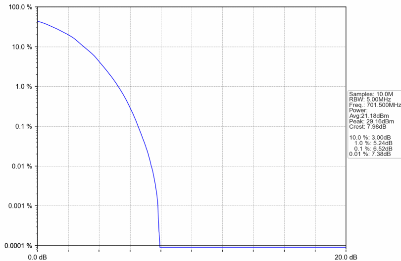
Band12_5MHz_64QAM_LCH_701.5MHz_RB_25_0_NTNV
