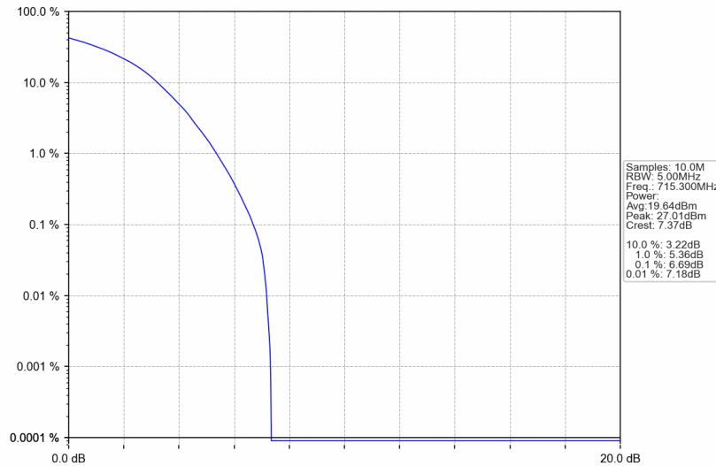
Band12_1.4MHz_256QAM_HCH_715.3MHz_RB_6_0_NTNV
