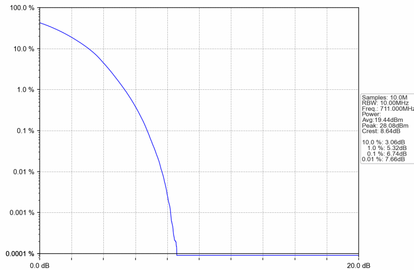
Band12_10MHz_256QAM_HCH_711MHz_RB_50_0_NTNV
