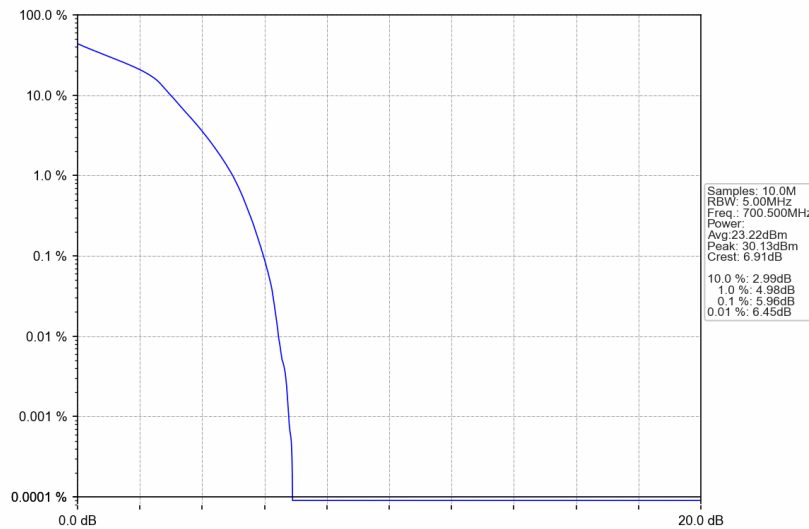
Band12_3MHz_16QAM_LCH_700.5MHz_RB_15_0_NTNV
