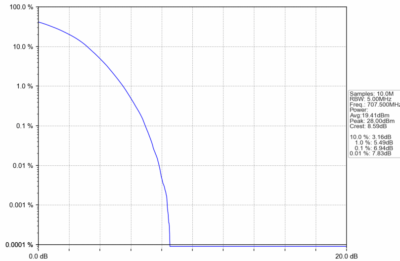
Band12_3MHz_256QAM_MCH_707.5MHz_RB_15_0_NTNV
