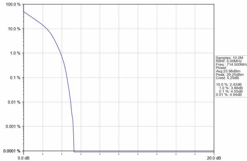
Band12_3MHz_QPSK_HCH_714.5MHz_RB_15_0_NTNV
