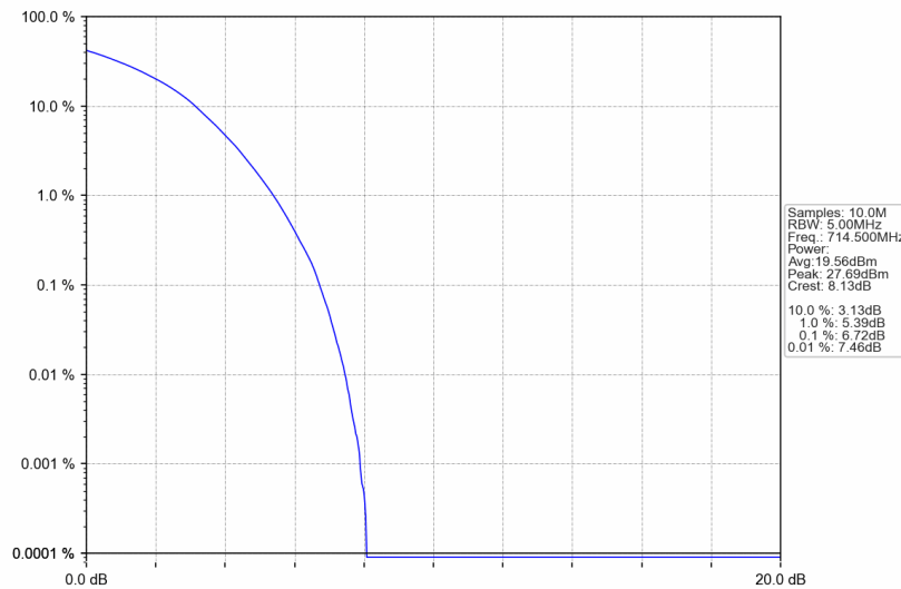
Band12_3MHz_256QAM_HCH_714.5MHz_RB_15_0_NTNV
