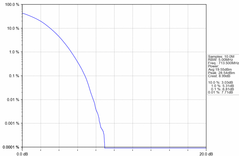
Band12_5MHz_256QAM_HCH_713.5MHz_RB_25_0_NTNV
