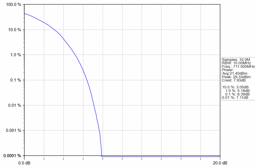
Band12_10MHz_64QAM_HCH_711MHz_RB_50_0_NTNV
