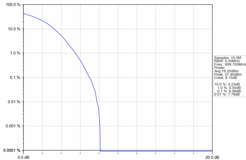
Band12_1.4MHz_256QAM_LCH_699.7MHz_RB_6_0_NTNV
