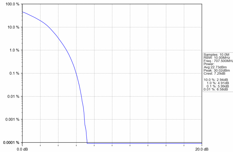
Band12_10MHz_16QAM_MCH_707.5MHz_RB_50_0_NTNV
