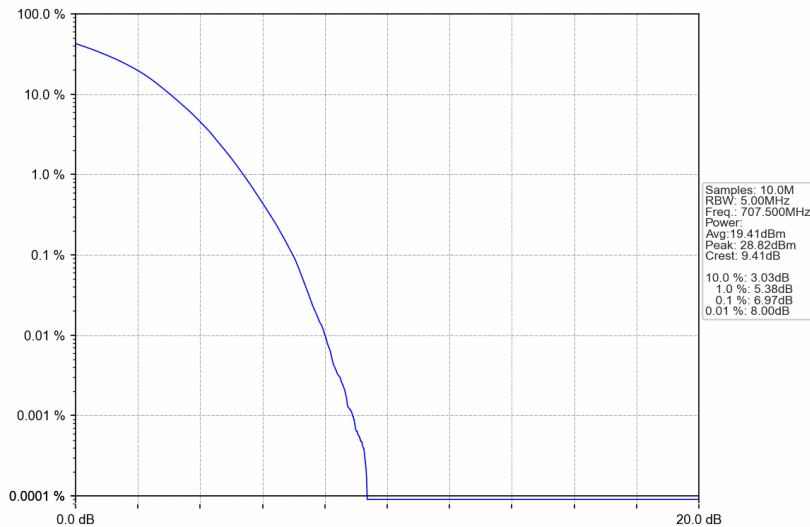
Band12_5MHz_256QAM_MCH_707.5MHz_RB_25_0_NTNV
