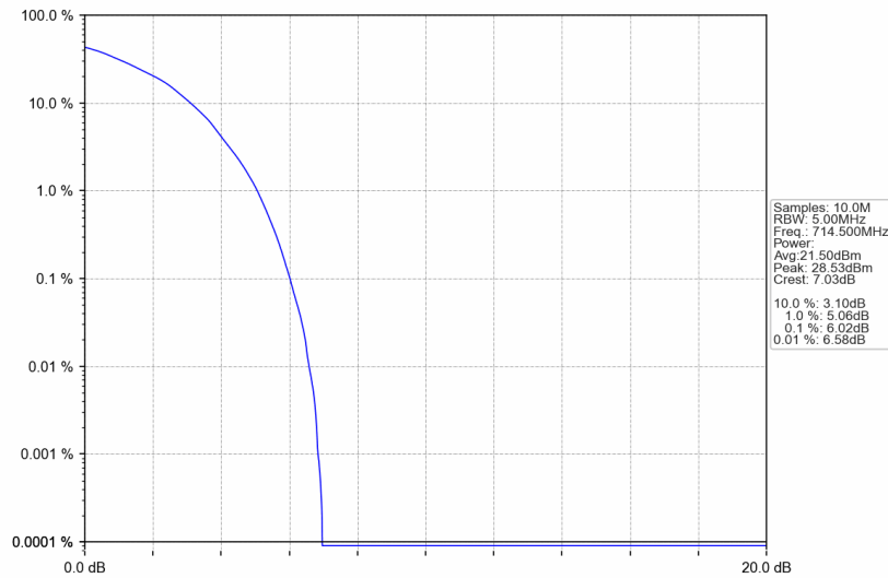
Band12_3MHz_64QAM_HCH_714.5MHz_RB_15_0_NTNV
