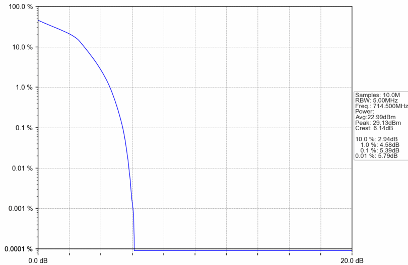
Band12_3MHz_16QAM_HCH_714.5MHz_RB_15_0_NTNV
