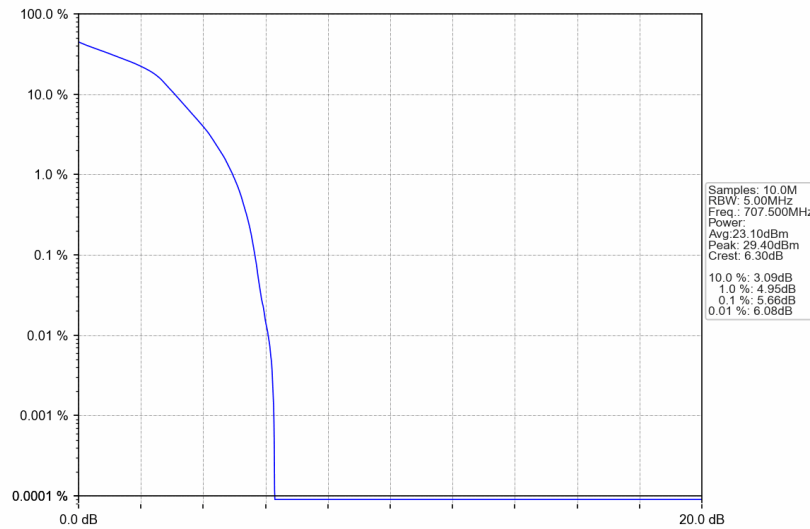
Band12_1.4MHz_16QAM_MCH_707.5MHz_RB_6_0_NTNV
