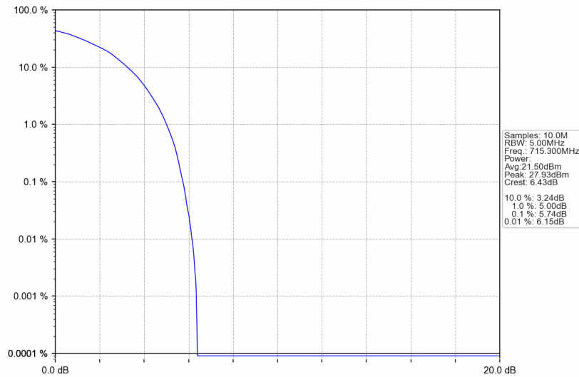
Band12_1.4MHz_64QAM_HCH_715.3MHz_RB_6_0_NTNV
