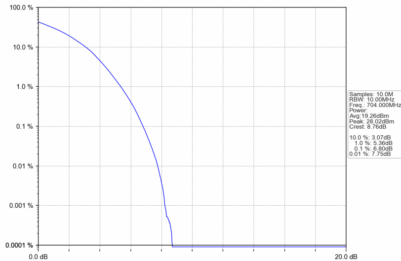
Band12_10MHz_256QAM_LCH_704MHz_RB_50_0_NTNV
