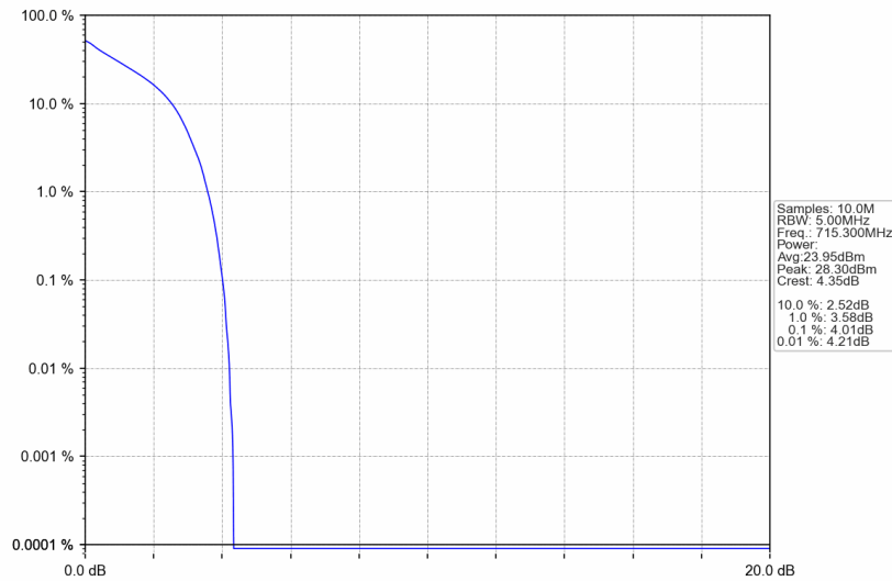
Band12_1.4MHz_QPSK_HCH_715.3MHz_RB_6_0_NTNV
