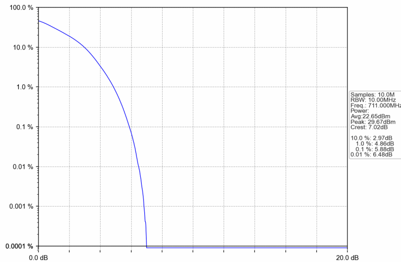
Band12_10MHz_16QAM_HCH_711MHz_RB_50_0_NTNV
