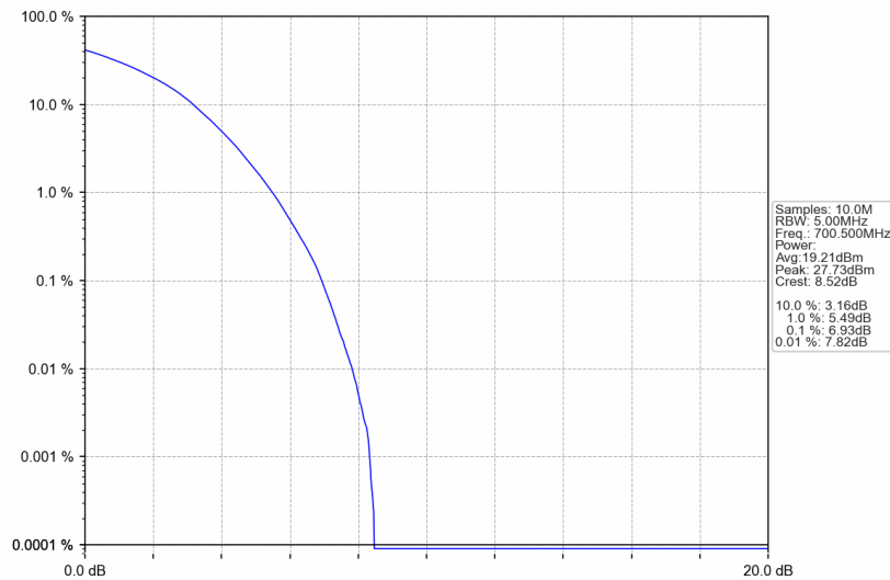
Band12_3MHz_256QAM_LCH_700.5MHz_RB_15_0_NTNV
