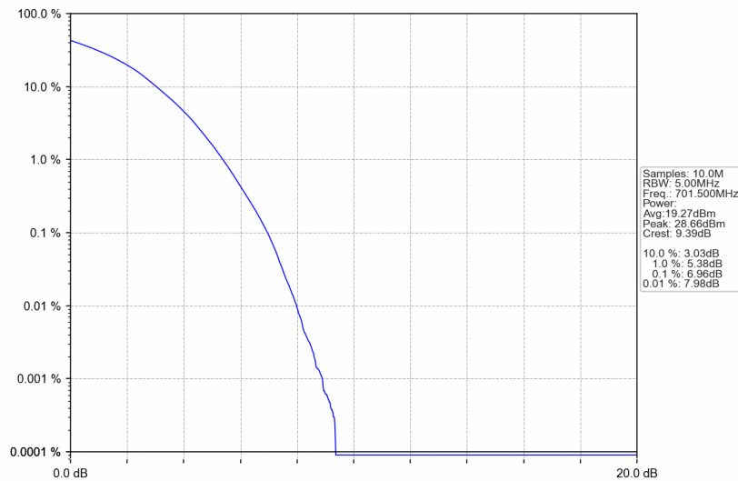
Band12_5MHz_256QAM_LCH_701.5MHz_RB_25_0_NTNV
