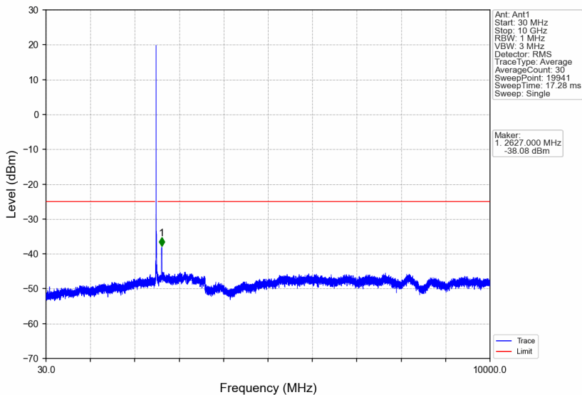
Band7_15MHz_256QAM_LCH_2507.5MHz_RB_1_0_NTNV
