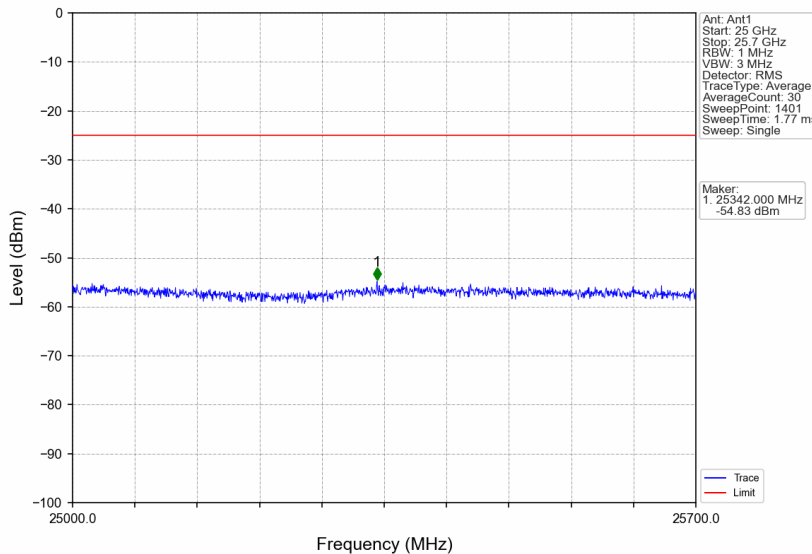
Band7_15MHz_64QAM_MCH_2535MHz_RB_1_0_NTNV
