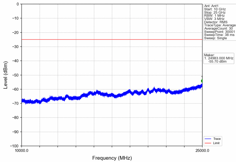
Band7_15MHz_256QAM_HCH_2562.5MHz_RB_1_0_NTNV
