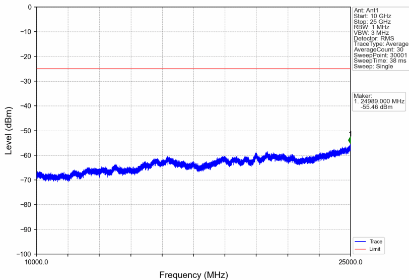
Band7_15MHz_64QAM_LCH_2507.5MHz_RB_1_0_NTNV
