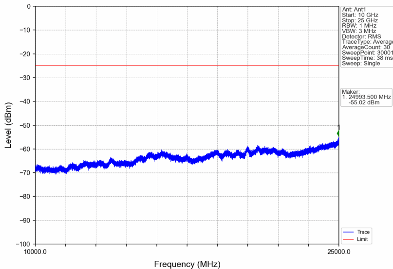
Band7_15MHz_256QAM_LCH_2507.5MHz_RB_1_0_NTNV
