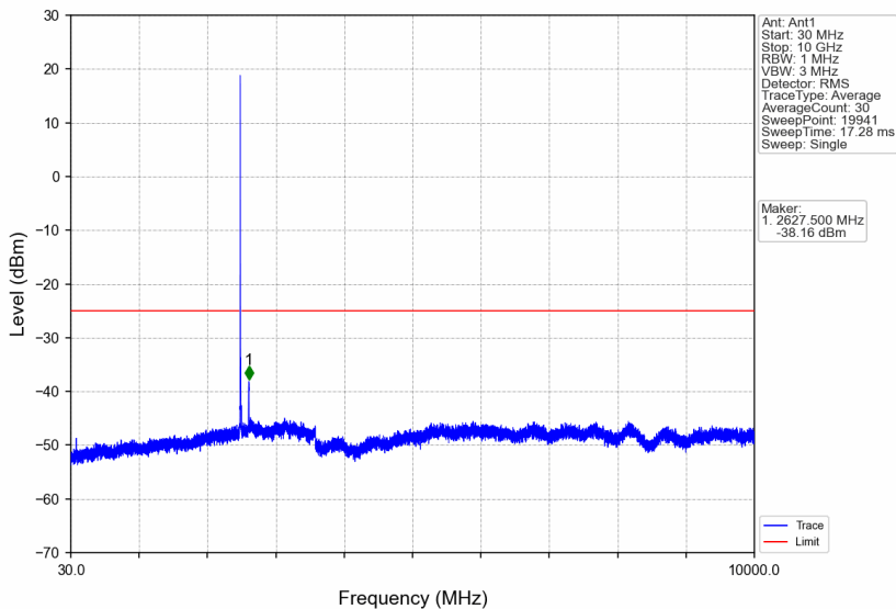
Band7_10MHz_256QAM_LCH_2505MHz_RB_1_0_NTNV
