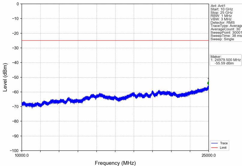
Band7_5MHz_256QAM_LCH_2502.5MHz_RB_1_0_NTNV
