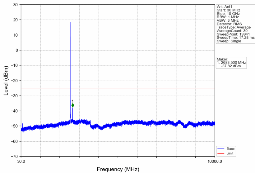
Band7_10MHz_256QAM_HCH_2565MHz_RB_1_0_NTNV
