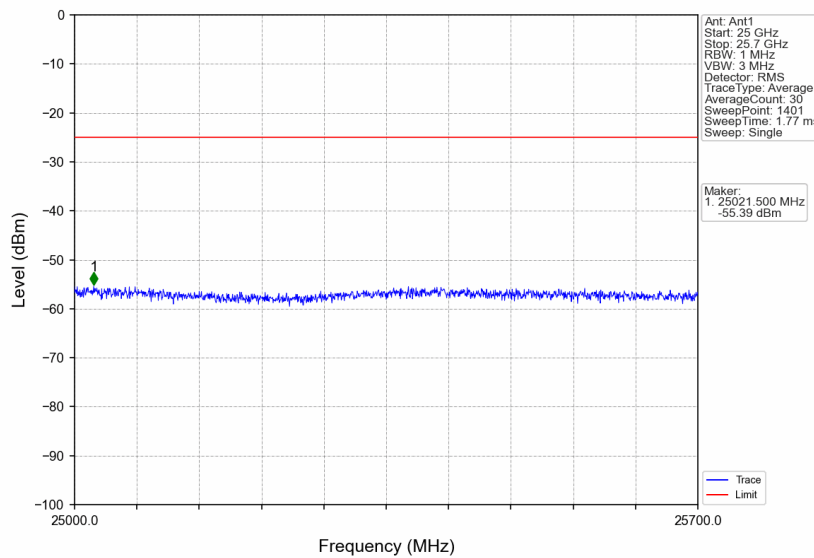
Band7_10MHz_256QAM_HCH_2565MHz_RB_1_0_NTNV
