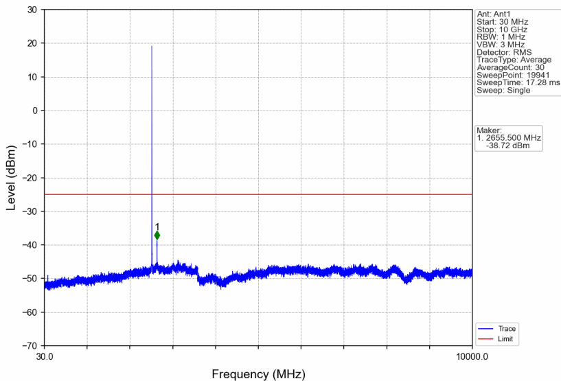
Band7_5MHz_256QAM_MCH_2535MHz_RB_1_0_NTNV
