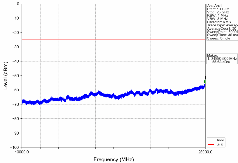
Band7_5MHz_64QAM_HCH_2567.5MHz_RB_1_0_NTNV
