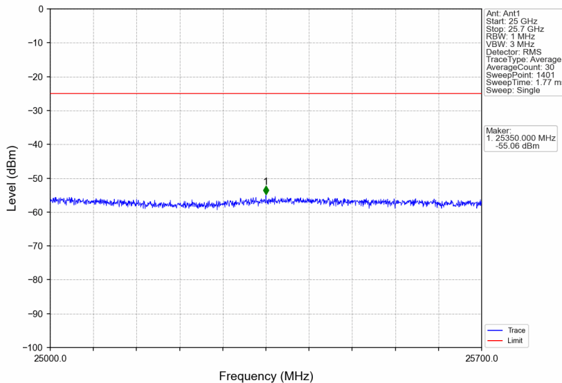
Band7_5MHz_256QAM_HCH_2567.5MHz_RB_1_0_NTNV
