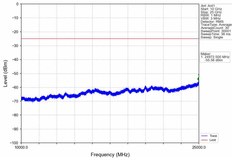
Band7_10MHz_256QAM_HCH_2565MHz_RB_1_0_NTNV
