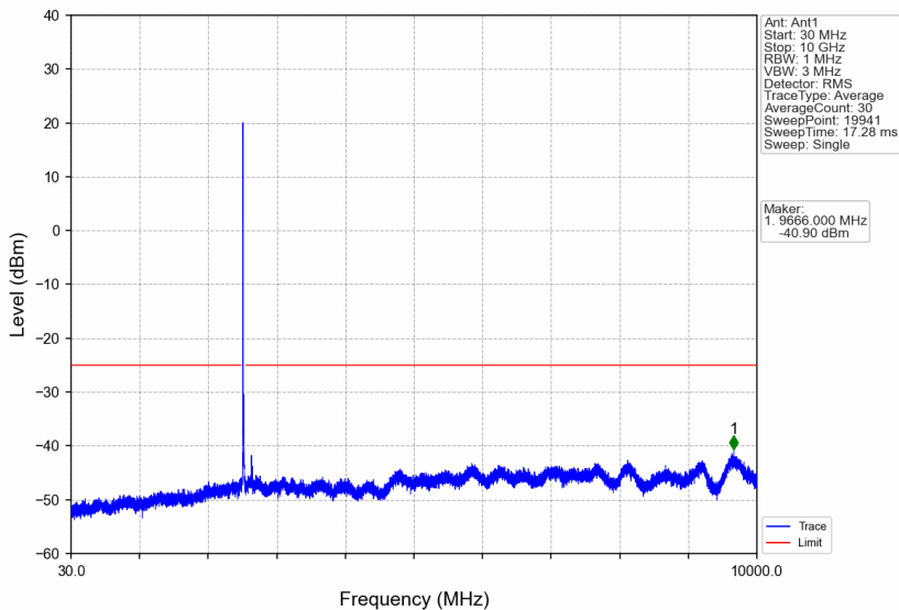
Band7_15MHz_16QAM_MCH_2535MHz_RB_1_0_NTNV
