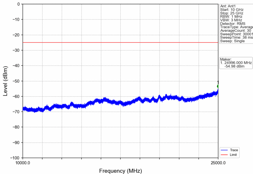
Band7_10MHz_256QAM_MCH_2535MHz_RB_1_0_NTNV
