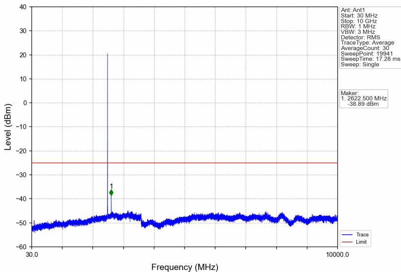
Band7_5MHz_256QAM_LCH_2502.5MHz_RB_1_0_NTNV
