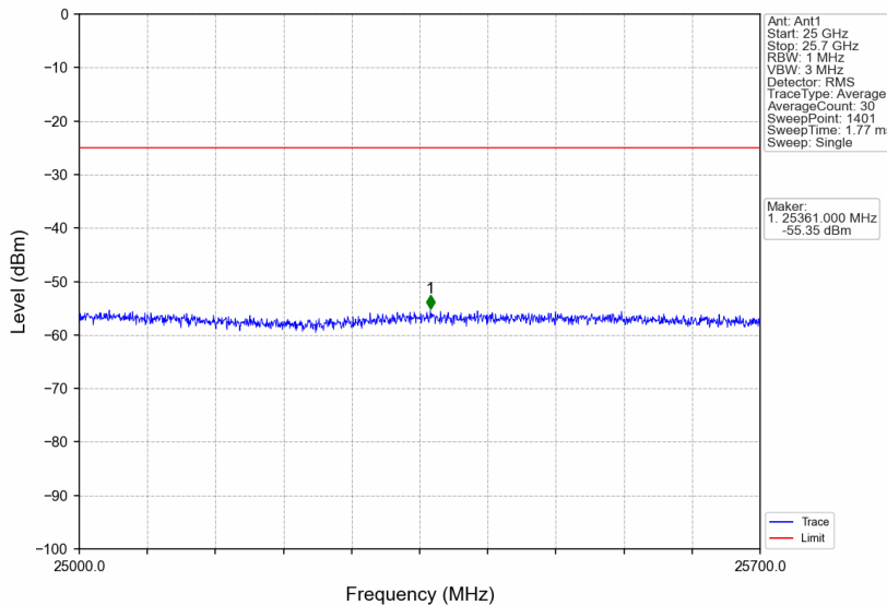
Band7_10MHz_64QAM_MCH_2535MHz_RB_1_0_NTNV
