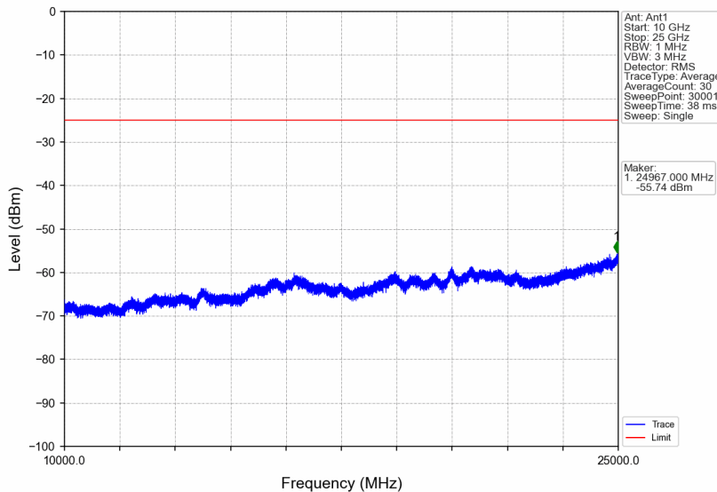
Band7_5MHz_256QAM_MCH_2535MHz_RB_1_0_NTNV
