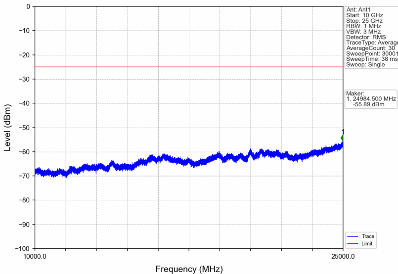
Band7_10MHz_256QAM_LCH_2505MHz_RB_1_0_NTNV
