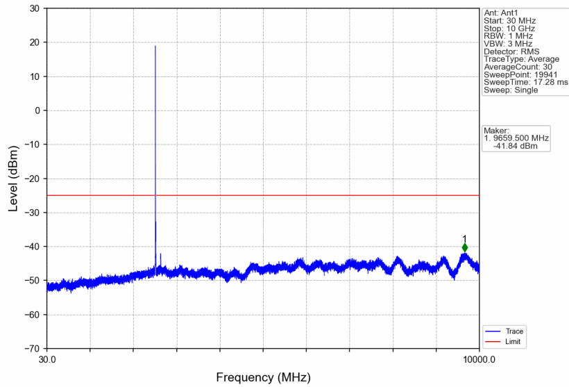
Band7_10MHz_16QAM_MCH_2535MHz_RB_1_0_NTNV
