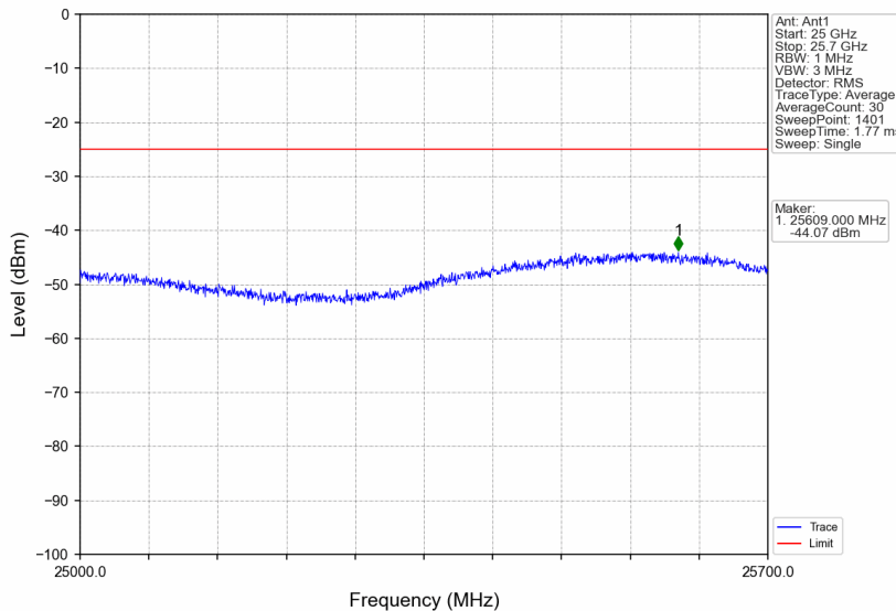
Band7_15MHz_QPSK_MCH_2535MHz_RB_1_0_NTNV
