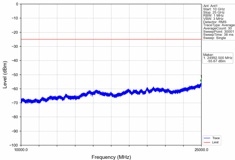
Band7_10MHz_64QAM_LCH_2505MHz_RB_1_0_NTNV
