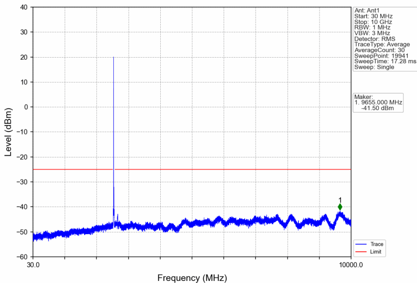
Band7_15MHz_QPSK_HCH_2562.5MHz_RB_1_0_NTNV
