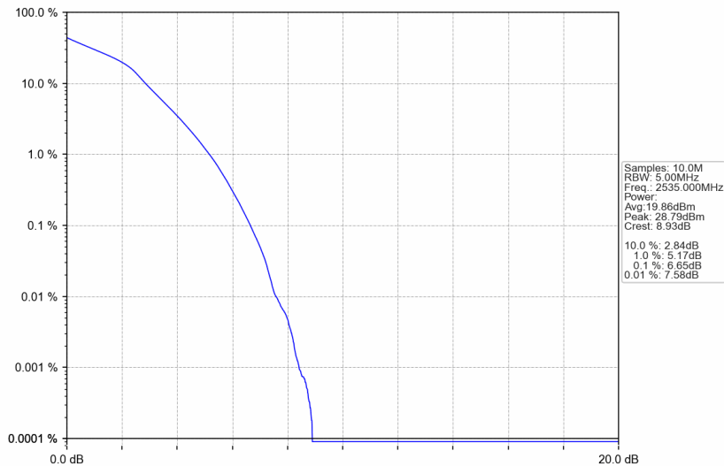
Band7_5MHz_16QAM_MCH_2535MHz_RB_25_0_NTNV
