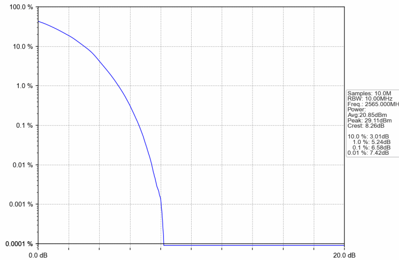
Band7_10MHz_64QAM_HCH_2565MHz_RB_50_0_NTNV
