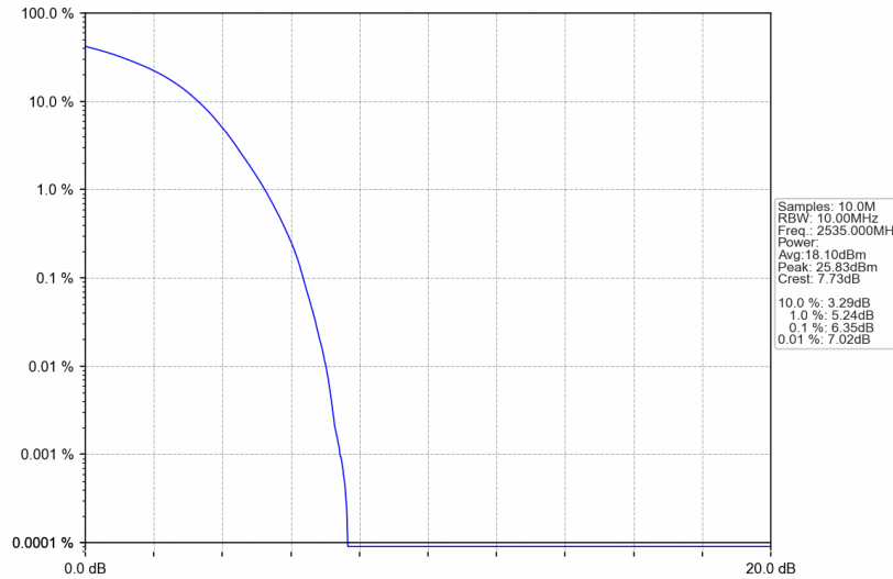
Band7_15MHz_16QAM_MCH_2535MHz_RB_75_0_NTNV
