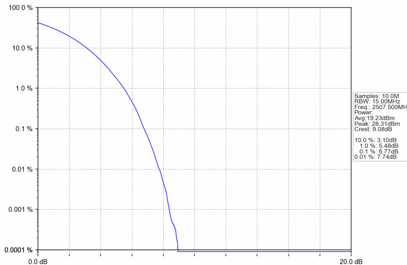
Band7_15MHz_256QAM_LCH_2507.5MHz_RB_75_0_NTNV
