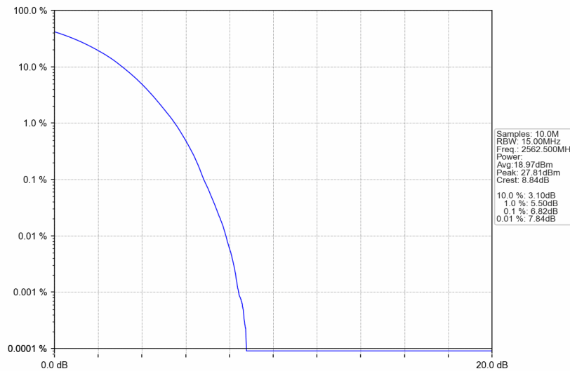
Band7_15MHz_256QAM_HCH_2562.5MHz_RB_75_0_NTNV
