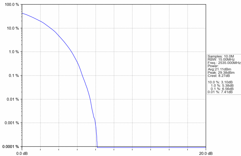
Band7_15MHz_64QAM_MCH_2535MHz_RB_75_0_NTNV
