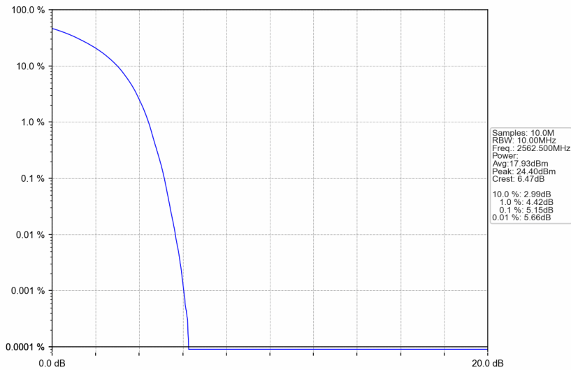
Band7_15MHz_QPSK_HCH_2562.5MHz_RB_75_0_NTNV
