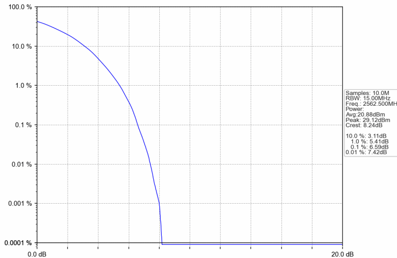
Band7_15MHz_64QAM_HCH_2562.5MHz_RB_75_0_NTNV
