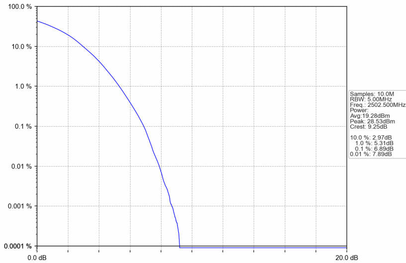
Band7_5MHz_256QAM_LCH_2502.5MHz_RB_25_0_NTNV
