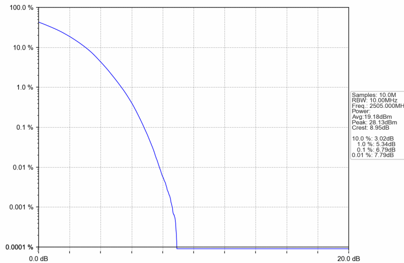
Band7_10MHz_256QAM_LCH_2505MHz_RB_50_0_NTNV
