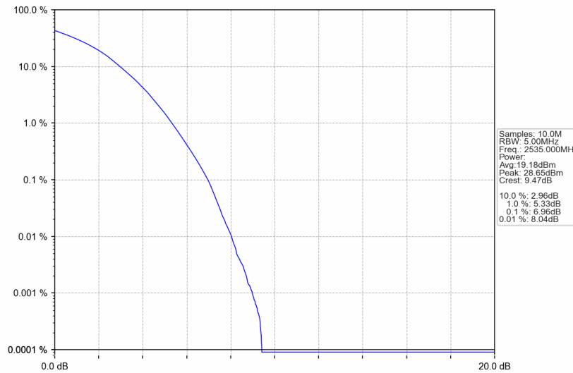
Band7_5MHz_256QAM_MCH_2535MHz_RB_25_0_NTNV
