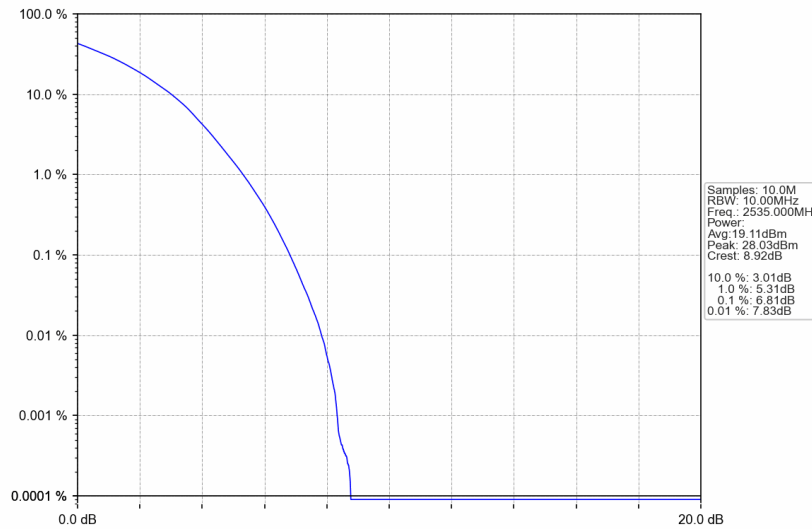
Band7_10MHz_256QAM_MCH_2535MHz_RB_50_0_NTNV
