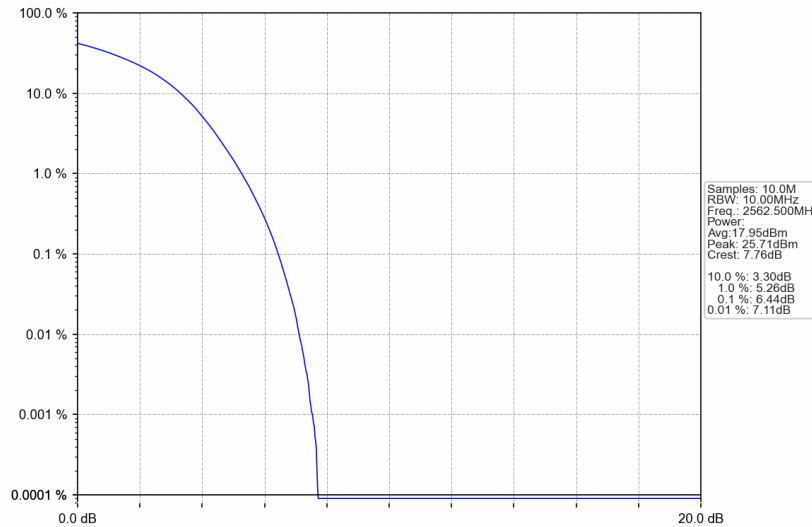
Band7_15MHz_16QAM_HCH_2562.5MHz_RB_75_0_NTNV
