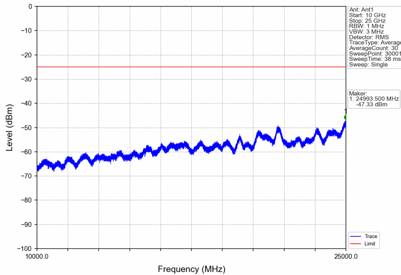
Band7_5MHz_16QAM_MCH_2535MHz_RB_1_0_NTNV
