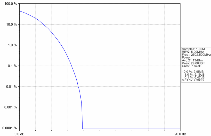
Band7_5MHz_64QAM_LCH_2502.5MHz_RB_25_0_NTNV
