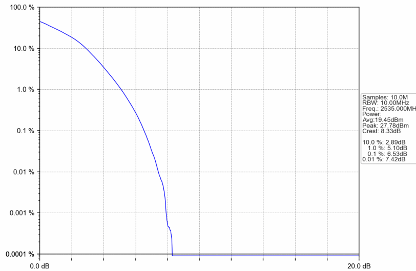
Band7_10MHz_16QAM_MCH_2535MHz_RB_50_0_NTNV
