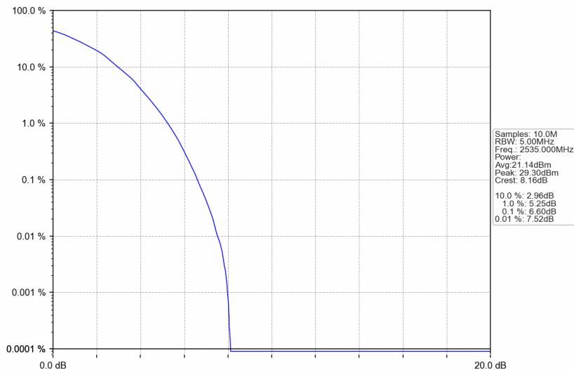
Band7_5MHz_64QAM_MCH_2535MHz_RB_25_0_NTNV
