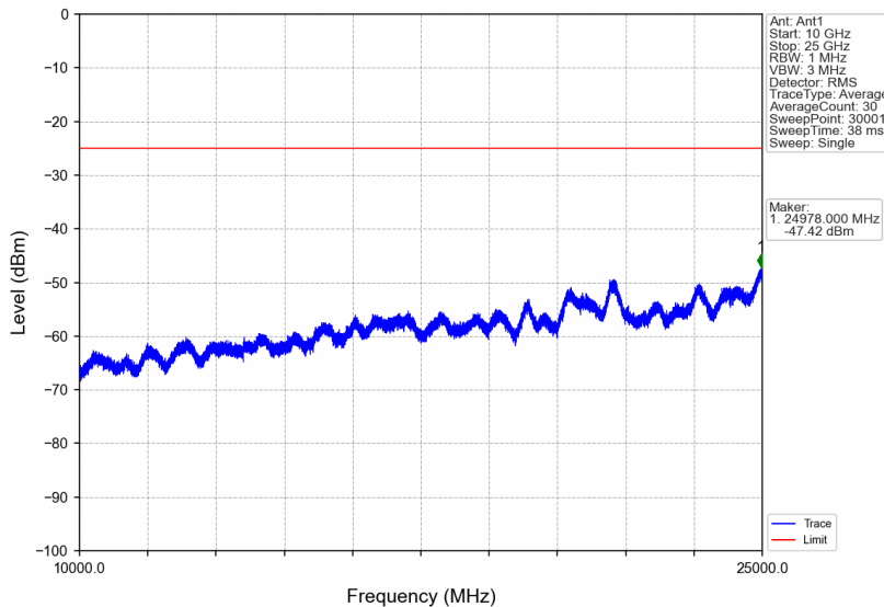
Band7_5MHz_16QAM_LCH_2502.5MHz_RB_1_0_NTNV
