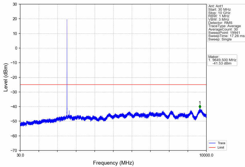
Band7_5MHz_16QAM_MCH_2535MHz_RB_1_0_NTNV
