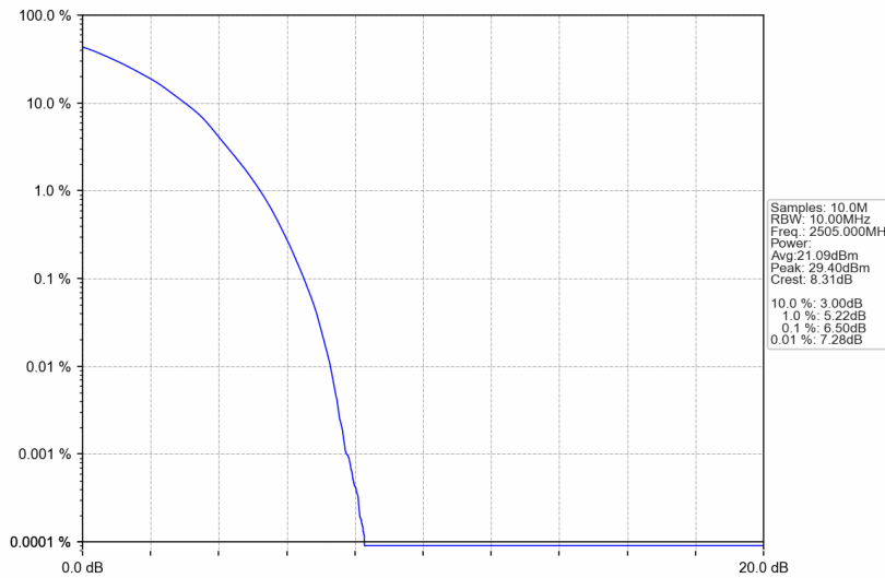
Band7_10MHz_64QAM_LCH_2505MHz_RB_50_0_NTNV
