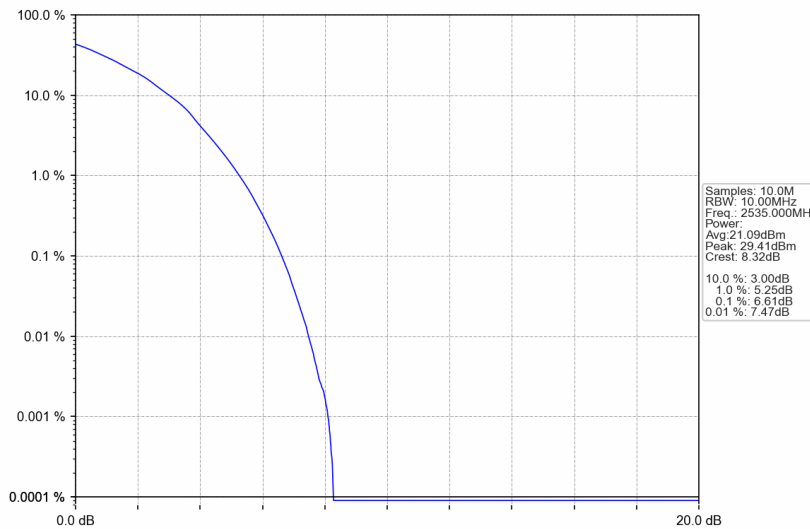
Band7_10MHz_64QAM_MCH_2535MHz_RB_50_0_NTNV
