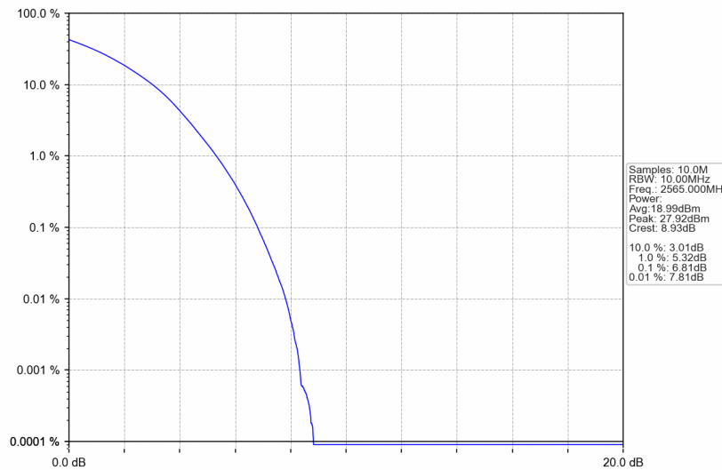
Band7_10MHz_256QAM_HCH_2565MHz_RB_50_0_NTNV
