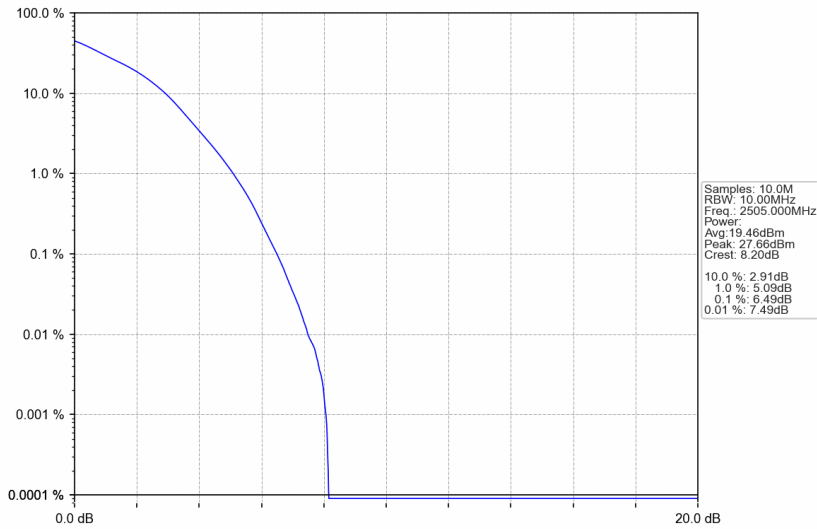
Band7_10MHz_16QAM_LCH_2505MHz_RB_50_0_NTNV
