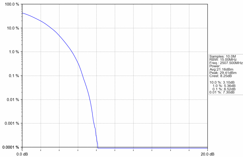
Band7_15MHz_64QAM_LCH_2507.5MHz_RB_75_0_NTNV
