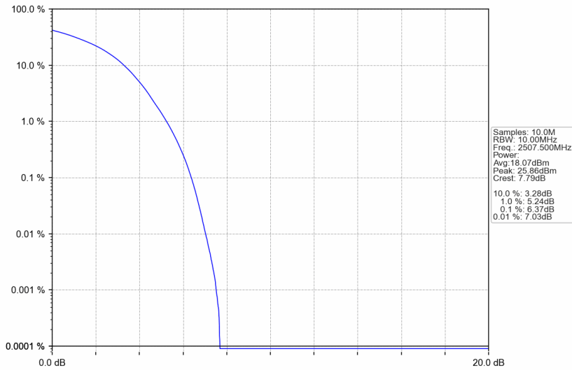
Band7_15MHz_16QAM_LCH_2507.5MHz_RB_75_0_NTNV
