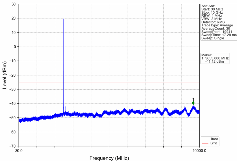
Band7_5MHz_16QAM_LCH_2502.5MHz_RB_1_0_NTNV
