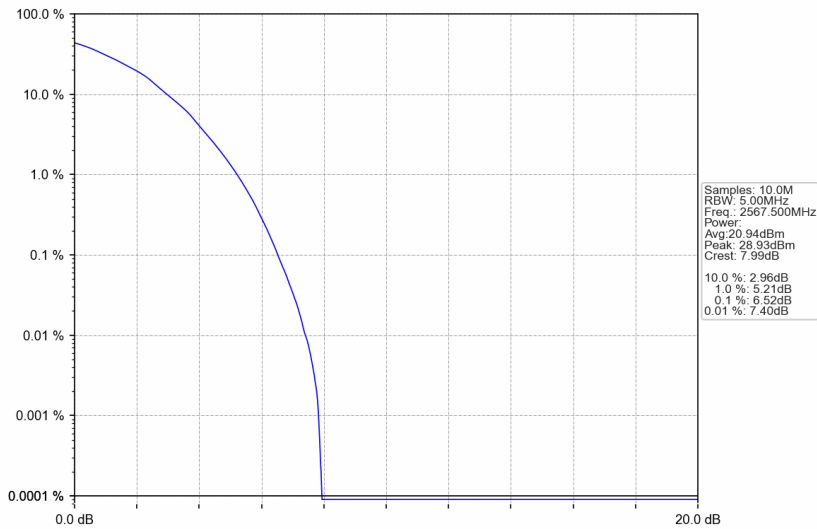
Band7_5MHz_64QAM_HCH_2567.5MHz_RB_25_0_NTNV
