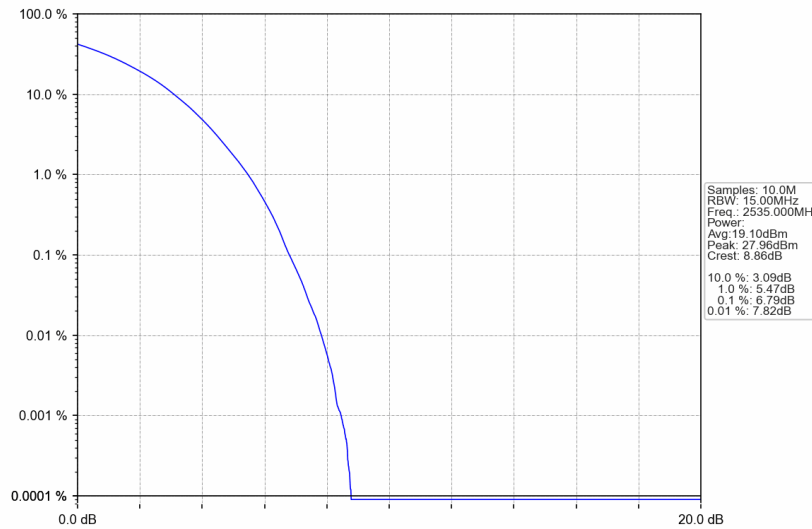
Band7_15MHz_256QAM_MCH_2535MHz_RB_75_0_NTNV
