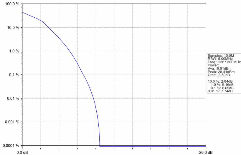
Band7_5MHz_16QAM_HCH_2567.5MHz_RB_25_0_NTNV
