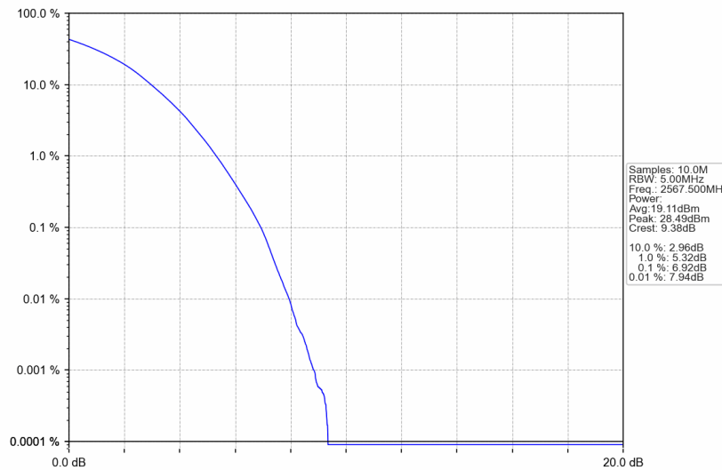
Band7_5MHz_256QAM_HCH_2567.5MHz_RB_25_0_NTNV
