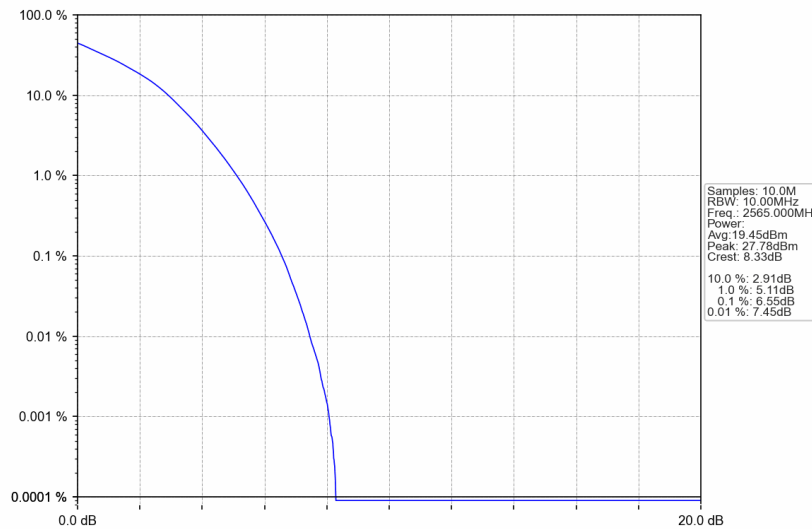
Band7_10MHz_16QAM_HCH_2565MHz_RB_50_0_NTNV
