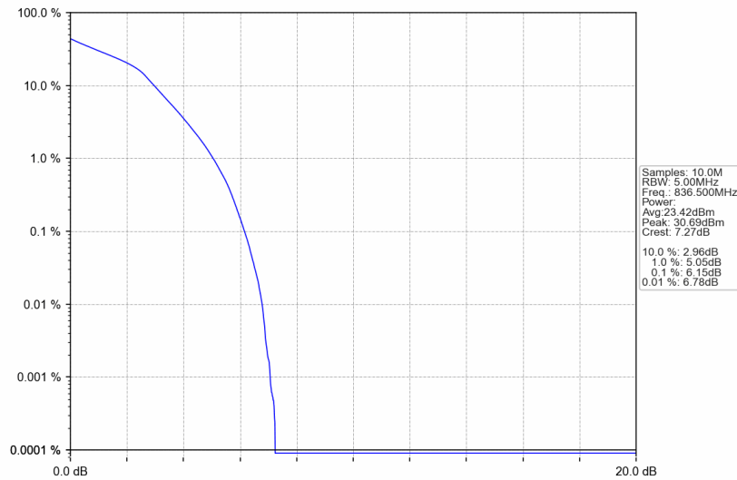
Band5_3MHz_16QAM_MCH_836.5MHz_RB_15_0_NTNV
