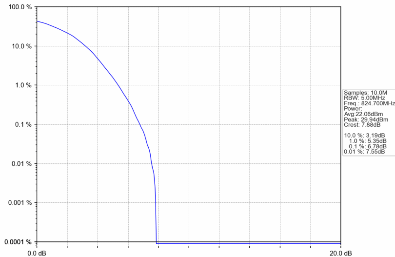
Band5_1.4MHz_64QAM_LCH_824.7MHz_RB_6_0_NTNV
