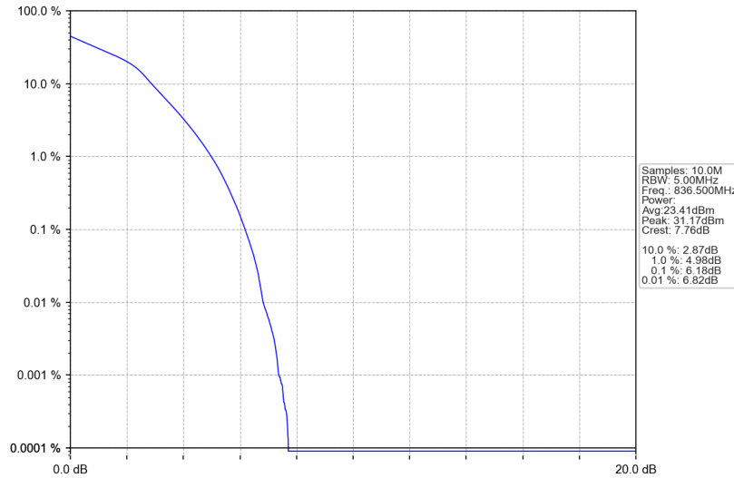
Band5_5MHz_16QAM_MCH_836.5MHz_RB_25_0_NTNV
