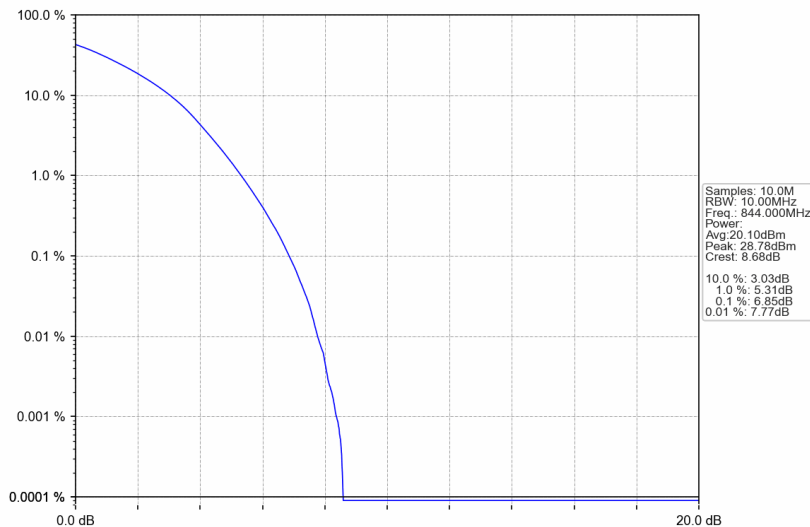
Band5_10MHz_256QAM_HCH_844MHz_RB_50_0_NTNV
