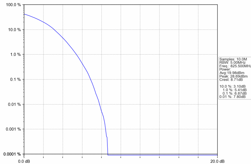
Band5_3MHz_256QAM_LCH_825.5MHz_RB_15_0_NTNV
