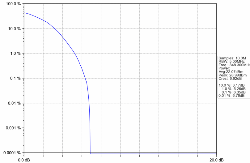
Band5_1.4MHz_64QAM_HCH_848.3MHz_RB_6_0_NTNV
