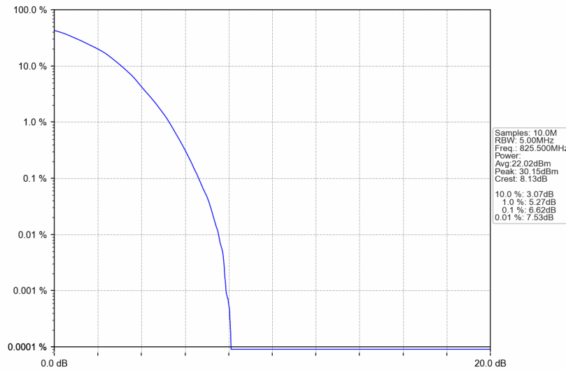
Band5_3MHz_64QAM_LCH_825.5MHz_RB_15_0_NTNV
