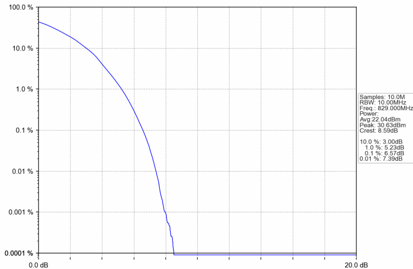
Band5_10MHz_64QAM_LCH_829MHz_RB_50_0_NTNV
