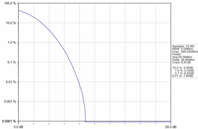
Band5_5MHz_256QAM_HCH_846.5MHz_RB_25_0_NTNV
