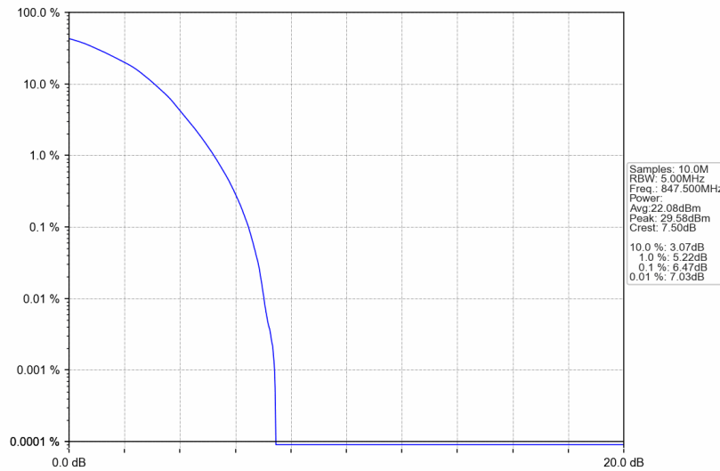
Band5_3MHz_64QAM_HCH_847.5MHz_RB_15_0_NTNV
