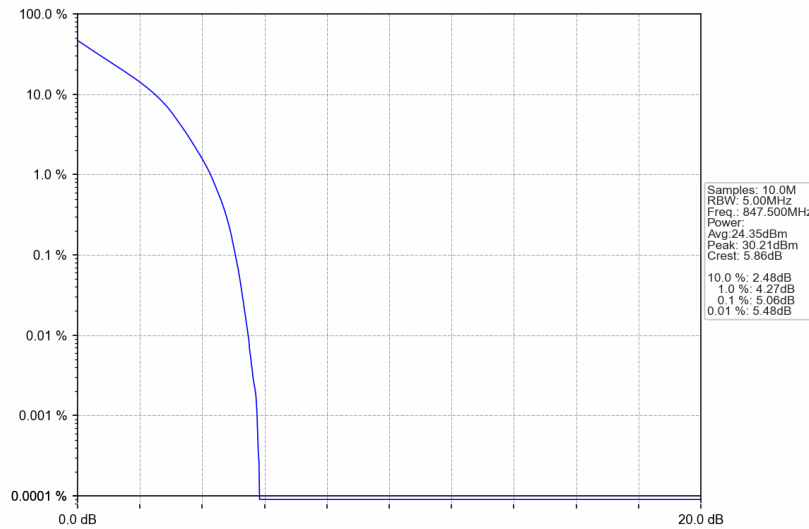
Band5_3MHz_QPSK_HCH_847.5MHz_RB_15_0_NTNV
