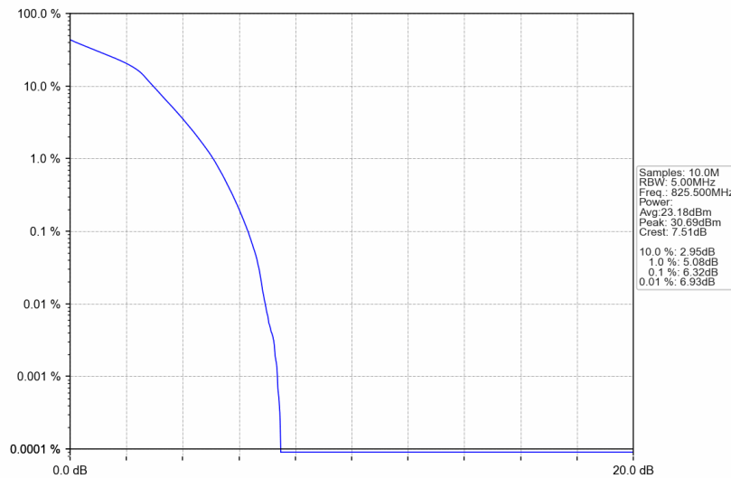
Band5_3MHz_16QAM_LCH_825.5MHz_RB_15_0_NTNV
