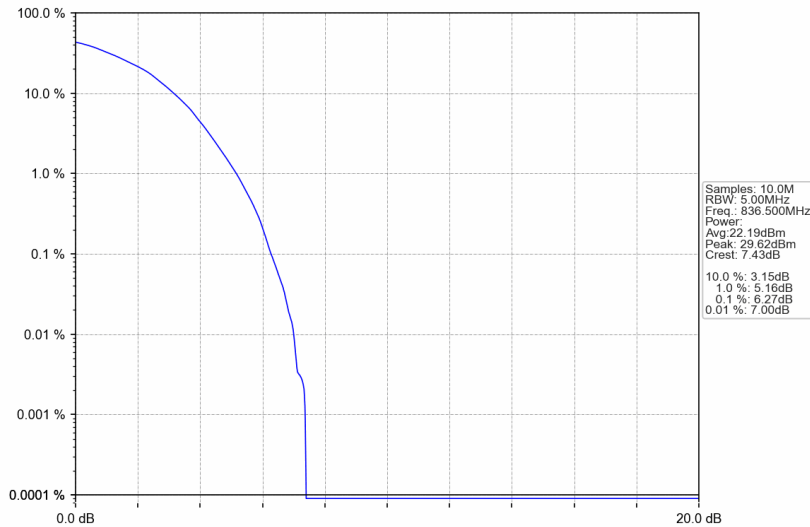
Band5_1.4MHz_64QAM_MCH_836.5MHz_RB_6_0_NTNV
