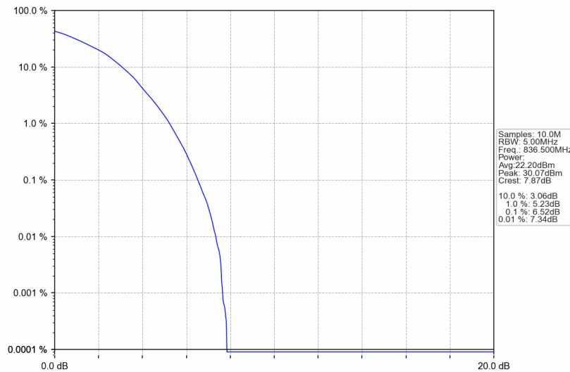
Band5_3MHz_64QAM_MCH_836.5MHz_RB_15_0_NTNV
