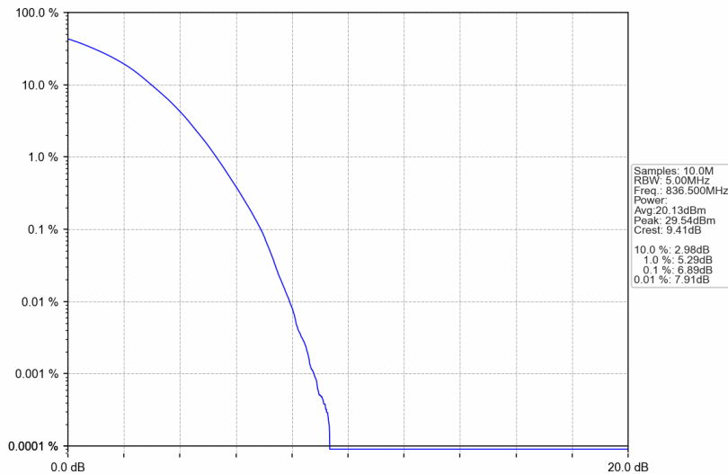
Band5_5MHz_256QAM_MCH_836.5MHz_RB_25_0_NTNV
