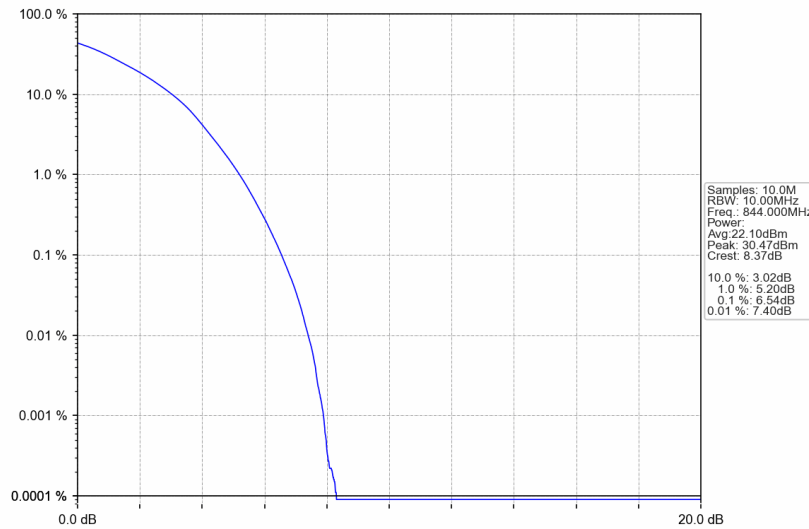
Band5_10MHz_64QAM_HCH_844MHz_RB_50_0_NTNV
