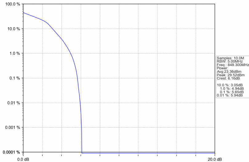
Band5_1.4MHz_16QAM_HCH_848.3MHz_RB_6_0_NTNV
