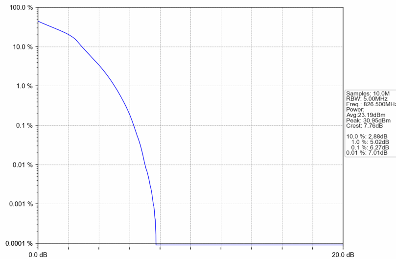
Band5_5MHz_16QAM_LCH_826.5MHz_RB_25_0_NTNV
