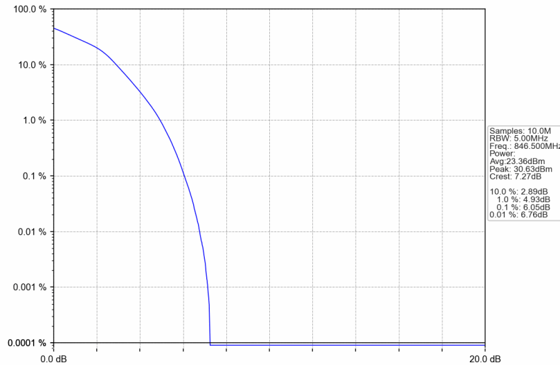
Band5_5MHz_16QAM_HCH_846.5MHz_RB_25_0_NTNV
