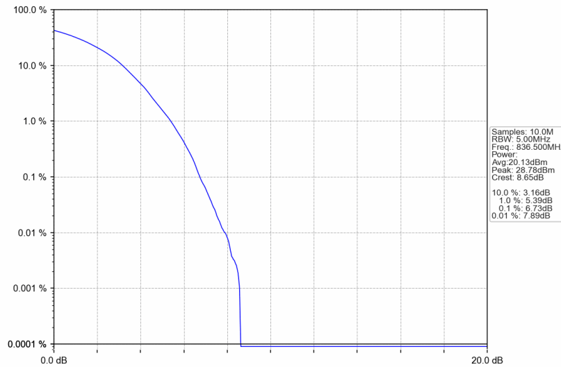
Band5_1.4MHz_256QAM_MCH_836.5MHz_RB_6_0_NTNV
