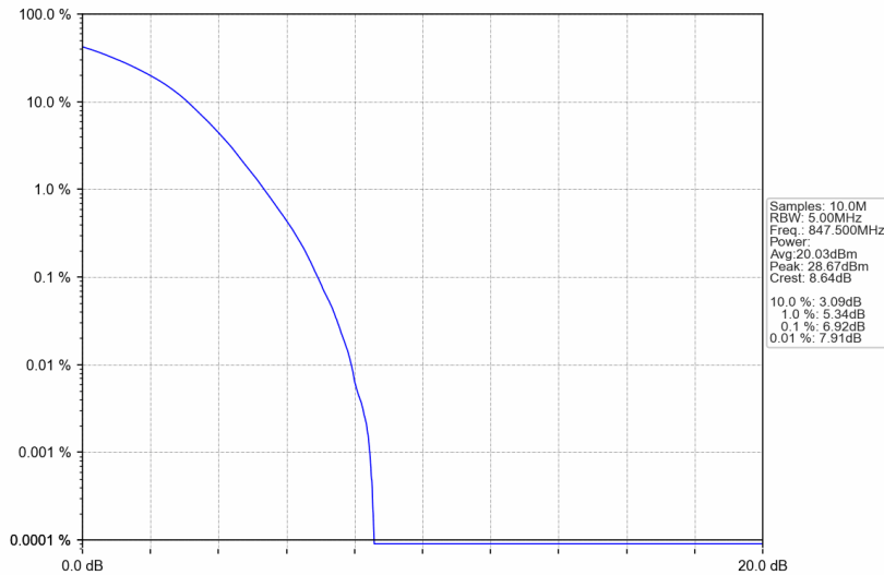
Band5_3MHz_256QAM_HCH_847.5MHz_RB_15_0_NTNV
