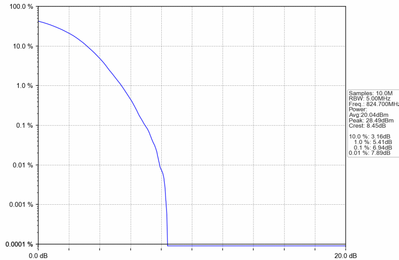
Band5_1.4MHz_256QAM_LCH_824.7MHz_RB_6_0_NTNV
