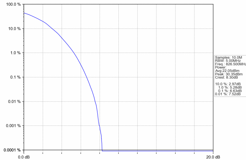
Band5_5MHz_64QAM_LCH_826.5MHz_RB_25_0_NTNV
