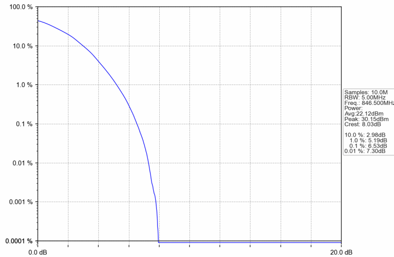
Band5_5MHz_64QAM_HCH_846.5MHz_RB_25_0_NTNV
