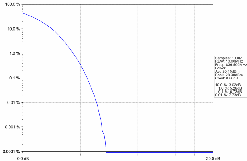
Band5_10MHz_256QAM_MCH_836.5MHz_RB_50_0_NTNV
