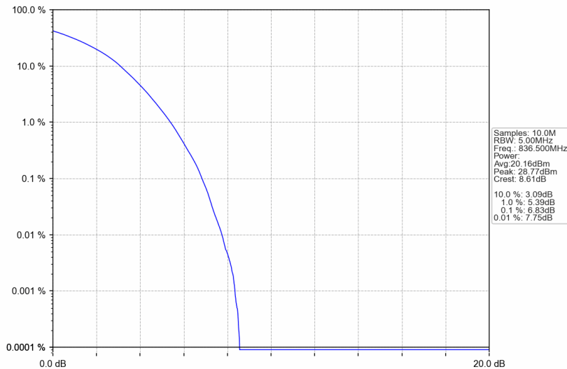
Band5_3MHz_256QAM_MCH_836.5MHz_RB_15_0_NTNV
