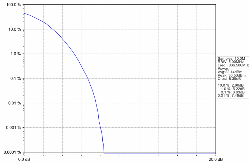
Band5_5MHz_64QAM_MCH_836.5MHz_RB_25_0_NTNV
