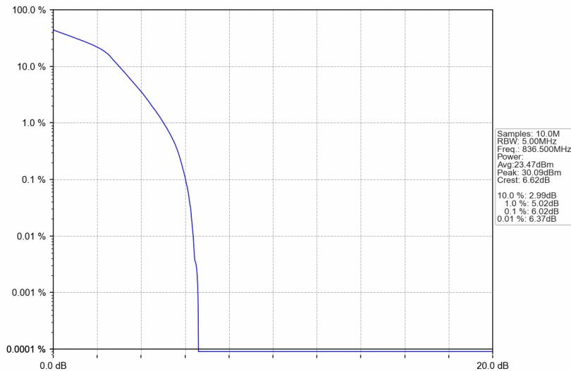
Band5_1.4MHz_16QAM_MCH_836.5MHz_RB_6_0_NTNV
