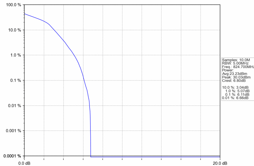
Band5_1.4MHz_16QAM_LCH_824.7MHz_RB_6_0_NTNV
