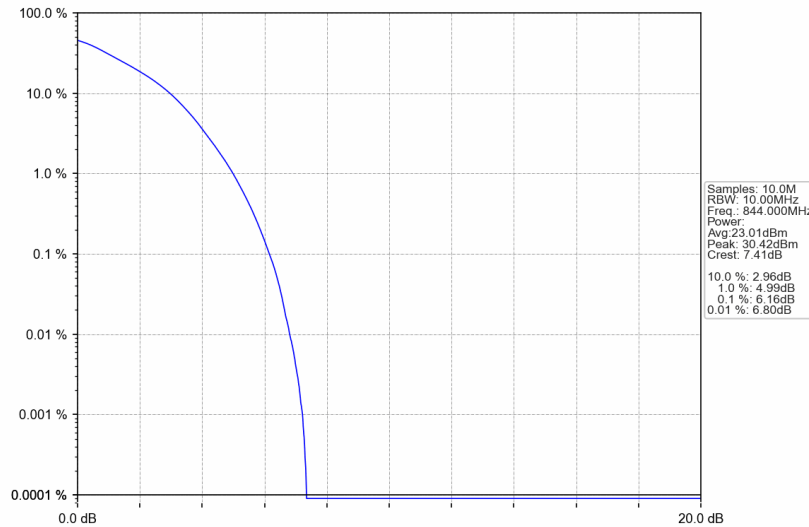
Band5_10MHz_16QAM_HCH_844MHz_RB_50_0_NTNV
