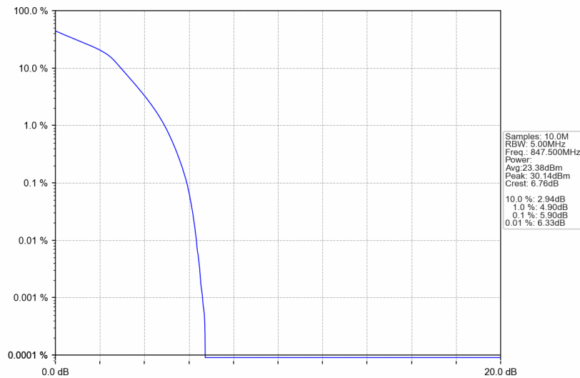
Band5_3MHz_16QAM_HCH_847.5MHz_RB_15_0_NTNV
