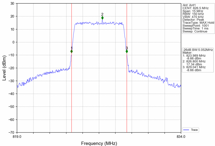
Band5_5MHz_256QAM_LCH_826.5MHz_RB_25_0_NTNV
