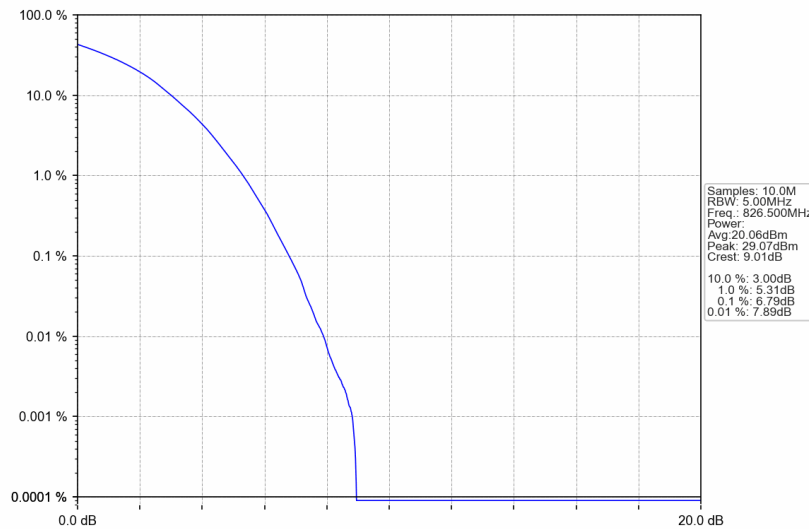
Band5_5MHz_256QAM_LCH_826.5MHz_RB_25_0_NTNV
