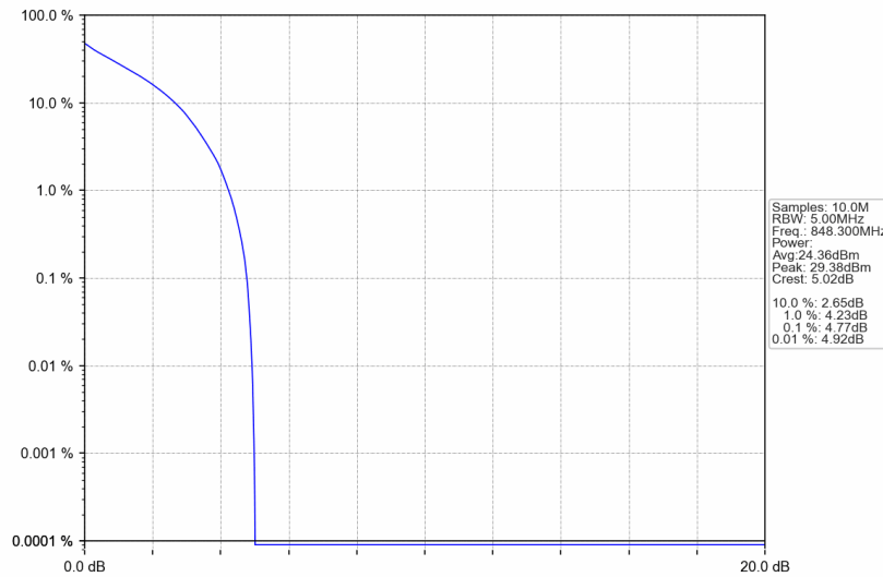
Band5_1.4MHz_QPSK_HCH_848.3MHz_RB_6_0_NTNV
