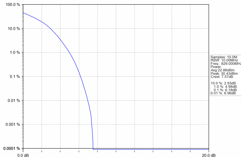
Band5_10MHz_16QAM_LCH_829MHz_RB_50_0_NTNV
