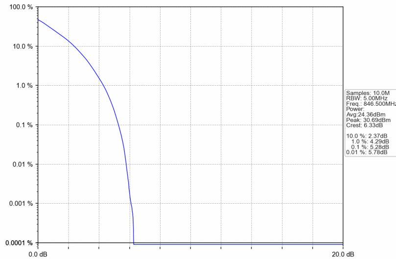
Band5_5MHz_QPSK_HCH_846.5MHz_RB_25_0_NTNV
