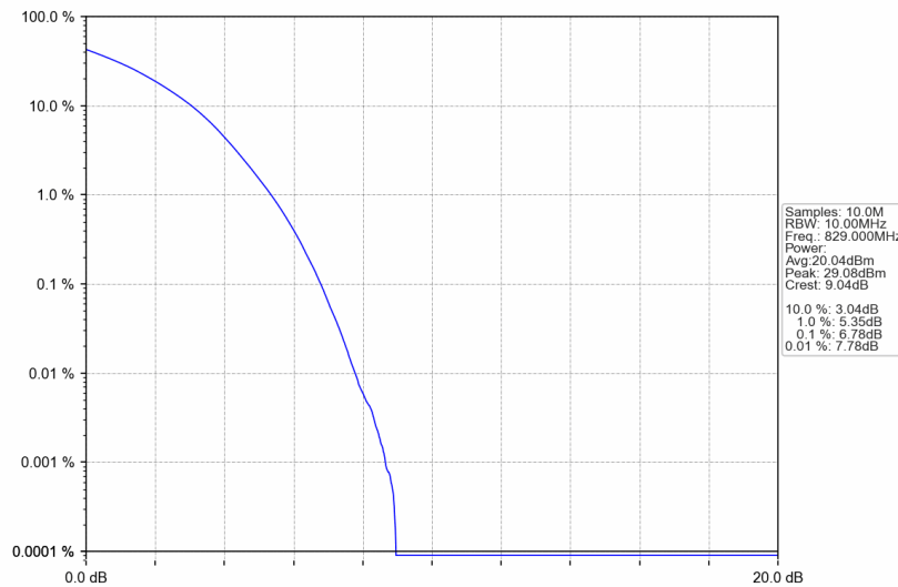
Band5_10MHz_256QAM_LCH_829MHz_RB_50_0_NTNV
