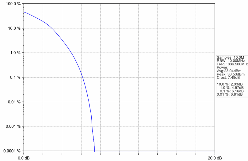
Band5_10MHz_16QAM_MCH_836.5MHz_RB_50_0_NTNV
