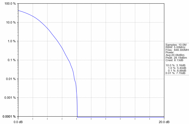
Band5_1.4MHz_256QAM_HCH_848.3MHz_RB_6_0_NTNV
