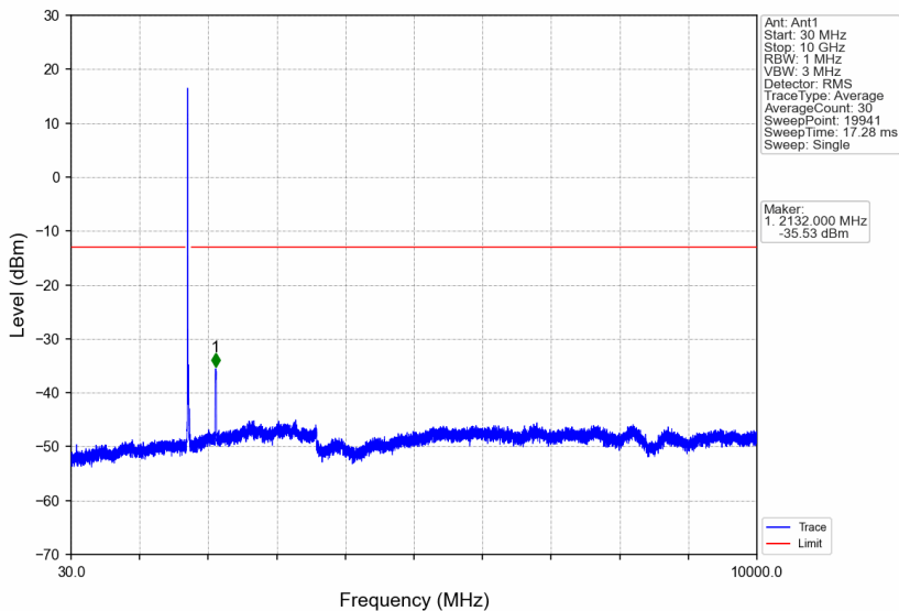
Band4_20MHz_256QAM_MCH_1732.5MHz_RB_1_0_NTNV
