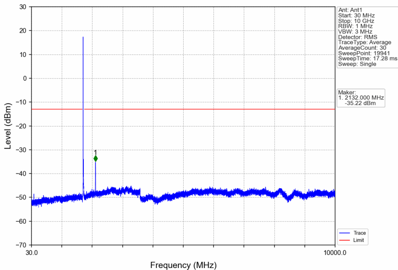
Band4_15MHz_256QAM_MCH_1732.5MHz_RB_1_0_NTNV
