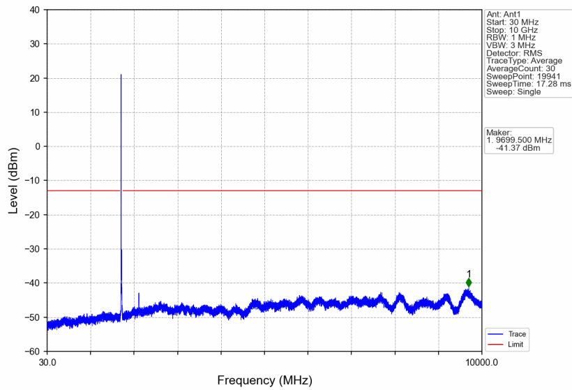
Band4_15MHz_QPSK_MCH_1732.5MHz_RB_1_0_NTNV
