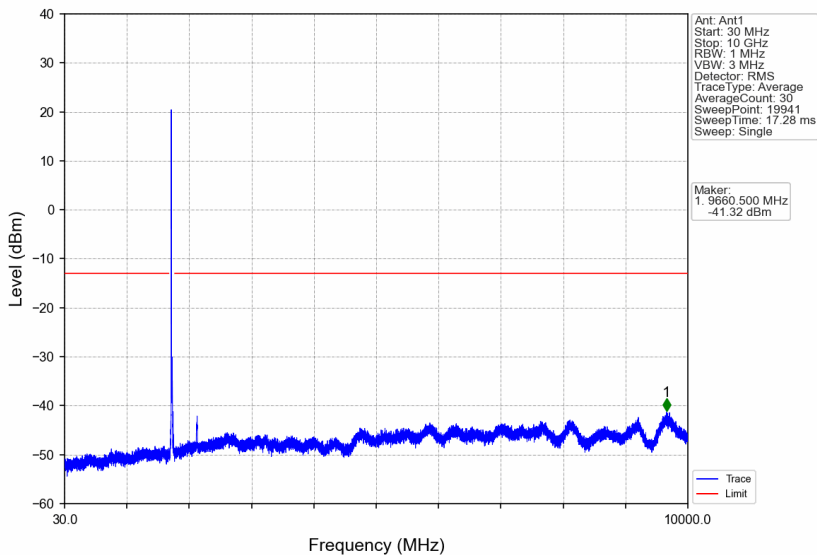
Band4_20MHz_16QAM_HCH_1745MHz_RB_1_0_NTNV
