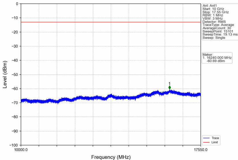
Band4_20MHz_256QAM_MCH_1732.5MHz_RB_1_0_NTNV
