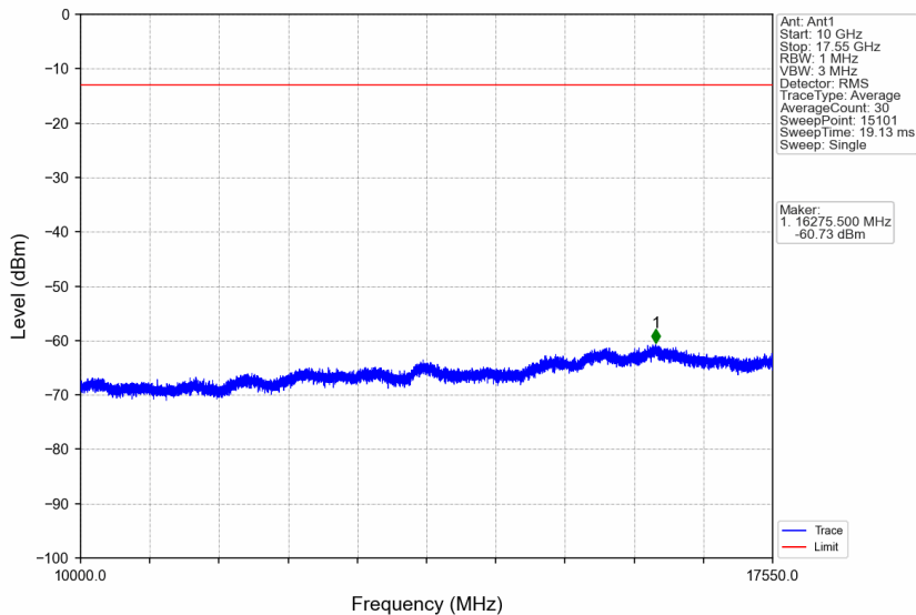
Band4_15MHz_256QAM_MCH_1732.5MHz_RB_1_0_NTNV
