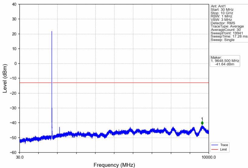
Band4_15MHz_16QAM_MCH_1732.5MHz_RB_1_0_NTNV
