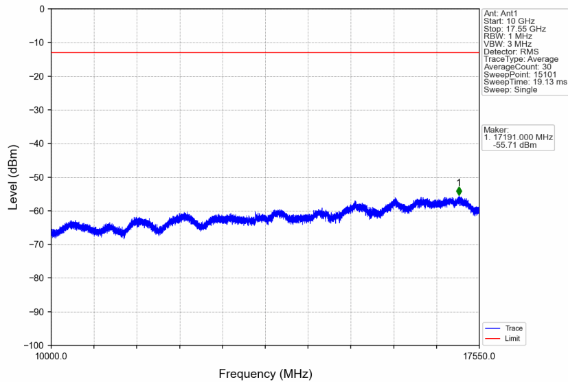
Band4_15MHz_QPSK_MCH_1732.5MHz_RB_1_0_NTNV
