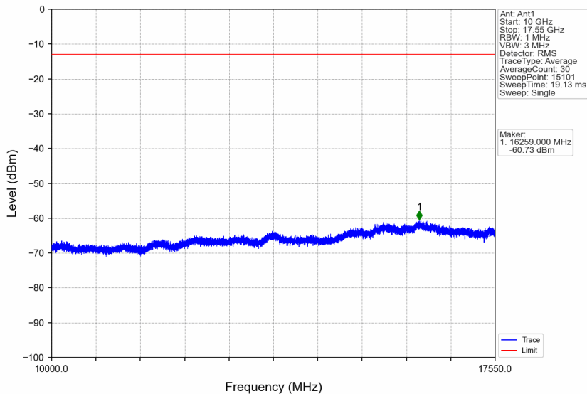
Band4_5MHz_256QAM_HCH_1752.5MHz_RB_1_0_NTNV
