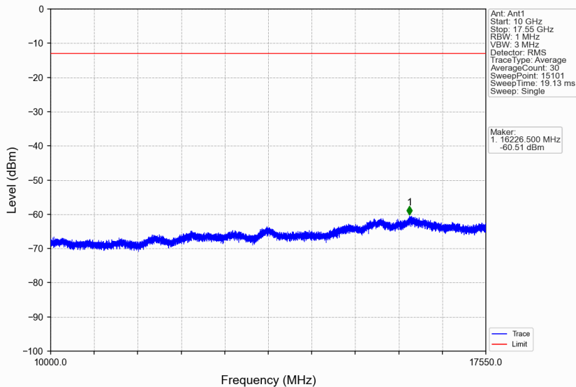
Band4_3MHz_256QAM_MCH_1732.5MHz_RB_1_0_NTNV
