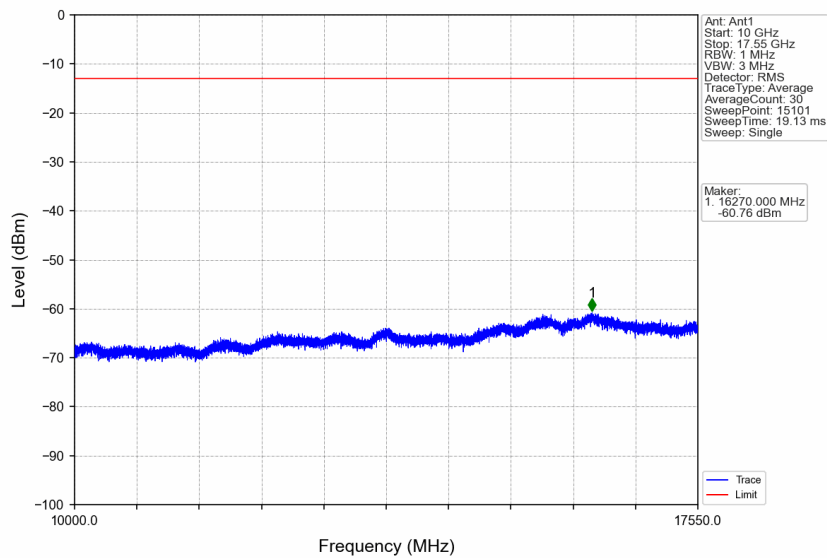
Band4_3MHz_256QAM_HCH_1753.5MHz_RB_1_0_NTNV
