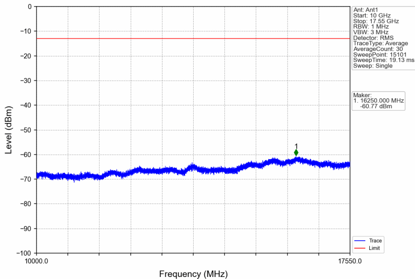
Band4_5MHz_64QAM_MCH_1732.5MHz_RB_1_0_NTNV
