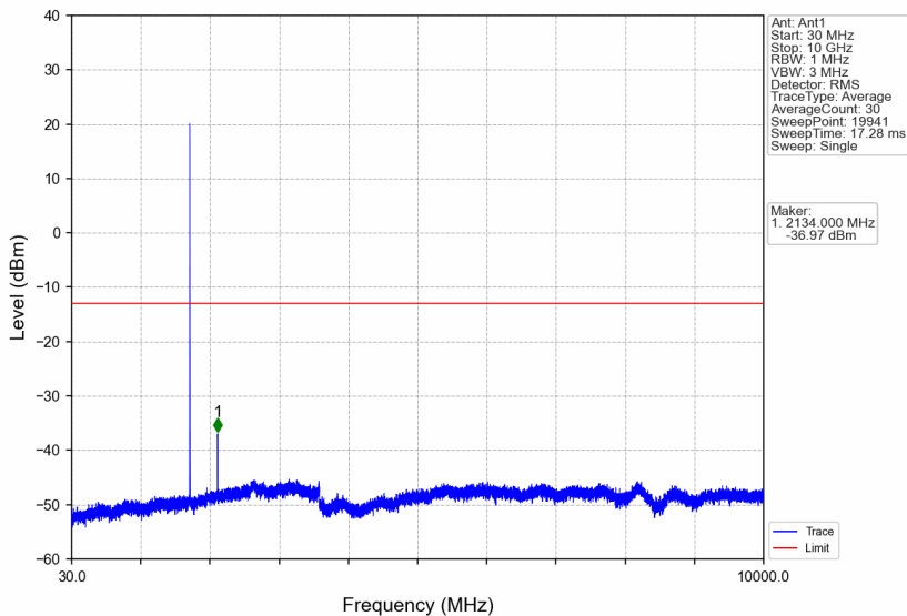
Band4_3MHz_64QAM_MCH_1732.5MHz_RB_1_0_NTNV
