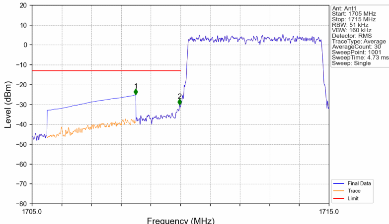
Band4_5MHz_16QAM_LCH_1712.5MHz_RB_25_0_NTNV
