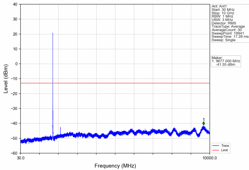
Band4_10MHz_QPSK_MCH_1732.5MHz_RB_1_0_NTNV
