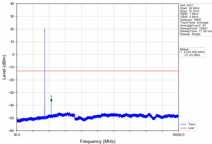
Band4_5MHz_64QAM_HCH_1752.5MHz_RB_1_0_NTNV
