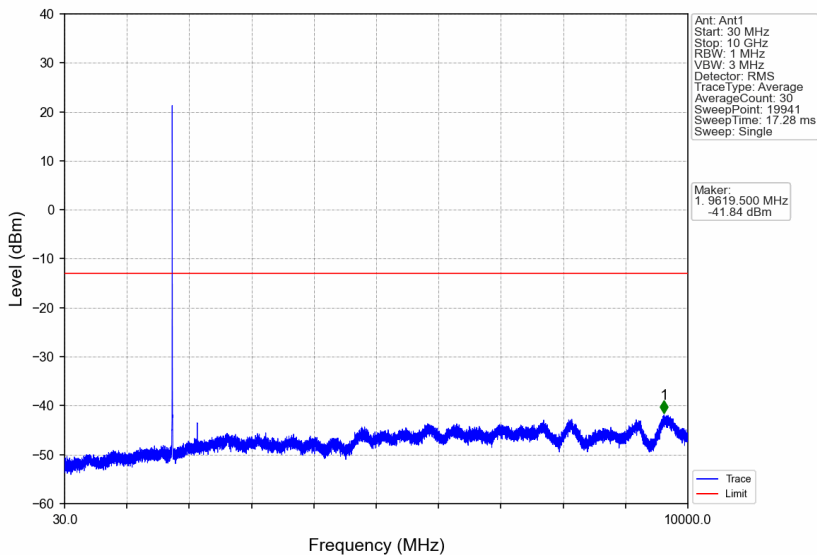
Band4_5MHz_16QAM_HCH_1752.5MHz_RB_1_0_NTNV
