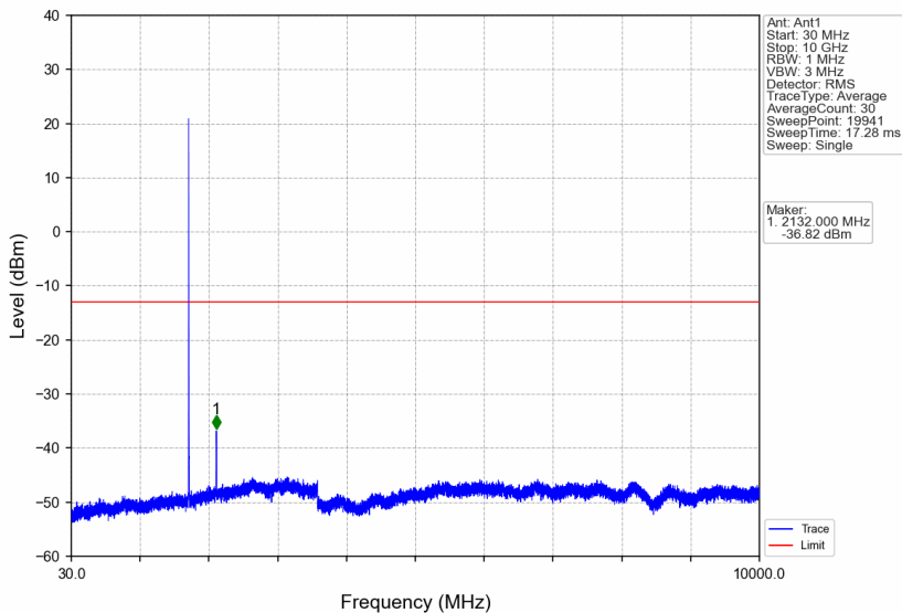
Band4_5MHz_64QAM_MCH_1732.5MHz_RB_1_0_NTNV
