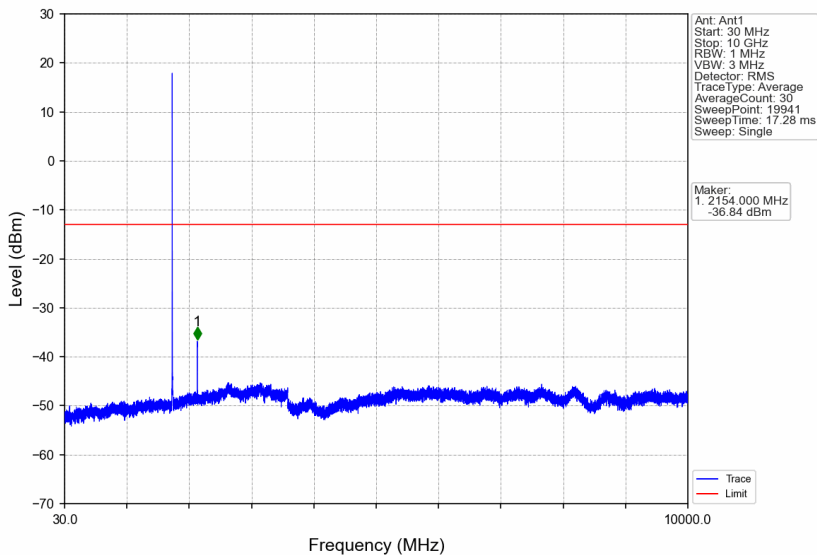
Band4_5MHz_256QAM_HCH_1752.5MHz_RB_1_0_NTNV
