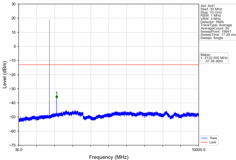
Band4_3MHz_256QAM_MCH_1732.5MHz_RB_1_0_NTNV
