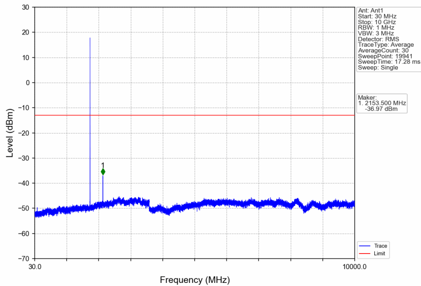
Band4_3MHz_256QAM_HCH_1753.5MHz_RB_1_0_NTNV
