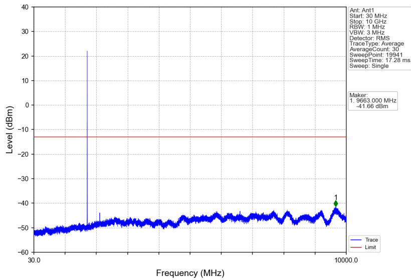
Band4_3MHz_16QAM_MCH_1732.5MHz_RB_1_0_NTNV
