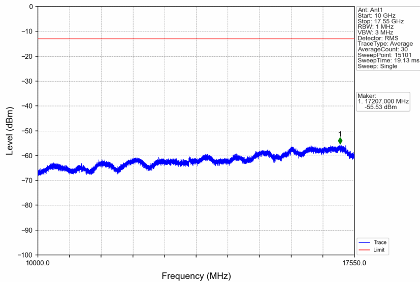
Band4_3MHz_16QAM_MCH_1732.5MHz_RB_1_0_NTNV
