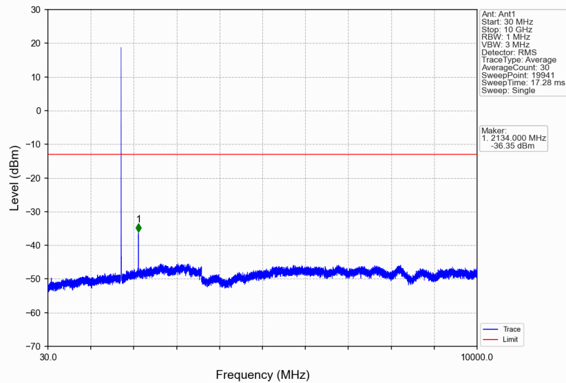
Band4_5MHz_256QAM_MCH_1732.5MHz_RB_1_0_NTNV
