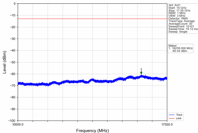
Band4_5MHz_256QAM_MCH_1732.5MHz_RB_1_0_NTNV
