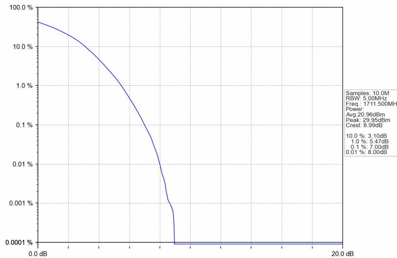
Band4_3MHz_256QAM_LCH_1711.5MHz_RB_15_0_NTNV
