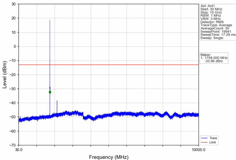
Band4_1.4MHz_256QAM_HCH_1754.3MHz_RB_1_0_NTNV
