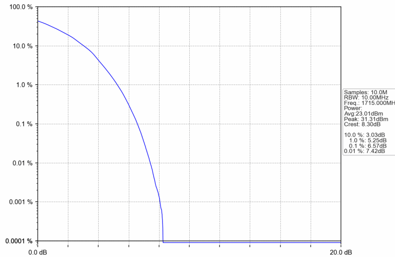
Band4_10MHz_64QAM_LCH_1715MHz_RB_50_0_NTNV
