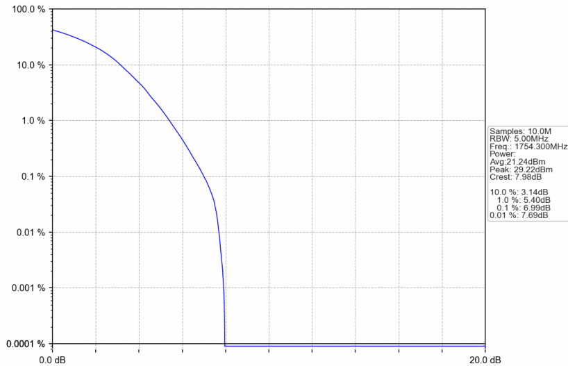
Band4_1.4MHz_256QAM_HCH_1754.3MHz_RB_6_0_NTNV
