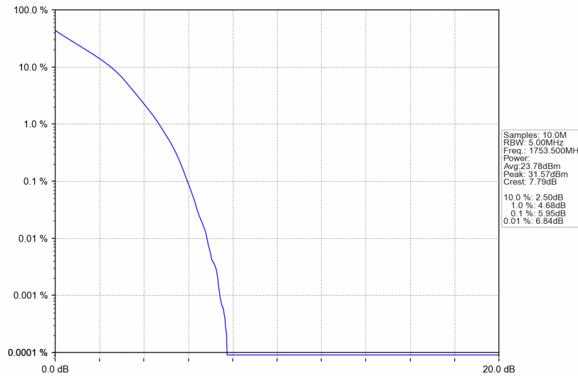
Band4_3MHz_QPSK_HCH_1753.5MHz_RB_15_0_NTNV
