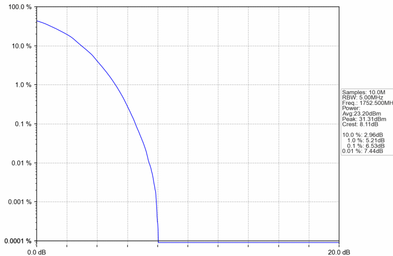
Band4_5MHz_64QAM_HCH_1752.5MHz_RB_25_0_NTNV
