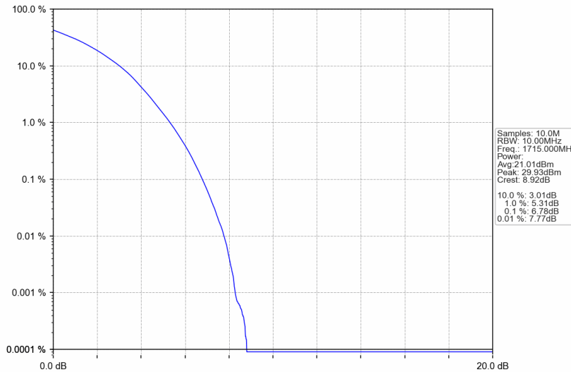
Band4_10MHz_256QAM_LCH_1715MHz_RB_50_0_NTNV
