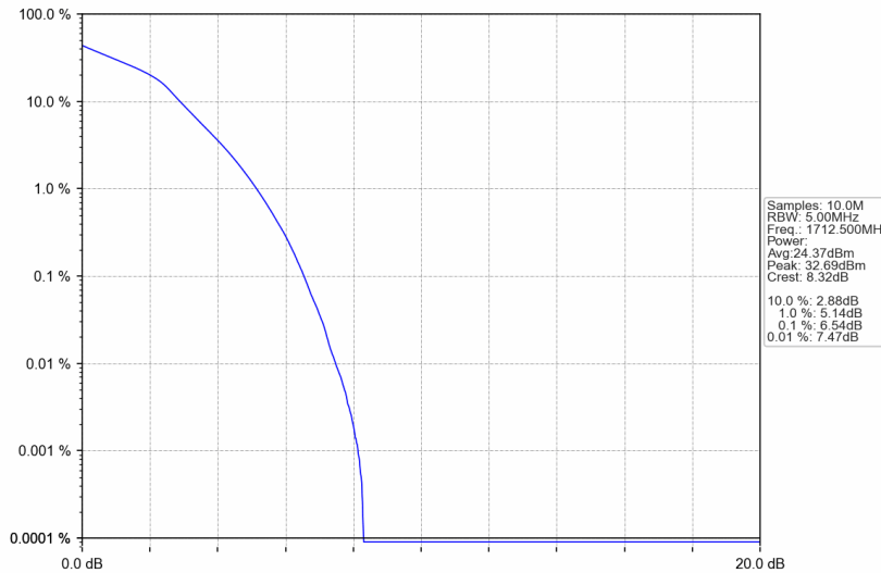
Band4_5MHz_16QAM_LCH_1712.5MHz_RB_25_0_NTNV
