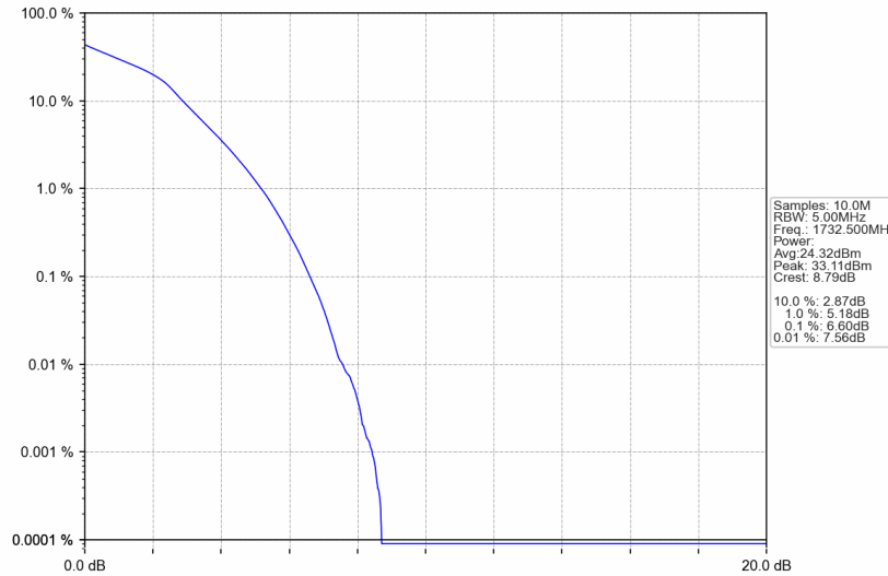
Band4_5MHz_16QAM_MCH_1732.5MHz_RB_25_0_NTNV
