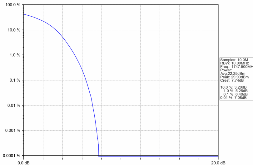
Band4_15MHz_16QAM_HCH_1747.5MHz_RB_75_0_NTNV
