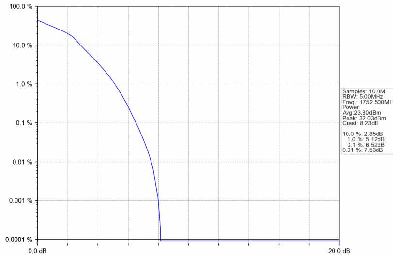
Band4_5MHz_16QAM_HCH_1752.5MHz_RB_25_0_NTNV
