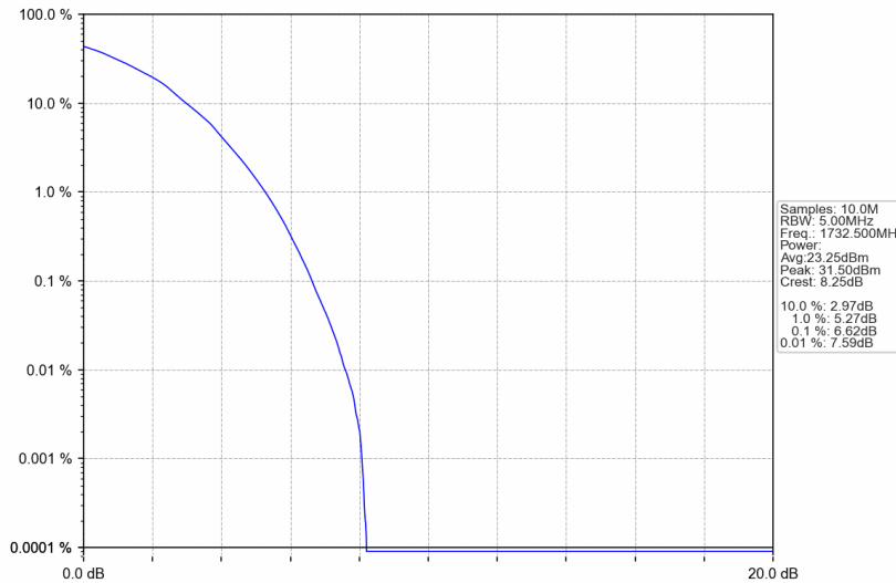
Band4_5MHz_64QAM_MCH_1732.5MHz_RB_25_0_NTNV
