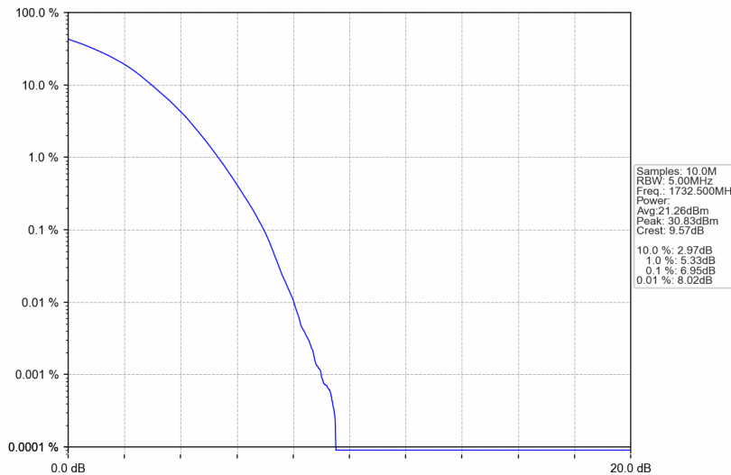
Band4_5MHz_256QAM_MCH_1732.5MHz_RB_25_0_NTNV
