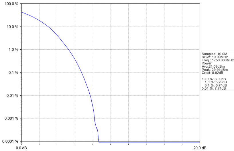
Band4_10MHz_256QAM_HCH_1750MHz_RB_50_0_NTNV
