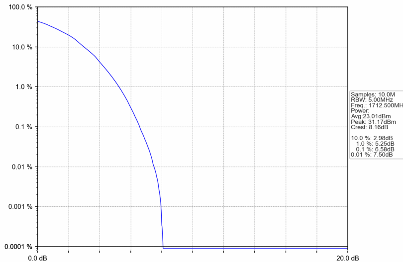
Band4_5MHz_64QAM_LCH_1712.5MHz_RB_25_0_NTNV
