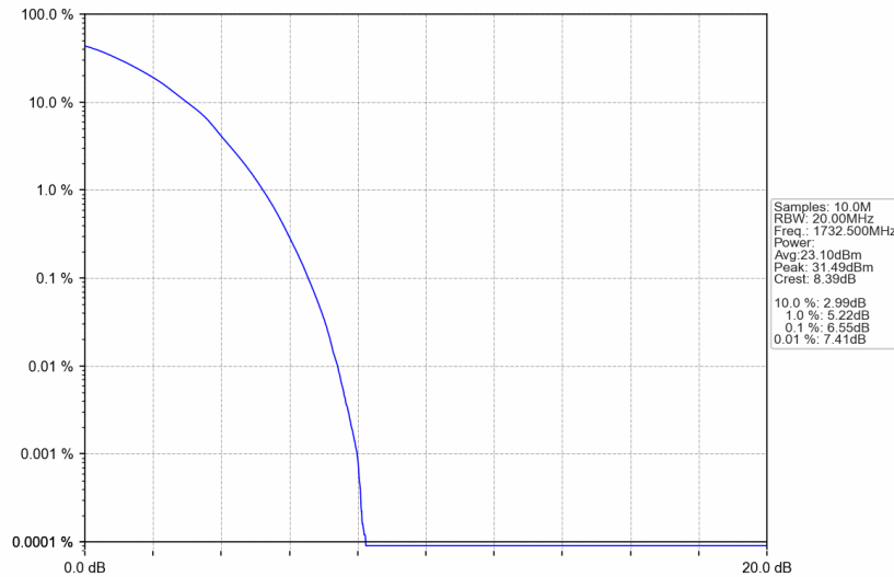
Band4_20MHz_64QAM_MCH_1732.5MHz_RB_100_0_NTNV
