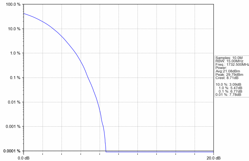
Band4_15MHz_256QAM_MCH_1732.5MHz_RB_75_0_NTNV
