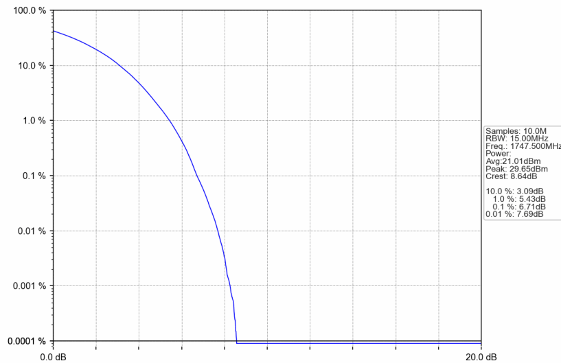
Band4_15MHz_256QAM_HCH_1747.5MHz_RB_75_0_NTNV
