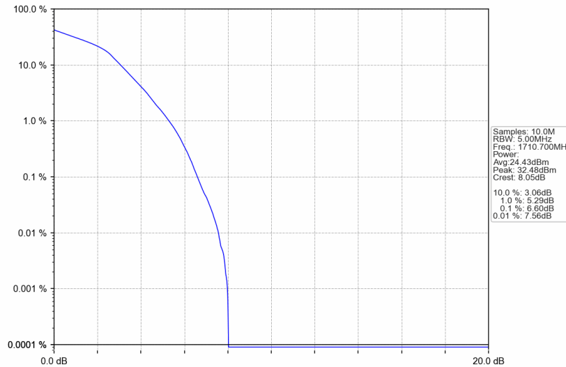
Band4_1.4MHz_16QAM_LCH_1710.7MHz_RB_6_0_NTNV
