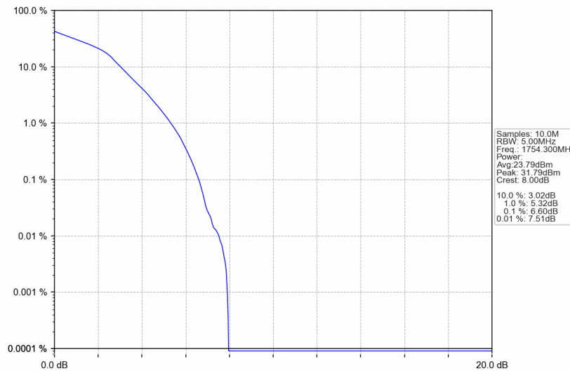
Band4_1.4MHz_16QAM_HCH_1754.3MHz_RB_6_0_NTNV
