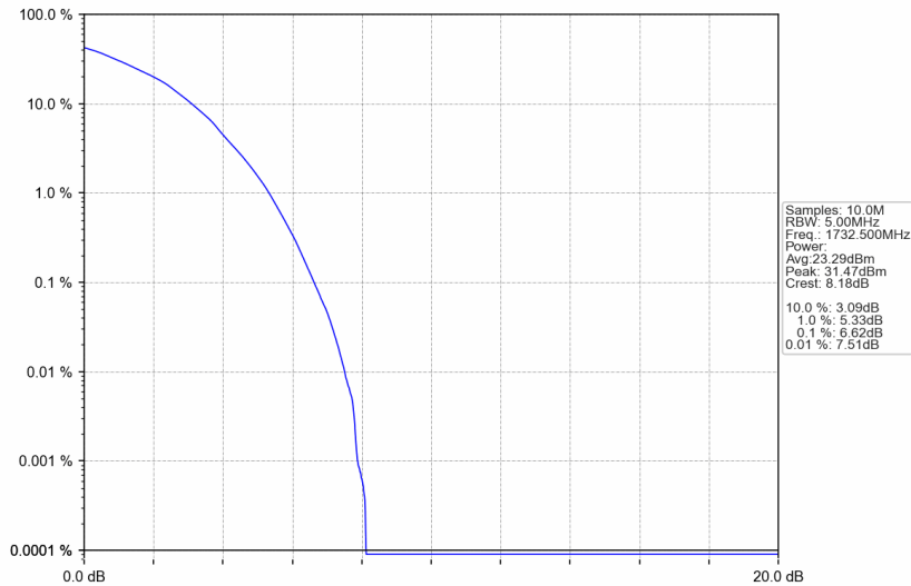
Band4_3MHz_64QAM_MCH_1732.5MHz_RB_15_0_NTNV
