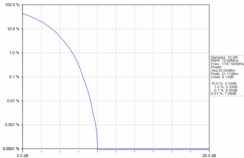
Band4_15MHz_64QAM_HCH_1747.5MHz_RB_75_0_NTNV
