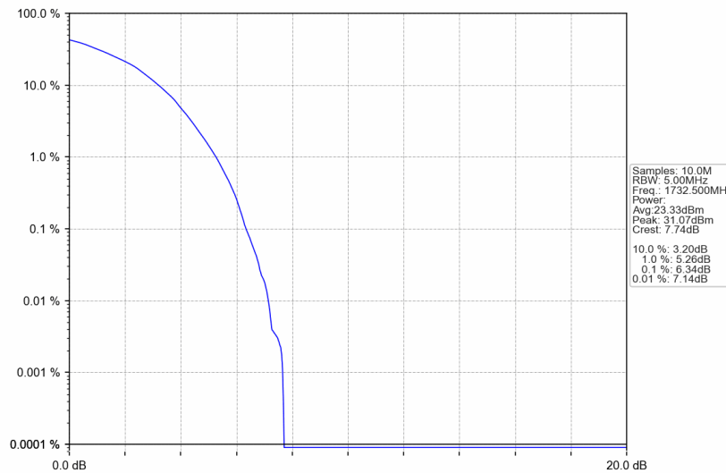
Band4_1.4MHz_64QAM_MCH_1732.5MHz_RB_6_0_NTNV
