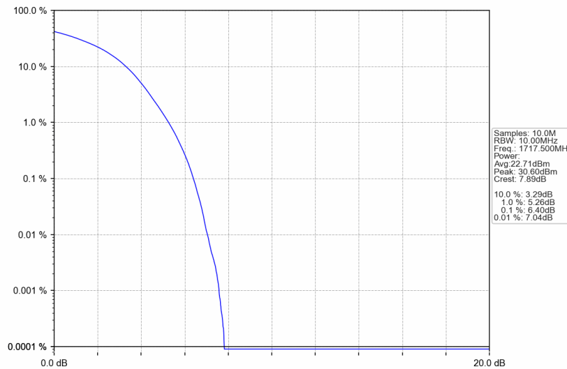
Band4_15MHz_16QAM_LCH_1717.5MHz_RB_75_0_NTNV
