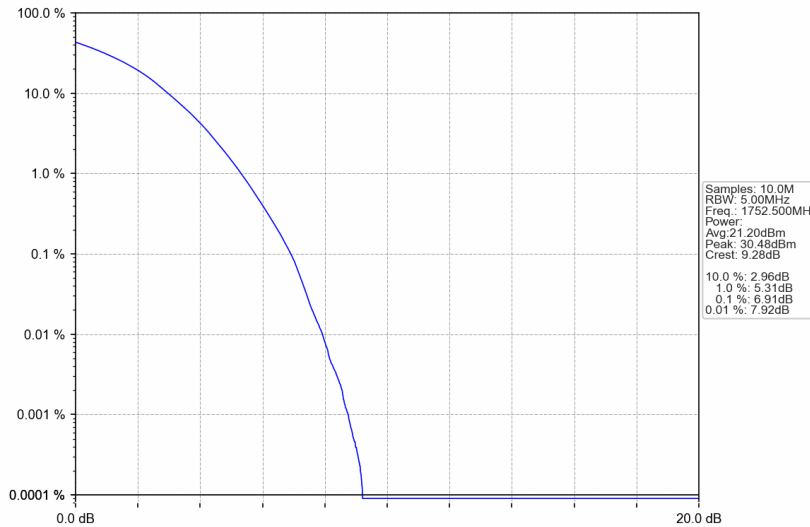
Band4_5MHz_256QAM_HCH_1752.5MHz_RB_25_0_NTNV
