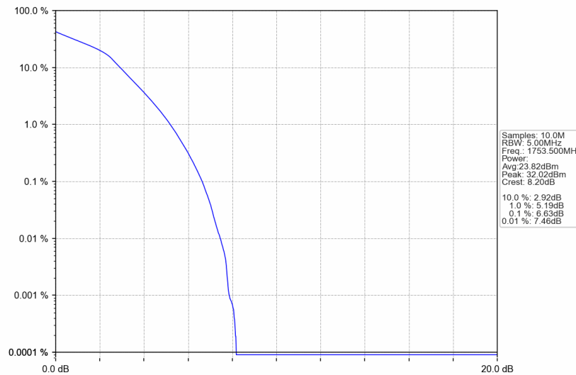
Band4_3MHz_16QAM_HCH_1753.5MHz_RB_15_0_NTNV
