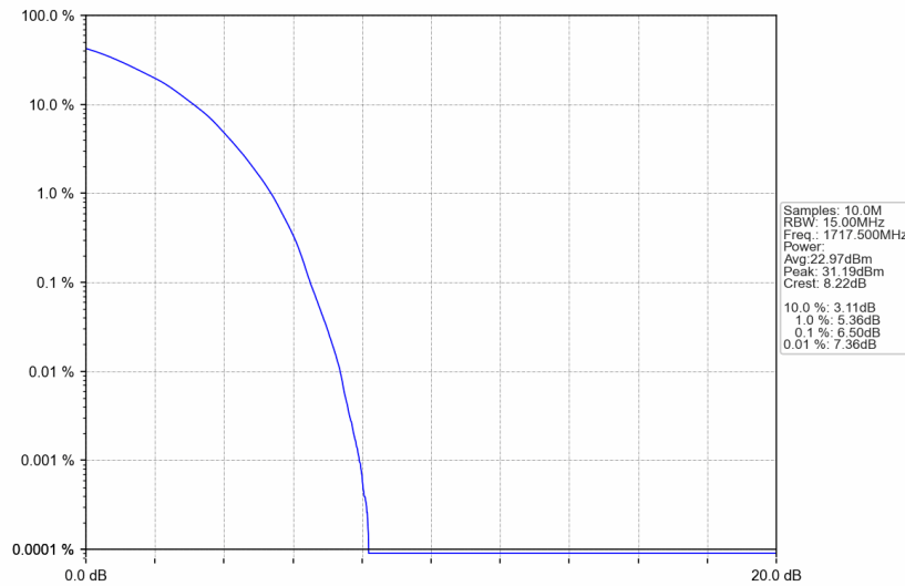
Band4_15MHz_64QAM_LCH_1717.5MHz_RB_75_0_NTNV
