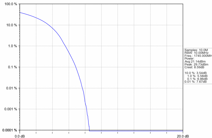
Band4_20MHz_16QAM_HCH_1745MHz_RB_100_0_NTNV
