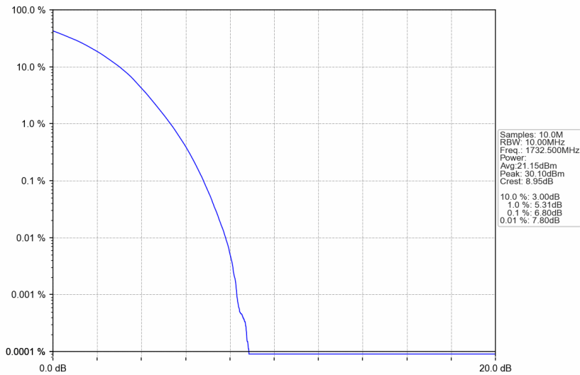
Band4_10MHz_256QAM_MCH_1732.5MHz_RB_50_0_NTNV
