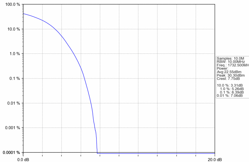
Band4_15MHz_16QAM_MCH_1732.5MHz_RB_75_0_NTNV
