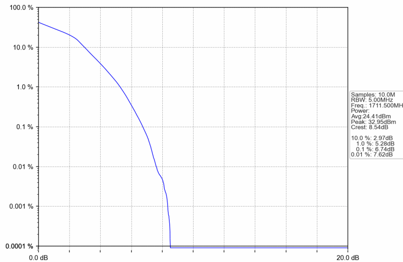
Band4_3MHz_16QAM_LCH_1711.5MHz_RB_15_0_NTNV
