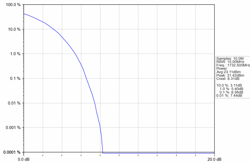
Band4_15MHz_64QAM_MCH_1732.5MHz_RB_75_0_NTNV
