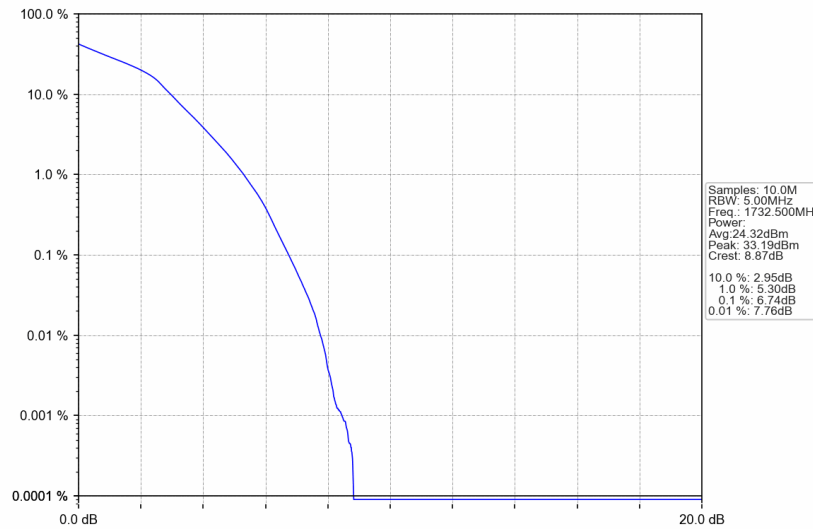
Band4_3MHz_16QAM_MCH_1732.5MHz_RB_15_0_NTNV
