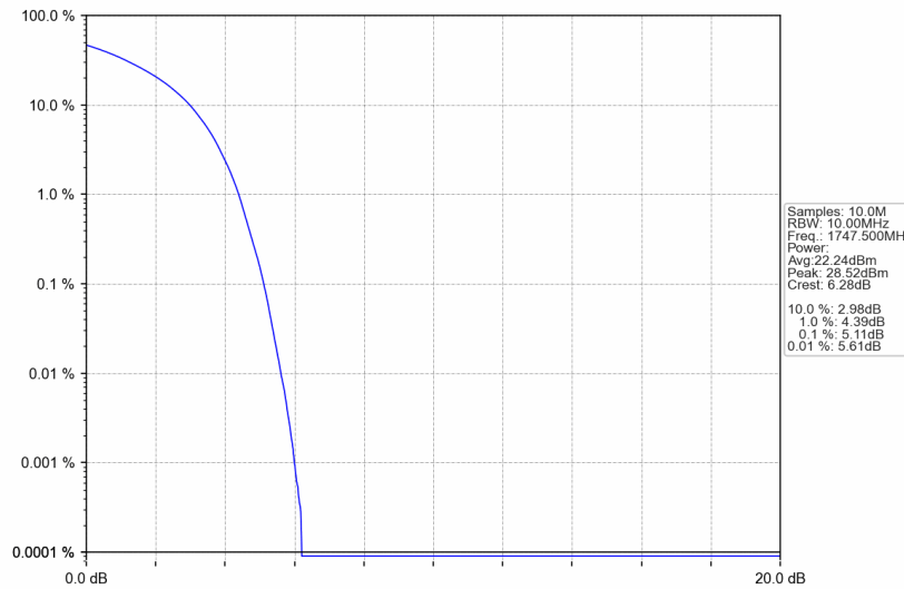
Band4_15MHz_QPSK_HCH_1747.5MHz_RB_75_0_NTNV
