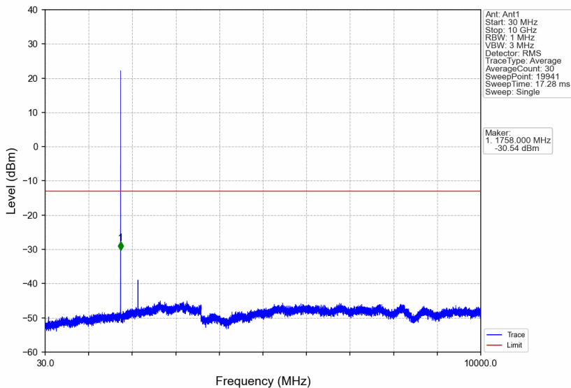
Band4_1.4MHz_64QAM_HCH_1754.3MHz_RB_1_0_NTNV
