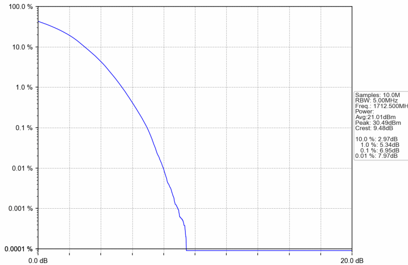
Band4_5MHz_256QAM_LCH_1712.5MHz_RB_25_0_NTNV
