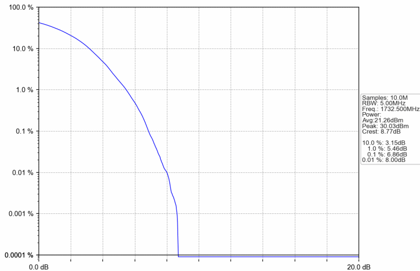
Band4_1.4MHz_256QAM_MCH_1732.5MHz_RB_6_0_NTNV
