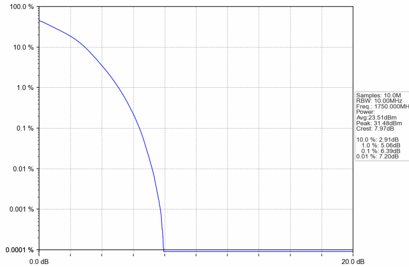
Band4_10MHz_16QAM_HCH_1750MHz_RB_50_0_NTNV
