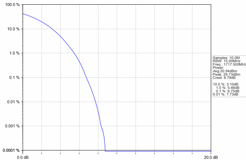
Band4_15MHz_256QAM_LCH_1717.5MHz_RB_75_0_NTNV
