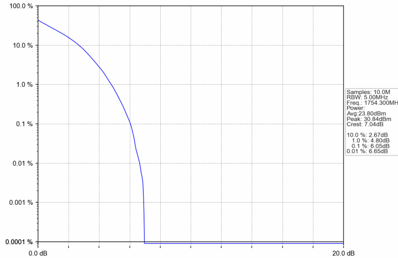
Band4_1.4MHz_QPSK_HCH_1754.3MHz_RB_6_0_NTNV
