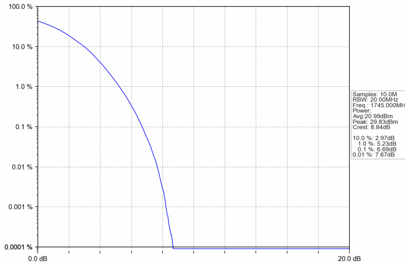
Band4_20MHz_256QAM_HCH_1745MHz_RB_100_0_NTNV
