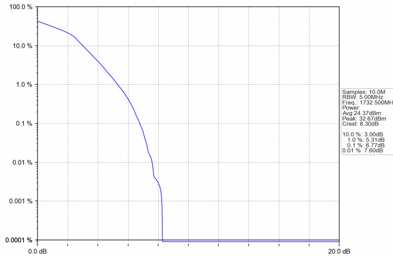
Band4_1.4MHz_16QAM_MCH_1732.5MHz_RB_6_0_NTNV
