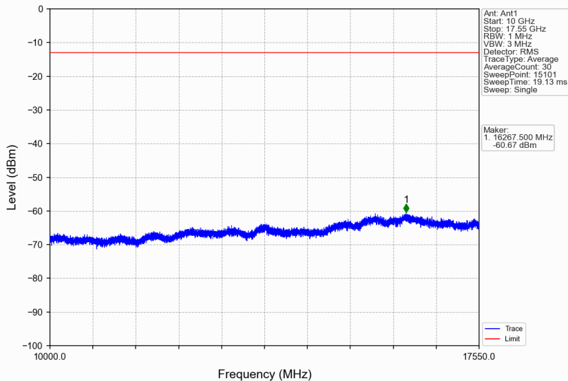
Band4_1.4MHz_256QAM_HCH_1754.3MHz_RB_1_0_NTNV
