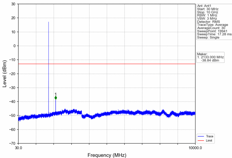
Band4_1.4MHz_256QAM_MCH_1732.5MHz_RB_1_0_NTNV
