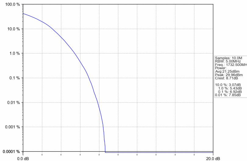
Band4_3MHz_256QAM_MCH_1732.5MHz_RB_15_0_NTNV
