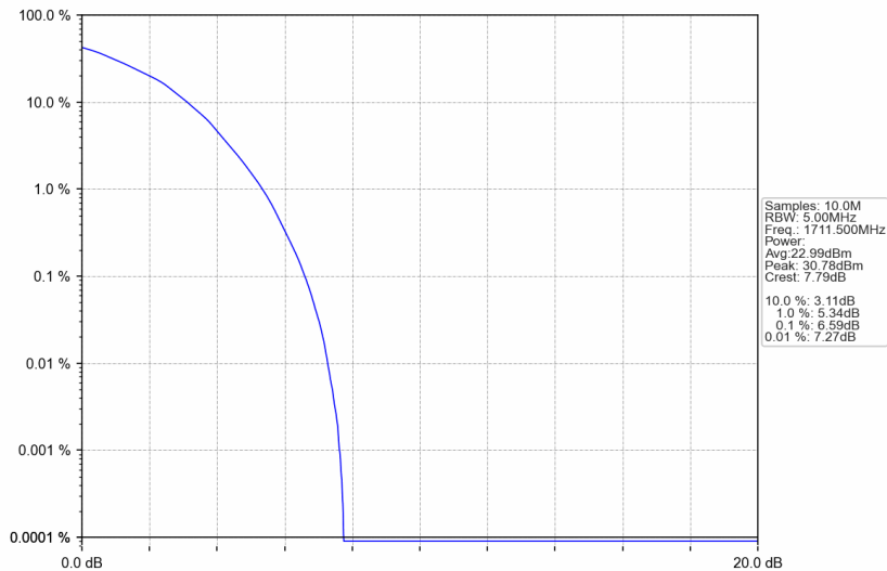
Band4_3MHz_64QAM_LCH_1711.5MHz_RB_15_0_NTNV
