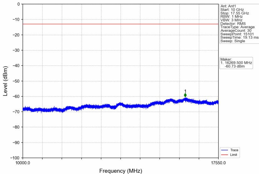
Band4_1.4MHz_256QAM_MCH_1732.5MHz_RB_1_0_NTNV
