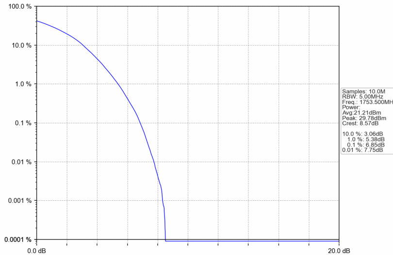
Band4_3MHz_256QAM_HCH_1753.5MHz_RB_15_0_NTNV
