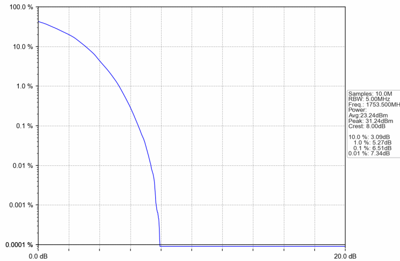
Band4_3MHz_64QAM_HCH_1753.5MHz_RB_15_0_NTNV
