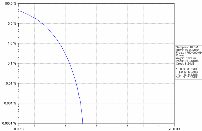
Band4_10MHz_64QAM_HCH_1750MHz_RB_50_0_NTNV
