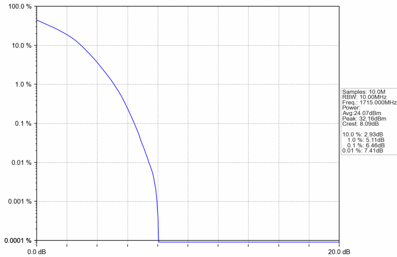
Band4_10MHz_16QAM_LCH_1715MHz_RB_50_0_NTNV
