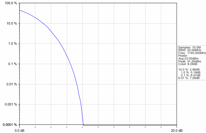
Band4_20MHz_64QAM_HCH_1745MHz_RB_100_0_NTNV
