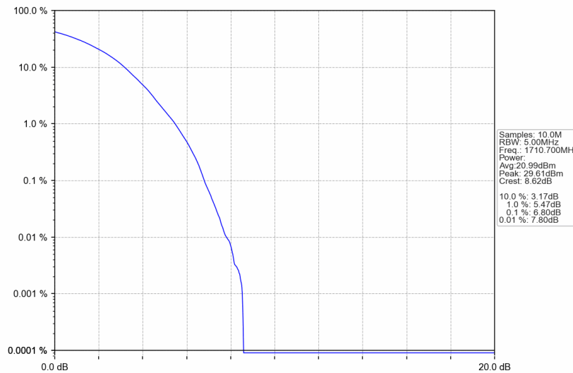
Band4_1.4MHz_256QAM_LCH_1710.7MHz_RB_6_0_NTNV
