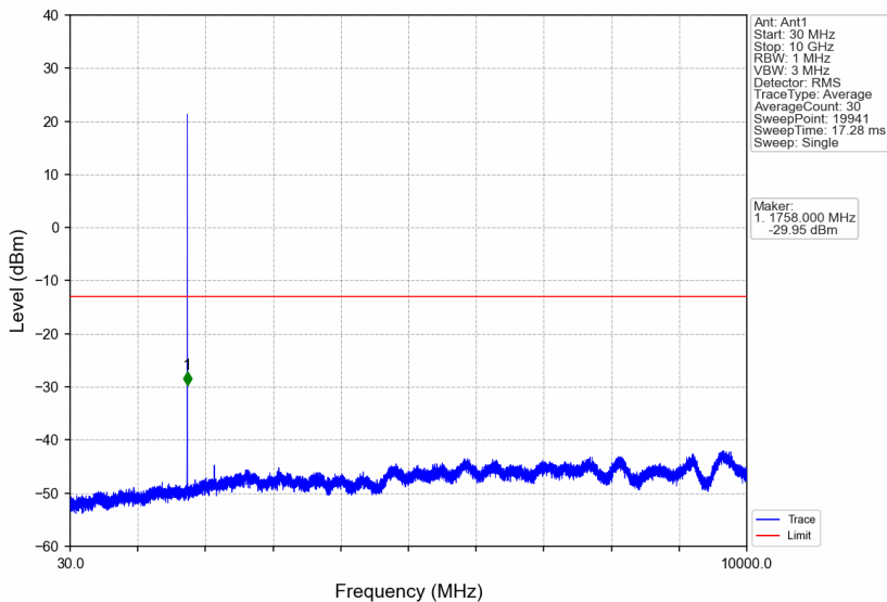
Band4_1.4MHz_16QAM_HCH_1754.3MHz_RB_1_0_NTNV
