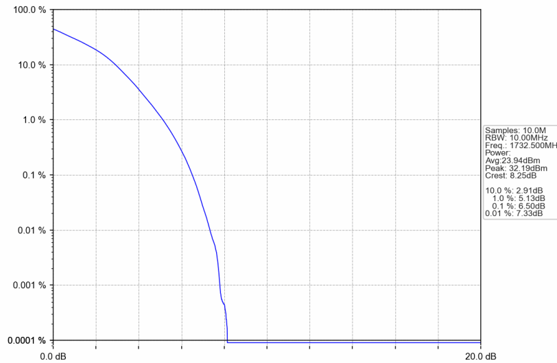
Band4_10MHz_16QAM_MCH_1732.5MHz_RB_50_0_NTNV
