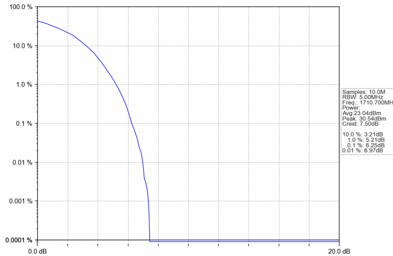
Band4_1.4MHz_64QAM_LCH_1710.7MHz_RB_6_0_NTNV
