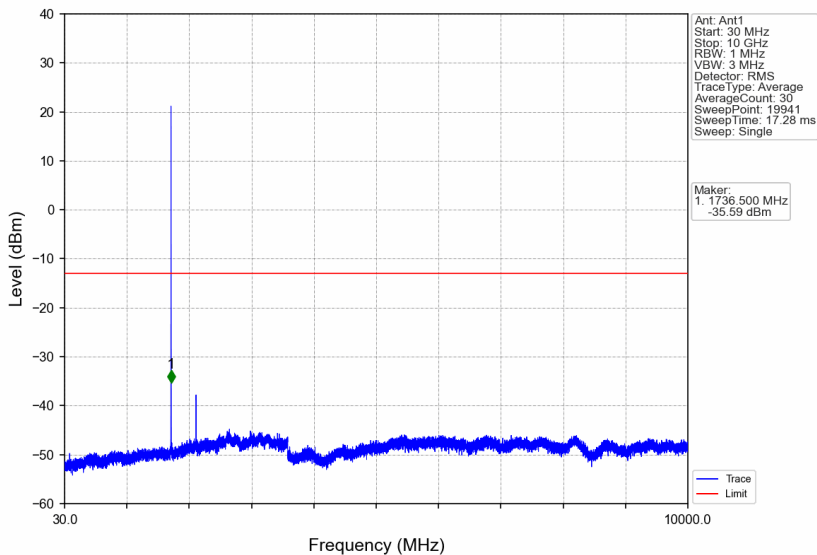
Band4_1.4MHz_64QAM_MCH_1732.5MHz_RB_1_0_NTNV
