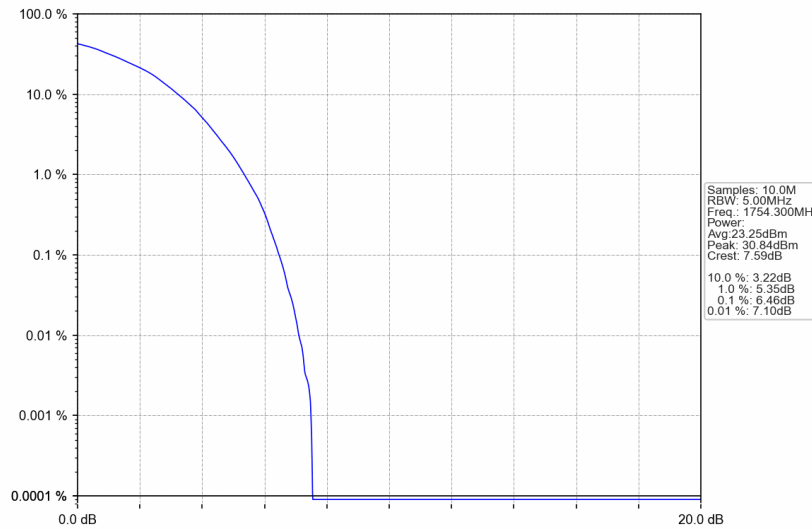
Band4_1.4MHz_64QAM_HCH_1754.3MHz_RB_6_0_NTNV
