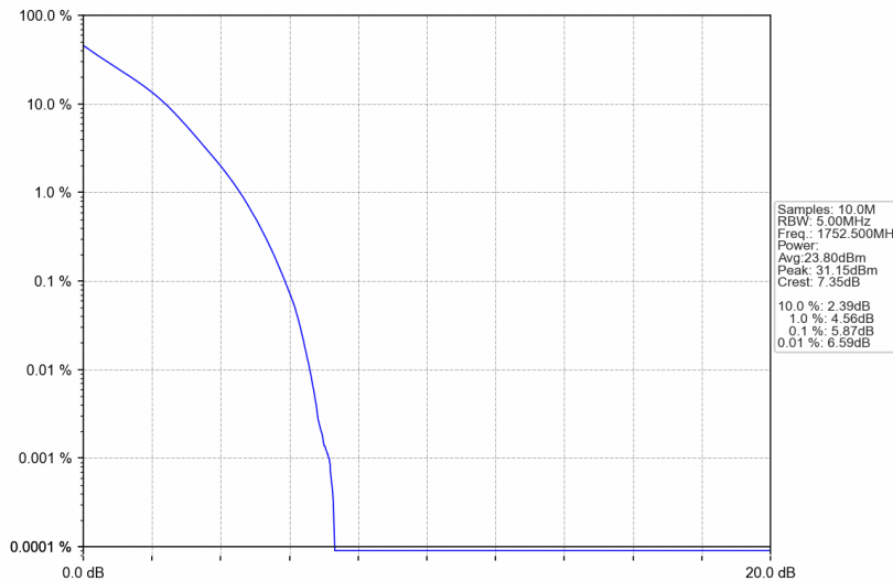
Band4_5MHz_QPSK_HCH_1752.5MHz_RB_25_0_NTNV
