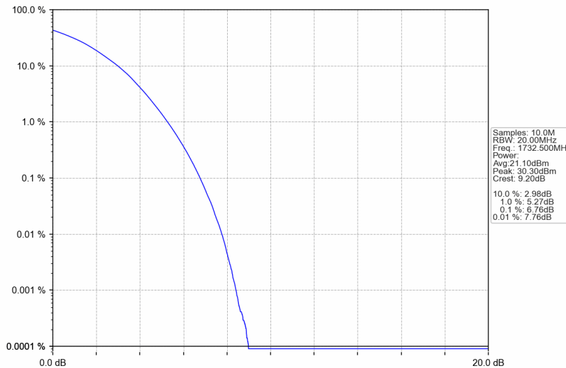
Band4_20MHz_256QAM_MCH_1732.5MHz_RB_100_0_NTNV
