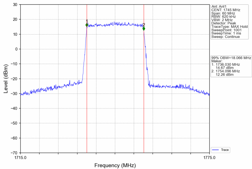
Band4_20MHz_16QAM_HCH_1745MHz_RB_100_0_NTNV
