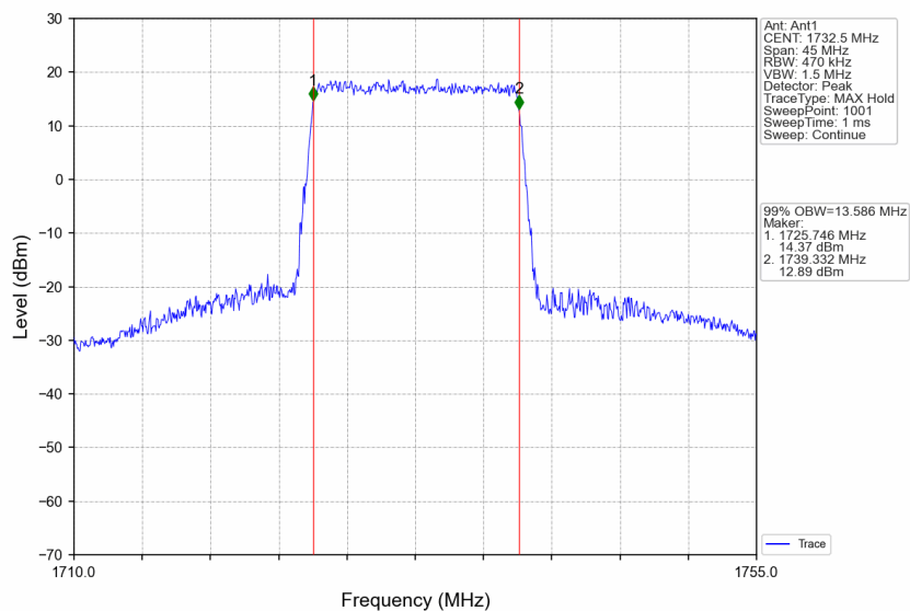
Band4_15MHz_64QAM_MCH_1732.5MHz_RB_75_0_NTNV
