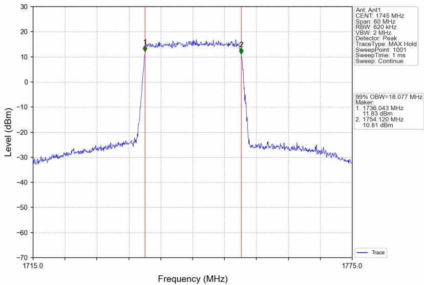
Band4_20MHz_256QAM_HCH_1745MHz_RB_100_0_NTNV
