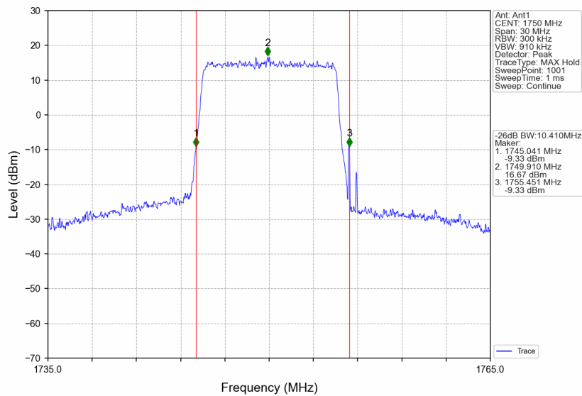
Band4_10MHz_256QAM_HCH_1750MHz_RB_50_0_NTNV
