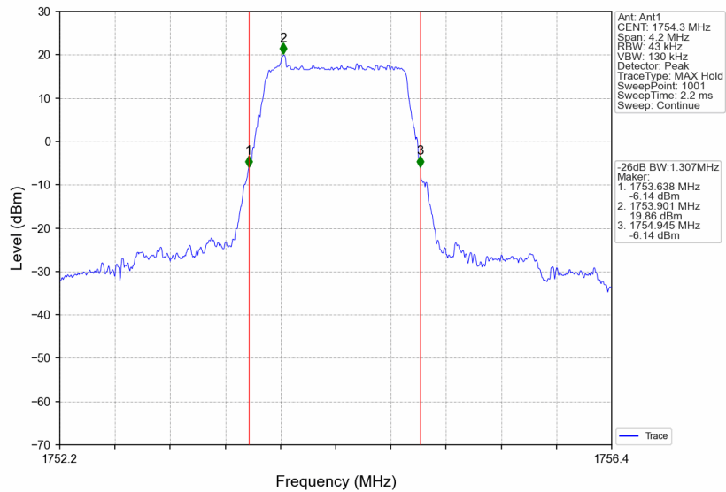
Band4_1.4MHz_16QAM_HCH_1754.3MHz_RB_6_0_NTNV
