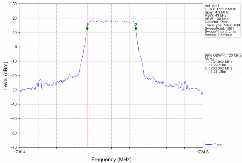
Band4_1.4MHz_64QAM_MCH_1732.5MHz_RB_6_0_NTNV
