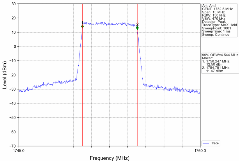
Band4_5MHz_16QAM_HCH_1752.5MHz_RB_25_0_NTNV
