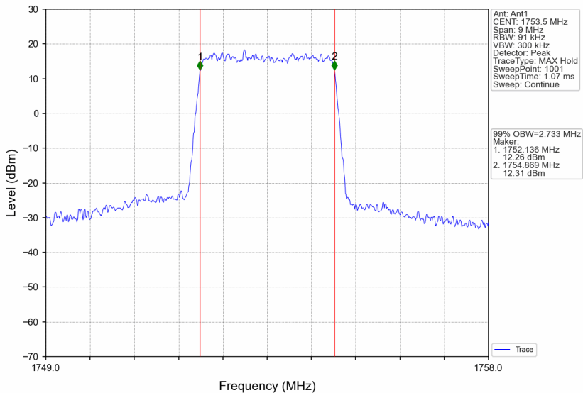
Band4_3MHz_16QAM_HCH_1753.5MHz_RB_15_0_NTNV
