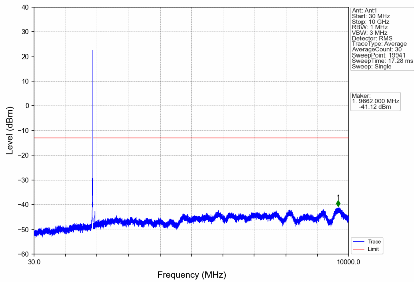
Band2_15MHz_16QAM_MCH_1880MHz_RB_1_0_NTNV
