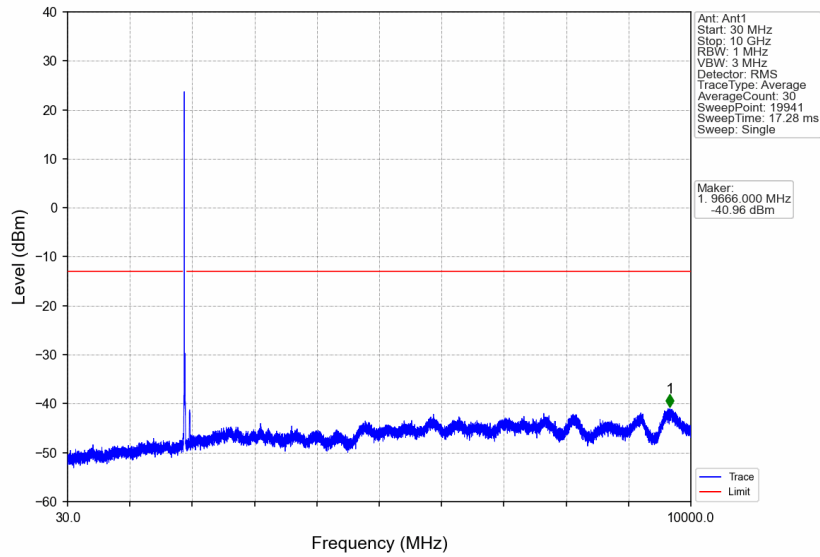
Band2_15MHz_16QAM_HCH_1902.5MHz_RB_1_0_NTNV
