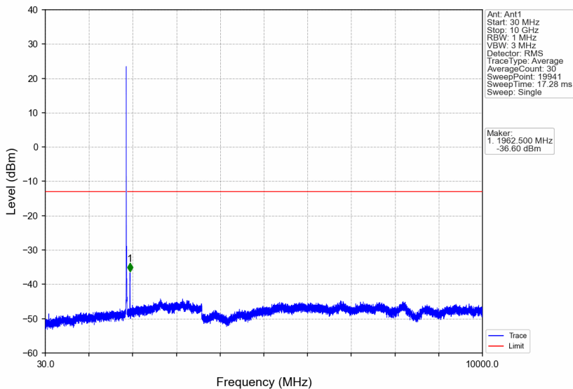
Band2_10MHz_64QAM_MCH_1880MHz_RB_1_0_NTNV
