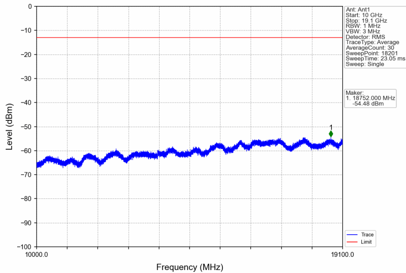
Band2_15MHz_16QAM_HCH_1902.5MHz_RB_1_0_NTNV
