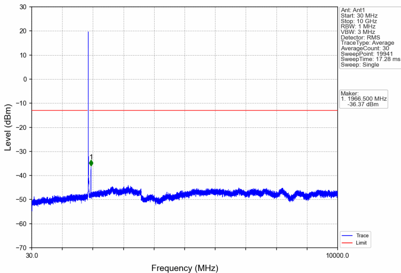
Band2_15MHz_256QAM_MCH_1880MHz_RB_1_0_NTNV
