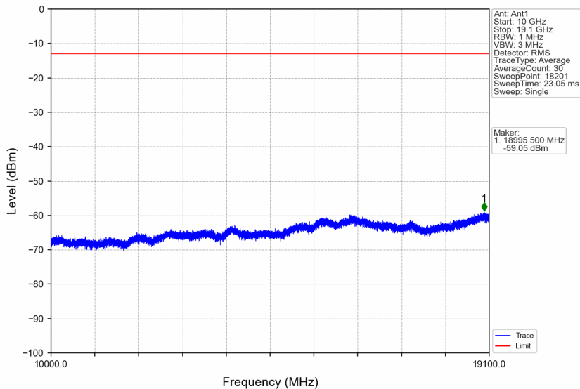
Band2_15MHz_256QAM_MCH_1880MHz_RB_1_0_NTNV
