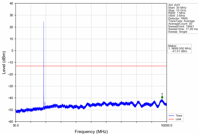
Band2_5MHz_16QAM_MCH_1880MHz_RB_1_0_NTNV
