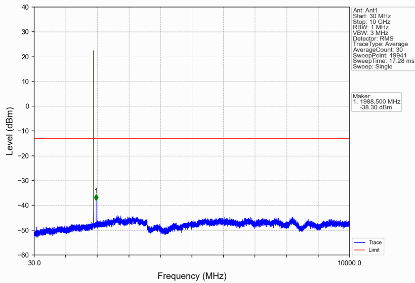
Band2_3MHz_64QAM_HCH_1908.5MHz_RB_1_0_NTNV
