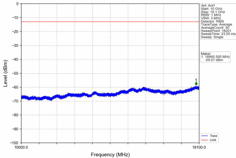
Band2_5MHz_256QAM_HCH_1907.5MHz_RB_1_0_NTNV
