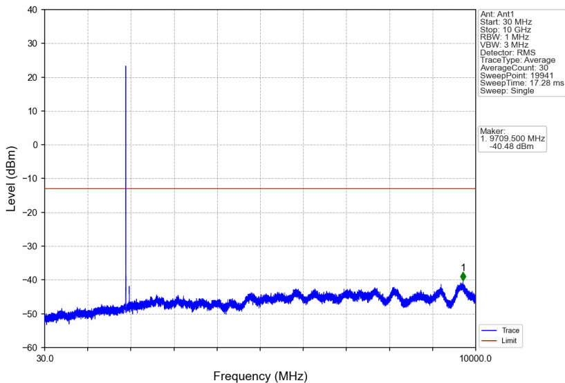
Band2_5MHz_16QAM_HCH_1907.5MHz_RB_1_0_NTNV
