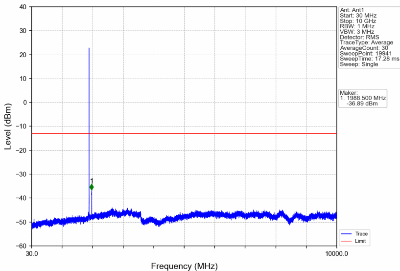
Band2_5MHz_64QAM_HCH_1907.5MHz_RB_1_0_NTNV
