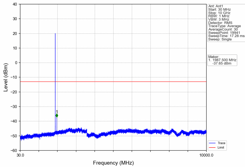
Band2_5MHz_256QAM_HCH_1907.5MHz_RB_1_0_NTNV
