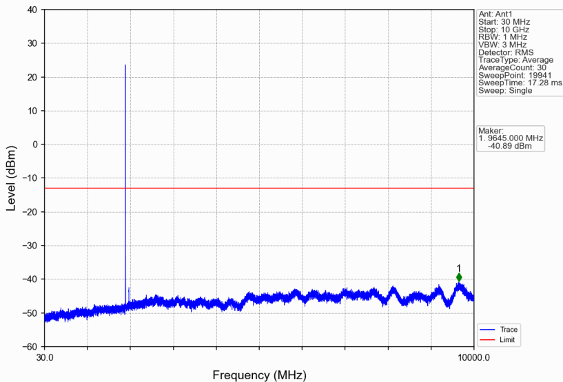
Band2_3MHz_16QAM_HCH_1908.5MHz_RB_1_0_NTNV
