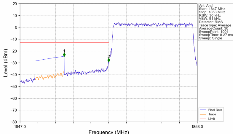
Band2_3MHz_64QAM_LCH_1851.5MHz_RB_15_0_NTNV
