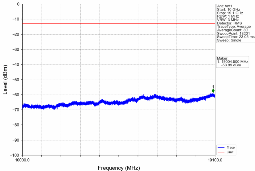
Band2_5MHz_64QAM_HCH_1907.5MHz_RB_1_0_NTNV
