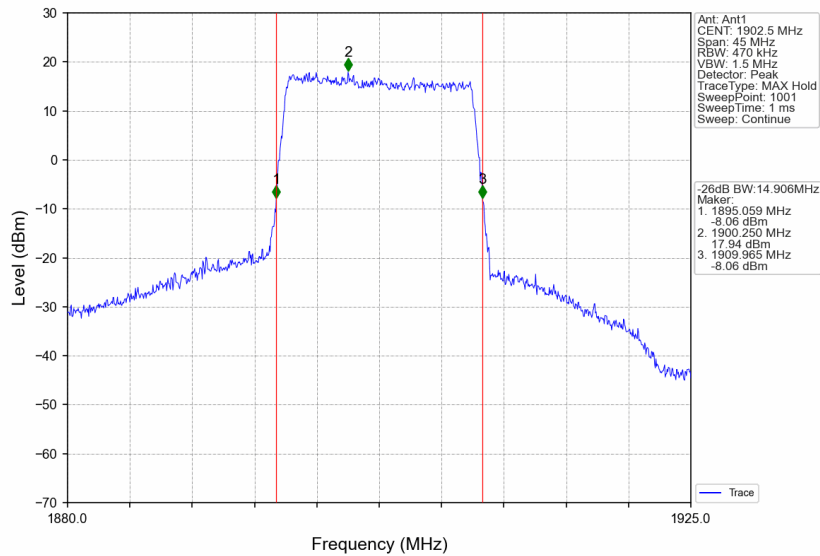
Band2_15MHz_256QAM_HCH_1902.5MHz_RB_75_0_NTNV
