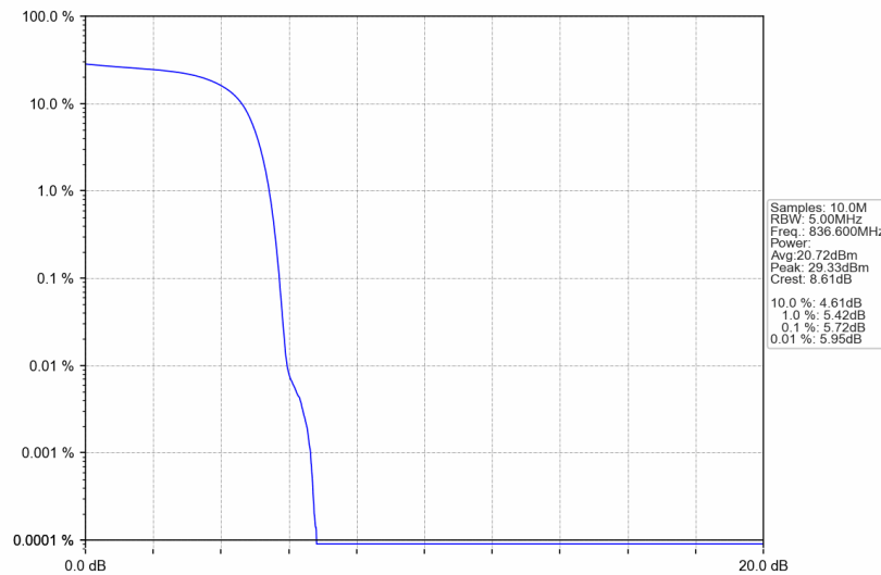
Band V_HSUPA_MCH_836.6MHz_Subtest 1_NTNV
