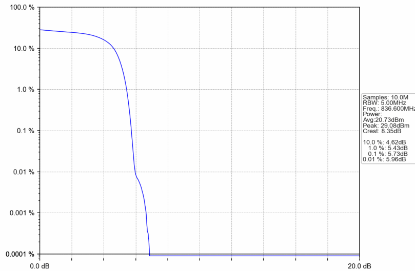
Band V_HSDPA_MCH_836.6MHz_Subtest 1_NTNV
