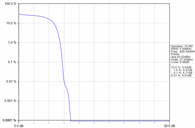
Band V_HSDPA_LCH_826.4MHz_Subtest 1_NTNV
