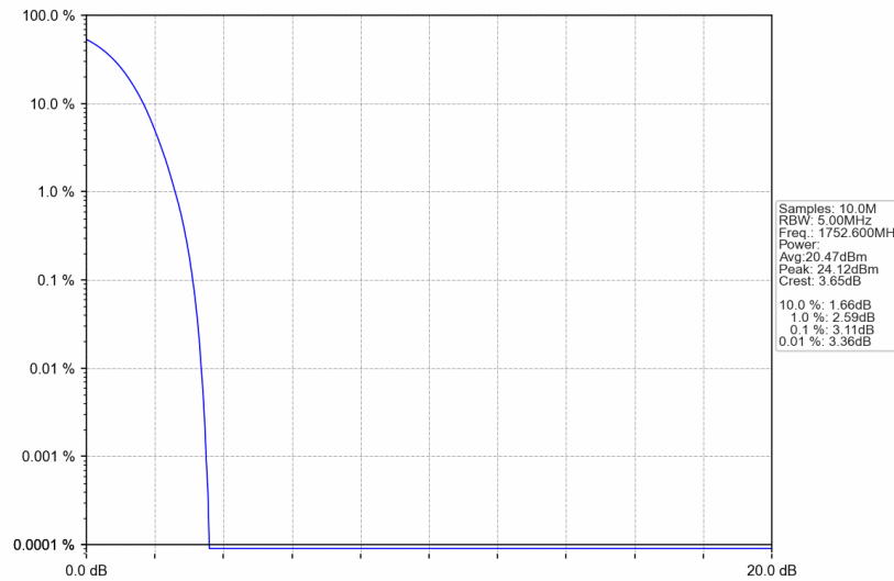
Band IV_RMC_HCH_1752.6MHz_12.2kbps RMC_NTNV
