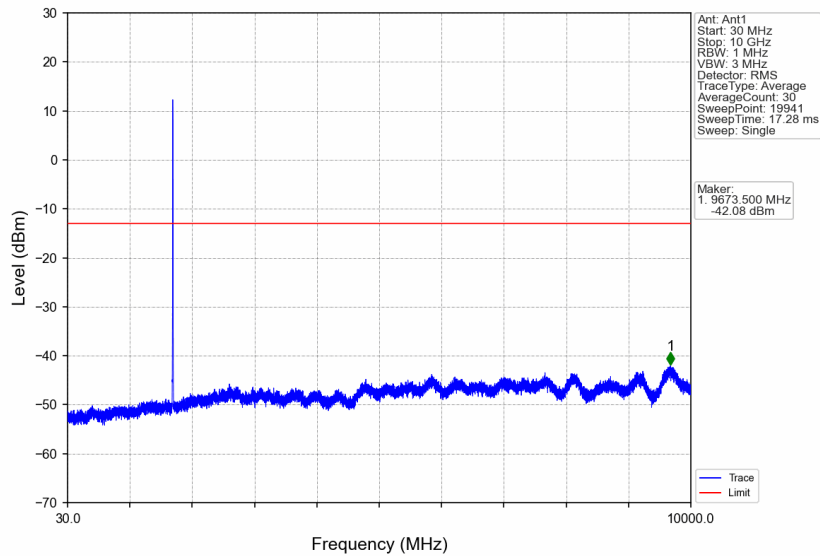
Band IV_HSUPA_LCH_1712.4MHz_Subtest 1_NTNV
