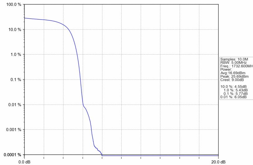
Band IV_HSDPA_MCH_1732.6MHz_Subtest 1_NTNV
