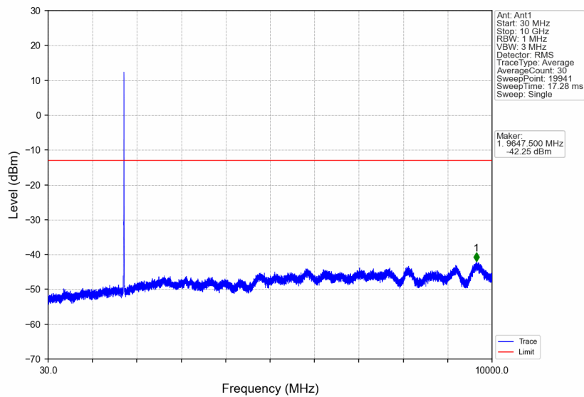
Band IV_HSDPA_MCH_1732.6MHz_Subtest 1_NTNV
