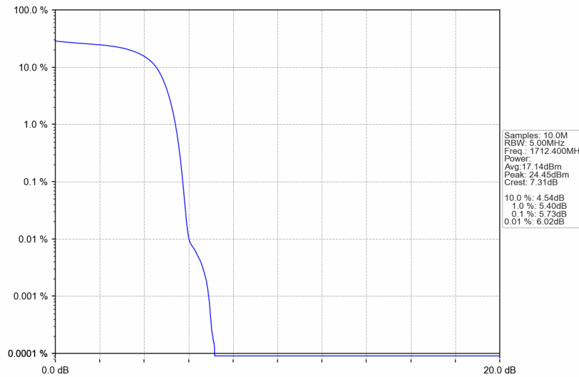
Band IV_HSUPA_LCH_1712.4MHz_Subtest 1_NTNV
