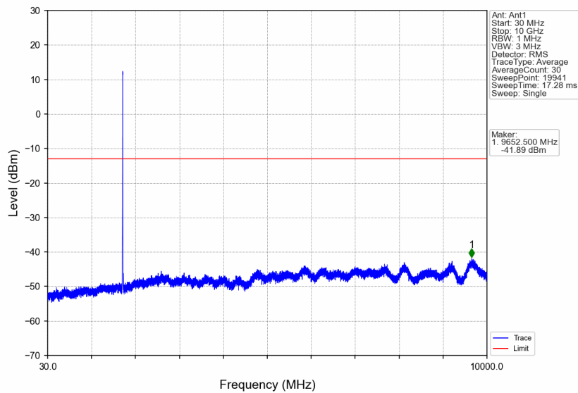
Band IV_HSUPA_MCH_1732.6MHz_Subtest 1_NTNV
