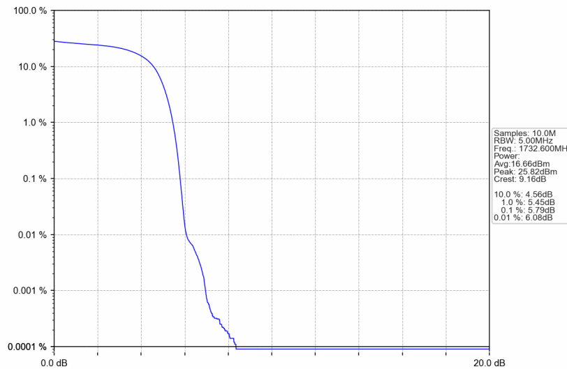
Band IV_HSUPA_MCH_1732.6MHz_Subtest 1_NTNV
