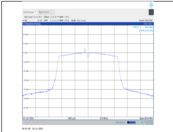
11ac40SISO-Ant6-5670-PASS
