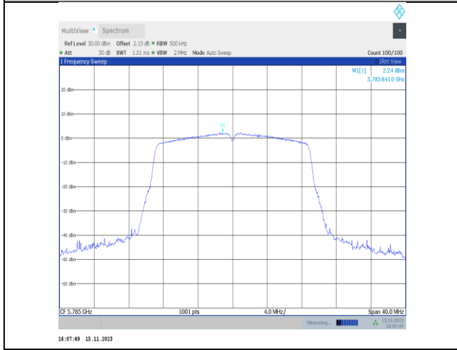
11ac20SISO-Ant6-5785-PASS
