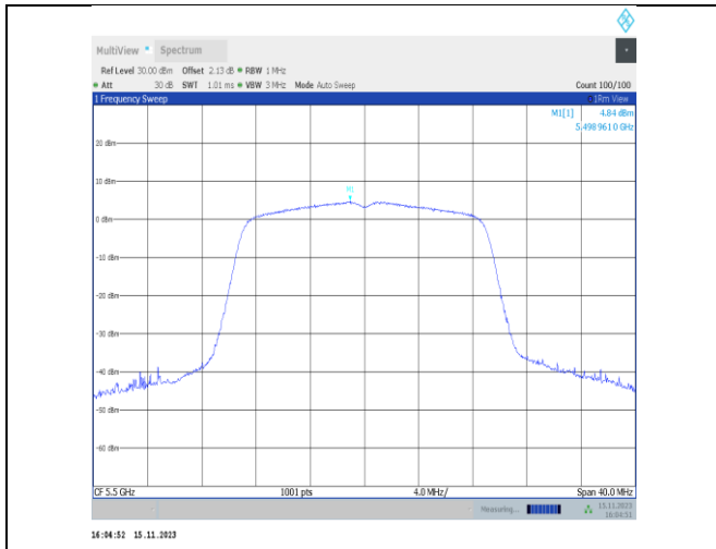
11ac20SISO-Ant6-5500-PASS
