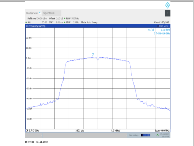
11ac20SISO-Ant6-5745-PASS
