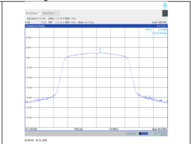
11ac20SISO-Ant6-5580-PASS
