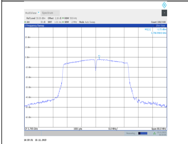
11ac40SISO-Ant6-5795-PASS
