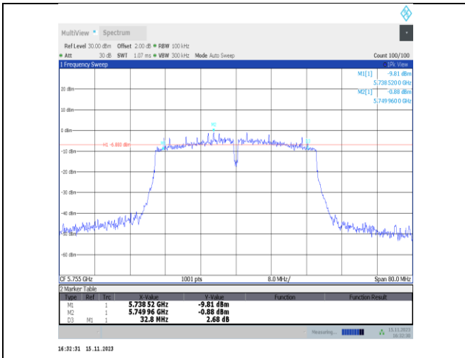
11ac40SISO-Ant6-5755-PASS
