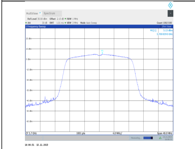
11ac20SISO-Ant6-5700-PASS
