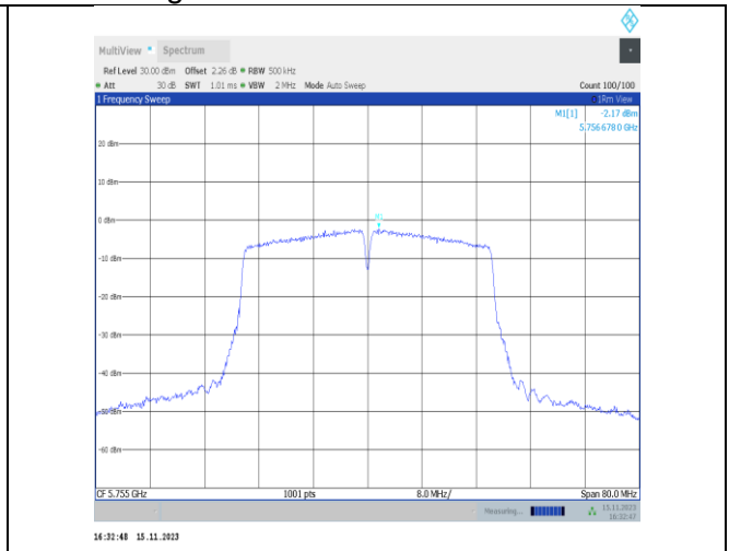
11ac40SISO-Ant6-5755-PASS
