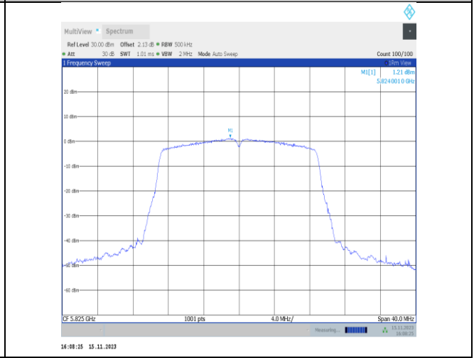
11ac20SISO-Ant6-5825-PASS
