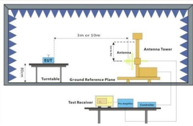
Figure 2. Above 30MHz
